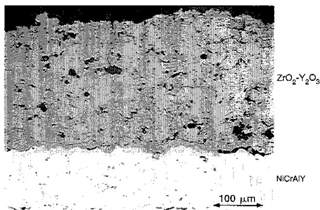
FIGURE 4-4 Photomicrograph of a plasma-sprayed TBC.
