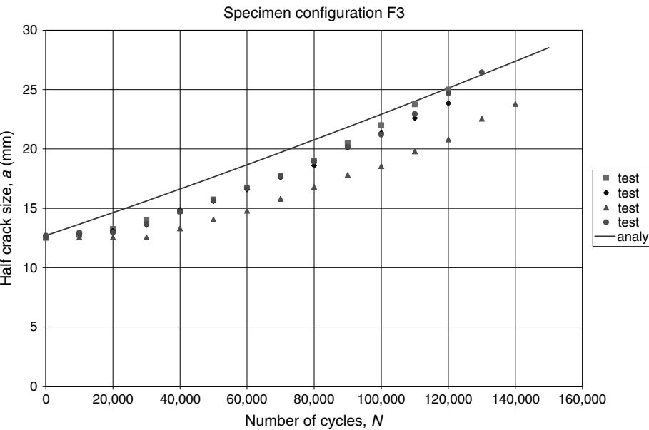
Fig. 11.11. Crack growth predictions and test results for specimen configuration F3.
