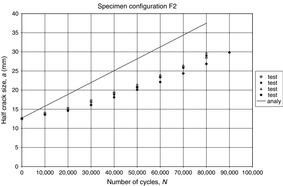
Fig. 11.10. Crack growth predictions and test results for specimen configuration F2.
