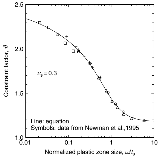
Fig. 8.2. Constraint factor versus normalized plastic zone size.
