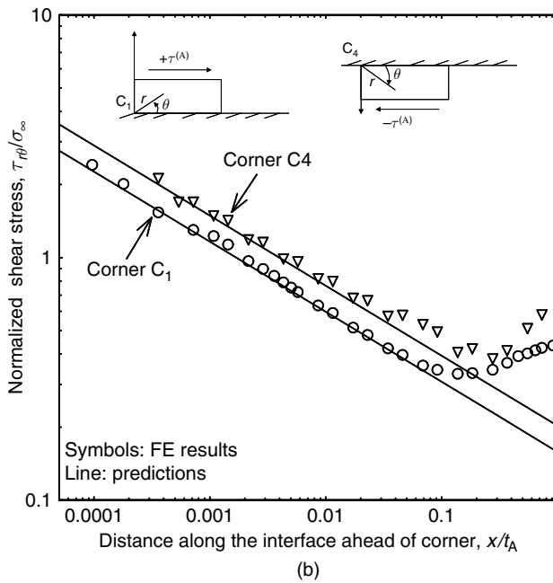
Fig. 2.14. Distribution of (a) normal stress and (b) shear stress along the interface ahead of the corners C_1 and C_4 in a double-lap joint.
