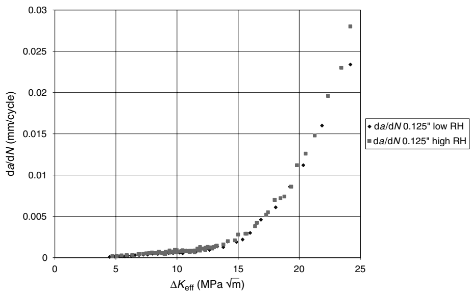
Fig. 11.4. da/dN versus \Delta K_{\text{eff}} for Al 7075-T6 3.175 mm thick sheet.
