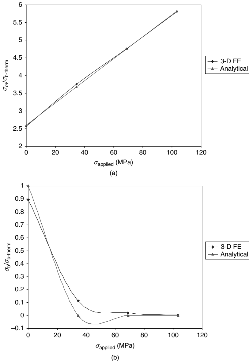
Fig. 5.18. Normalized stresses in the skin of a repair with a 40.64 \times 40.64 cm square patch under thermo-mechanical loading: (a) normalized mean stress; and (b) normalized bending stresses.
