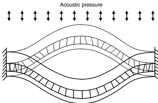
Fig. 12.4. Deflection under acoustic pressure showing the shear deformation of the damping layer.
