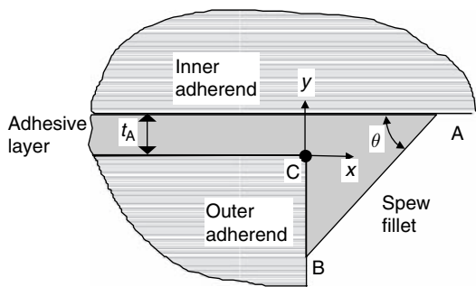
Fig. 2.15. Configuration of a spew fillet.
