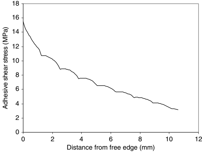
Fig. 7.19. Distribution of adhesive shear stress in a balanced two-sided doubler with a taper ratio of 10:1, t_s = 2.54 mm, and a full thickness of each doubler equal to 1.27 mm.
