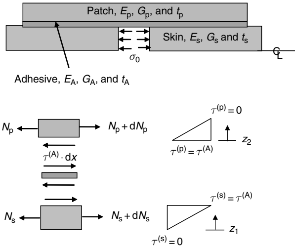
Fig. 13.5. Geometry of a semi-infinite double-strap joint used to derive the spring constant of the crack-bridging model, accounting for adherend shear deformations.
