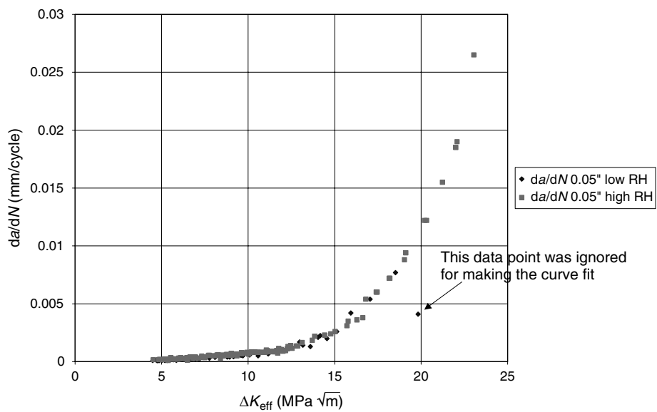
Fig. 11.5. da/dN versus \Delta K_{\text{eff}} for Al 7075-T6 1.27 mm thick sheet.
