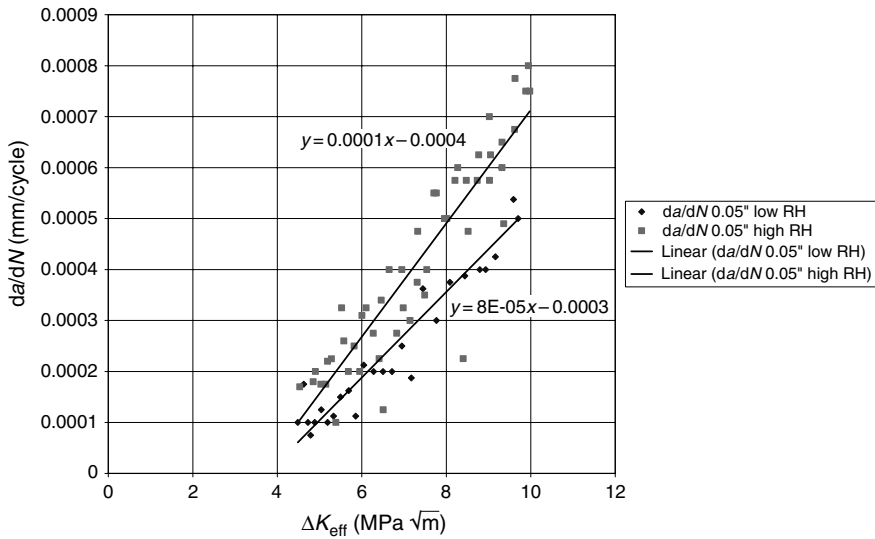
Fig. 11.7. A linear fit of da/dN versus \Delta K_{\text{eff}} for Al 7075-T6 1.27 mm thick plate at low \Delta K_{\text{eff}} range.
