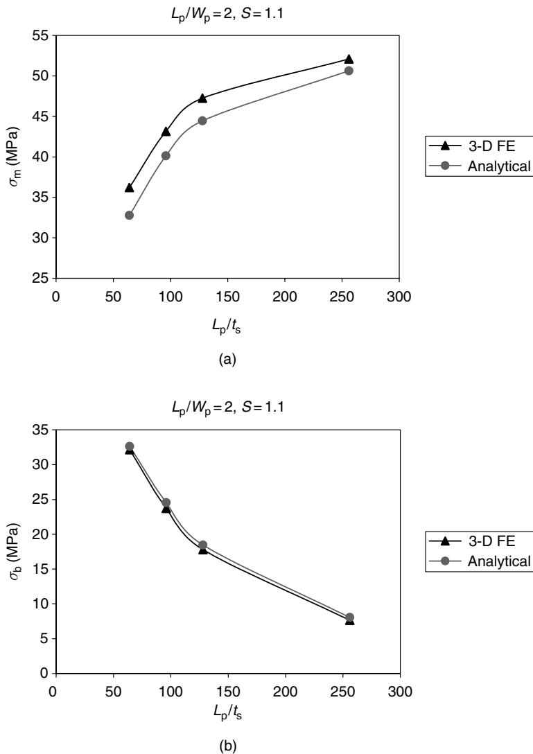
Fig. 5.11. Thermal stresses in the middle of a skin reinforced with a rectangular patch ( L_p/W_p = 2 ) for different normalized half patch lengths: (a) the mean stresses; and (b) the bending stresses.
