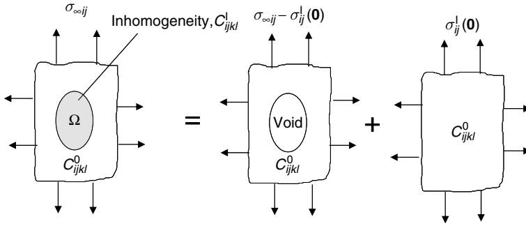
Fig. 6.2. Tanaka–Mura method for calculating the elastic field at a point outside \Omega . \sigma_{ij}^I(\mathbf{0}) is the stress in the inhomogeneity at its center inside \Omega .
