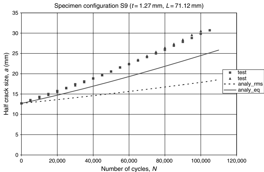
Fig. 11.23. Analytical predictions versus test results of crack growth in specimen configuration S9.
