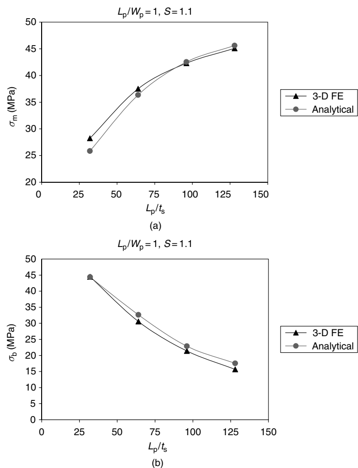
Fig. 5.10. Thermal stresses in the middle of a skin reinforced with a square patch for different normalized half patch lengths: (a) the mean stresses; and (b) the bending stresses.
