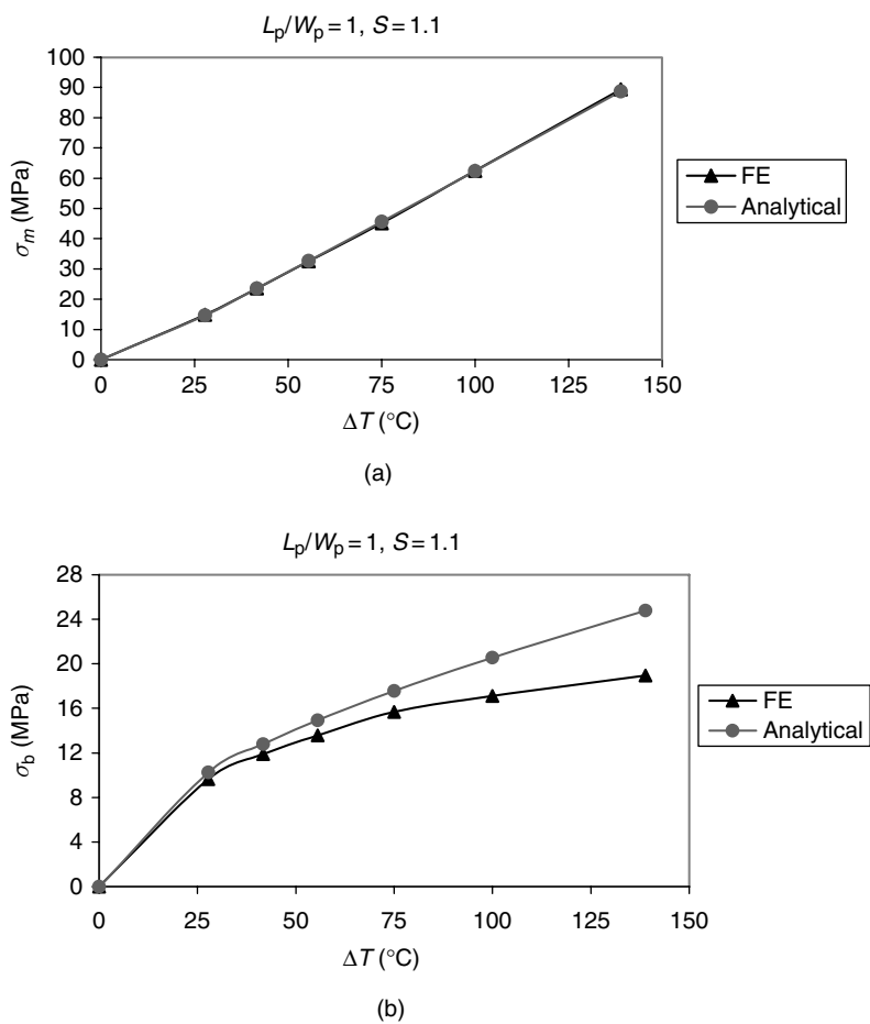
Fig. 5.13. Thermal stresses in the middle of a skin reinforced with a square patch for different temperature excursions: (a) the mean stresses; and (b) the bending stresses.
