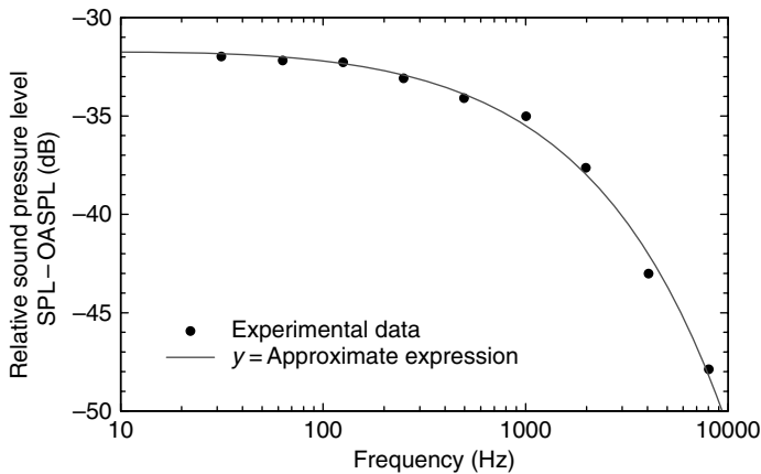
Fig. 12.5. Relative sound pressure levels (RSPL) over an external nacelle inlet.
