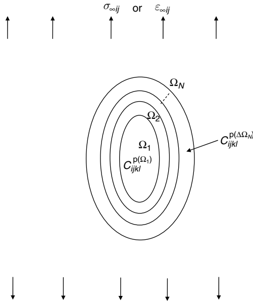
Fig. 13.1. Geometry of a tapered patch with concentric and similar ellipses.
