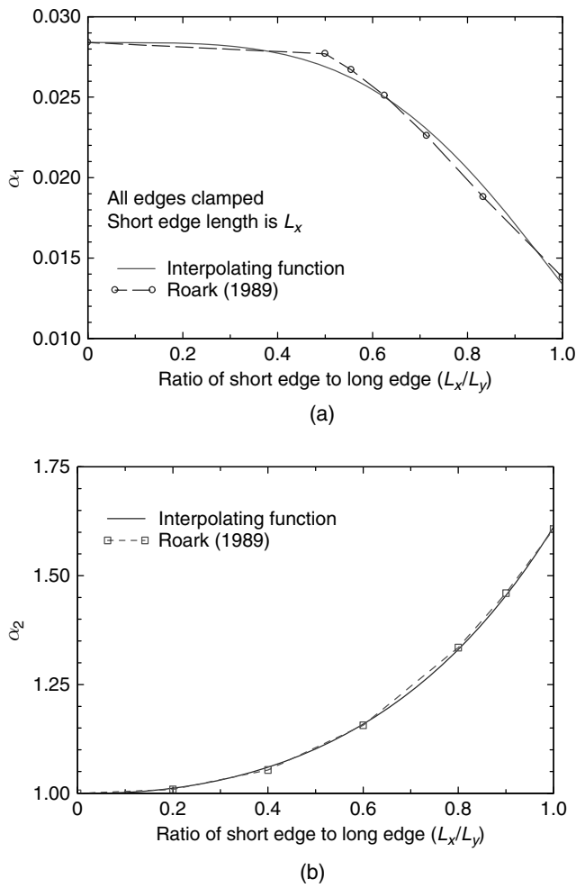
Fig. 12.2. Shape factors for: (a) displacement; and (b) resonant frequency.
