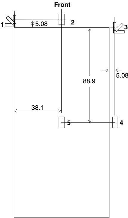
Fig. 11.25. Strain gauge locations for a sandwich plate with rectangular patches.
