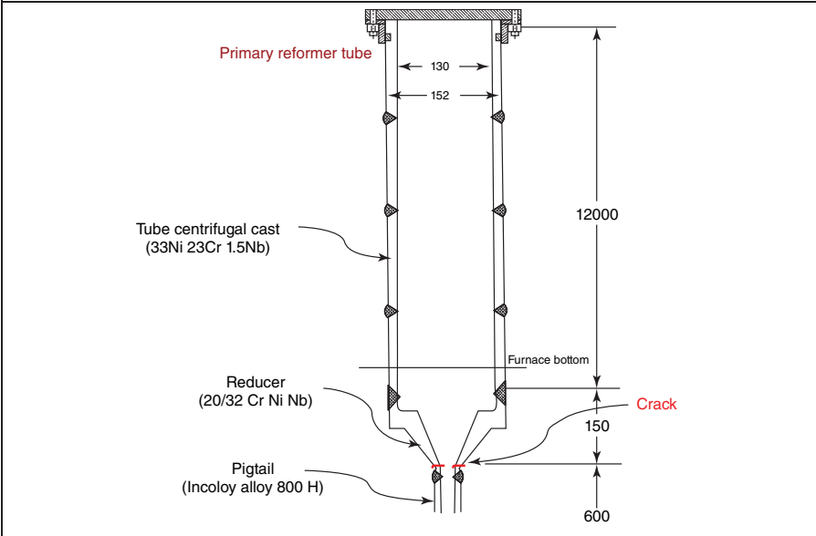
Case 15 Cross section of a reformer tube showing crack at the reducer at the bottom.
