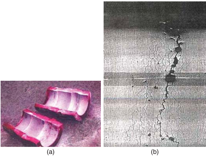
Case 45 (a) Dye penetrant test indications on the heat affected zones of the weld. (b) Intergranular corrosion and cracking initiated on the outside surface in the weld heat affected zone (200X).
