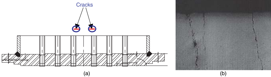
Case 13 (a) Longitudinal sketch of the bottom portion of tubes and bottom tube-sheet showing the location of the circumferential cracks in alcohol vapor super-heater. (b) Microstructure of the longitudinal cross section of the inside surface of a failed tube of the alcohol vapor super heater showing multiple cracks initiating on localized pits, (50X).
