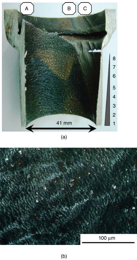
Figure 3.13 (a) Heavy thickness reduction near the socket weld (at location 8) and lower thickness reduction as seen at a distance 40 mm away from the socket weld (location 1) due to flow-induced corrosion is shown. (b) Characteristic features (Tiger Strips) of flow-induced corrosion seen at high magnification is shown (Source: Kain et al.(2011). Reprinted with permission from Elsevier.).
