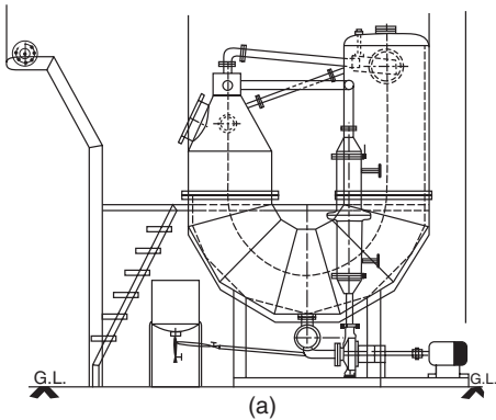
Case 27 (a) Elevation drawing of the U shape jet dyeing machine. (b) Localized sharp pitting corrosion marks on the inside surface of the perforated basket of jet dyeing machine.
