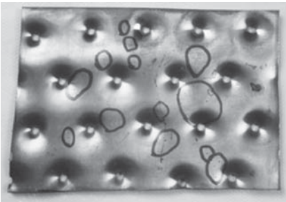
Case 27 (a) Elevation drawing of the U shape jet dyeing machine. (b) Localized sharp pitting corrosion marks on the inside surface of the perforated basket of jet dyeing machine.
