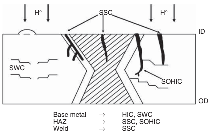
Figure 3.21 Forms of hydrogen damage in H_2S service. See the text for the explanations of the abbreviations. (Source: Elboudjaini (2011). Reprinted with permission from John Wiley & Sons, Inc.)
