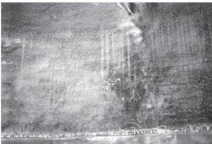
Case 68 (a) Corrosion pits on a baffle support bracket and nearby areas on the shell. (b) Corrosion pits on the shell above the weld line.
