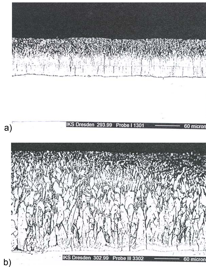
Figure 1: Zinc coatings in accordance with EN ISO 1461 on steel with different silicon content, metallographic transverse section with magnification 200:1, etched a) with pronounced pure-zinc layer b) with overalloyed iron-zinc-alloy layer
