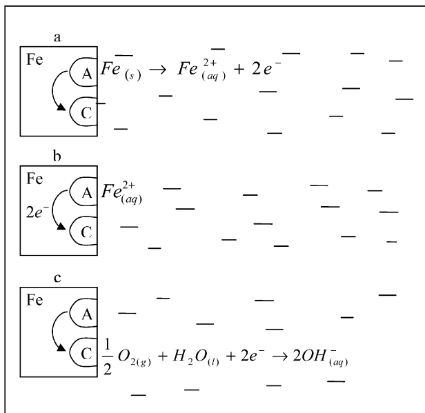
Fig. 1.14 Corrosion on a single whole carbon steel; (a) anodic process; (b) flow of electrons from an anode “A” to a cathode “C”; (c) cathodic process.
