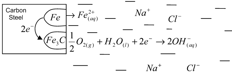
Fig. 1.16 Electrochemical corrosion of carbon steel in water and aqueous salt solutions. Iron (Fe) is an anode; cementite ( \text{Fe}_3\text{C} ) is a cathode.
