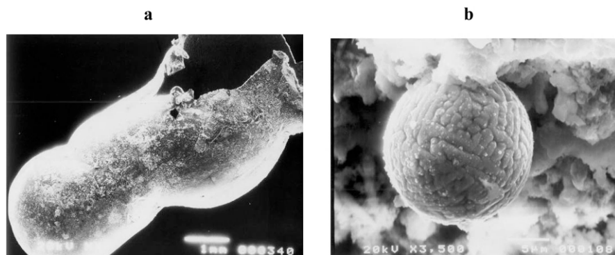
Fig. 3.12 SEM photo of a corrosion "cylinder" (a) with length 7.4 mm and magnification ( \times 3,500 ) of the inner surface of the "cylinder" (b). Diameter of the "ball" 17 \mu m .
