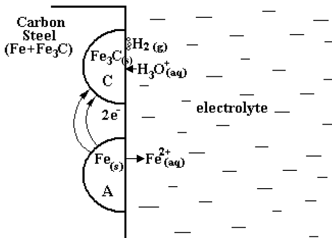
Fig. 1.19 Electrochemical corrosion mechanism of carbon steel in acid. “A” (Fe) – anode; “C” ( \text{Fe}_3\text{C} ) – cathode.
