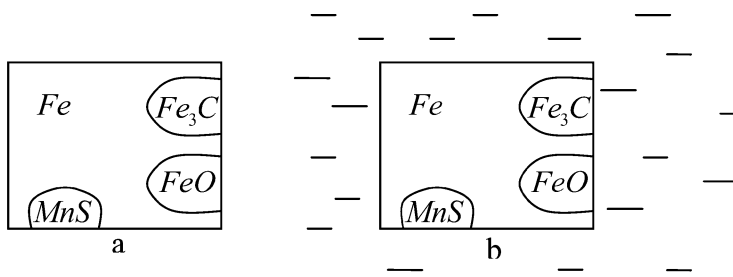
Fig. 1.13 Carbon steel surface; (a) in a dry atmosphere; (b) in the presence of liquid electrolytes (solution of NaCl in water).
