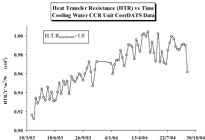
Fig. 5.14 Heat transfer resistance (HTR) versus time (cooling water system).
