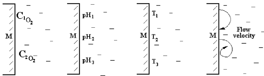
Fig. 2.2 Heterogeneity of the environment on the metal (M) surface. C_1(O_2) , C_2(O_2) -various concentrations of dissolved oxygen. pH_1 , pH_2 , pH_3 -different values of pH. T_1 , T_2 , T_3 -various temperatures.
