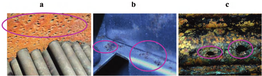
Fig. 2.3 Pits on the carbon steel tube-sheet of a heat exchanger (a), stainless steel 316 bath (b) and Admiralty brass tubes (c). Pits are encircled.
