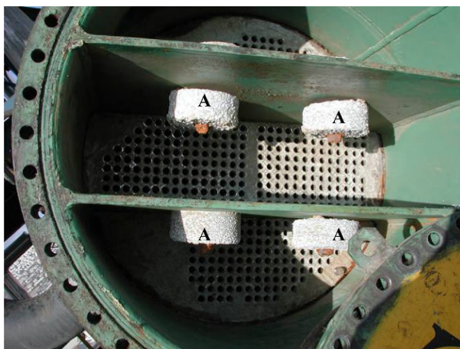
Fig. 4.8 Aluminum sacrificial anodes (A) installed on the inside of heat exchangers coated with epoxy paint (green). The cooling water flows inside the tubes.
