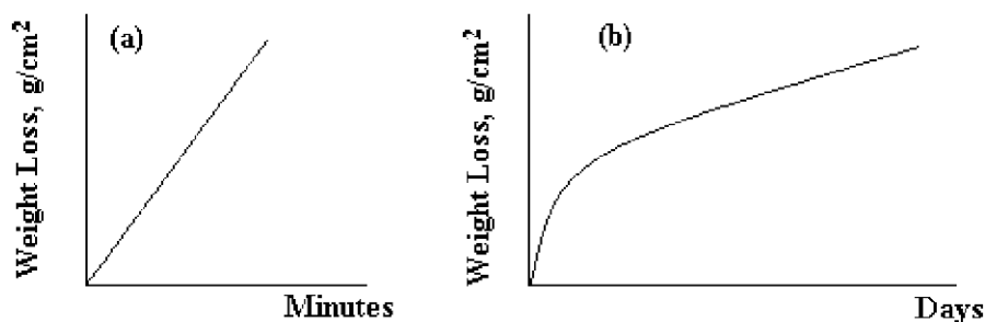
Fig. 1.6 Kinetic curves for corrosion of iron in hydrochloric acid (a) and in water (b).
