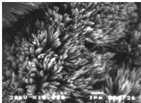
Fig. 1.18 Scanning electron microphotograph of rust formed in warm water: Lepidokrochite [ \gamma -FeO(OH)] ( \times 10,000 ).
