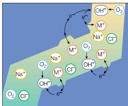
□ Crevice corrosion. This type of corrosion often starts at drillpipe joints, tubing collars or casing collars. The gap in the joint becomes devoid of oxygen and anodic. In salty water the corrosion is promoted by the migration of negatively charged chlorine ions [ \text{Cl}^- ] to the crevice. These not only counteract the buildup of positive charges around the crevice, but also act as a catalyst accelerating the dissolution of metal [ \text{M}^+ ]. This ongoing process leads to a deep pit.
