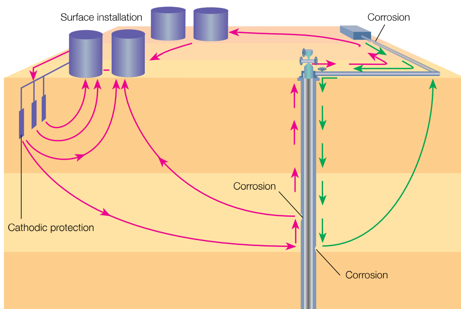
□ Stray-current corrosion. Current paths are shown between surface installation, electrical machinery, pipelines and a well. Current leaving the casing sets up an anodic area and corrosion.
