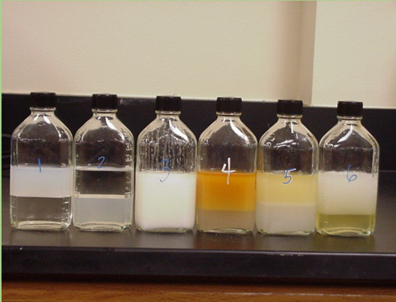
Emulsion Tendency test
