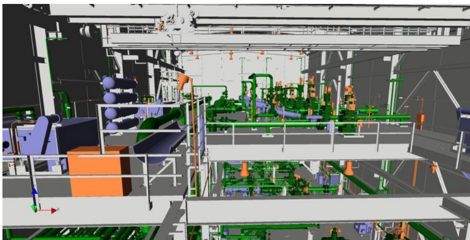
Figure 18.4 A 3D model of a processing facility created using 3D laser scanning. (see colour plate section).
