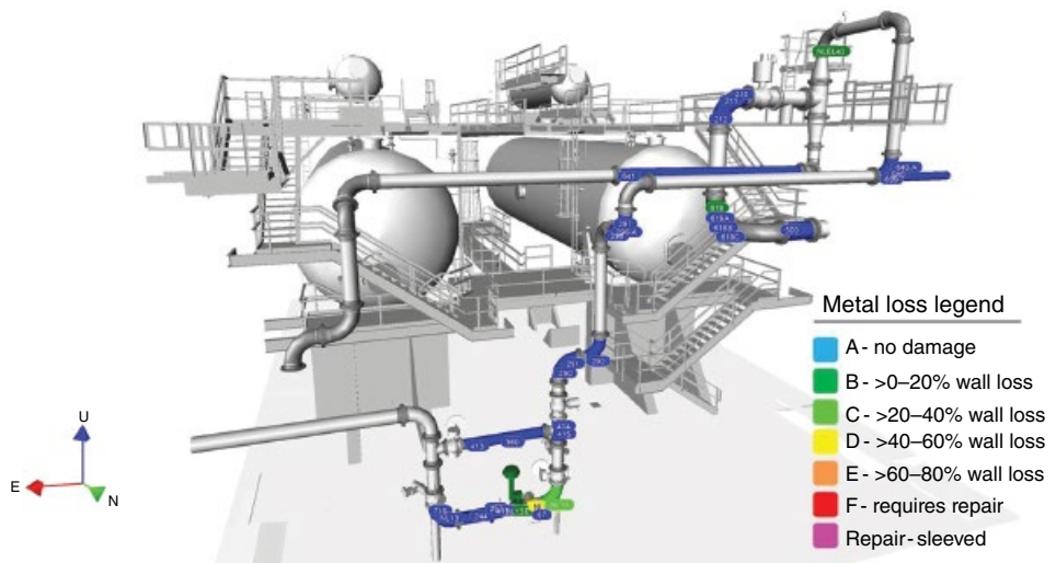
Figure 18.5 A 3D model of indoor facility piping showing inspection data.
