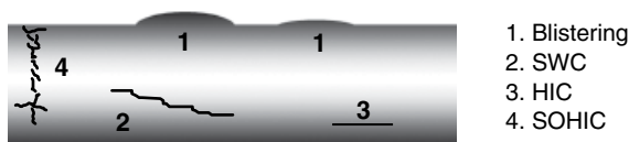
Figure 6.2 Principal types of corrosion threat in H_2S -containing environments.
