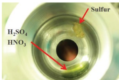
Figure 12.3 \text{H}_2\text{SO}_4 , (7 M) \text{HNO}_3 (0.2 M) and elemental sulphur formed in corrosion experiment performed at 45 °C, 100 bar and \text{CO}_2 composition, as given in last column in Table 12.1, Source: [11].
