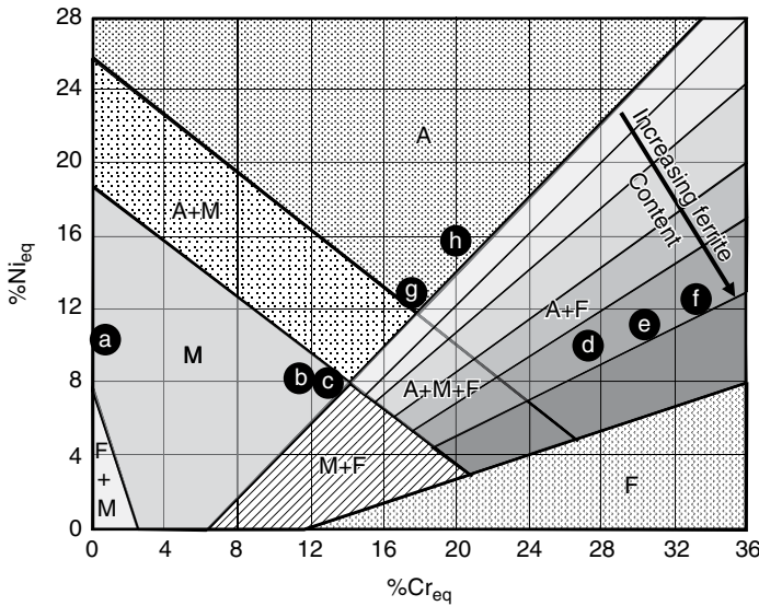
Figure 3.1 A typical Schaeffler diagram. (A: Austenite, M: Martensite, F: Ferrite) typical position of different steels: (a): Grade API 5CT L80 CLAS, (b): 13%Cr, (c): Alloyed 13%Cr, (d): 22Cr DSS, (e): 25Cr DSS, (f): 25Cr SDSS, (g): 304 SS, (h): 316SS.
