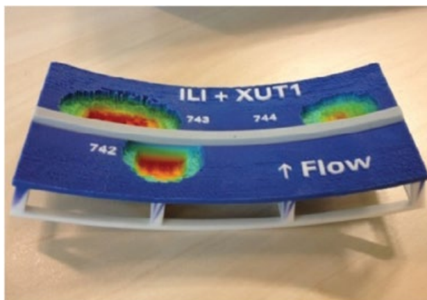
Figure 10.6 (a) Combined external and ILI UT data showing pipeline anomalies adjacent to a weld; and (b) a 3D-printed model of the pipeline anomalies.
