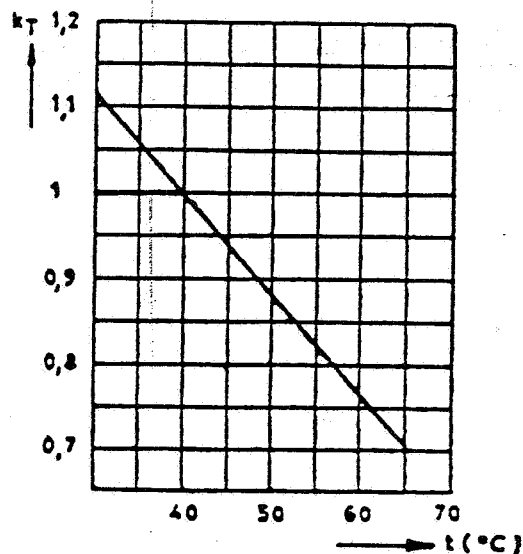
Figure 5.8.2.1.2.b. k_T : Correction factor for cooling medium temperature
