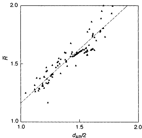
Figure 18. Plot of d_{AB} vs. \bar{R} for the binary compounds crystallizing in oP12 Co_2Si
