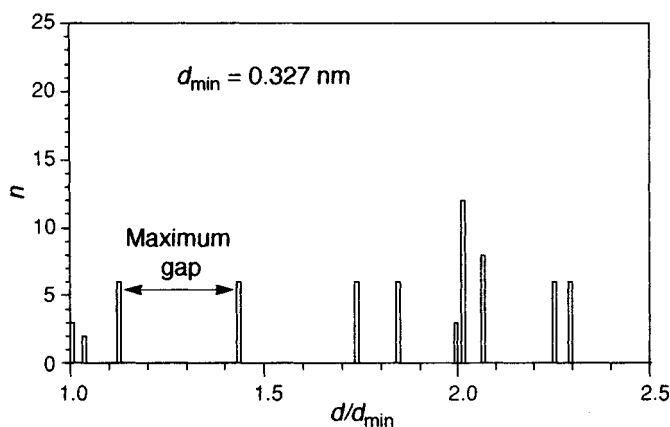
Figure 6. The NNH of the Bi atom in hP3 \text{Bi}_2\text{Tl} ; the AET is shown in Figure 2 with label 11-a
