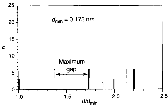
Figure 4. The NNH of the B atom in hP3 \text{AlB}_2 ; the AET is shown in Figure 2 with label 9-a
