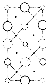
Cu_2(Zn,Fe)SnS_4 kesterite
