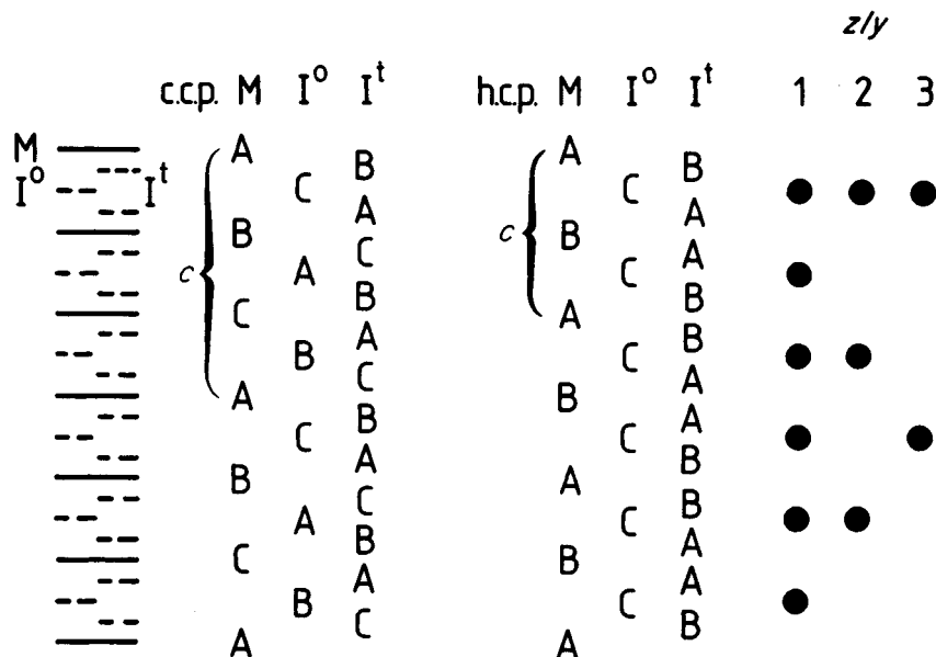
Figure 19. Position of interstitial atoms I^o and I^t in octahedral and tetrahedral sites of the ABC c.c.p. or AB h.c.p. M lattice. Only 1/2 or 1/3 (for \epsilon -Ni 3 C) of the octahedral sites I^o at identical positions in c direction of h.c.p. M lattice are occupied at z/y = 2 or 3, respectively
