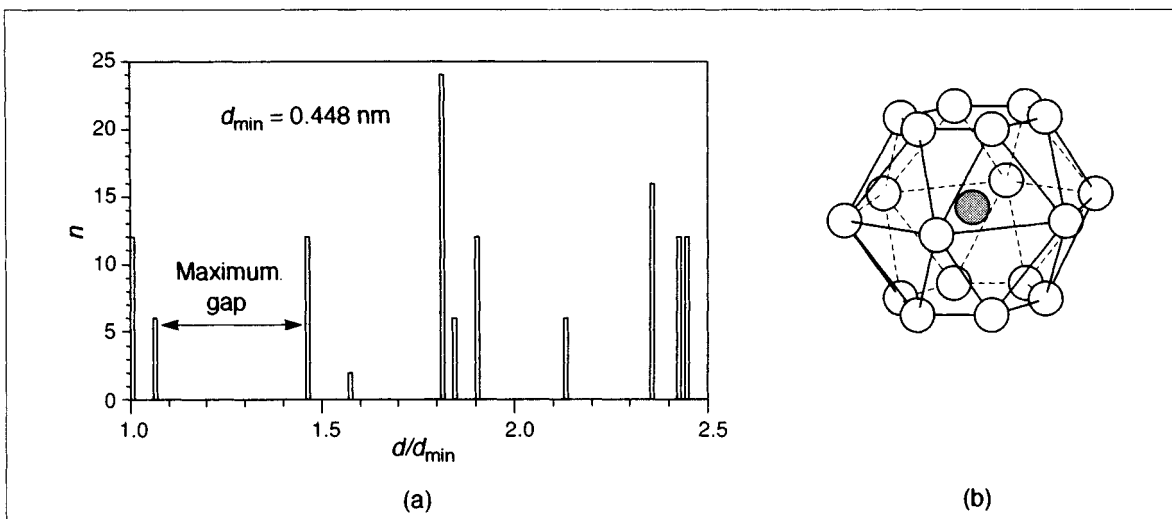
Figure 7. (a) The NNH of the Nd atom in hP3 \text{Ag}_2\text{Nd} and (b) the corresponding AET (CN=18, label 18-d)
