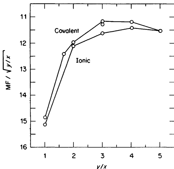
Figure 25. Madelung factors MF/\sqrt{y/x} versus concentration y/x for the undistorted covalent and ionic compounds of Figure 24
