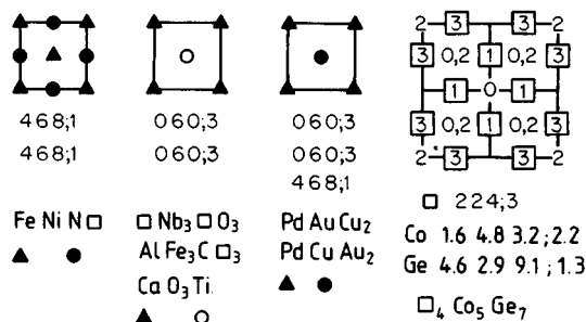
Figure 28. Ternary and quaternary compounds with T_1, T_2, T_3; y/x of different components with composition y/x . Only positions of minority elements are plotted, full and open symbols for elements at projection height z=0 and 0.5, respectively, or as multiples of a_0/4 in cubic \text{Co}_5\text{Ge}_7 .
