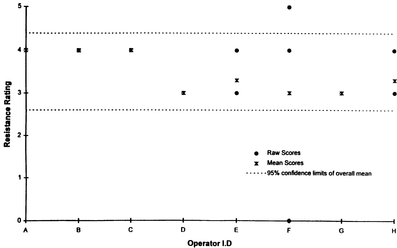
FIG. X1.3 Thick Film, 6-Hour Cure
