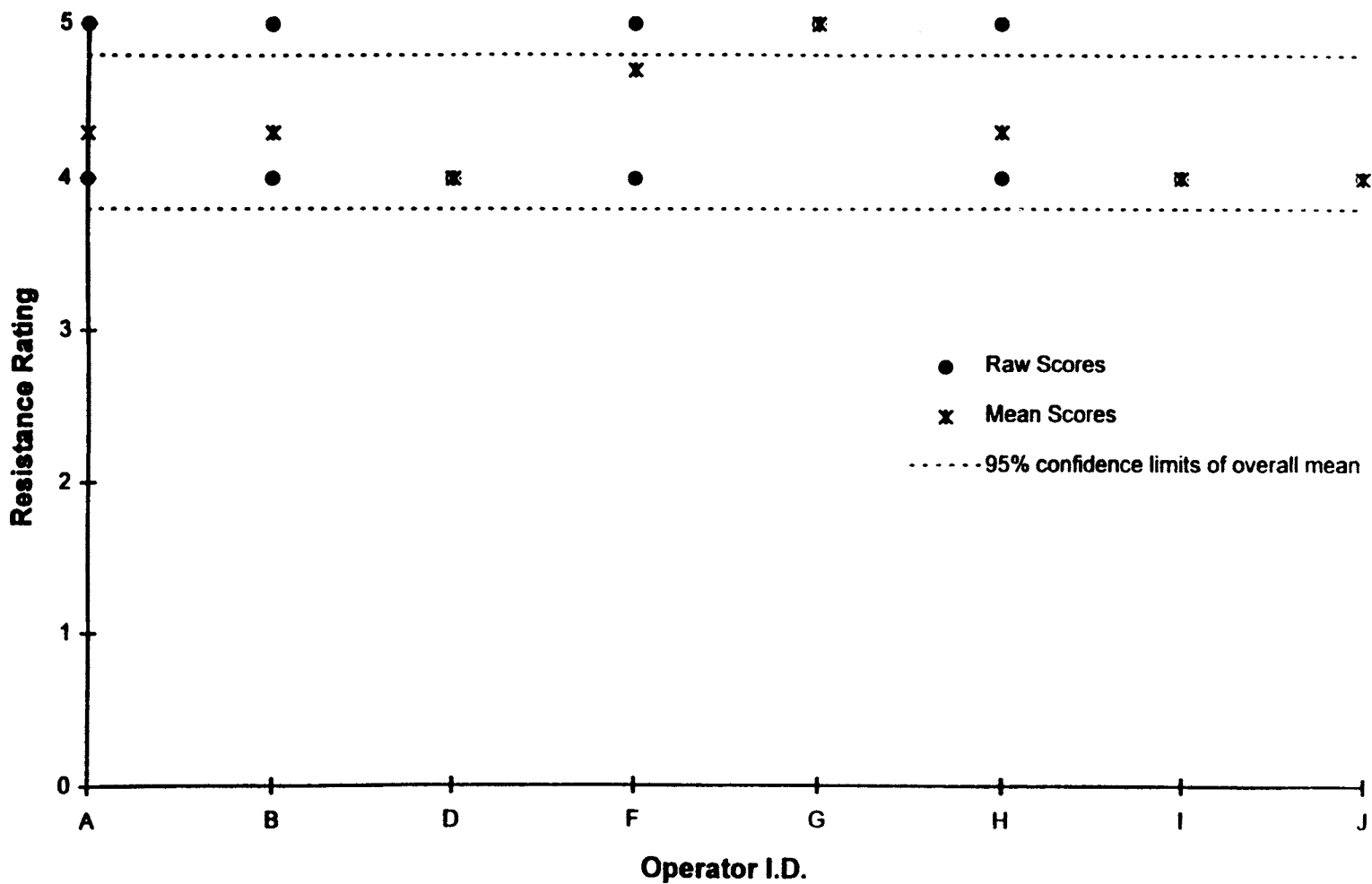
FIG. X1.2 Thin-Film, 24-Hour Cure
