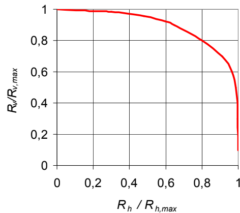
Figure 10-1 Schematic resistance diagram for suction anchor.
