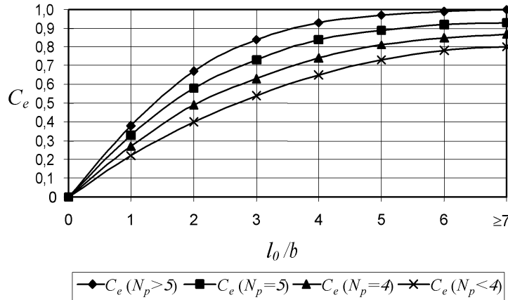
Figure 4-1 Graphs for the effective flange parameter C_e
