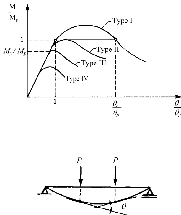
Figure A-1 Relation between moment M and plastic moment resistance M_p , and rotation \theta for cross sectional types. M_y is elastic moment resistance
