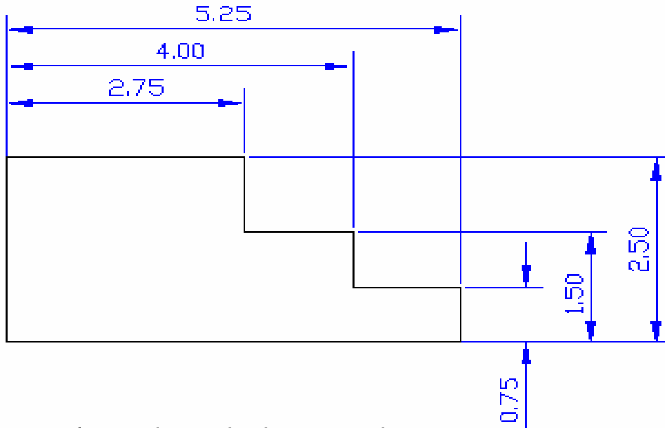
Datum Plane Dimensioning - Continuous
