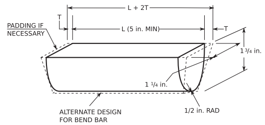
Design for "Attached" Coupon
