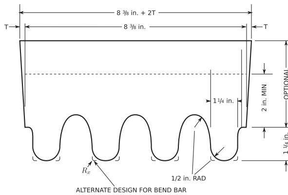
Design for Multiple Keel Block Coupon (4 legs)
