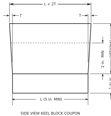
Design for Double Keel Block Coupon
