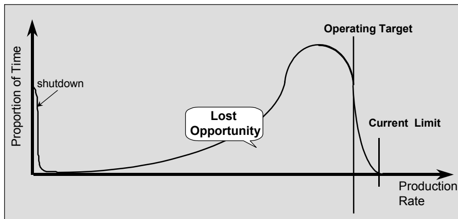
Figure 24 Productivity histogram
