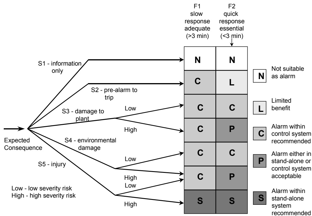
Figure 9 Example of risk graph for qualitative risk assessment
