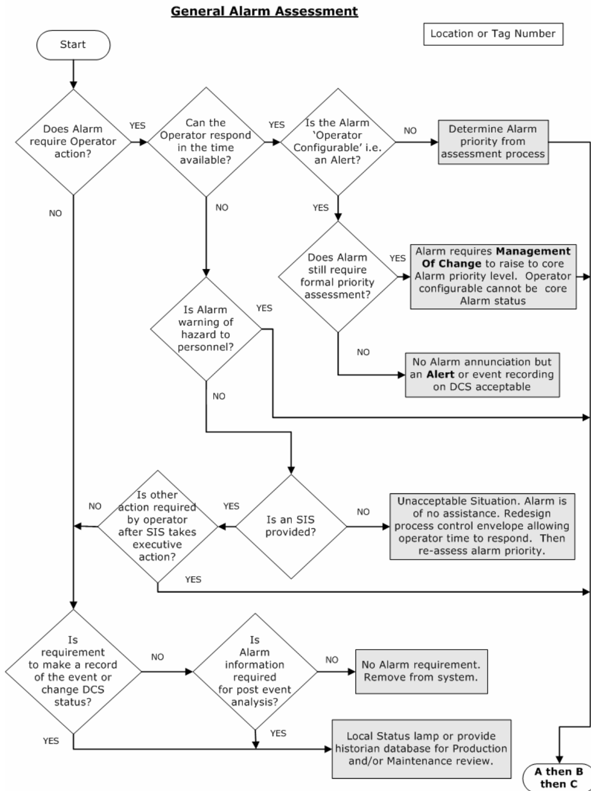
Figure 12 General Alarm Assessment
