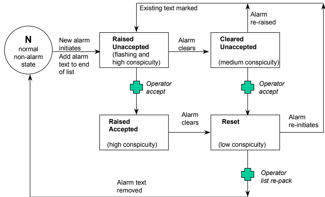
Figure 20 Alarm state transition diagram
