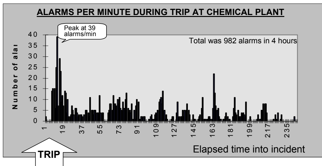
Figure 22 Example plot of alarms per minute
