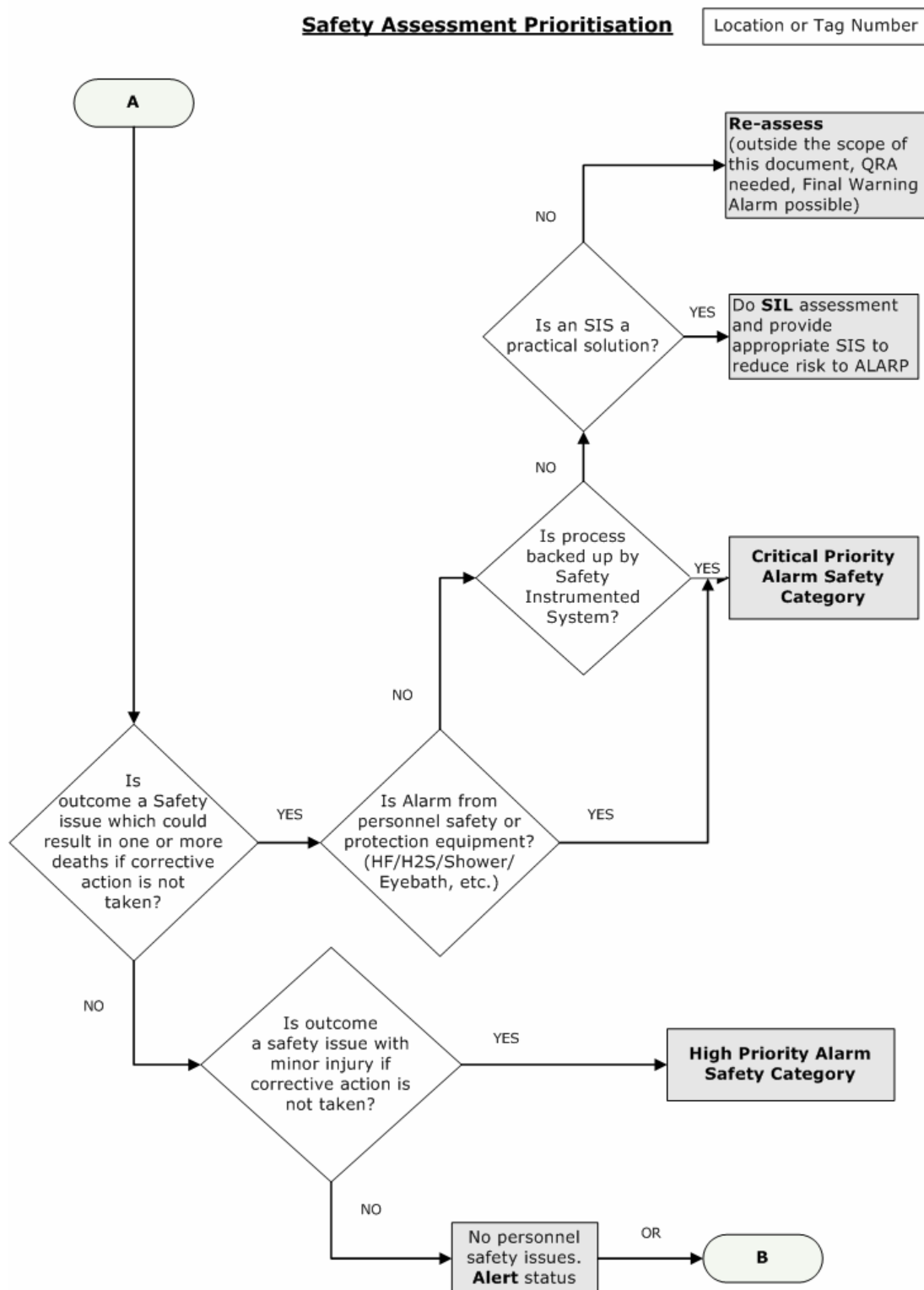
Figure 13 Safety Assessment Prioritisation
