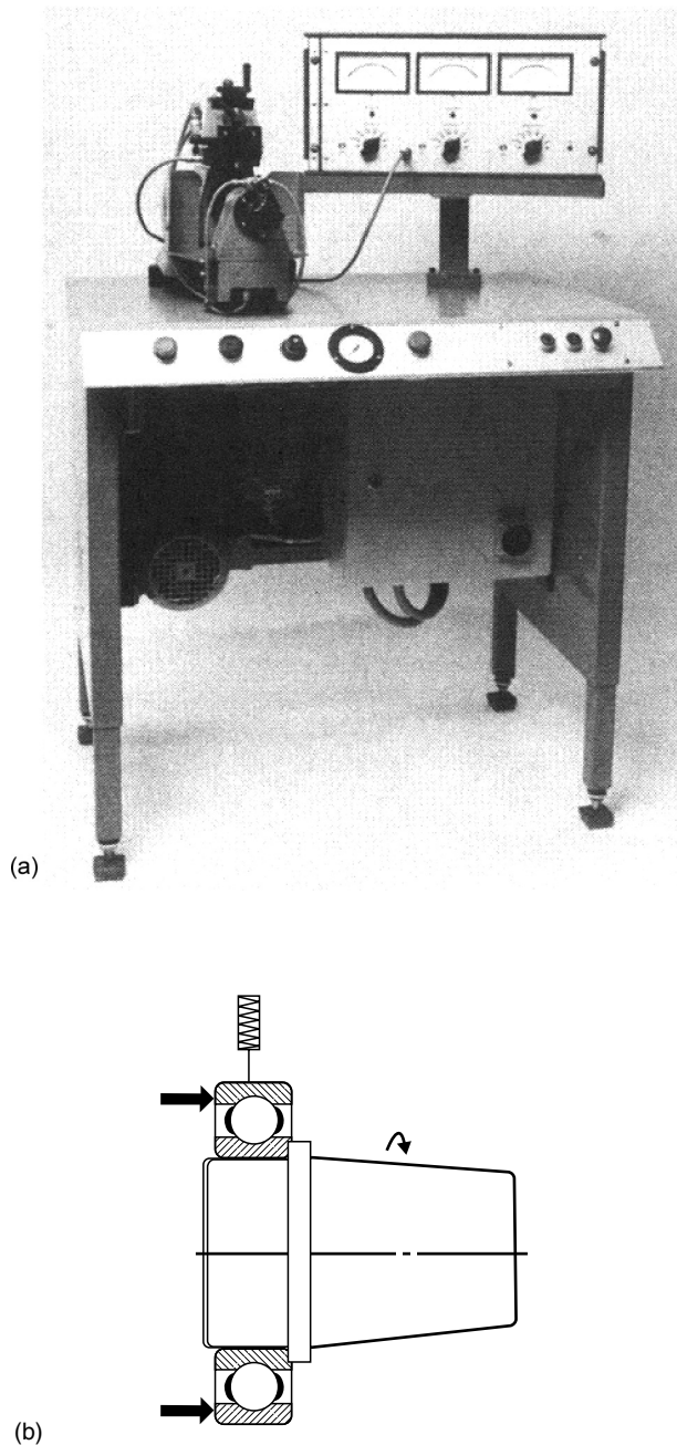
FIGURE 14.11 Bearing vibration tester: (a) test stand and (b) schematic of bearing loading and accelerometer on bearing outside diameter.
