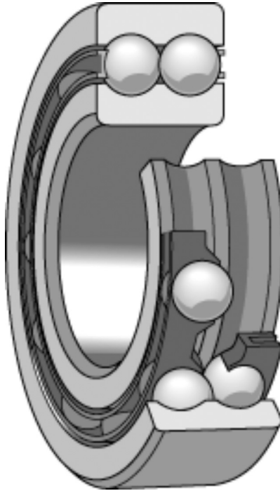
FIGURE 1.21 A double-row deep-groove radial ball bearing. (Courtesy of SKF.)
