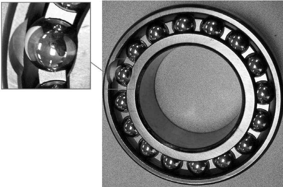
FIGURE 1.20 View of a single-row deep-groove filling slot-type ball bearing assembly. (Courtesy of the Timken Company.)
