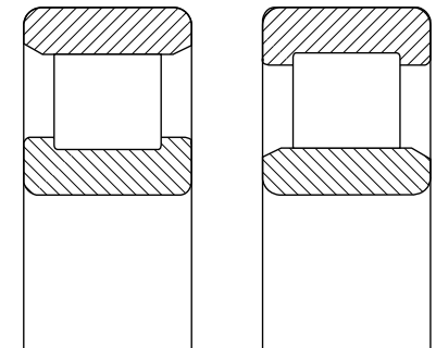
FIGURE 1.36 Cylindrical roller bearings without thrust flanges.
