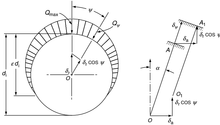
FIGURE 7.13 Rolling bearing displacements due to combined radial and axial loadings.
