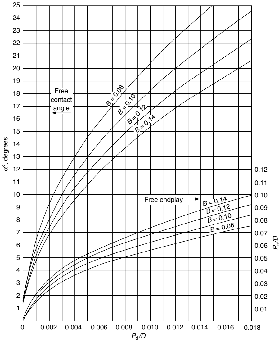
FIGURE 2.3 Free contact angle and endplay versus B = f_o + f_i - 1 for single-row ball bearings.
