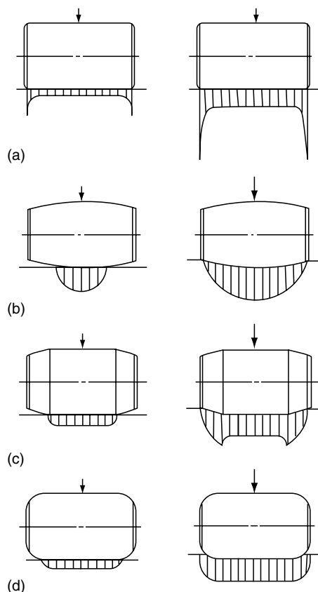
FIGURE 6.26 Roller–raceway contact load vs. length and applied load: a comparison of straight, fully crowned, partially crowned, and logarithmic profiles.
