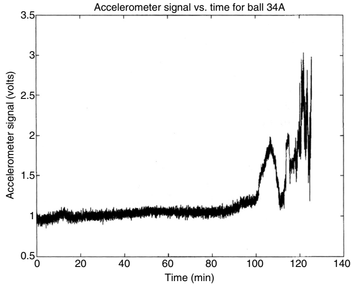
FIGURE 14.19 Accelerometer voltage signal for ball operating conditions in Figure 14.18 . (Courtesy of Oceana Sensor Technologies, Virginia Beach, Virginia.)
