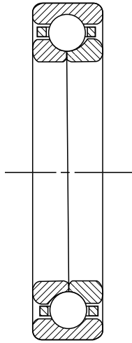
FIGURE 1.30 A split inner-ring ball bearing assembly.
