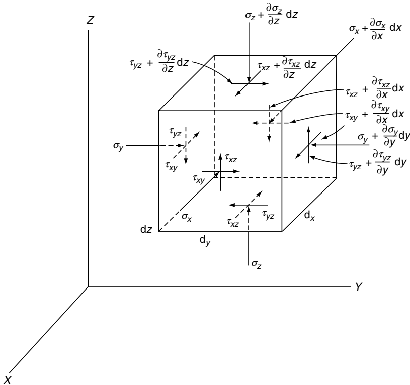
FIGURE 6.1 Stresses acting on an infinitesimal cube of material under load.
