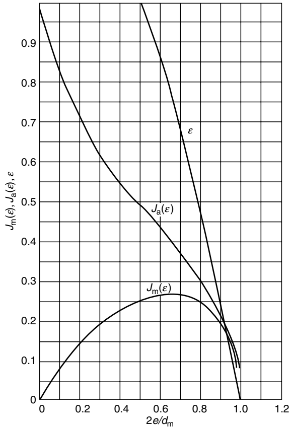
FIGURE 7.9 J_m(\varepsilon) , J_a(\varepsilon) , \varepsilon vs. 2e/d_m for line-contact thrust bearings.
