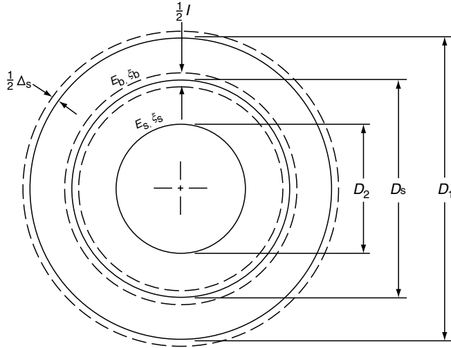
FIGURE 3.4 Schematic diagram of a bearing inner ring mounted on a shaft.
