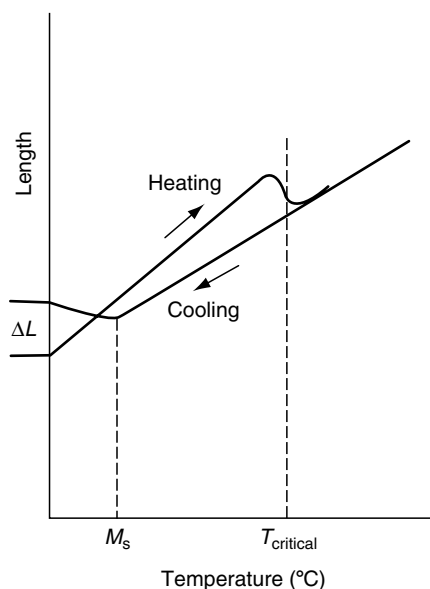
FIGURE 13.12 Volume changes during heating and quenching (hardening) of high-carbon bearing steel.
