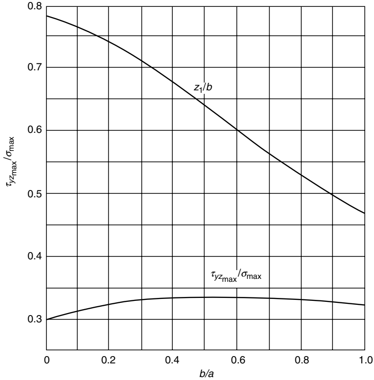
FIGURE 6.12 \tau_{yz\max}/\sigma_{\max} and z_1/b vs. b/a .
