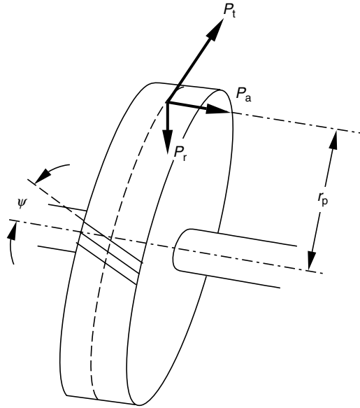
FIGURE 4.13 Loads transmitted by a helical gear.
