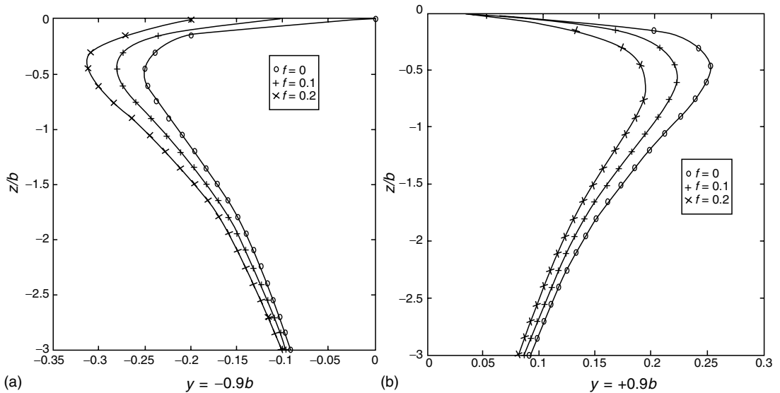
FIGURE 6.21 Orthogonal shear stress \tau_{yz}/\sigma_{\max} (abscissa) vs. depth z/b at contact area location x = 0 for friction coefficients f = 0, 0.1, 0.2 .
