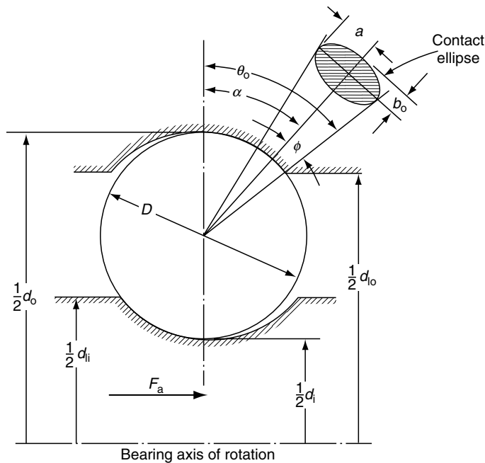
FIGURE 8.11 Ball-raceway contact under limiting thrust load.
