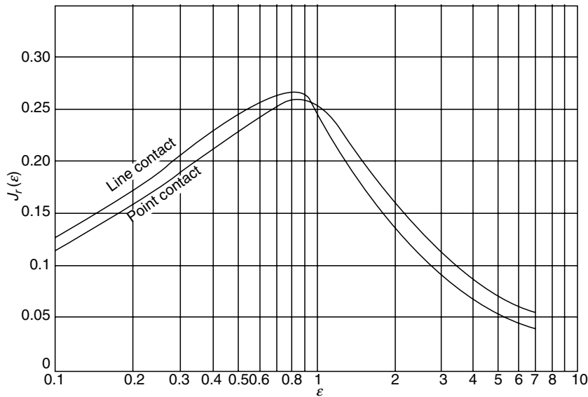
FIGURE 7.2 J_r(\varepsilon) vs. \varepsilon for radial bearings.
