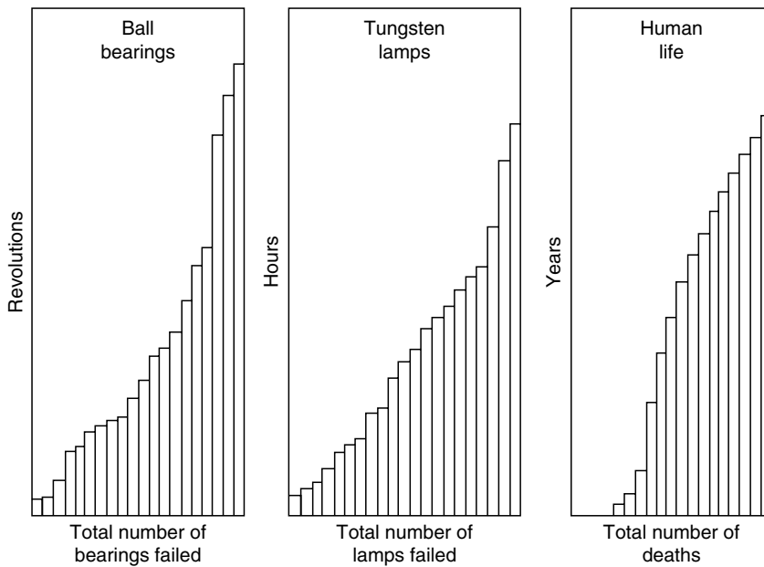
FIGURE 1.11 Comparison of rolling bearing fatigue life distribution with those of humans and light bulbs.
