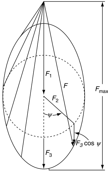
FIGURE 11.21 Load vector diagram for generalizing bearing loading consisting of steady load F_1 , rotating load F_2 , and sinusoidal load F_3 in phase with F_1 .
