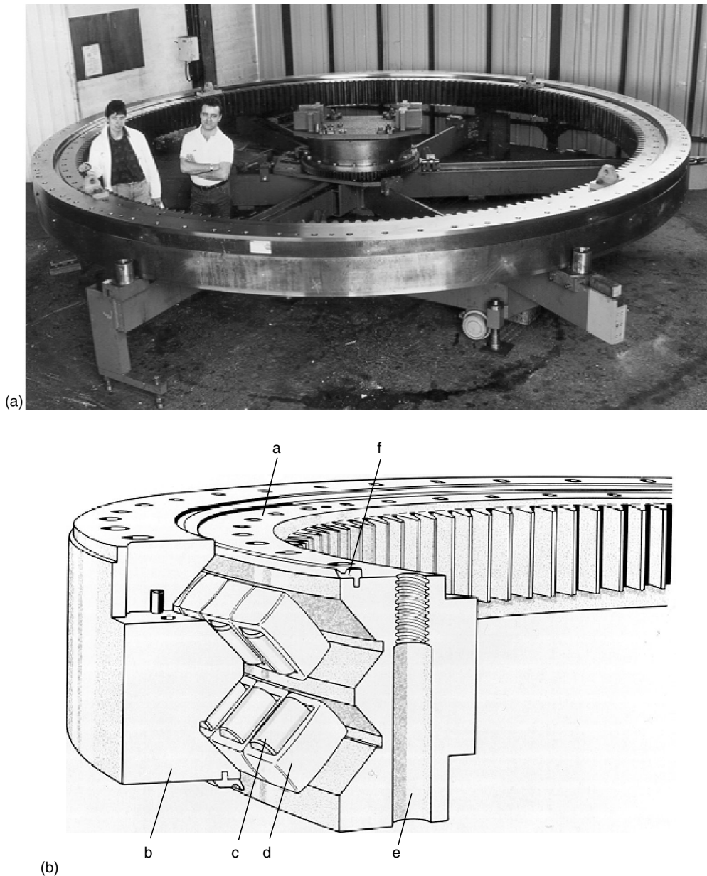
FIGURE 1.5 Large slewing bearing used in an English Channel tunneling machine. (a) Photograph; (b) schematic drawing of the assembly. (Courtesy of SKF.)
