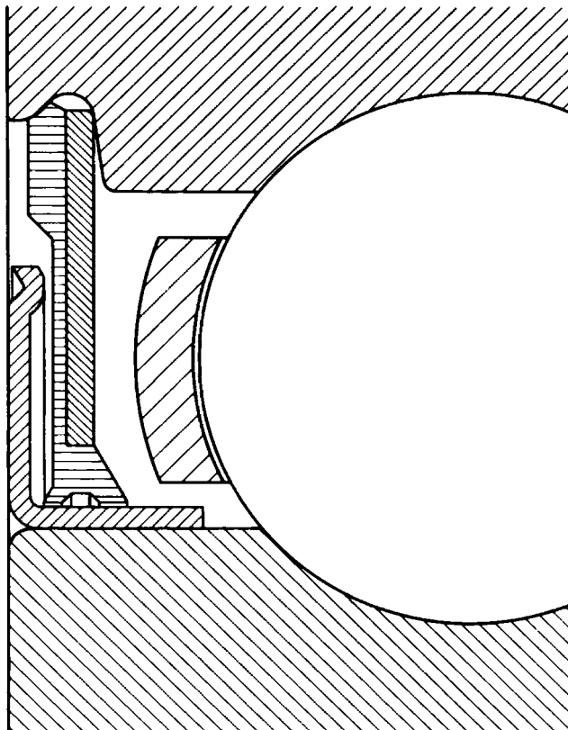
FIGURE 12.8 Deep-groove ball bearing assembly with integral labyrinth seal and flinger ring.
