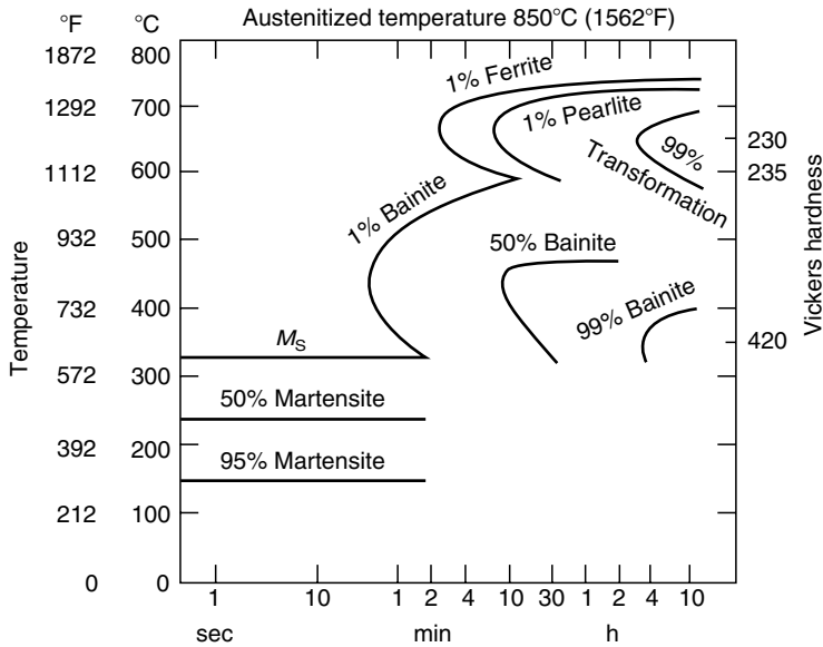
FIGURE 13.10 Time-temperature transformation diagram for AISI 4337 steel. (From SKF Steel, The Black Book , Vol. 151, 1984. With permission.)
