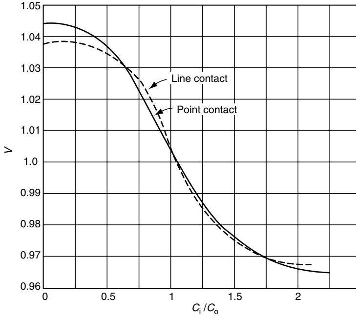
FIGURE 11.14 Rotation factor V vs. C_i/C_o .
