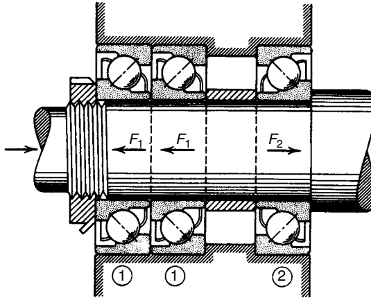
FIGURE 8.8 Triplex set of angular-contact bearings, two mounted in tandem and one opposed. This arrangement provides an even higher axial stiffness and longer bearing life than with a duplex set, but requires more space.
