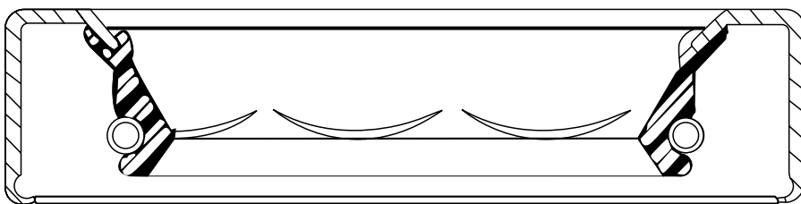
FIGURE 12.13 Radial seal with “quarter moon” projections molded on the lip to develop a hydrodynamic lubricant film during operation.
