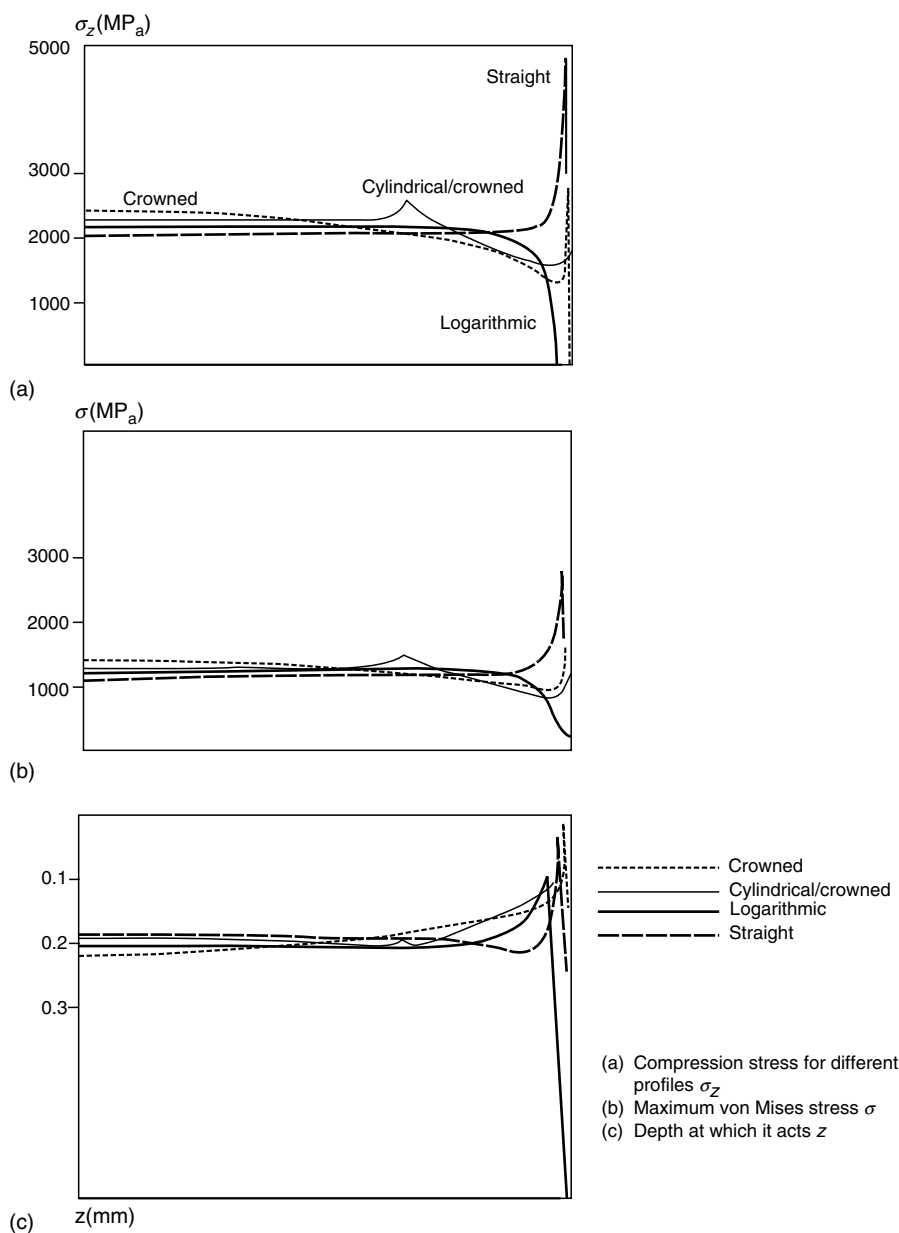
FIGURE 6.28 Comparison of surface compressive stress \sigma_z , maximum von Mises stress \sigma_{VM} , and depth z to the maximum von Mises stress for various roller (or raceway) profiles. (From Reusner, H., Ball Bearing J. , 230, SKF, June 1987. With permission.)
