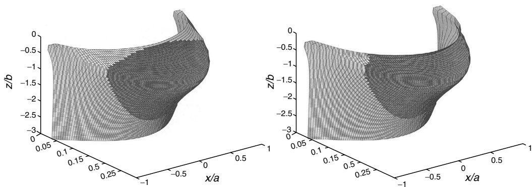
FIGURE 6.22 Octahedral shear stress \tau_{\text{oct}}/\sigma_{\max} ( y direction) vs. depth z/b and location x/a .
