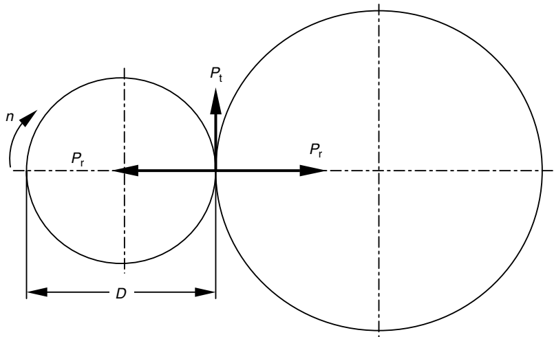
FIGURE 4.8 Schematic illustration of friction wheel loading.
