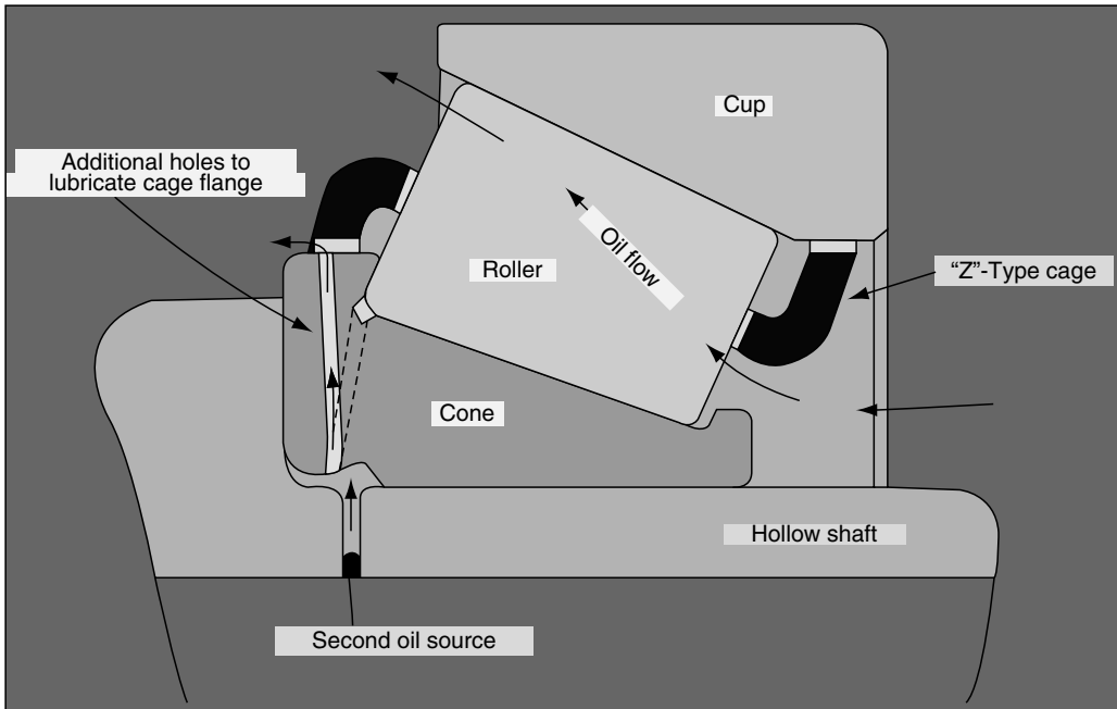
FIGURE 1.49 High-speed tapered roller bearing with radial oil holes and manifold. The “Z”-type cage is guided on the cone rib and cup lands. (Courtesy of the Timken Company.)
