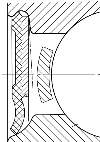
FIGURE 12.10 Radial ball bearing with integral single-lip seal.
