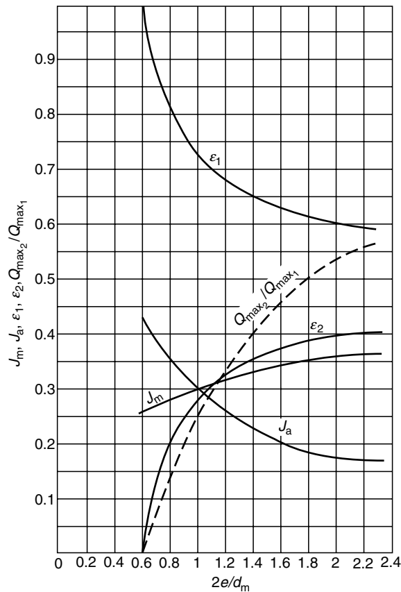
FIGURE 7.11 J_m, J_a, \epsilon_1, \epsilon_2, Q_{\max_2}/Q_{\max_1} vs. 2e/d_m for double-row point-contact thrust bearings.
