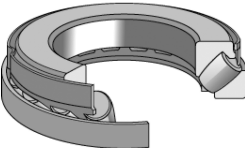
FIGURE 1.53 Cutaway view of a spherical roller thrust bearing assembly. (Courtesy of SKF.)
