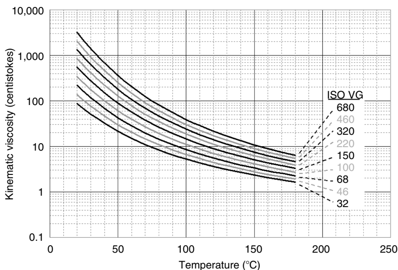
FIGURE 12.2 Variation of lubricant viscosity with temperature for various mineral oils (at atmospheric pressure).
