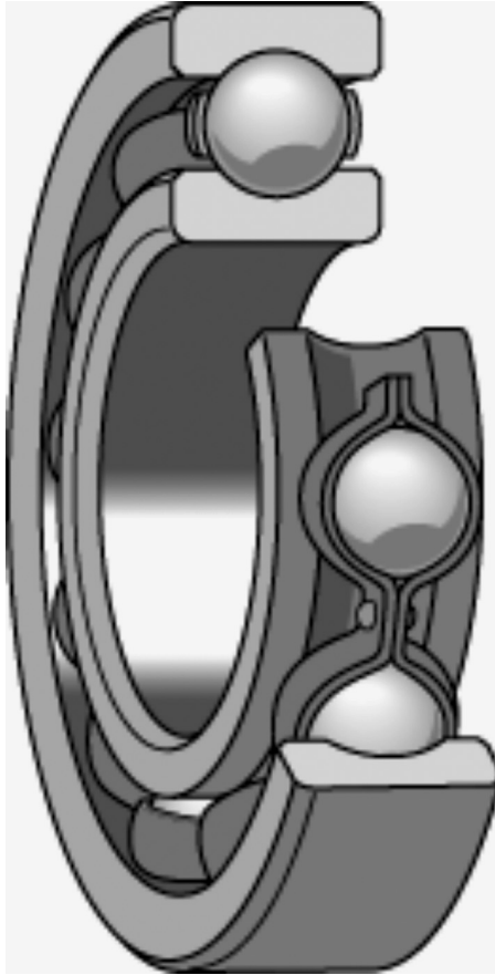
FIGURE 1.12 A single-row deep-groove Conrad-assembly radial ball bearing. (Courtesy of SKF.)
