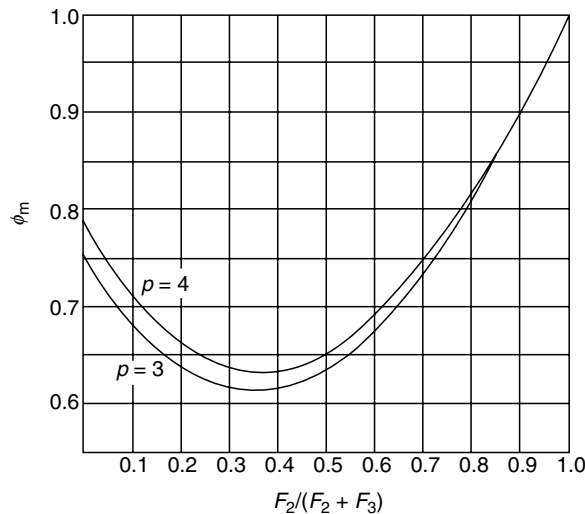
FIGURE 11.27 \phi_m vs. F_2/(F_2 + F_3) for the loading in Figure 11.26.
