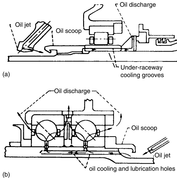
FIGURE 12.5 Under-raceway lubricating systems for mainshaft bearings in an aircraft gas turbine engine. (a) Cylindrical roller bearing. (b) Ball bearing.
