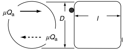
FIGURE 5.8 Schematic diagram of friction forces between roller ends and ring flanges. (The black dot represents a force vector passing into the page; the gray dot represents a force vector coming out of the page.)
