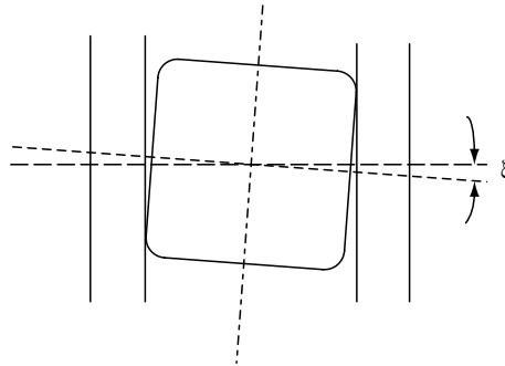
FIGURE 5.9 Roller skewing angle \xi limited by axial clearance between roller and guide flanges.
