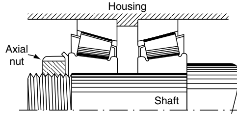
FIGURE 8.7 Lightly preloaded tapered roller bearings.
