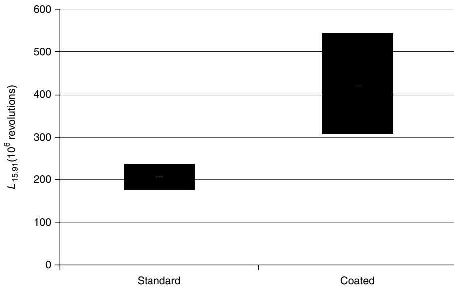
FIGURE 13.24 Endurance test results with 65% confidence bands for tapered roller bearings operating in thin lubricant films with (coated) and without (standard) TiC/aC:H-coated rollers.
