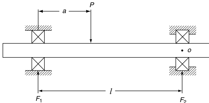
FIGURE 4.1 Two-bearing-shaft system.
