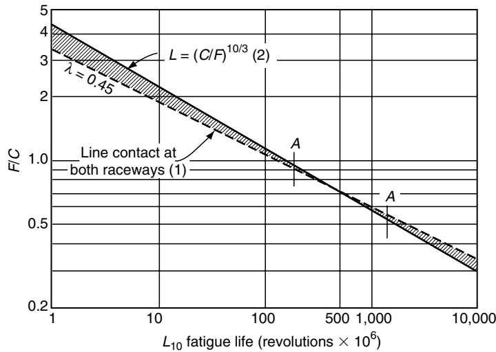
FIGURE 11.16 L_{10} vs. F/C for line contact at both raceways.
