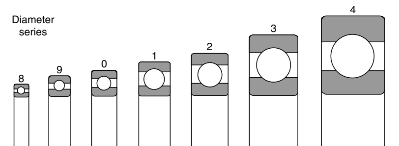
FIGURE 1.19 Size comparison of popular deep-groove ball bearing dimension series.
