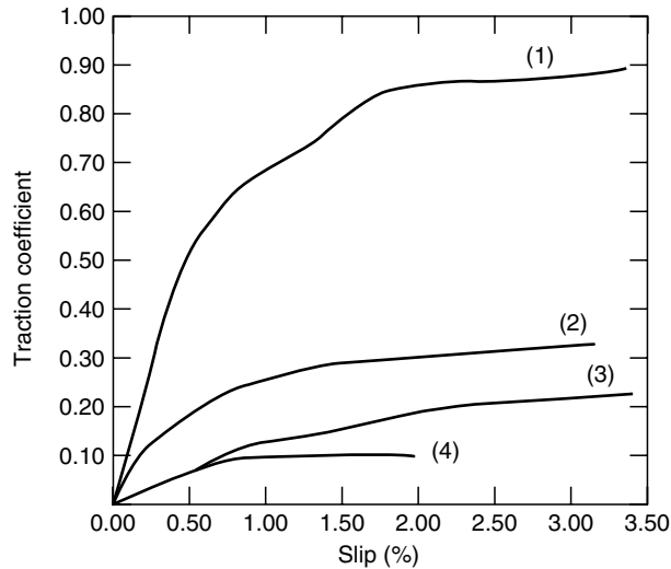
FIGURE 13.17 Traction coefficient vs percent slip in the contact between two bodies of hot-pressed silicon nitride. Contact stress is 2,068 MP a (300,000 psi); nominal speed is 3,800 mm/sec (150 in./sec). (From Pallini, R., Turbine engine bearings for ultrahigh temperatures, Ball Bearing J. , SKF, 234, 12–15, July 1989. With permission.) Operating conditions: (1) 25°C (77°F)—dry contact; (2) 370°C (698°F)—graphite lubrication; (3) 538°C (1000°F)—graphite lubrication; (4) 25°C (77°F)—oil lubrication.
