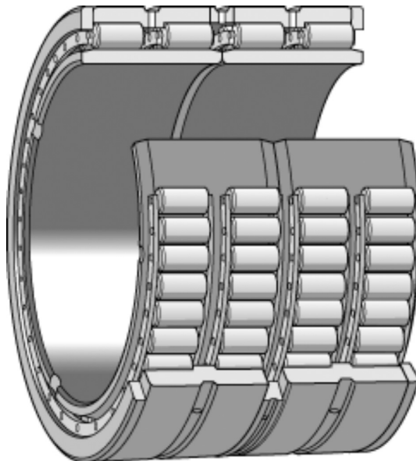
FIGURE 1.40 A multirow cylindrical roller bearing for a steel rolling mill application. (Courtesy of SKF.)
