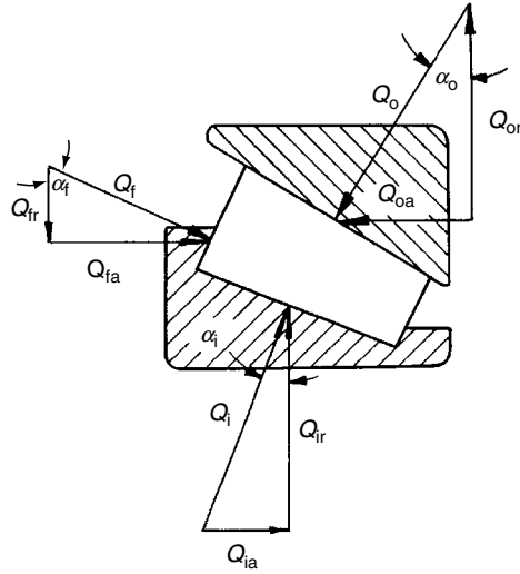
FIGURE 5.3 Radially loaded asymmetrical roller.
