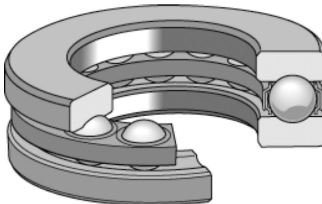
FIGURE 1.33 A 90^\circ contact angle thrust ball bearing assembly. (Courtesy of SKF.)
