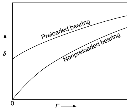
FIGURE 8.4 Deflection vs. load characteristics for ball bearings. As the load increases, the rate of increase of deflection decreases; therefore, preloading (top line) tends to reduce the bearing deflection under additional loading.
