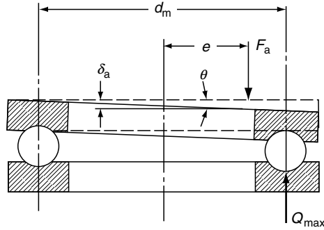
FIGURE 7.7 90° ball thrust bearing under an eccentric load.
