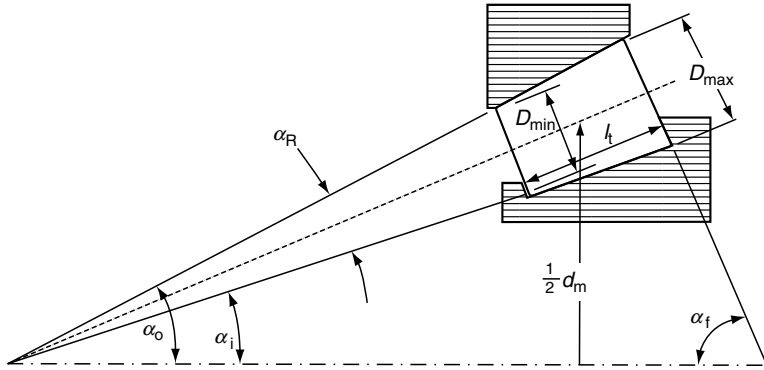
FIGURE 2.13 Internal dimensions for tapered roller bearing performance analysis.
