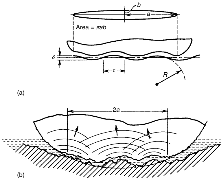
FIGURE 6.20 Models for less-than-ideal elastic conformity. (a) Hertzian contact model used in developing elastic conformity parameter. (b) Elastic conformity envisaged with real roughness would be preferential to certain asperity wavelengths. For convenience, the figure shows only one compliant rolling element, whereas in practice if materials of similar modulus were employed the deformation would be shared.
