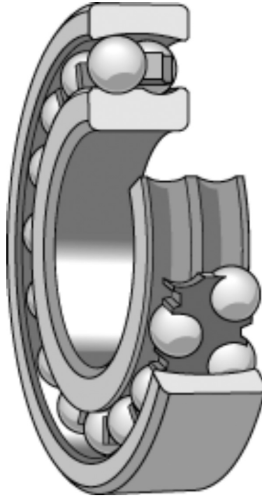
FIGURE 1.28 A double-row internally self-aligning ball bearing assembly. (Courtesy of SKF.)
