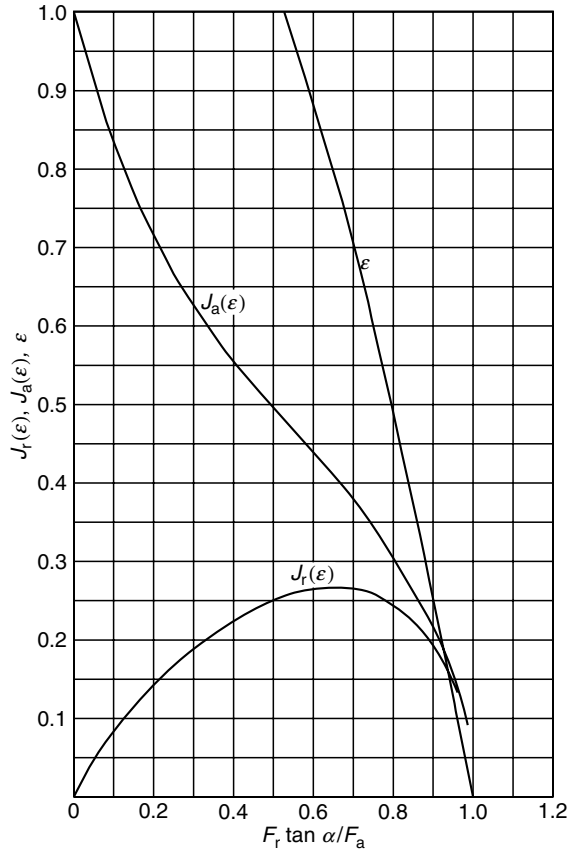
FIGURE 7.15 J_r(\varepsilon) , J_a(\varepsilon) , \varepsilon vs. F_r \tan \alpha / F_a for line-contact bearings.
