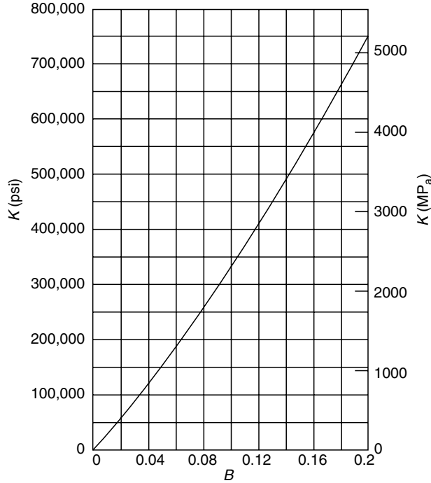
FIGURE 7.5 Axial deflection constant K vs. total curvature B for ball bearings ( B = f_o + f_i - 1 , f = r/D [2]).
