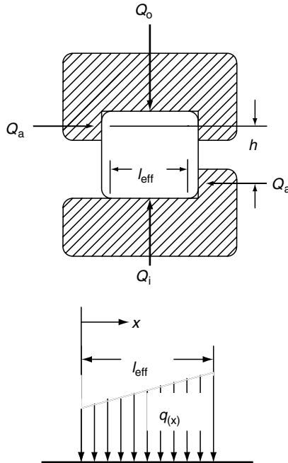
FIGURE 5.6 Loading of cylindrical roller on inner raceway under applied combined radial and axial loads, loading with straight profile rollers (no edge loading).
