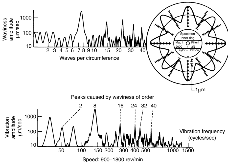
FIGURE 14.7 Waviness and vibration spectra from an inner ring with accentuated waviness. (From Yhland, E., Waviness measurement—an instrument for quality control in rolling bearing industry, Proc. Inst. Mech. Eng. , 182, Pt. 3K, 438–445, 1967–1968.)
