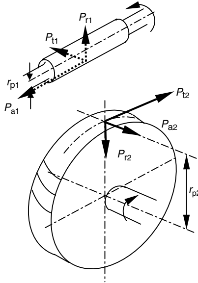
FIGURE 4.18 Schematic of tooth loading in a worm gear drive.
