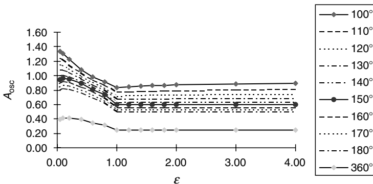
FIGURE 11.29 A_{osc} vs. load zone extent and 100–360° oscillation angles.
