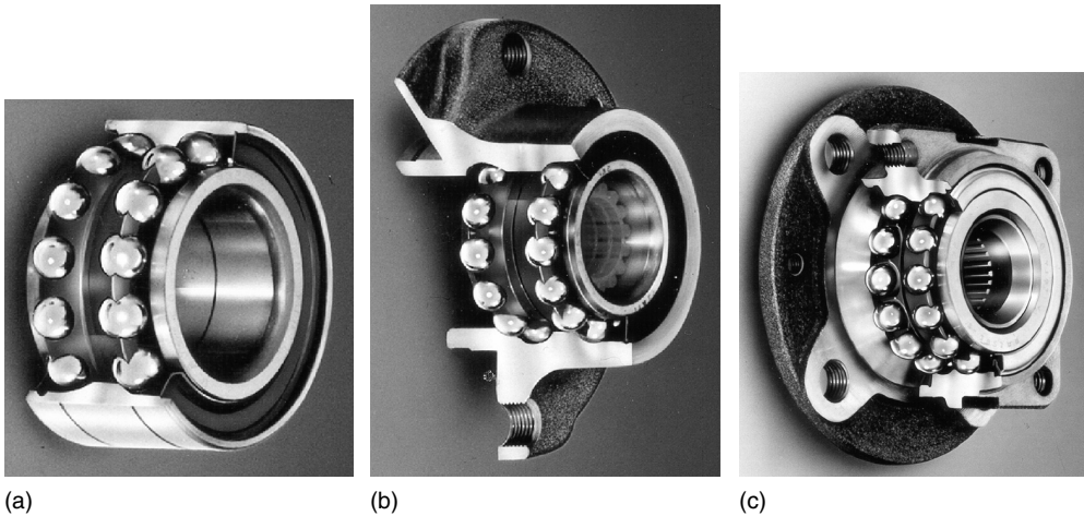
FIGURE 1.62 Modern automobile wheel preadjusted, greased, and sealed-for life, ball bearing units. (a) Without flanges; unit is press-fitted into wheel hub and slip-fitted onto the axle; (b) with a single flange integral with the outer ring of the bearing; (c) with flanges integral with the outer and inner rings of the bearing. (Photographs courtesy of SKF.)
