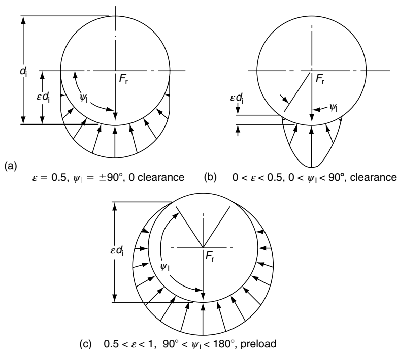
FIGURE 7.3 Rolling element load distribution for different amounts of clearance.
