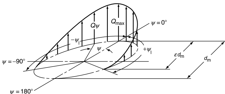
FIGURE 7.10 Load distribution in a 90° thrust bearing under eccentric load.
