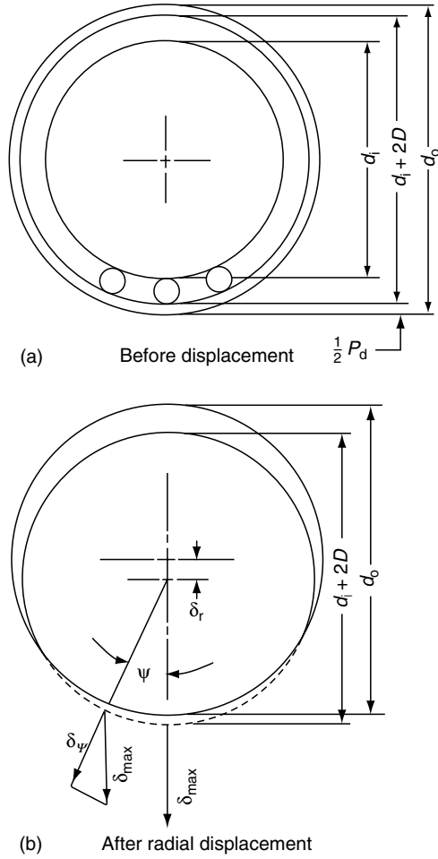
FIGURE 7.1 Bearing ring displacement.
