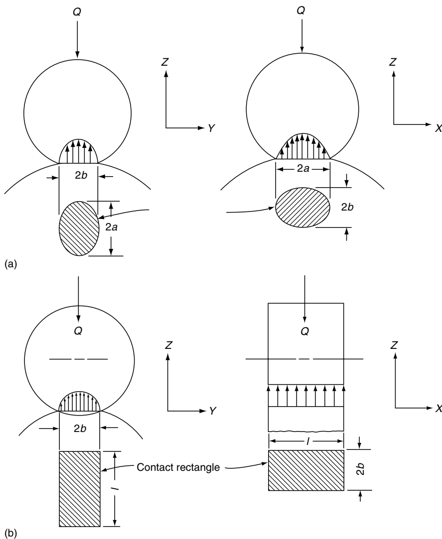
FIGURE 6.23 Surface compressive stress distribution. (a) Point contact; (b) ideal line contact.
