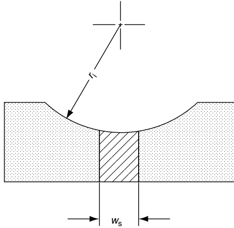
FIGURE 2.4 Inner rings of split inner-ring ball bearings showing shim for grinding.
