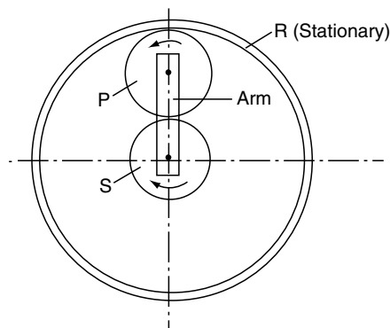
FIGURE 4.20 Schematic diagram of a simple epicyclic power transmission.
