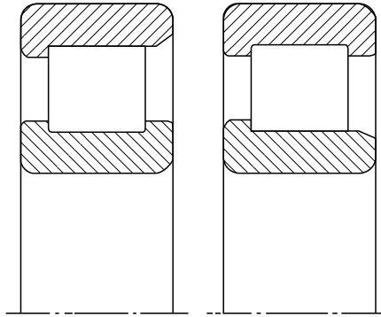
FIGURE 1.37 Cylindrical roller bearings with thrust flanges.
