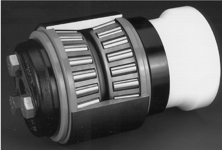
FIGURE 1.47 Sealed, greased, and preadjusted double-row tapered roller bearing for railroad wheel bearings. (Courtesy of the Timken Company.)
