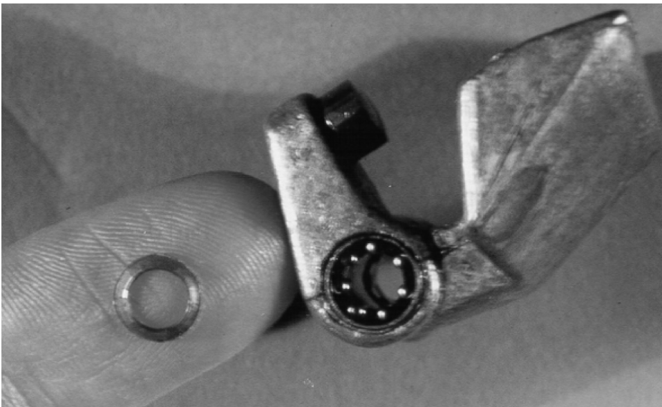
FIGURE 1.3 Miniature ball bearing. (Courtesy of SKF.)
