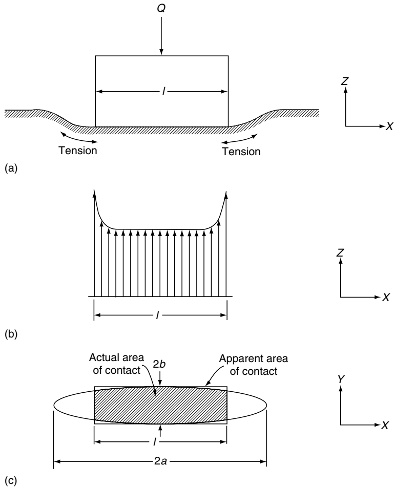
FIGURE 6.24 Line contact: (a) roller contacting a surface of infinite length; (b) roller–raceway compressive stress distribution; (c) contact ellipse.
