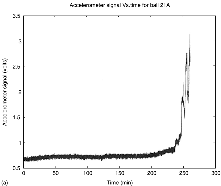
FIGURE 14.20 Accelerometer voltage signal for an AISI 52100 steel, 22.22-mm (0.875 in.) diameter ball, endurance tested at 45,000 rpm, and 37.8°C (100°F) lubricant supply temperature in a ball/v-ring test rig at (a) 3,170 MPa (460,000 psi) maximum Hertz stress.
