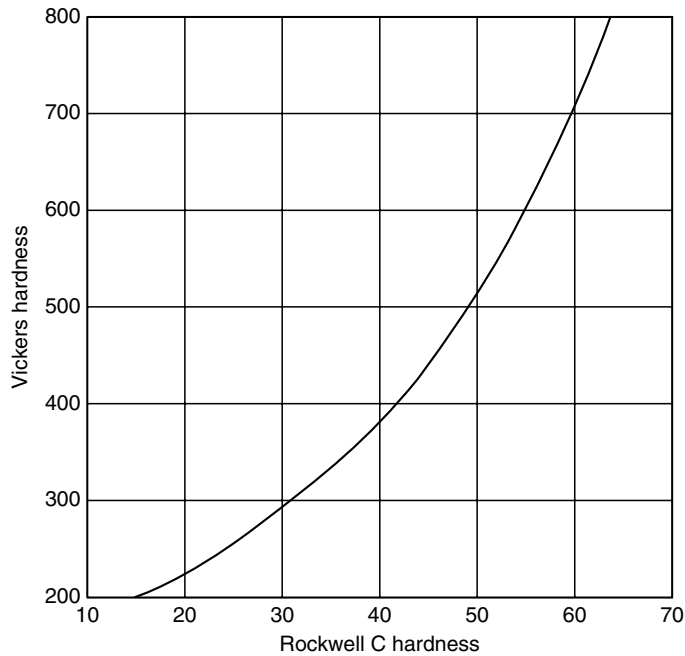
FIGURE 9.4 Vickers hardness vs. Rockwell C hardness.
