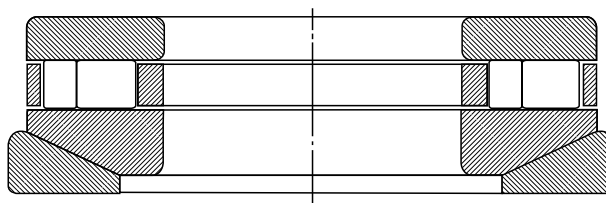
FIGURE 1.55 Cylindrical roller thrust bearing that has two rollers in each cage pocket; the bearing has a spherical seat for external alignment capability.
