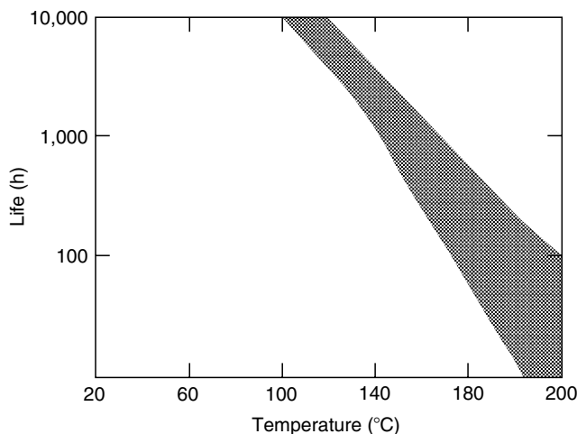
FIGURE 13.19 Life expectancy vs. operating temperature for nylon-6,6 with 25% glass-fiber fill. (From Lankamp, H., Materials for plastic cages in rolling bearings, Ball Bearing J. , SKF, 227, 14–18, August 1986. With permission.)
