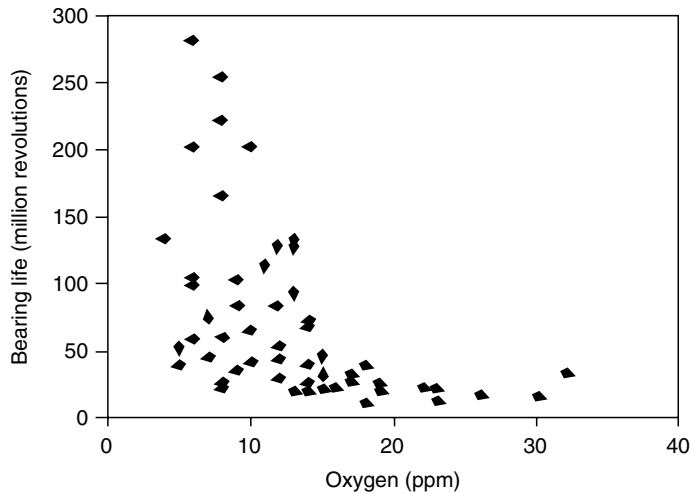
FIGURE 13.5 Fatigue life of carburized tapered roller bearings vs. oxygen content. (From Eckel, J., et al., Clean engineered steels—progress at the end of the twentieth century, in Advances in the Production and Use of Steel with Improved Internal Cleanliness , J. Mahoney (Ed.), ASTM STP 1361, 1999. With permission.)
