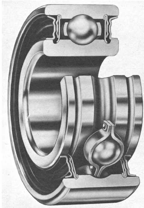
FIGURE 1.18 A single-row deep-groove ball bearing assembly with shields and seals. The shields are used to exclude large particles of foreign matter. (Courtesy of SKF.)
