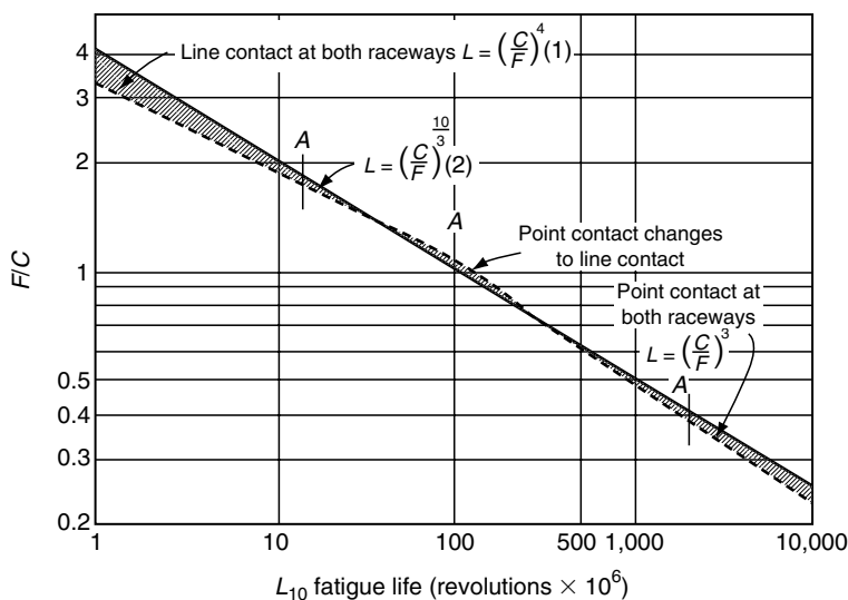
FIGURE 11.17 L_{10} vs. F/C for point or line contact at both raceways.
