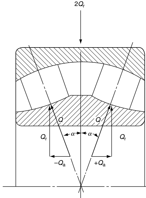
FIGURE 5.2 Radially loaded symmetrical rollers.
