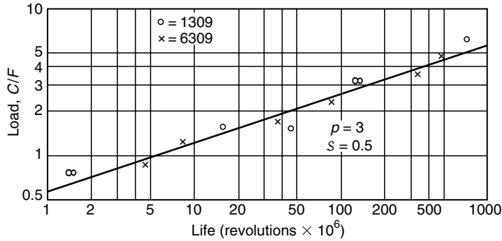
FIGURE 11.11 Load vs. life for ball bearings. (From Lundberg, G. and Palmgren, A., Dynamic capacity of rolling bearings, Acta Polytech. Mech. Eng. , Ser. 1, No. 3, 7, Royal Swedish Acad. Eng., 1947. Reprinted with permission.)
