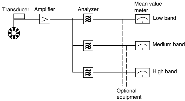
FIGURE 14.12 Schematic of bearing vibration measurements.
