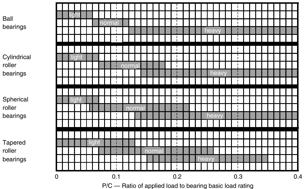
FIGURE 3.1 Classification of loading for ball, cylindrical roller, spherical roller, and tapered roller bearings used to determine required amount of press-fitting to prevent inner-ring rotation on the shaft “and/or” outer-ring rotation in the housing.
