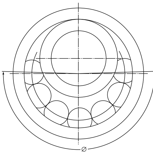
FIGURE 1.13 Diagram illustrating the method of assembly of a Conrad-type, deep-groove ball bearing.
