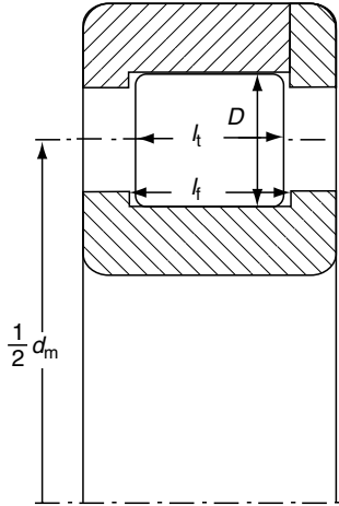
FIGURE 2.11 Schematic drawing of a radial cylindrical roller bearing having two integral roller guide flanges on the inner ring and one integral and one separable guide flange on the outer ring.
