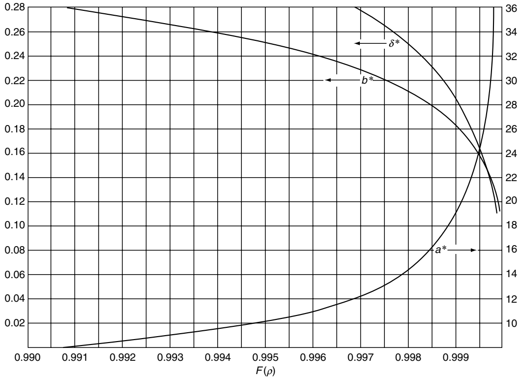
FIGURE 6.5 a^* , b^* , and \delta^* vs. F(\rho) .
