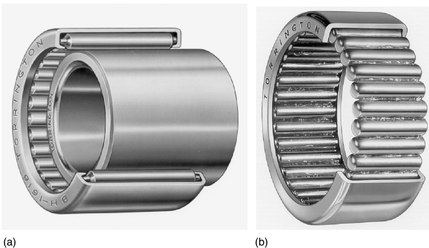
FIGURE 1.42 Full-complement needle roller bearings. (a) Drawn cup assembly with trunnion-end rollers and inner ring; (b) drawn cup assembly with rollers retained by grease pack. (Courtesy of the Timken Company.)
