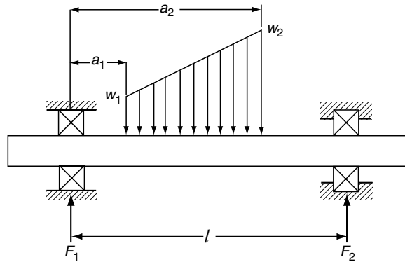
FIGURE 4.22 Simple two-bearing-shaft system, uniform continuous loading.
