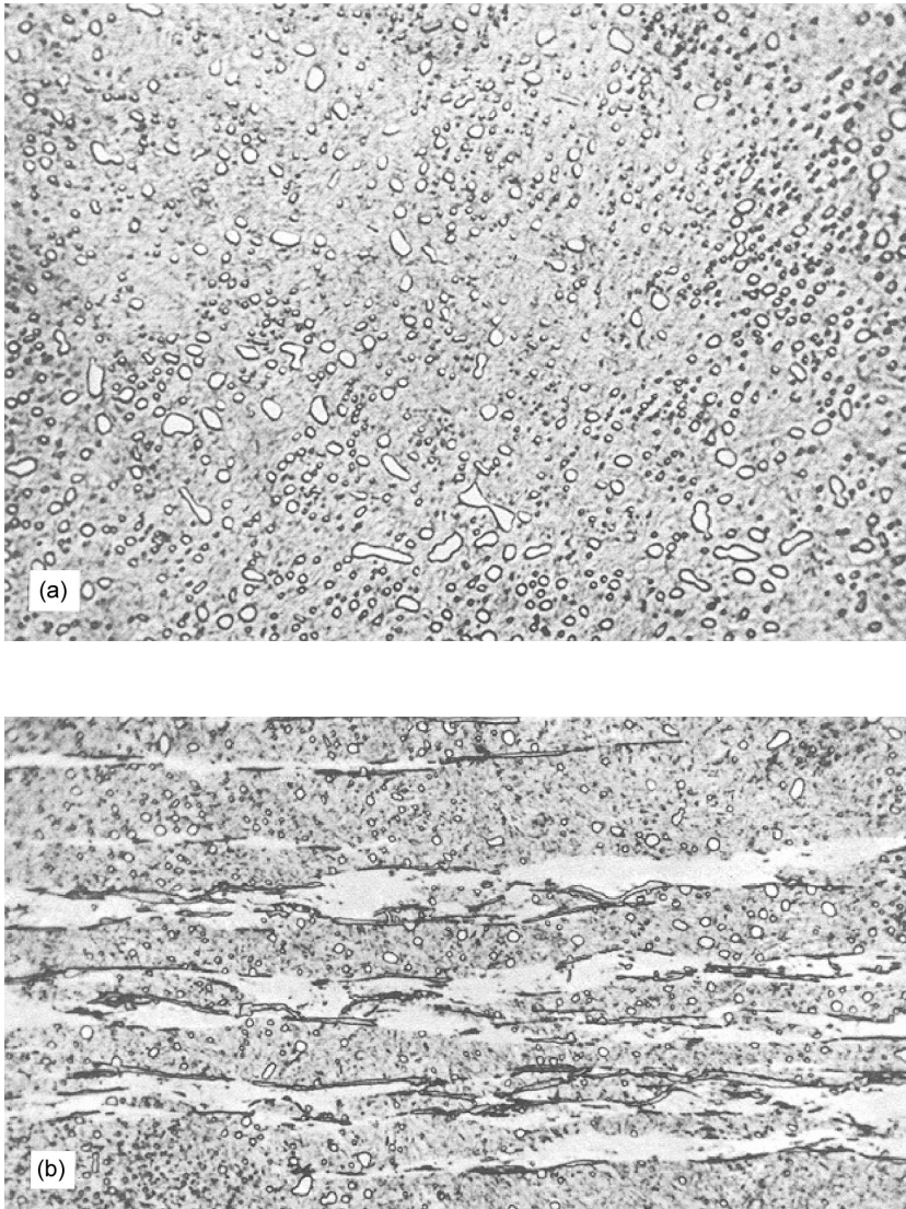
FIGURE 6.15 Subsurface metallurgical structure (1300 times magnification after picral etch) showing change due to repeated rolling under load. (a) Normal structure; (b) stress-cycled structure—white deformation bands and lenticular carbide formations are visible.
