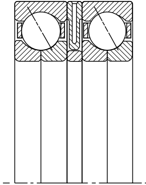
FIGURE 1.32 A tandem-mounted pair of split inner-ring ball bearings.
