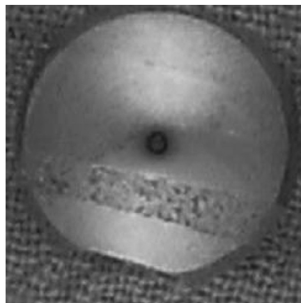
FIGURE 14.18 AISI 52100 steel, 22.22-mm (0.875 in.) diameter ball (a) showing initial spall after endurance testing at 45,000 rpm, 3,170 MPa (460,000 psi) maximum Hertz stress, and 71.1°C (160°F) lubricant supply temperature in a ball/v-ring test rig; (b) showing progression to 33% spalling over track; (c) showing progression to 100% spalling over track (From Kotzalas, M., Power transmission component failure and rolling contact fatigue progression, Ph.D. thesis in Mech. Eng., Pennsylvania State Univ., August 1999.)
