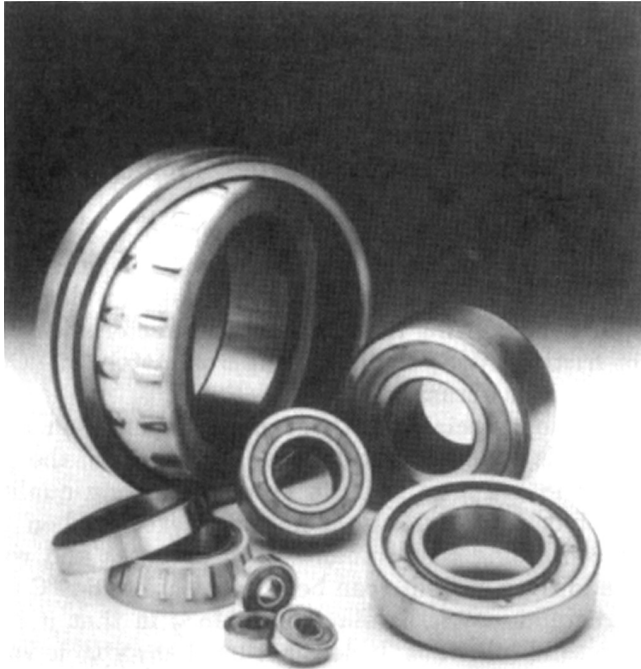
FIGURE 12.6 Polymeric-lubricated rolling bearings.
