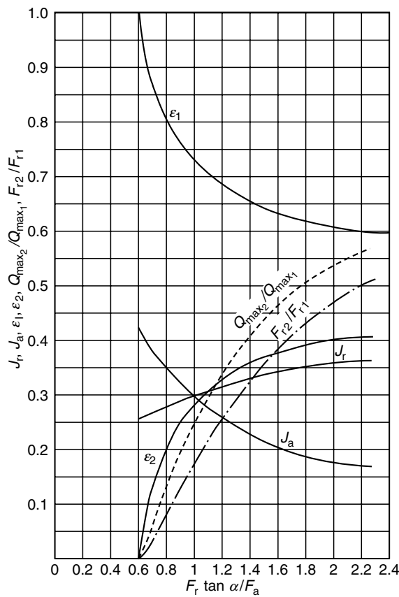
FIGURE 7.16 J_r , J_a , \varepsilon_1 , \varepsilon_2 , Q_{\max 2} / Q_{\max 1} , F_{r2} / F_{r1} vs. F_r \tan \alpha / F_a for double-row point-contact bearings.
