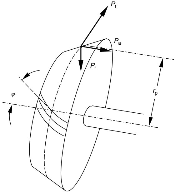
FIGURE 4.15 Loads transmitted by a spiral bevel gear.
