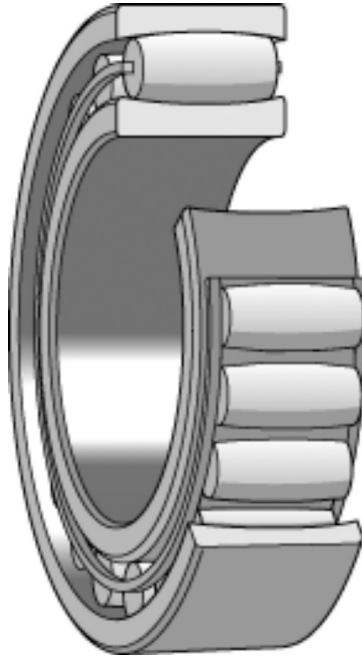
FIGURE 1.52 Single-row, radial, toroidal roller bearing. (Courtesy of SKF.)
