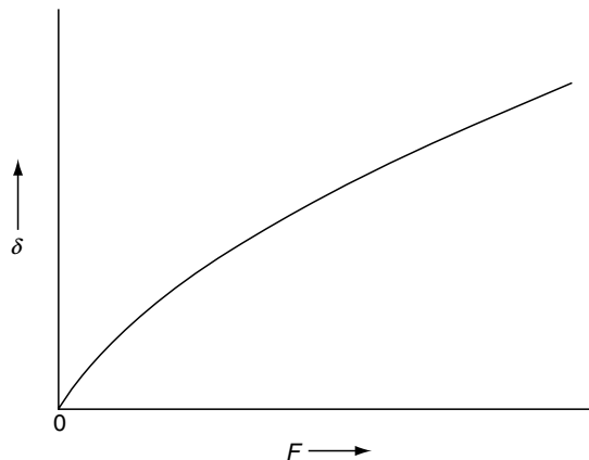
FIGURE 8.1 Deflection vs. load characteristic for ball bearings.
