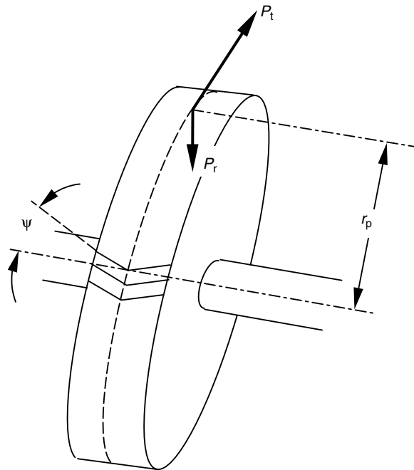
FIGURE 4.5 Loads transmitted by a herringbone gear; \psi is the helix angle.
