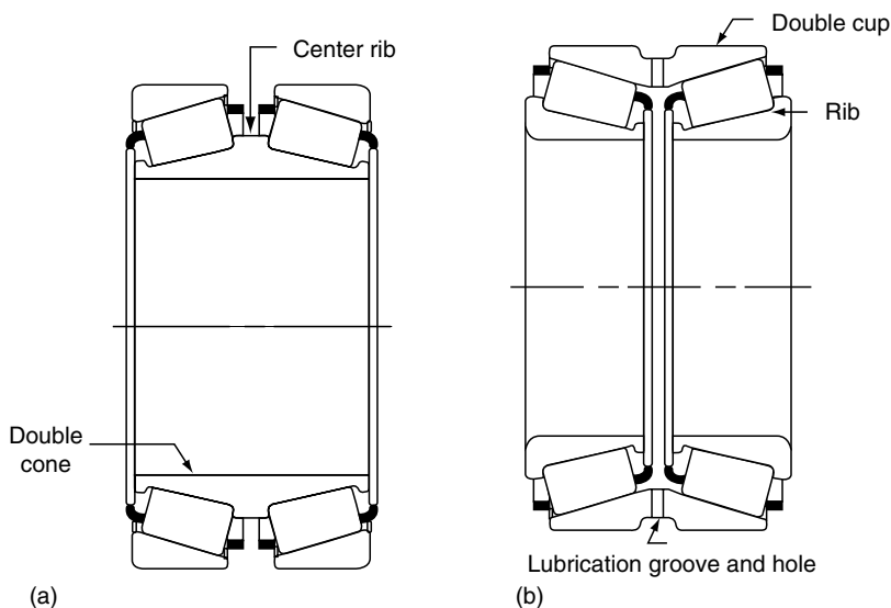
FIGURE 1.46 Double-row tapered rolling bearings. (a) Double cone assembly; (b) double cup assembly. (Courtesy of the Timken Company.)
