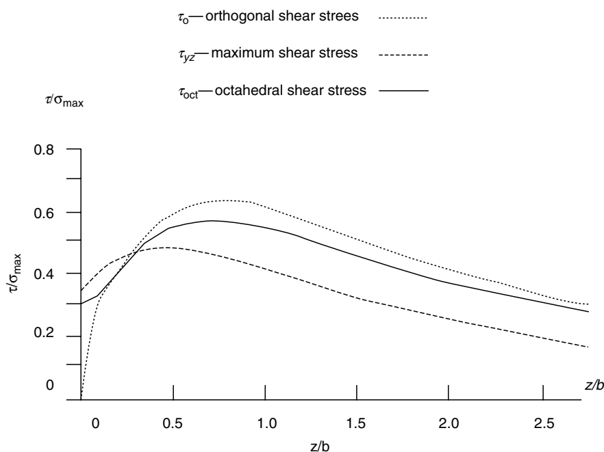
FIGURE 6.17 Comparison of shear stresses at depths beneath the contact surface ( x = y = 0 ).
