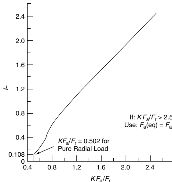
FIGURE 10.2 Values of f_t for radial loaded tapered roller bearings.
