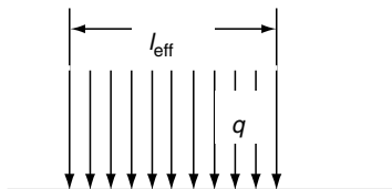
FIGURE 5.5 Uniform loading of cylindrical roller on inner raceway under applied radial load, ideal loading with straight profile rollers.
