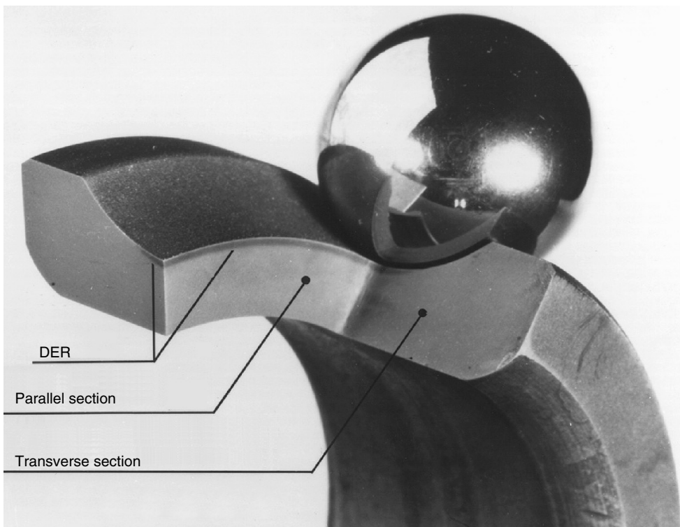
FIGURE 11.2 Orientation of viewing sections and location of region of microstructural alterations in a 309 deep-groove ball bearing inner ring. (From Swahn, H., Becker, P., and Vingsbo, O., Martensite decay during rolling contact fatigue in ball bearings, Metallurgical Trans. A , 7A, 1099–1110, August 1976. With permission.)
