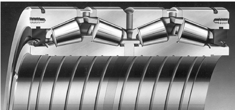
FIGURE 1.48 A four-row tapered roller bearing with integral seals for a hot strip mill application. (Courtesy of SKF.)
