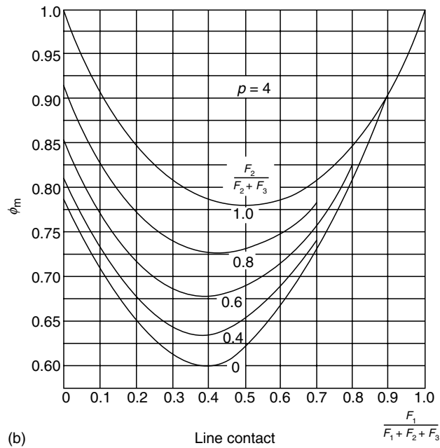
FIGURE 11.25 \phi_m vs. F_1/(F_1 + F_2 + F_3) for the generalized loading of Figure 11.24.
