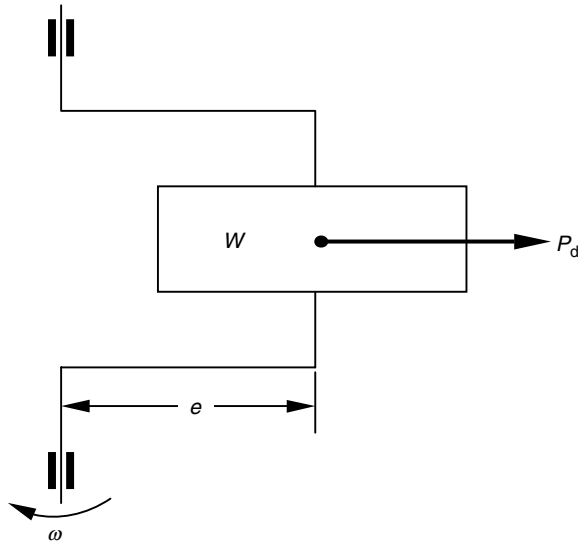
FIGURE 4.9 Rotor with eccentric mass.
