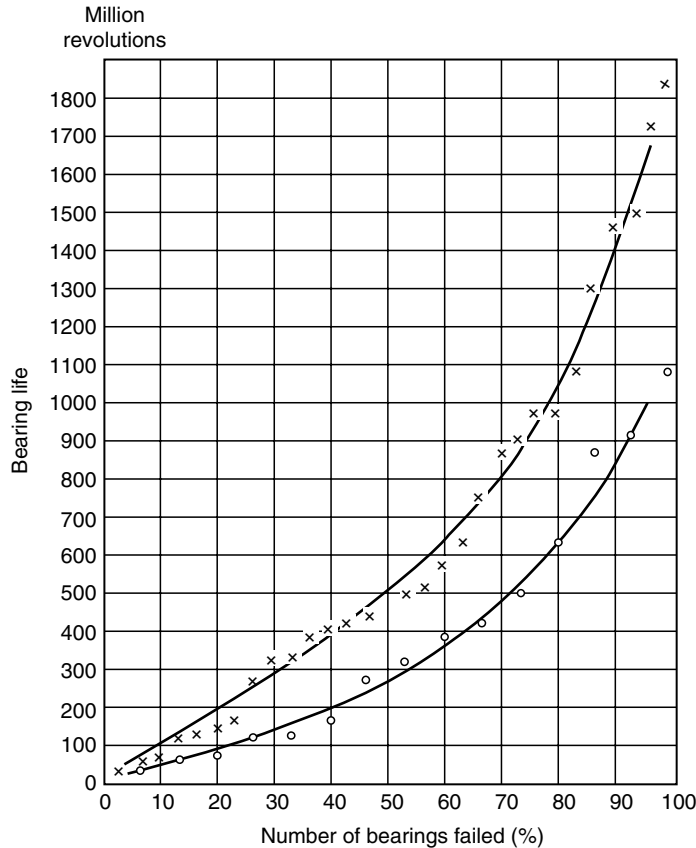
FIGURE 11.9 Fatigue life comparison of a single-row bearing to a two-row bearing. A group of single-row bearings programmed for fatigue testing was numbered by random selection, No. 1–30, inclusive. The resultant lives, plotted individually, give the upper curve. The lower curve results if bearing Nos. 1 and 2, Nos. 3 and 4, Nos. 5 and 6, and so on were considered two-row bearings and the shorter life of the two plotted as the life of a two-row bearing.
