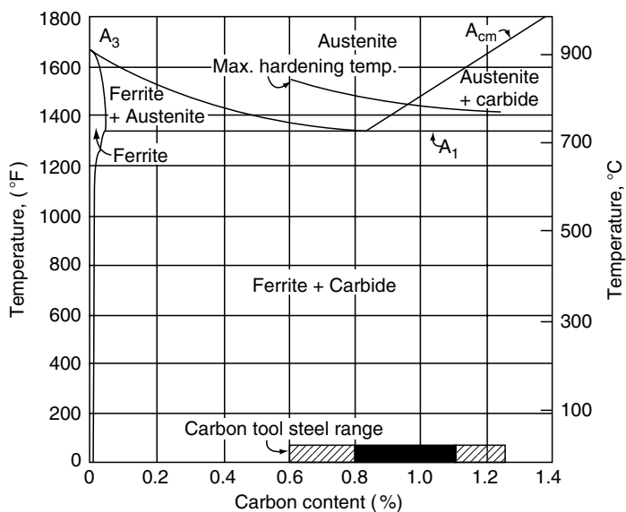
FIGURE 13.8 Section of the iron–carbon phase diagram.
