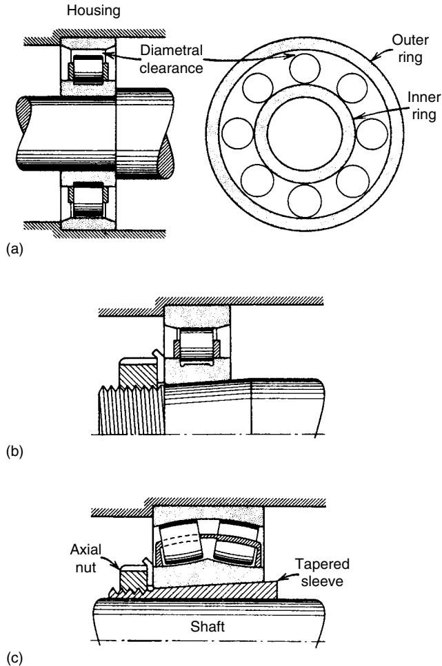
FIGURE 8.9 (a) Diametral (radial) clearance found in most off-the-shelf rolling bearings. One object of preloading is to remove this clearance during assembly. (b) Cylindrical roller bearing mounted on tapered shaft, to expand inner ring. Such bearings are usually made with a taper on the inner surface of \frac{1}{12} mm/mm. (c) Spherical roller bearing mounted on tapered sleeve to expand the inner ring.
