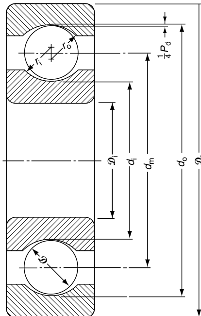
FIGURE 2.1 Radial ball bearing showing diametral clearance.
