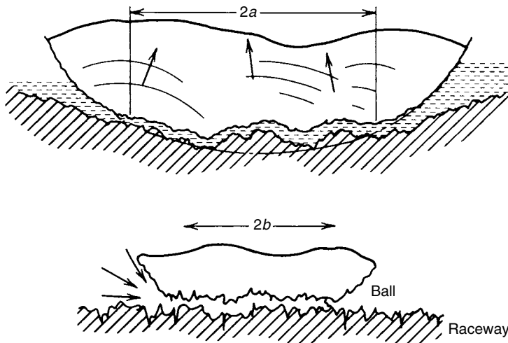
FIGURE 9.1 Ball and raceway contacting surfaces (greatly magnified). (From Sayles, R. and Poon, S., Surface topography and rolling element vibration, Precis. Eng. , 137–144, 1981.
