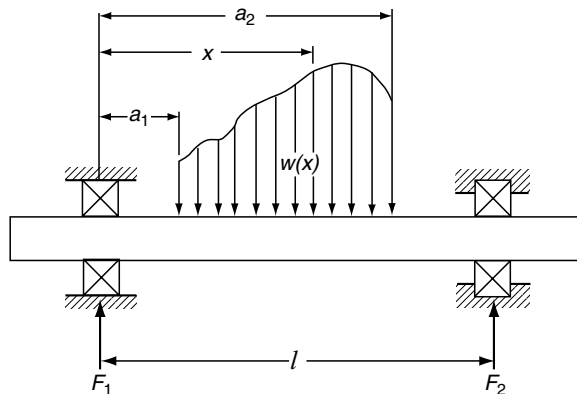
FIGURE 4.21 Simple two-bearing-shaft system, continuous loading.
