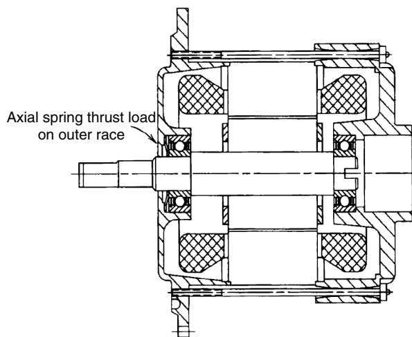
FIGURE 14.1 Schematic drawing of electric motor.
