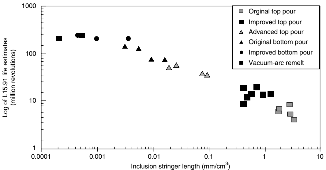
FIGURE 13.6 Fatigue life of carburized tapered roller bearings vs. ultrasonic inclusion stringer length. (From Eckel, J., et al., Clean engineered steels—progress at the end of the twentieth century, in Advances in the Production and Use of Steel with Improved Internal Cleanliness , J. Mahoney (Ed.), ASTM STP 1361, 1999. With permission.)
