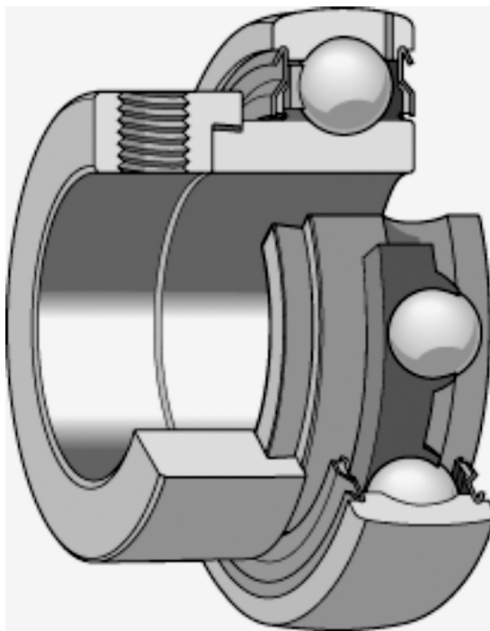
FIGURE 1.15 A single-row deep-groove ball bearing assembly that has a sphered outer surface to make it externally aligning. (Courtesy of SKF.)
