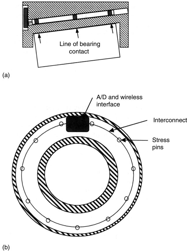
FIGURE 14.17 Stress pins inserted into the cup of a tapered roller bearing: (a) locations to determine axial stress distribution; (b) circumferential locations to determine distribution of load among the rollers—showing wireless connection of analog/digital converter for transmission of signal. (Courtesy of Oceana Sensor Technologies, Virginia Beach, Virginia.)
