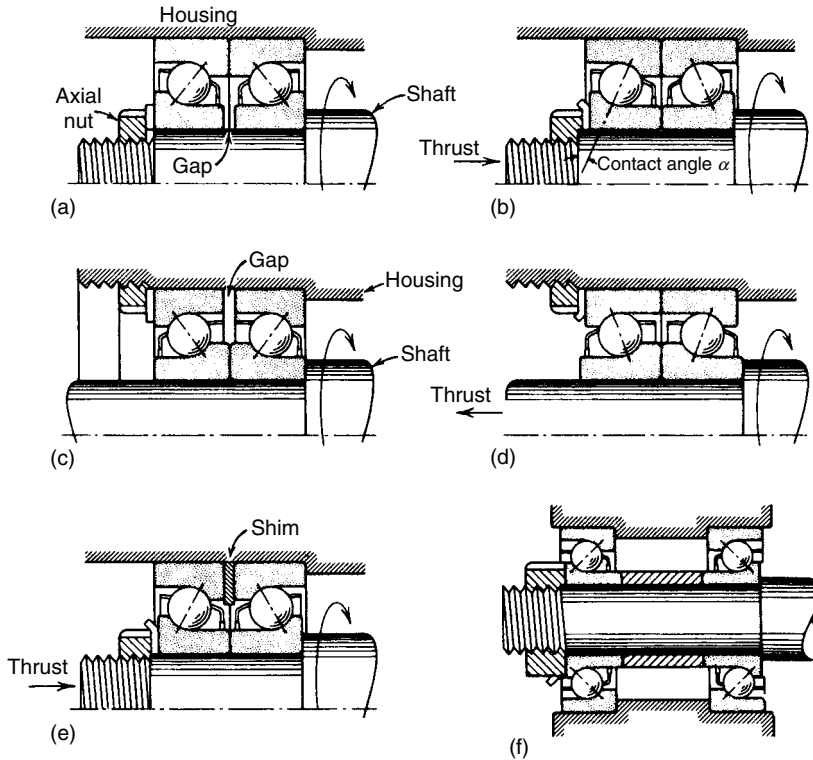
FIGURE 8.3 (a) Duplex set with back-to-back angular-contact ball bearings before axial preloading. The inner-ring faces are ground to provide a specific axial gap. (b) Same unit as in (a) after tightening axial nut to remove gap. The contact angles have increased. (c) Face-to-face angular-contact duplex set before preloading. In this case it is the outer-ring faces that are ground to provide the required gap. (d) Same set as in (c) after tightening the axial nut. The convergent contact angles increase under preloading. (e) Shim between two standard-width bearings avoids need for grinding the faces of the outer rings. (f) Precision spacers in between automatically provide proper preload by making the inner spacer slightly shorter than the outer.
