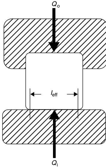
FIGURE 5.4 Cylindrical roller–raceway loading under simple applied radial load.
