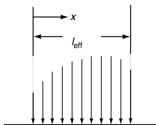
FIGURE 5.7 Loading of cylindrical roller on inner raceway under applied combined radial and axial loads, loading with crowned profile rollers.
