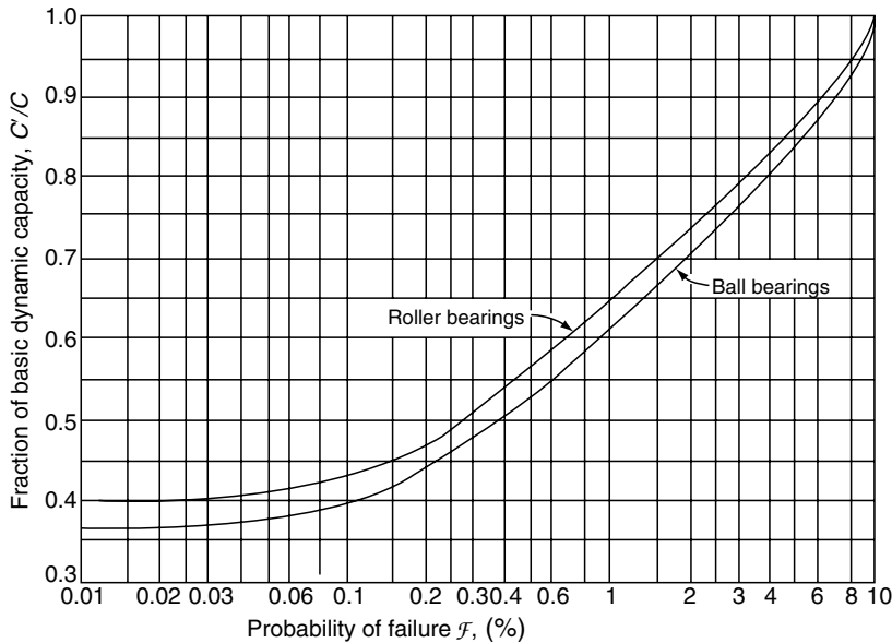
FIGURE 11.32 Reduction in basic dynamic capacity required for increased reliability. (From Harris, T., Predicting bearing reliability, Mach. Des. , 129–132, January 3, 1963.)
