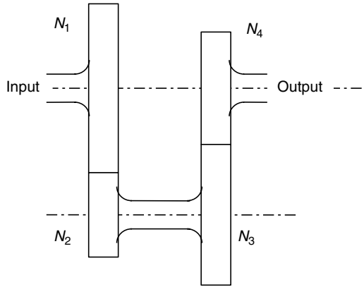
FIGURE 4.19 Simple four-gear train.
