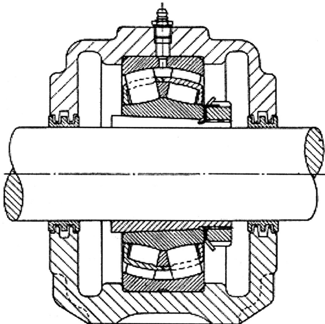
FIGURE 12.7 Bearing housing with labyrinth seals.
