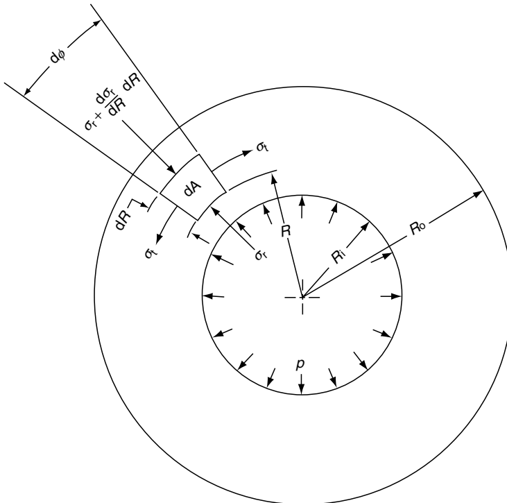
FIGURE 3.3 Thick ring loaded by internal pressure p .
