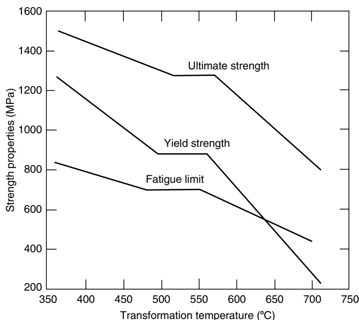
FIGURE 13.13 Properties of a 0.8% C steel vs. transformation temperature.
