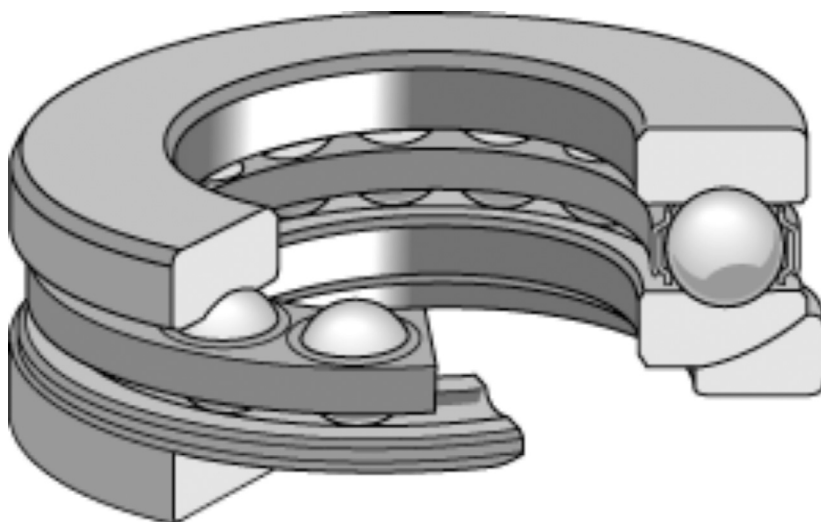
FIGURE 1.34 A 90° contact-angle thrust ball bearing with a spherical seat to make it externally aligning. (Courtesy of SKF.)
