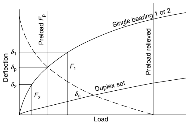
FIGURE 8.6 Deflection vs. load for a preloaded duplex set of ball bearings.
