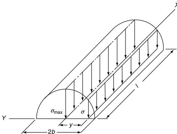
FIGURE 6.7 Semicylindrical surface compressive stress distribution of ideal line contact.
