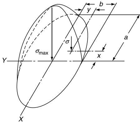
FIGURE 6.6 Ellipsoidal surface compressive stress distribution of point contact.
