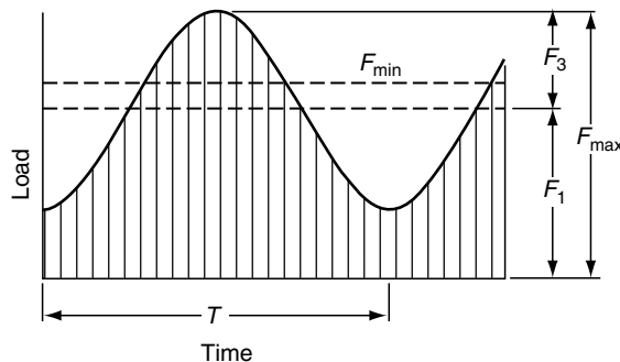
FIGURE 11.20 Sinusoidal load F_3 superimposed on a steady load F_1 .
