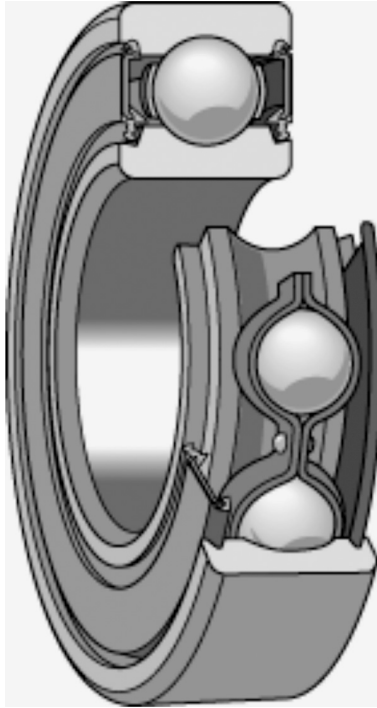
FIGURE 1.16 A single-row deep-groove ball bearing that has two seals to retain lubricant (grease) and prevent ingress of dirt into the bearing. (Courtesy of SKF.)
