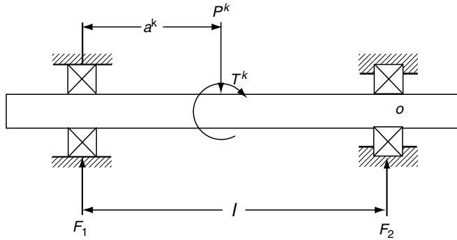
FIGURE 4.12 Two-bearing-shaft system with concentrated radial and moment loads.
