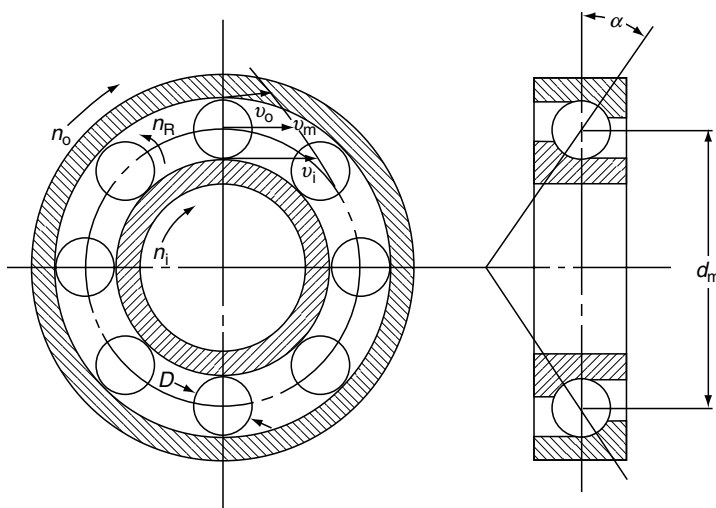
FIGURE 10.1 Rolling speeds and velocities in a bearing.
