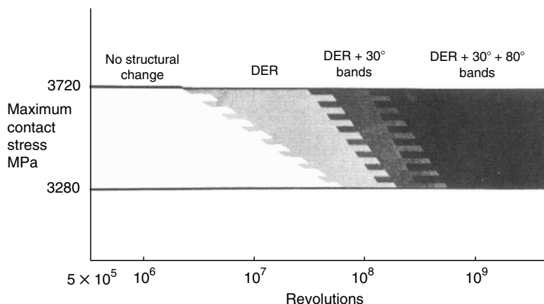
FIGURE 11.3 Microstructural alterations as a function of stress level and number of inner-ring revolutions. (From Swahn, H., Becker, P., and Vingsbo, O., Martensite decay during rolling contact fatigue in ball bearings, Metallurgical Trans. A , 7A, 1099–1110, August 1976. With permission.)
