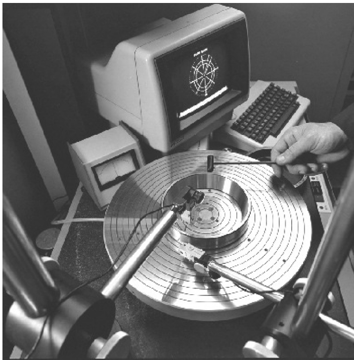
FIGURE 14.10 Bearing component waviness tester. (Courtesy of Timken Company.)
