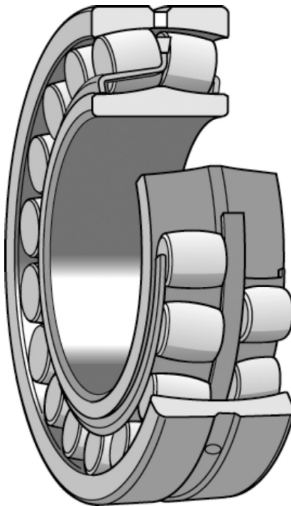
FIGURE 1.50 Cutaway view of a double-row spherical roller bearing with symmetrical rollers and a floating guide flange. (Courtesy of SKF.)
