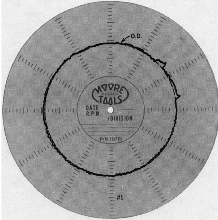
FIGURE 14.9 Low-amplitude, high-frequency waviness.
