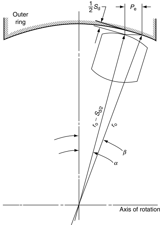
FIGURE 2.9 Schematic diagram of spherical roller bearing showing nominal contact angle \alpha , dimetral play S_d , and endplay P_e .
