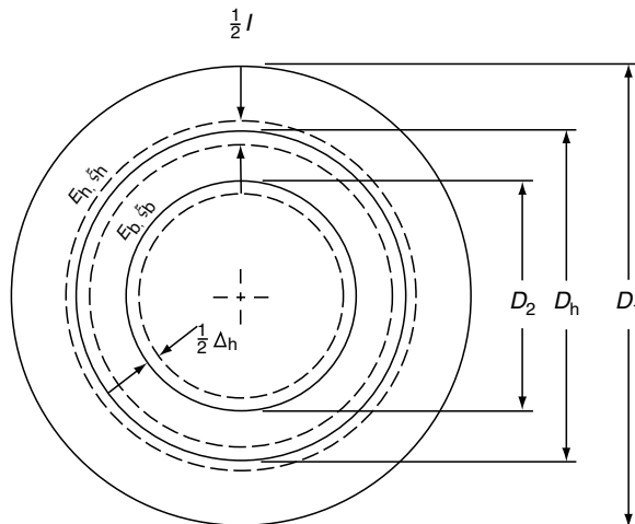
FIGURE 3.5 Schematic diagram of a bearing outer ring mounted in a housing.
