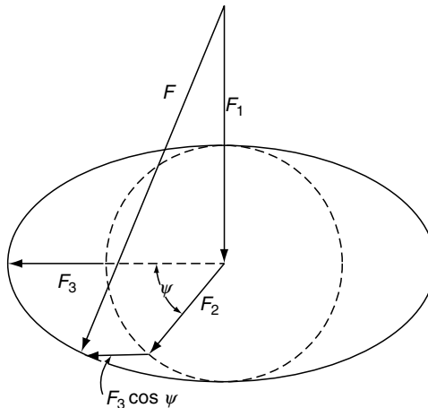
FIGURE 11.24 Load vector diagram for generalized bearing loading consisting of steady load F_1 , rotating load F_2 , and sinusoidal load F_3 , 90^\circ out-of-phase with F_1 .
