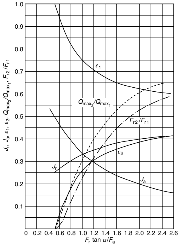
FIGURE 7.17 J_r , J_a , \epsilon_1 , \epsilon_2 , Q_{\max_2}/Q_{\max_1} , F_{r2}/F_{r1} vs. F_r \tan \alpha / F_a for double-row line-contact bearings.
