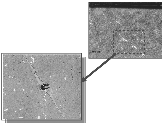
FIGURE 11.7 Subsurface “butterfly” in M50 steel ring, shown at 45° orientation to the rolling contact surface. The surface friction force is directed to the left. (From Nélías, D., Contribution a L’étude des Roulements, Dossier d’Habilitation a Diriger des Recherches, Laboratoire de Mécanique des Contacts, UMR-CNRS-INSA de Lyon No. 5514, December 16, 1999. With permission.)
