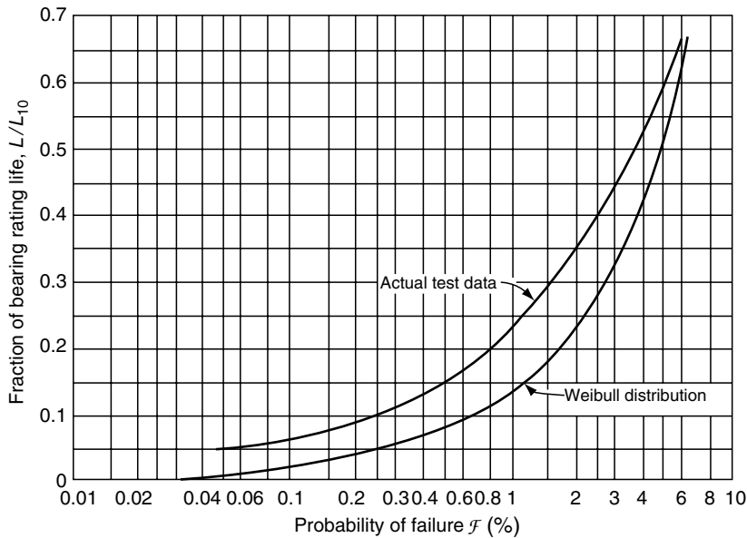
FIGURE 11.31 Fraction L_{10} life vs. probability of failure.
