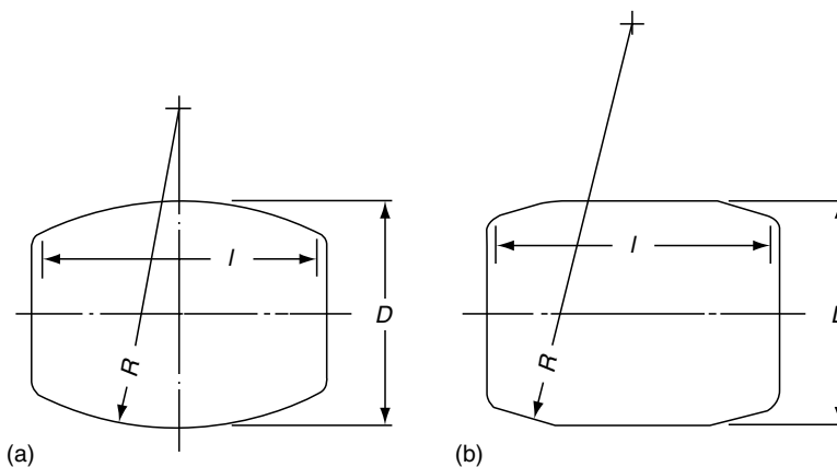
FIGURE 1.38 (a) Spherical roller (fully crowned); (b) partially crowned cylindrical roller (crown radius is greatly exaggerated for clarity).
