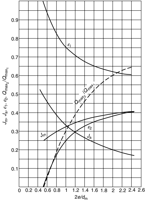
FIGURE 7.12 J_m , J_a , \varepsilon_1 , \varepsilon_2 , Q_{\max_2}/Q_{\max_1} vs. 2e/d_m for double-row line-contact thrust bearings.
