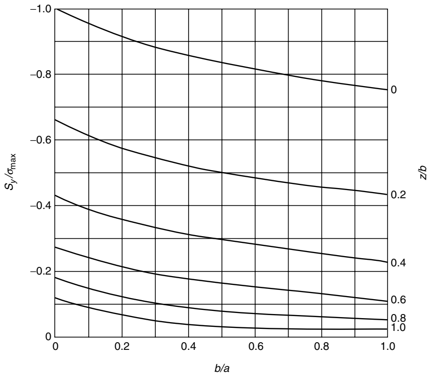
FIGURE 6.10 S_y/\sigma_{\max} vs. b/a and z/b .
