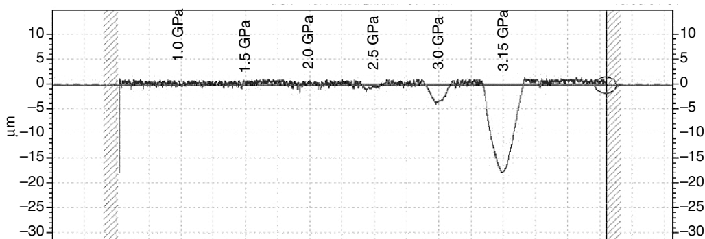
FIGURE 13.21 Steel disk wear marks after ball-on-disk testing with a WC/aC:H coated ball for 15 min in a 75W-90 oil with 10 m/s (32.8 ft/s) rolling and 5 m/s (16.4 ft/s) sliding speed.
