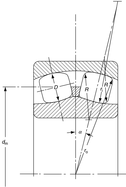
FIGURE 2.10 Spherical roller bearing geometry.
