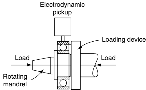
FIGURE 14.6 Schematic view of VKL vibration tester. (From Yhland, E., Waviness measurement—an instrument for quality control in rolling bearing industry, Proc. Inst. Mech. Eng. , 182, Pt. 3K, 438–445, 1967–1968.)
