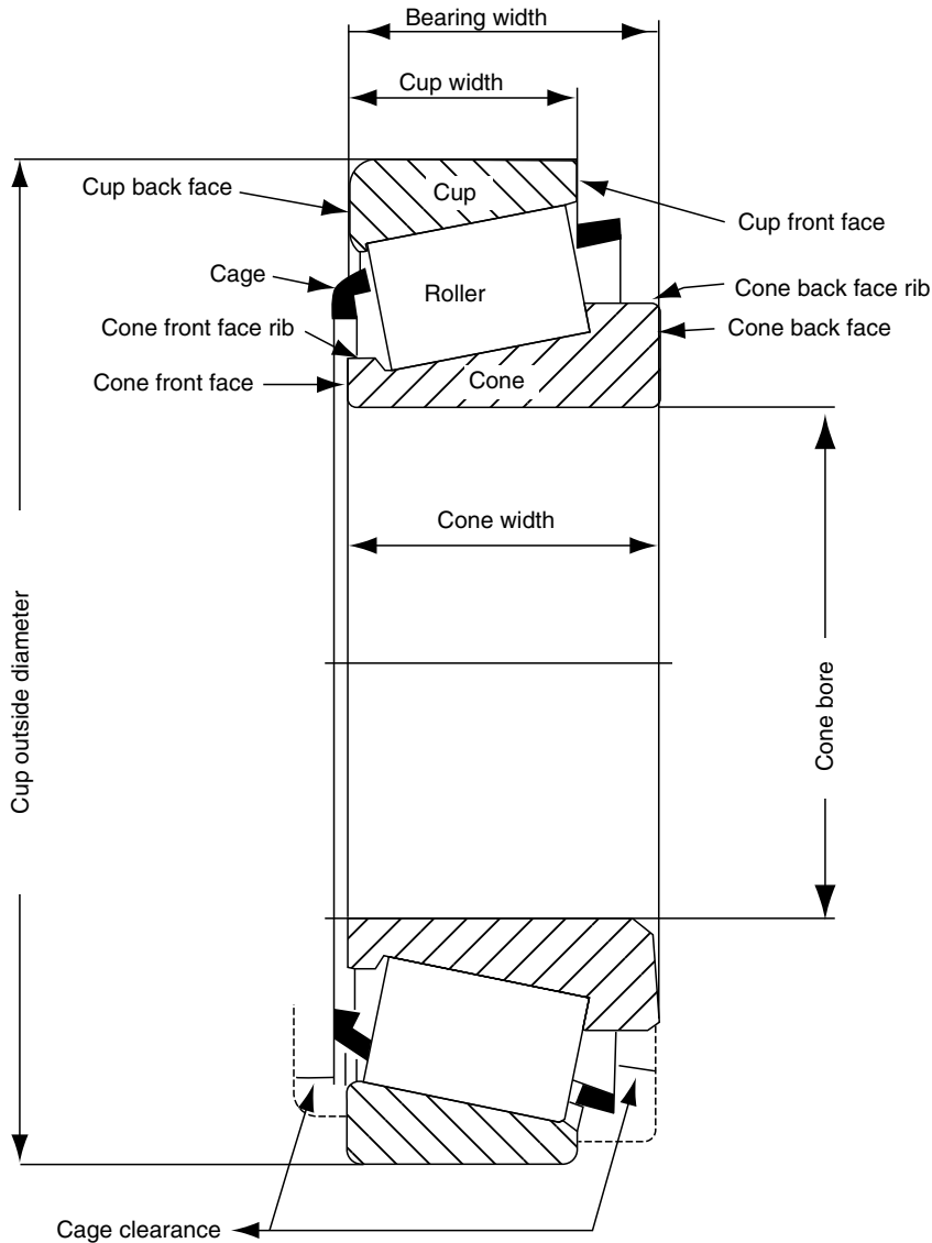
FIGURE 2.12 Schematic drawing of tapered roller bearing indicating nomenclature.
