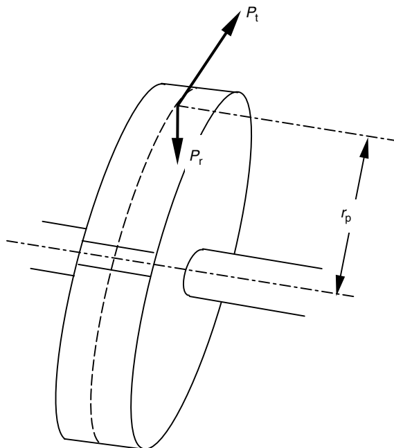
FIGURE 4.4 Loads transmitted by a spur gear.
