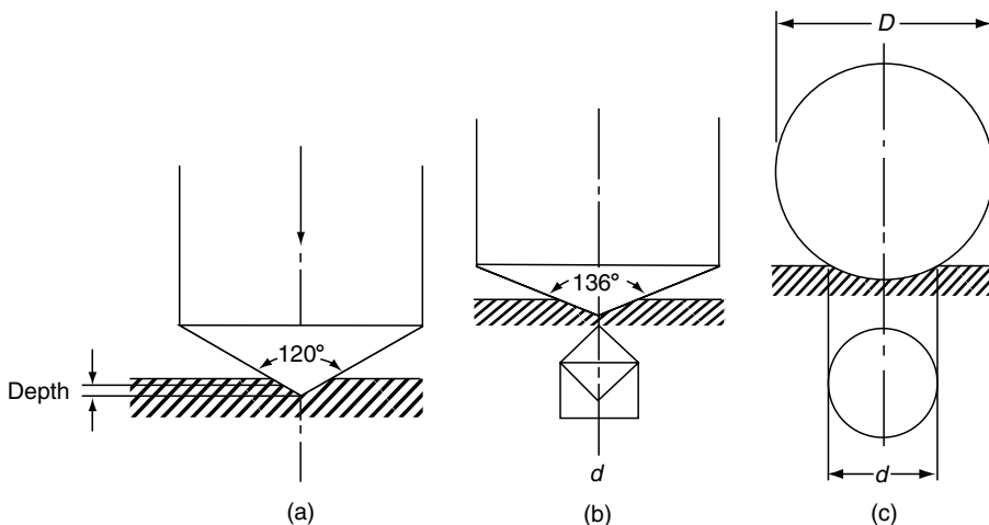
FIGURE 13.14 Hardness tests. (a) Rockwell R_C ; indentation body: diamond cone, load 150 kgf (including 10 kgf preload), indentation depth for R_C 63: 74 \mu\text{m} , hardness testing range: R_C 20–67. (b) Vickers; indentation body: diamond pyramid 136°, indentation depth: 1/7d —for V 782 \approx R_C : 22 \mu\text{m} , hardness testing range: up to V 2000. (c) Brinell; indentation body: hardened steel ball ( D ), hard metal ball ( D ), indentation depth: 1/5d , Hardness testing range: up to 400 B ( \sim 42.5 R_C ), up to 600 B ( \sim 57 R_C ).
