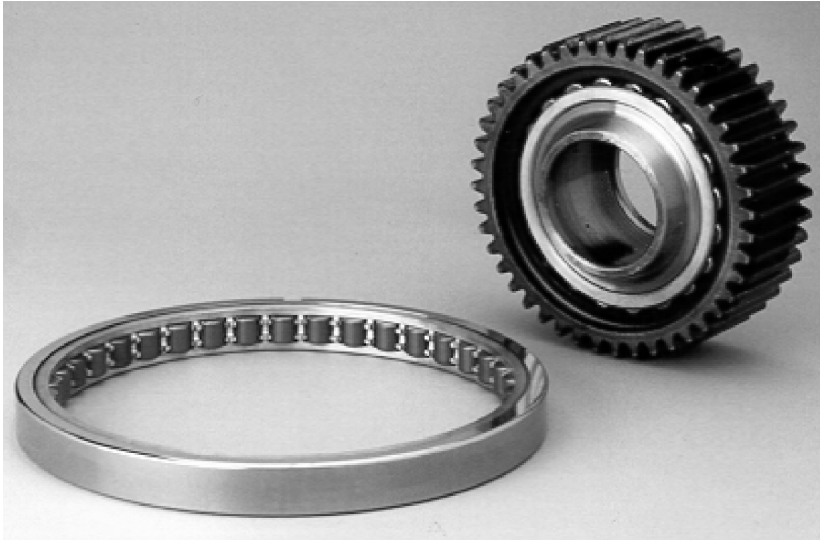
FIGURE 1.66 Aircraft power transmission bearings: (left) cylindrical roller bearing; (right) spherical planet gear bearing. (Courtesy of NTN.)
