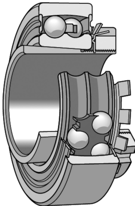
FIGURE 1.29 A double-row internally self-aligning ball bearing assembly with a tapered sleeve and locknut adapter for simplified mounting on a shaft of uniform diameter. (Courtesy of SKF.)
