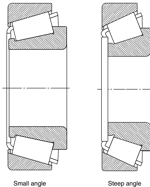
FIGURE 1.44 Small and steep contact angle tapered roller bearings.
