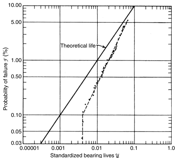
FIGURE 11.30 Life distribution in the early failure region. (From Tallian, T., Weibull distribution of rolling contact fatigue life and deviations there from, ASLE Trans. , 5(1), April 1962.)
