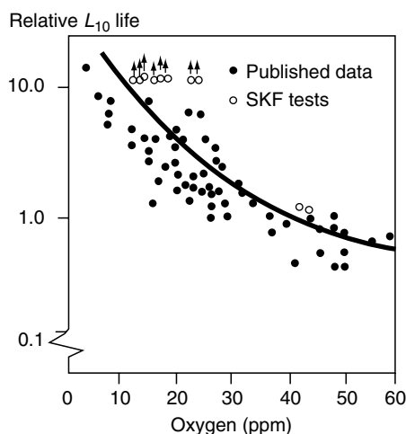
FIGURE 13.4 Fatigue life of AISI 52100 steel ball bearings vs oxygen content. (From Åkesson, J. and Lund, T., SKF rolling bearing steels—properties and processes, Ball Bearing J. , 217, 32–44, 1983. With permission.)
