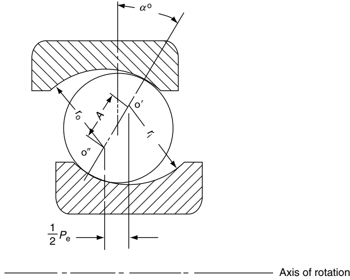
FIGURE 2.2 Radial ball bearing showing ball–raceway contact due to axial shift of inner and outer rings.
