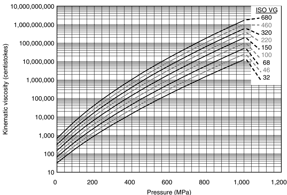
FIGURE 12.1 Variation of lubricant viscosity with pressure for various mineral oils.
