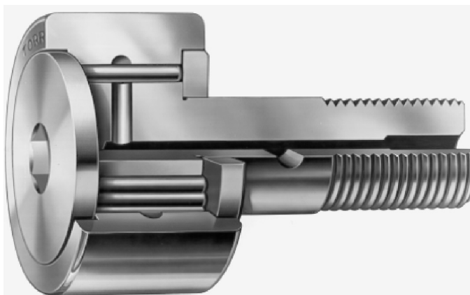
FIGURE 1.65 Needle roller cam follower assembly. (Courtesy of the Timken Company.)
