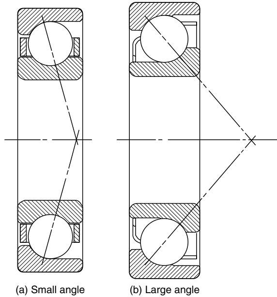
FIGURE 1.24 Angular-contact ball bearings.
