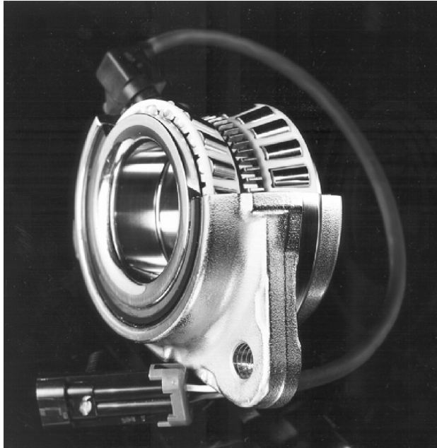
FIGURE 1.64 Self-contained, tapered roller bearing with an integral speed sensor to provide signal to the antilock braking system. (Courtesy of the Timken Company.)
