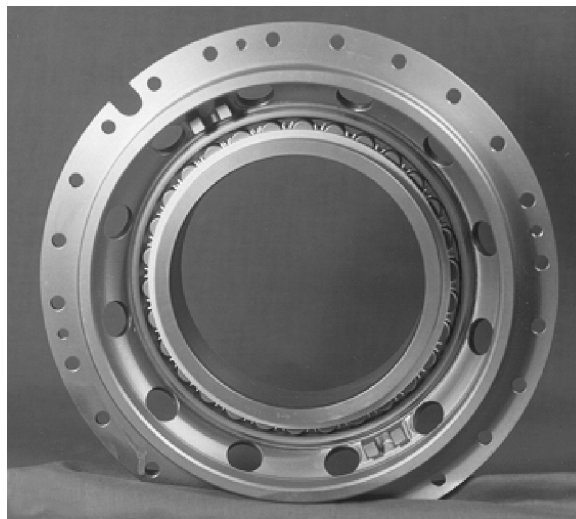
FIGURE 1.67 Aircraft gas turbine engine, cylindrical roller bearing. (Courtesy of SKF.)
