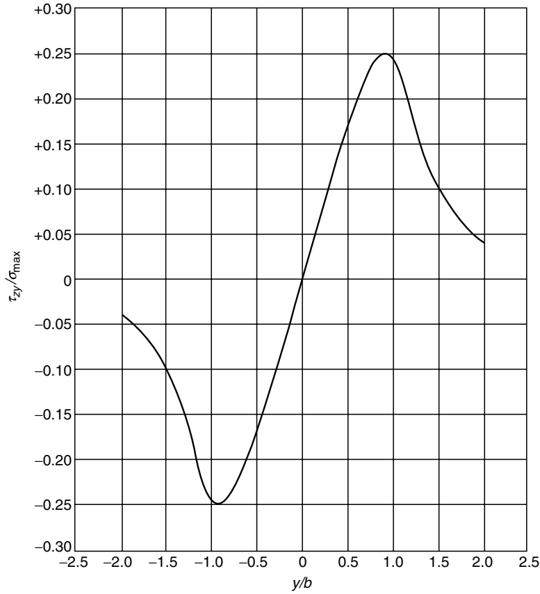
FIGURE 6.13 \tau_{zy}/\sigma_{max} vs. y/b for b/a = 0 and z = z_0 (concentrated normal load).
