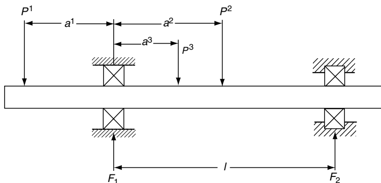
FIGURE 4.3 Two-bearing-shaft system, multiple loading.
