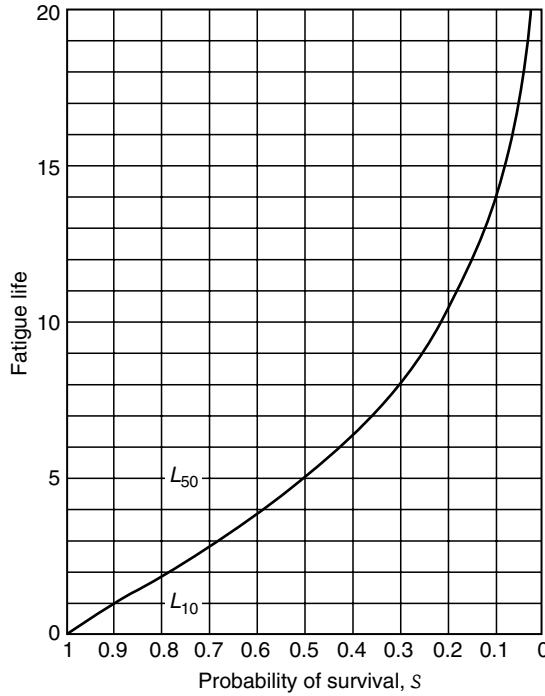
FIGURE 11.8 Rolling bearing fatigue life distribution.
