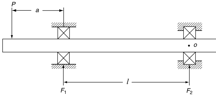
FIGURE 4.2 Two-bearing-shaft system, overhung load.
