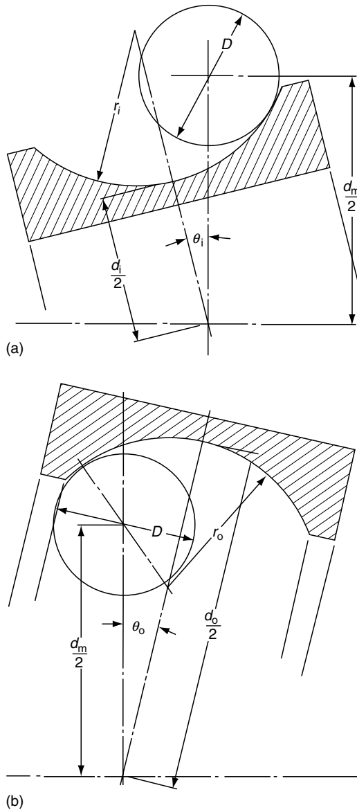
FIGURE 2.6 (a) Free misalignment of inner ring of single-row ball bearing and (b) free misalignment of outer ring of single-row ball bearing.
