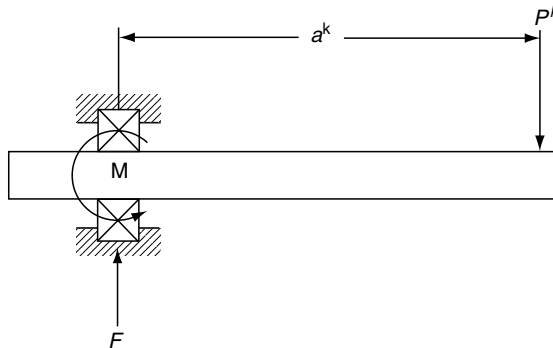
FIGURE 4.11 Single-bearing-shaft system.
