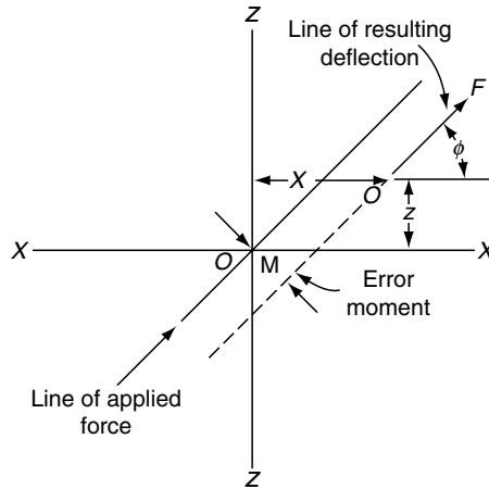
FIGURE 8.10 Effect of disturbing force F on the center of gravity of spring mass. It is frequently desirable to obtain isoelasticity in bearings in which the displacement in any direction is in line with the disturbing force.
