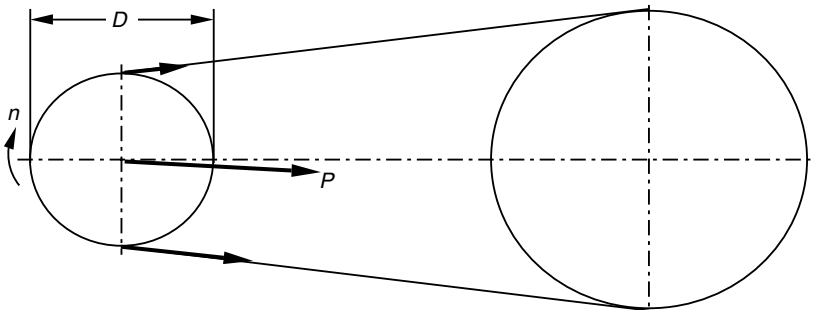
FIGURE 4.7 Belt-and-pulley arrangement.
