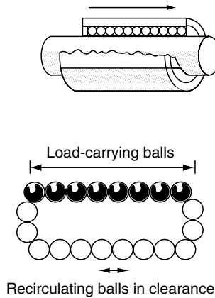
FIGURE 1.59 Schematic illustration of a ball bushing.
