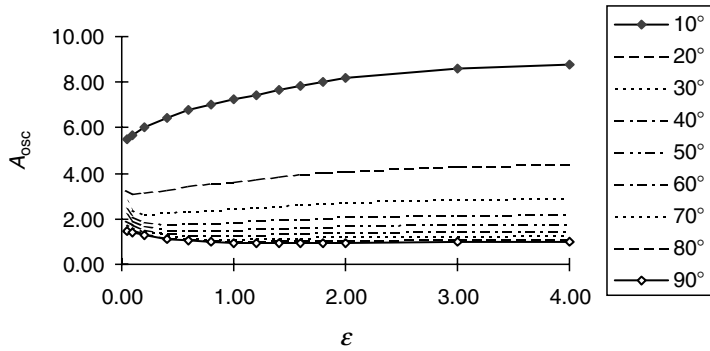
FIGURE 11.28 A_{osc} vs. load zone extent and 10–90° oscillation angles.
