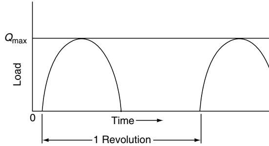
FIGURE 11.13 Typical load cycle for a point on the inner raceway of a radial bearing.
