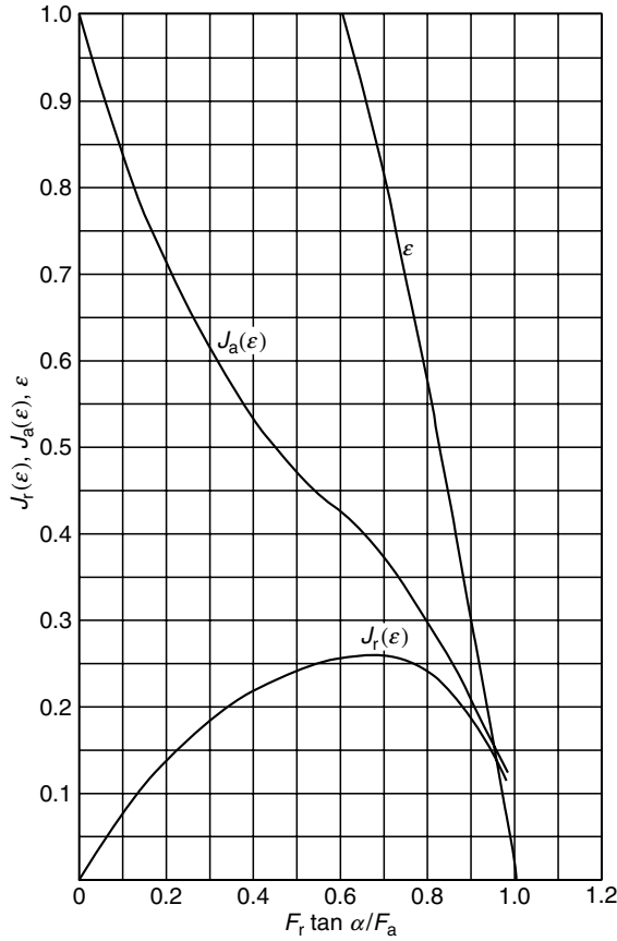
FIGURE 7.14 J_r(\varepsilon) , J_a(\varepsilon) , \varepsilon vs. F_r \tan \alpha / F_a for point-contact bearings.
