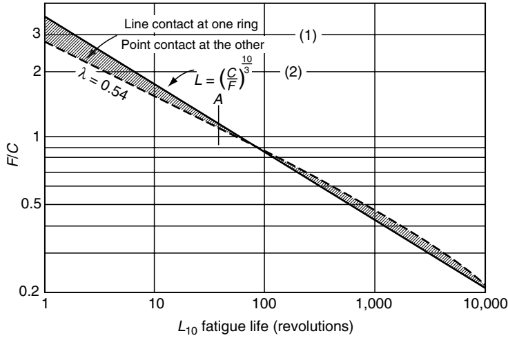
FIGURE 11.18 L_{10} vs. F/C for combination of line and point contact. (From Voskamp, A., Material response to rolling contact loading, ASME Trans., J. Tribol. , 107, 359–366, 1985. Reprinted with permission.)
