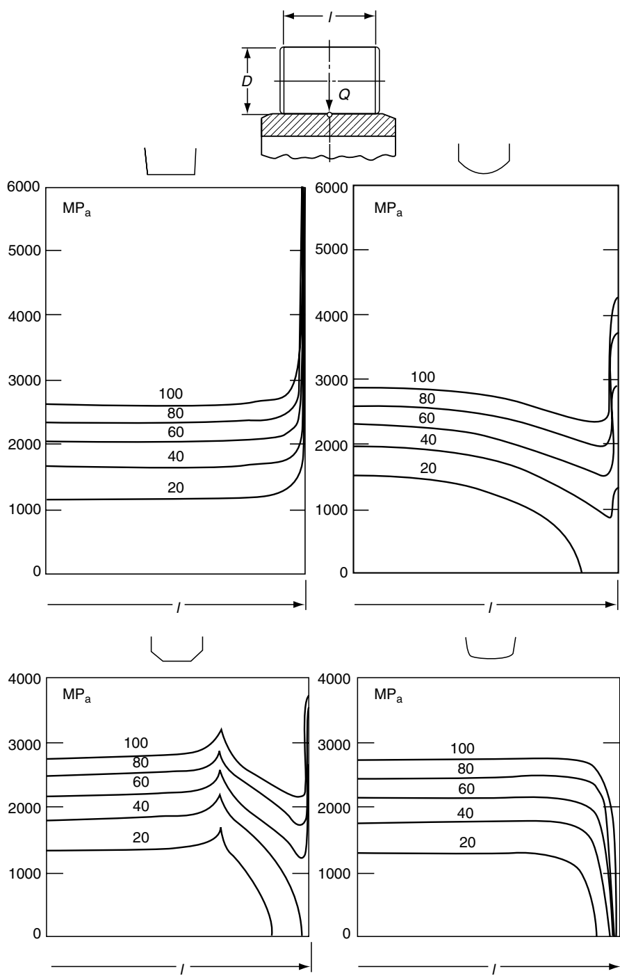
FIGURE 6.27 Compressive stress vs. length and specific roller load ( Q/D ) for various roller (or raceway) profiles. (From Reusner, H., Ball Bearing J. , 230, SKF, June 1987. With permission.)
