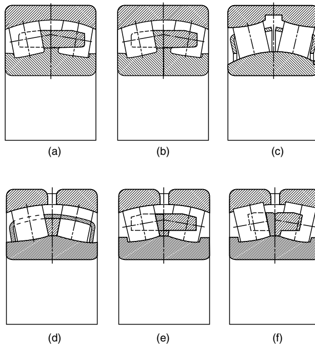
FIGURE 1.51 Various executions of double-row spherical roller bearings.
