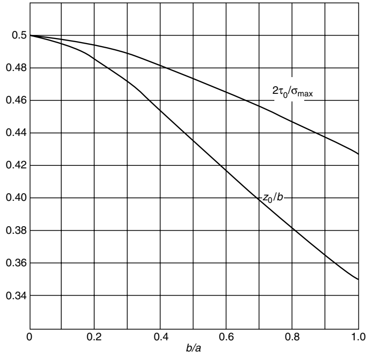
FIGURE 6.14 2\tau_0/\sigma_{\max} and z_0/b vs. b/a (concentrated normal load).
