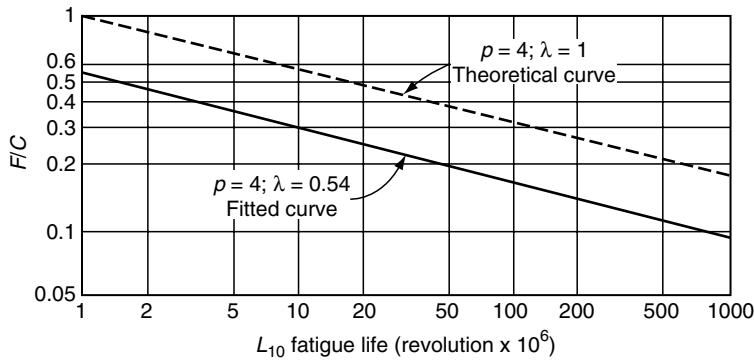
FIGURE 11.15 L_{10} vs. F/C for roller bearing. Test points are for an SKF 21309 spherical roller bearing. (From Lundberg, G. and Palmgren, A., Dynamic capacity of roller bearings, Acta Polytech. Mech. Eng. , Ser. 2, No. 4, 96, Royal Swedish Acad. Eng., 1952.)
