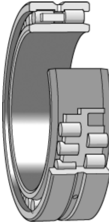
FIGURE 1.39 A double-row cylindrical roller bearing for precision machine tool spindle applications. (Courtesy of SKF.)
