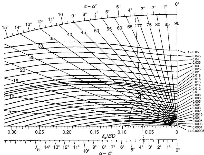
FIGURE 7.6 \delta_a/BD and \alpha - \alpha^\circ vs. t = F_a/ZD^2K and \alpha^\circ .
