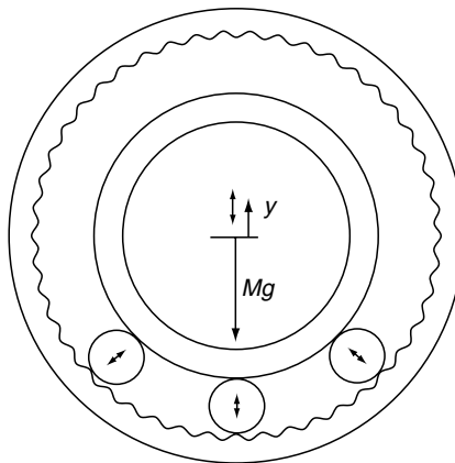
FIGURE 14.4 Vibration from raceway waviness. (Courtesy of Oceana Sensor Technologies, Virginia Beach, Virginia.)
