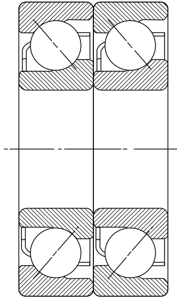
FIGURE 1.26 A tandem-mounted pair of angular-contact ball bearings.
