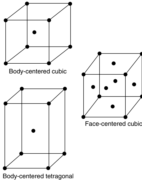
FIGURE 13.7 Crystal structures of steel.
