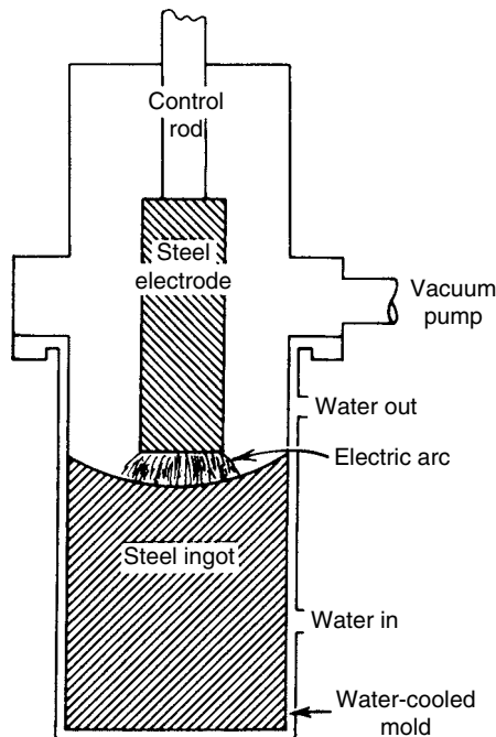
FIGURE 13.3 Vacuum-arc remelting furnace.
