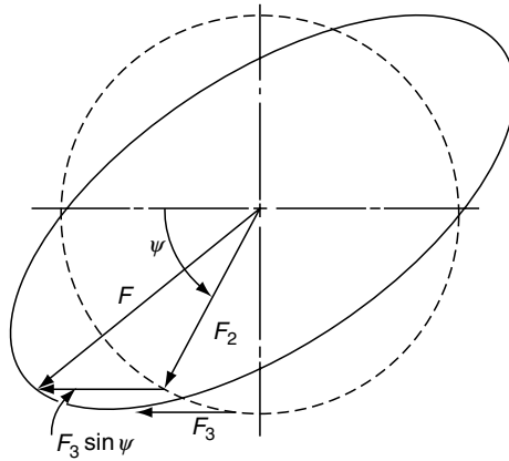
FIGURE 11.26 Load vector diagram for bearing loading consisting of a rotating load F_2 and a sinusoidal load F_3 . Maximum F_3 occurs 90^\circ out-of-phase with F_2 .
