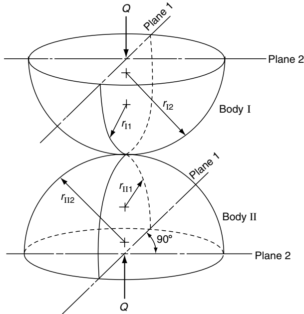
FIGURE 2.7 Geometry of contacting bodies.
