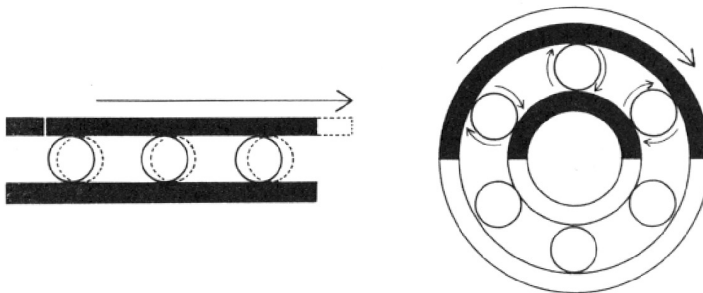
FIGURE 1.1 The evolution of rolling bearings. (Courtesy of SKF.)
