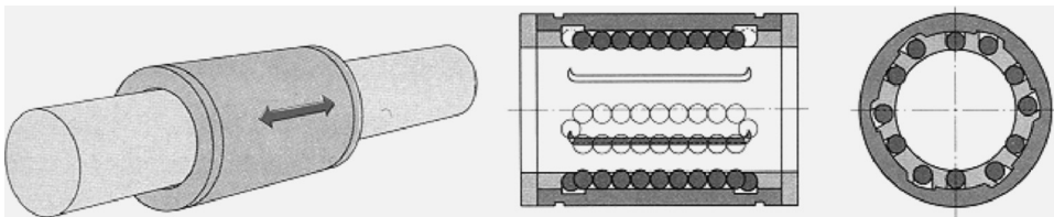
FIGURE 1.60 Schematic diagram of a ball bushing showing a recirculating ball set.
