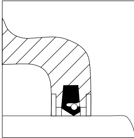
FIGURE 12.12 Garter seal cross-section showing retaining spring.
