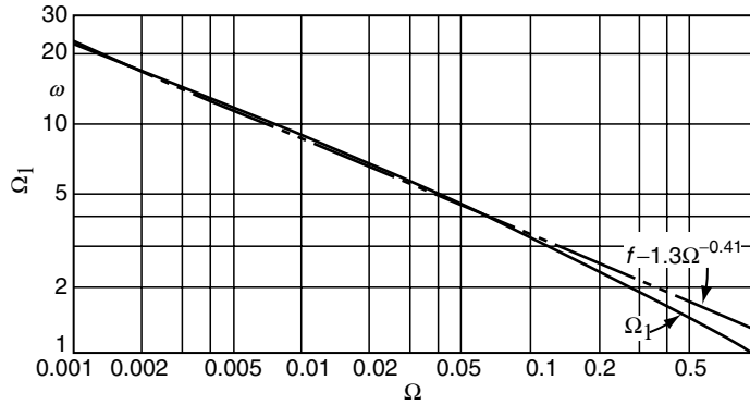
FIGURE 11.12 \Omega_1 vs. \Omega for point-contact ball and roller bearings. (From Lundberg, G. and Palmgren, A., Dynamic capacity of rolling bearings, Acta Polytech. Mech. Eng. , Ser. 1, No. 3, 7, Royal Swedish Acad. Eng., 1947. Reprinted with permission.)
