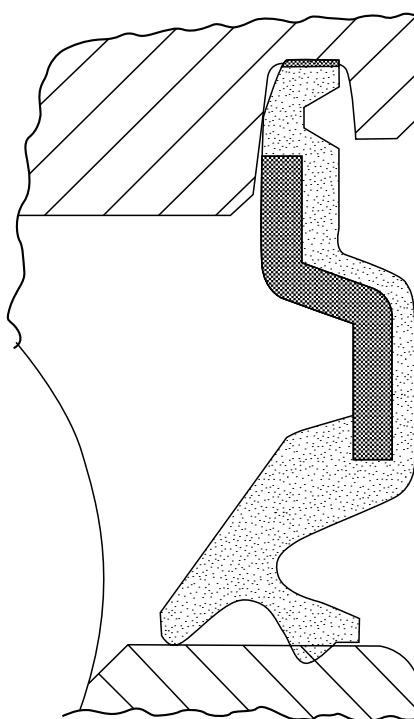
FIGURE 12.11 Double-lip seal. Inside lip is for fluid retention; outside lip is for dust exclusion.
