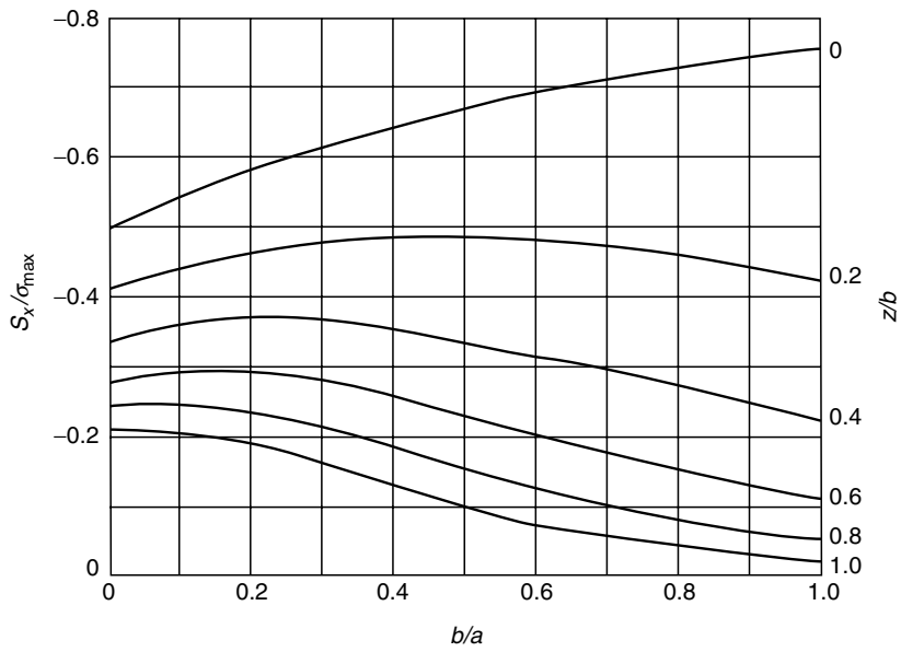
FIGURE 6.9 S_x/\sigma_{\max} vs. b/a and z/b .
