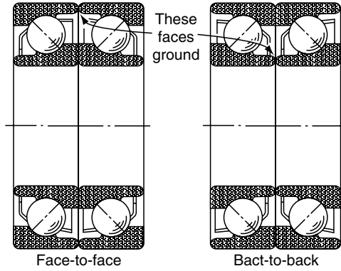
FIGURE 8.2 Duplex sets of angular-contact ball bearings.
