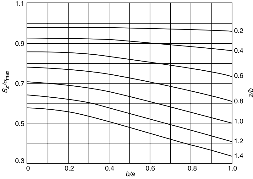
FIGURE 6.11 S_z/\sigma_{\max} vs. b/a and z/b .
