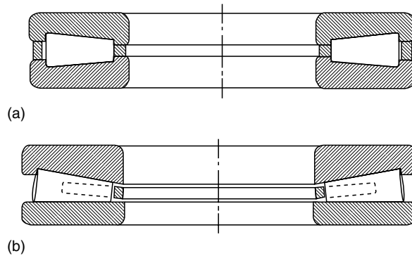
FIGURE 1.56 Tapered roller thrust bearing. (a) Both washers tapered; (b) one washer tapered.
