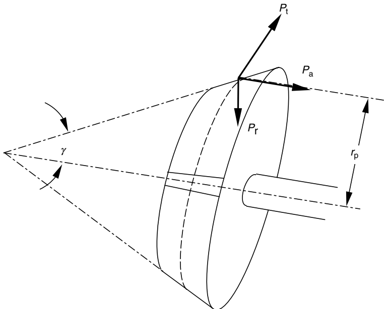
FIGURE 4.14 Loads transmitted by a straight bevel gear.
