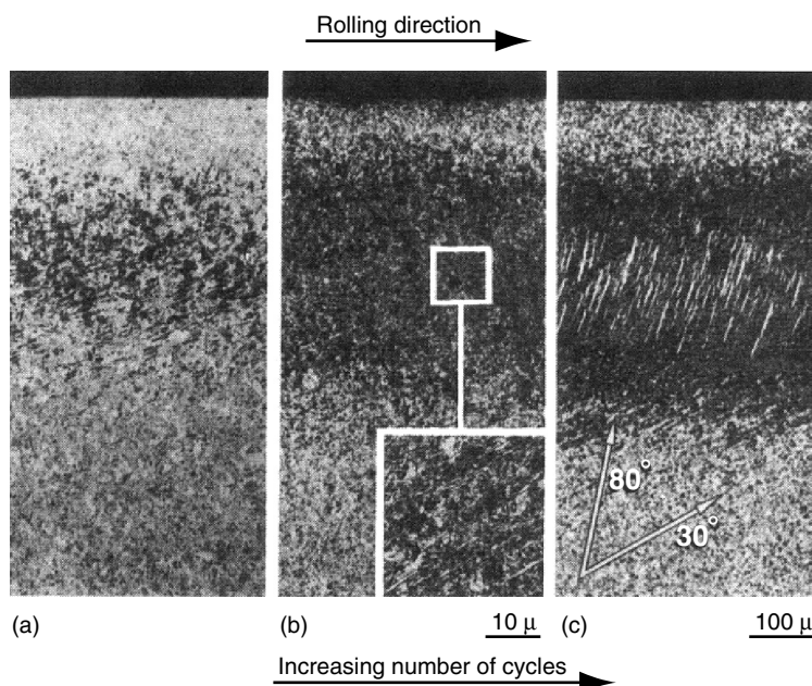
FIGURE 11.4 Optical micrographs of structural changes in 309 deep-groove ball bearing inner rings (parallel section). (a) DER in early stage. (b) Fully developed DER and 30° bands. (c) DER, 30° bands and 80° bands. (From Swahn, H., Becker, P., and Vingsbo, O., Martensite decay during rolling contact fatigue in ball bearings, Metallurgical Trans. A , 7A, 1099–1110, August 1976. With permission.)
