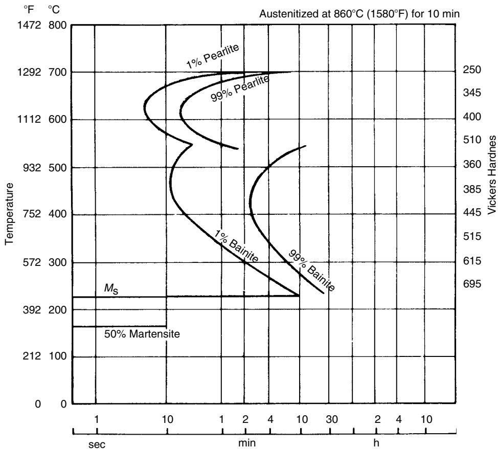
FIGURE 13.9 Time–temperature transformation diagram for AISI 52100 steel. (From SKF Steel, The Black Book , Vol. 194, 1984. With permission.)
