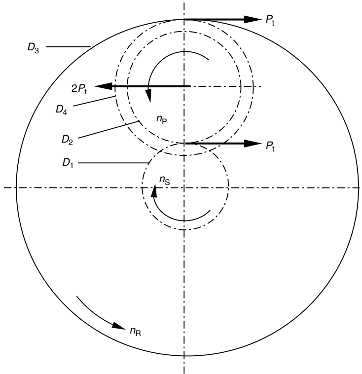
FIGURE 4.6 Planet gear loading.
