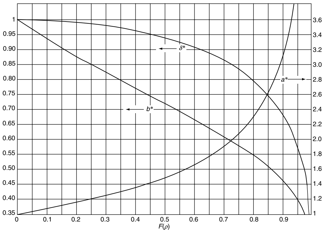
FIGURE 6.3 a^* , b^* , and \delta^* vs. F(\rho) .
