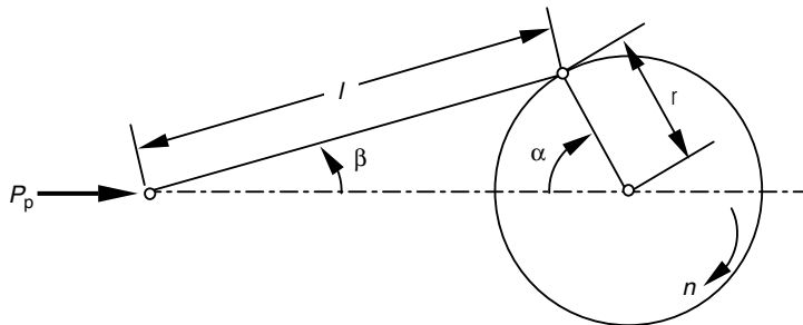
FIGURE 4.10 Schematic diagram of crank mechanism.
