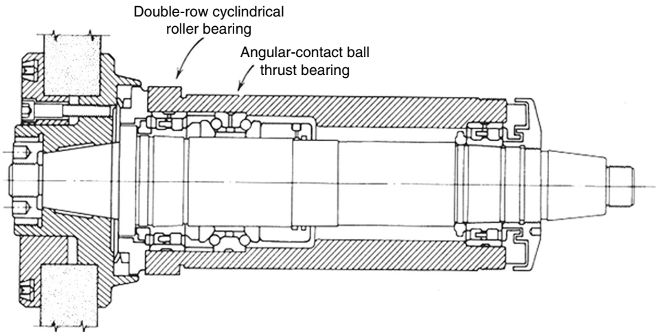
FIGURE 14.2 Grinding wheel spindle.
