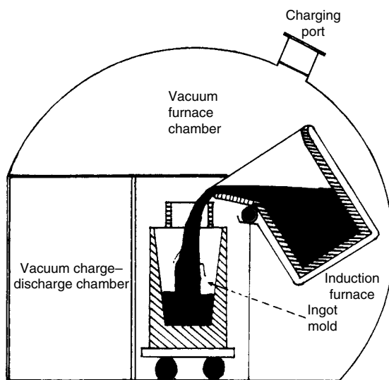
FIGURE 13.2 Schematic view of induction vacuum melting furnace.
