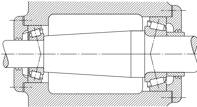
FIGURE 1.45 Typical mounting of tapered roller bearings.
