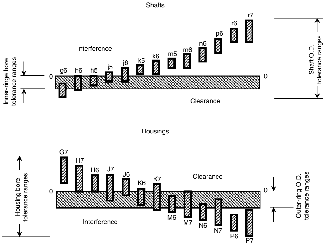
FIGURE 3.2 Graphical representation of bearing inner ring-shaft and bearing outer ring-housing standard fit classifications.
