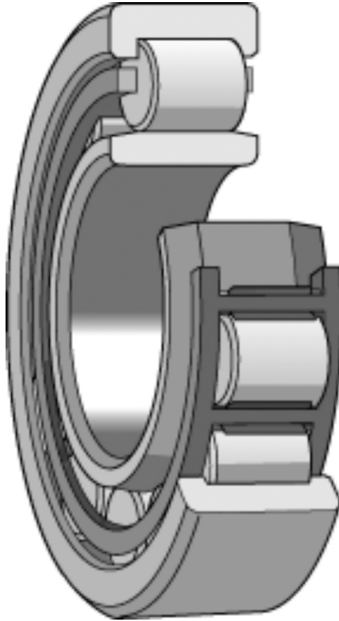
FIGURE 1.35 A radial cylindrical roller bearing. (Courtesy of SKF.)
