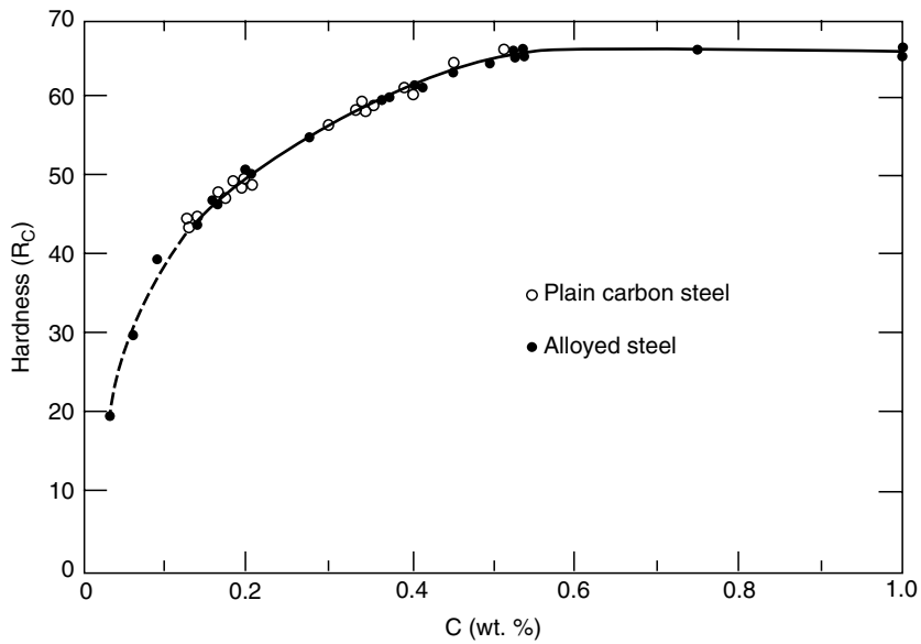
FIGURE 13.15 Maximum hardness vs. carbon content.
