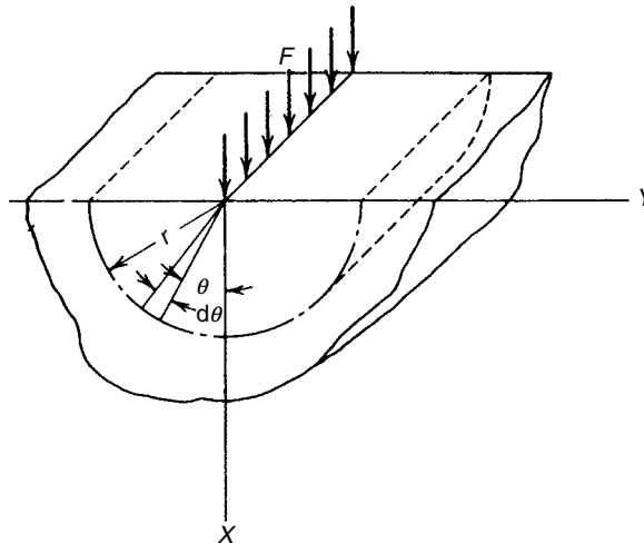
FIGURE 6.2 Model for Boussinesq analysis.
