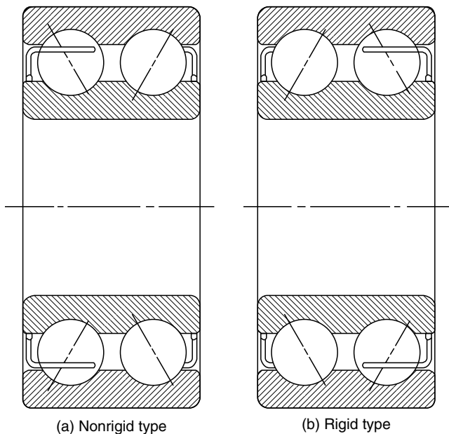
FIGURE 1.27 Double-row angular-contact ball bearings.
