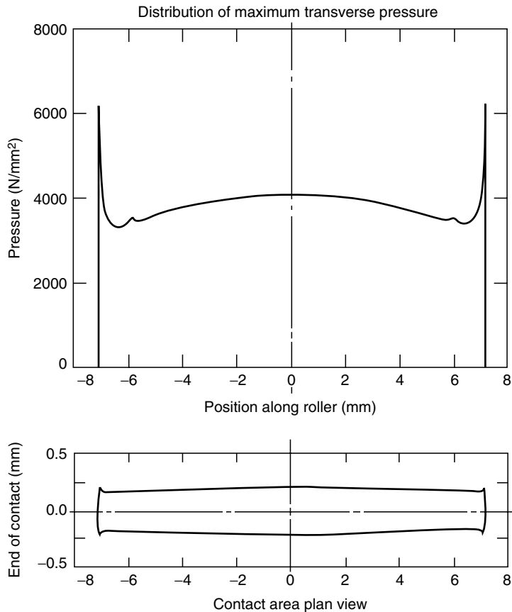
FIGURE 6.25 Heavy edge-loaded roller bearing contact (example of non-Hertzian contact).
