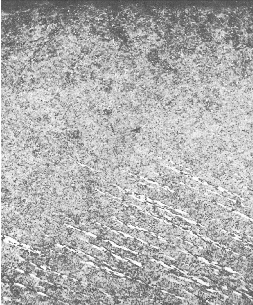
FIGURE 6.16 Subsurface structure (300 times magnification after picral etch) showing orientation of carbides to direction of rolling. Carbides are thought to be weak locations at which fatigue failure is initiated.
