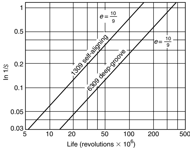
FIGURE 11.10 Typical Weibull plot for the ball bearings. (From Lundberg, G. and Palmgren, A., Dynamic capacity of rolling bearings, Acta Polytech. Mech. Eng. , Ser. 1, No. 3, 7, Royal Swedish Acad. Eng., 1947. Reprinted with permission.)
