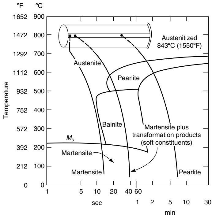
FIGURE 13.11 CCT diagram for AISI 52100 steel.
