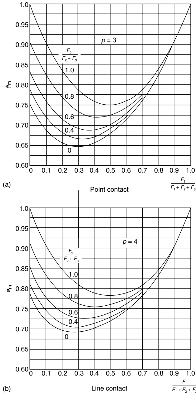
FIGURE 11.22 \phi_m vs. F_1/(F_1 + F_2 + F_3) for the generalized loading in Figure 11.21 .
