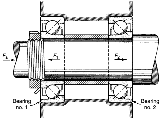
FIGURE 8.5 Preloaded set of duplex bearings subjected to F_a , an external thrust load. The computation for the resulting deflection is complicated by the fact that the preload at bearing 1 is increased by load F_a while the preload at bearing 2 is decreased.
