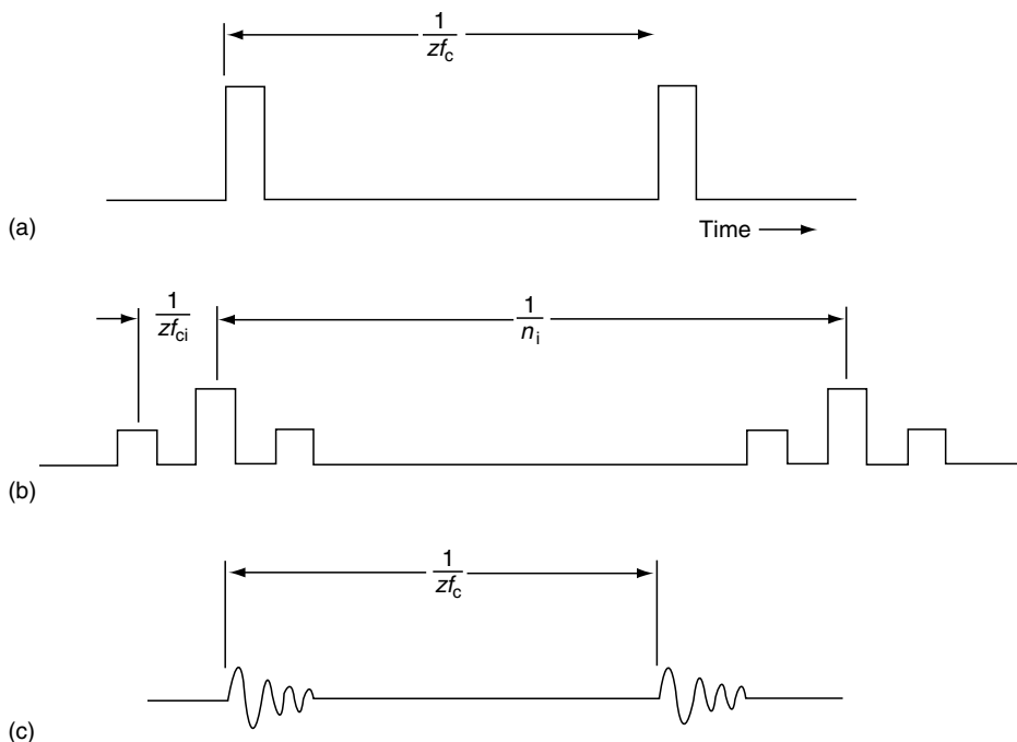
FIGURE 14.13 Impulse train. (a) Outer raceway damage. (b) Inner raceway damage. (c) Resonant vibration.
