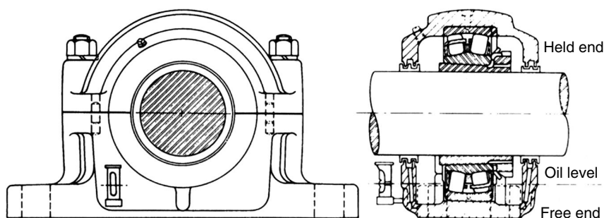
FIGURE 12.4 Pillow block with oil sump.
