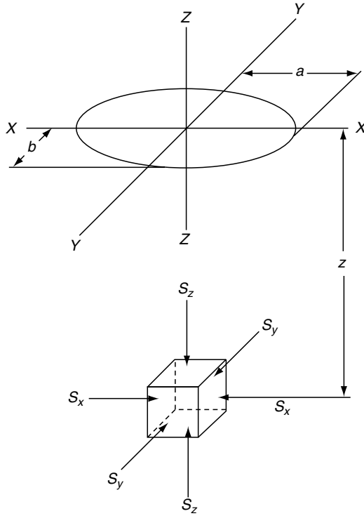
FIGURE 6.8 Principal stresses occurring on element on Z axis below contact surface.
