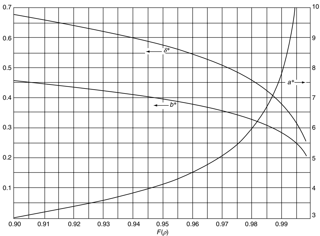
FIGURE 6.4 a^* , b^* , and \delta^* vs. F(\rho) .
