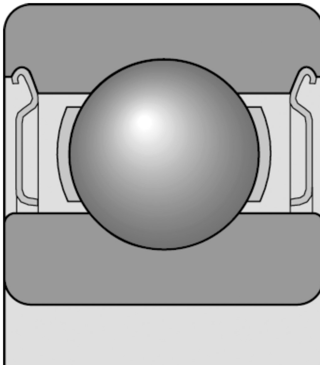
FIGURE 1.17 A single-row deep-groove ball bearing that has two shields to exclude dirt from the bearing. (Courtesy of SKF.)
