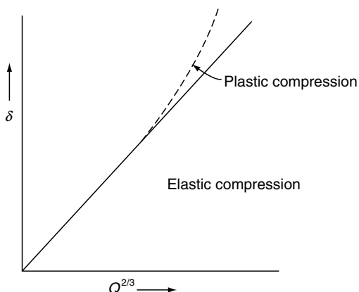
FIGURE 9.3 Deflection vs. load in point contact.
