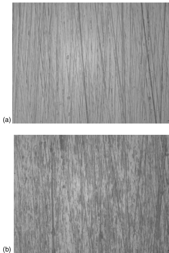
FIGURE 13.25 Optical images of outer raceways at 100 \times : (a) before testing, (b) after testing with standard rollers, and
