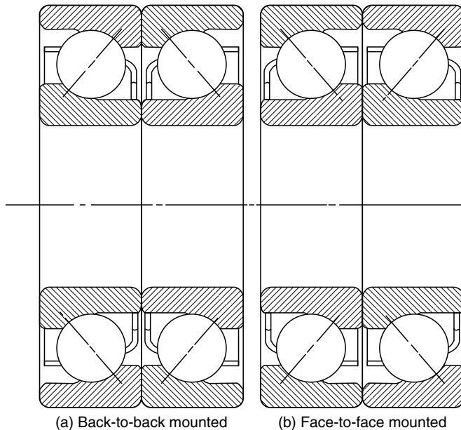
FIGURE 1.25 Duplex pairs of angular-contact ball bearings.
