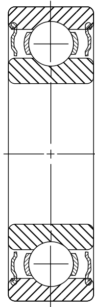
FIGURE 12.9 Radial ball bearing with double shields.
