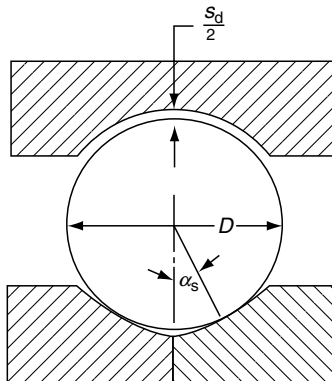
FIGURE 2.5 Split inner-ring ball bearing assembly showing bearing shim angle.
