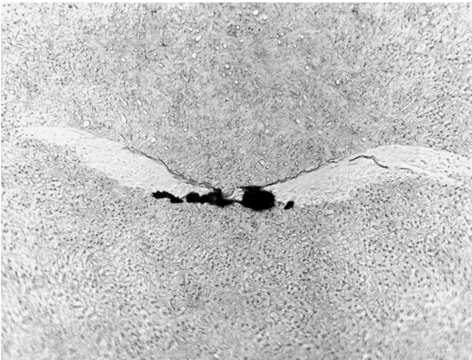
FIGURE 11.5 Fatigue crack in the subsurface of a ball bearing raceway.
