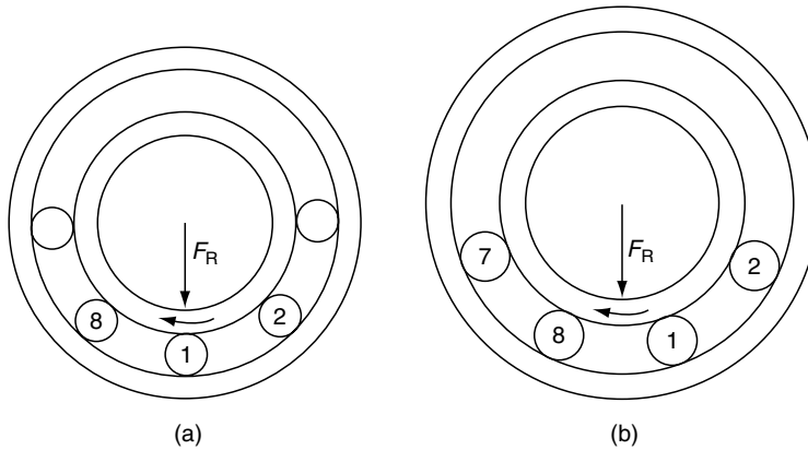
FIGURE 14.3 (a) Angular position of ball set, time = 0. (b) Angular position, time = \frac{1}{2} [1/Z (cage rotation frequency)].
