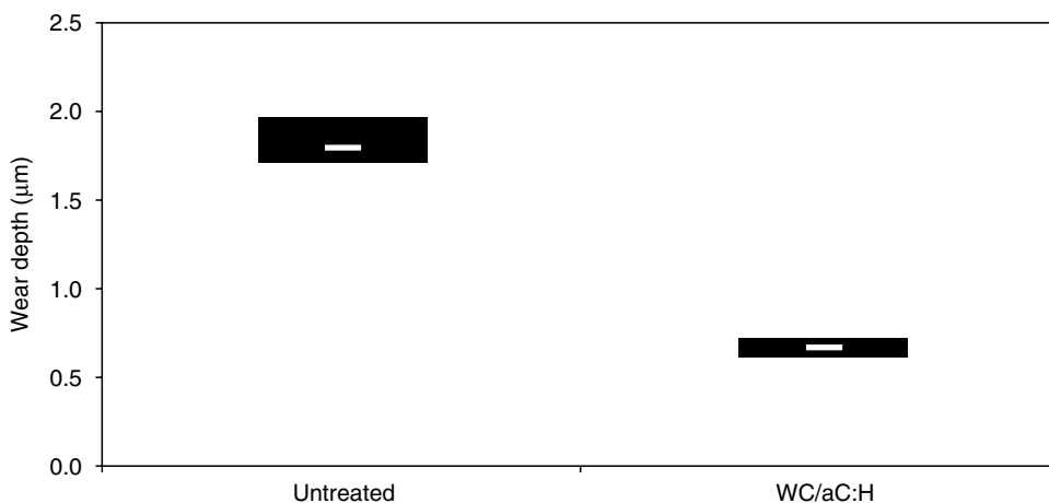
FIGURE 13.20 Tapered roller bearing false brinelling test of untreated steel and WC/aC:H-coated rollers showing the mean with bars of one standard deviation of the resulting groove depth. Twenty-five tests for each condition were conducted with a GL-4 gear oil oscillating under an 18,700 N (4,204 lb) axial load for 500,000 cycles.
