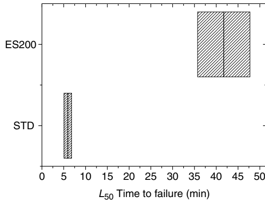
FIGURE 13.23 Rib-roller end scuffing test results with 90% confidence bands for bearings with standard (STD) and TiC/aC:H-coated (ES200) roller large ends. (Evans, R., et al., Nanocomposite tribological coatings for rolling element bearings, Mat. Res. Soc. Symp. Proc. , 750, 407–417, 2003. With permission.)
