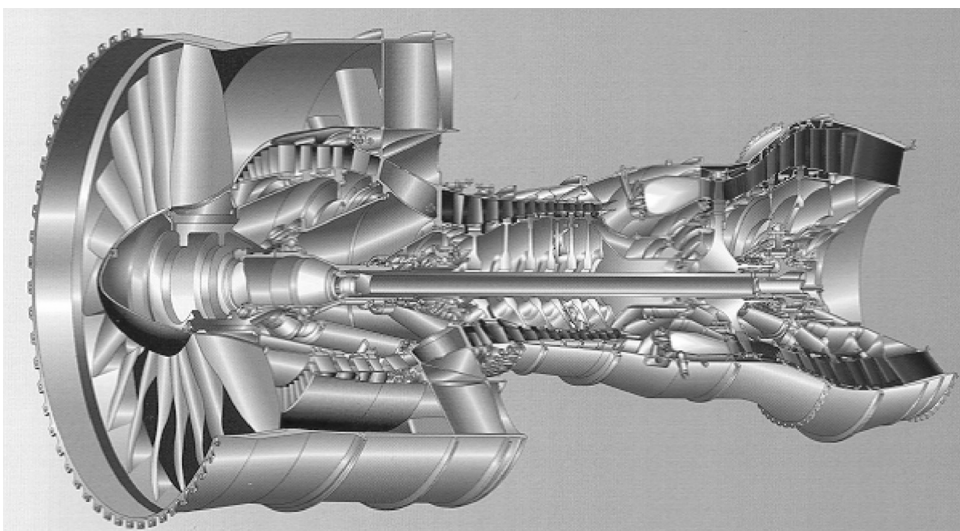
FIGURE 1.31 Cutaway view of turbofan gas turbine engine showing mainshaft bearing locations. (Courtesy of Pratt and Whitney, United Technologies Corp.)
