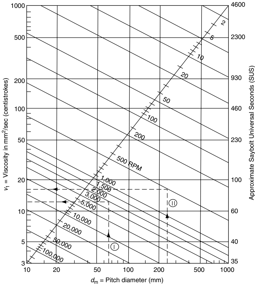
FIGURE 12.3 Minimum required lubricant kinematic viscosity ( \nu_1 ) vs. bearing pitch diameter ( d_m ) and speed. (From SKF, General Catalog 4000US , 2nd Ed., 1997–2001. With permission.)
