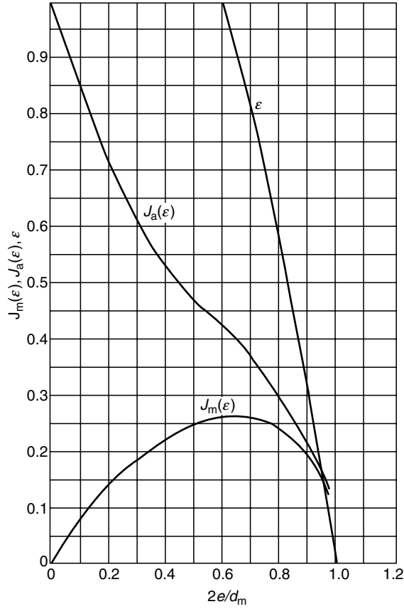
FIGURE 7.8 J_m(\varepsilon) , J_a(\varepsilon) , \varepsilon vs. 2e/d_m for point-contact thrust bearings.
