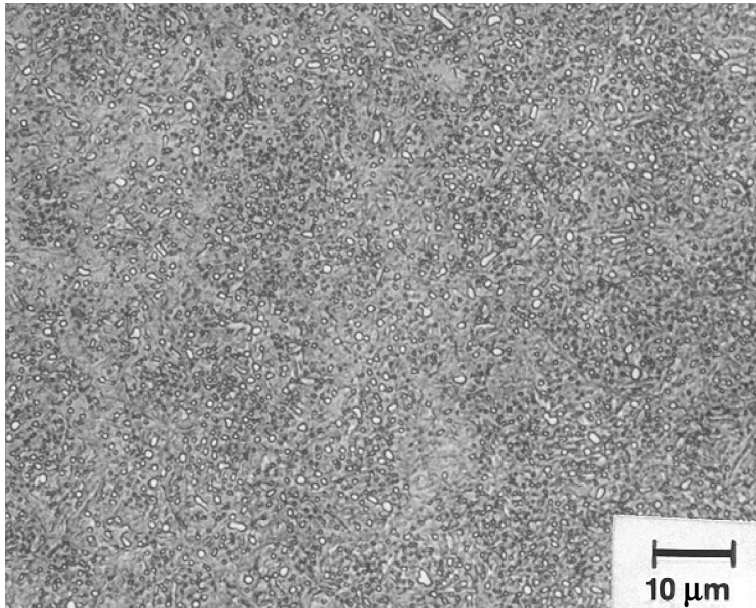
FIGURE 11.1 Microstructure of hardened and tempered AISI 52100 steel.
