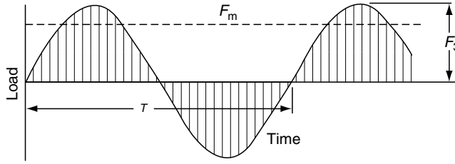
FIGURE 11.23 Sinusoidal bearing load.
