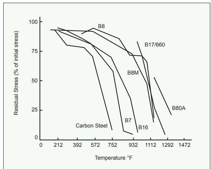
Stress Retention Properties of Bolt Materials
