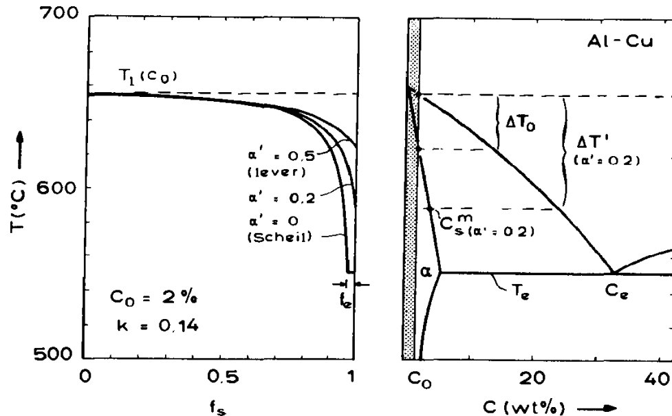
Figure 6.5: RELATIONSHIP OF THE SEGREGATE FREEZING POINT TO THE PHASE DIAGRAM. An increasing concentration (for distribution coefficients less than unity) is associated with a decreasing liquidus temperature since the slope, m , is then less than zero. Using the curves of figure 6.4, the temperature of the liquid as a function of volume fraction solidified can be derived. The use of realistic diffusion coefficients shows that, for small systems (such as interdendritic regions - figure 6.6) interstitial C in delta- and gamma-Fe will behave according to the lever-rule. Hence, the last liquid of a binary Fe-C melt will solidify at a temperature close to the solidus while substitutional alloys, such as Al-Cu, which typically have much smaller solid-state diffusion coefficients will usually contain eutectic material in the last (interdendritic) regions to solidify even when the overall composition is less than the solubility limit at T_e .
