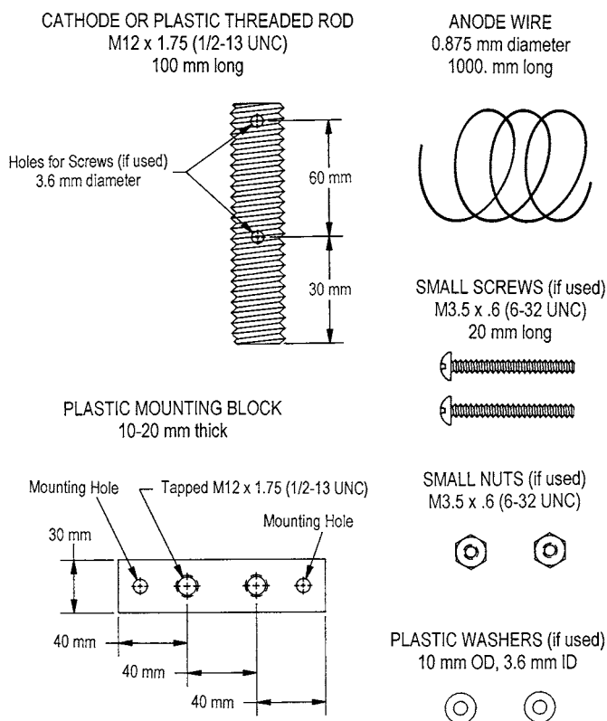
FIG. 1 Components for Making Wire-on-Bolt Exposure Assemblies
