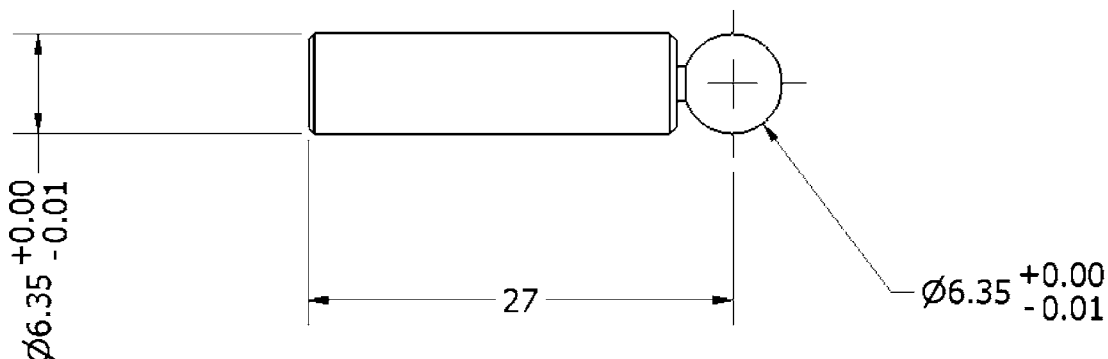
FIG. 1 Geometry of Alignment Pin (all dimensions are in mm)
