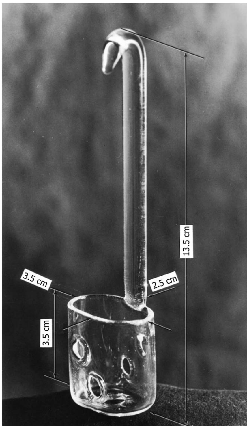
FIG. 2 Glass Cradle
