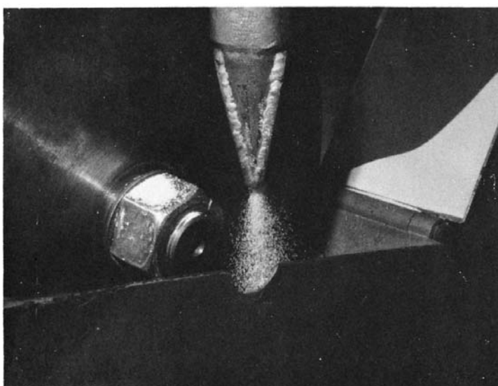
FIG. 10 Sand Flow—Turbulence
