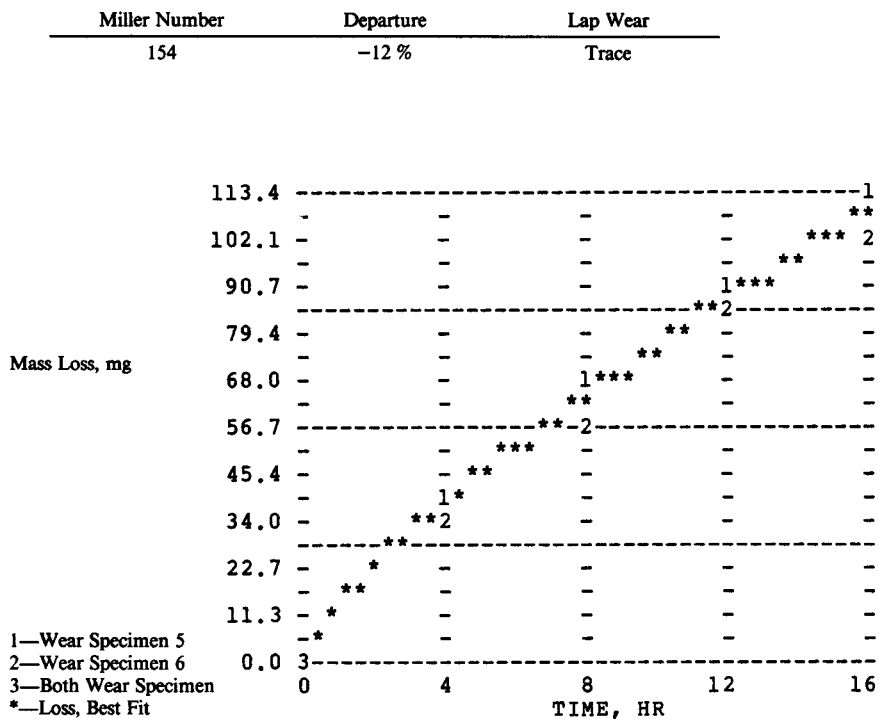
FIG. X1.6 Slurry Abrasivity Determination by Miller Number System—Test RM-3 (Test Method G75)
