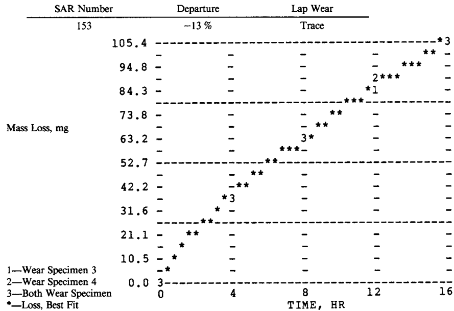
FIG. X1.8 Slurry Abrasion Response (SAR Number) Determination by Miller Number System—Test RS-2
