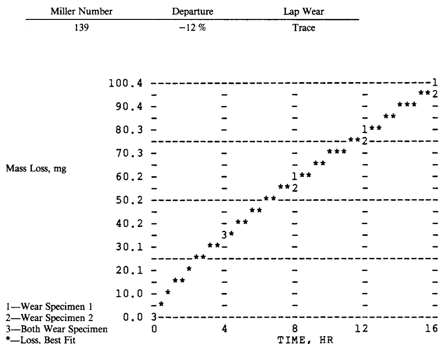
FIG. X1.4 Slurry Abrasivity Determination by Miller Number System—Test RM-1 (Test Method G75)
