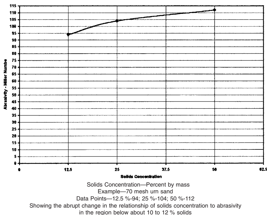
FIG. A1.1 Solids Concentration Versus Abrasivity
