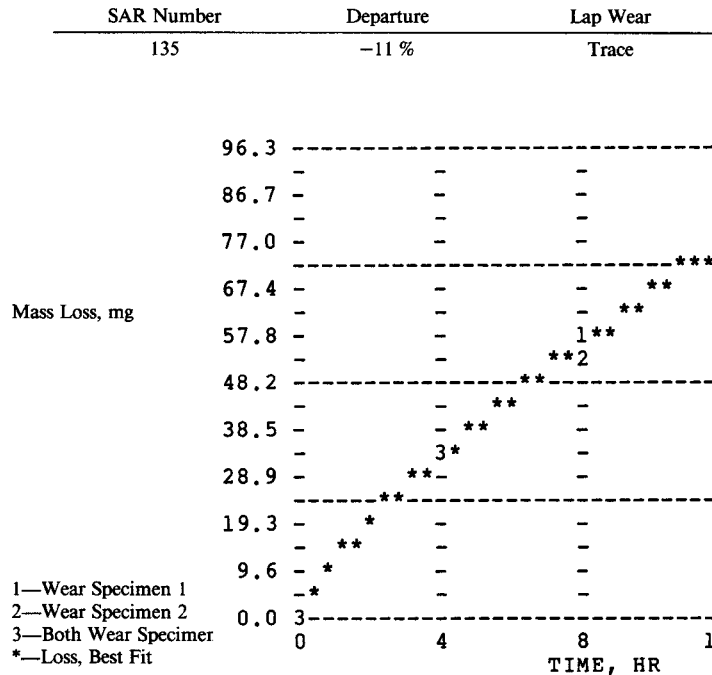
FIG. X1.7 Slurry Abrasion Response (SAR Number) Determination by Miller Number System—Test RS-1
