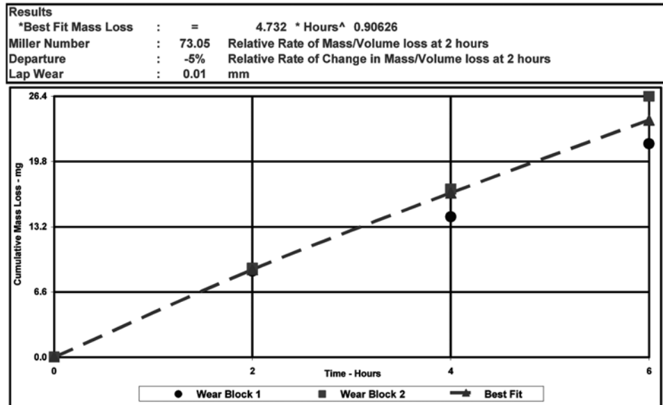
FIG. X1.1 Slurry Abrasivity Determination by Miller Number System (Test Method G75)
