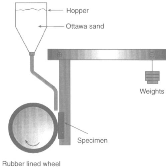
ASTM G65 test system
