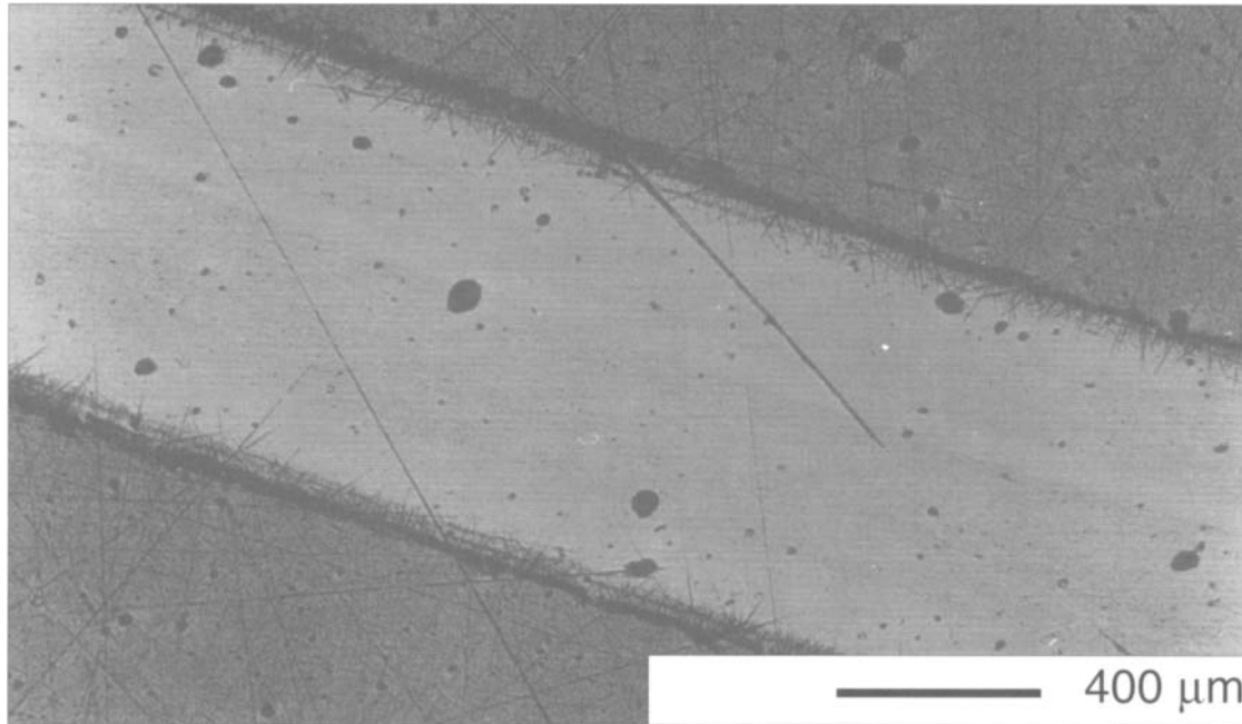
(b) More heavily worn wear track with removal of scratches from centre of wear track by wear process
