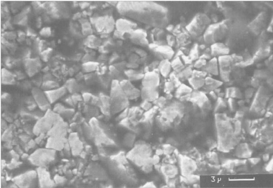
Fig. 5.4 A view with a scanning electron microscope at high magnification. A worn tungsten carbide in cobalt hard metal surface showing deformed and fractured grains
