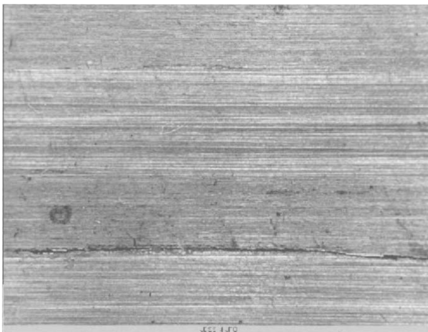
Fig. 2.2 Abrasive wear from hard particles trapped between moving surfaces
