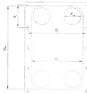
Figure 45-6.1 Typical PHE Geometry
