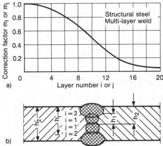
Fig. 196. Correction factors m_i or m_j dependent on layer number i or j (a); layer total thickness h_i or h_j of four-layer butt weld in double-V groove and layer sequence i = 1 , i = 2 , j = 1 , j = 2 (b); after Vinokurov [8]
