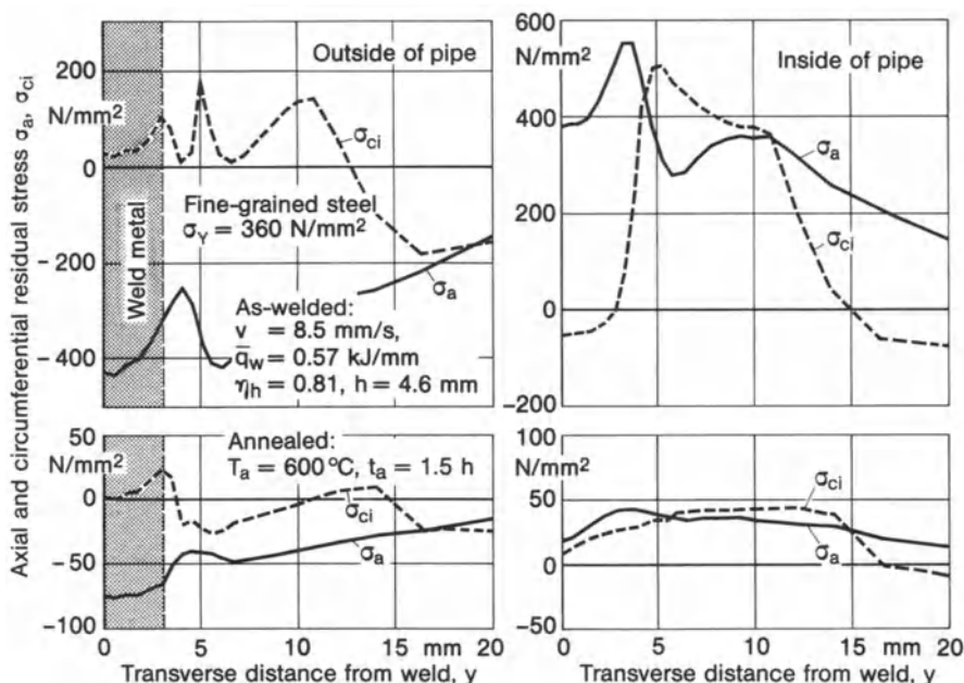
Fig. 245. Axial and circumferential residual stresses, \sigma_a and \sigma_{cl} , in outer and inner surface of pipe made of CMn-alloyed steel, as-welded and after annealing, analytical results; after Josefson [380]
