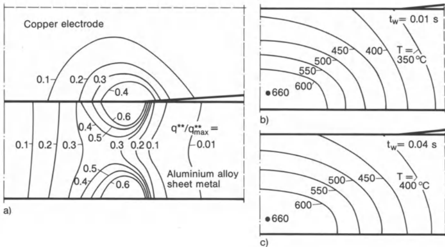
Fig. 77. Heat source density q^{**}/q^{**}_{\max} (a) and isotherms (b, c) during resistance spot welding of aluminium sheet metal, thickness 1 mm, time after onset of welding t_w , unobstructed heat transfer between copper electrode and aluminium plate, finite difference analysis based on electrical analogy introducing simplified modelling assumptions; after Ruge and Hildebrandt [50]
