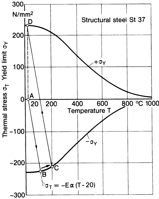
Fig. 166. Stress-temperature cycle in rod rigidly restrained on both ends, heating to 200°C with subsequent cooling, residual stress equal to tension yield limit; after Buttenschön [261]
