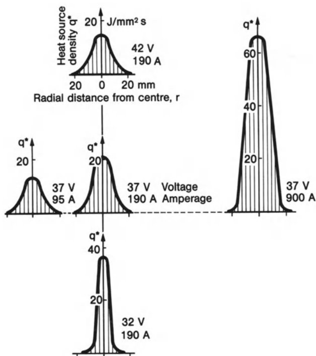
Fig. 47. Heat source density q^* of rapidly moving arc over radial distance from centre r , carbon electrode, dependency on amperage I and voltage U ; experimental results according to Kulagin in Ref. [1]
