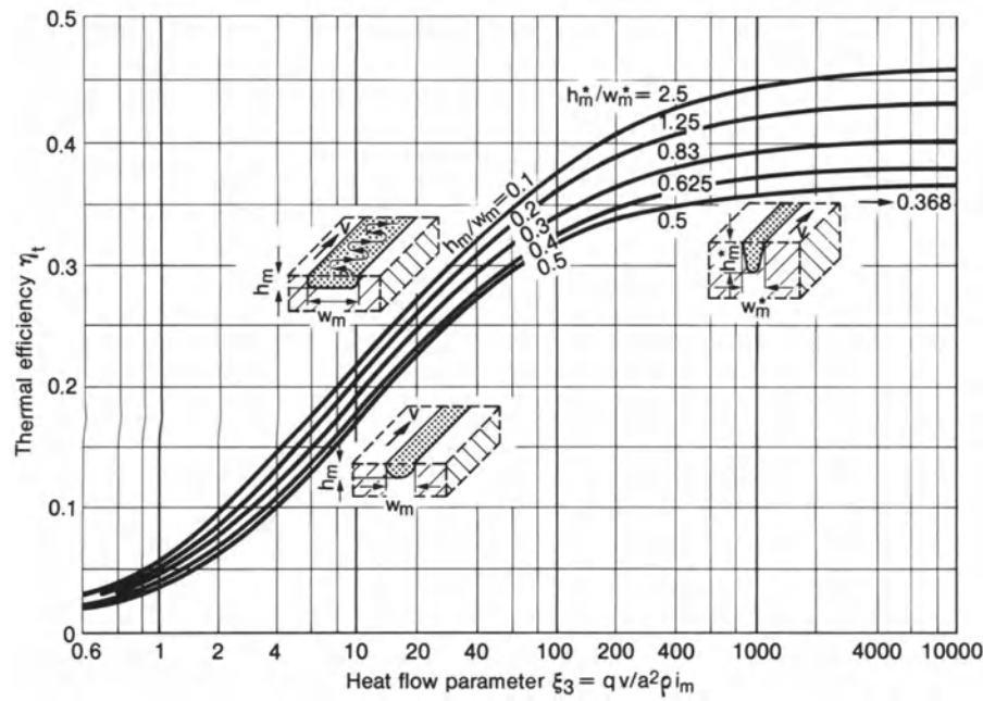
Fig. 54. Thermal efficiency \eta_t of surface welding with three-dimensional heat diffusion dependent on heat flow q , welding speed v , thermal diffusivity a and melting heat content q i_m for different ratios h_m/w_m or h_m^*/w_m^* ; after Rykalin [1]
