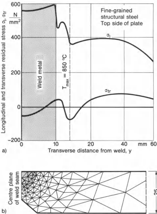
Fig. 154. Longitudinal and transverse residual stresses in top surface of structural steel plate with single-side submerged-arc butt weld (a) and appertaining finite element cross-section model (b); after Andersson [235]
