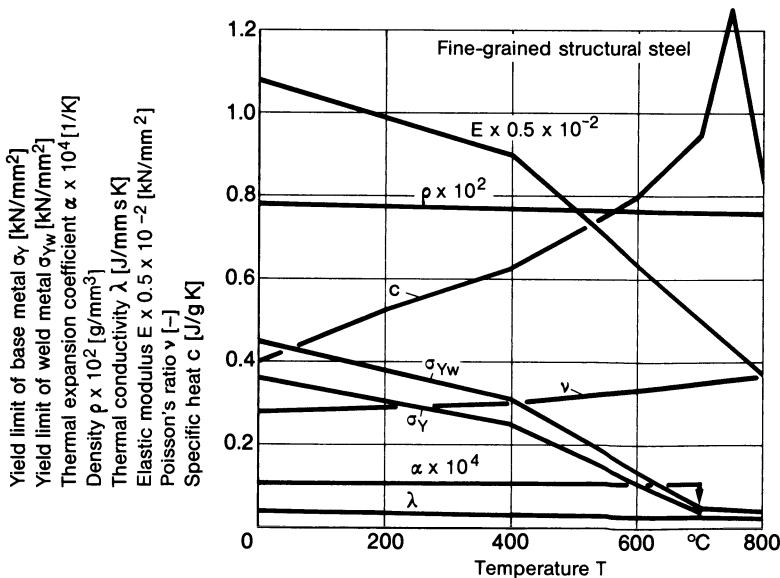
Fig. 114. Thermal and mechanical material characteristic values of fine-grained structural steel suitable for welding (micro-alloyed CMn steel) dependent on temperature (transformation heat at 700 °C covered by specific heat capacity c ); after Karlsson [234]
