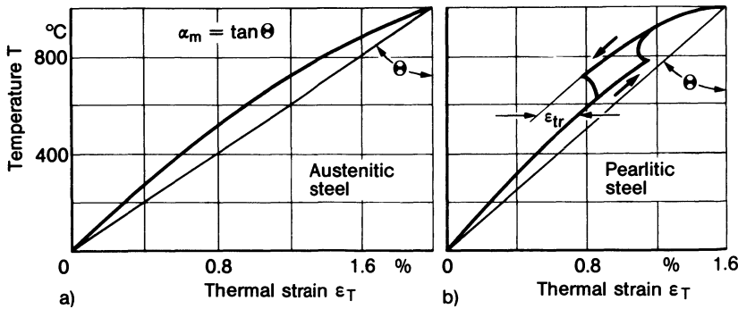
Fig. 109. Dilatometer curves for austenitic steel without transformation (a) and pearlitic steel with transformation (b), transformation strain \epsilon_{tr} ; after Vinokurov [8]
