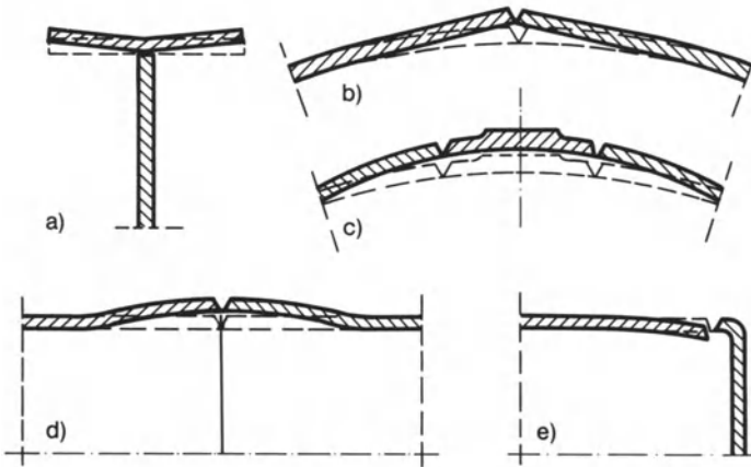
Fig. 226. Reduction of distortion by preshaping, pre-welding shape traced in solid lines, post-welding shape in broken lines: roof shaping of girder chords (a), plane end sections of cylindrical shells (b), outward bulging of spherical shell with block flange (c), outward bulging of pipe with circumferential weld (d), inward drawing of pipe at plane end (e); after Malisius [5] and Vinokurov [8]
