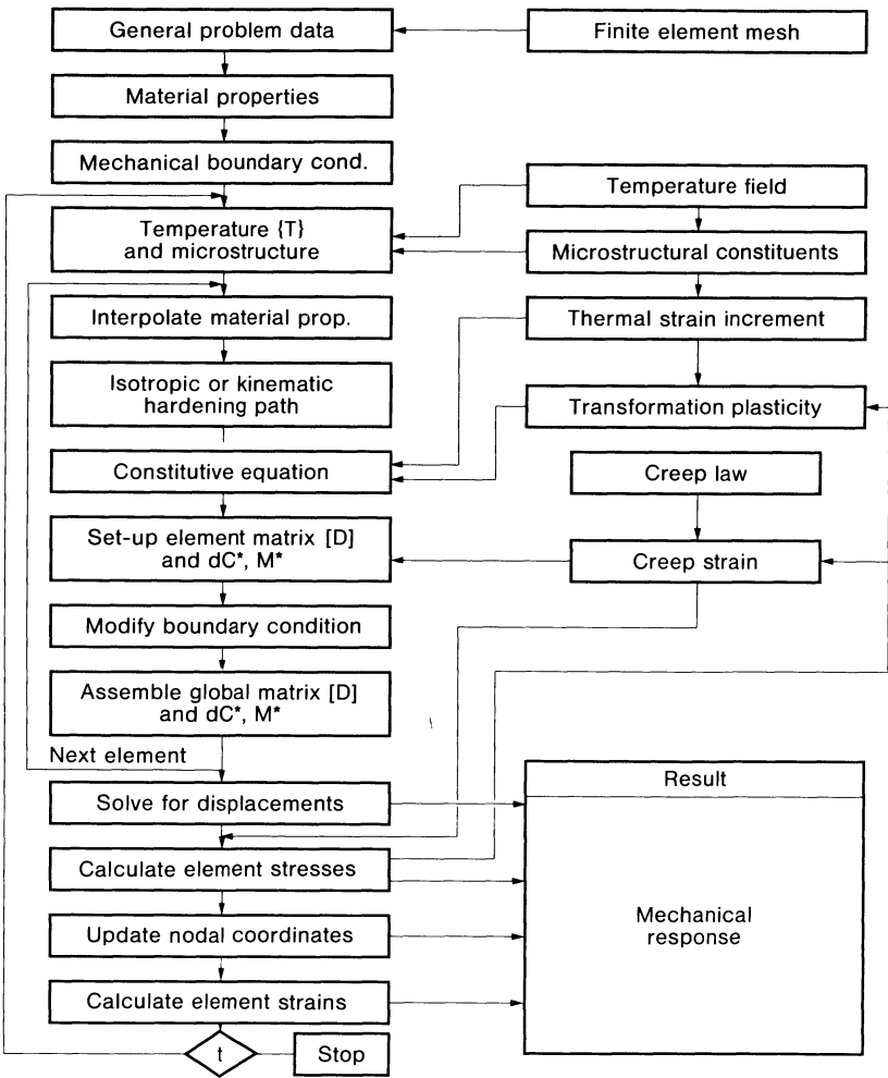
Fig. 91. Flow chart of finite element analysis of coupled thermal, mechanical and microstructural effects during heat treatment processes including welding; after Buchmayr and Kirkaldy [138]
