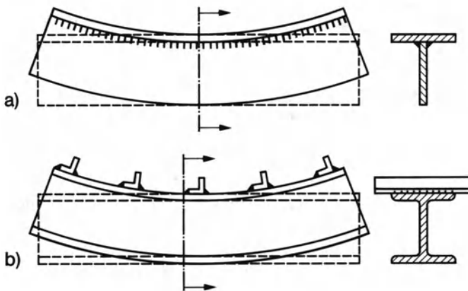
Fig. 14. Bending deformation of girders with eccentric longitudinal weld (a) and eccentric transverse weld (b)
