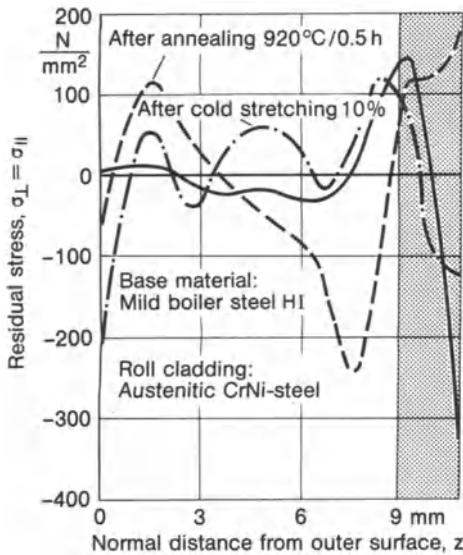
Fig. 186. Plane-hydrostatic residual stresses, \sigma_{\perp} = \sigma_{||} , in ferritic mild boiler steel with austenitic roll cladding, as-delivered, after annealing and after cold-stretching, experimental results; after Schimmöller [281] (ibid. mean values of \sigma_1 and \sigma_2 of specimen types 1.1 to 1.3)
