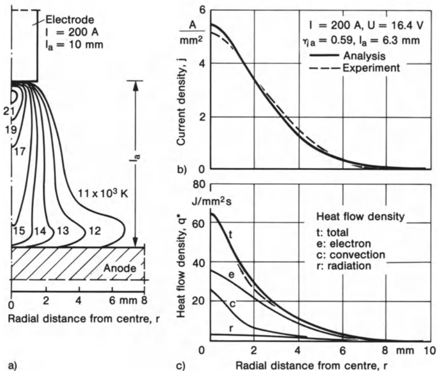
Fig. 60. Temperature field isotherms (a), anode current density (b) and anode heat flow density (c) in stationary gas tungsten arc ( I = 200 A, plane pool surface, arc length 10 mm), analytical and experimental results; after Szekely [81]
