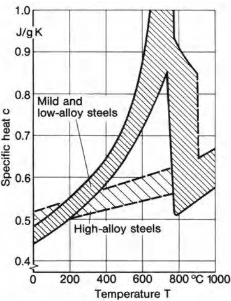
Fig. 18. Mass-specific heat capacity c of steels dependent on temperature, transformation heat at 700 °C covered by c ; areas of individual curves according to Richter [23]
