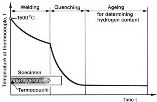
Fig. 107. Temperature profile over time (schematic representation) for weld surface point in centre section of bead specimen standardized for measuring hydrogen content after welding; after Dickehut and Ruge [176]
