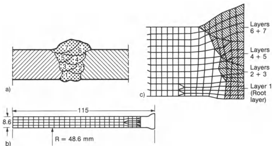
Fig. 146. Discretization into solid ring elements of multilayer circumferential weld in pipe; layer structure in reality (a), solid ring element model with enlarged detail (b, c), symmetry half with combined weld layers; after Rybicki and Stonesifer [229]
