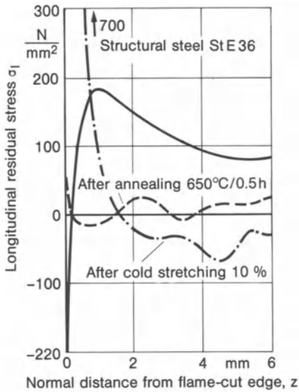
Fig. 187. Longitudinal residual stress \sigma_l in flame-cut edge of structural steel StE36 as-delivered, after annealing and after cold-stretching, experimental results; after Schimmöller [285]
