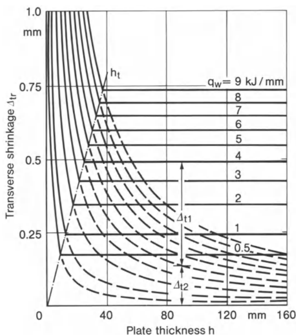
Fig. 190. Transverse shrinkage \Delta_{tr} dependent on plate thickness h and heat input per unit length of weld, q_w , for structural steel: \Delta_{tr} = \Delta_{t2} for h < h_t , \Delta_{tr} = \Delta_{t1} + \Delta_{t2} for h > h_t , results from calculation; after Satoh et al. [266, 277, 297]
