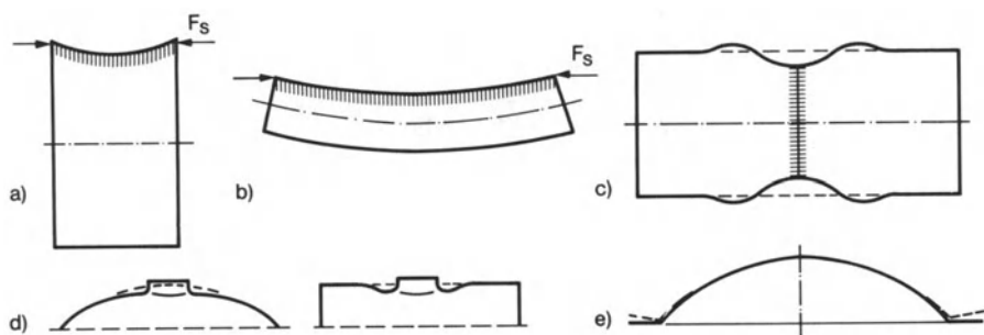
Fig. 194. Longitudinal and bending shrinkage at longitudinal weld (a, b), circumferential weld (c) and ring weld (d, e) of cylindrical and spherical shell
