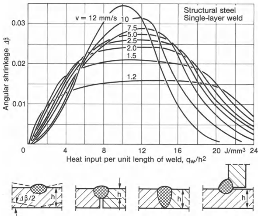
Fig. 195. Angular shrinkage \Delta\beta dependent on heat input per unit length of weld, q_w , and weld or plate thickness h for different welding speeds v ; after Vinokurov [8]
