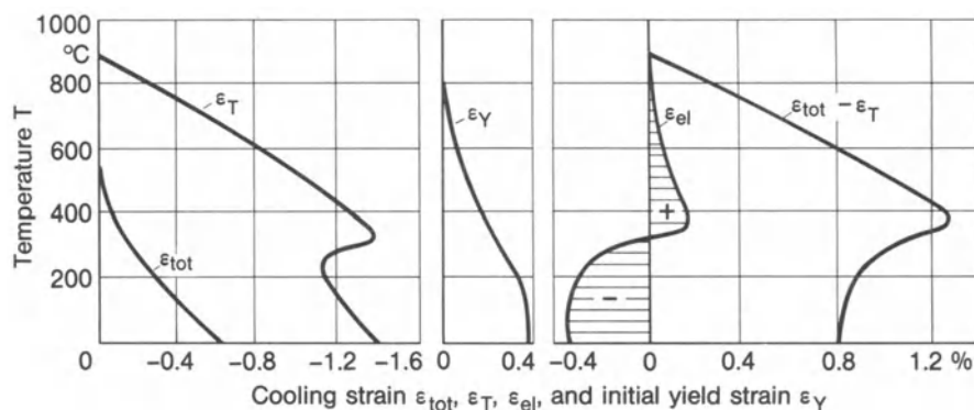
Fig. 205. Cooling strain profile at weld seam \varepsilon_{\text{tot}} and in dilatometer \varepsilon_T , initial yield strain \varepsilon_Y and elastic strain profile at weld seam \varepsilon_{\text{el}} over temperature; after Vinokurov [8]
