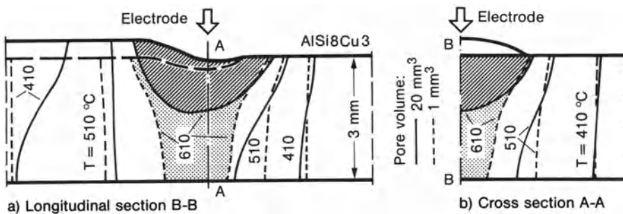
Fig. 71. Temperature field isotherms and weld reinforcement in plasma arc welding of aluminium die casting alloy GD-AlSi8Cu3 (liquidus temperature 610^\circ\text{C} , solidus temperature 510^\circ\text{C} ) for low and high pore volumes ( 1 and 20 \text{ mm}^3 per 23.2 \text{ mm} weld length), longitudinal section (a) and cross-section (b), analytical results based on hydrostatic modelling; after Na and Ruge [100]
