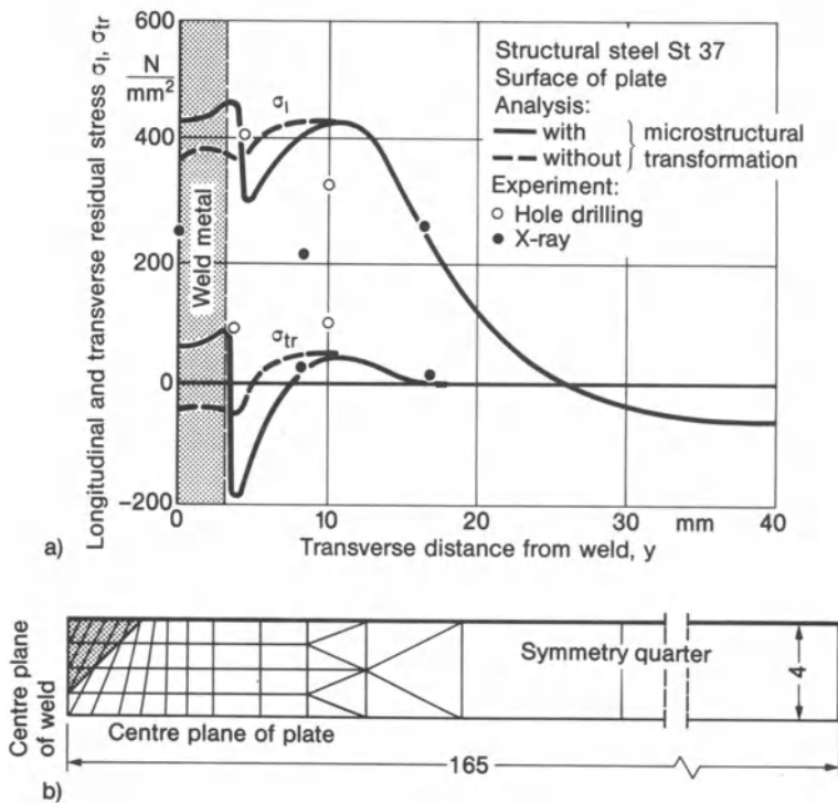
Fig. 155. Longitudinal and transverse residual stresses in surface of structural steel plate (St37) with double-V groove butt weld (a), analysis with and without microstructural transformation (to martensite), appertaining finite element cross-section model (b), comparison of analytical with experimental results; after Argyris, Szimmat and Willam [248]
