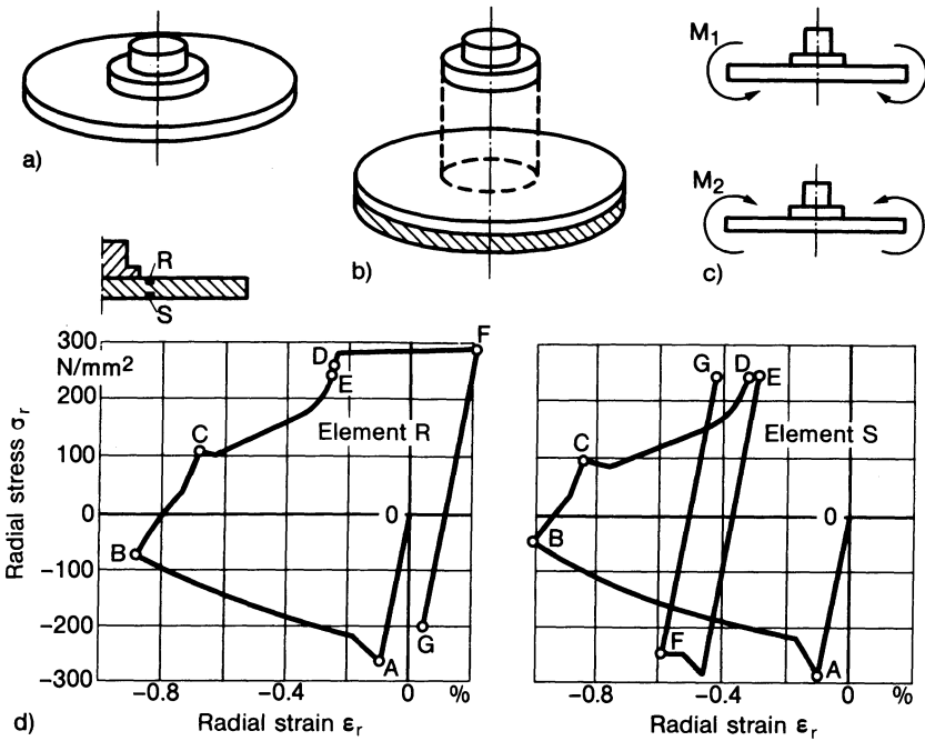
Fig. 141. Bolt on plate of beryllium (a), pressure butt welding followed by machining of the hatched layer (b), loading of plate edge by alternating bending moments M_1 and M_2 (c), stress-strain cycle in solid ring elements R and S (d): heating OAB, cooling BCD, machining DE, loading EFG; after Cyr, Teter and Stocks [224]
