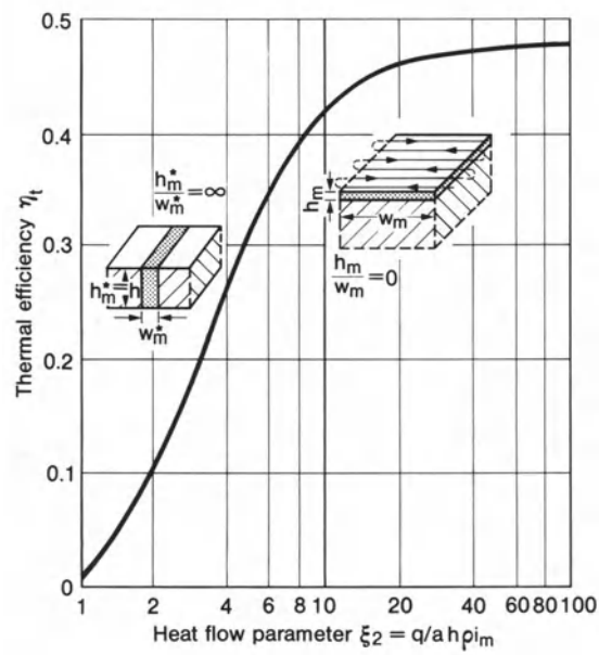
Fig. 55. Thermal efficiency \eta_t of butt welding or large-width surface welding with two-dimensional heat diffusion dependent on heat flow q/h , thermal diffusivity a and melting heat content q i_m ; after Rykalin [1]
