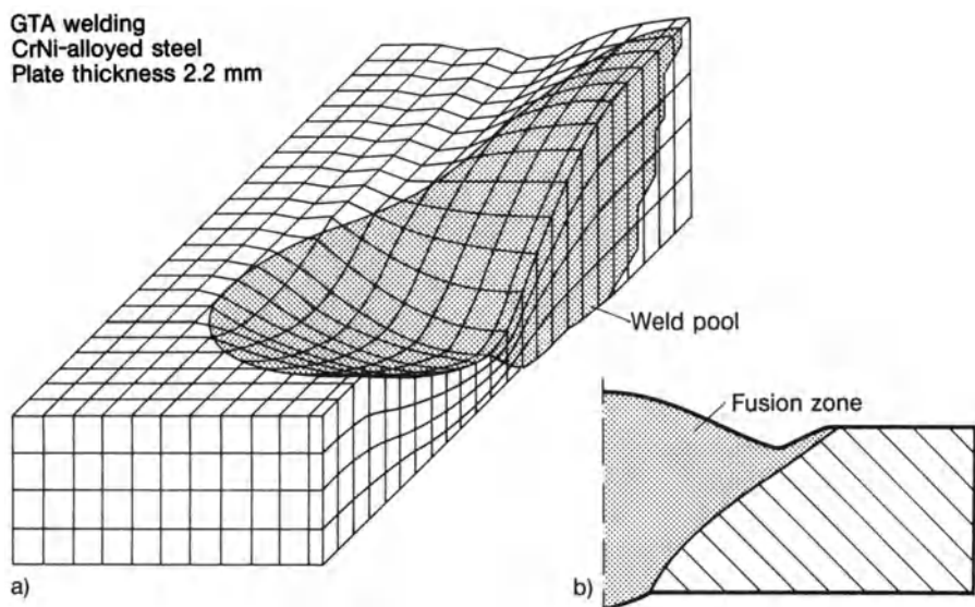
Fig. 68. Weld pool (a) and finished weld shape (b), analytical results based on hydrostatic modelling, gas tungsten arc welding ( I = 430 A, v = 30 mm/s, l_a = 1 mm) of CrNi-alloyed steel (plate thickness 2.2 mm); after Sudnik [86]
