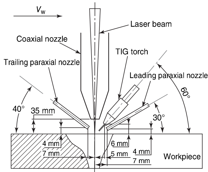
4.11 Schematic diagram of gas nozzle arrangement of hybrid CO 2 laser–TIG welding.
