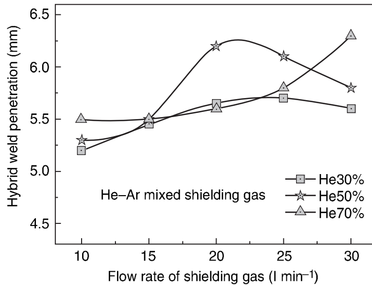
4.10 Effects of shielding gas flow on the weld penetration of hybrid laser–MAG welding for mild steel, He–Ar mixed shielding gas, plate thickness 7 mm.
