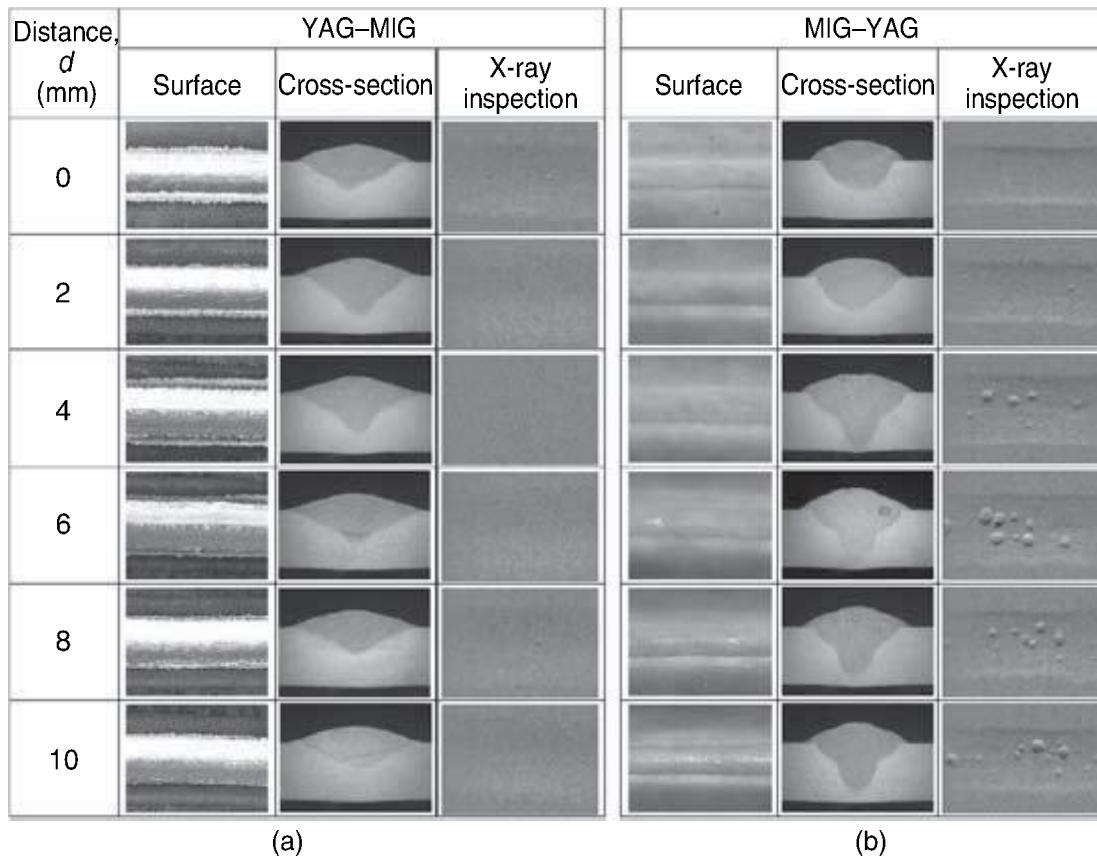
2.20 Comparison of surface, cross section and x-ray inspection results between (a) YAG laser–MIG or (b) MIG–YAG laser showing effect of distance ( d ) on weldability.
