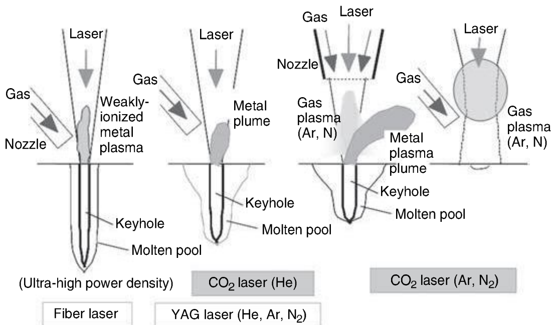
2.6 Schematic representation of plume, plasma and keyhole behavior during fiber, YAG and CO 2 laser welding, showing effect of plasma on energy transfer and consequent weld penetration.
