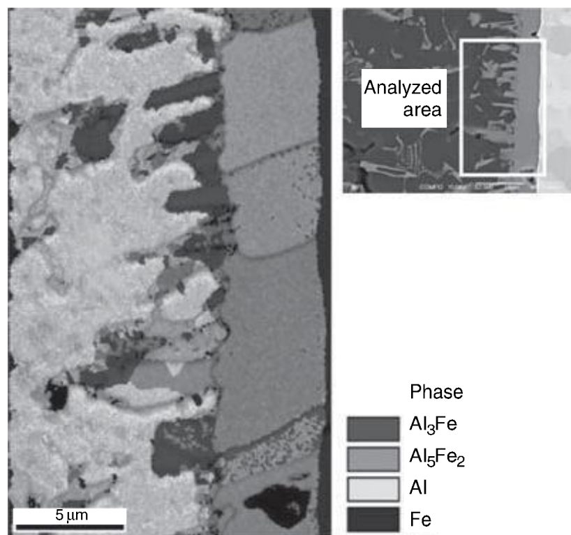
11.6 EBSD Image of part of the phase seam on the face side [aluminium EN AW-6056 (thickness 3.8 mm); steel THM 180BH + Z (thickness 1.95 mm)] (Courtesy: MPIE, Düsseldorf).
