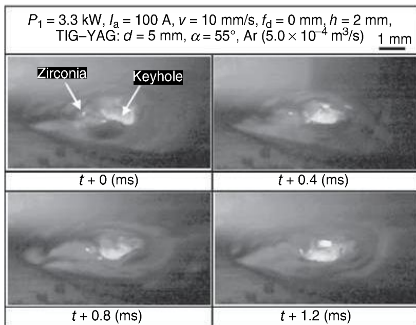
2.12 Observation results of molten pool surface and ZrO 2 particle tracer during hybrid TIG–YAG laser welding at 100 A in Ar gas.
