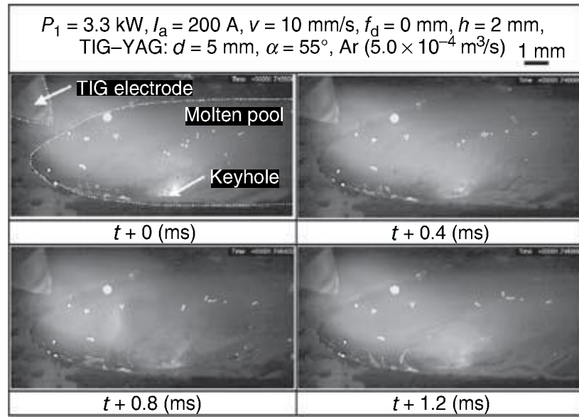
2.13 Observation results of molten pool surface and \text{ZrO}_2 particle tracer during hybrid TIG–YAG laser welding at 200 A in Ar gas.
