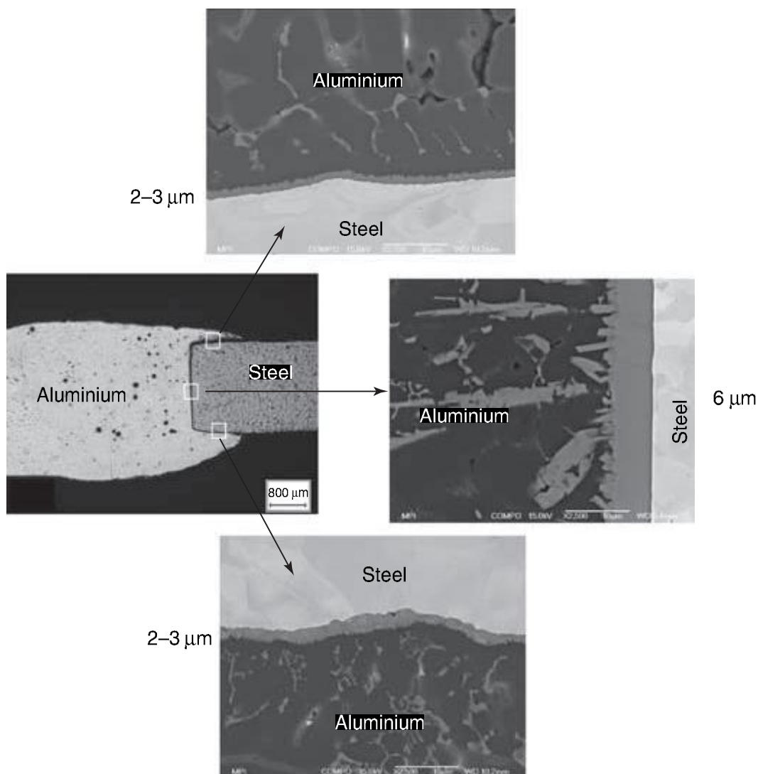
11.5 SEM images of the phase seam in the top, face and bottom region of a laser MIG hybrid welded aluminium–steel specimen aluminium EN AW-6056 (thickness 3.8 mm); steel THM 180BH + Z (thickness 1.95 mm)] (Courtesy: MPIE, Düsseldorf).
