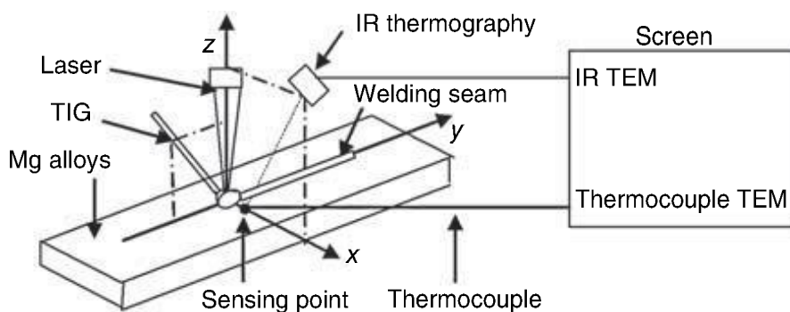
7.35 Sketch image of the infrared temperature measuring system. 38
