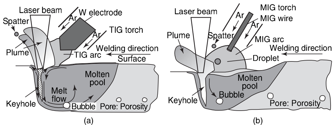
2.1 Schematic representation of hybrid laser–TIG (a) and laser–MIG welding.
