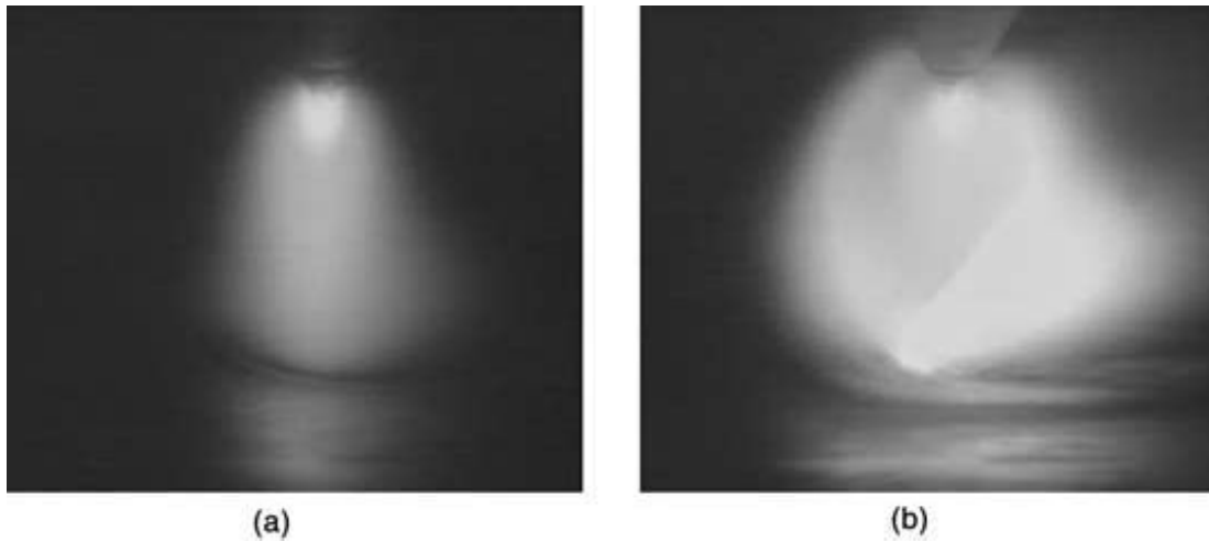
2.3 Observation results of arc behaviour of Type 304 steel during (a) TIG and (b) hybrid TIG–YAG laser welding.
