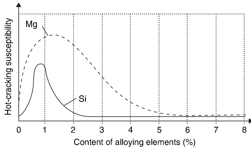
10.3 Hot-cracking susceptibility of EN AW-6XXX alloys depending on the content of Si and Mg (Kou, 2003).
