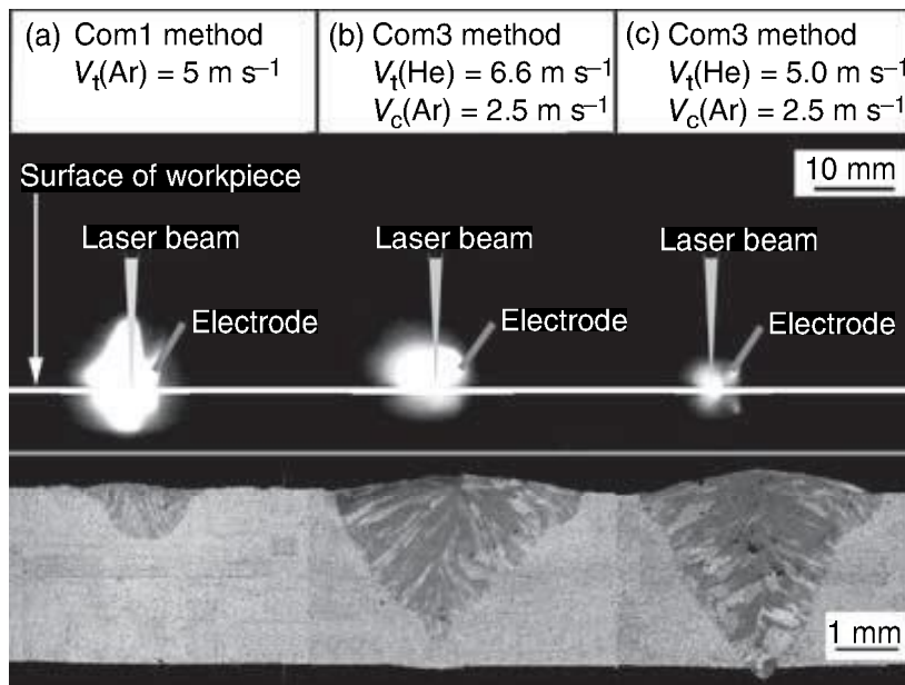
4.13 Effects of gas nozzle arrangement on plasma shape and weld penetration depth in hybrid CO 2 laser–TIG welding, 316L stainless steel with 3 mm thickness.
