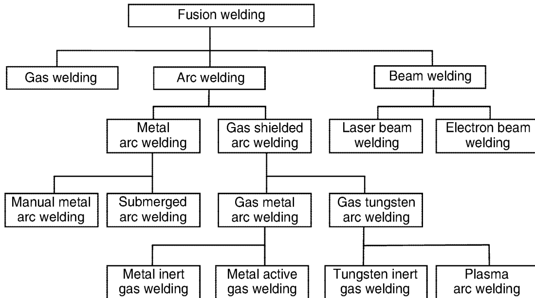
3.1 Schematic presentation of the most common fusion welding methods.
