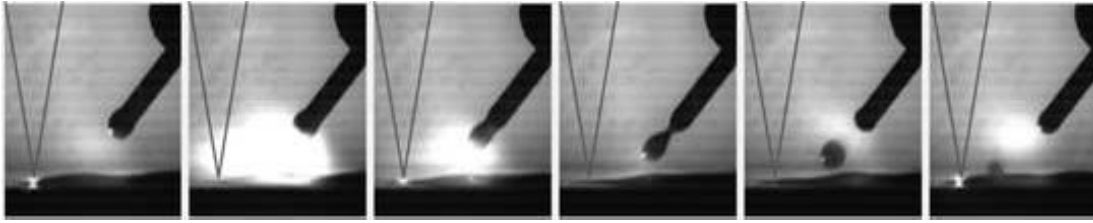
9.2 Metal transfer (background current phase, current rise phase, high current phase, necking, droplet detachment, dipping in molten pool).
