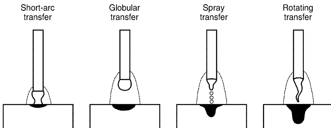
3.8 Basic metal transfer modes in gas–metal arc welding.
