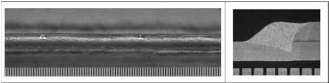
12.11 Example of hybrid weld bead with Ar+CO 2 +O 2 mixture.
