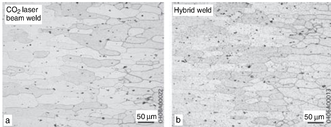
10.15 Change in the microstructure of the heat affected area close to the base material in (a) CO 2 laser beam weld and (b) hybrid weld in a 3.2 mm thick AA6013 sheet butt-welded in T6 (Vaidya et al. , 2006).
