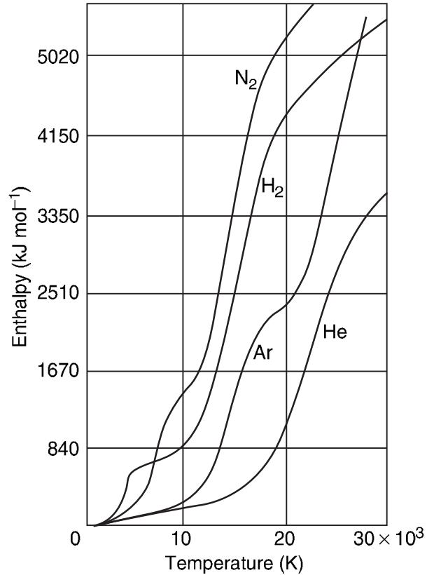
4.2 Gas enthalpy as a function of temperature (Tusek, 2000).
