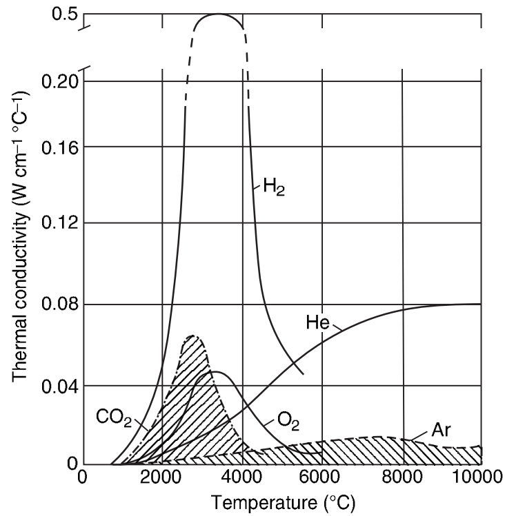
4.1 Thermal conductivity of gases as a function of temperature (Tusek, 2000).
