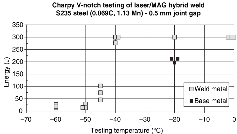
8.3 Charpy V-notch transition curve for the 0.5 mm gap weld made in 12 mm S235 structural steel. The maximum energy of the testing equipment is 300 J.
