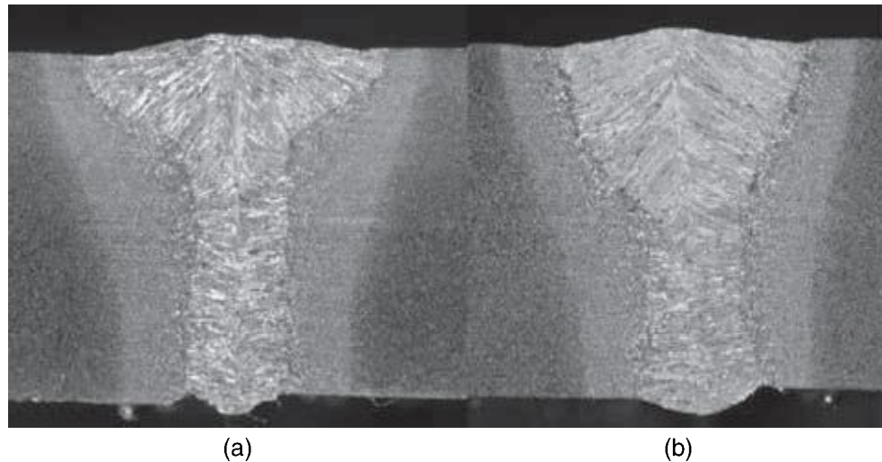
5.2 The effect of the shielding gas \text{CO}_2 content on the width of the penetration profile: (a) 0%, (b) 10%. Air gap 0.8 mm (Fellman et al. 2003).
