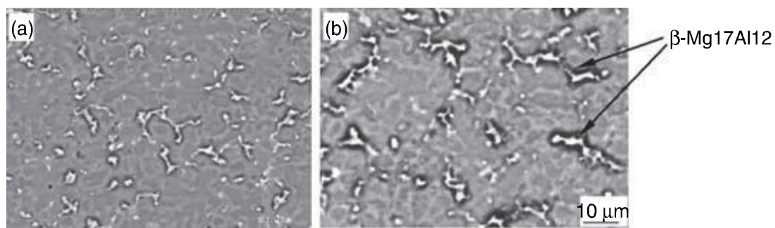
7.14 Back scattering electron image of weld metal 29 (a) dissimilar weld of AZ61 to AZ31, (b) dissimilar weld of AZ91 to AZ31.
