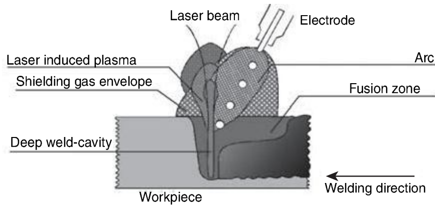
9.1 Schematic representation: laser-hybrid welding.
