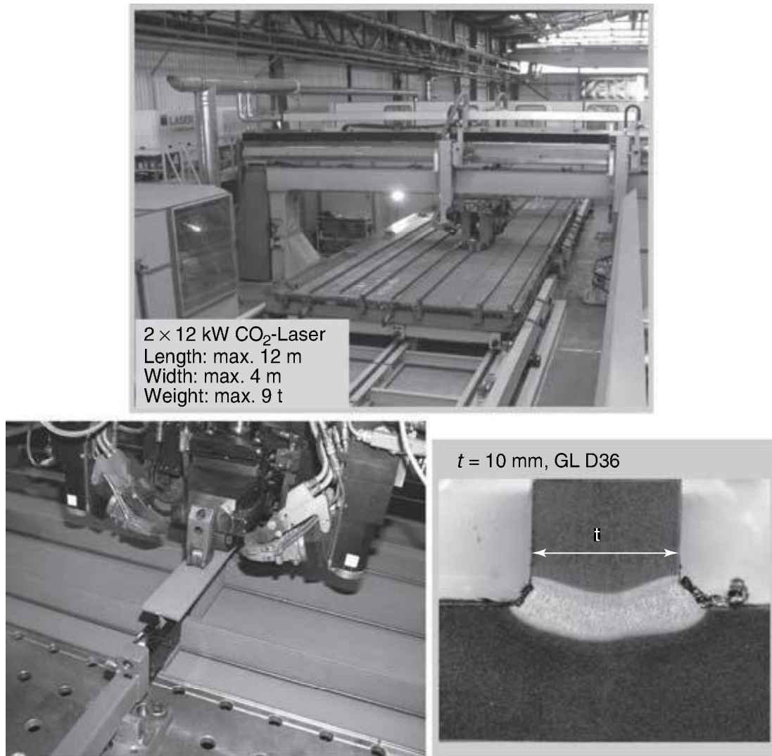
8.8 An overview of the installation as well as a T-joint welding head and cross section (Courtesy: Jens Keil, Blohm + Voss).
