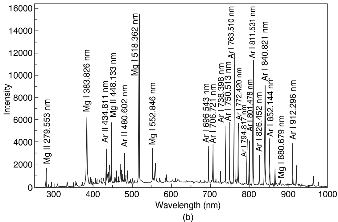
7.37 Spectra of (a) TIG welding plasma and (b) hybrid welding plasma.
