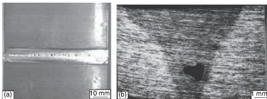
7.22 Micrographs of AZ31B weld joint: 27 (a) the top view of weld; (b) the cross-section of weld.
