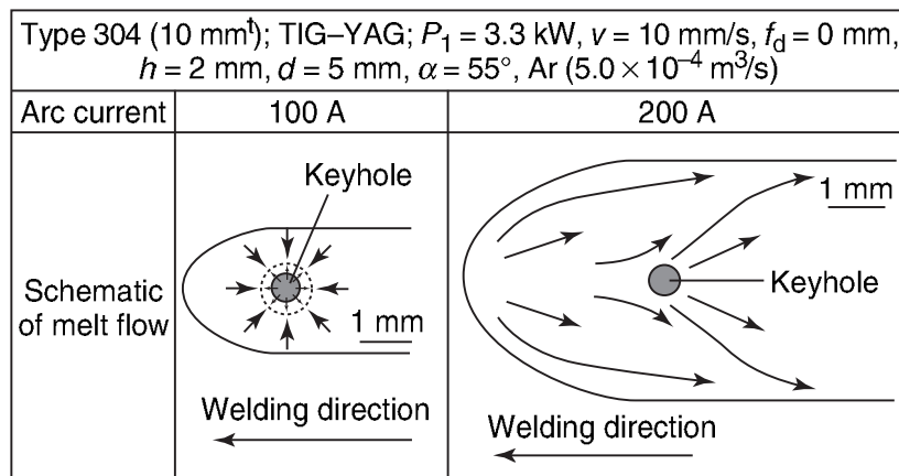
2.14 Schematic melt flow patterns on molten pool surface during hybrid TIG–YAG laser welding at 100 A and 200 A.
