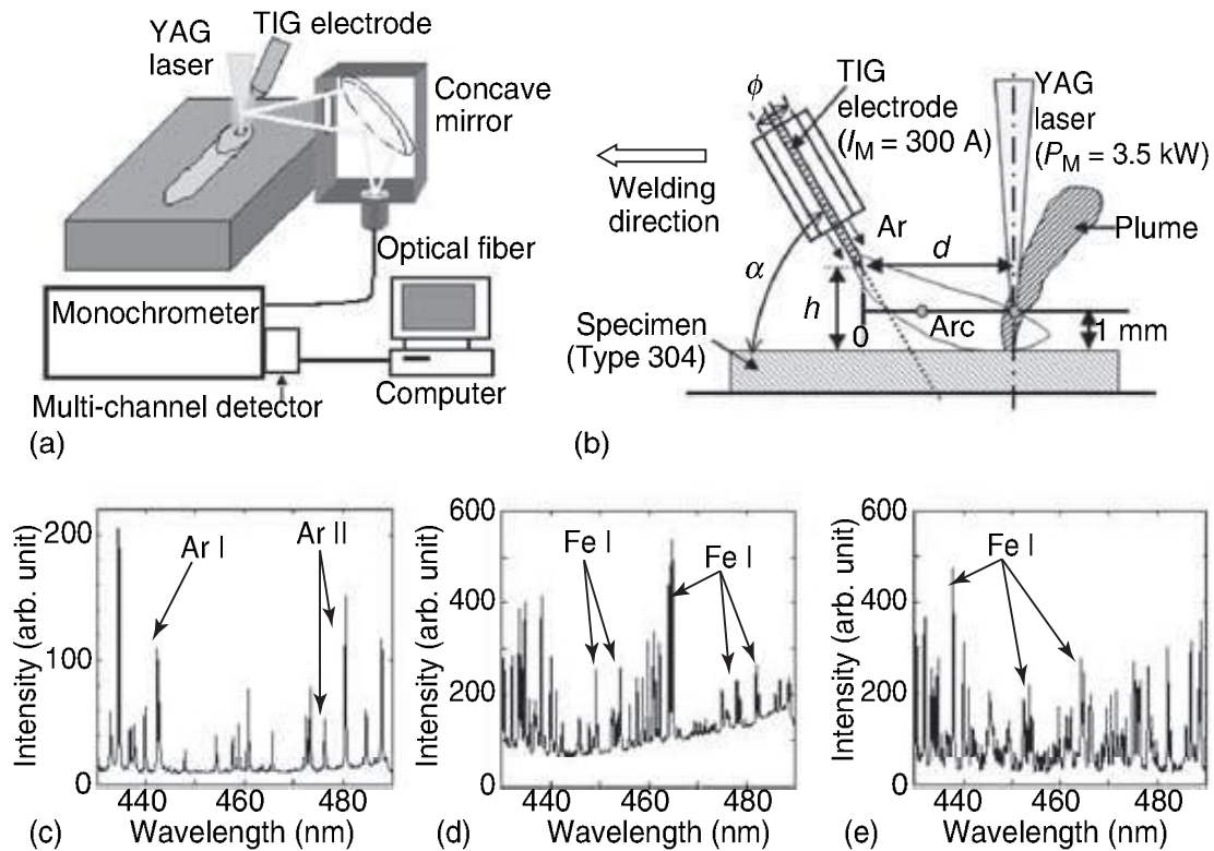
2.2 Schematic arrangement for spectroscopic analyses of plume and/or plasma formed during welding, measurement locations and results during TIG, YAG laser and hybrid TIG–YAG laser welding.
