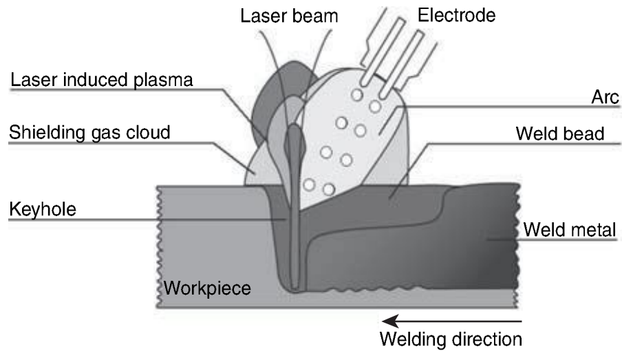
9.10 Schematic outline: laser-hybrid-tandem welding.
