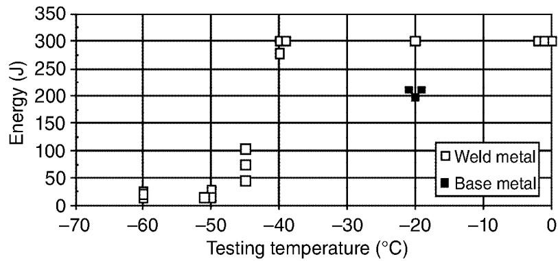
5.16 Charpy V-notch transition curve for the 0.5 mm gap weld made in 12 mm S235 structural steel. The maximum energy of the testing equipment is 300 J (Kristensen, 2007).
