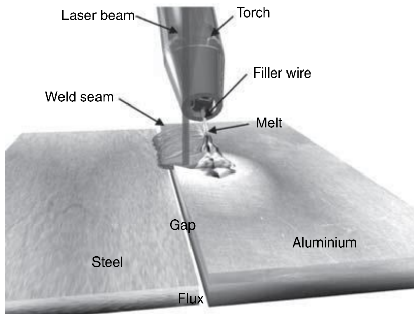
11.3 Principle of the laser MIG hybrid joining process.
