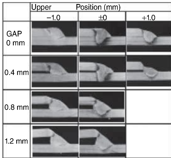
12.5 Effect of welding location on weldability of lap fillet sheets with gap, and process window for sound weld bead formation.
