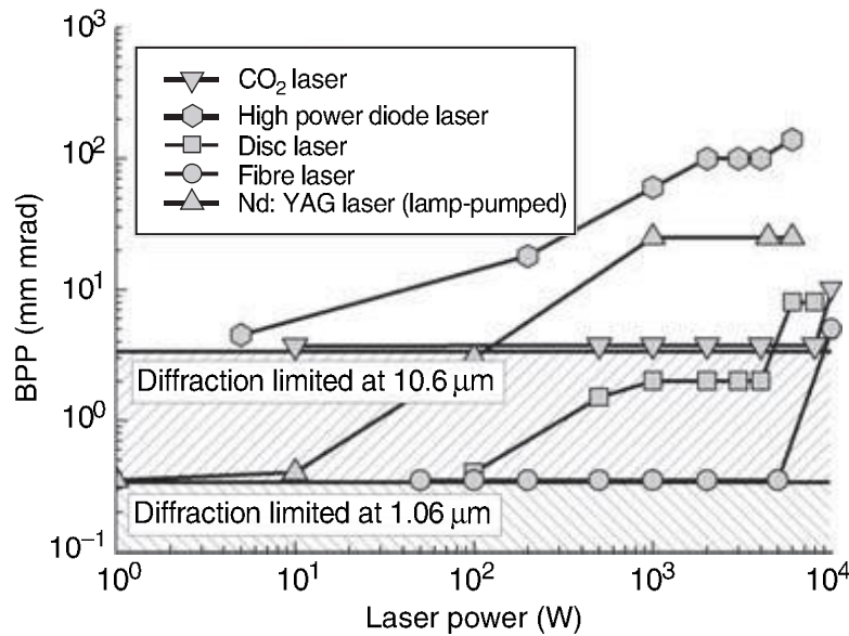
3.5 Characteristic beam parameter products (BPP) vs. laser power for different laser types.
