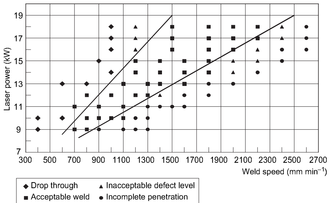
6.2 Weldability lobe for a 0.10%C–1.5%Mn–0.004%S–0.011%P grade S 355 TMCR steel. The welds are evaluated with respect to EN ISO 13919-1:1996, level C.
