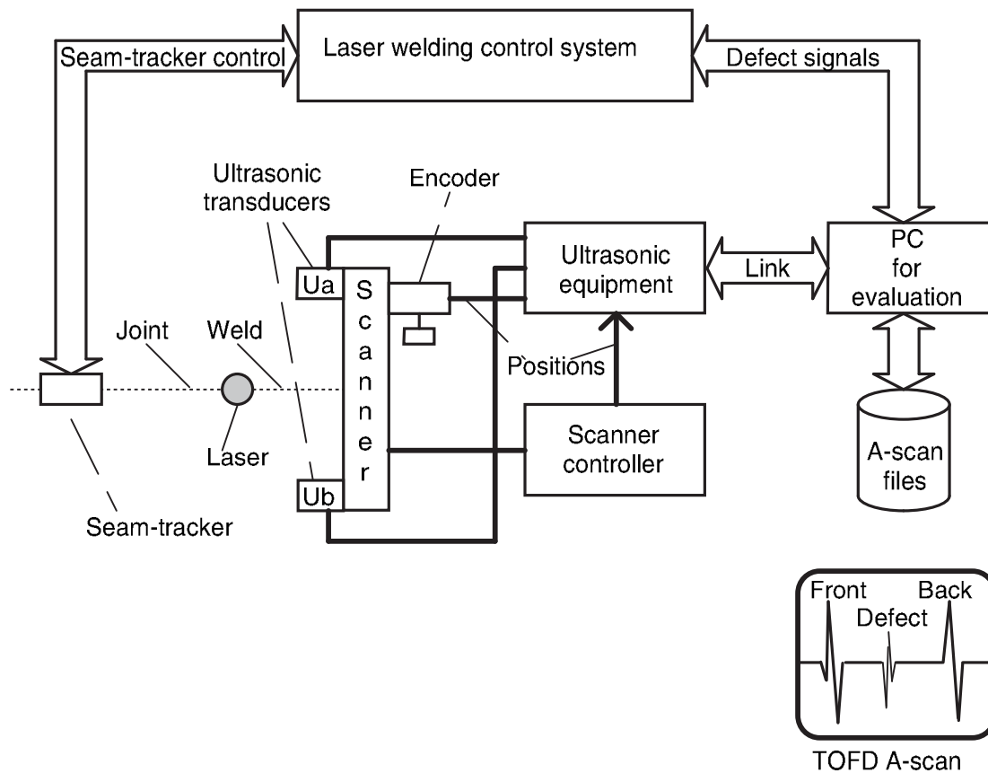
6.4 Defect detection using ultrasonic NDT.
