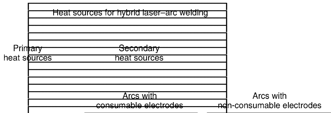
3.12 Schematic presentation of heat sources available for hybrid laser–arc combinations.
