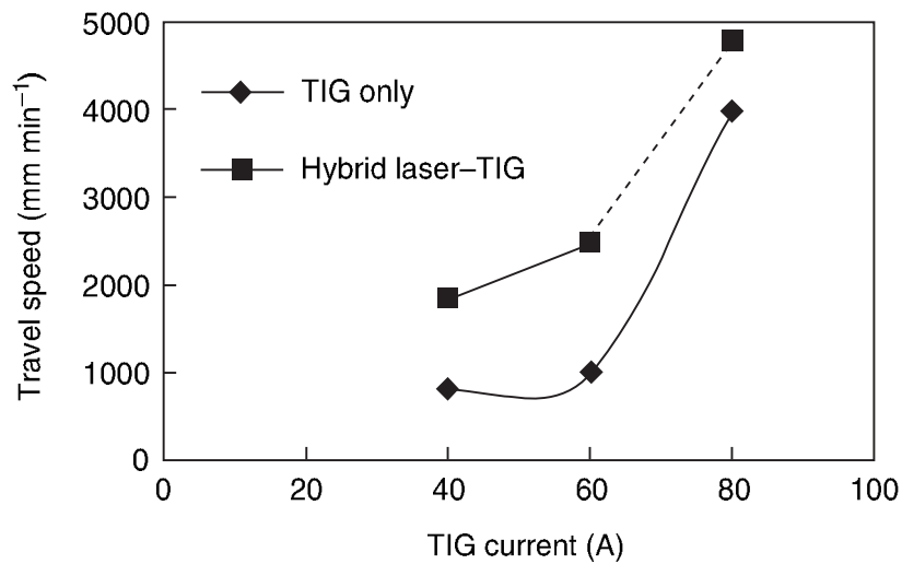
7.6 Stability of hybrid laser–TIG welding and TIG at various travel speed as a function of TIG current. 31
