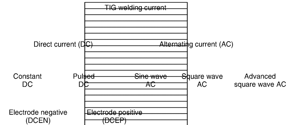
3.10 Schematic presentation of the common TIG welding process variants.
