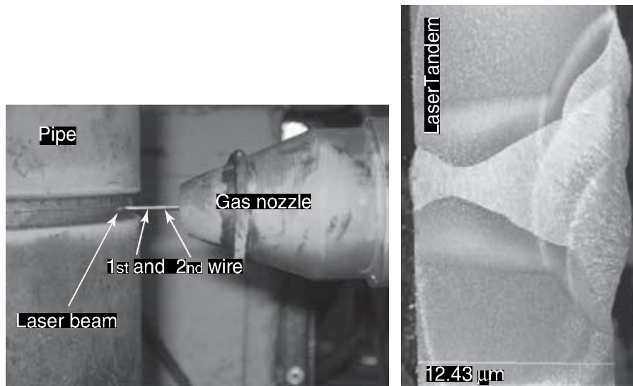
9.13 (a) Welding of a pipe in the position 2G with LaserTandem and (b) macrosection of the welded pipe (Courtesy: Fronius).
