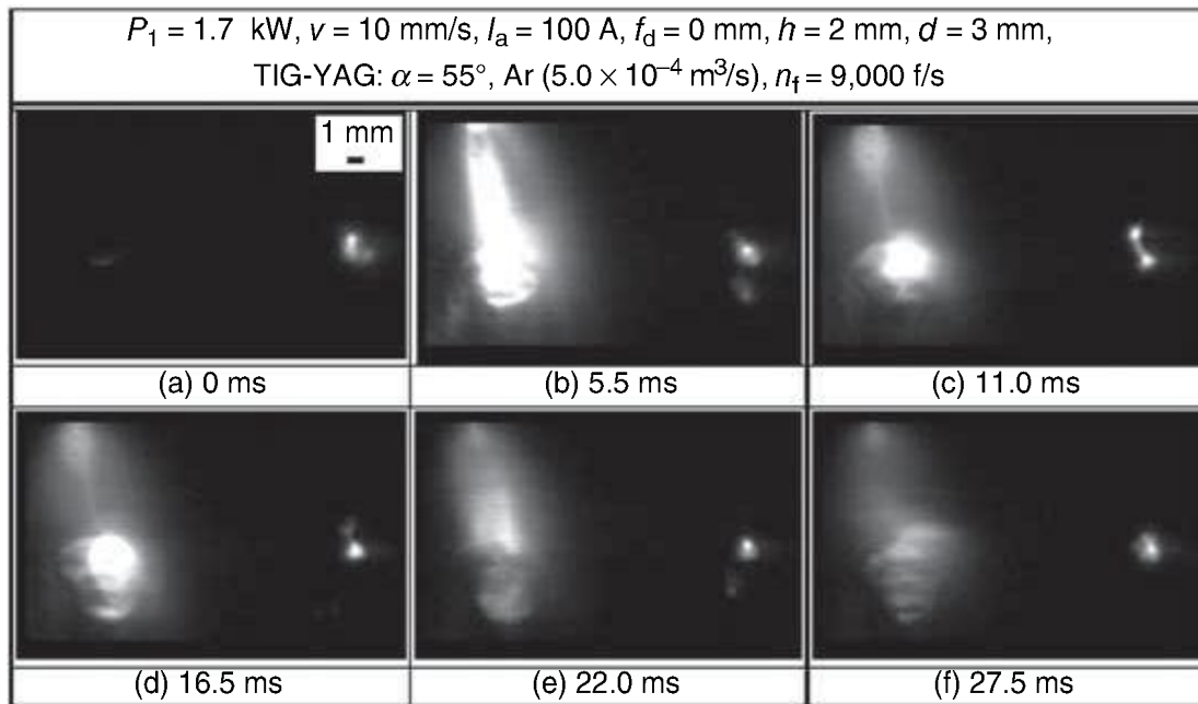
2.7 Simultaneous observation results of TIG arc and reflected laser beam during hybrid TIG–YAG laser welding of Type 304 steel.
