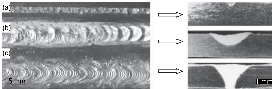
7.2 Comparison of welded joints and macrosections 28 (a) laser welding (b) TIG welding (c) hybrid welding.
