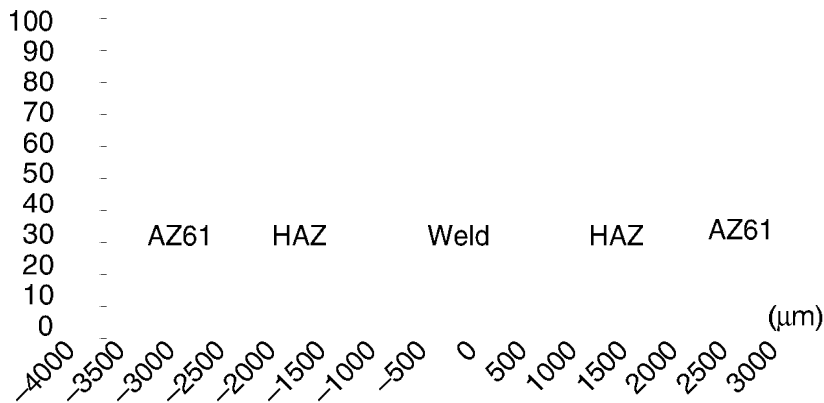
7.20 Hardness profile in the weld of AZ61 to AZ31. 29
