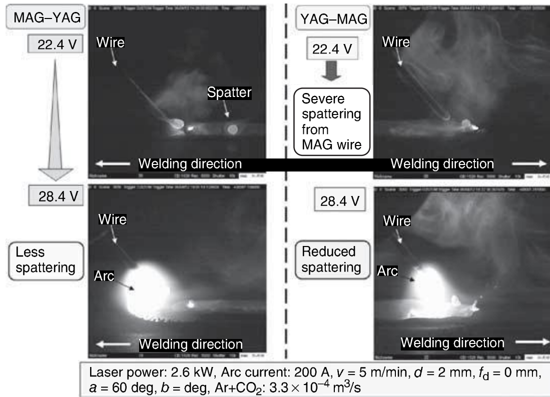
2.10 Arc and droplet behavior during hybrid YAG laser–MAG or MAG–YAG laser welding of steel at low and high voltages.
