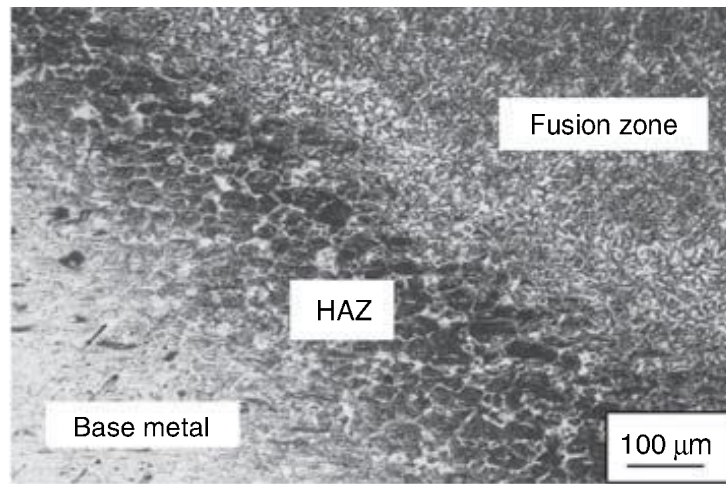
7.11 Microstructure of welded joint by TIG 28 ( I_{\text{arc}} = 60 \text{ A} , V = 500 \text{ mm min}^{-1} ).
