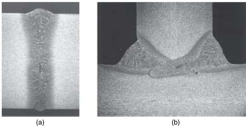
6.1 Solidification flaws in hybrid laser-arc welded structural steels: (a) an I-butt 15 mm butt weld and (b) a T-joint in 12 mm plate thickness.
