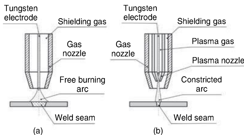
3.11 Schematic diagram of a plasma torch used for (a) tungsten inert gas welding compared with (b) a torch used for plasma arc welding.
