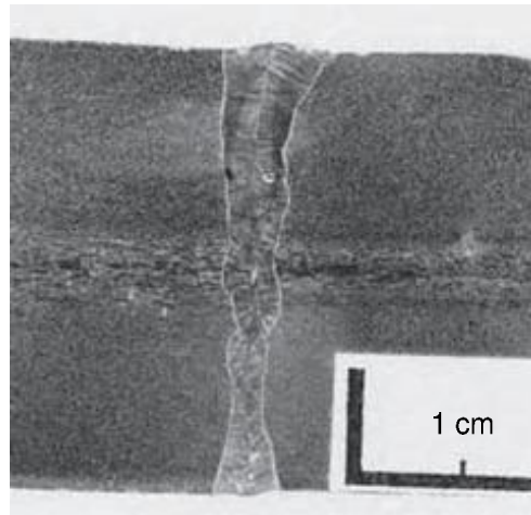
5.5 Cross-section of the hybrid weld with thickness of 20 mm filled with 4 passes. Groove angle 10^\circ , welding speed 0.5\text{--}0.7\text{ m min}^{-1} , wire feeding rate 9.7\text{ m min}^{-1} (Jokinen et al. 2002).
