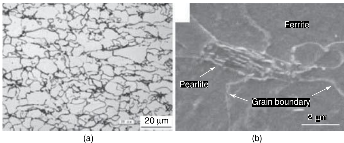
5.3 Micrographs of base metal observed by (a) optical microscopy and (b) SEM (Liu et al. 2006).
