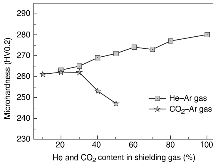
4.16 Effects of shielding gas on microhardness of hybrid CO 2 laser–MAG welded mild steel with 7 mm thickness.
