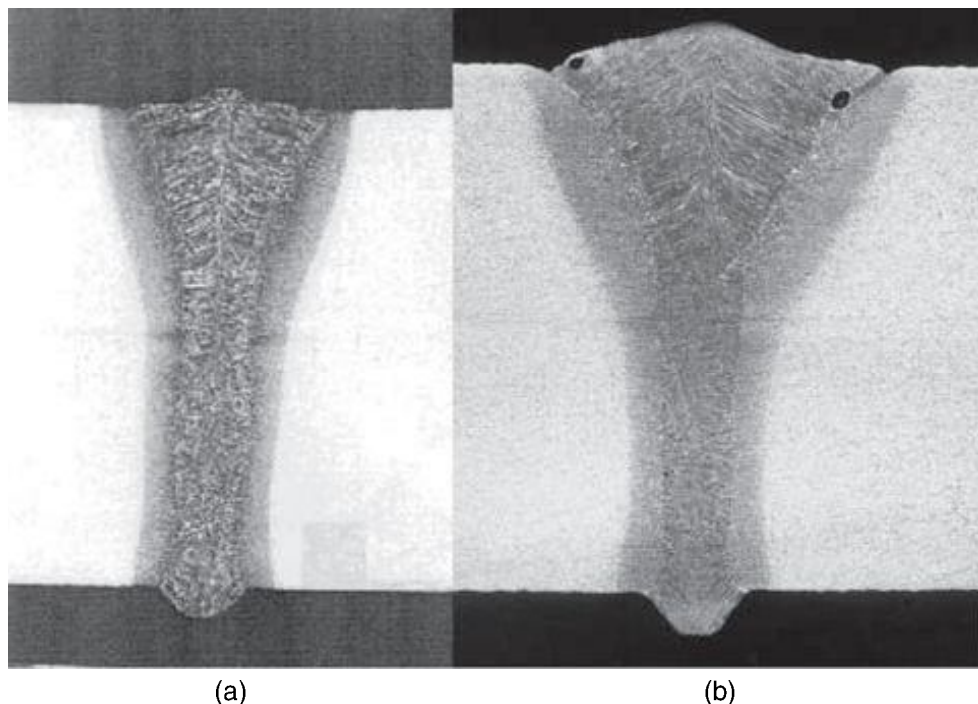
5.1 Cross-section in 12 mm structural steel of: (a) a pure laser weld (laser peak power at wp 9 kW, speed 0.8 m/min and zero gap); and (b) a hybrid MAG–laser weld (laser power at 11 kW, arc power 7.0 kW, speed) 1.4 m min -1 , wire feed speed 15.8 m min -1 and gap 0.5 mm (Kristensen, 2007).
