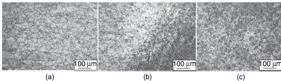
7.10 Microstructure of welded joint by hybrid welding 28 (a) base metal, (b) transition zone, (c) bond area.
