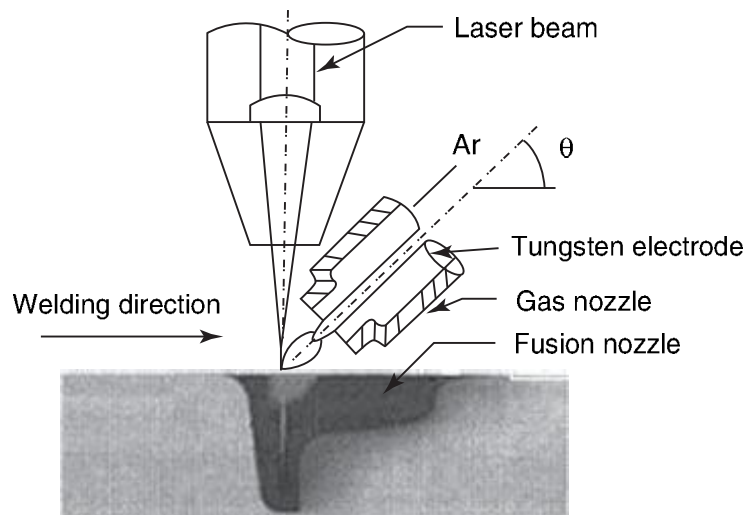
7.1 Schematic diagram of low-power laser–arc hybrid welding. 27
