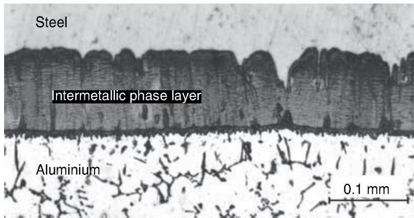
11.1 Example of an intermetallic phase layer in an inadequate aluminium–steel joint.
