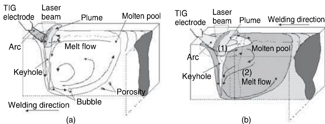
2.19 Schematic welding phenomena during hybrid TIG–YAG laser welding at (a) 100 and (b) 200 A, showing melt flows, bubble and porosity formation or no porosity.
