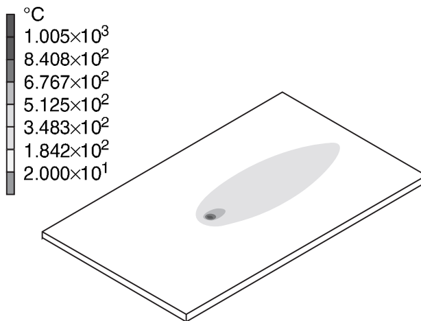
7.32 Temperature distribution of hybrid butt-welding at quasi-stable state. 36
