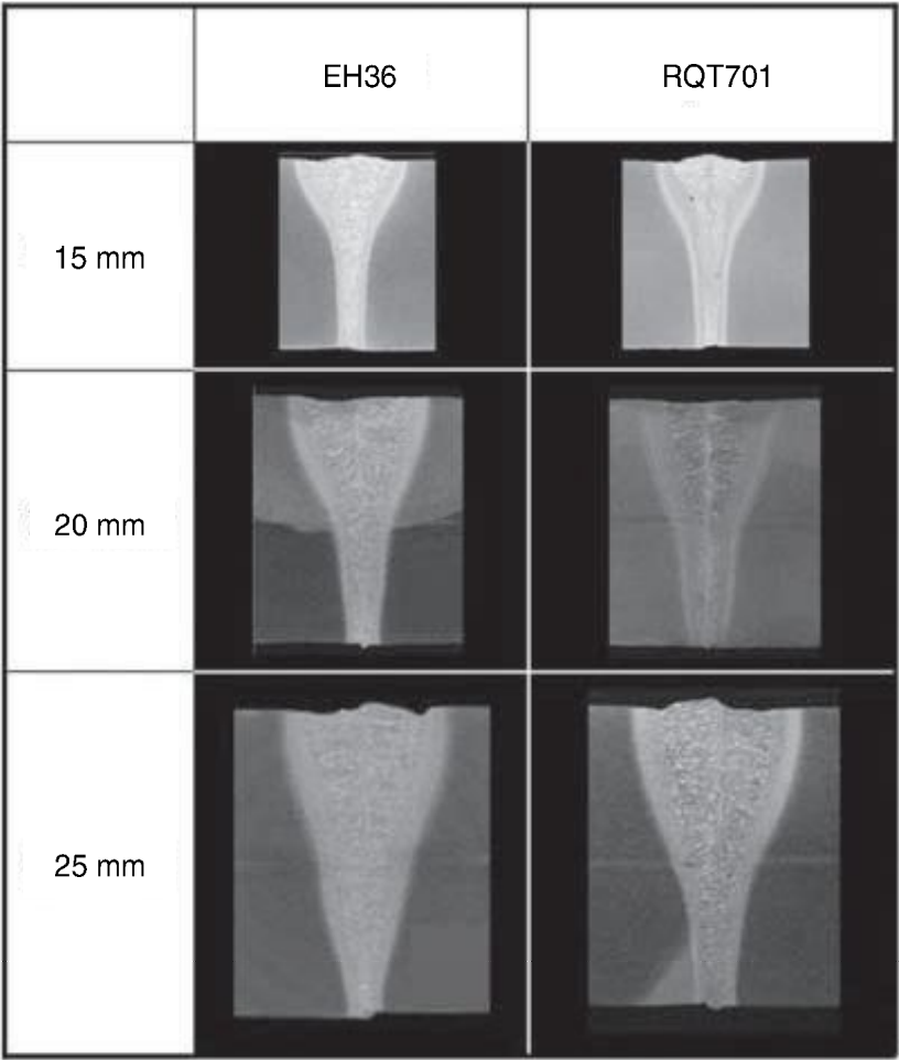
12.8 Cross-sections of optimized hybrid welds.
