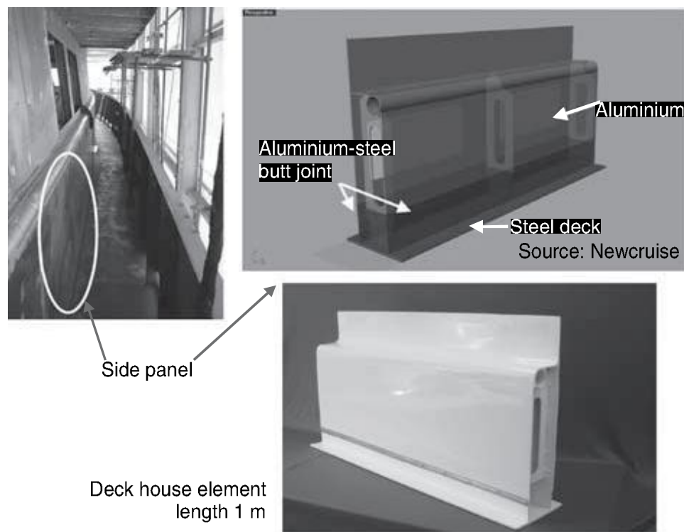
11.18 Concept for aluminium–steel in yacht construction and yacht deckhouse element produced accordingly (length: 1 m, material thickness: 3 mm).
