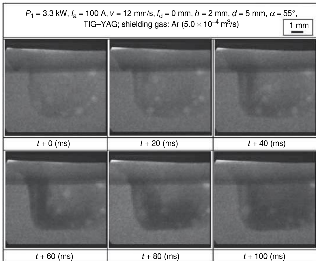
2.15 X-ray transmission observation results during hybrid welding with Ar gas at 100 A in air, showing diffusion of Pt inside molten pool.
