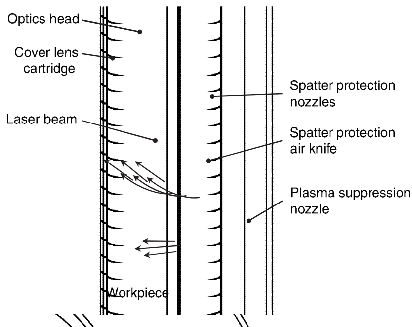
1.4 Sketch of a laser welding head with multiple gas assist.
