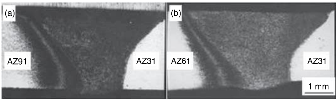
7.4 Cross-section of laser-TIG hybrid welded magnesium alloys 29 (a) dissimilar weld of AZ91 to AZ31; (b) dissimilar weld of AZ61 to AZ31.
