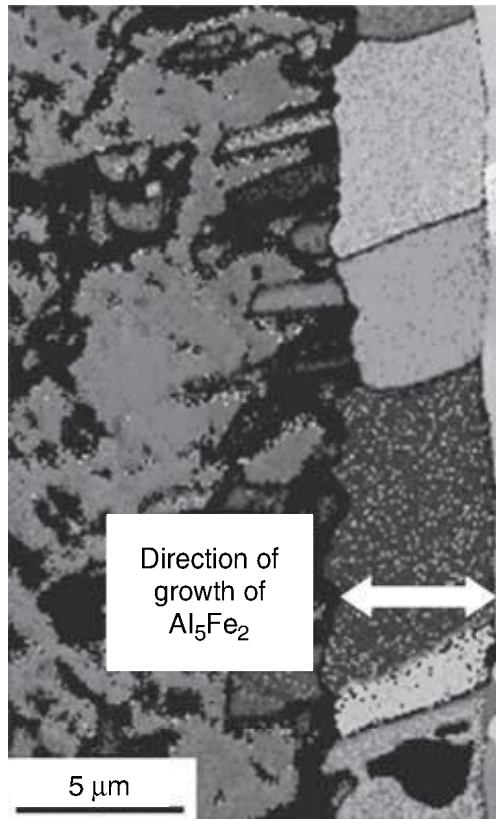
11.7 Orientation of the grains in the joining zone [aluminium EN AW-6056 (thickness 3.8 mm); steel THM 180BH + Z (thickness 1.95 mm)] (Courtesy: MPIE, Düsseldorf).
