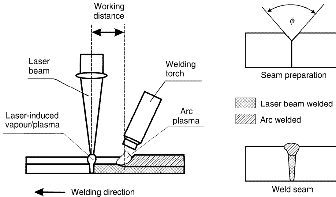
3.15 Schematic diagram of hybrid laser–arc welding with separate operation points.
