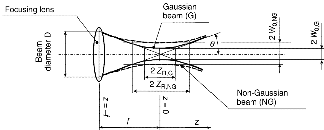
3.2 Beam propagation of a Gaussian and a non-Gaussian beam after focusing through a lens.
