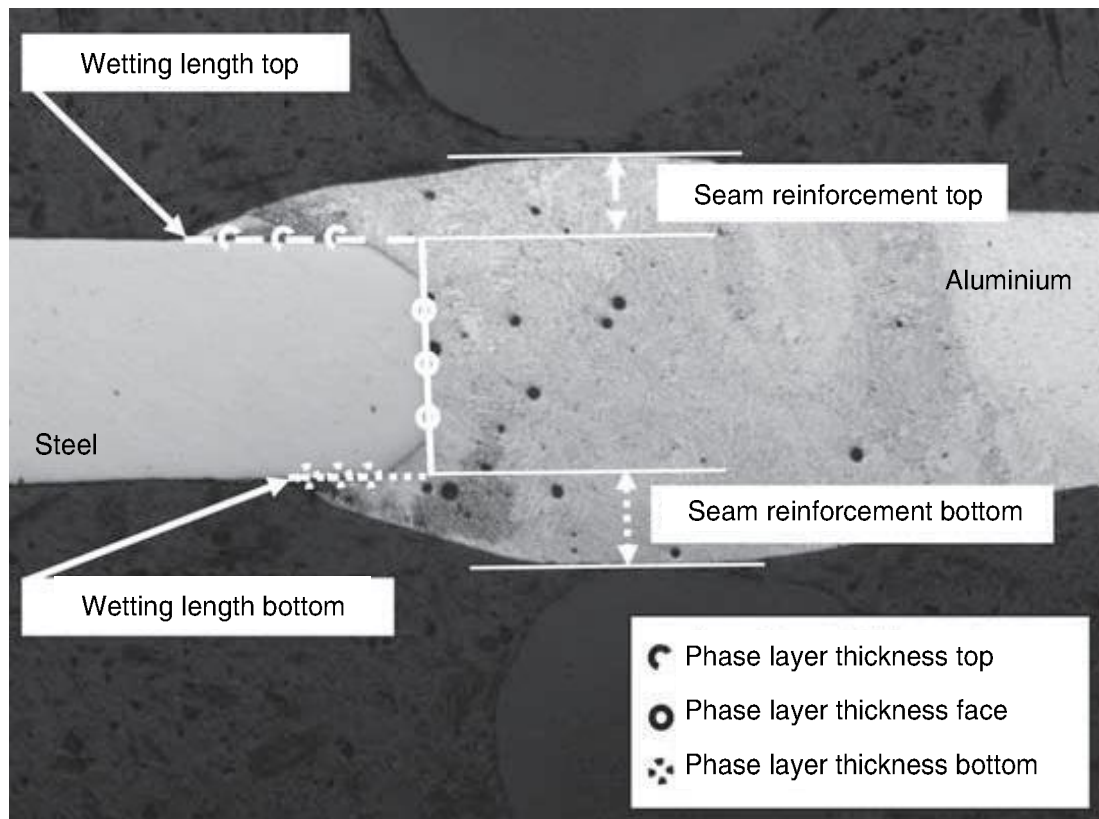
11.8 Micro-geometrical parameters for seam assessment.
