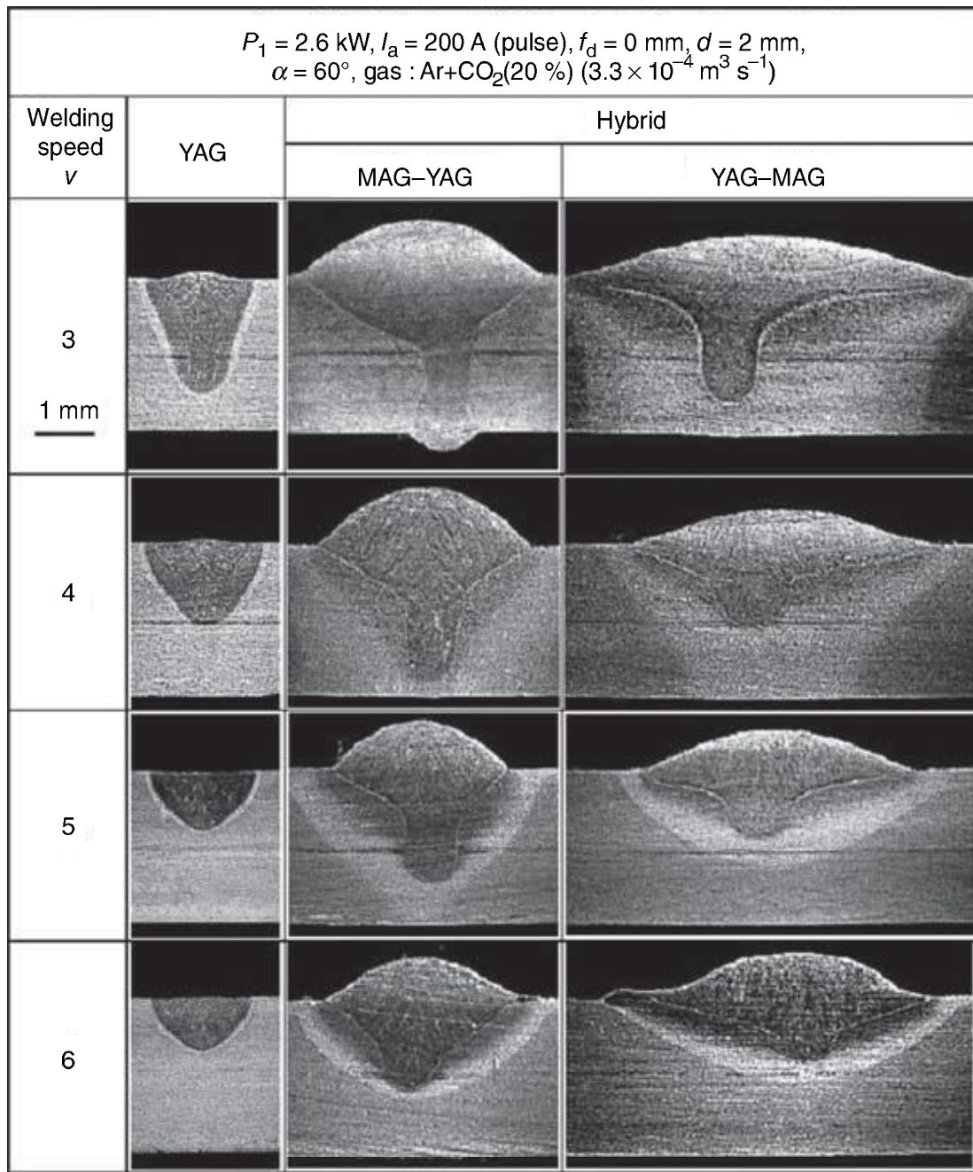
12.1 Cross-sections of weld beads produced by YAG laser, hybrid MAG–YAG laser and hybrid YAG laser–MAG welding at various traveling speeds.
