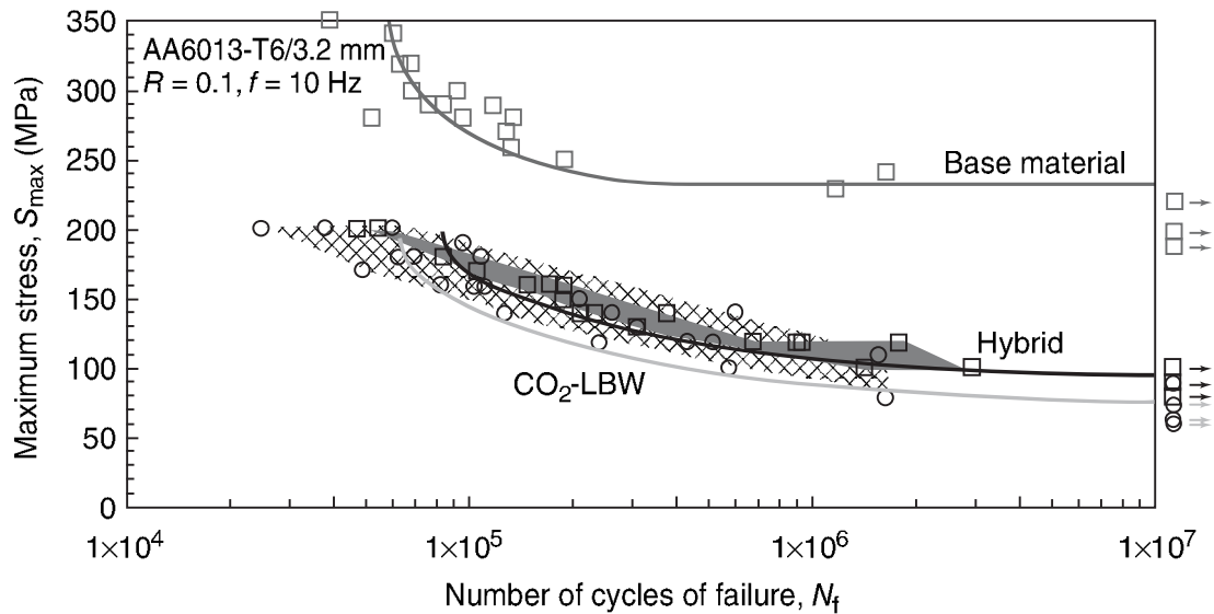
5.20 Comparative fatigue behaviour of the CO 2 laser beam weld and the hybrid weld in a 3.2 mm thick AA6013 sheet butt-welded in T6. Run-outs (i.e., unbroken specimens) are indicated by arrows (Vaidyaa, 2006).
