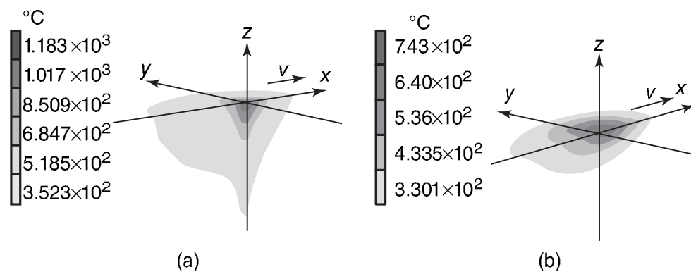
7.30 Heat source model of hybrid welding. 36 (a) The effect between laser and arc is considered; (b) The effect between laser and arc is not considered.
