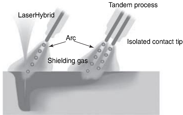
9.15 Schematic outline: LaserHybrid + tandem welding.
