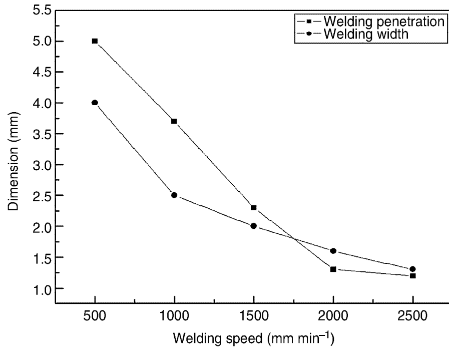
7.8 Influence of welding speed on welding quality ( I = 120 A, P = 300 W).
