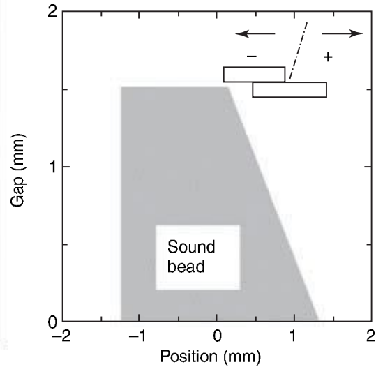
12.5 Effect of welding location on weldability of lap fillet sheets with gap, and process window for sound weld bead formation.
