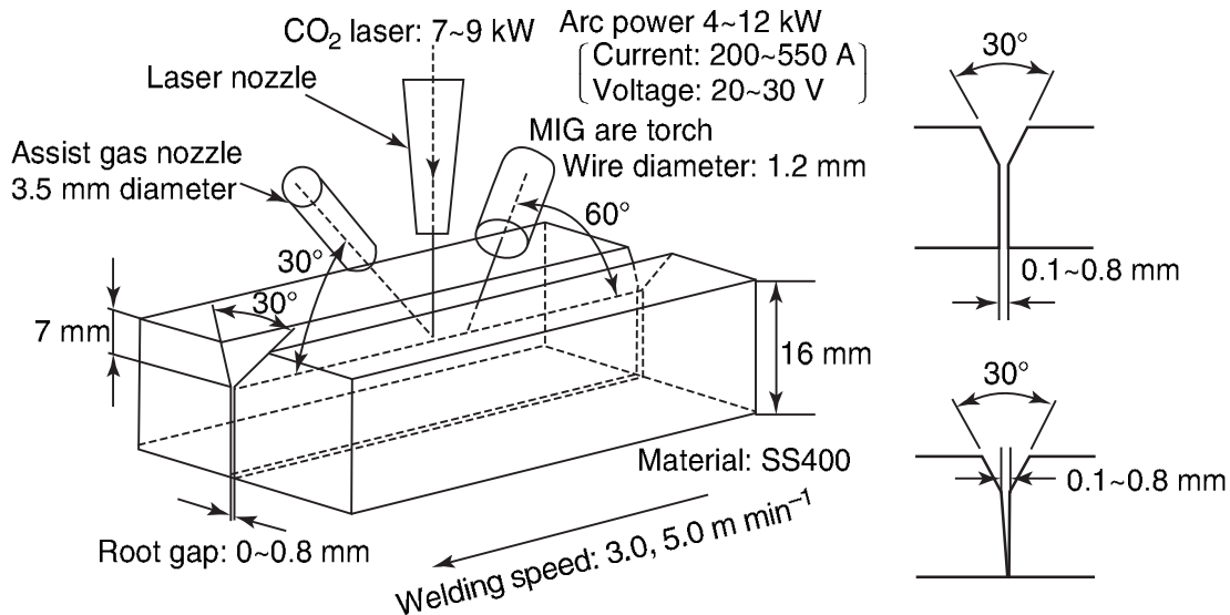
12.7 Schematic representation of LPLAC (leading path laser-arc combination) method.
