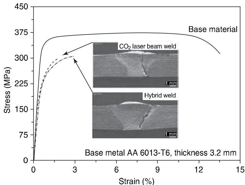
10.17 Tensile curves and the fracture location in the CO 2 laser beam weld and the hybrid weld in a 3.2 mm thick AA6013 sheet butt-welded in T6. The fracture is restricted to the weld (Vaidya et al. , 2006).
