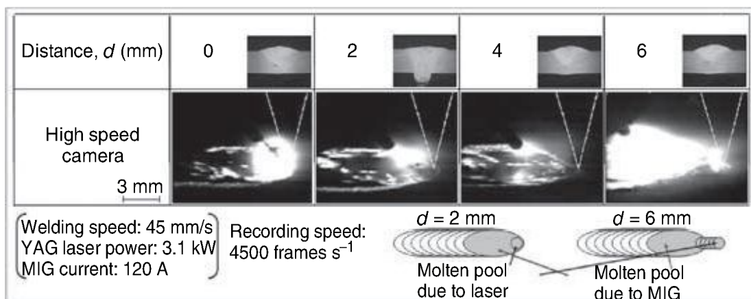
2.9 Cross sections of A5052 welds obtained by hybrid YAG laser-pulsed MIH welding with A5356 wire and welding phenomena, showing effect of target distance between wire and laser beam ( d ) on penetration.
