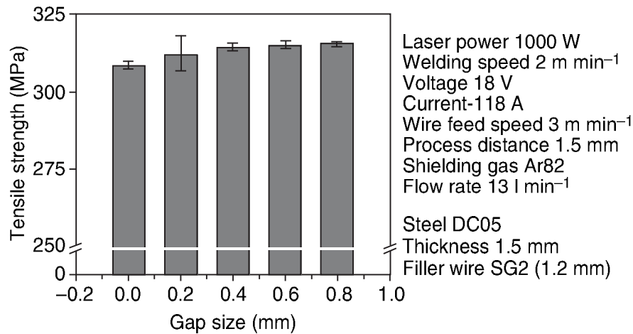
5.14 Effect of gap on tensile strength (Thomy et al. 2007).
