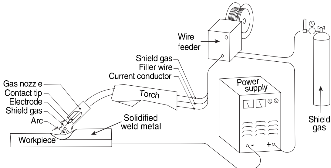
1.1 Schematic of a typical gas metal arc weld (GMAW) set up (not to scale).
