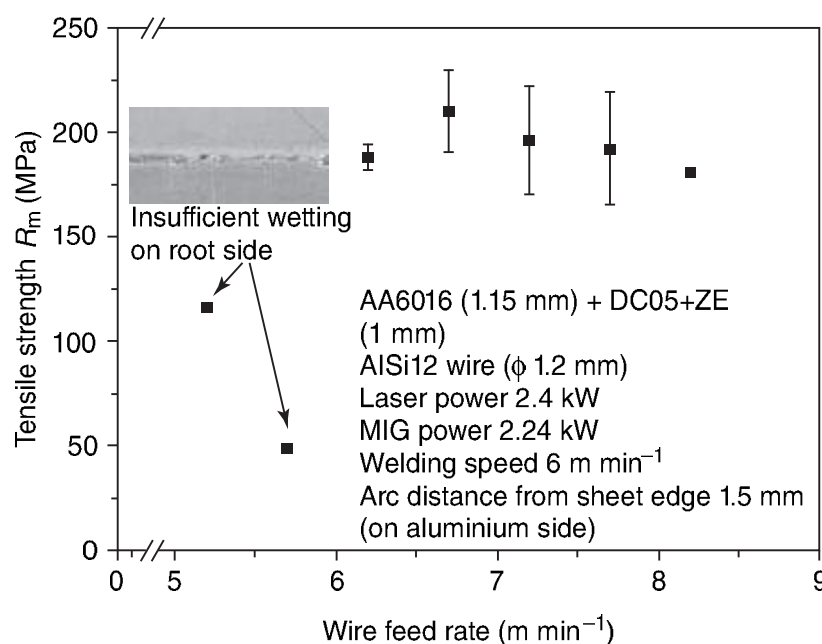
11.10 Effect of wire feed rate on tensile strength in laser–MIG hybrid welding.
