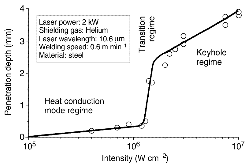
3.4 Penetration depth versus intensity for laser beam welding processes.
