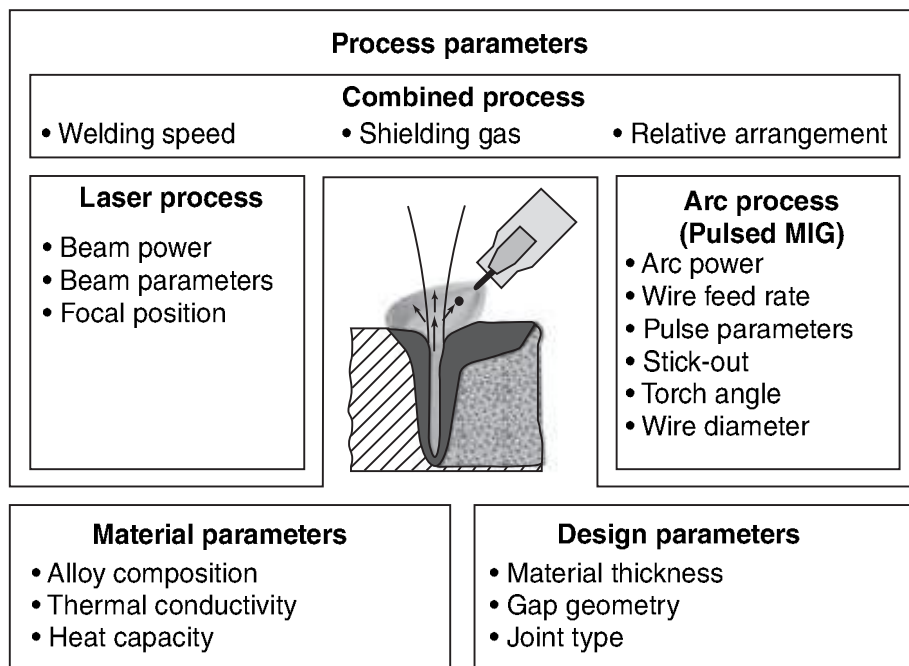
10.7 Governing parameters in Nd:YAG laser MIG hybrid welding (not exhaustive).
