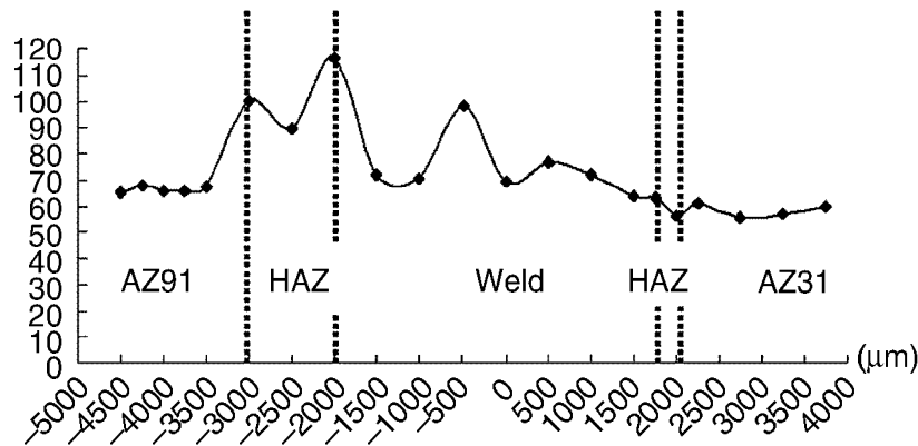
7.21 Hardness profile in the weld of AZ91 to AZ31. 29
