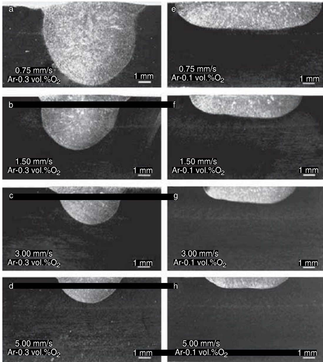
4.4 The effects of oxygen content in Ar–O 2 mixture on weld shape of TIG welds.
