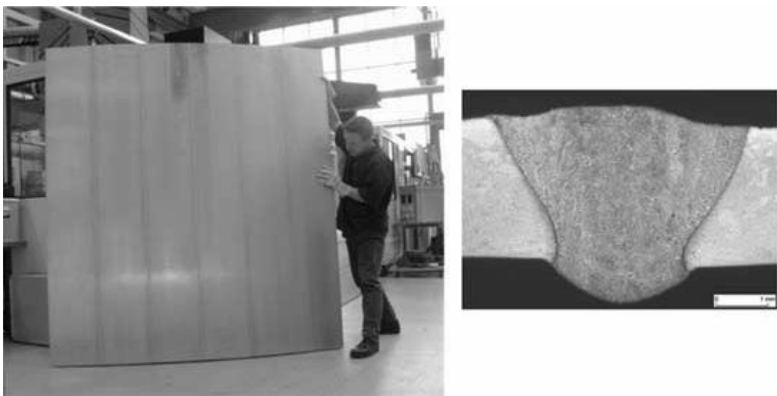
10.19 Roof segment of the ICE train/cross-section of the weld.
