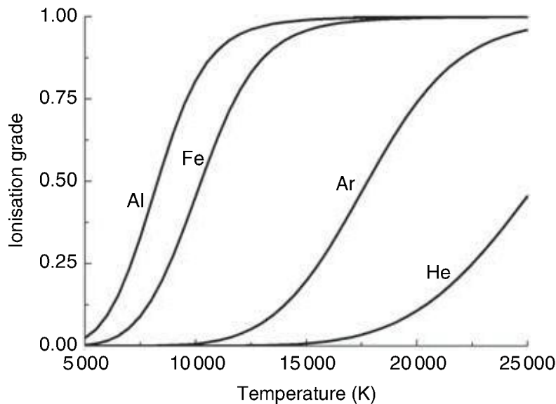
3.6 Ionisation grade vs. temperature of typical elements present in the welding zone.
