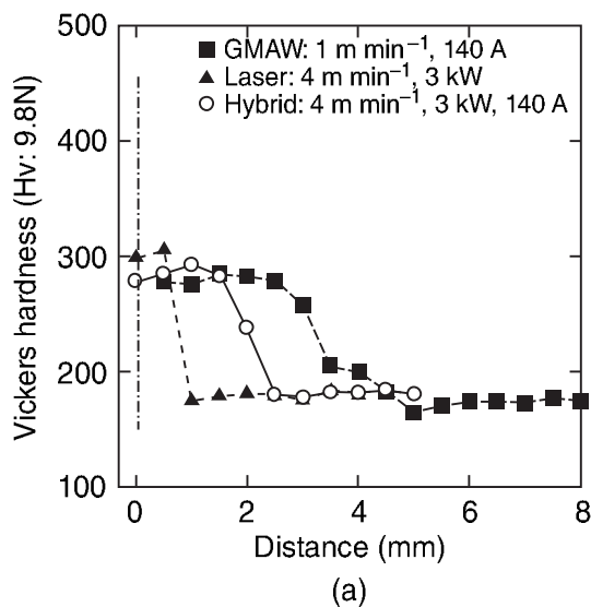
12.6 Comparison of hardness profiles across welds produced by different processes: (a) 590 MPa steel; (b) 980 MPa steel.
