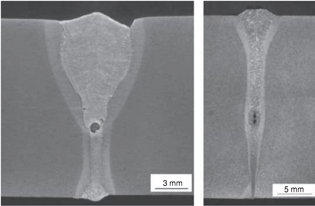
12.9 Examples of porosity (a) and pore or crack (b) in hybrid weld beads.
