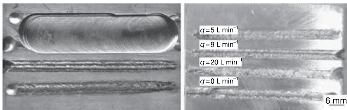
7.25 Number of pores in weld metal using laser coaxial shielding. 27
