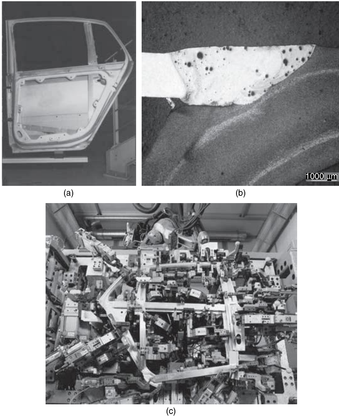
9.3 Laser-hybrid welded door, macro section and clamping device of the VW Phaeton.
