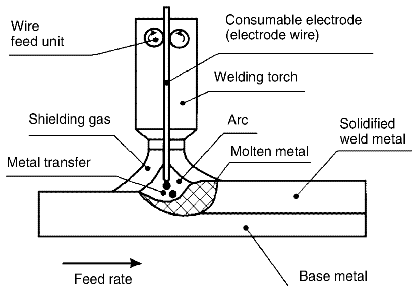
3.7 Schematic diagram of gas–metal arc welding with consumable electrode.
