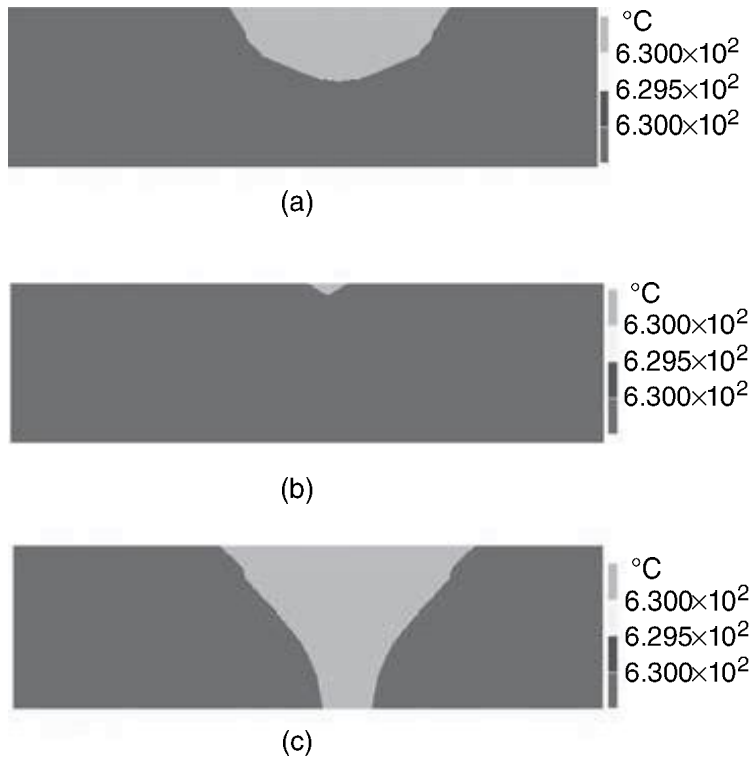
7.31 Numerical simulation of weld joints. (a) TIG welding alone; (b) Laser welding alone; and (c) Hybrid welding.
