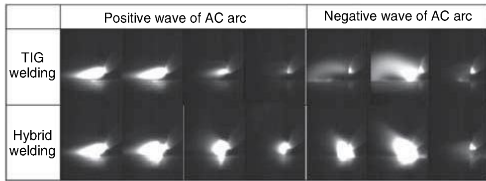
7.27 Plasma behavior in the welding process of magnesium alloy. 33
