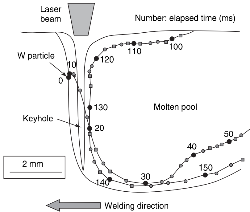
2.16 Motion of W particle observed during hybrid welding with Ar gas at 100 A in air, showing melt flows inside molten pool.
