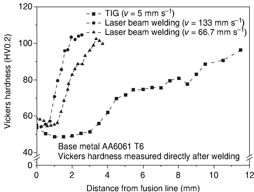
10.2 Hardness distributions in welded specimens of alloy AA 6061 T6 directly after welding for laser beam welding and TIG welding at different welding speeds (Hirose, 1999).
