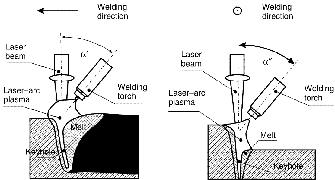
3.14 Schematic diagrams of hybrid laser–arc welding with a common operation point.
