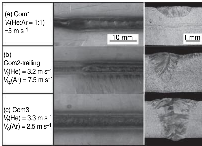
4.12 Effects of gas nozzle arrangement on weld surface and cross-section shape in hybrid CO 2 laser–TIG welding, 316L stainless steel with 3 mm thickness.
