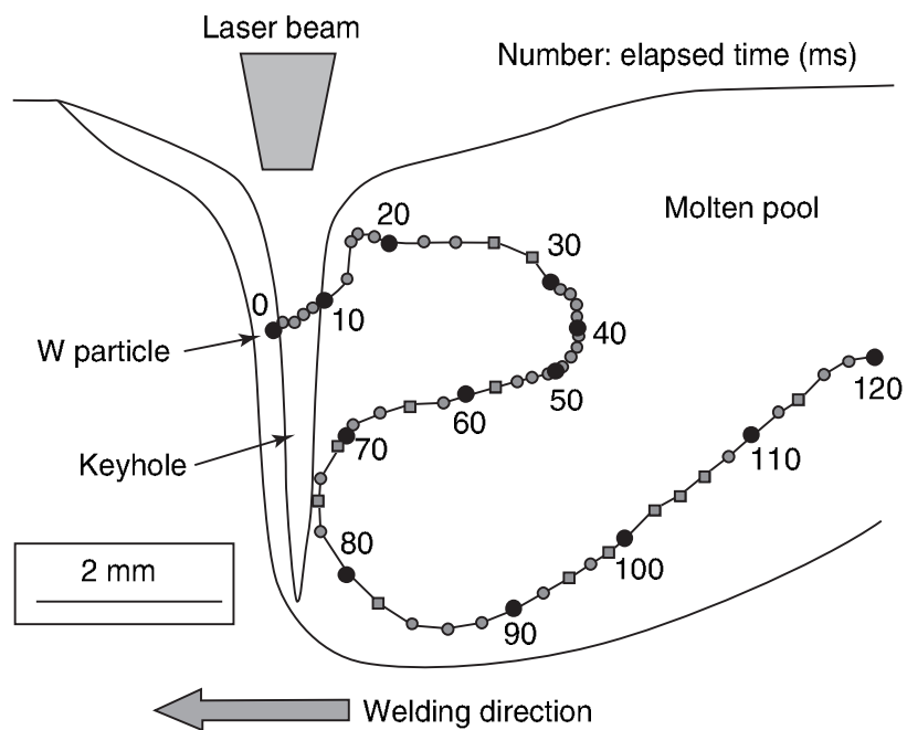
2.17 Motion of W particle observed during hybrid welding with Ar gas at 100 A in air, showing melt flows inside molten pool.
