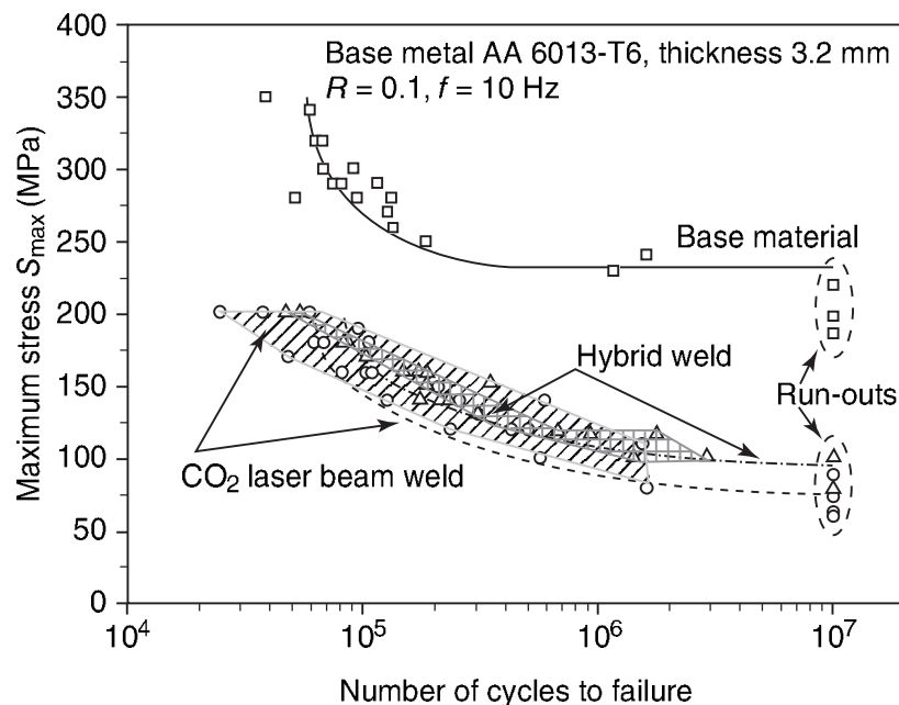
10.18 Comparative fatigue behaviour of the CO 2 laser beam weld and the hybrid weld in a 3.2 mm thick AA6013 sheet butt-welded in T6 (Vaidya et al. , 2006).
