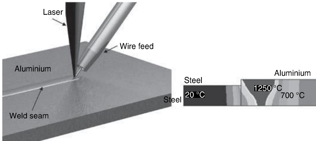
11.2 Process principle and temperature distribution for aluminium–steel butt joints obtained by laser beam welding (Kreimeyer et al. , 2002a).
