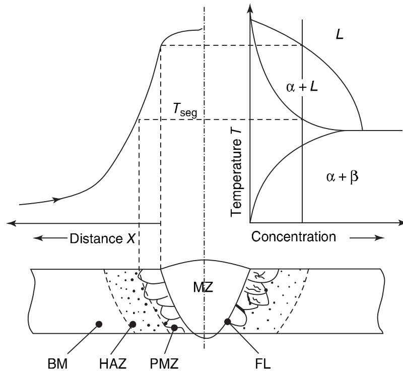
10.1 Schematic illustration of temperature profile, phase diagram and resulting microstructural zones in fusion welding of aluminium alloys: BM base material; HAZ heat-affected zone, PMZ partially melted zone; MZ molten zone; FL fusion line; T_{seg} temperature region for the dissolution of precipitates (Schubert, 2003).
