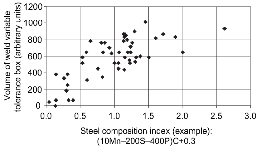
6.3 Weldability with respect to solidification flaw formation as a function of an index developed from the steel composition. The steel composition index shown is one example on a correlation, only.
