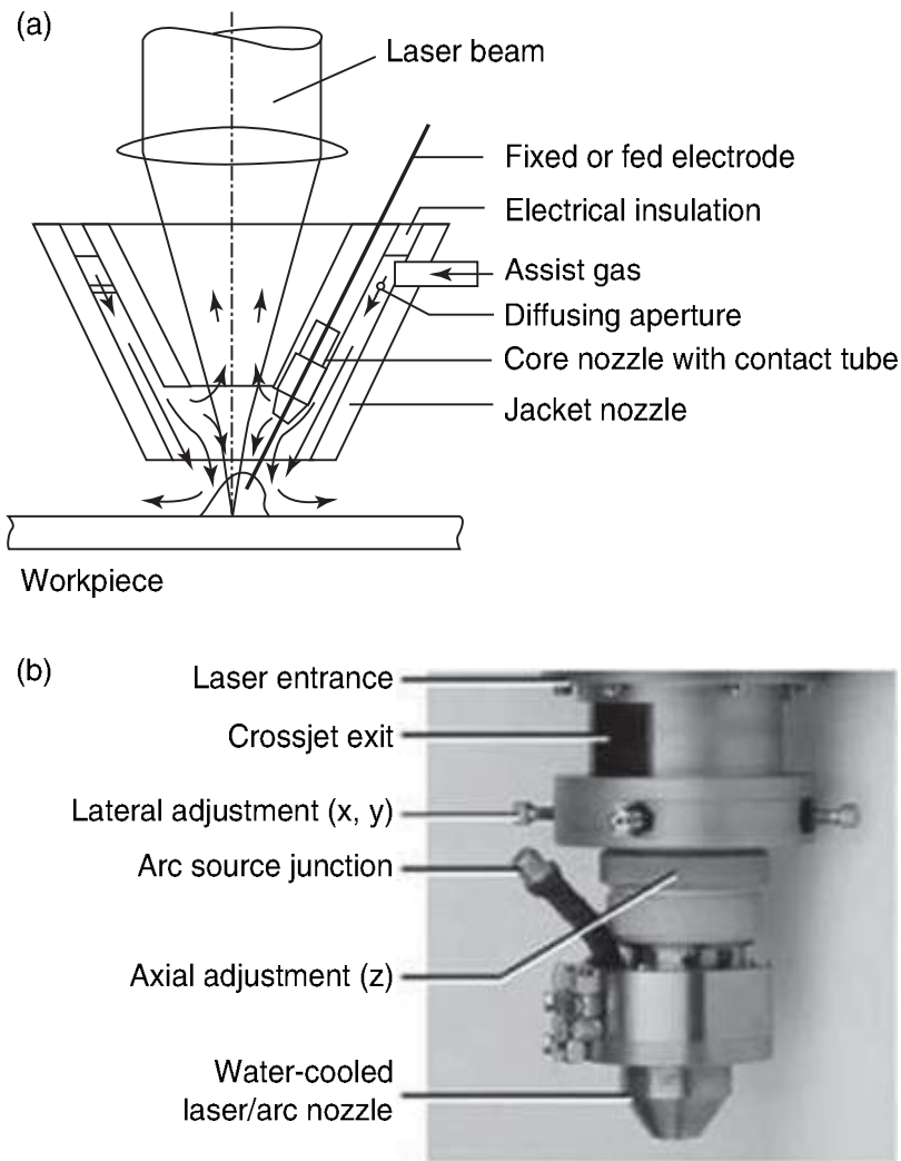
4.14 Schematic diagram (a) and entity (b) of Fraunhofer ILT hybrid welding head.
