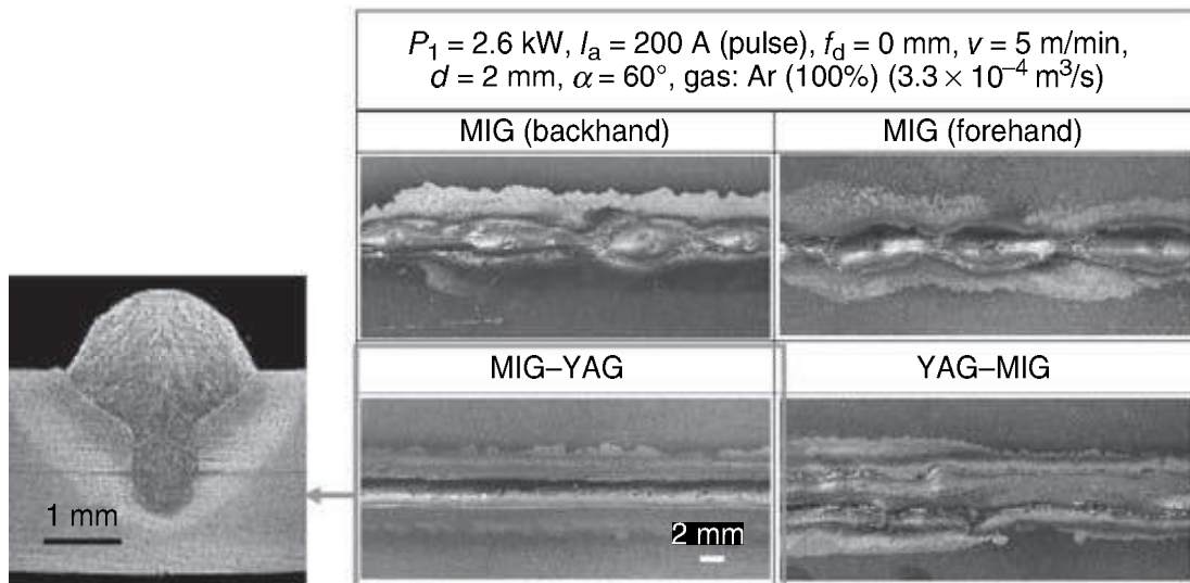
2.11 Comparison of MIG welds and hybrid YAG laser–MIG or MIG–YAG laser welds in steel with Ar gas, and cross section of good weld made by hybrid MIG–YAG laser welding.
