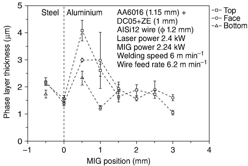
11.11 Effect of MIG position relative to sheet edge on phase layer thickness in laser–MIG hybrid welding.
