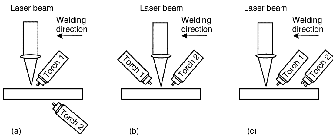
3.16 Schematic diagrams of hybrid laser–arc processes with two secondary heat sources.
