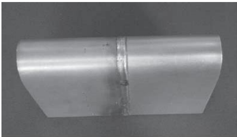
11.14 Cracking of an aluminium–steel specimen (AA6016 (thickness: 1.15 mm) and zinc coated steel DC05 + ZE (thickness: 1 mm)) under tensile load (tensile strength 193 MPa).
