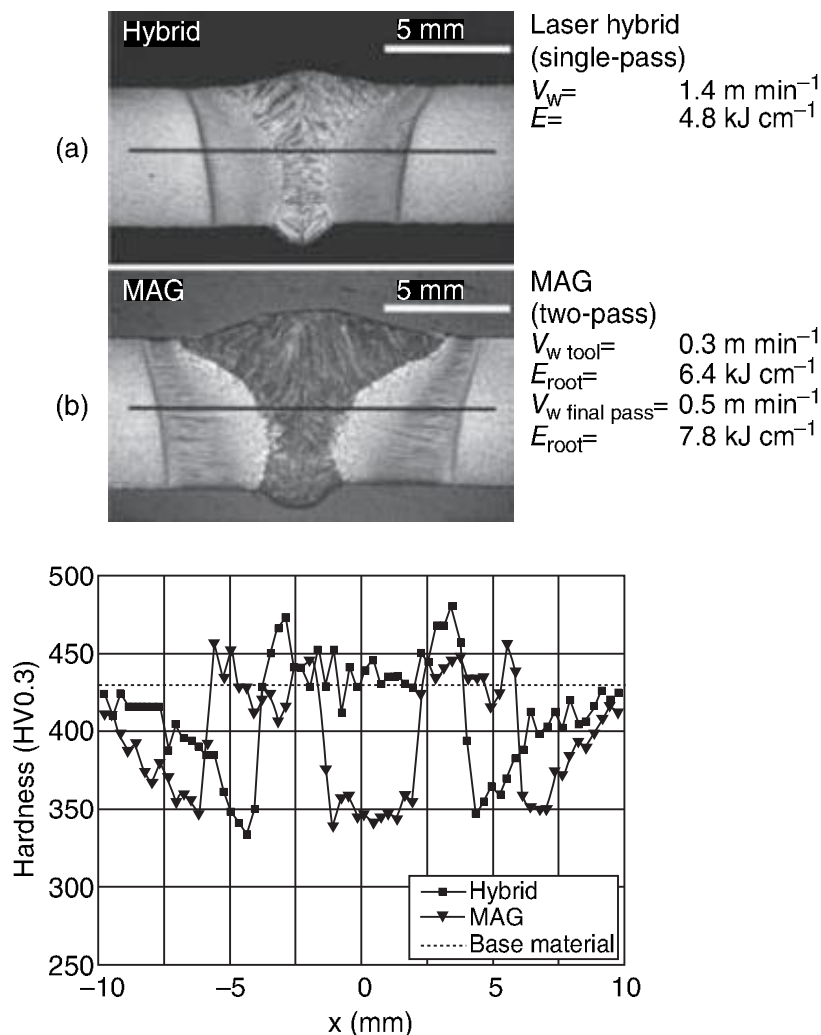
5.10 Micrographs and hardness distribution of (a) a hybrid weld and (b) a two-layer MAG weld, S1100QL ( E = heat input per unit length) (Jahn et al. 2005).
