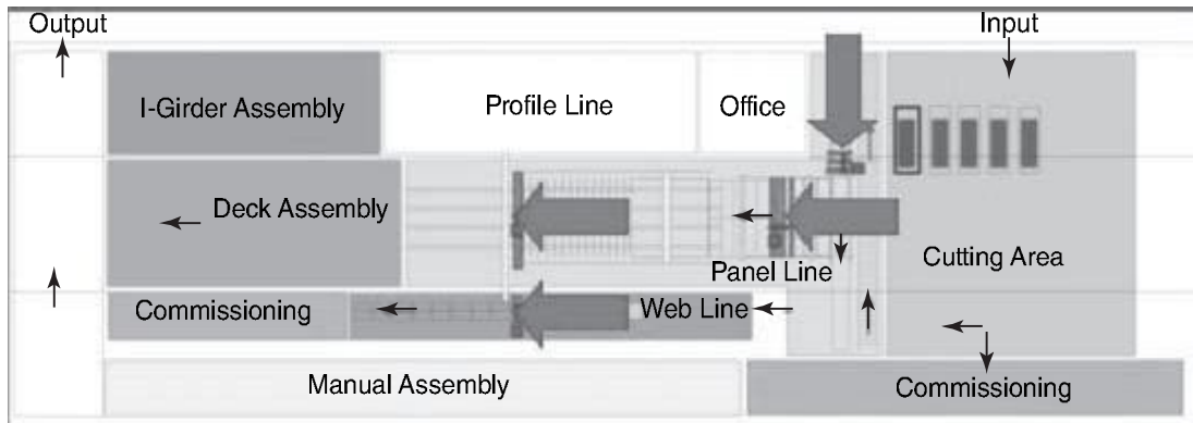
8.6 Layout of new pre-manufacturing workshop at Meyer Werft, red arrows indicate laser hybrid welding positions (Courtesy: Guido Pethan, Meyer Werft).
