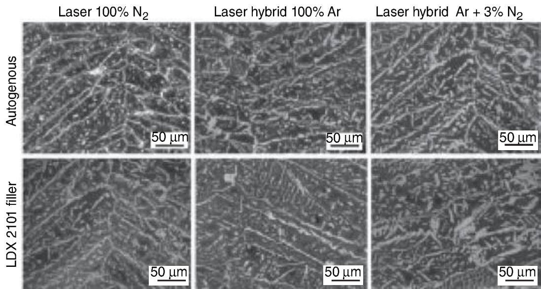
5.6 Lean duplex LDX2101 weld microstructure (Westin et al. 2007).
