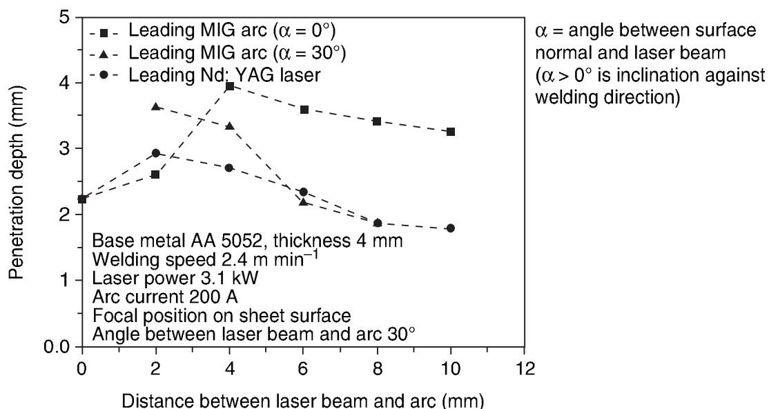
10.12 Effect of the distance between laser beam and arc on penetration in Nd:YAG laser MIG hybrid welding of aluminium (Uchiumi et al. , 2004).
