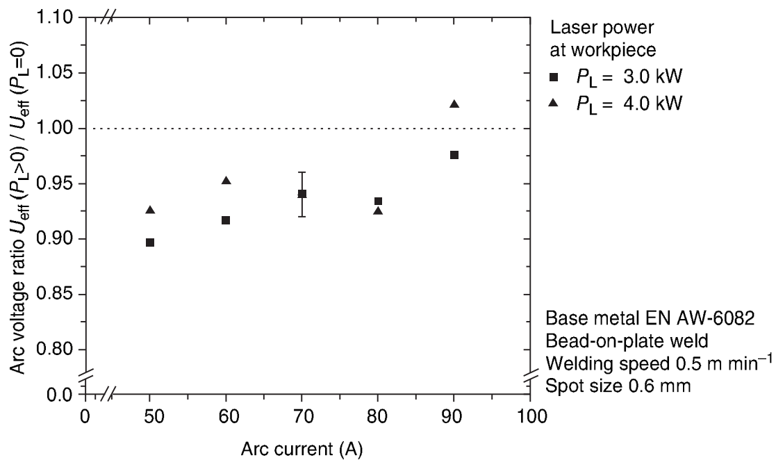
10.9 Effect of arc current and laser power at workpiece on the effective arc voltage ratio in coaxial Nd:YAG laser plasma arc welding of EN AW-6082 (Thomy et al. , 2008).
