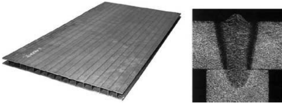
8.5 First laser welded sandwich panels produced at Meyer Werft, Germany (Courtesy: Guido Pethan, Meyer Werft).
