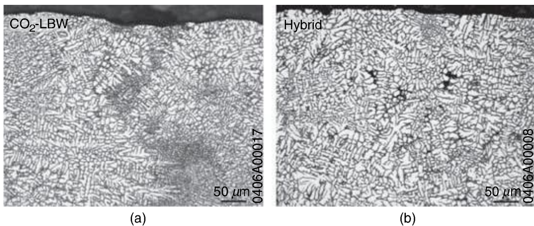
5.8 Typical dendritic structure in the upper section of the fusion zone in (a) CO 2 laser beam weld and (b) hybrid weld in a 3.2 mm thick AA6013 sheet butt-welded in T6 (Vaidyaa, 2006).
