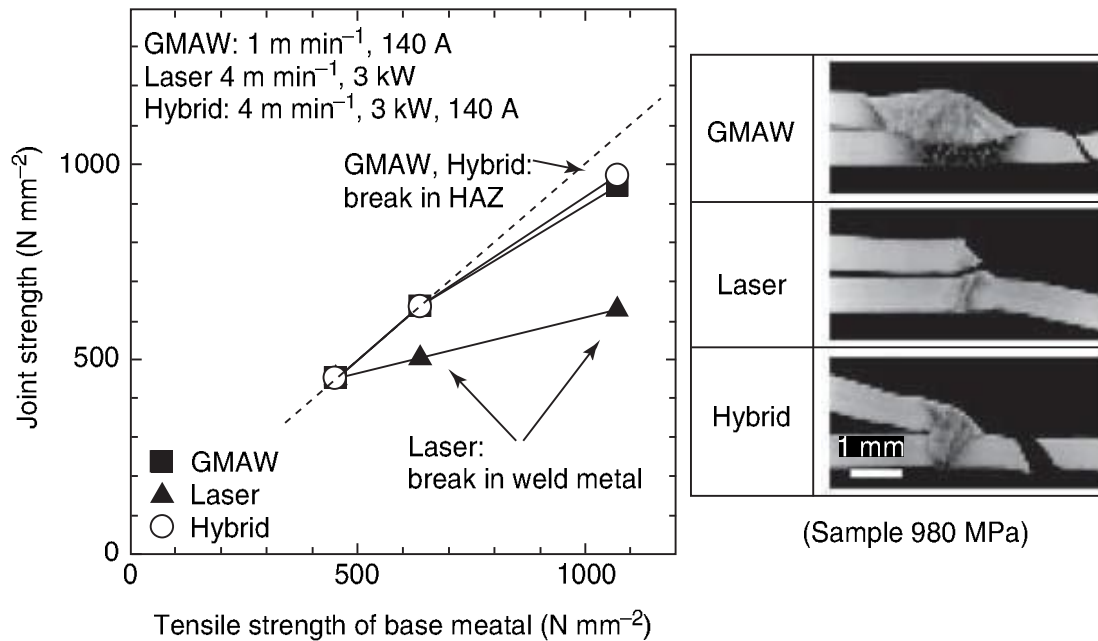
12.3 Comparison of joint strengths between spot, laser and hybrid welds, and cross-sections of specimens after test.
