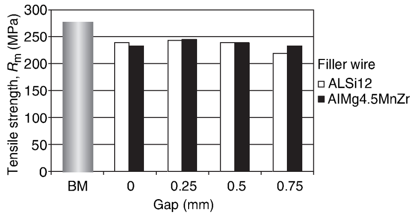
5.15 Tensile strength of square butt welds after artificial ageing on 3 mm AlMgSi1 with different gaps compared with the base material (BM), welded with filler wires AlSi12 and AlMg4.5MnZr (Dilthey et al. 2005).
