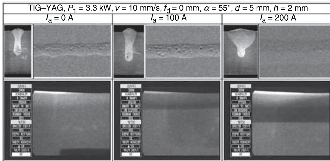
2.18 Cross-sections and x-ray inspection results of weld beads, and transmission real-time observation results of molten pools of hybrid TIG–YAG laser welding.
