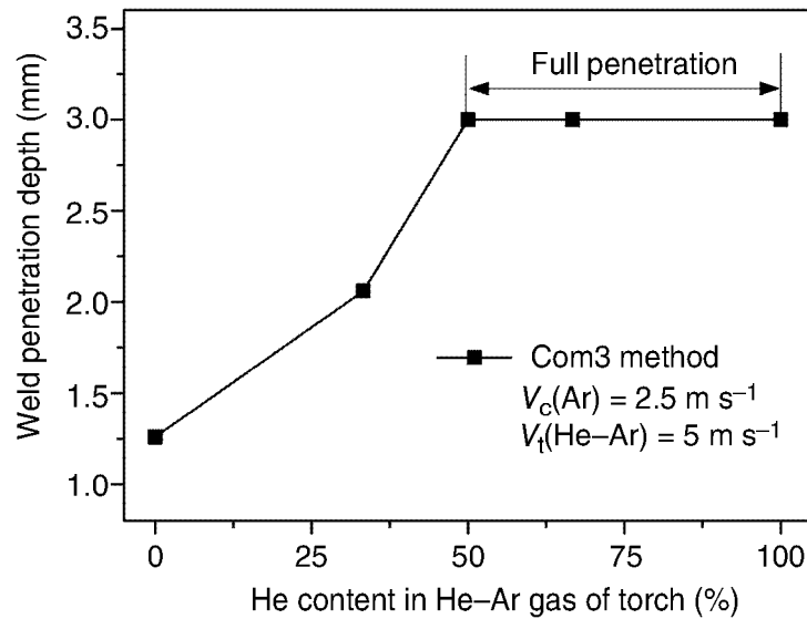
4.6 Effects of helium content in He–Ar shielding gas on penetration depth of CO 2 laser–TIG hybrid weld, the substrate is 316L stainless steel plate with 3 mm thickness.
