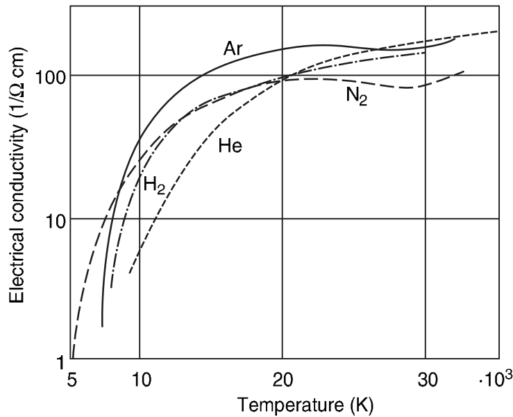
4.3 Electrical conductivity of gases as a function of temperature (Tusek, 2000).
