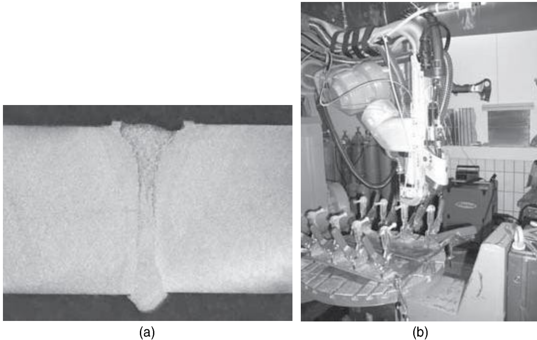
9.8 LaserHybrid welding with a fibre laser ( P_l 6.9 kW, V_s 2.4 m min -1 , s 8 mm, base material S235JR, Filler wire G3Si1)
