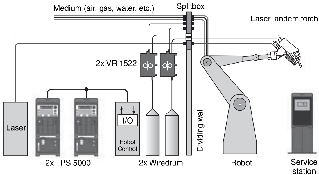
9.14 LaserTandem welding system including laser, power sources, wire feeder, welding head, dividing wall and service station.
