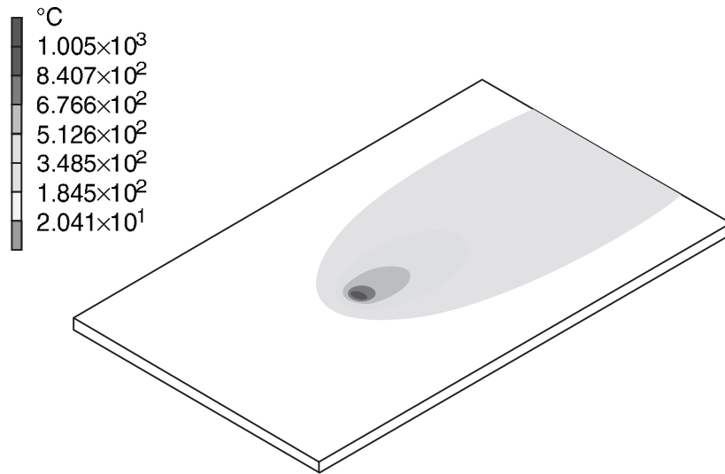
7.33 Temperature distribution of TIG butt-welding alone at quasi-stable state. 36
