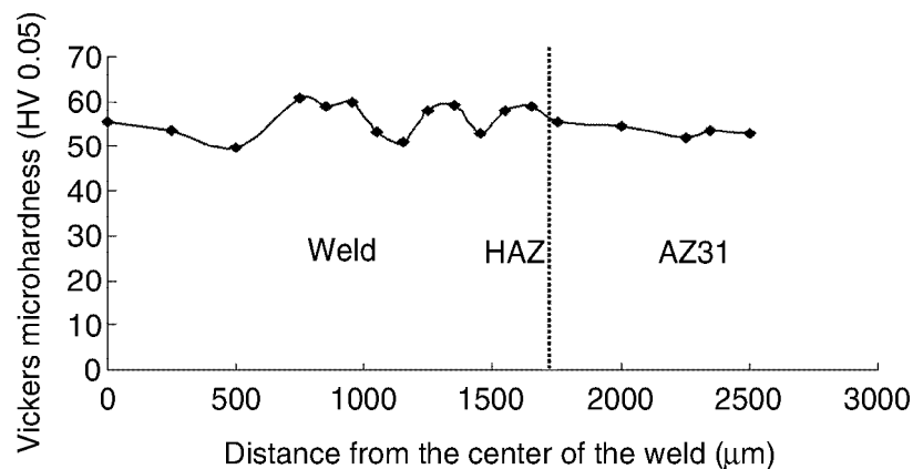
7.17 Hardness profile across weld in AZ31. 35
