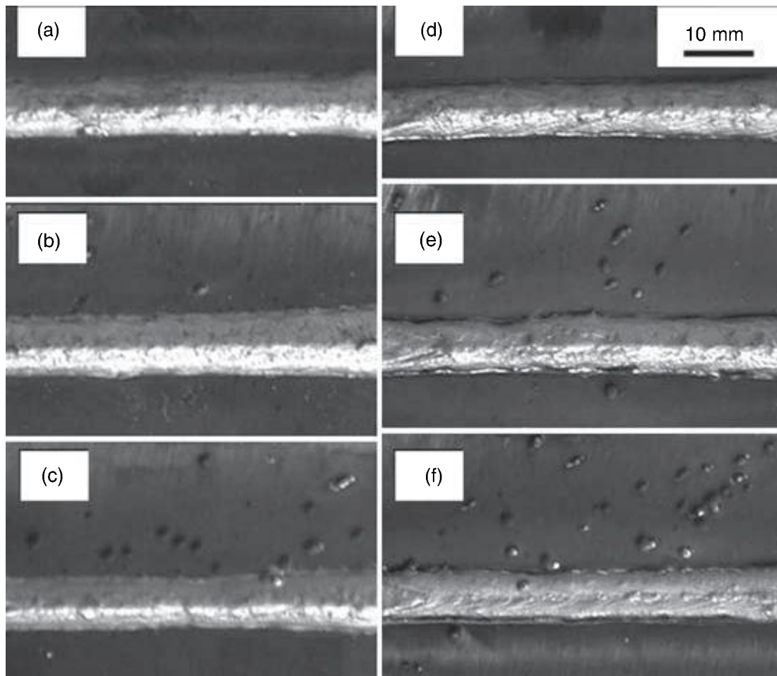
4.7 Effect of CO 2 and He content in shielding gas on spatter of hybrid laser-MAG welding for mild steel, He-Ar mixed gas: (a) He 20%, (b) He 60%, (c) He 100%, Ar balance; CO 2 -Ar mixed gas: (d) CO 2 10%, (e) CO 2 30%, (f) CO 2 50%.
