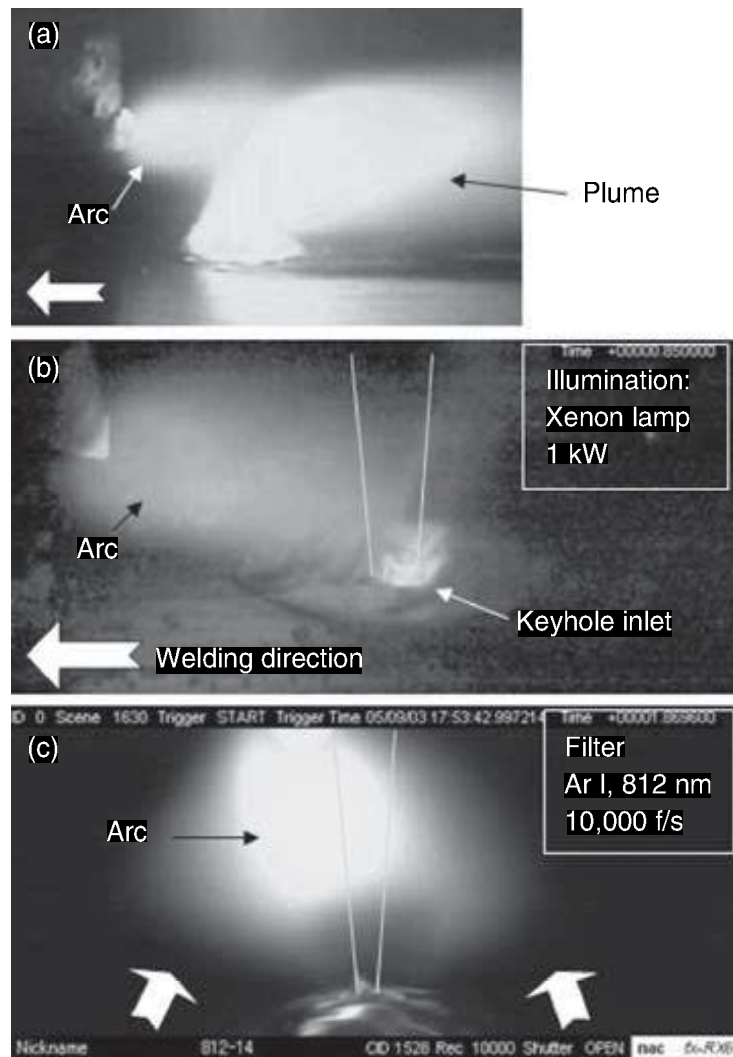
2.8 CCD and high-speed video observation results of arc and plume behavior during hybrid TIG–YAG laser welding.
