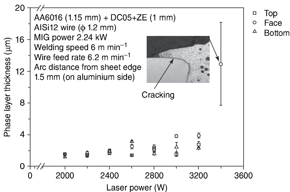
11.9 Effect of laser power on phase layer thickness in laser–MIG hybrid welding.
