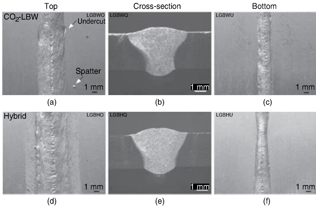
5.7 Surface appearance of the CO 2 laser beam weld (upper micrographs; a–c) and the hybrid weld (lower micrographs; d–e) in a 3.2 mm thick AA6013 sheet butt-welded in T6. The surface was cleaned, the cross-section was polished and lightly etched. Local height differences in the weld are seen as surface irregularities (Vaidyaa et al. 2006).
