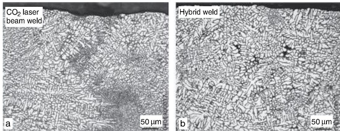
10.14 Difference in the dendritic structure in (a) CO 2 laser beam weld and (b) hybrid weld in a 3.2 mm thick AA6013 sheet butt-welded in T6 in the top centre region of the weld metal (Vaidya et al. , 2006).
