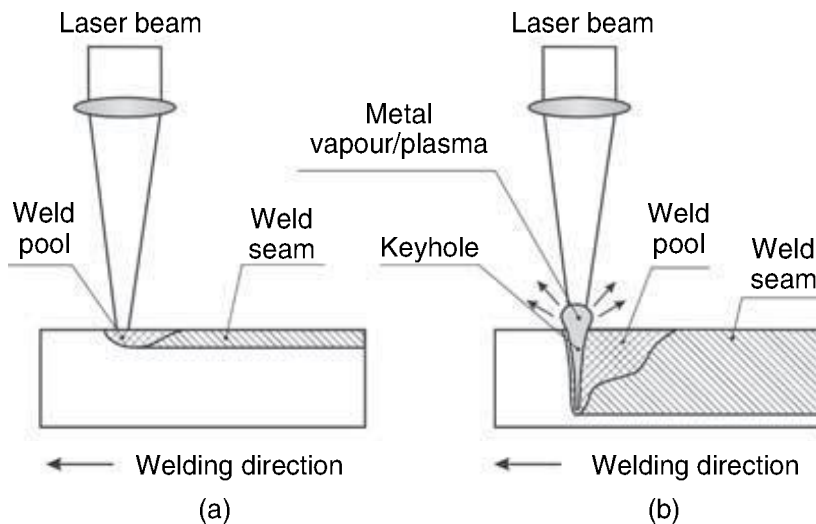
3.3 Schematic diagrams of (a) conduction mode laser beam welding and (b) keyhole mode laser beam welding.
