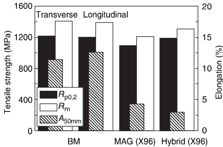
5.13 Strength and elongation of S1100QL, base metal, MAG and hybrid welds (Jahn et al. 2005).
