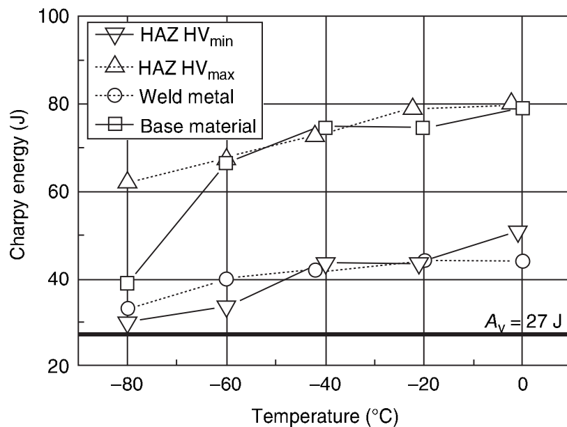
5.17 Charpy energy in dependence to the test temperature, S1100QL (Jahn et al. 2005).
