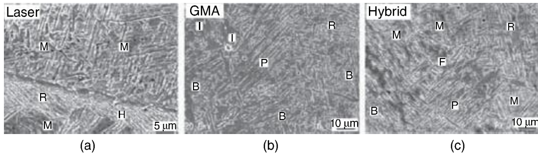
5.4 SEM images of laser weld metal, GMA weld metal and laser–GMA hybrid weld metal (Liu et al. 2006).
