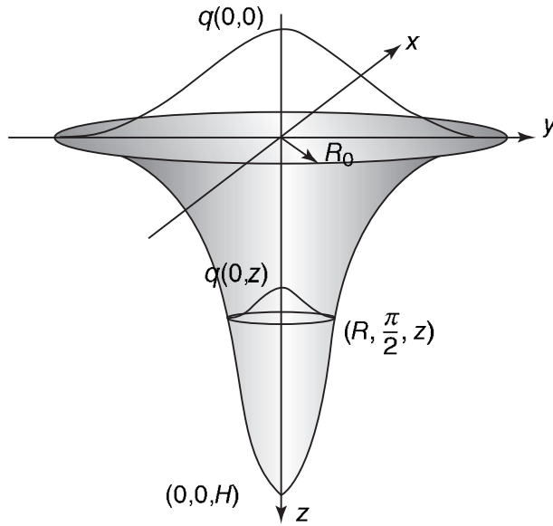
7.29 Rotary-Gauss body heat source model. 36
