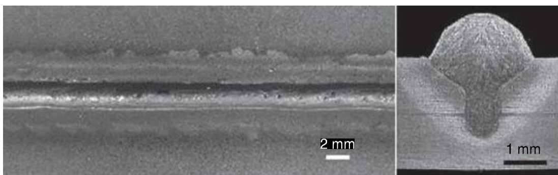
12.2 Surface and cross-section of hybrid MIG–YAG laser weld bead.
