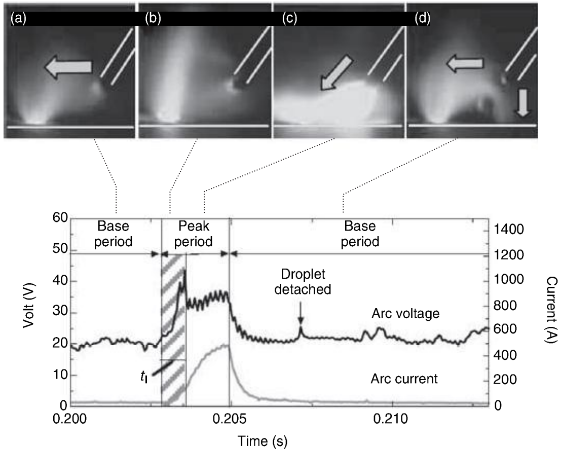
2.5 Variation in arc voltage and current and high speed images during transition of base to peak periods in hybrid welding. Pulse frequency: 50 Hz, leading arc, DLA: 3 mm, v = 2 \text{ m min}^{-1} .
