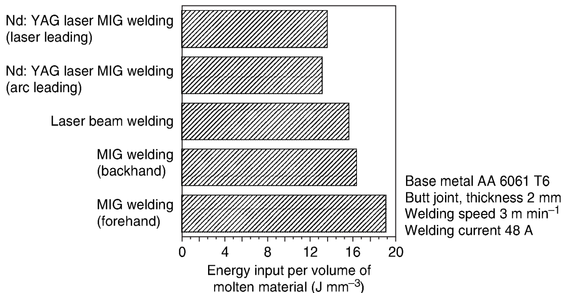
10.5 Energy input per volume of molten material for various welding processes for a given joint configuration and welding speed (Lee and Park, 2003).
