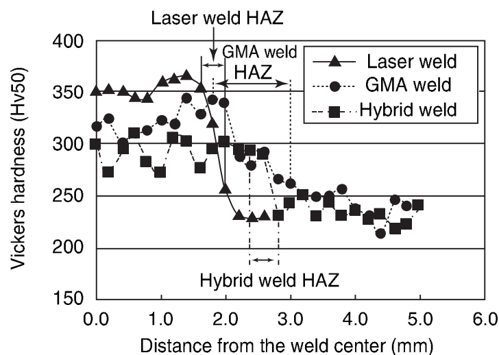
5.9 Hardness distribution in laser weld, GMA weld and laser–GMA hybrid weld (Liu et al. 2006).
