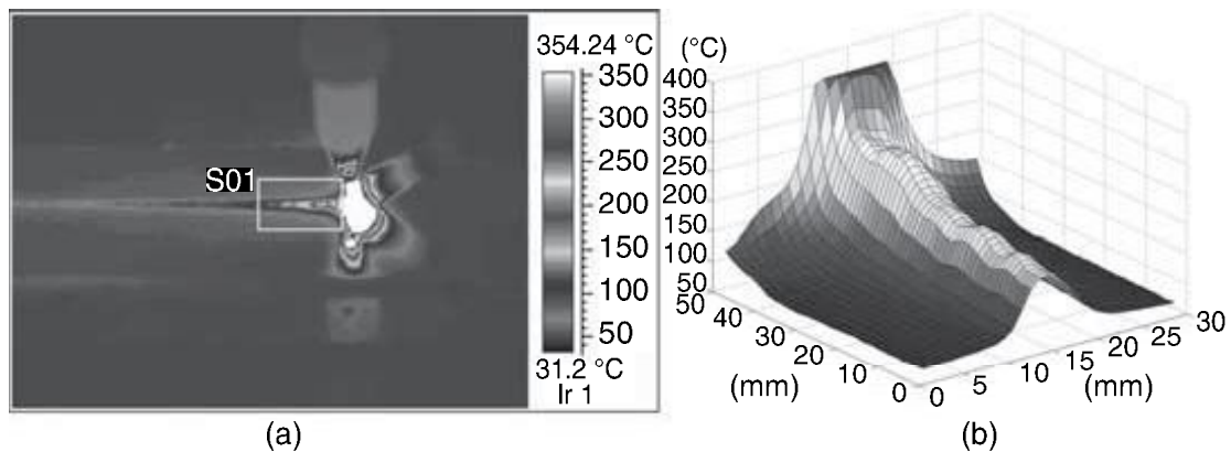
7.36 Infrared image and the zone analysis of S01 in hybrid welding. 38
