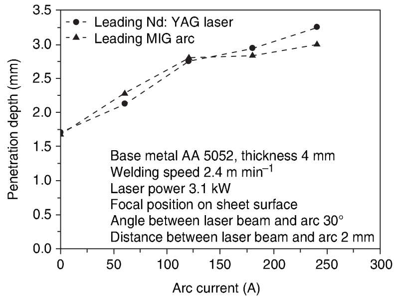
10.11 Effect of arc current on penetration in Nd:YAG laser MIG hybrid welding of aluminium (Uchiumi et al. , 2004).
