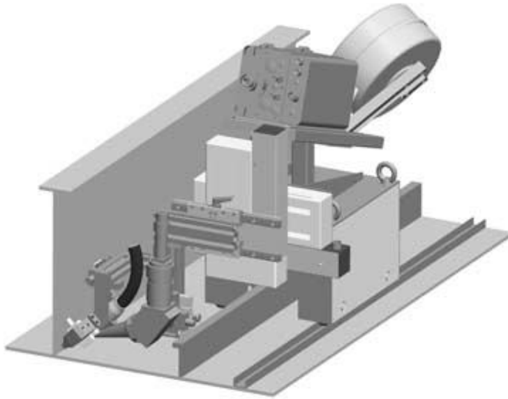
9.7 Welding system of a fillet weld.
