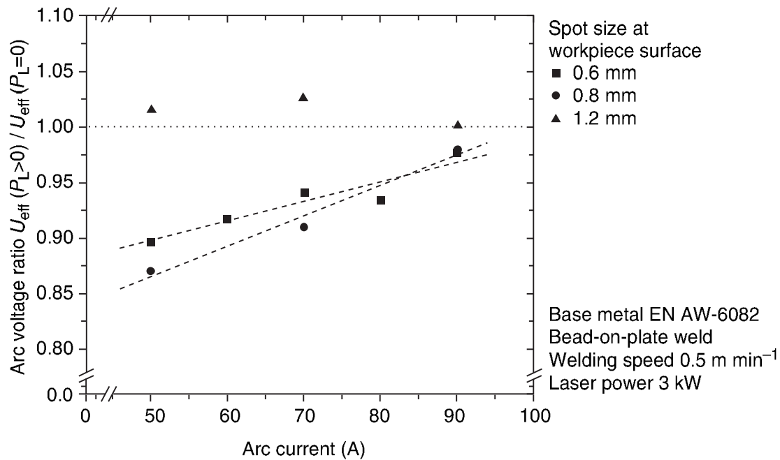
10.10 Effect of arc current and spot diameter at workpiece on the effective arc voltage ratio in coaxial Nd:YAG laser plasma arc welding of EN AW-6082 (Thomy et al. , 2008).
