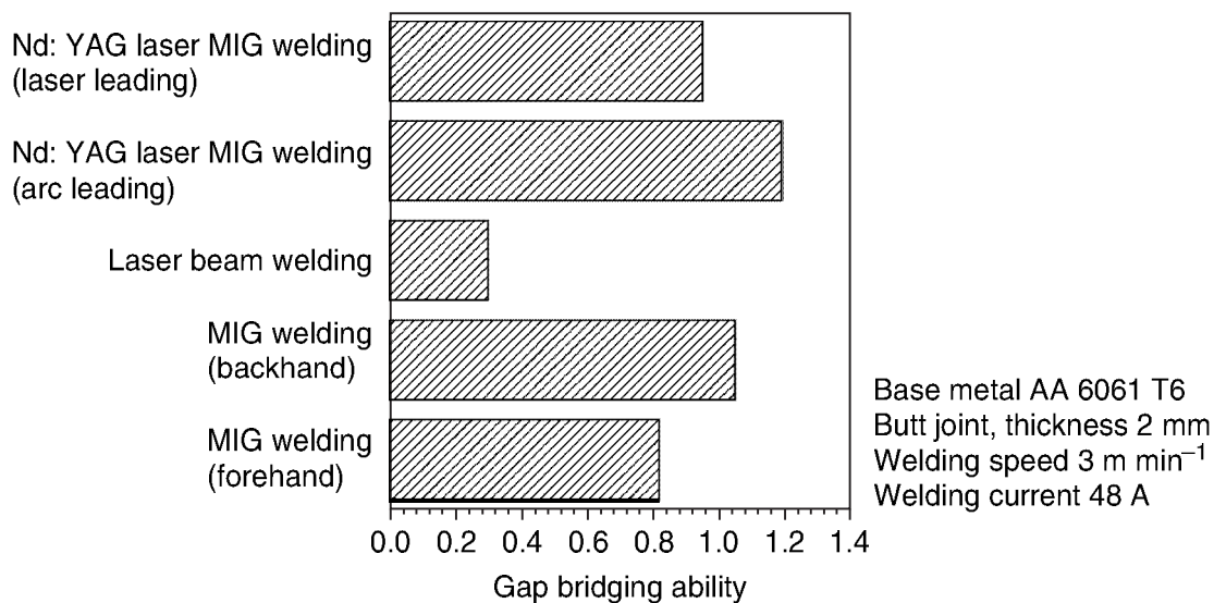
10.6 Gap bridging ability of various welding processes for given process parameters and joint configuration (Lee and Park, 2003).
