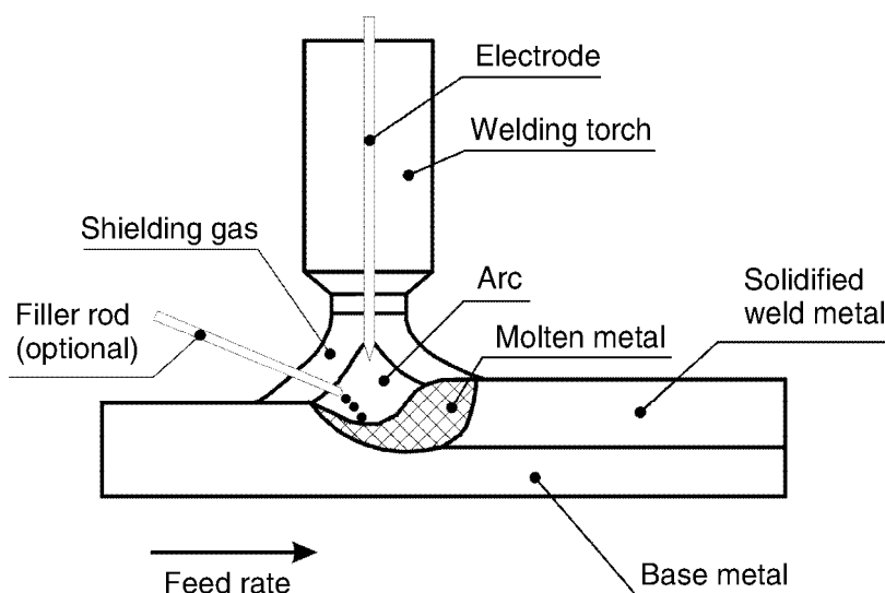
3.9 Schematic diagram of tungsten inert gas welding with non-consumable electrode.
