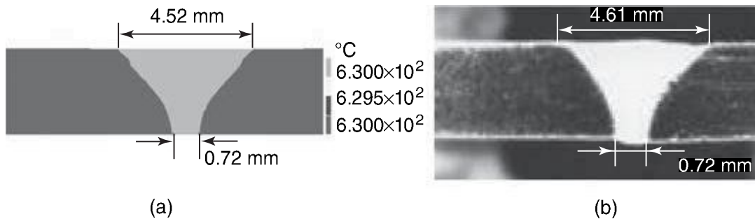
7.34 Comparison of experimental butt-welding joint and simulative result. 36 (a) Simulative weld joint of hybrid welding; (b) Experimental weld joint of hybrid welding.
