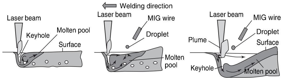
2.21 Schematic welding phenomena during laser welding and during hybrid YAG laser–MIG welding at 120 and 240 A, showing melt flows, bubble and porosity formation or no porosity.
