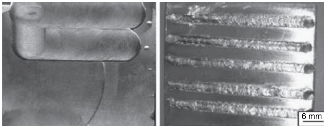
7.26 Number of pores in weld metal using laser lateral shielding. 27
