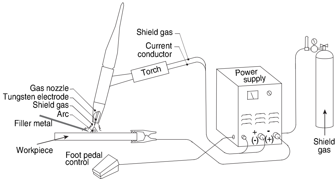
1.2 Schematic of a typical gas tungsten arc weld (GTAW) set up (not to scale).
