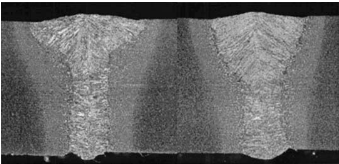
4.9 Effect of carbon dioxide on hybrid weld bead cross section width: 0% CO 2 (left), 10% CO 2 (right); 40% He, balance argon. A gap of 0.8 mm was present in the joint. Plate thickness 6 mm.
