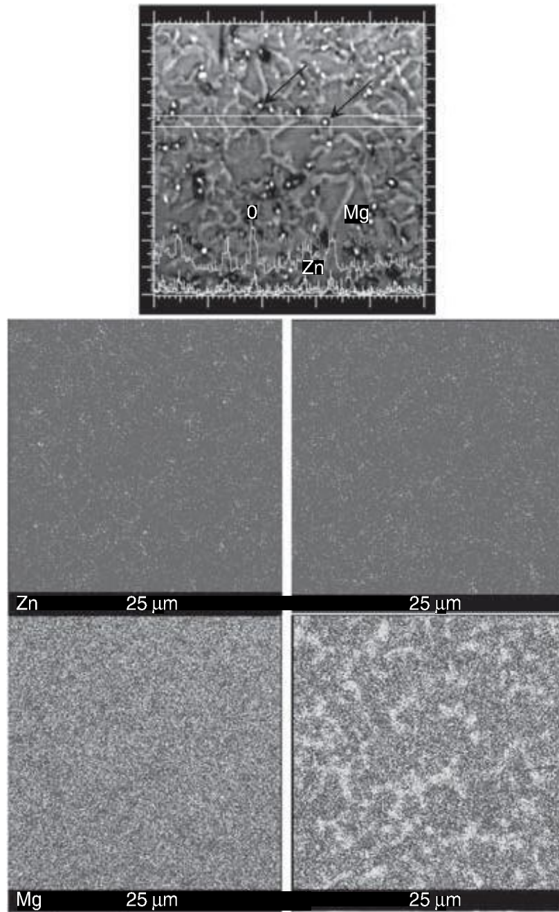
7.15 EPMA patterns obtained from AZ31B after hybrid overlaps welding. 32 (a) Backscattered electron image of fusion zone; (b), (c), (d), (e) show the distributions of Zn, Al, Mg, O, respectively, within fusion zone.
