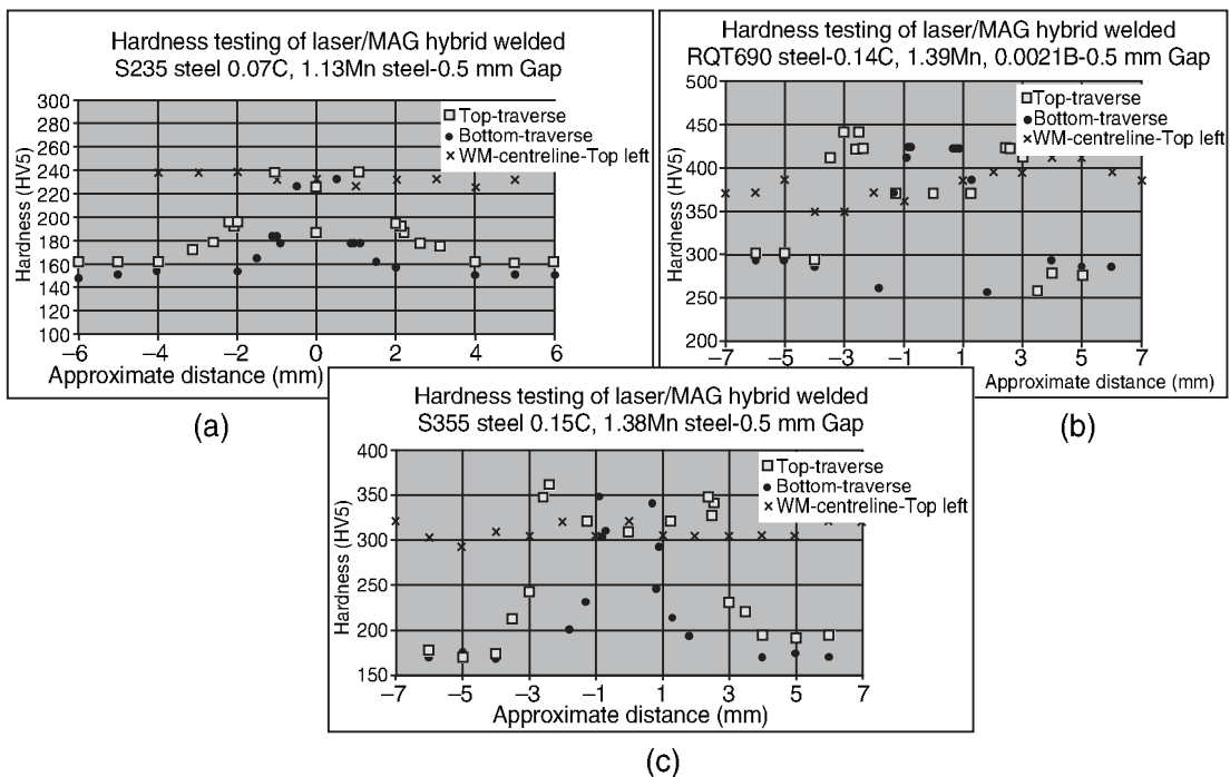
8.2 Hardness profiles for welds in (a) S235 (0.07C, 1.13Mn), (b) RQT 690 (0.14C, 1.39Mn, 0.0021B) and (c) S355 (0.15C, 1.38Mn) steels.
