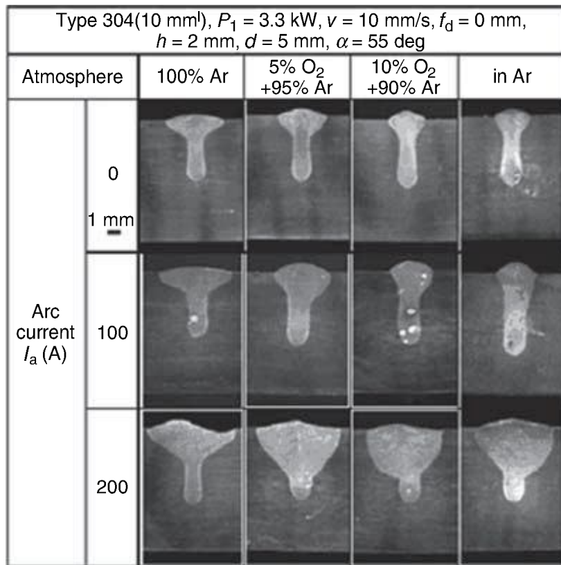
4.5 Effects of oxygen content on the hybrid YAG laser–TIG weld shape of 304 stainless steel.
