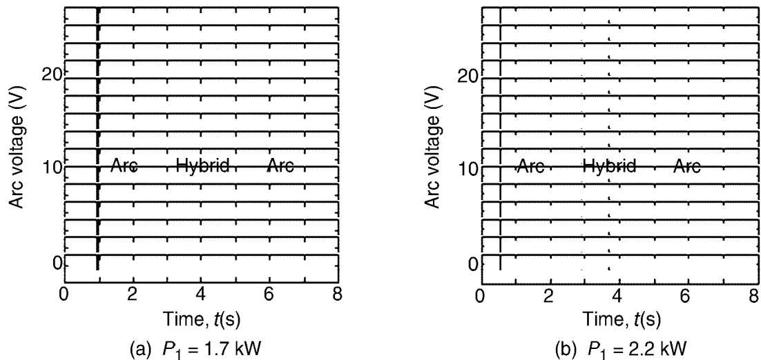
2.4 Voltage variation during TIG welding and hybrid welding.
