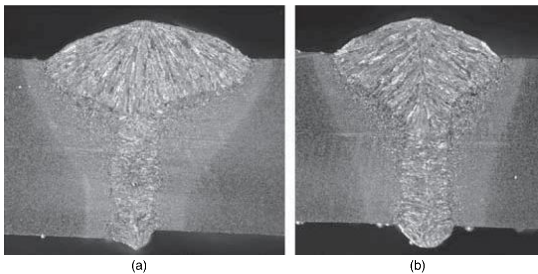
4.8 Effect of He on hybrid weld bead cross section width in close-fitting I-butt joints: (a) 30% He, (b) 80% He; 2% CO 2 , balance argon. Plate thickness is 6 mm.
