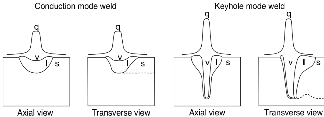
1.3 Illustration of conduction mode and keyhole mode weld definitions.
