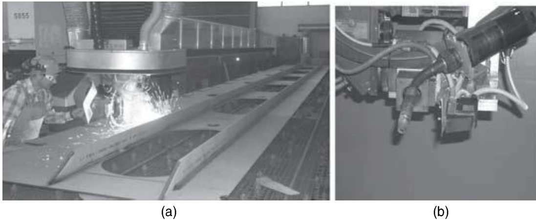
8.11 (a) Laser installation at Odense Steel Shipyard and (b) the T-joint hybrid welding head (Courtesy: Mads Elvang, Odense Steel Shipyard).
