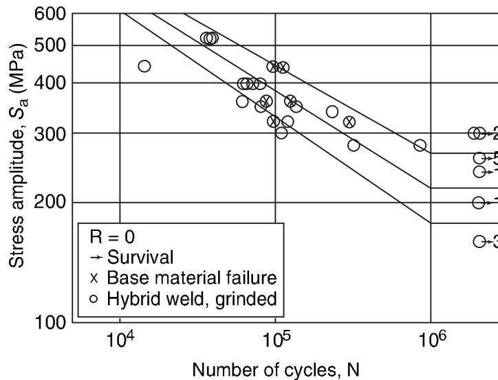
5.18 S–N curve of laser hybrid welds, R = 0 , S1100QL, S_{A\ 50\%} = 218 MPa (Jahn et al. 2005).
