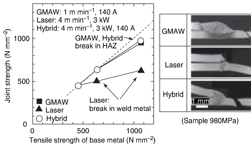
5.12 The tensile strength of welded joints of high-strength steel sheets with three different welding processes (Masato and Kiyoyuki, 2005).
