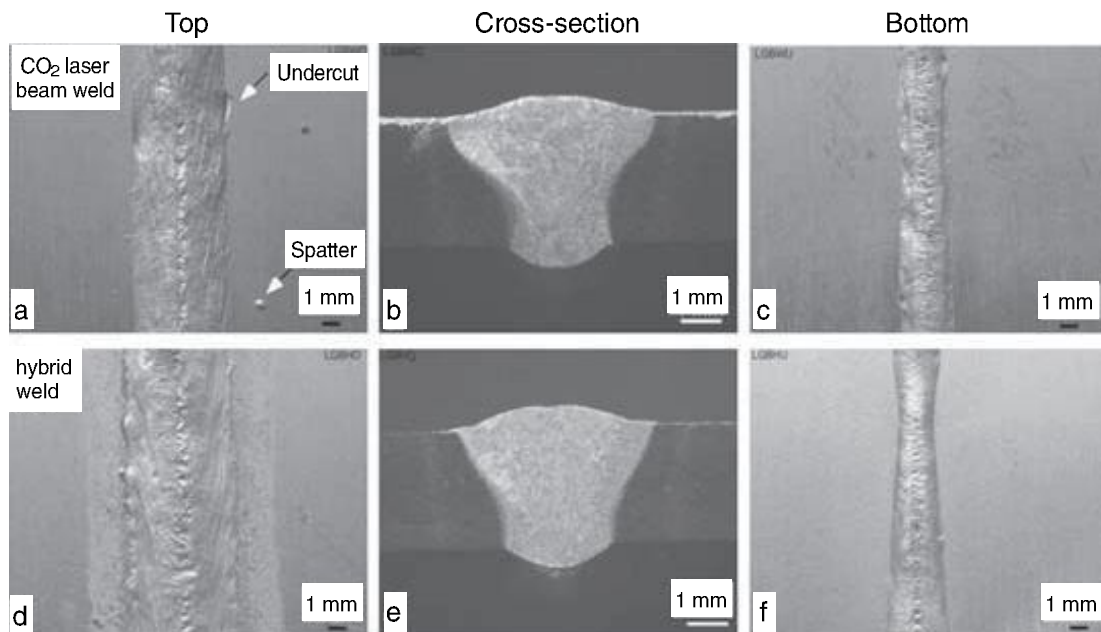
10.13 Surface appearance and cross-section of the CO 2 laser beam weld (upper micrographs; a–c) and the hybrid weld (lower micrographs; d–f) in a 3.2 mm thick AA6013 sheet butt-welded in T6 (Vaidya et al. , 2006).
