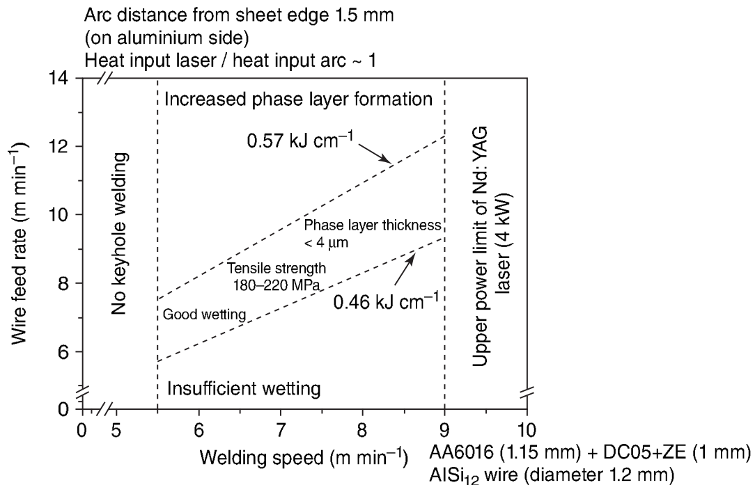
11.13 Process parameter envelope for laser–MIG hybrid welding of aluminium to steel.
