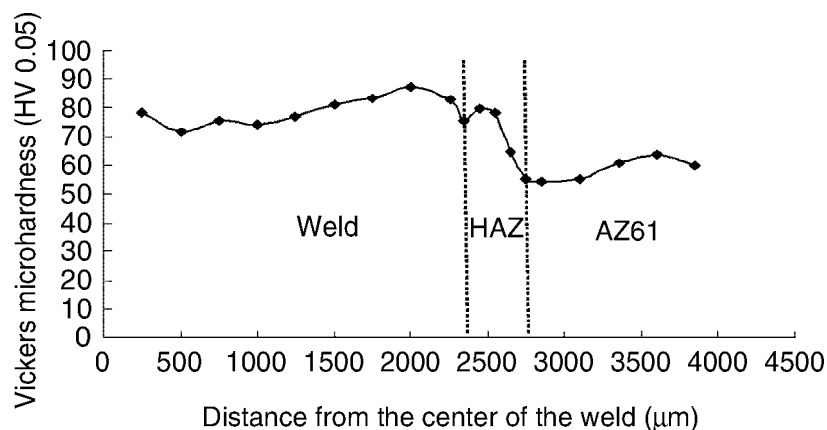
7.18 Hardness profile across weld in AZ61. 35
