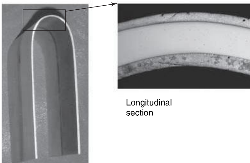
11.15 Bend test, radius 10 mm, angle 180° for AA6016 (thickness: 1.15 mm) and zinc-coated steel DC05 + ZE (thickness: 1 mm).
