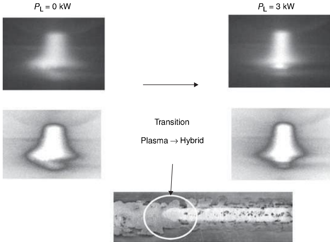
10.8 Example for the effect of laser power P_L on top bead appearance and arc zone geometry in coaxial Nd:YAG laser plasma arc welding of EN AW-6082 (spot size 0.6 mm, current 50 A, bead-on-plate weld) (Thomy et al. , 2008).
