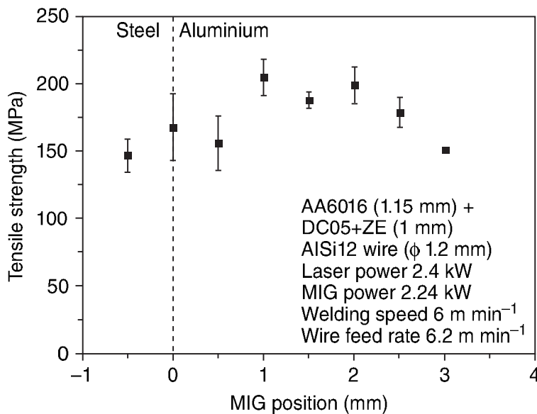
11.12 Effect of MIG position relative to sheet edge on tensile strength in laser–MIG hybrid welding.
