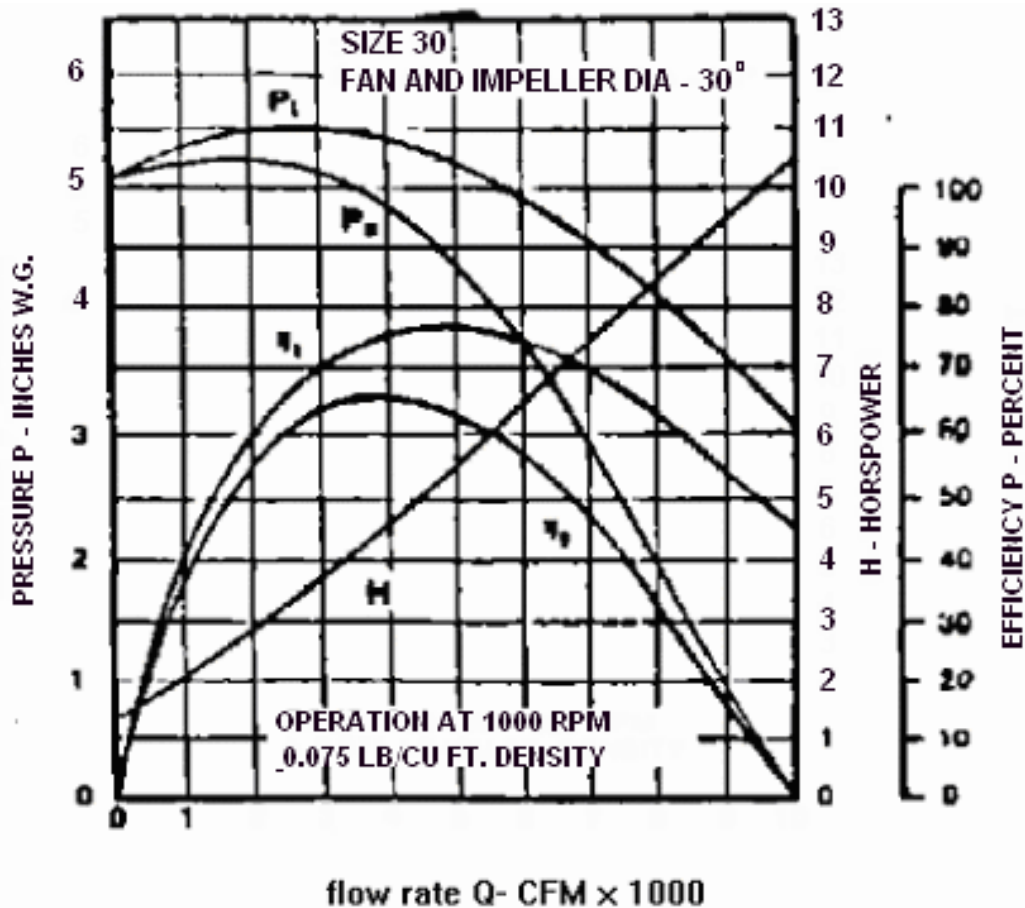
FAN PERFORMANCE CURVE
