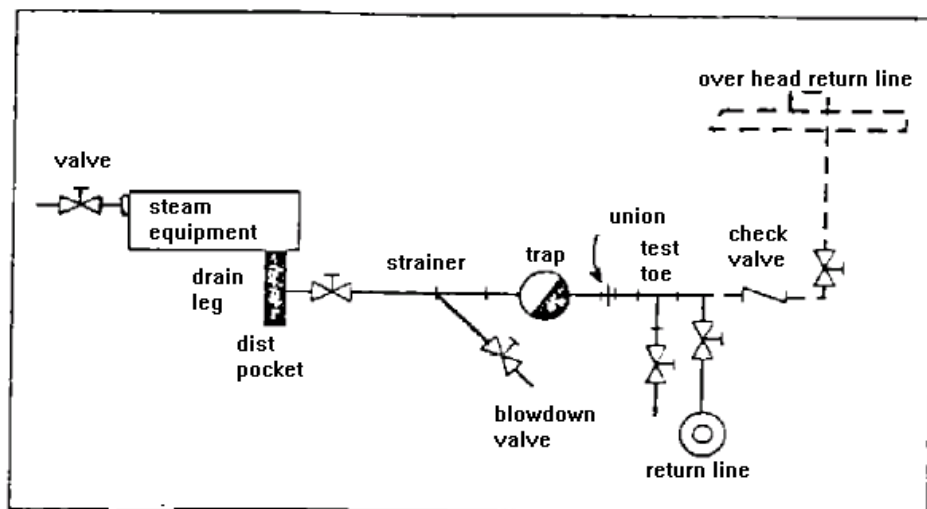
A TYPICAL STEAM TRAP STATION WITH ASSOCIATED PIPING AND AUXILIARY EQUIPMENT
