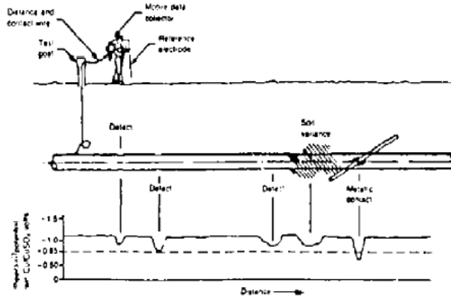
CLOSE INTERVAL PIPE/SOIL POTENTIAL SURVEY Fig. B.11.2.A
