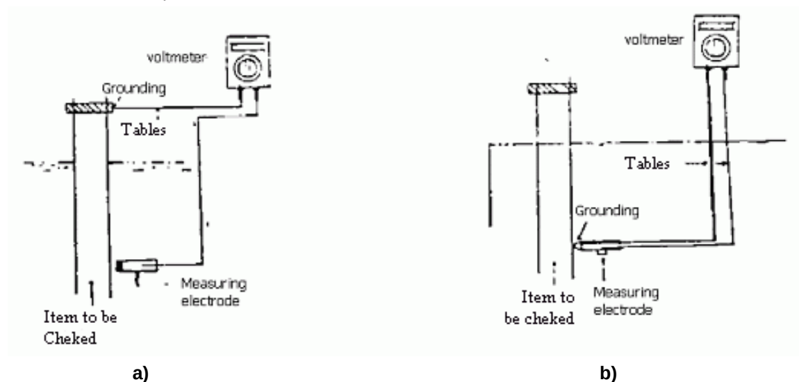
SCHEMATIC WIRING DIAGRAM FOR POTENTIAL MEASUREMENTS
