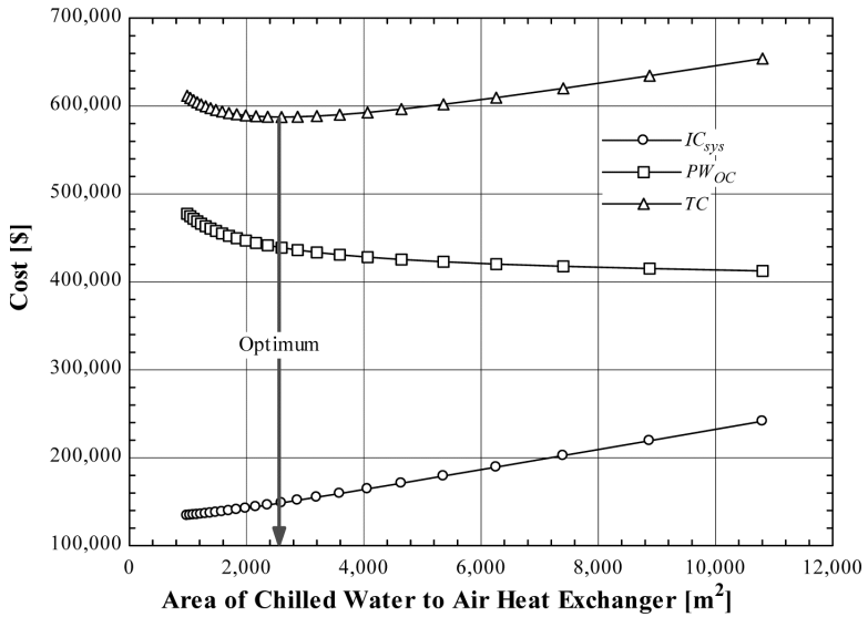
Figure 3.9. Optimum chilled water heat exchanger area (2,604 m 2 ) based on minimum total costs
