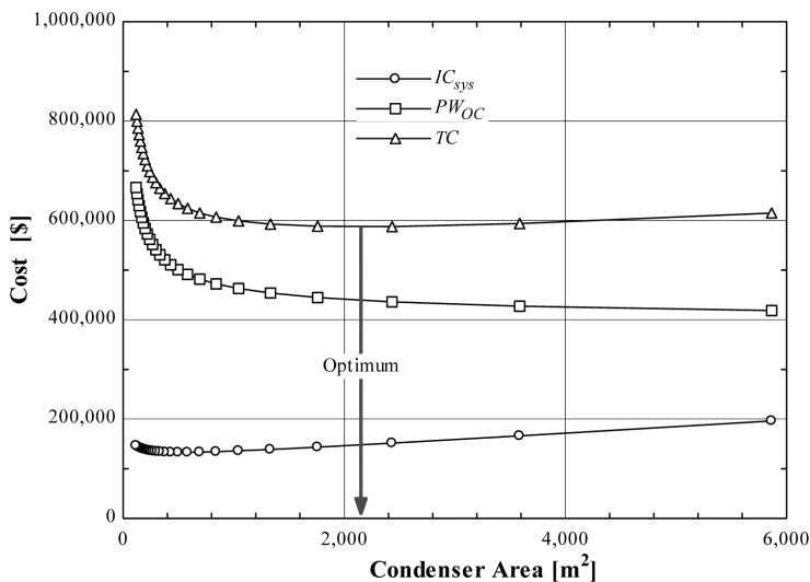
Figure 3.8. Optimum condenser area (2,180 m 2 ) based on minimum total costs (EES, 2014)
