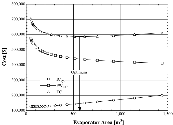
Figure 3.7. Optimum evaporator area (588.2 m 2 ) based on minimum total costs ( TC ). The initial cost of the system ( IC_{sys} ) is composed of the cost for the chilled water heat exchanger, evaporator, compressor, and condenser. The present worth of the operating costs ( PW_{OC} ) accounts for the time value of money ( i = 5 percent) for the annual energy costs at ($0.07/kW-hr) over the life of the chiller (30 years). The total costs are the sum of the initial and operating costs. The remaining design variables are at their optimum values (EES, 2014).
