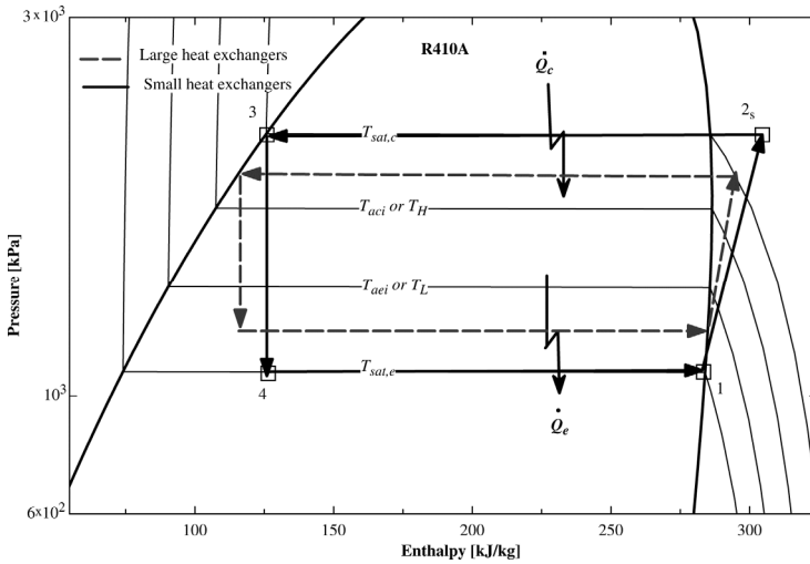
Figure 1.4. Property plot of the vapor-compression cycle (EES, 2014).
