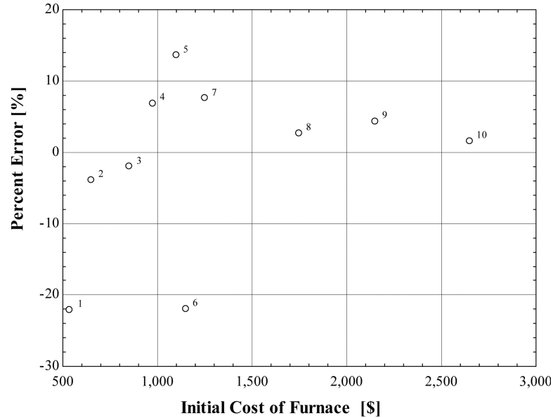
Figure 2.12. Percent error in model of initial cost for furnace (EES, 2014)
