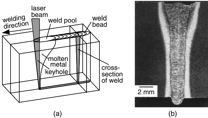
Figure 1.30 Laser beam welding with CO 2 laser: (a) process; (b) weld in 13-mm-thick A633 steel. (b) Courtesy of E.A. Metzbowyer.
