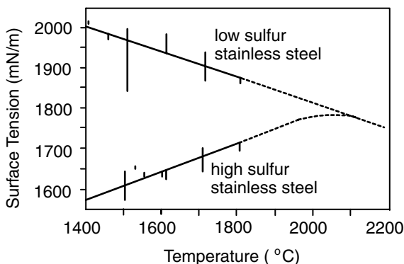
Figure 4.14 Surface tension data of two different heats of 316 stainless steel, one with 160 ppm more sulfur than the other. Modified from Heiple and Burgardt (26).
