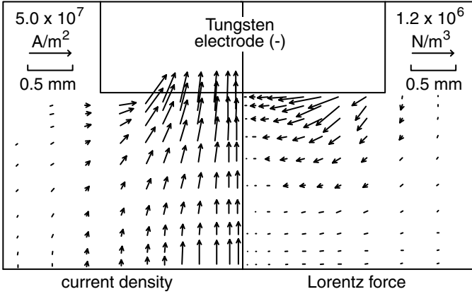
Figure 4.6 Current density field (left) and Lorentz force field (right) in an arc produced by a tungsten electrode with a flat end. Modified from Tsai and Kou (1).
