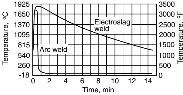
Figure 2.24 Thermal cycles of electrosag and arc welds. Reprinted from Liu et al. (60).
