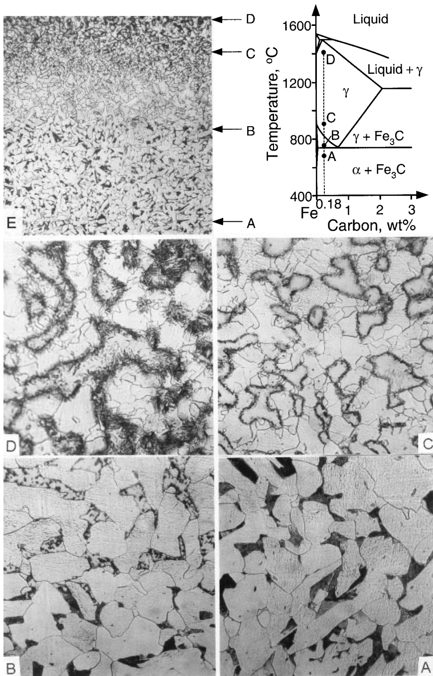
Figure 17.6 HAZ microstructure of 1018 steel produced by a high-power \text{CO}_2 laser. Magnification of (A)–(D) 415 \times and of (E) 65 \times . From Kou et al. (11).
