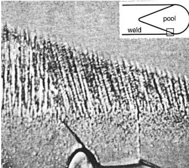
Figure 7.3 Epitaxial growth during the “welding” of camphene in the area indicated by the square (magnification 75×). Modified from Savage (6).
