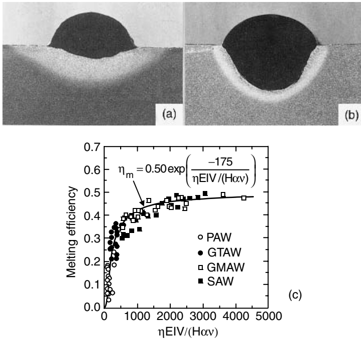
Figure 2.9 Melting efficiency: (a) lower at lower heat input and welding speed; (b) higher at higher heat input and welding speed; (c) variation with dimensionless parameter \eta EIV / H\alpha v . Reprinted from DuPont and Marder (7). Courtesy of American Welding Society.
