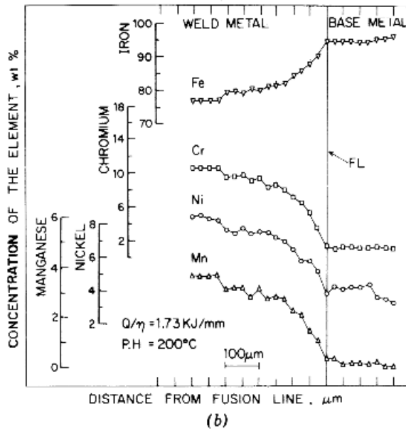
Figure 10.11 Fusion boundary of a low-alloy steel welded with an austenitic stainless steel electrode: (a) microstructure (magnification 55 \times ); (b) segregation. Reprinted from Ornath et al. (46). Courtesy of American Welding Society.
