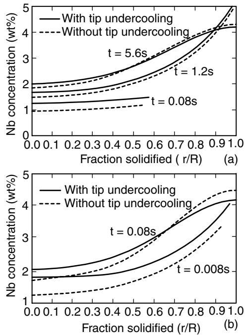
Figure 10.5 Calculated microsegregation in a Fe-3.3Nb weld: (a) slower cooling rate; (b) higher cooling rate. Reprinted from Brooks et al. (19).
