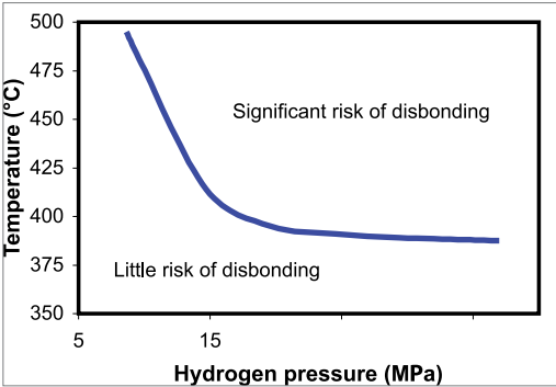
Figure 10. Influence of operating temperature and hydrogen partial pressure on the susceptibility to disbonding in refinery high-pressure hydrogen service [5, 7].
