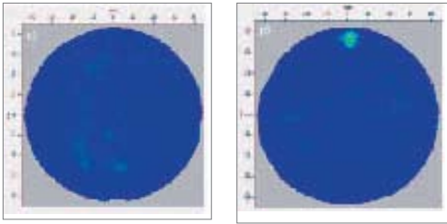
Figure 7. Ultrasonic top view scans showing the area of disbonding after testing. Left: No disbonding. Right: With some disbonding. Classification A1 (< 5%, isolated disbonded areas) according to [5].
