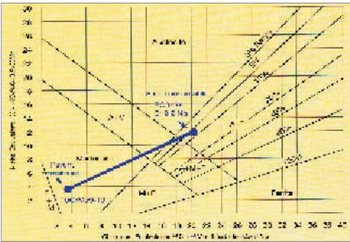
Figure 6. Schaeffler-diagram with line illustrating all possible compositions for different mixtures between parent material and welding strip.
