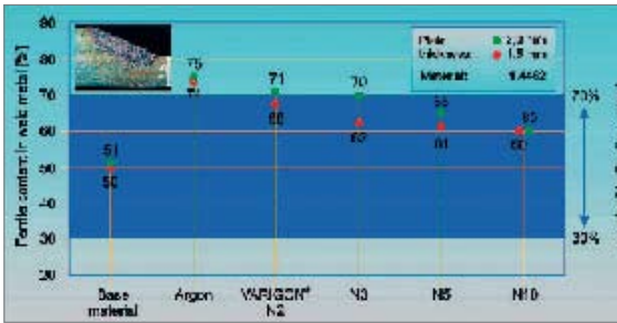
Figure 6. Application example - overlap weld with N 2 -containing gases, without filler metal
