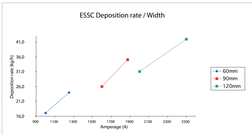
Figure 4. ESW deposition rate.
