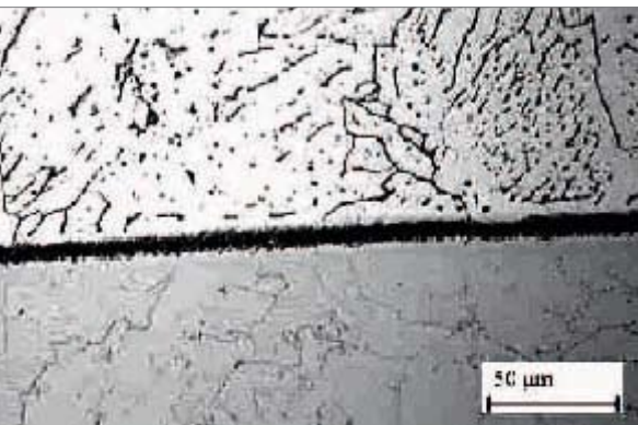
Figure 5. A comparatively narrow dark etching band of tempered martensite and carbides seen in an electrosag welded overlay after PWHT.
