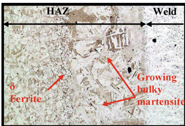
Fig. 5 HAZ zone in the SMSS
