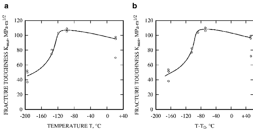
Fig. 7 The fracture toughness against temperature (a) and effective temperature (b)
