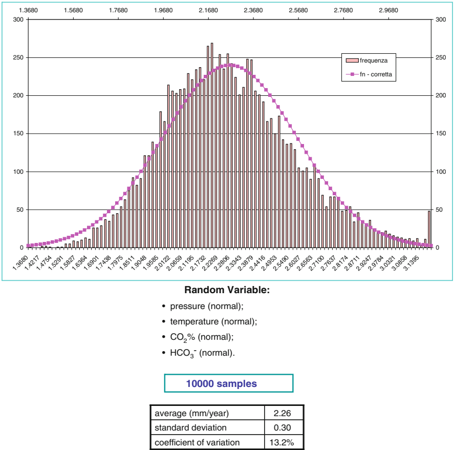
Fig. 7 Assessment of the cumulative distribution function of a function of random variable
