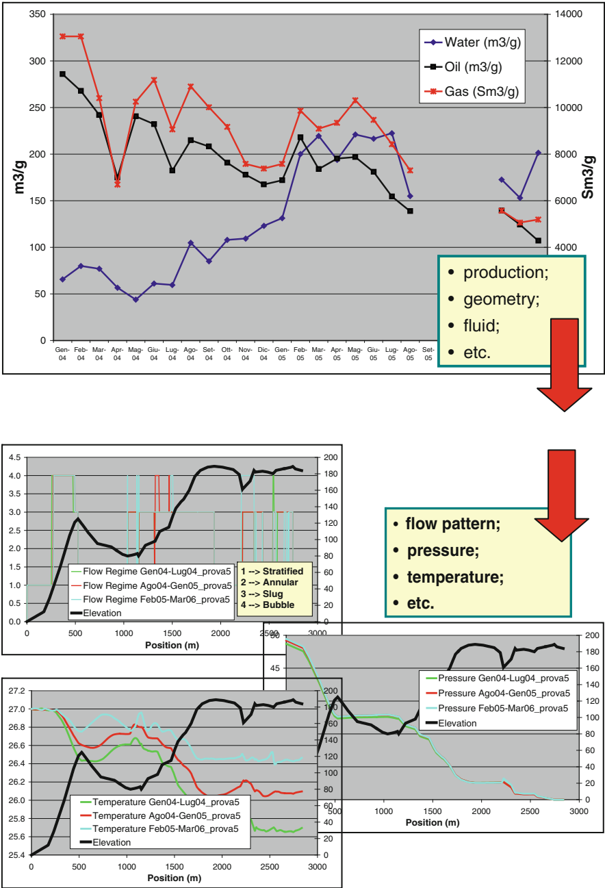
Fig. 6 Analysis of fluid dynamics, production, geometry, transported fluids, etc. along lifetime
