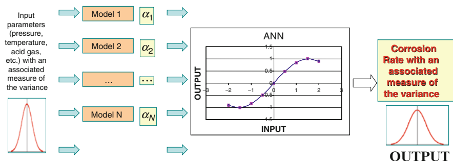
Fig. 9 Application of an Artificial Neural Network based model
