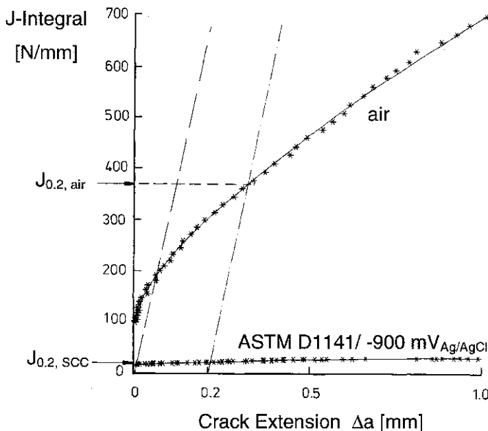
Fig. 3 J-R curves determined on pre-cracked compact specimens of the low-alloyed structural steel FeE 690T [11]
