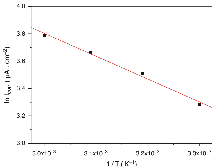
Fig. 3 Arrhenius plot calculated from corrosion current density for steel in NS4 simulating solution of corrosive soil environment ( \text{pH} \approx 6.7 )
