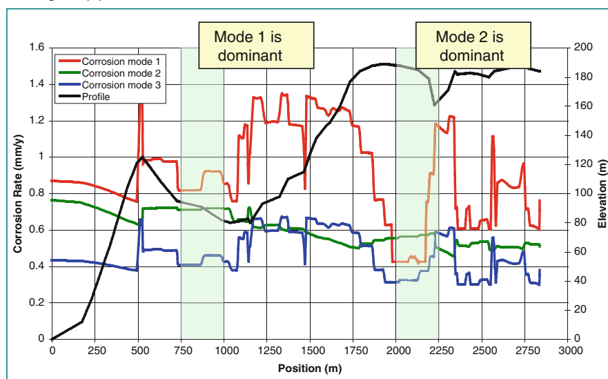
Fig. 11 Analysis of results and prevision of corrosion rate along lifetime
