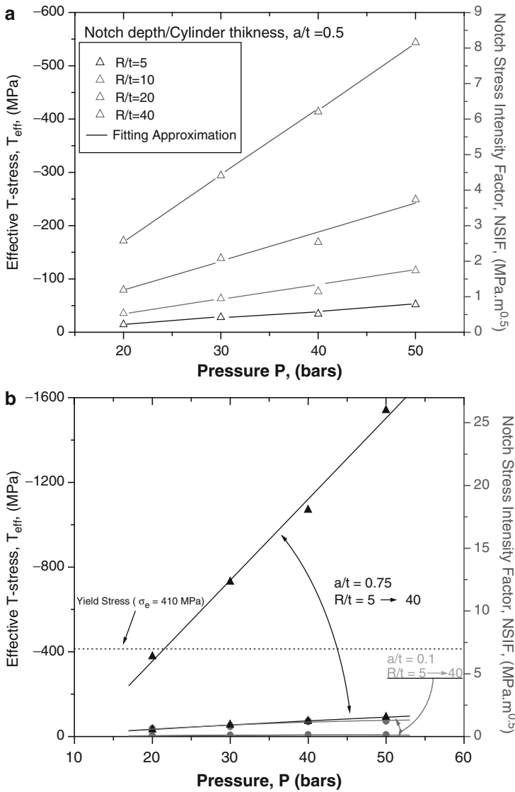
Fig. 9 (a) Evolution of the effective T-stress and the Notch Stress Intensity Factor with internal pressure, P for a/t = 0.5 and (b) transition of T_{eff} and NSIF for a/t = 0.1 to 0.75 for the diameter pipe R/t = 5 to 40
