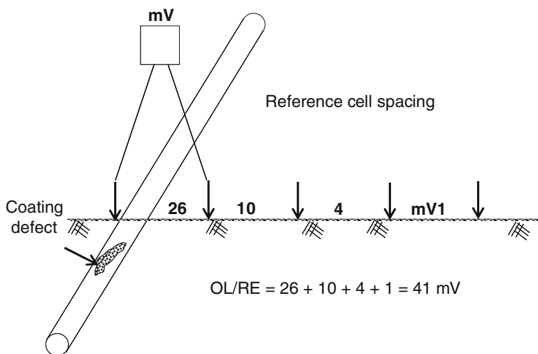
Fig. 4 Over-the-line/remote-earth measurements
