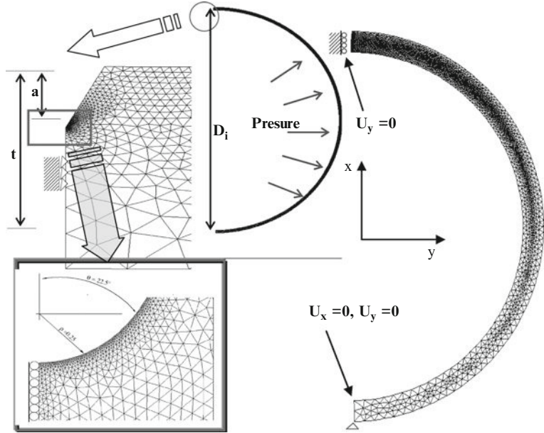
Fig. 4 Typical 2D finite element mesh and boundary conditions used in the model of the cracked pipeline
