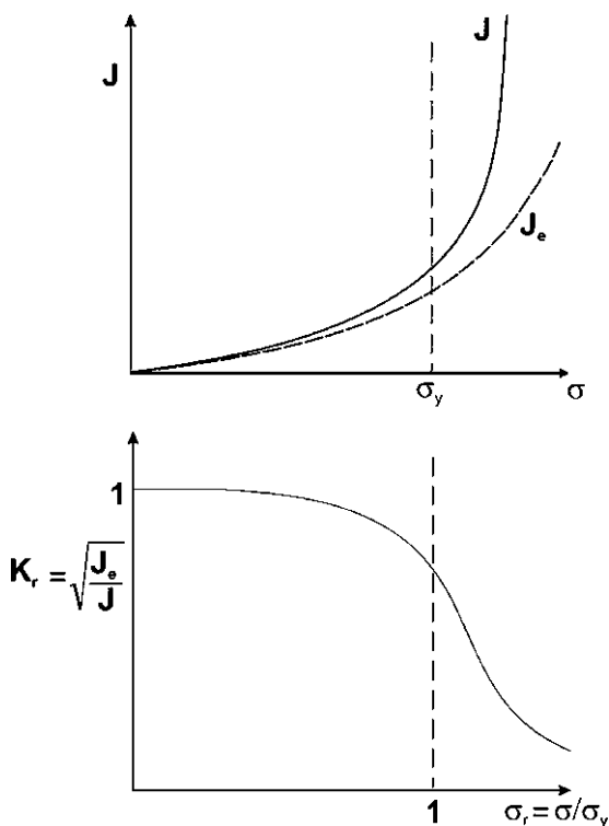
Fig. 8 Construction of FAD using EPFM
