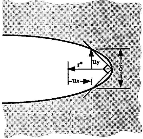
Fig. 5 Definition of CTOD
