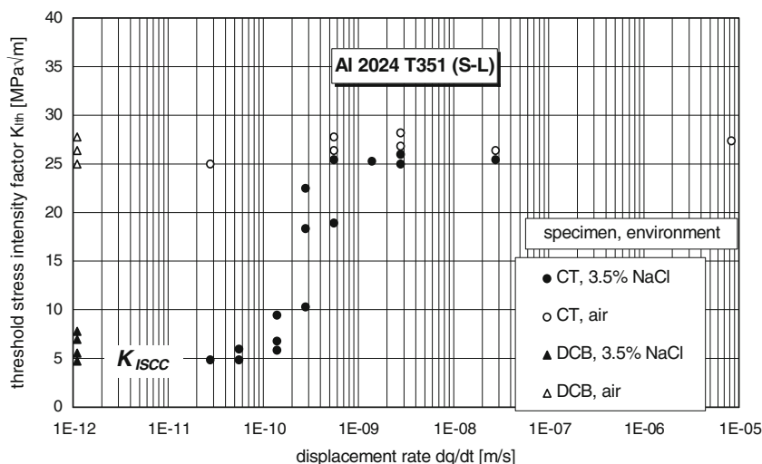
Fig. 1 Influence of the displacement rate, dq/dt , on the stress intensity factor at crack initiation, K_{Ith} , measured in rising displacement tests on CT specimens (circles); the results of long term constant displacement tests (10,000 h) on DCB specimens are shown for comparison (triangles) [2]
