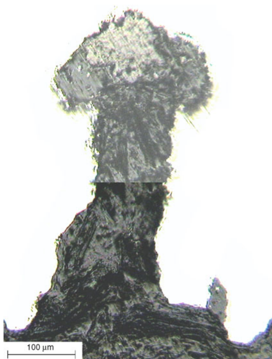
Fig. 9 Photograph of a blunt crack and the blunt crack tip on R-T surface for a specimen cyclically loaded in C2 solution under condition B-1
