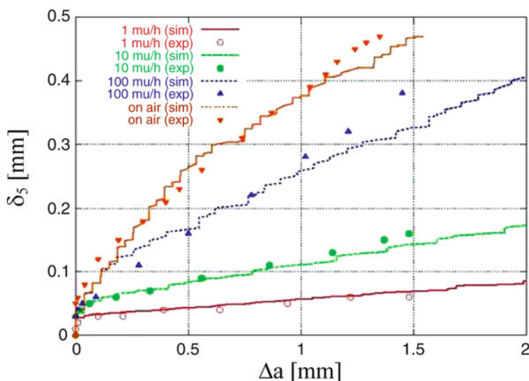
Fig. 7 Comparison of experimental and simulated CTOD R-curves under hydrogen charging conditions and in laboratory air (displacement rates: 1, 10 and 100 \mu\text{m/h} , cf. Fig. 5) [21, 22]
