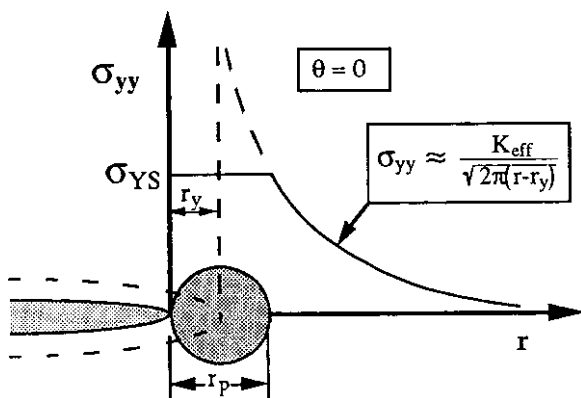
Fig. 3 Irwin plastic zone correction [6]
