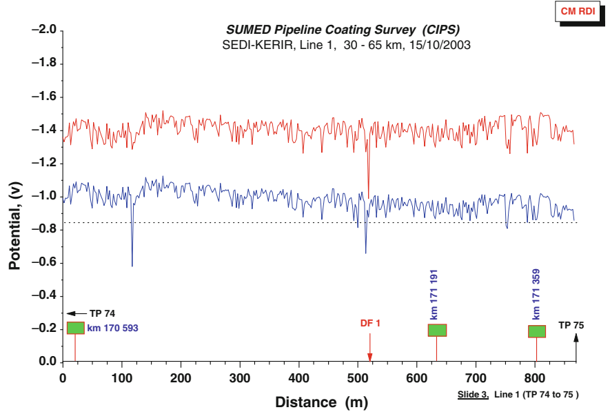
Fig. 8 CIPS graph showing one coating defect irrespective of spike of deceptive potential spikes
