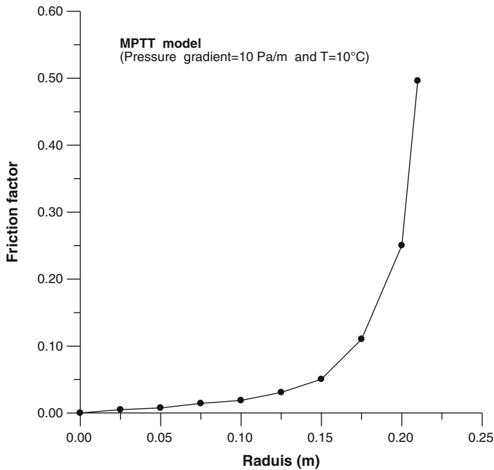
Fig. 9 Friction factor according to pipe radius for \Delta p/L= 10 \text{ Pa/m} and T=10^{\circ}\text{C}
