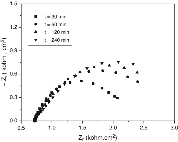
Fig. 4 Nyquist slopes for low carbon steel in NS4 simulating solution of corrosive soil environment (pH \approx 6.7) at different immersion times (t = 30°C)
