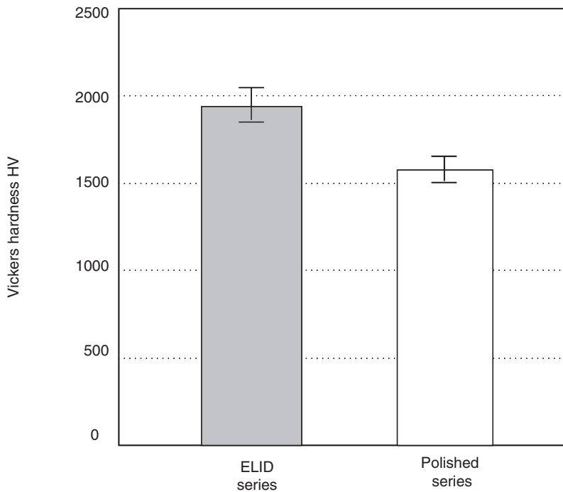
FIGURE 6.25 Results of hardness measurements using a nanoindenter.
