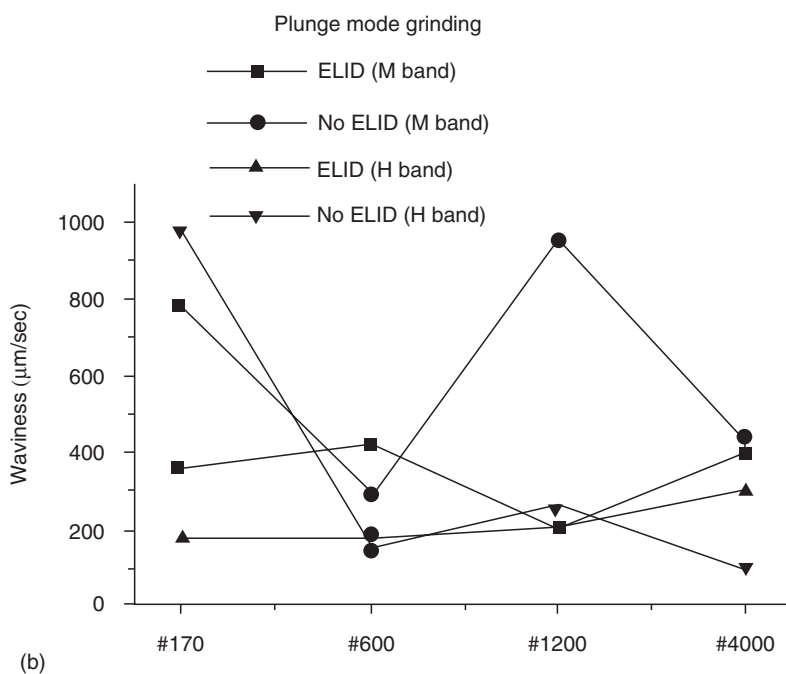
FIGURE 9.26 Comparison of waviness: (a) traverse; (b) plunge.
