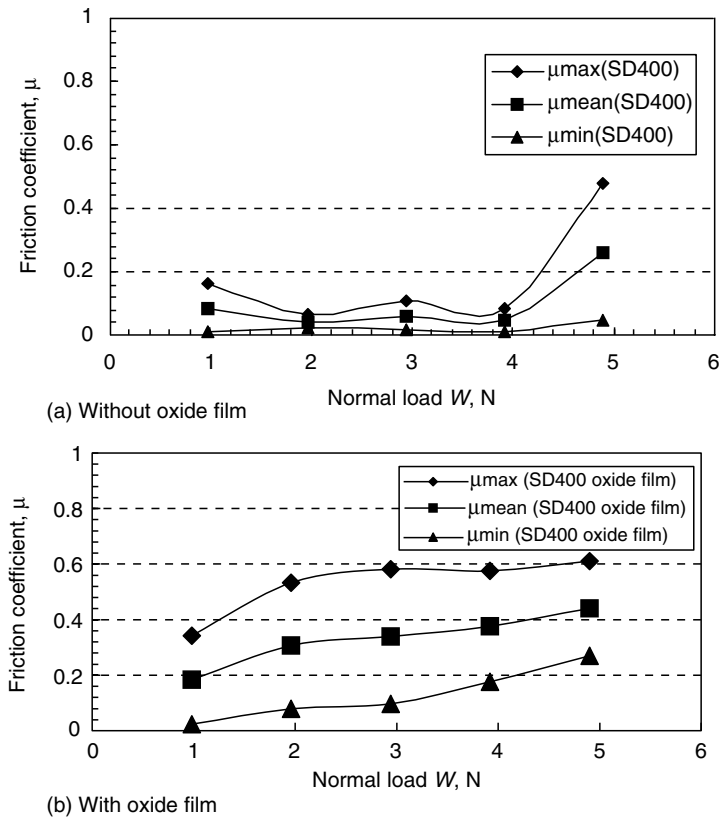
FIGURE 15.7 Relationship between normal load and friction coefficient at initial friction stage.
