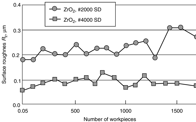
FIGURE 6.13 Change of surface roughness for grinding number of ZrO 2 optical fiber ferrule.
