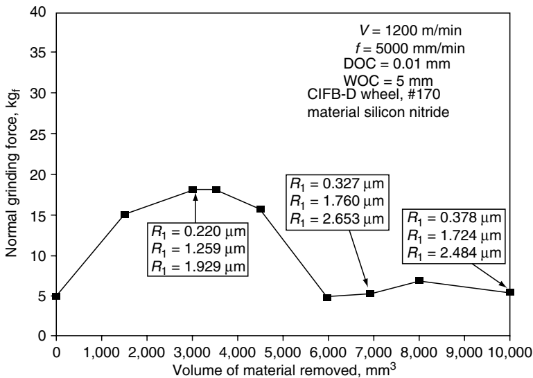
FIGURE 5.19 Relationship between the volume of material removed and the normal grinding force (ELID grinding; V = 90 V; I_p = 24 A; \tau_{on} = \tau_{off} = 4 \mu sec).
