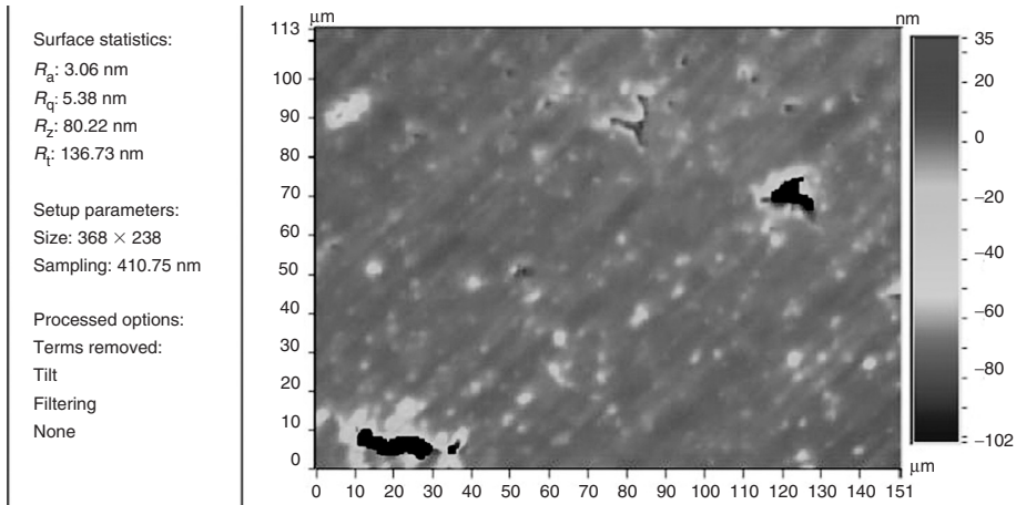
FIGURE 6.18 Surface roughness and topography.
