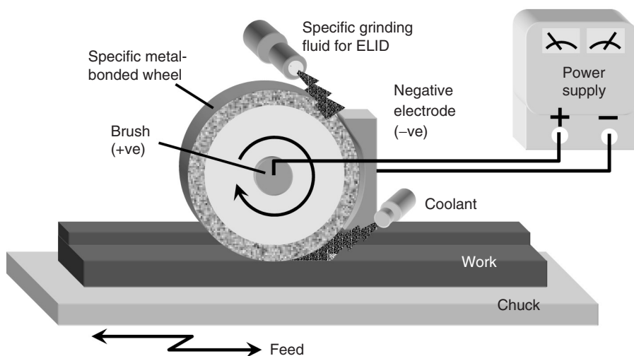
FIGURE 6.2 The principle of ELID grinding.
