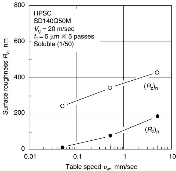
FIGURE 2.11 Relationship between the ground HPSC surface roughness and the table speed.
