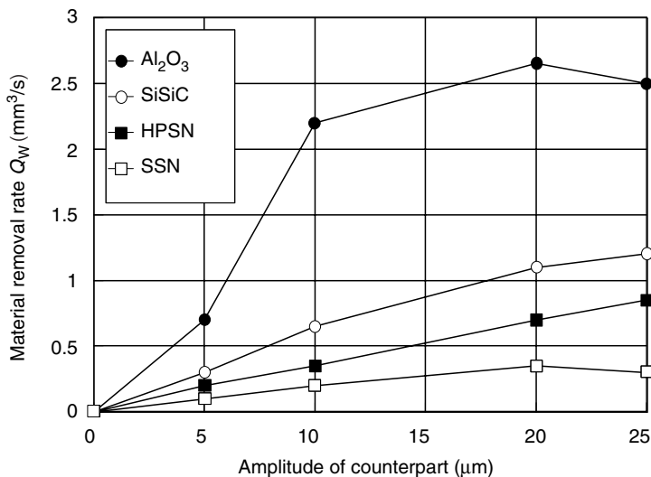
FIGURE 17.8 Relation of material removal rate and amplitude of shape-generating counterpart (abrasive: \text{B}_4\text{C} F280). (From Grathwohl, G. et al., Materialwissenschaft und Werkstofftechnik, Vol. 19, Germany, S81–86, 1988.)
