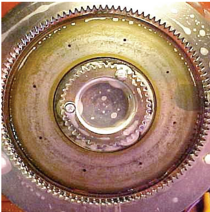
FIGURE 12.12 Radial wear gradient of the diamond wheel.
