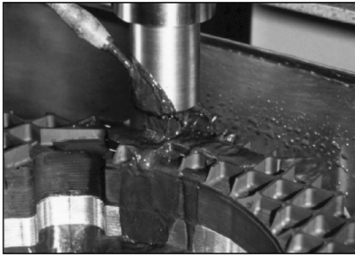
FIGURE 17.2 Process of ultrasonic lapping and machining (Photo from MAFELL Company, Oberndorf, a.n., Germany.)
