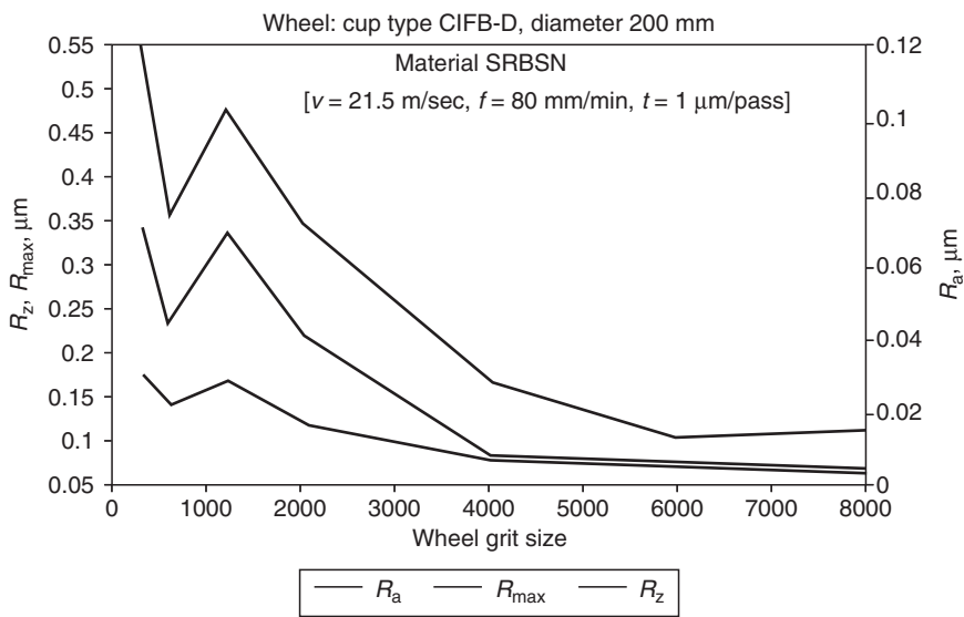
FIGURE 5.32 The effect of wheel grit size on surface finish.
