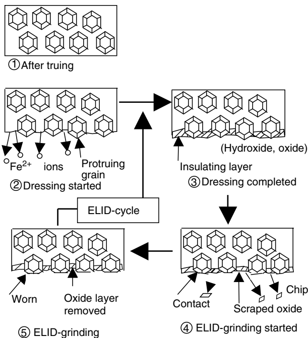
FIGURE 15.1 ELID-grinding mechanisms.
