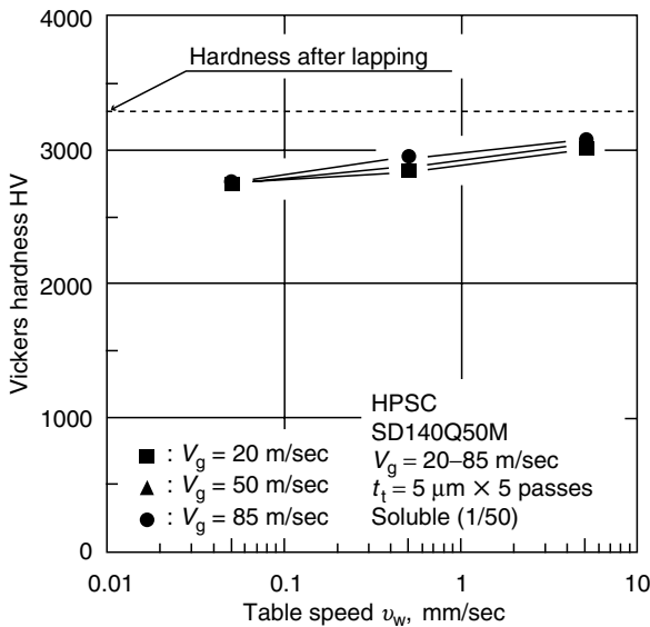
FIGURE 2.15 Influence of the ground workpiece hardness on the wheel speed.
