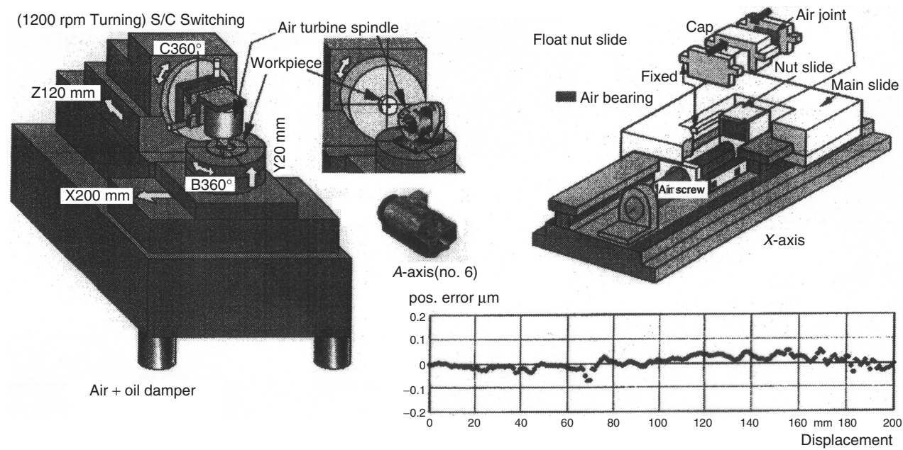
FIGURE 1.21 Schematic of the ultraprecision machining center developed by Y. Takeuchi et al. (From Takeuchi et al., Annu CIRP , 45, 1 (1996) 401.)
