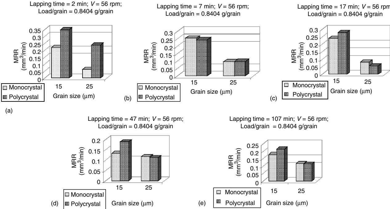
FIGURE 10.6 Material removal rate versus grain size (15 and 25 μm).
