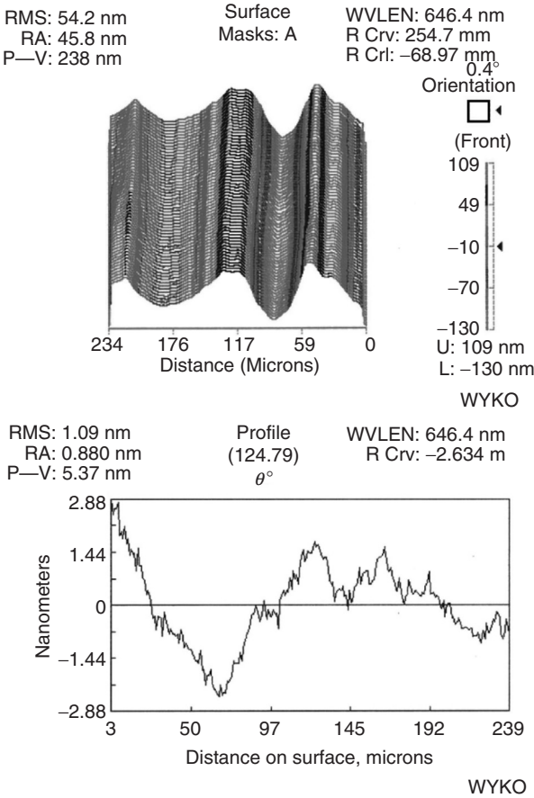
FIGURE 2.13 A WYKO 3D image and 2D profile of the HSPC surface ground at v_w = 0.05 mm/sec under V_g = 85 m/sec with the #140-mesh wheel [SD140Q50M, V_g = 20 m/sec, t_t = 5 \mu m, Soluble (1/50)].
