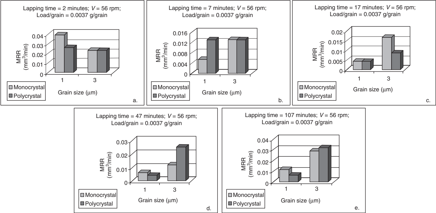
FIGURE 10.5 Material removal rate versus grain size (1 and 3 μm).
