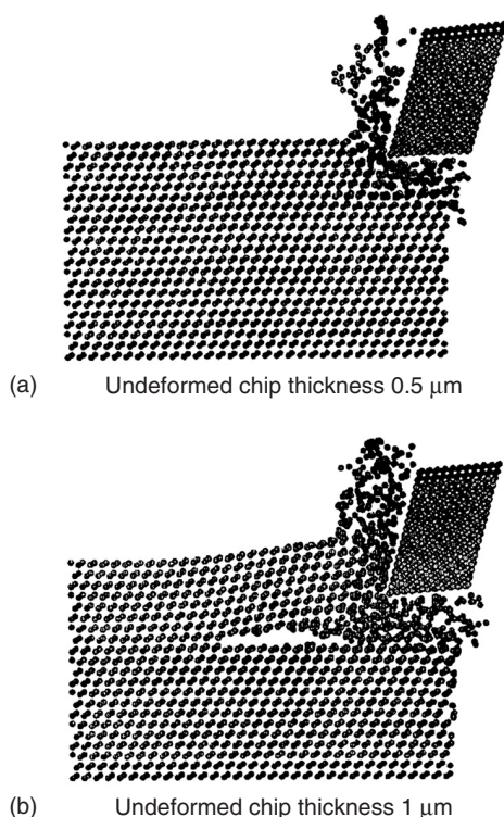
FIGURE 1.5 Result of simulation obtained by taking into account the effect of atmospheric gas.
