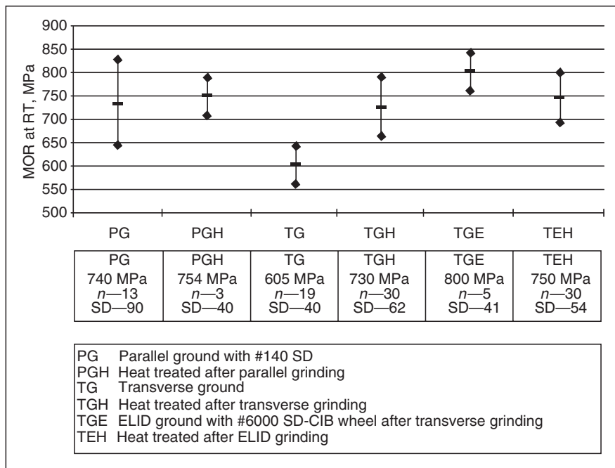
FIGURE 5.37 The effect of ELID grinding on the strength of \text{Si}_3\text{N}_4 .
