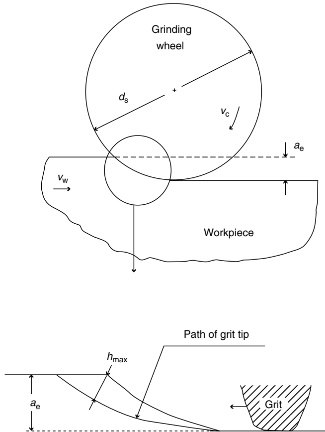
FIGURE 4.1 Illustration of the surface grinding process showing various process variables.
