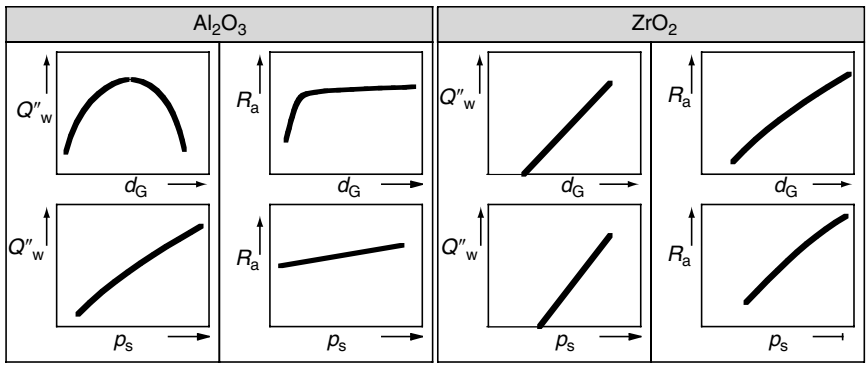
FIGURE 16.1 Material removal rate and roughness in relation to diamond grain size and stone pressure during honing of oxide ceramic materials. (From Weigmann, U-P.: Honen keramischer Werkstoffe. Dissertation TU Berlin, 1997. With permission.)
