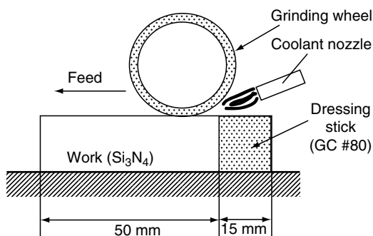
FIGURE 5.2 Schematic diagram of in-process dressing method with a dressing stick.
