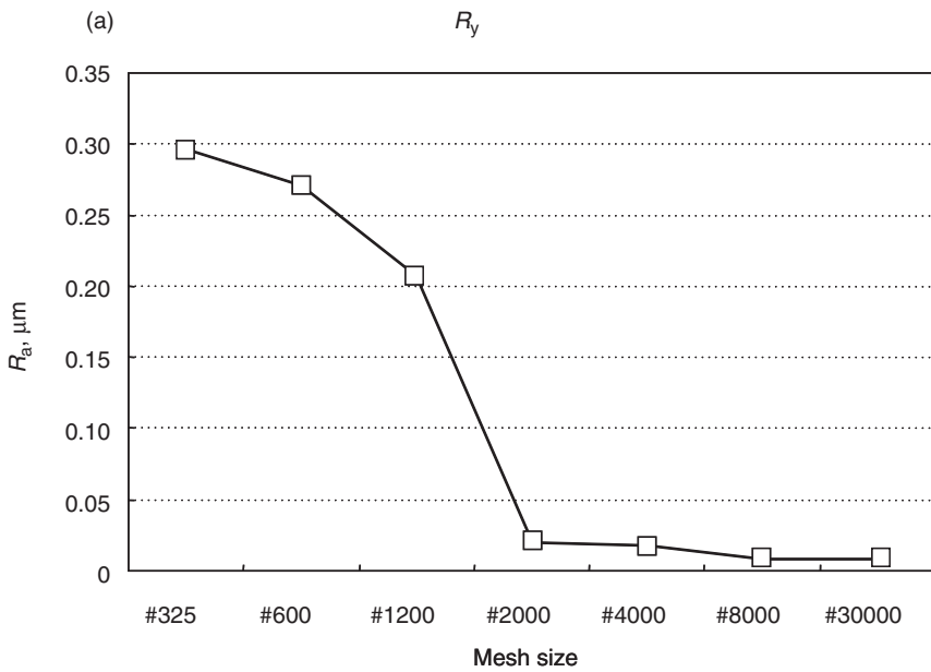
FIGURE 6.20 Relation between mesh size and surface roughness.
