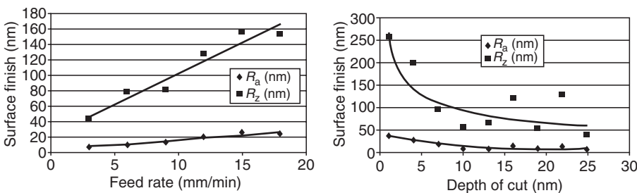
FIGURE 9.34 Surface finish vs. feed rate and depth of cut. (From Stephenson, D.J., Veselovac, D., Manley, S., and Corbett, J., J Int Soc Prec Eng Nanotechnol , 25, 336, 2001. With permission.)
