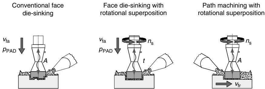
FIGURE 17.4 Process variants of ultrasonic lapping.
