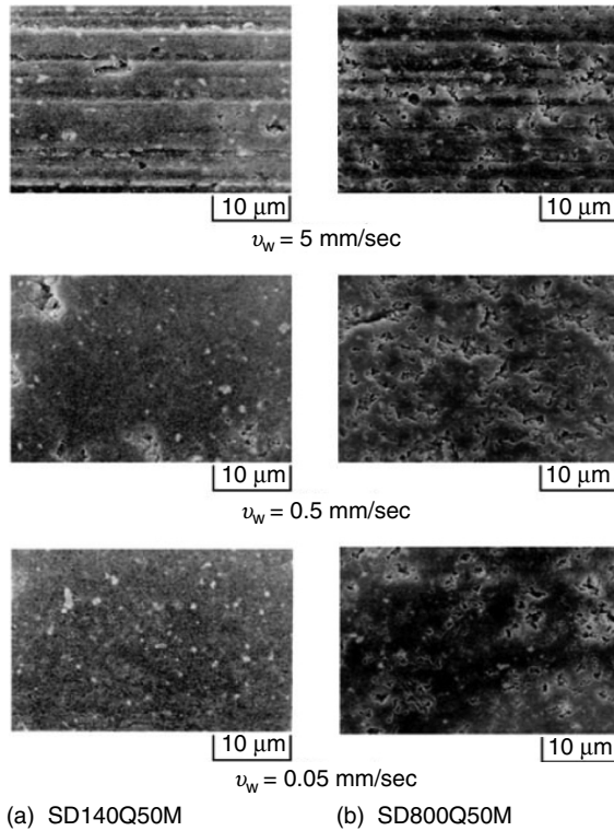
FIGURE 2.18 Influence of the table speed and wheel grain size on the ground HIPSN surface [ V_g = 20 m/sec, t_t = 5 \mu m, Soluble (1/50)].
