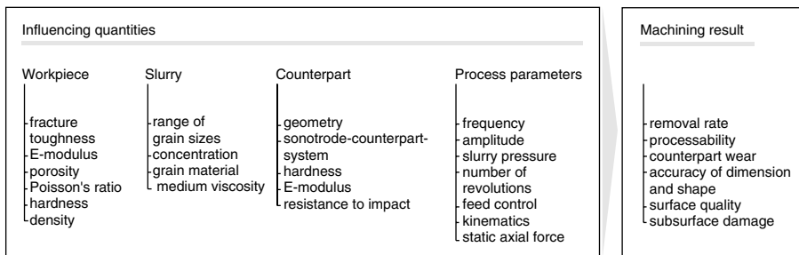
FIGURE 17.3 Influences on machining result during ultrasonic lapping.
