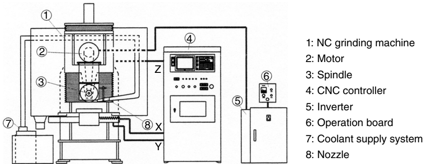
FIGURE 2.22 Schematic diagram of NC grinding machine.
