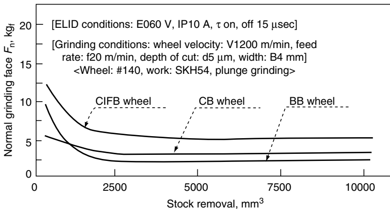
FIGURE 5.13 Difference in grinding force due to wheel bond material.
