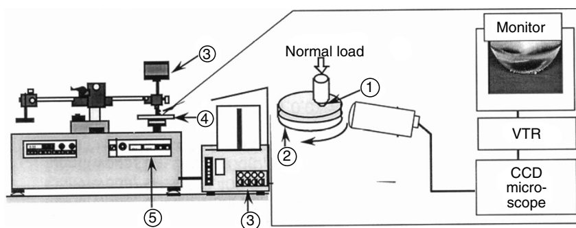
FIGURE 15.2 Schematic diagram of the CCD microscope tribosystem.
