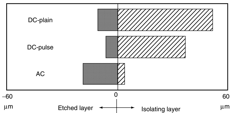
FIGURE 5.15 Difference in insulating layer and etched layer thickness due to power source.
