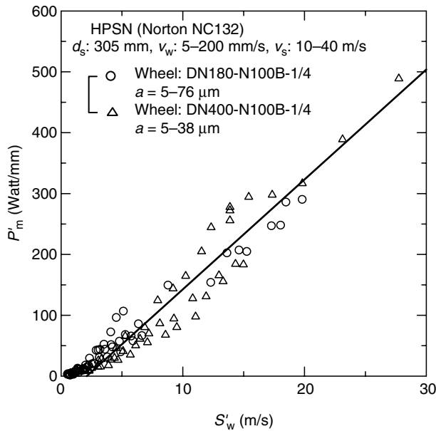
FIGURE 3.17 Power per unit width versus rate of plowed surface area generated per unit width.
