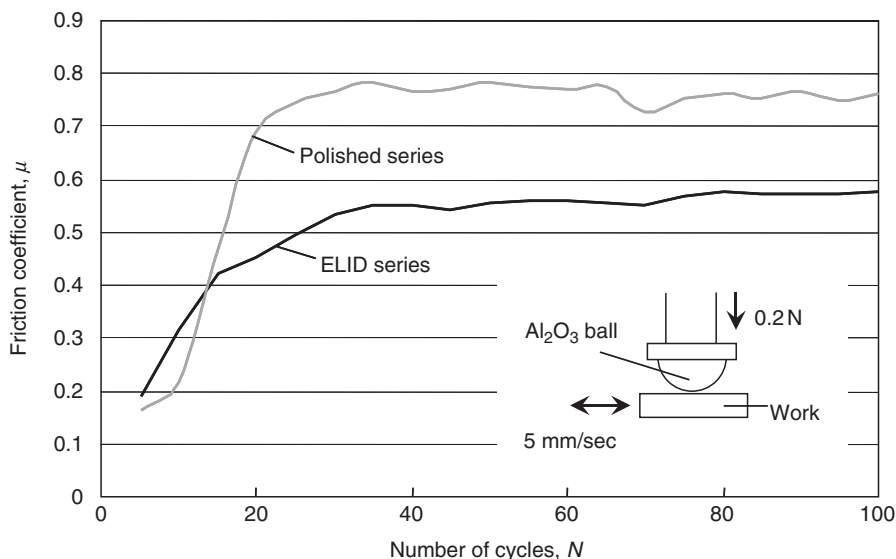
FIGURE 6.26 Relation between the frictional coefficient \mu and the number of sliding cycles.
