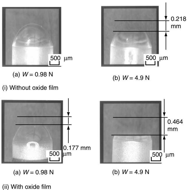
FIGURE 15.4 Worn pin specimens.
