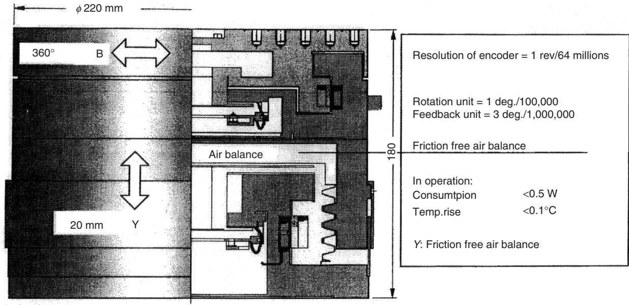
FIGURE 1.22 Intelligent ultraprecision unit with rotary table B ( \pm 0.04 \mu\text{m}/\phi 200 \text{ mm} ) and up-down feed Y-axis unit.
