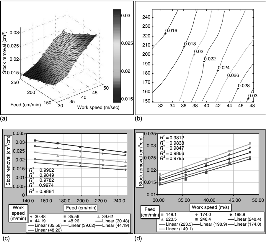
FIGURE 7.7 (a) Stock removal vs. feed and belt speed. (b) Contour bands for several values of stock removal. (c) Stock removal vs. feed for each of the used belt speeds. The sample coefficient of determination, R^2 , is also shown. (d) Stock removal vs. belt speed for each of the used feeds. The sample coefficient of determination, R^2 , is also shown.
