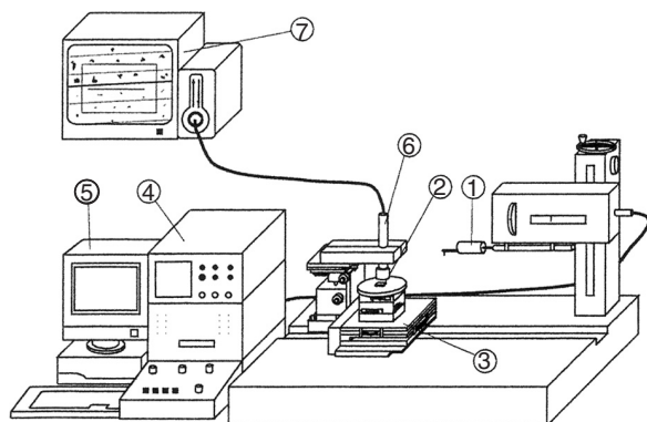
1. Stylus 2. Specimen 3. XTθ – stage 4. Profilometer 5. Personal computer 6. CCD camera 7. Monitor
