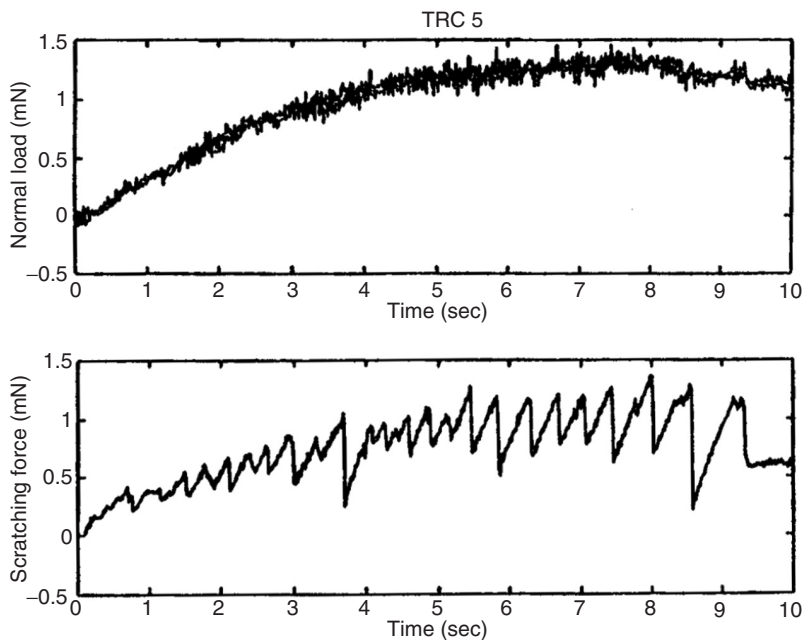
FIGURE 1.10 Force data measured during brittle scratching on surface of TRC 5, where scratching velocity was 5 mm/sec.
