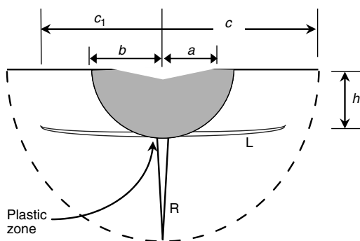
FIGURE 3.1 Plastic zone, median/radial cracks (R), and lateral cracks (L) for Vickers indentation. (From Lawn, B.R. and Swain, M.V., J. Mater. Sci. , 10, 113, 1975. With permission.)
