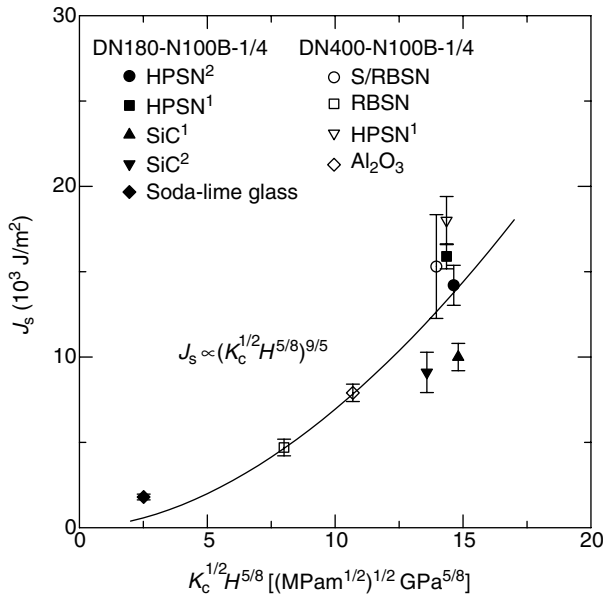
FIGURE 3.19 Plowed surface energy per unit area versus K_c^{1/2} H^{5/8} . (From Hwang, T.W. and Malkin, S., ASME J. Manuf. Sci. Eng. , 121, 623. With permission.)
