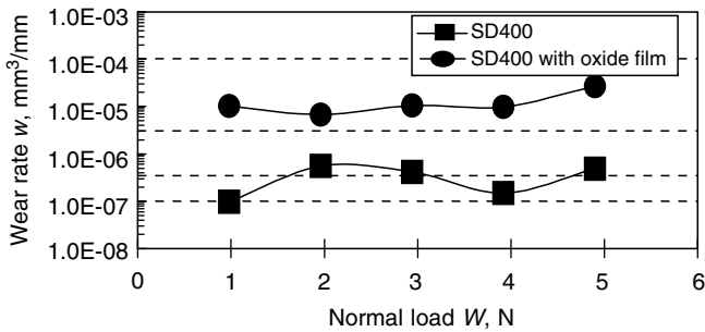
FIGURE 15.8 Relationship between normal load and wear rate of the wheel.
