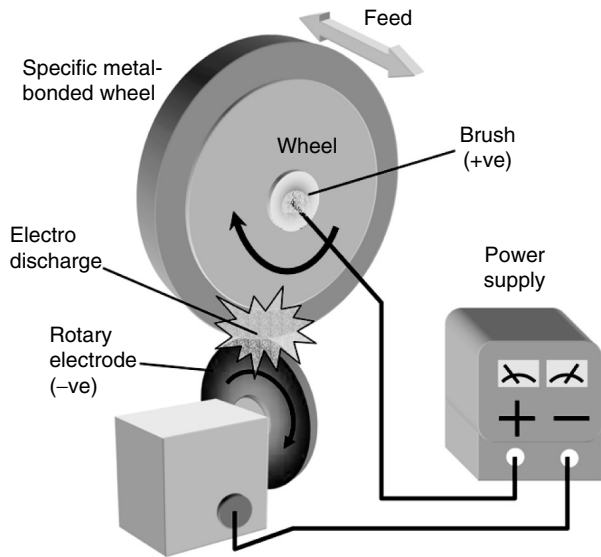
FIGURE 6.3 Overview of machine setup with electrodischarge truer. The ED truing system.
