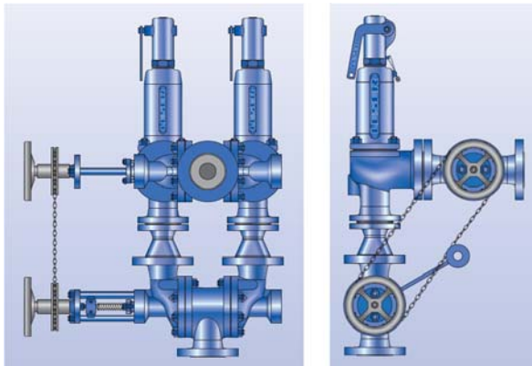
Figure 6.4.5-1: Lockable combination
