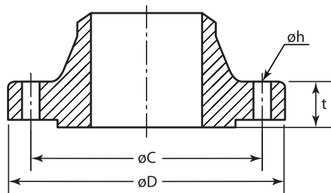
Figure 10.5.2-1: JIS B 2220 – types of flanges made of steel
