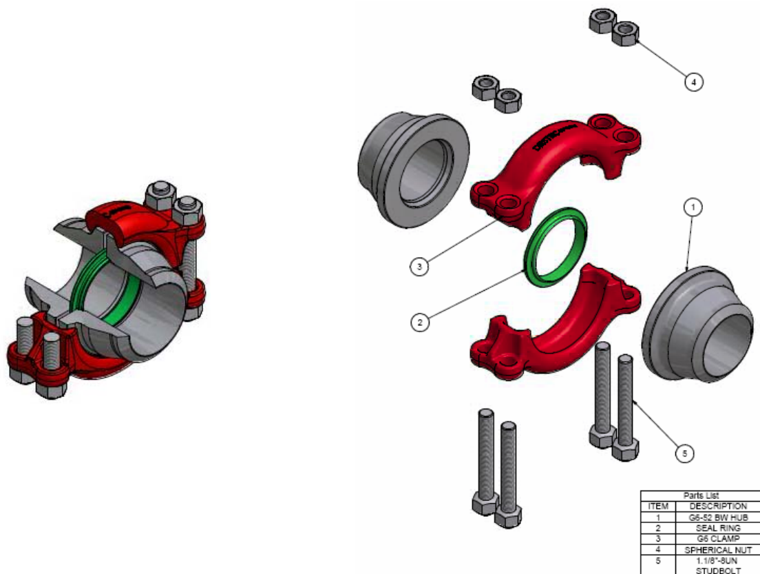
Figure 10.9-1: GRAYLOC connector
