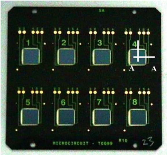
Fig. 6.3 FCOB test vehicle
