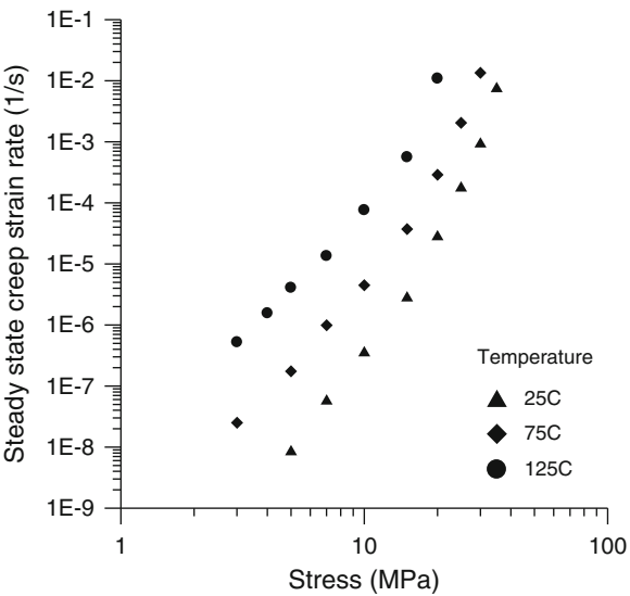
Fig. 3.25 Steady state creep behavior of Sn–Cu
