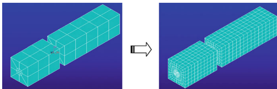
Fig. 5.7 Cut boundary for submodel (cb1)
