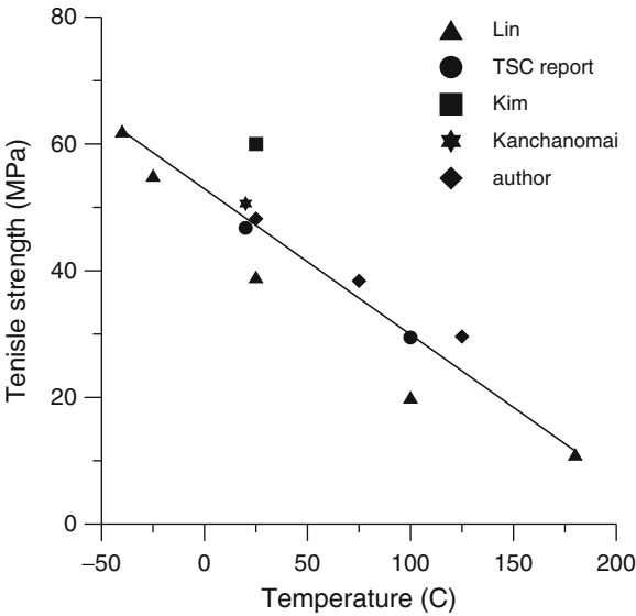
Fig. 3.15 Tensile strength for Sn–Ag–Cu
