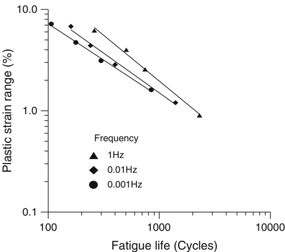
Fig. 4.9 Plastic strain versus fatigue life at 125°C for different frequencies
