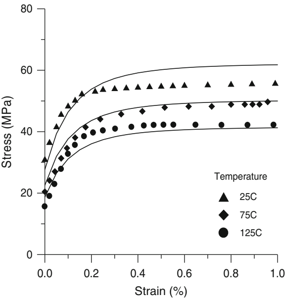
Fig. 3.34 Anand model at strain rate of 5.6 \times 10^{-2} \text{ s}^{-1}
