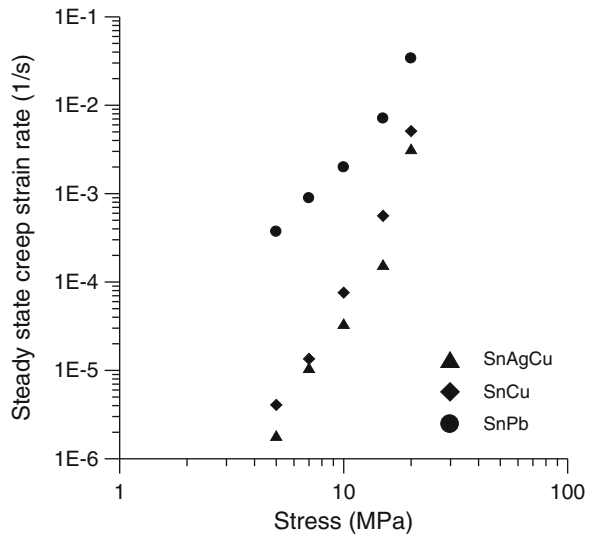
Fig. 3.27 Comparison of creep resistance at 125°C
