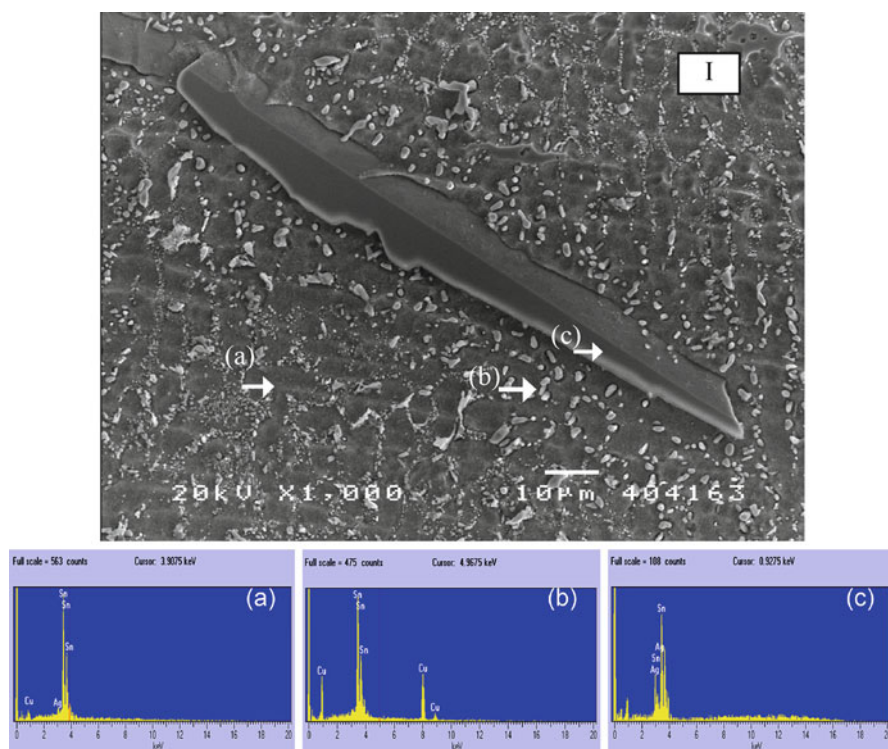
Fig. 6.24 The IMC and EDX features in the solder joint, plot I in Fig. 6.28. (a) Sn-rich; (b) Cu 6 Sn 5 ; (c) Ag 3 Sn
