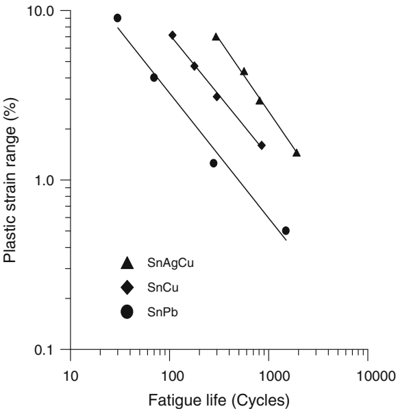
Fig. 4.12 Fatigue data at 125°C and 10 -3 Hz
