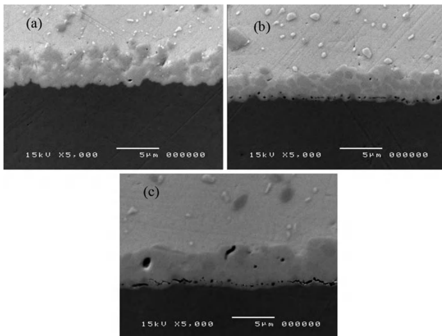
Fig. 8.12 SAC solder to copper pad interface after \text{Ar}^+ sputtering etch (a) as reflowed specimen, (b) TC 500 Kirkendall voids formed and occupied about 10% of the interface, and (c) TC 1,000, growth of Kirkendall voids is noted, micro-crack could be seen at the interface
