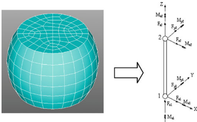
Fig. 5.14 FE model of a solder ball and its simple two-node beam element
