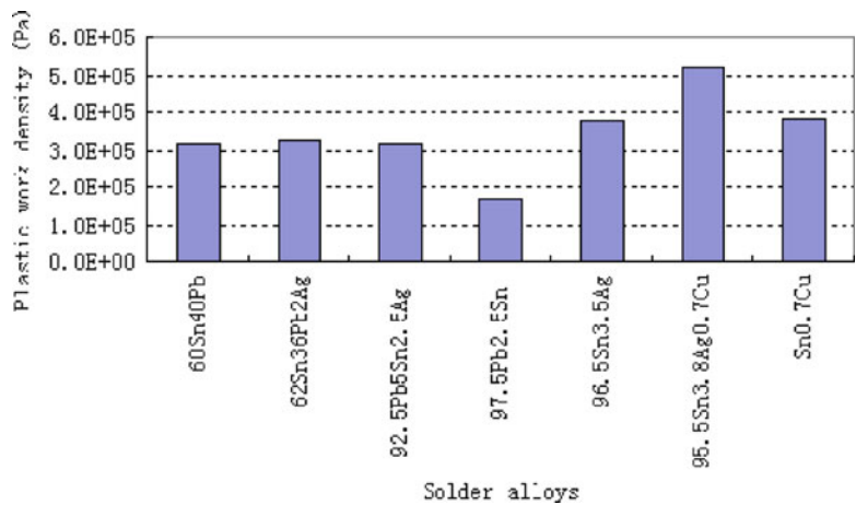
Fig. 5.17 Plastic work density comparisons for different solder joints
