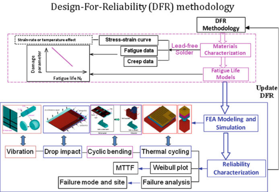
Fig. 1.2 DFR approach for FEA modeling and fatigue analysis
