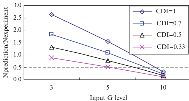
Fig. 7.15 CDI effect on fatigue life prediction
