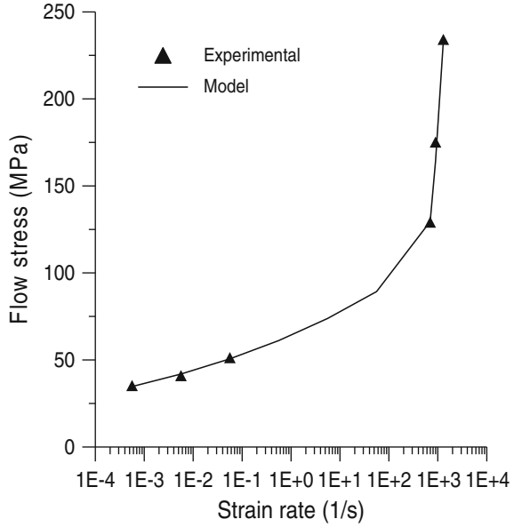
Fig. 3.22 Flow stress versus strain rate for SAC387
