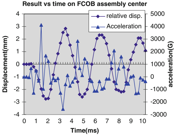
Fig. 7.32 Acceleration, displacement versus time
