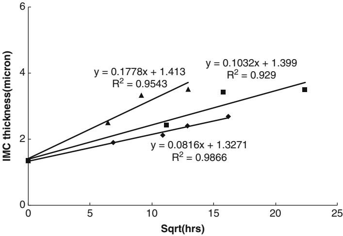
Fig. 6.27 Comparison of IMC data for TC, TS, and isothermal aging at 125°C. ( filled diamond ) ISO 125, ( filled square ) TC, ( filled triangle ) TS
