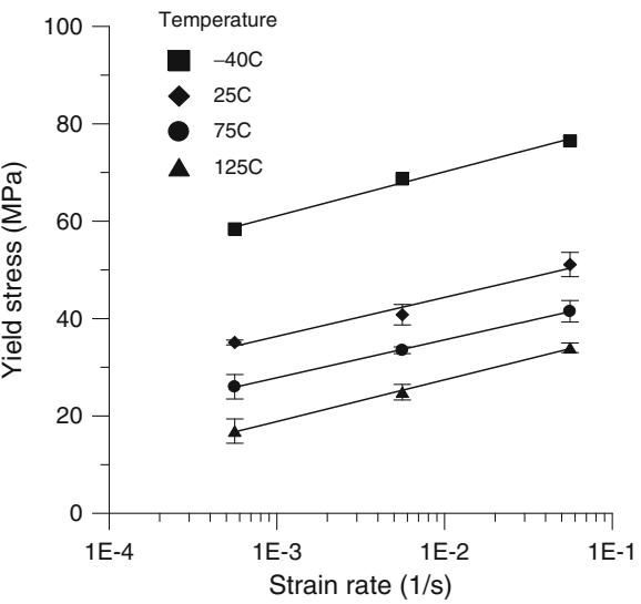
Fig. 3.9 Effect of strain rate on yield stress
