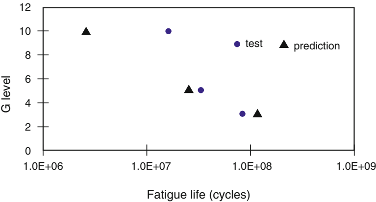
Fig. 7.14 G-N curve for different methods
