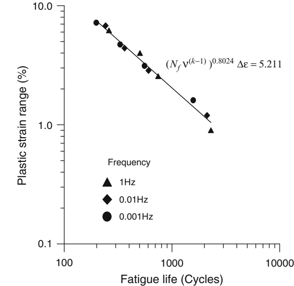
Fig. 4.16 Plastic strain versus frequency-modified fatigue life at 125°C for Sn-Cu ( k = 0.91 )
