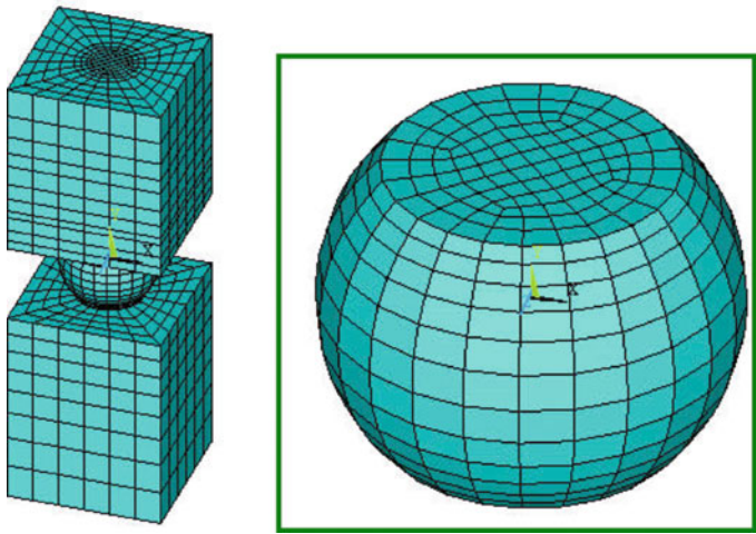
Fig. 6.16 Submodel including one critical BGA solder joint
