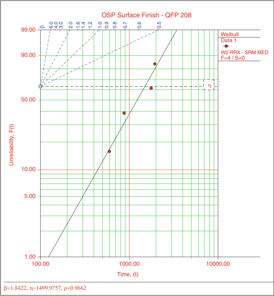
Fig. 6.13 Weibull plot for PQFP208 component with OSP surface finish
