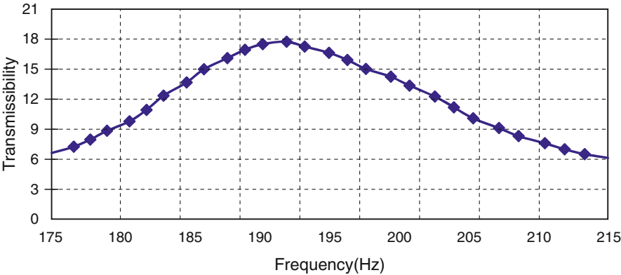
Fig. 7.13 Transmissibility versus frequency for 3G test
