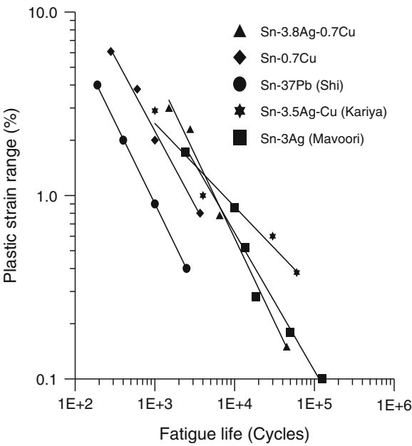
Fig. 4.13 Fatigue data for tin-lead and lead-free solders at 25°C and 1 Hz
