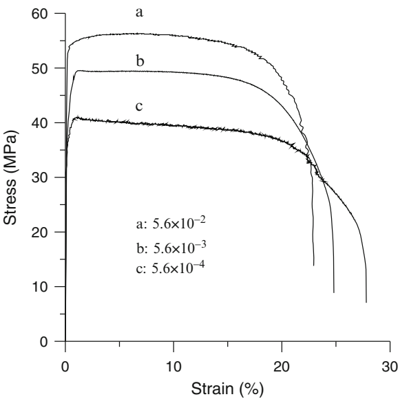
Fig. 3.4 Tensile test results at 25°C
