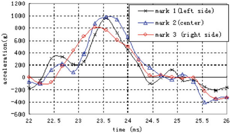
Fig. 7.20 Acceleration of the specimen (camera)
