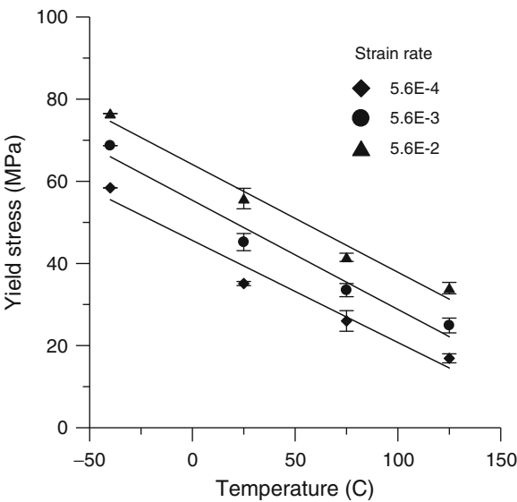
Fig. 3.8 Effect of temperature on yield stress
