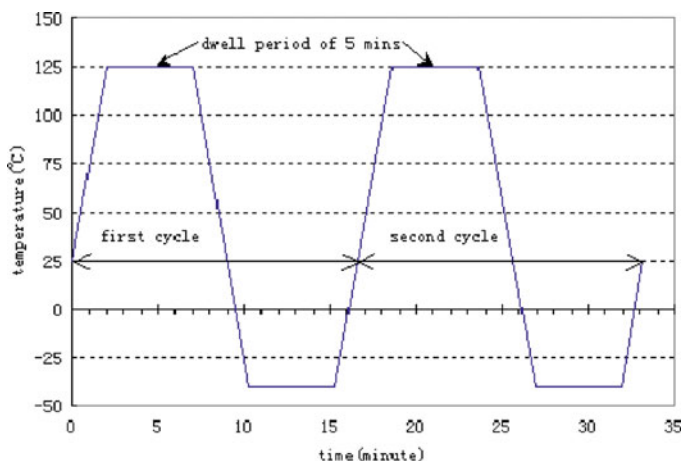
Fig. 5.10 Thermal cycling loading profile
