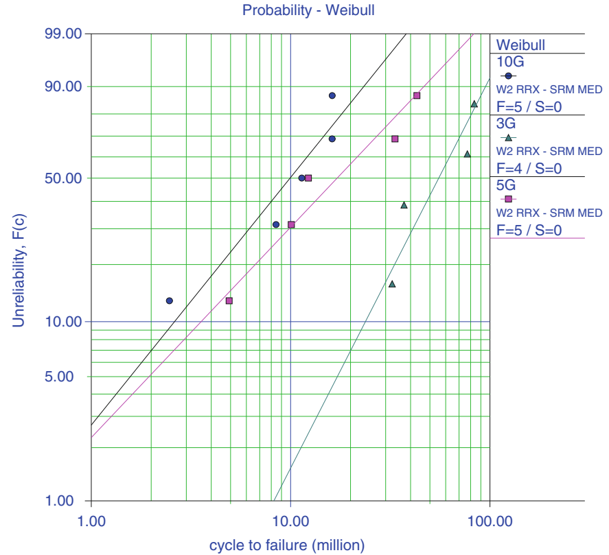
Fig. 7.4 Weibull plots of test results for different G_{in}
