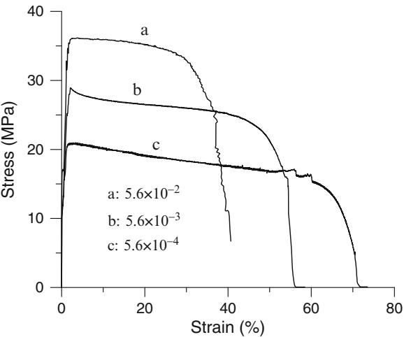
Fig. 3.5 Tensile test results at 125°C
