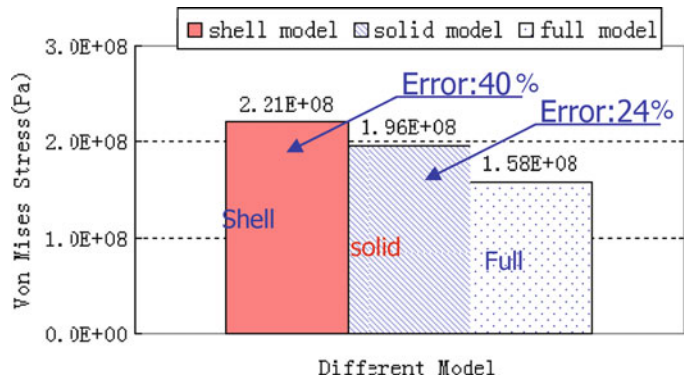
Fig. 5.15 Von Mises stress comparison for different model
