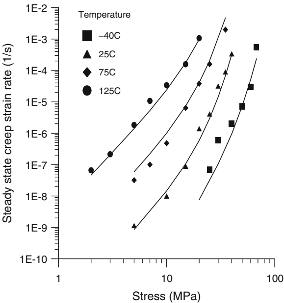
Fig. 3.30 Hyperbolic-sine model of Sn–Ag–Cu
