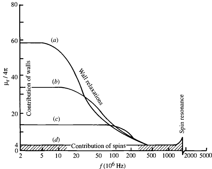
Fig. 4.59. Permeability spectra of \text{NiFe}_2\text{O}_4 samples with different grain size: (a) 11\text{ }\mu\text{m} ; (b) 5\text{ }\mu\text{m} ; (c) 2\text{ }\mu\text{m} ; and (d) size < 0.2\text{ }\mu\text{m} (single-domain behaviour) (Globus, 1962).
