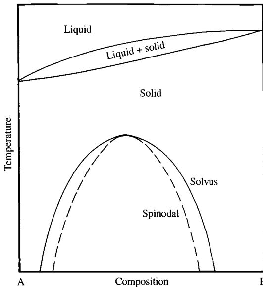
Fig. 6.25. Phase diagram of a spinodal decomposition (schematic).
