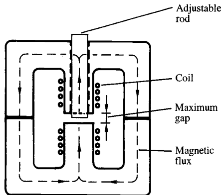
Fig. 5.7. Cross-sectional view of a pot core, showing the adjustable gap (schematic).
