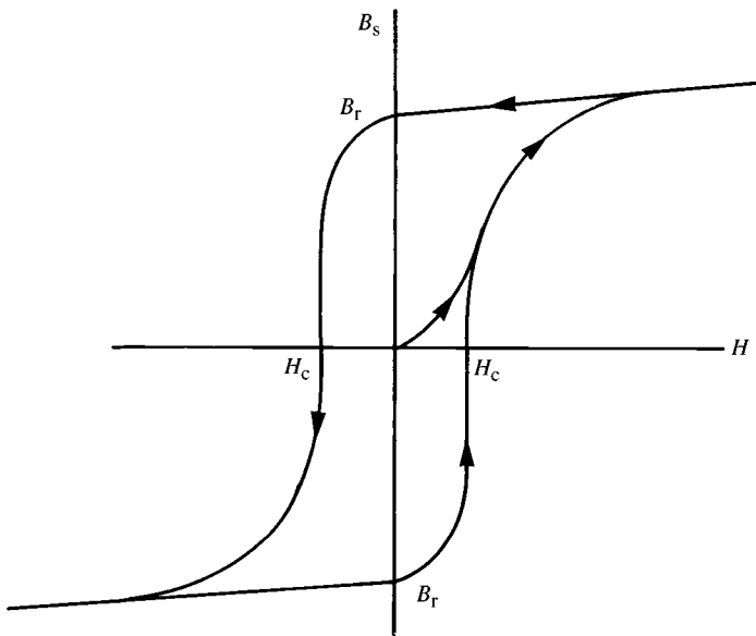
Fig. 4.40. Schematic hysteresis loop. B_s and B_r are the saturation and remanent inductions, respectively; the coercive field is H_c .
