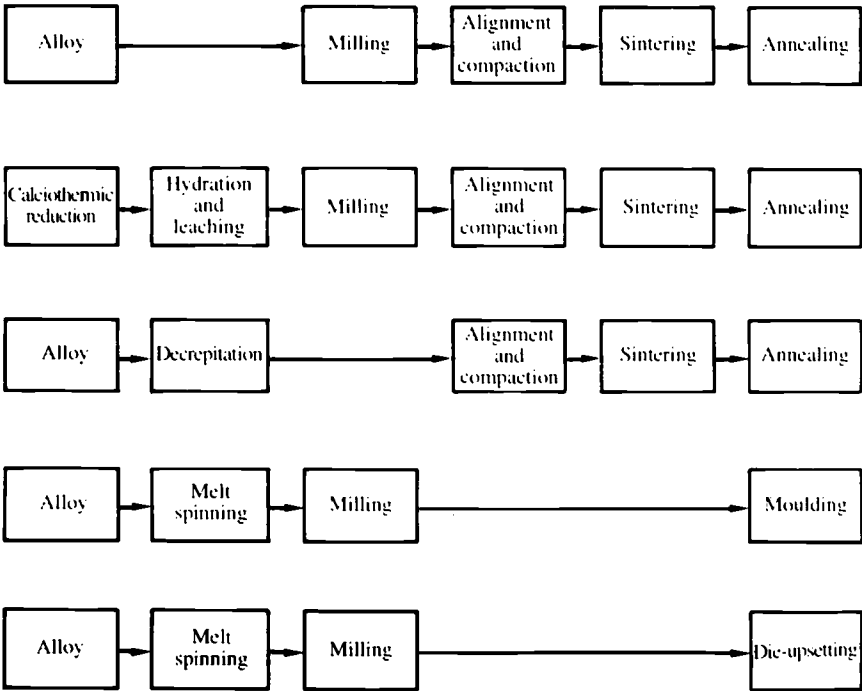
Fig. 6.31. Schematic preparation routes for Nd-Fe-B permanent magnets.
