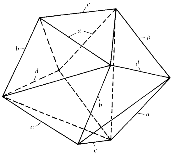
Fig. 2.19. Dodecahedral polyhedron in c sites; edge lengths are (in Å): a 2.68; b 2.81; c 2.87; and d 2.96. (Adapted from Geller & Gilleo, 1957.)
