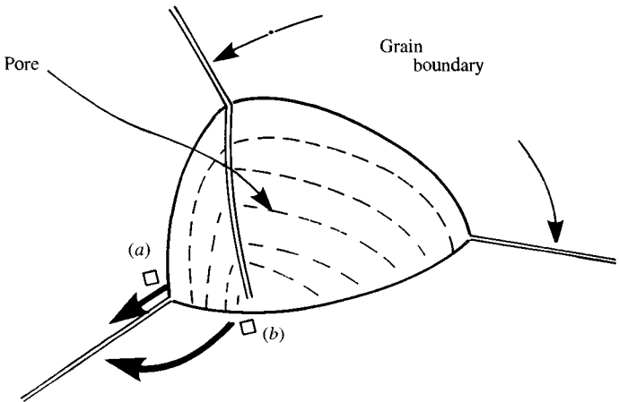
Fig. 3.11. Model for elimination of porosity. Vacancy flux by: (a) grain boundary diffusion, (b) volume diffusion.
