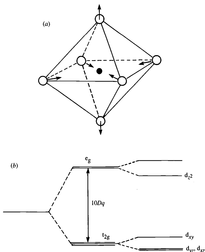
Fig. 2.12. (a) Deformation of a regular octahedron along the z -axis to produce c/a > 1 . A small contraction is also produced in the x - and y -axes; (b) schematic energy level diagram showing the free-atom degenerated levels, the splitting for a regular octahedron and for a distorted octahedron. (Adapted from Dunitz & Orgel, 1957.)
