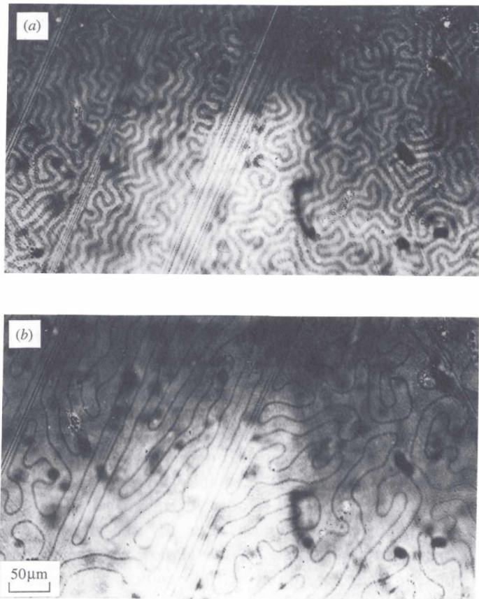
Fig. 4.32. Magnetic domains in a YIG single-crystal platelet, observed by the Faraday effect: (a) zero field; (b) field normal to the platelet plane ( H \sim 40 A/m).
