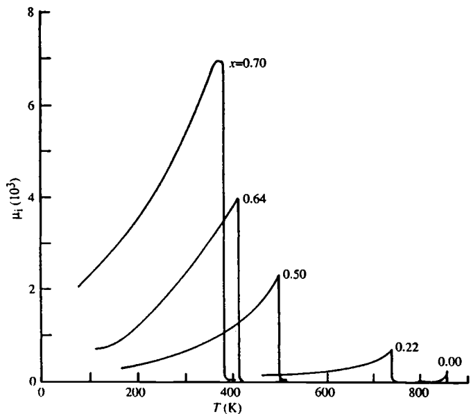
Fig. 4.47. Initial permeability as a function of temperature in \text{Zn}_x\text{Ni}_{1-x} spinels for various compositions.
