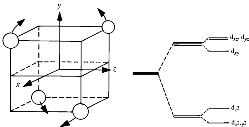
Fig. 2.13. Deformation of a tetrahedron to produce c/a > 1 and the corresponding energy level diagram. (Adapted from Dunitz & Orgel, 1957.)
