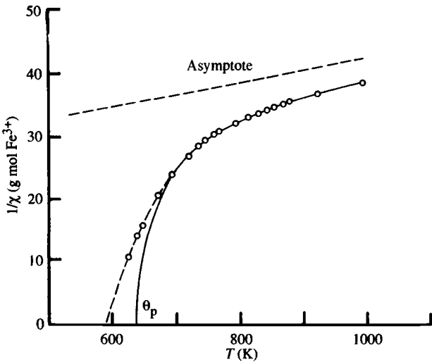
Fig. 4.18. The inverse susceptibility of Mg ferrite as a function of temperature for T > T_C , referred to one mole of \text{Fe}^{3+} . The solid line and \theta_p correspond to Eq. (4.33). (Adapted from Cullity, 1972; data from Serres, 1932; curve constants from Néel, 1948.)
