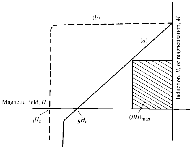
Fig. 6.23. Comparison between (a) induction, B , and (b) magnetisation, M , curves, as a function of applied field to illustrate the difference between coercivity, {}_B H_c , and intrinsic coercive field, {}_i H_c .
