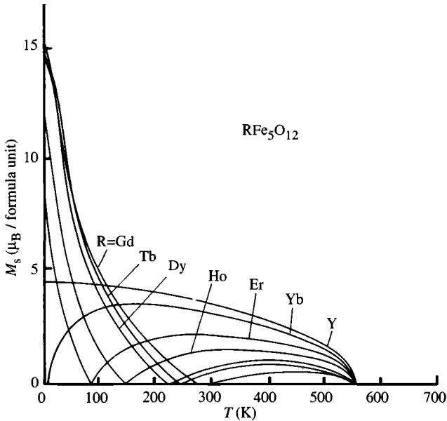
Fig. 4.23. Saturation magnetisation (in Bohr magnetons per formula unit) as a function of temperature, for rare-earth garnets RFe_5O_{12} , where R = Gd, Tb, Dy, Ho, Er, Yb and Y. (Adapted from Moulson & Herbert, 1990.)
