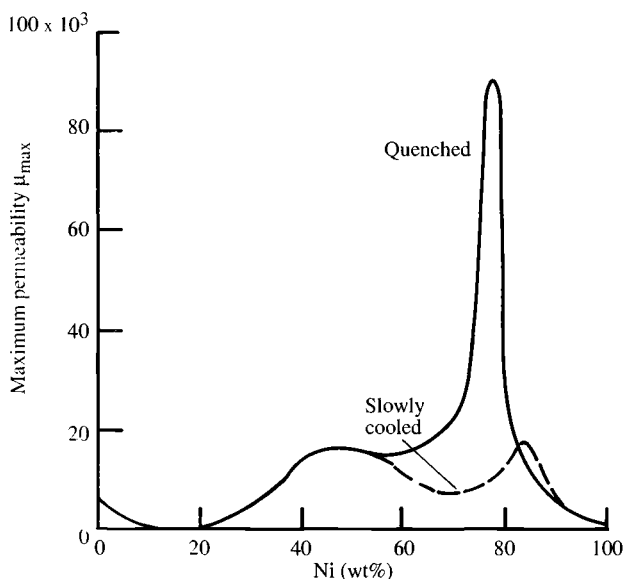
Fig. 6.7. Effects of cooling rate on maximum permeabilities of Ni–Fe alloys. (Adapted from Bozorth, 1953.)
