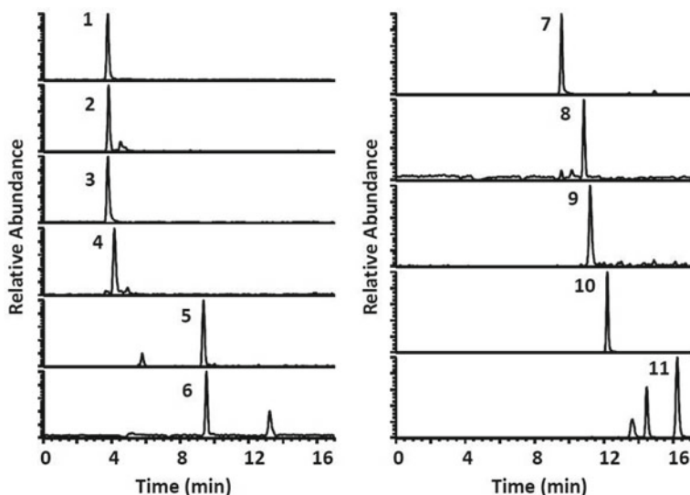
Fig. 8.13 Ion chromatography coupled with mass spectrometry for analysis of metabolites in mouse quadriceps muscle. The consecutive elution peaks correspond to (1) lactate, (2) pantothenate, (3) 3-hydroxyisobutyrate, (4) 2-hydroxybutyrate, (5) hippurate, (6) succinate, (7) malate, (8) fumarate, (9) pyruvate, (10) citrate, (11) 2-ketoglutarate. Reproduced (or adapted) from [66], ©2016, with permission from ACS publication
