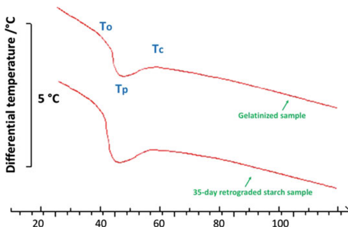
Fig. 5.12 DTA curves for the gelatinized and the 35-day retrograded starch specimens made from rice starch with low-level amylose. Reproduced (or adapted) with permission [55], © 2011, Elsevier
