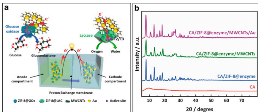
Fig. 4.23 a The components and operating principle of the EBFCs-based self-powered glucose detector. b The XRD patterns of each element. Reproduced (or adapted) with the permission [127], © 2021, Elsevier
