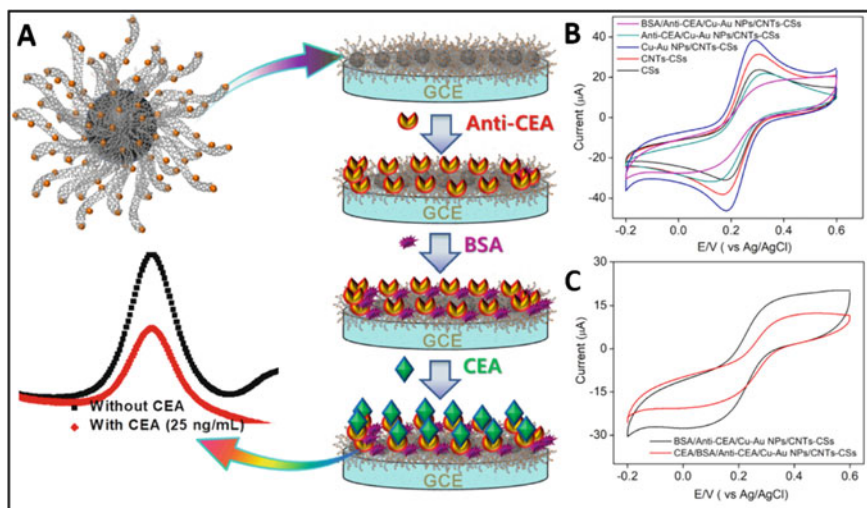
Fig. 7.4 a Fabrication of an electrochemical sensor for the identification of CEA. b CV curves of modified GCE in 0.1 M KCl with 5 mM \text{K}_4[\text{Fe}(\text{CN})_6] at a scan rate of 50 \text{mV s}^{-1} and c CV curves of BSA/anti-CEA/Cu-Au NPs/CNTs-CSs modified GCE with and without 25 \text{ng mL}^{-1} of CEA in 0.1 M KCl containing 5 mM \text{K}_4[\text{Fe}(\text{CN})_6] at a scan rate of 50 \text{mV s}^{-1} . Reproduced (or adapted) with permission [19], © 2018, Elsevier
