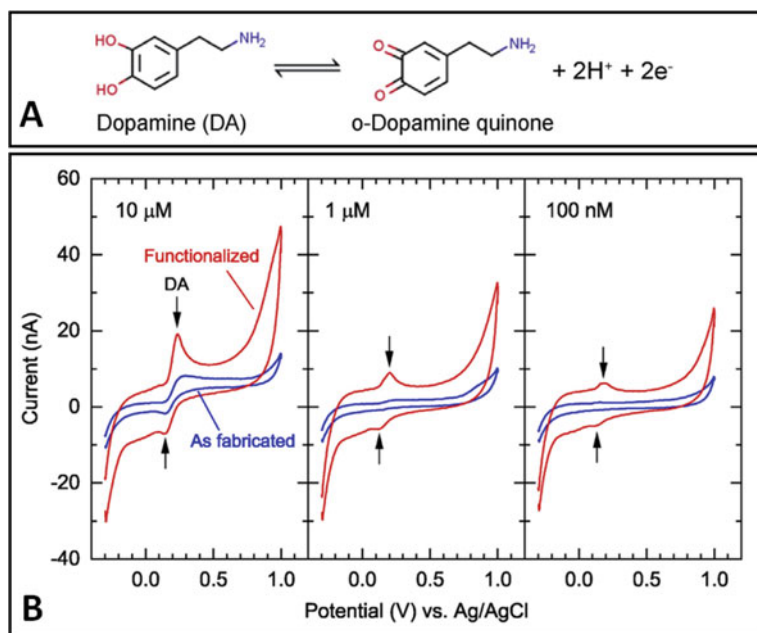
Fig. 7.6 a Redox reaction for dopamine. b Dopamine cyclic voltammograms obtained for as-fabricated and functionalized SWNTs with dopamine concentrations of (left) 10 \mu\text{M} , (middle) 1 \mu\text{M} , and (right) 100 nM. Reproduced (or adapted) with permission [21], © 2019, Elsevier
