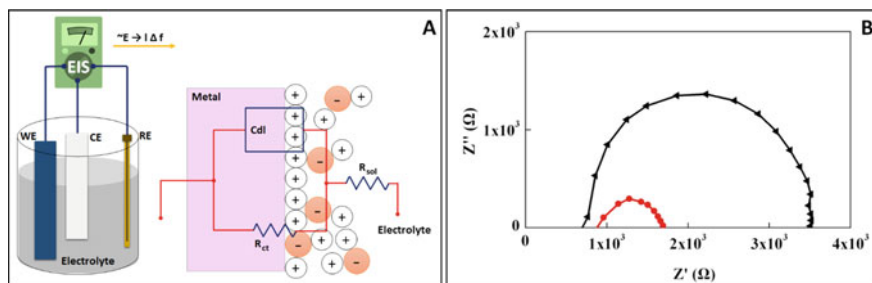
Fig. 7.8 a Illustration of the EIS test configuration. b Nyquist plot for a pure silicone-based material. Reproduced (or adapted) with permission [35], © 2014, American Physical Society
