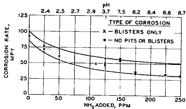
Figure 3.14 Effect of \text{NH}_3 addition on corrosion when only a sulfide film formed on the test coupons. Carbon steel coupons were in aqueous \text{HCl-H}_2\text{S-NH}_3 solutions for 24 hours at 300^\circ\text{F} ( 150^\circ\text{C} ) and 625 psig under nitrogen. 7
