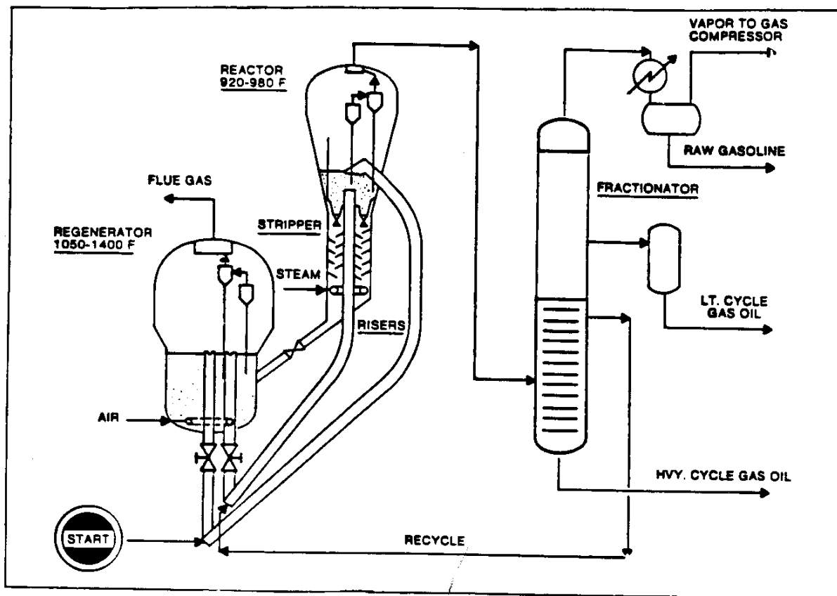
Figure 2.1 Fluid catalytic cracking 1
