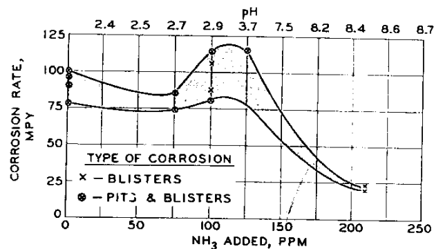
Figure 3.15 Effect of \text{NH}_3 addition on corrosion when nonremovable oxide film formed on the test coupons. Carbon steel coupons were in aqueous \text{HCl-H}_2\text{S-NH}_3 solutions for 24 hours at 300^\circ\text{F} ( 150^\circ\text{C} ) and 625 psig under nitrogen. 7
