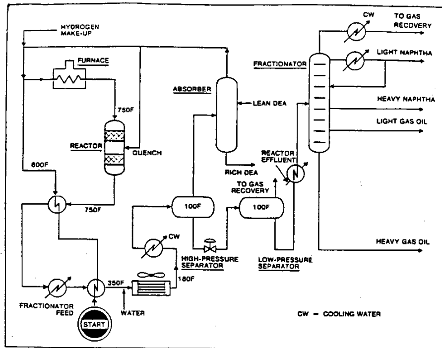
Figure 3.1 Hydrodesulfurizer 1
