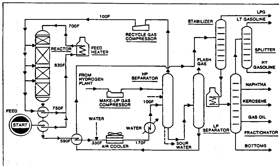
Figure 3.2 Hydrocracking 1
