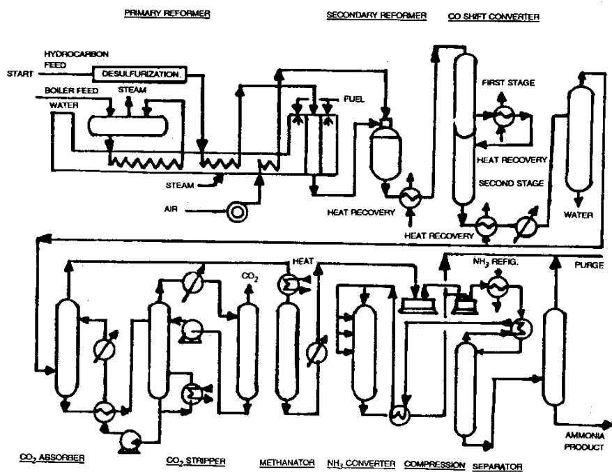
Figure 4.2 Ammonia 1
