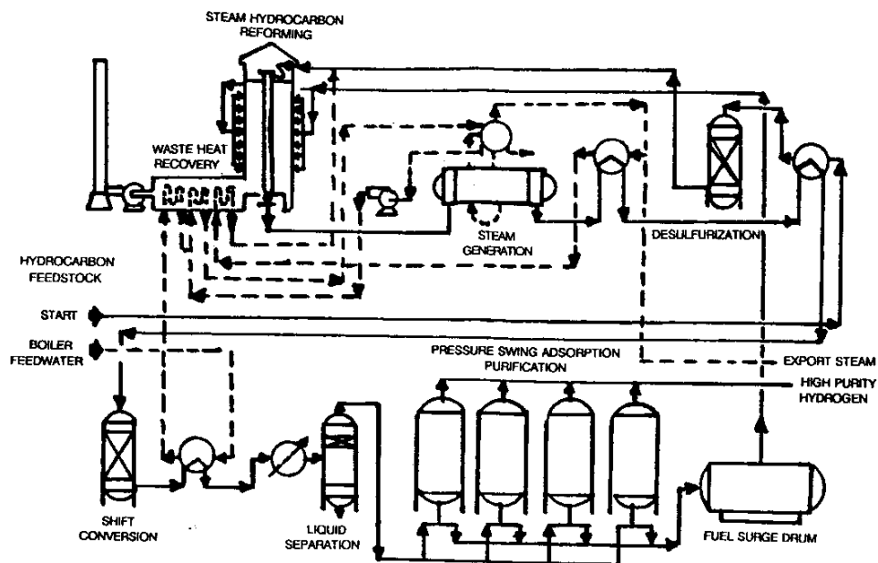
Figure 4.1 Hydrogen 1
