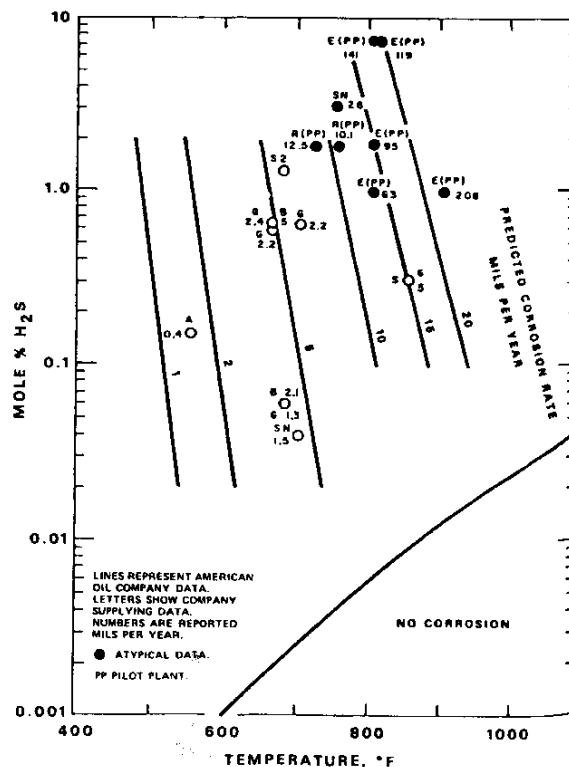
Figure 3.7h 12% Cr stainless steel, gas oil diluent
