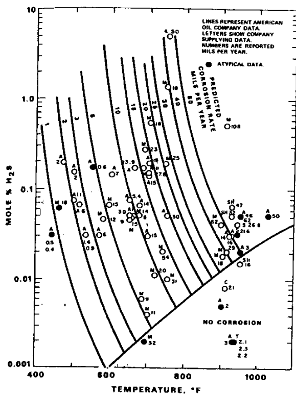
Figure 3.7a Carbon steel-naptha diluent
