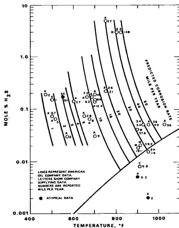
Figure 3.7e 9% Cr steel, naptha diluent
