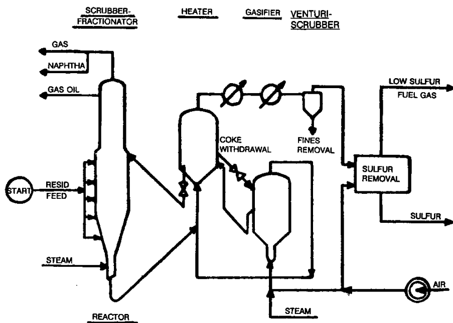
Figure 2.2 Flexicoking 2
