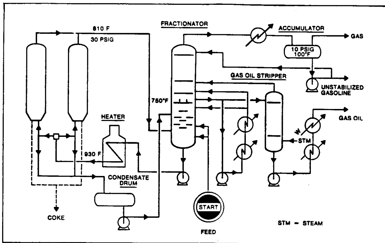
Figure 2.6 Delayed coking 1
