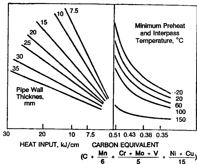
Figure 5.10 The permissible maximum carbon equivalent for butt welds in line pipe using cellulosic (EXX10) electrodes based on minimum preheat and interpass temperature, pipe wall thickness, and heat input. 5
