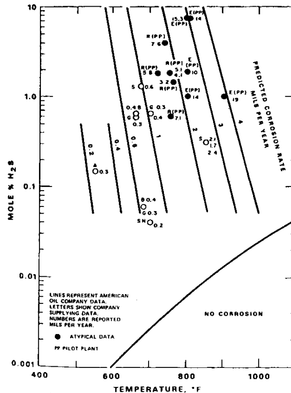
Figure 3.7j 18-8 stainless steel, gas oil diluent
