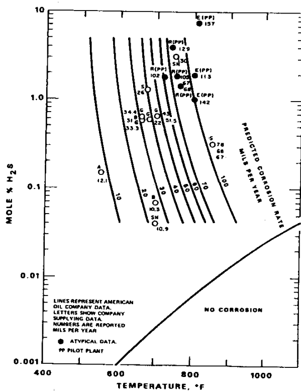
Figure 3.7b Carbon steel, gas oil diluent
