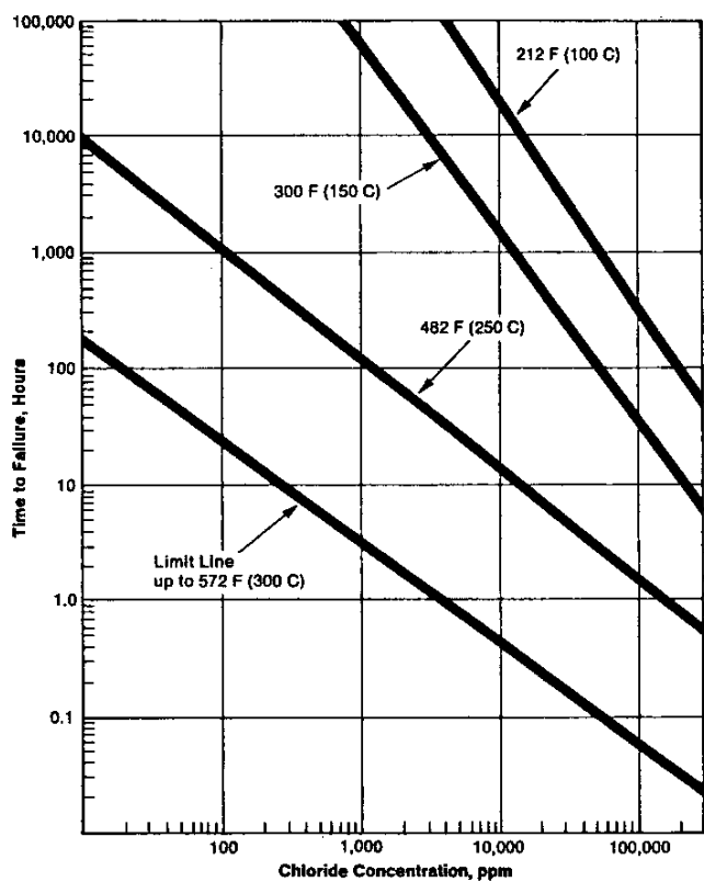
Figure 1.19 Stress corrosion cracking of 18-8 Stainless Steel in Chloride Solutions. 14
