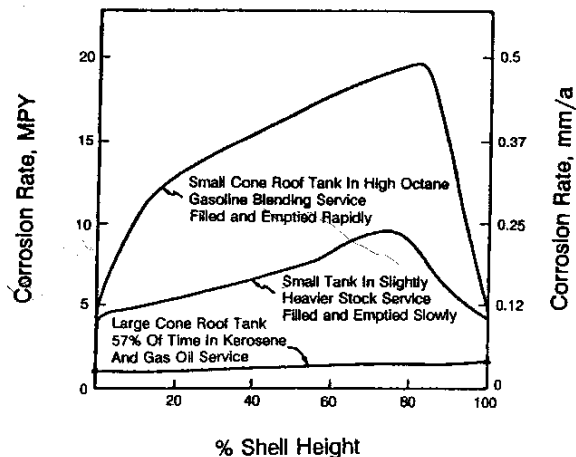
Figure 5.27 Shell corrosion in cone roof storage tanks handling gasoline and heavy distillates 9
