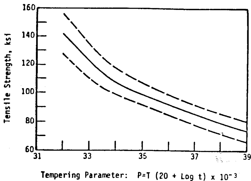
Figure 3.8 Tempering parameter vs tensile strength for quenched and tempered 2\frac{1}{4}Cr-1Mo steel. 5
