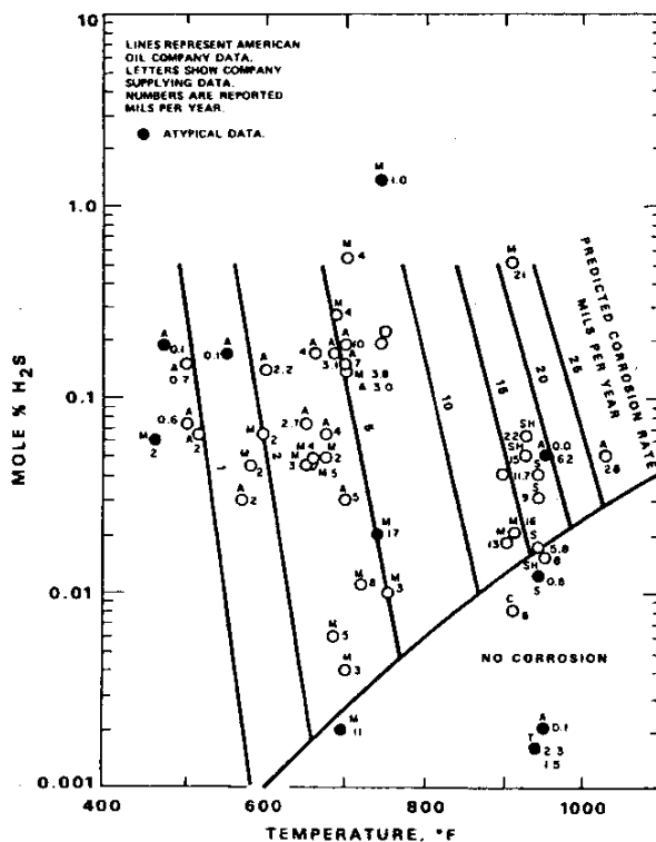
Figure 3.7g 12% Cr stainless steel, naptha diluent
