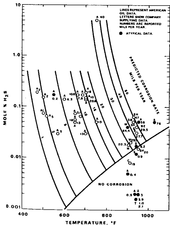
Figure 3.7c 5% Cr steel, naptha diluent
