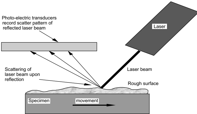
Figure 8.5 Measurement of surface roughness by laser reflection.
