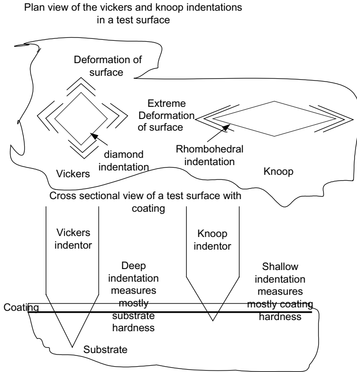
Figure 8.9 Comparison between Vickers and Knoop indentations.
