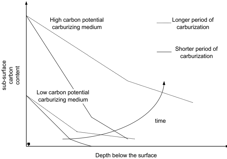
Figure 7.13 Effect of carbon potential on carbon distribution in a steel component (Adapted from Thelning).
