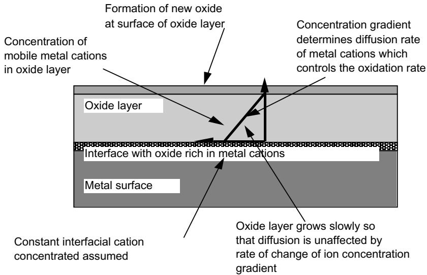
Figure 3.29 Wagner model of growth of corrosion product film by diffusion.
