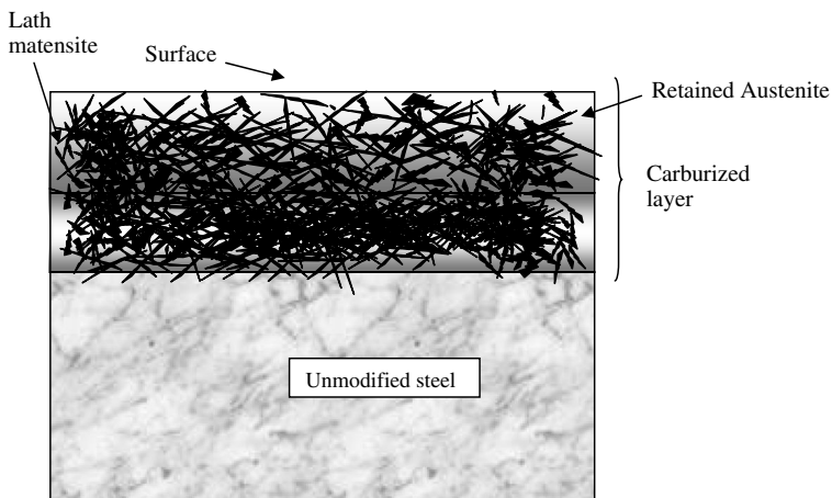
Figure 7.18 Schematic microstructure of a carburized steel showing an excess of retained austenite close to the surface.
