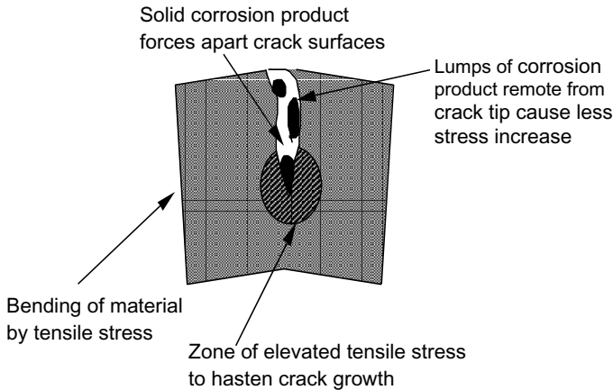
Figure 5.10 Crack enlargement by trapped corrosion products.
