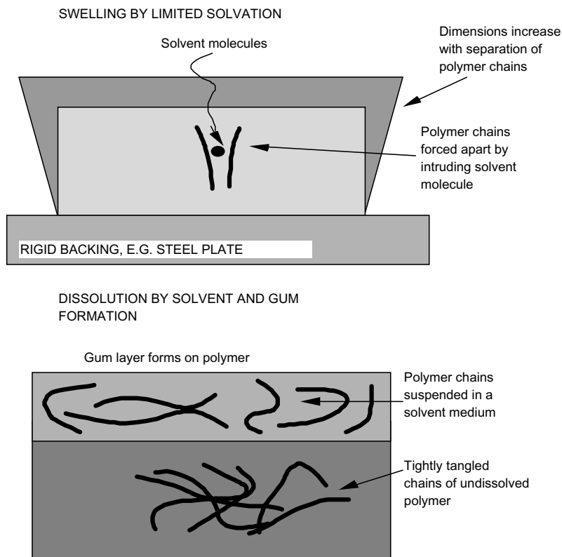
Figure 3.35 Solvation and partial solvation or swelling of polymers by a solvent.
