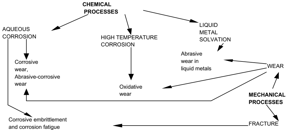
Figure 5.1 The different forms of destructive synergism between independent modes of materials degradation.
