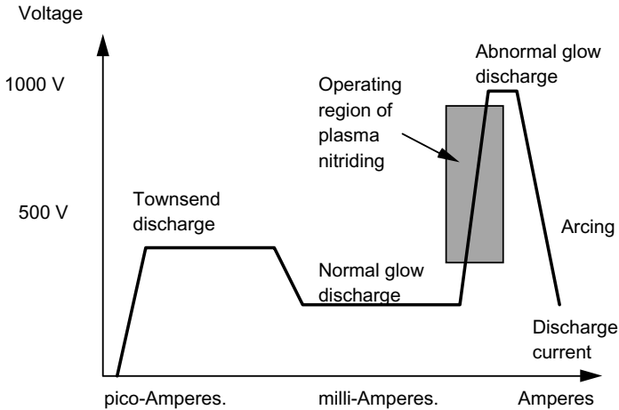
Figure 7.27 The electrical discharge characteristic of nitrogen.
