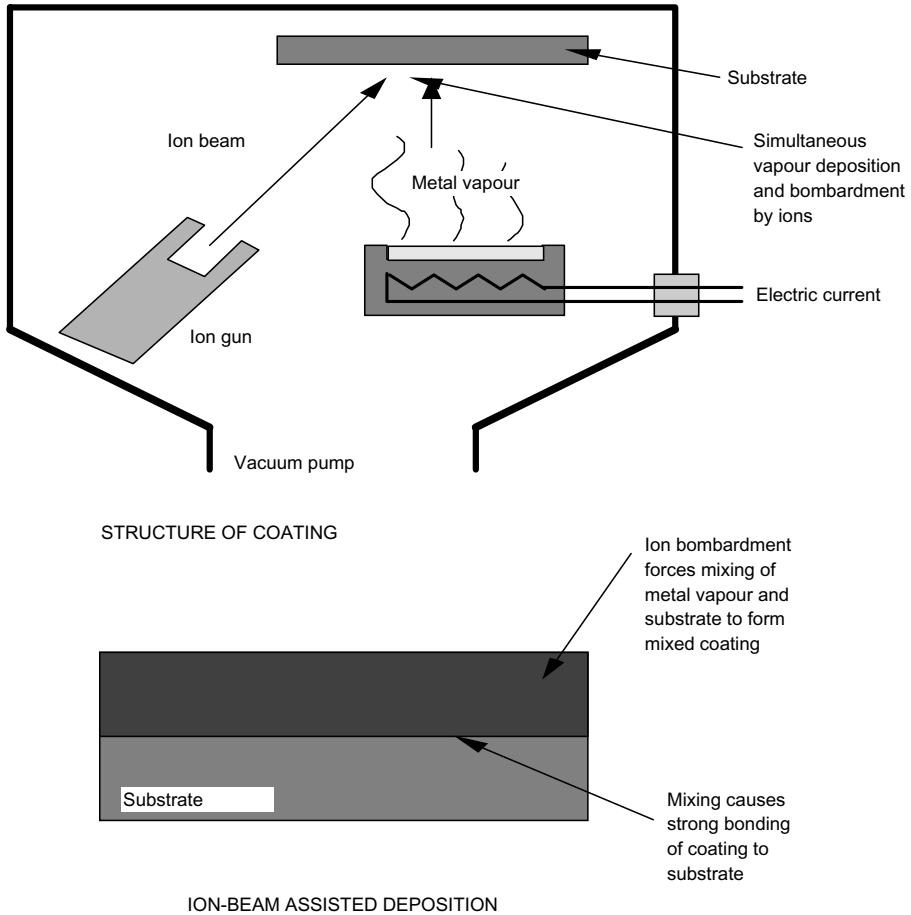
Figure 6.14 Mechanism of ion beam assisted deposition (IBAD).
