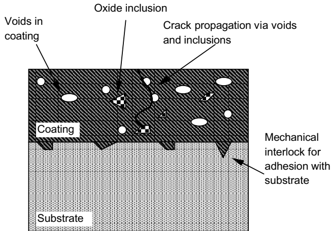
Figure 6.6 Structure of a plasma sprayed film.
