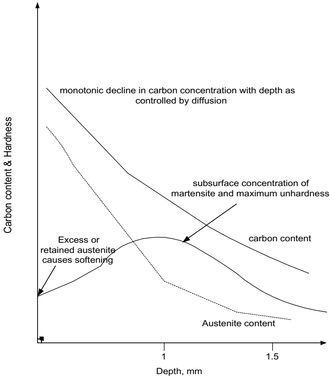
Figure 7.17 Schematic of hardness and carbon content profiles of carburized Ni steel (Adapted from Thelning).
