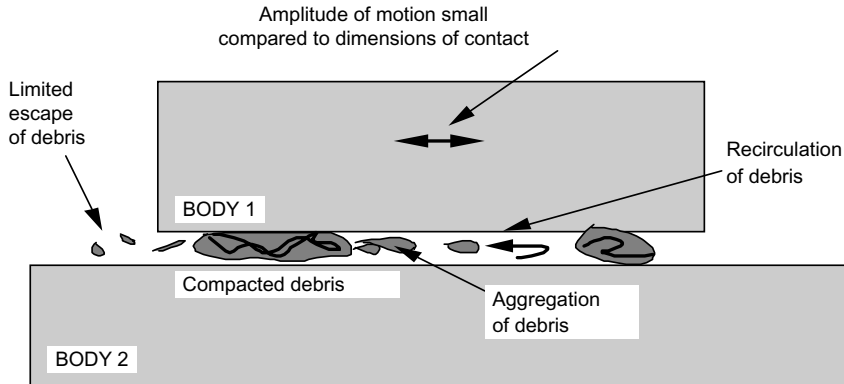
Figure 2.22 Formation of wear debris layer by entrapment in restricted amplitude sliding.
