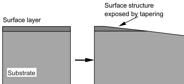
Figure 8.10 Taper-sectioning of a coating and substrate to reveal fine detail of the coating and substrate.
