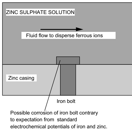
Figure 3.8 Generation of abnormal electrochemical potentials by large concentration differences in electrolytes and associated corrosion problems.
