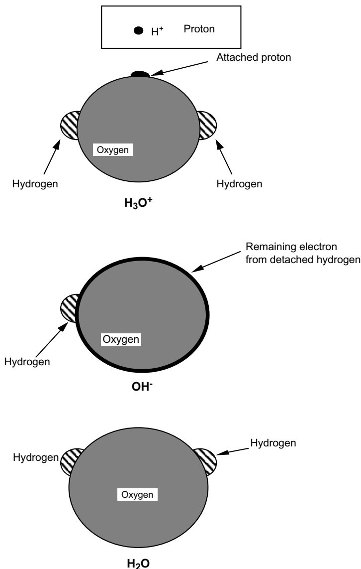
Figure 3.3 Molecular configuration of water in neutral and ionized form.
