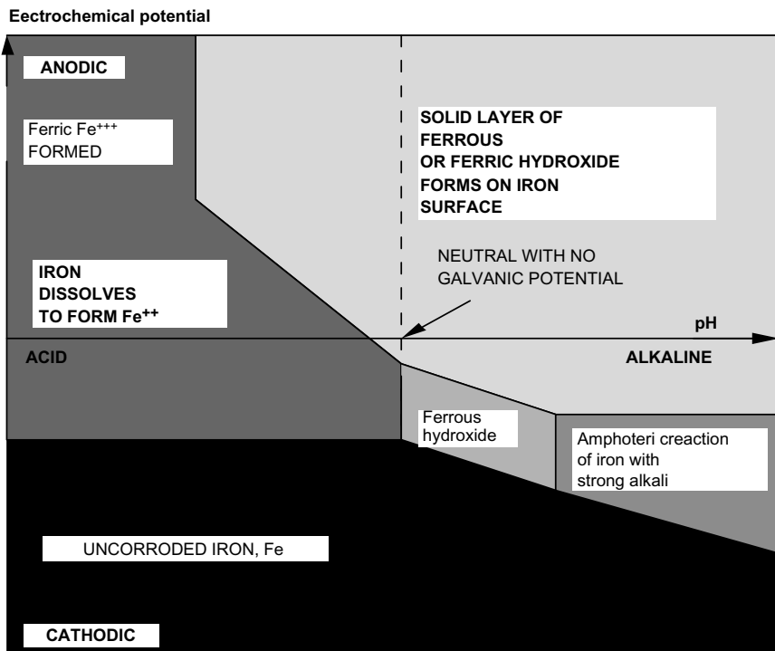
Figure 3.12 Example of Pourbaix diagram: corrosive response of iron to acidified and alkalinized water. Adapted from Fontana and Greene (1978).
