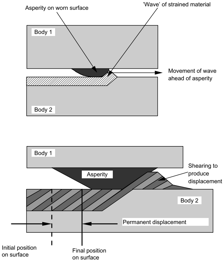
Figure 2.15 Wave formation at the worn surface of a material.
