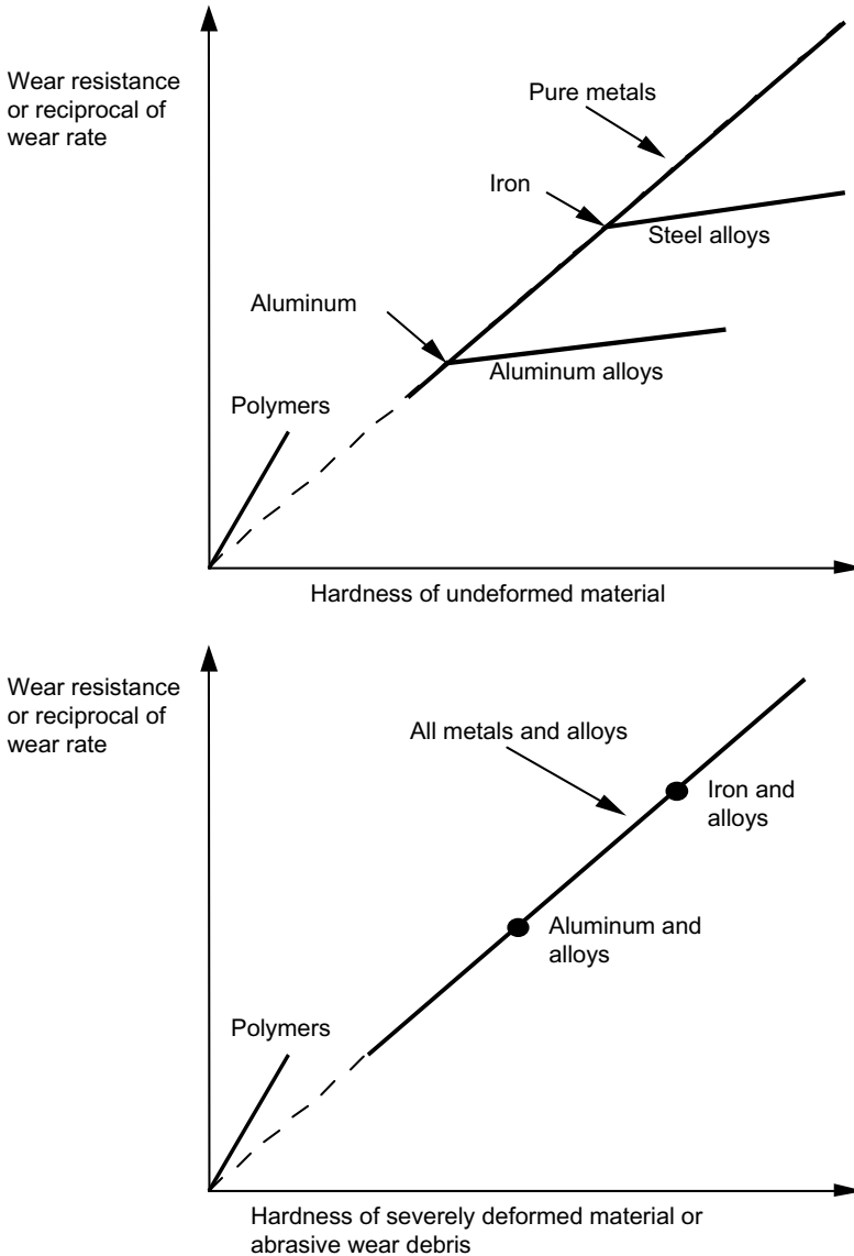
Figure 2.9 The relationship between wear rates with hard abrasives and the hardness of the worn material.
