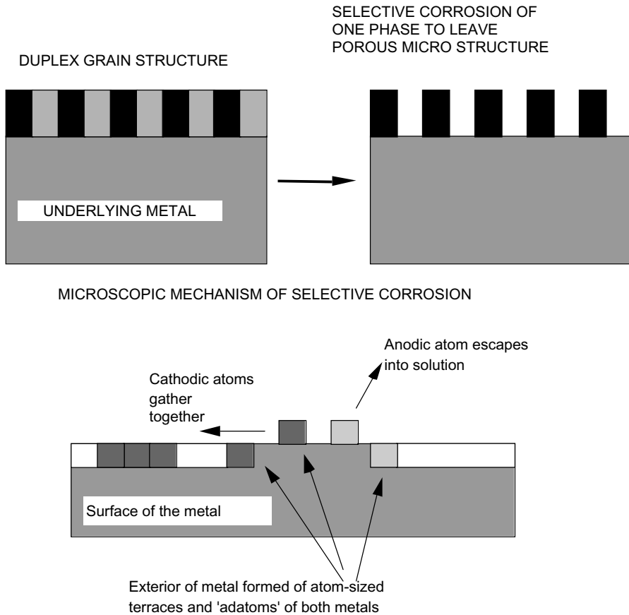
Figure 3.25 Dezincification of brass and its atomic mechanism.
