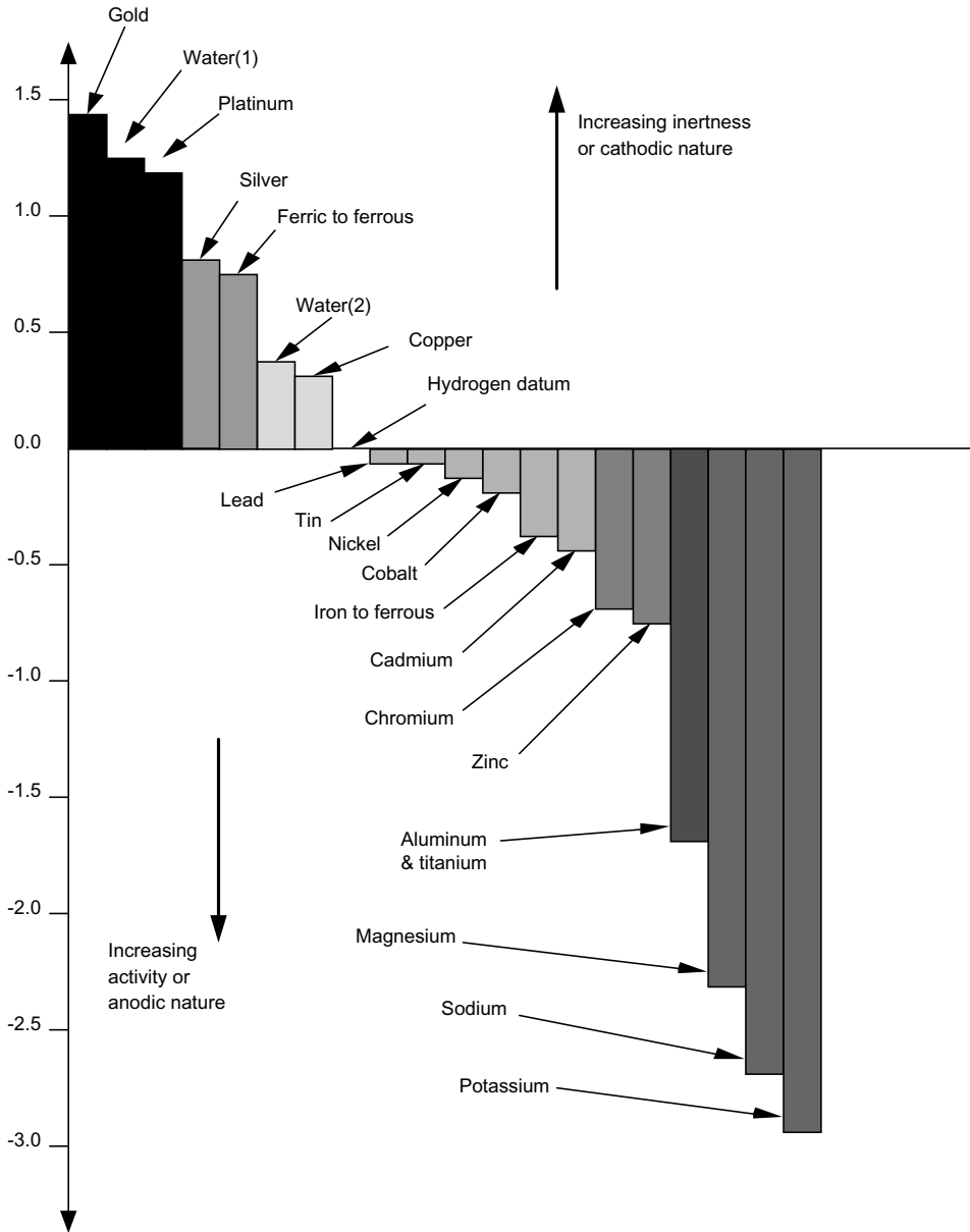
Figure 3.6 Electrochemical potentials of common elements.
