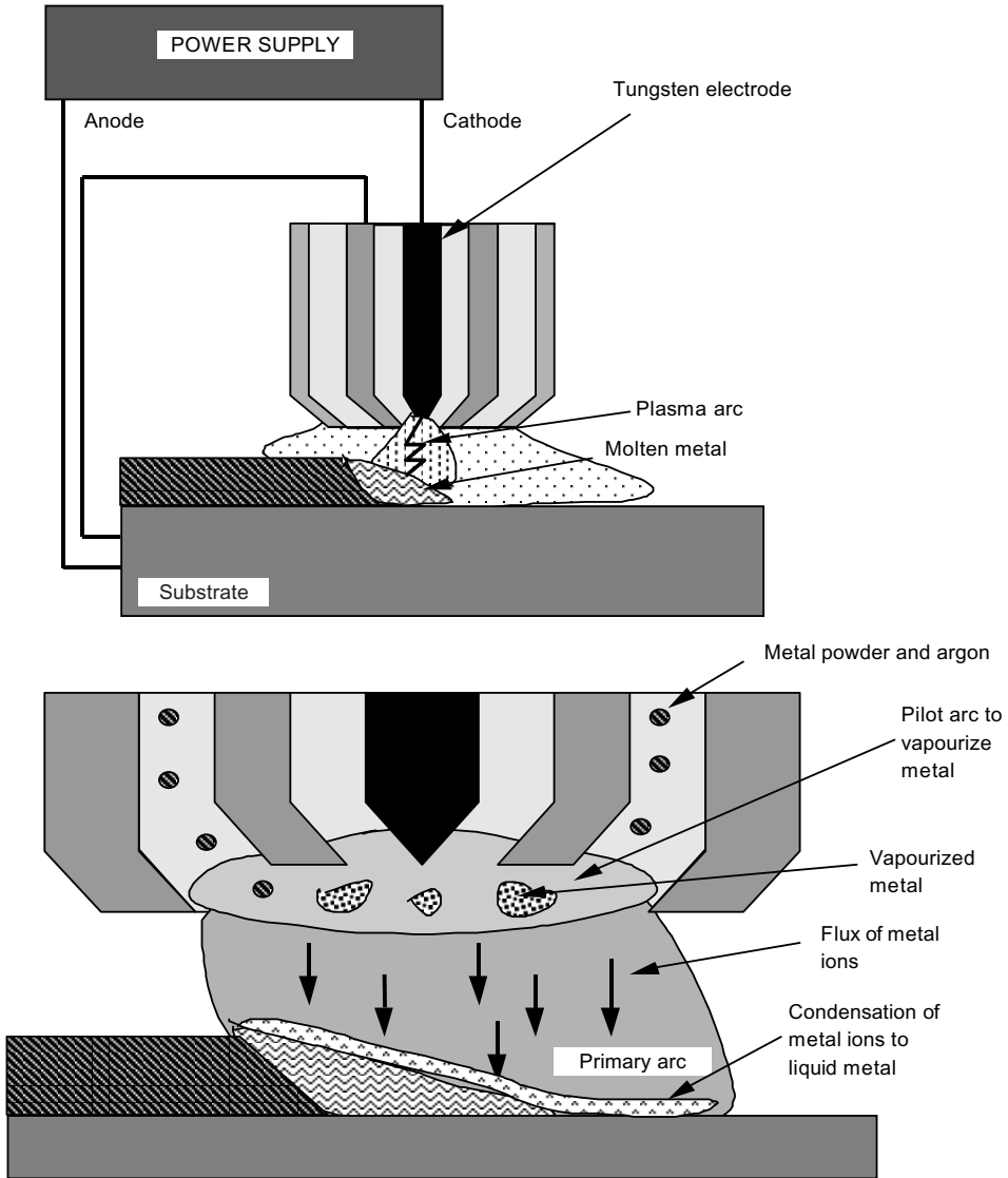
Figure 6.7 Operating system and mechanism of the Plasma Transferred Arc coating process.
