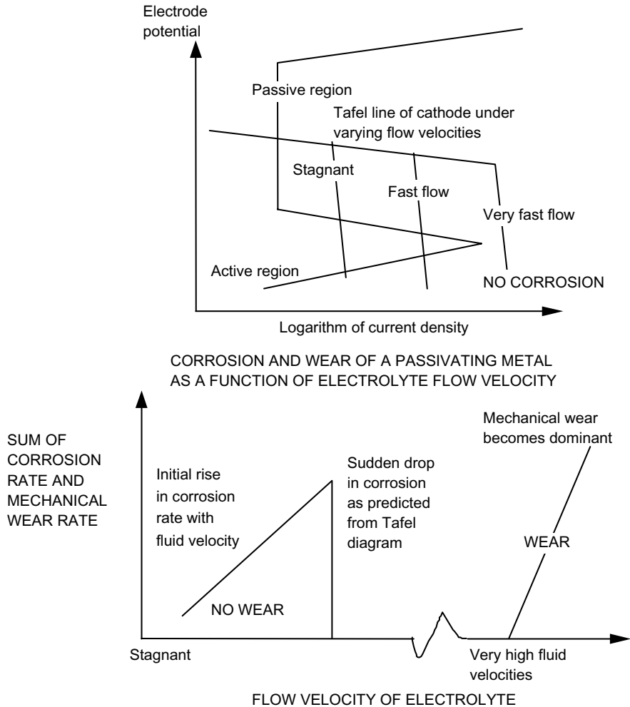
Figure 3.24 Tafel diagram illustrating passivation induced by fluid flow (adapted from Fontana and Greene).
