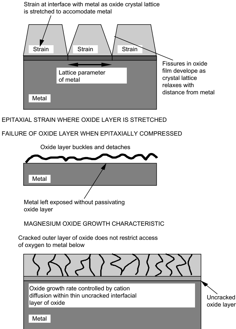
Figure 3.31 Effect on corrosion of epitaxy between a metal surface and overlying corrosion product film.
