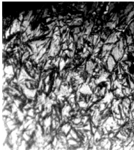
Figure 8.16 Micrograph of retained austenite in case hardened carburized steel.
