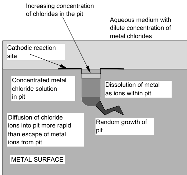
Figure 3.15 Mechanism of intensification of corrosion inside a pit where chloride ions are present in the corrosive medium.
