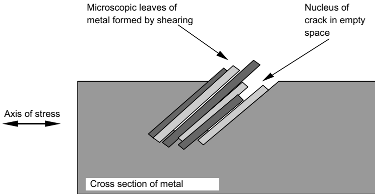
Figure 2.28 Mechanism of fatigue crack nucleation in a metal.
