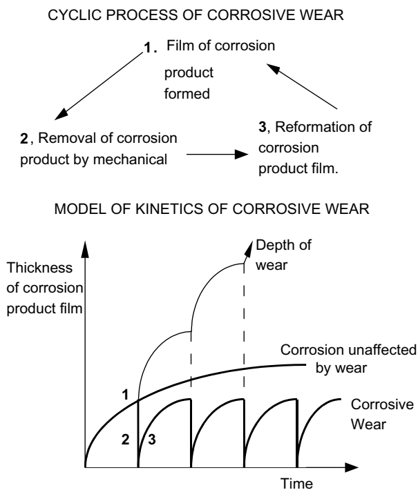
Figure 5.3 Corrosive wear by cyclic removal and formation of passivating films: mechanism and effect on corrosion kinetics.
