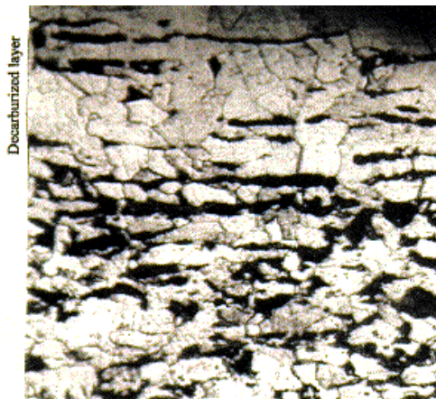
Figure 8.15 Microstructure of thermally decarburized steel.
