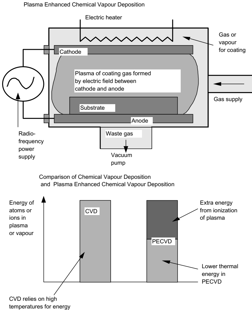
Figure 6.17 The operating principle of plasma enhanced chemical vapor deposition (PECVD).
