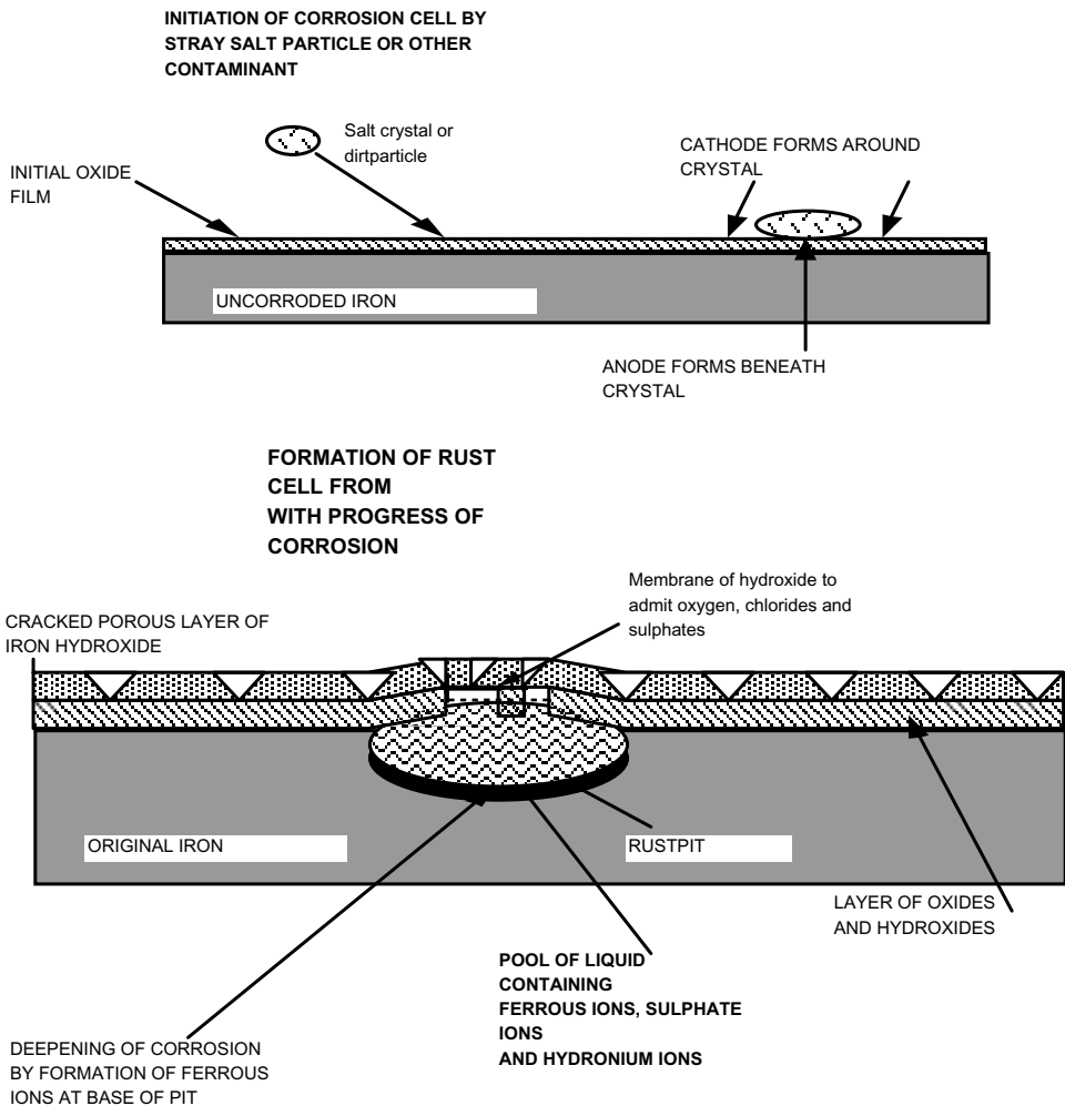
Figure 3.13 Mechanism of rusting of iron in open air.
