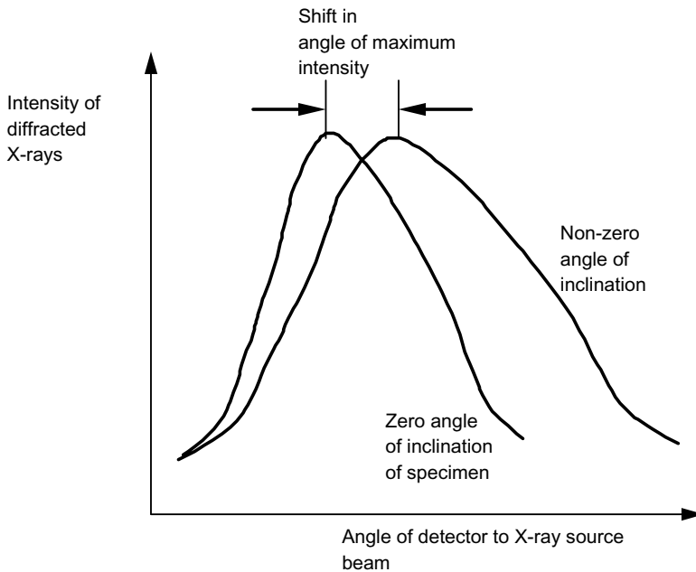
Figure 8.24 Distribution of intensity of reflected X-rays for various specimen inclinations.
