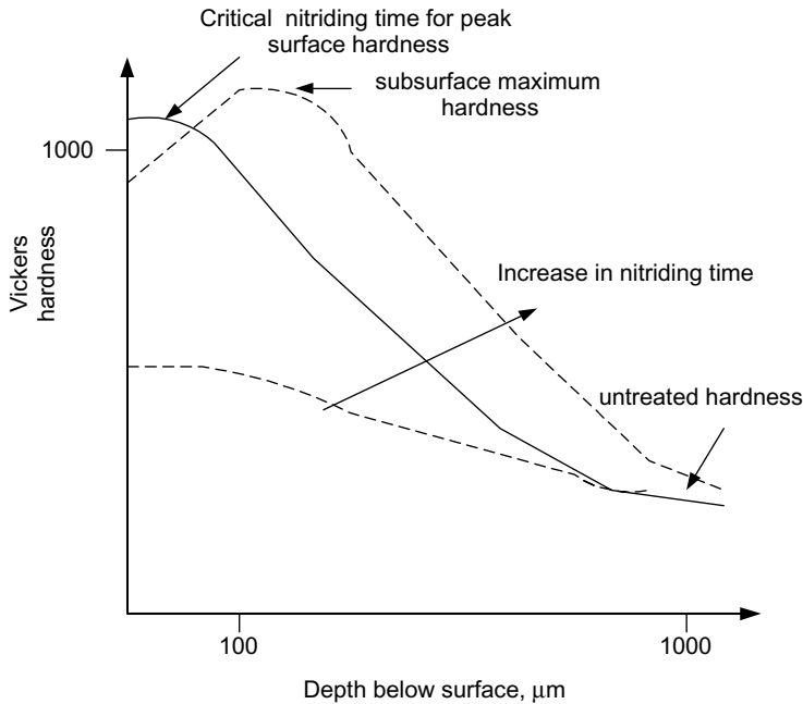
Figure 7.25 Schematic illustration of hardness distribution of nitrided alloy steel for different nitriding periods (Adapted from Thelning).
