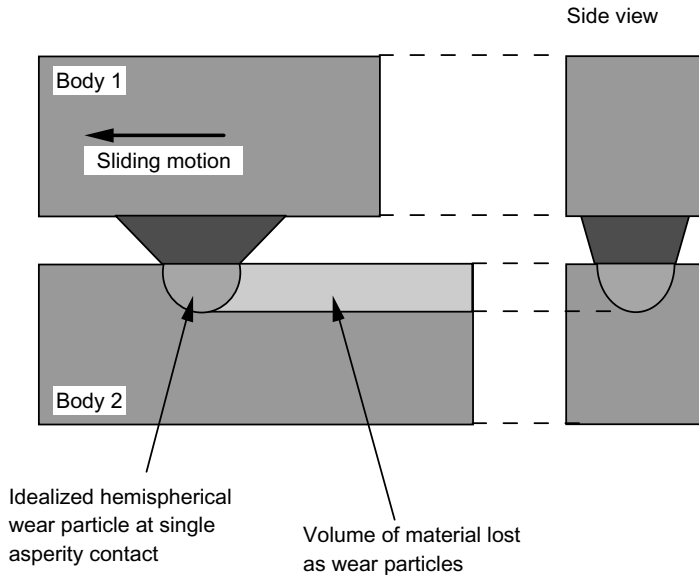
Figure 2.24 The Archard model of wear.
