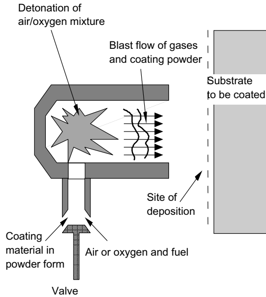
Figure 6.8 Operating mechanism of the detonation-gun coating system.
