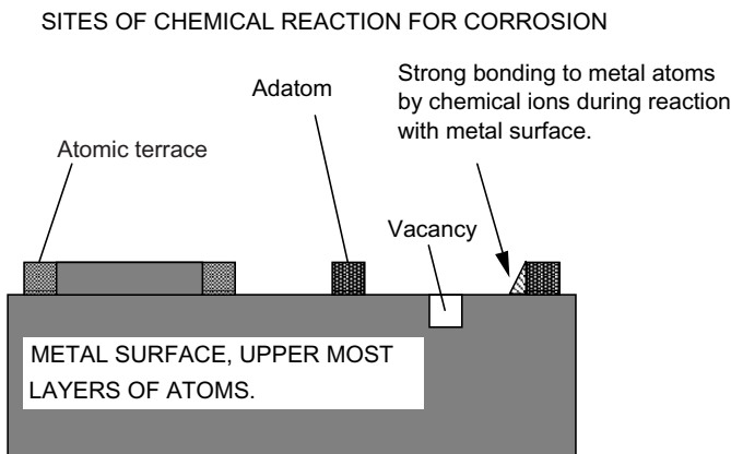
Figure 3.4 The role of imperfections in atomic layering of surfaces in promoting corrosion.
