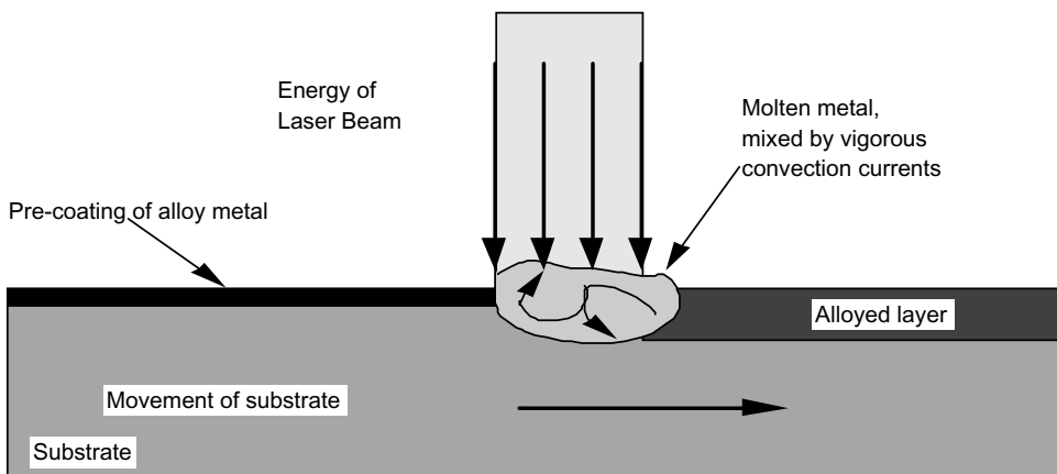
Figure 7.28 Principle of surface alloying of a metal by laser or electron beam.
