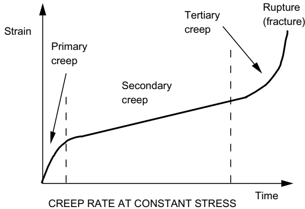
Figure 2.33 Development of creep at constant stress level and a model of different stages of creep.
