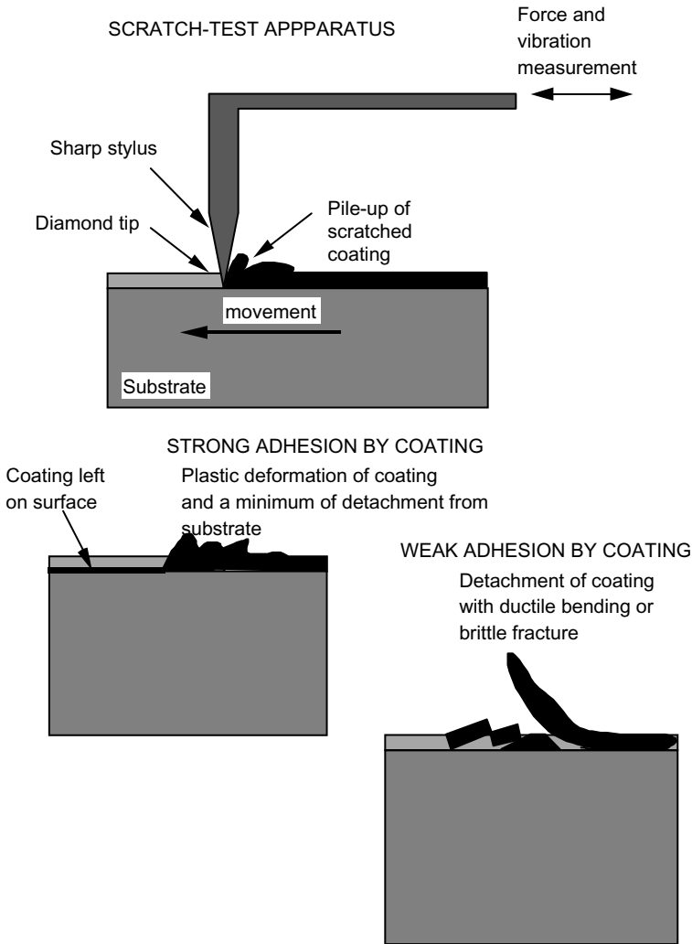
Figure 8.12 Principle of scratch testing of coating adhesion.
