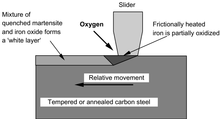
Figure 2.19 Structure and formation of white layers by melting wear.
