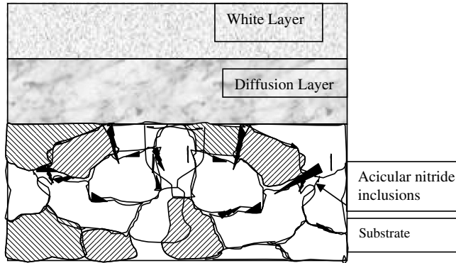
Figure 7.23 The structure and formation of the nitride coating on steel.
