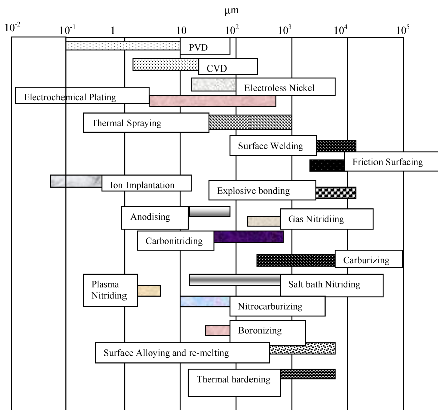
Figure 8.2 Thickness ranges of various coatings in current use (Adapted from Roberts).
