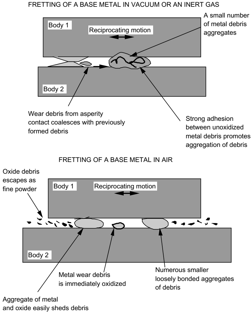
Figure 5.6 Model of acceleration of fretting wear by atmospheric oxygen.
