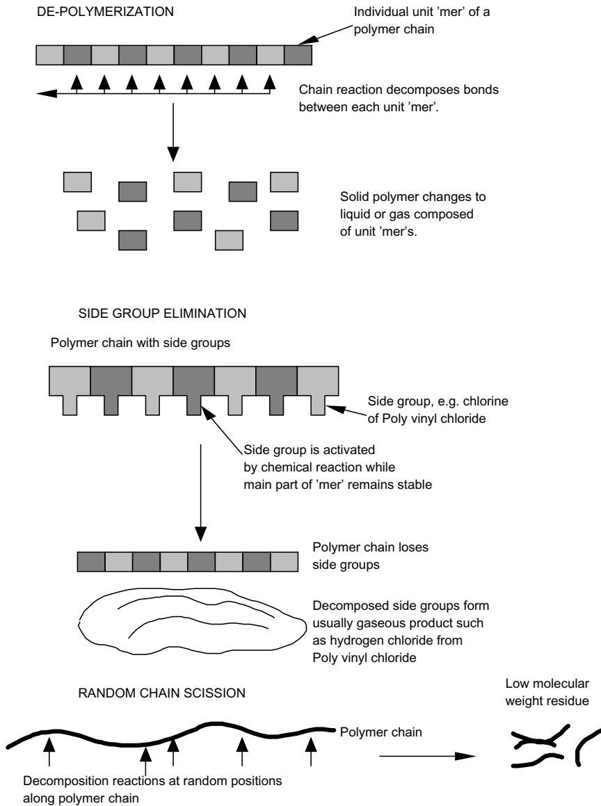
Figure 3.36 Degradation processes in polymers: de-polymerization, side group elimination and random chain scission.
