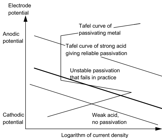
Figure 3.23 Discrimination between reliable and unreliable passivation in terms of the Tafel diagram. Adapted from Fontana and Greene.
