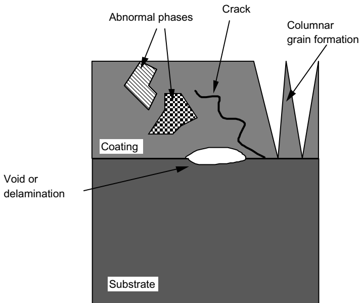
Figure 8.14 Microstructural evaluation of coatings.
