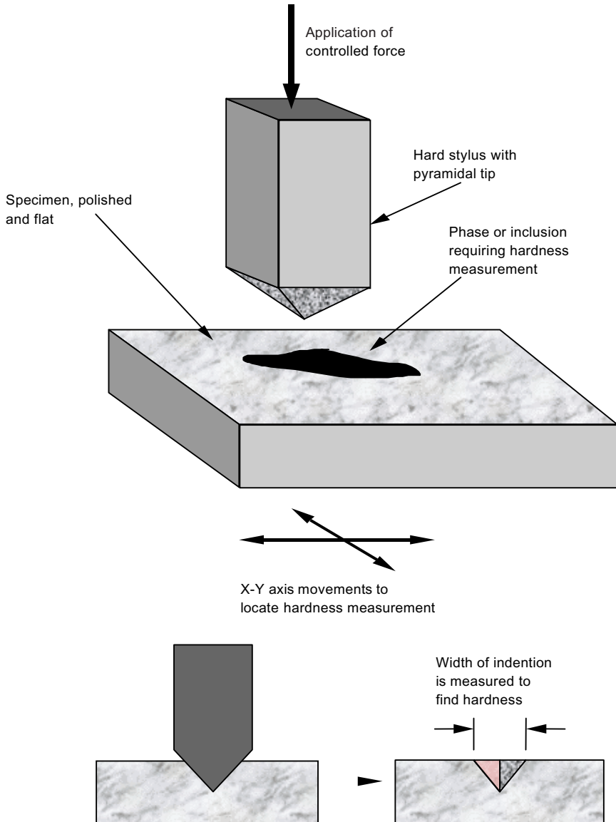
Figure 8.7 Operating principle of hardness measurement by indentation.
