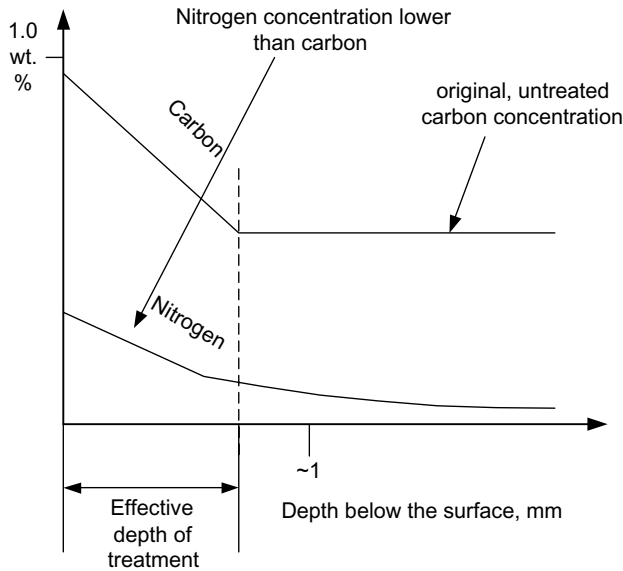
Figure 7.20 Carbon and nitrogen distribution versus depth in mild steel carbonitrided at 860°C (Adapted from Thelning).
