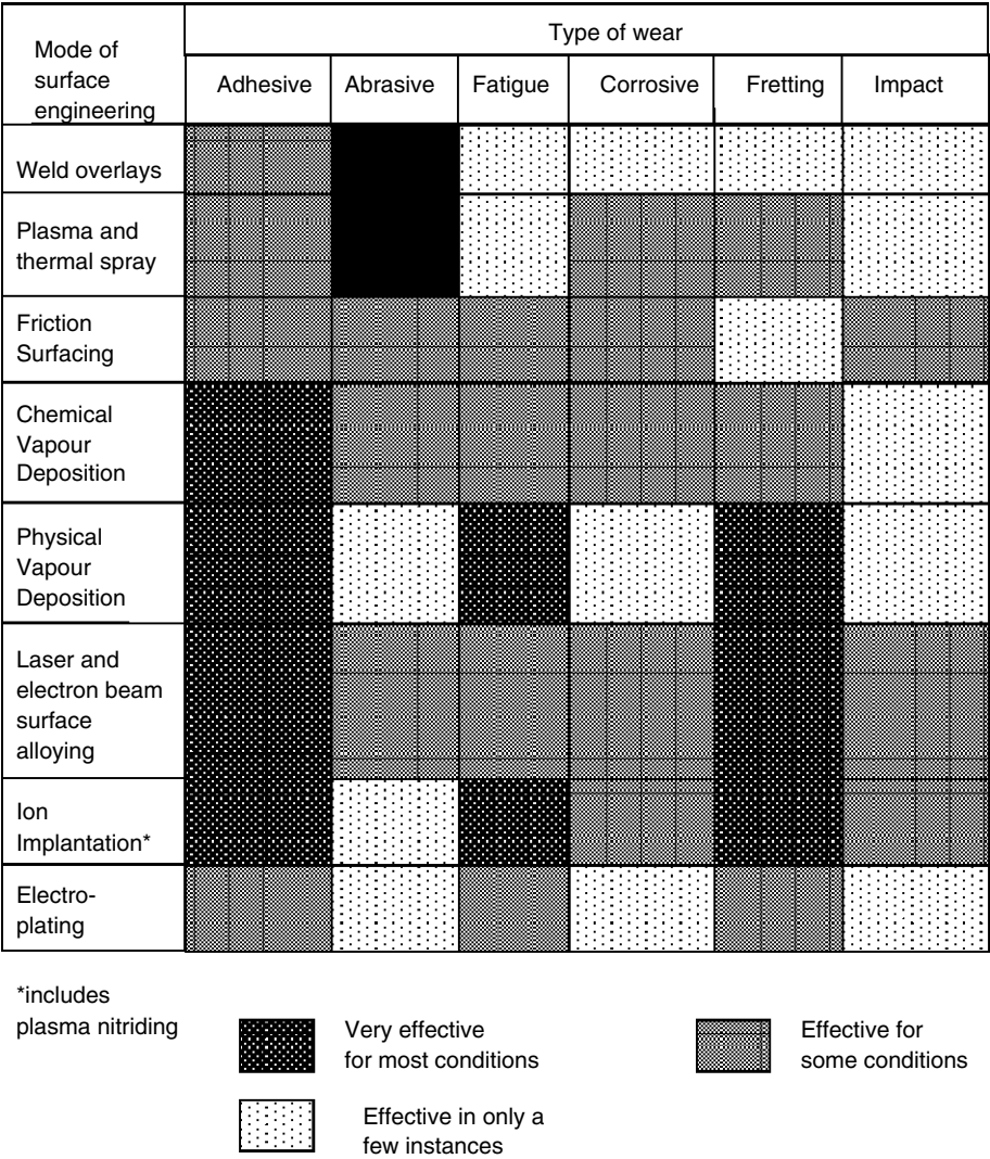
Figure 9.2 Tabular guide to selection of wear control techniques.
