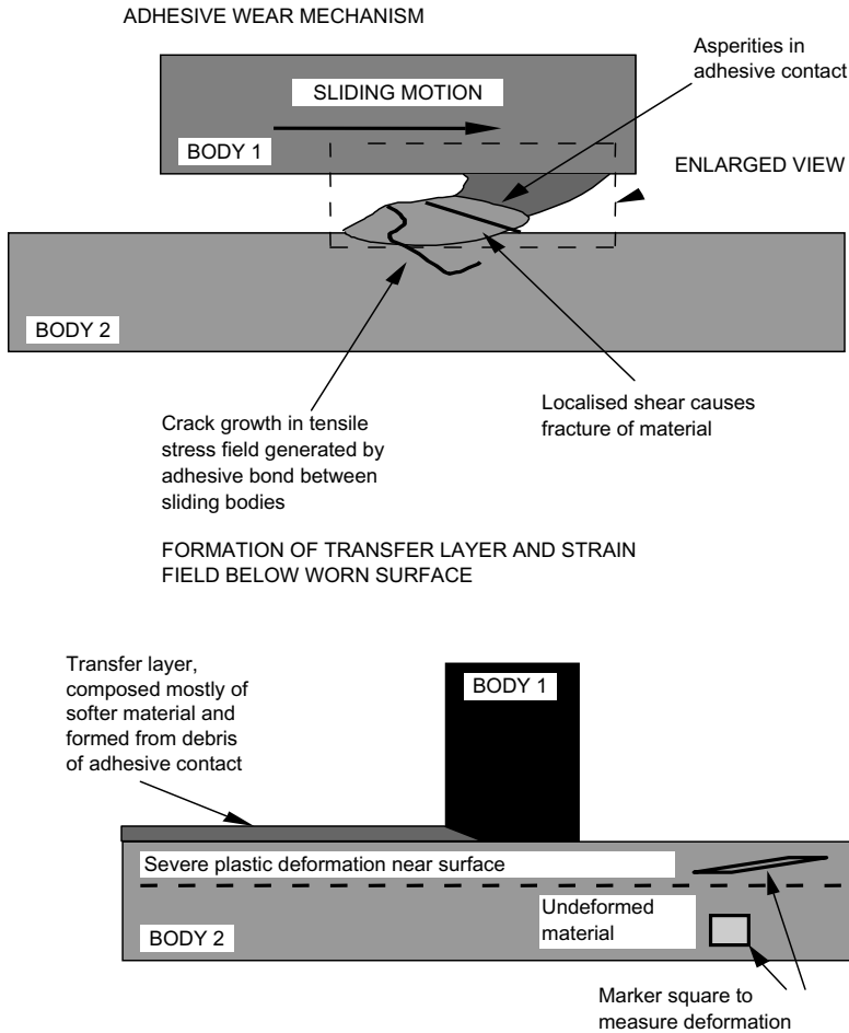
Figure 2.5 Mechanism of severe adhesive wear, asperity deformation and gouging by wear particles. The formation of transfer layers.
