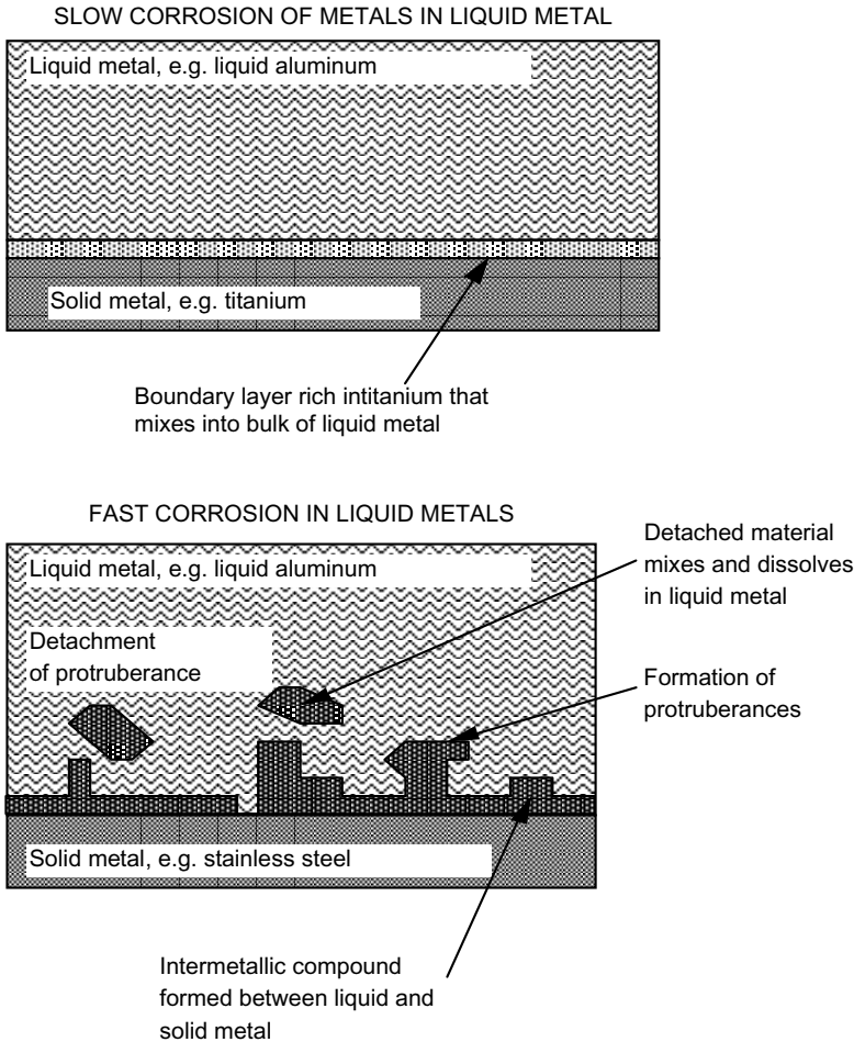
Figure 3.42 Mechanisms of corrosion of a solid metal immersed in a liquid metal.
