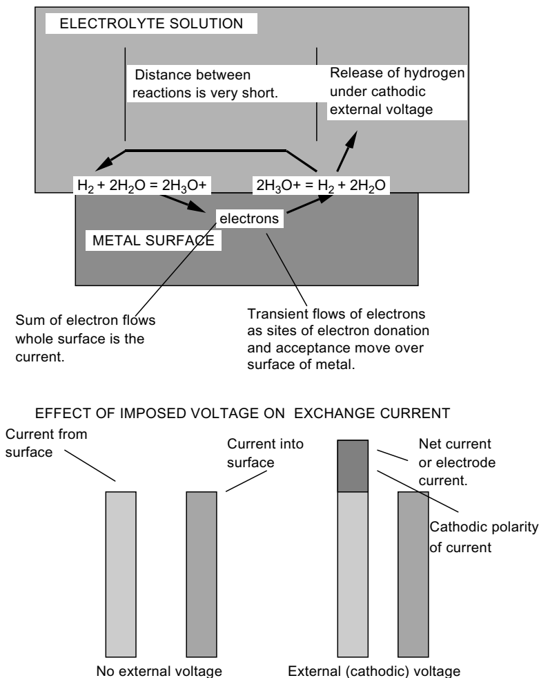
Figure 3.10 Exchange current between an electrode and electrolyte solution and the mechanism of current flow from an electrode.
