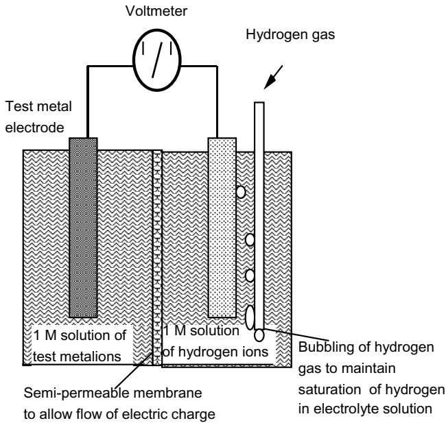
Figure 3.5 Use of the standard hydrogen electrode to measure the standard electrochemical potential of a metal.
