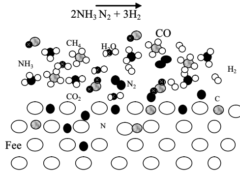
Figure 7.19 Dissociation of ammonia and penetration of steel by nitrogen in the carbonitriding process.
