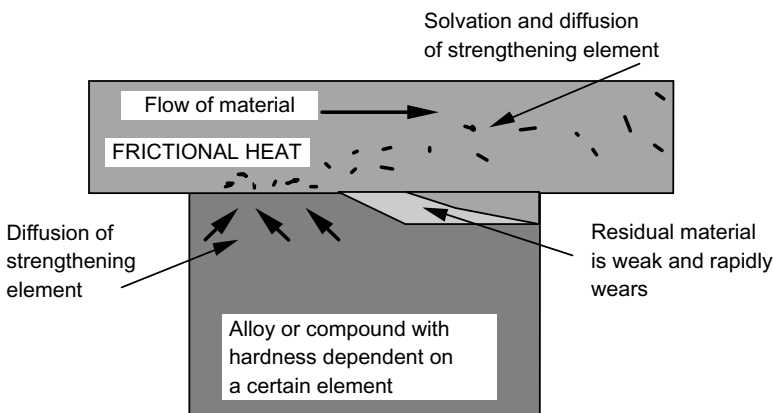
Figure 2.23 Schematic illustration of the mechanism of diffusive wear.
