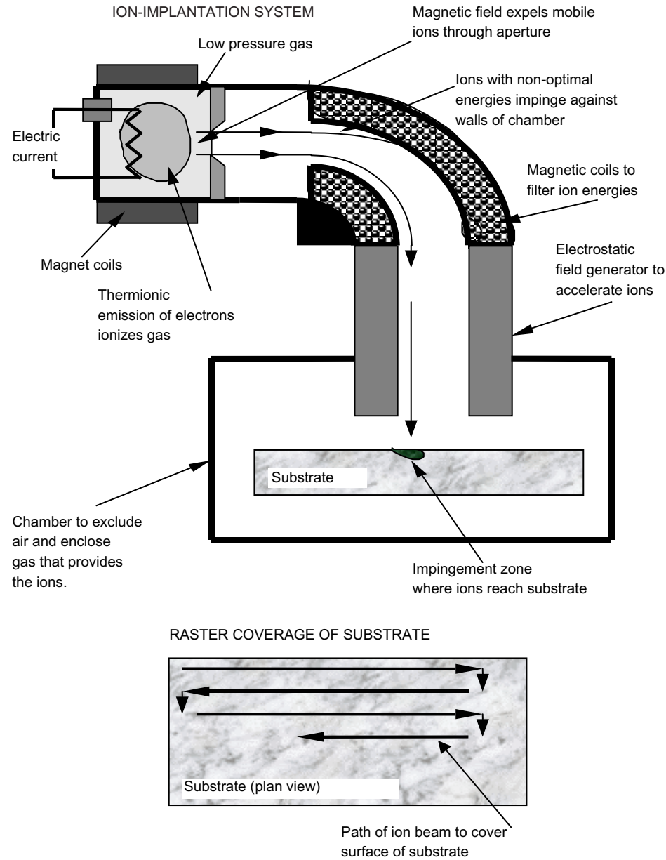
Figure 7.30 Ion-implantation apparatus and coating method.
