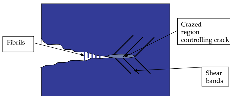
Figure 2.32 Fatigue mechanisms of polymers.
