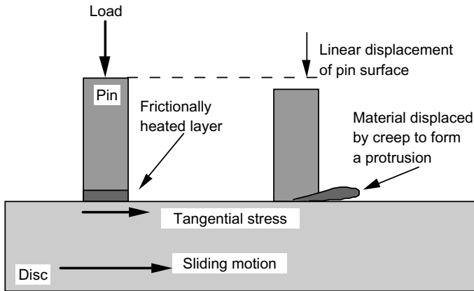
Figure 2.34 Pseudo-wear generated by creep and friction.
