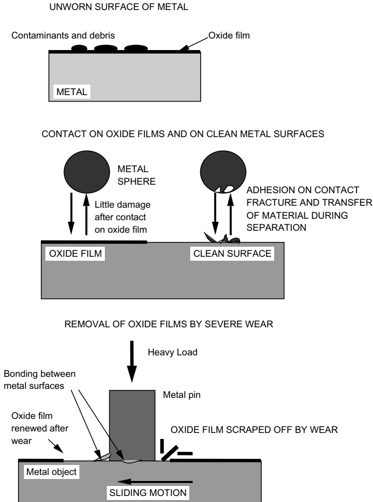
Figure 2.4 Contaminant and oxide layer removal on metals by wearing contact to initiate adhesive wear.
