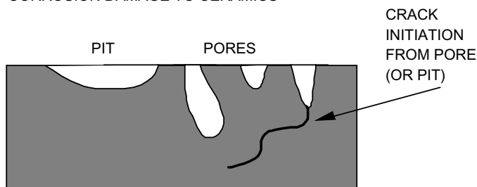
Figure 3.41 Hole and pit formation in ceramics during corrosion by a liquid.
