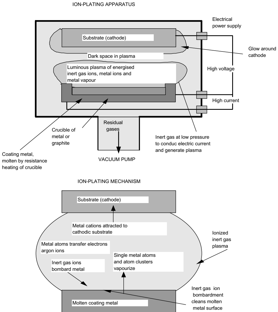
Figure 6.13 Principle of ion plating.
