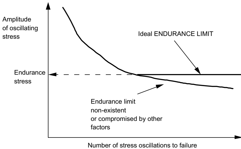
Figure 2.27 The endurance limit of metal fatigue.
