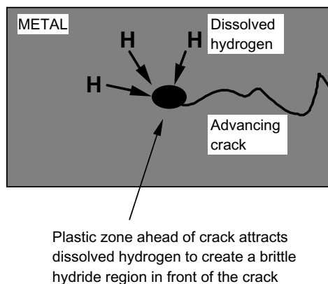
Figure 3.20 Mechanism of hydrogen embrittlement.
