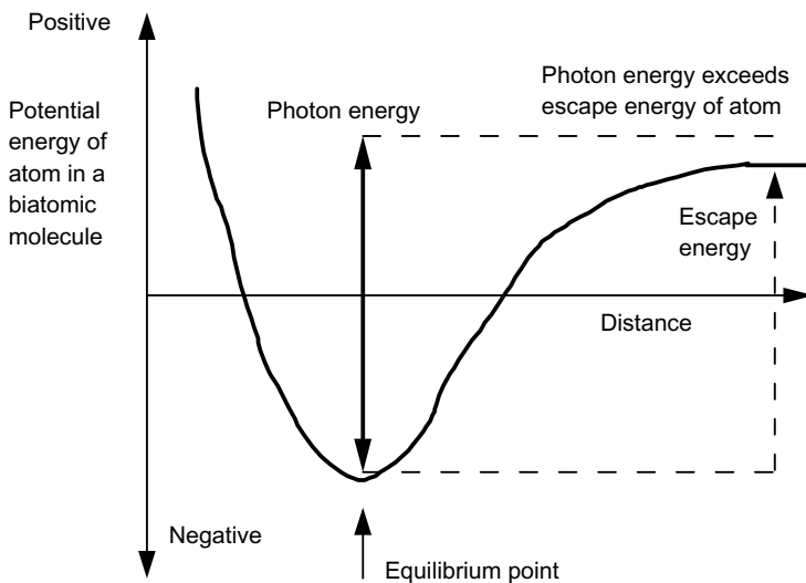
Figure 4.3 Mechanism of atom dissociation by photon energy.
