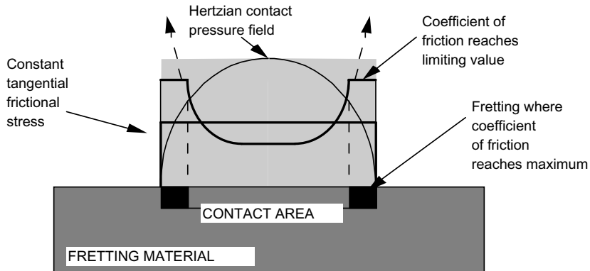
MECHANICS OF FRETTING IN A CONTACT
