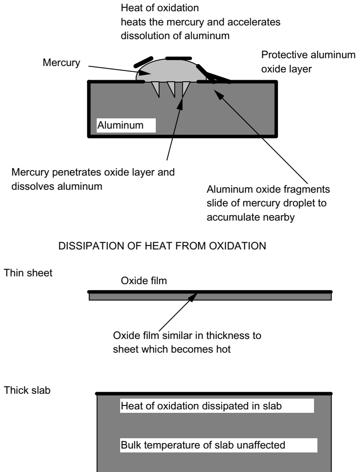
Figure 3.27 Mechanisms of uncontrolled oxidation of metals in atmospheric oxygen.
