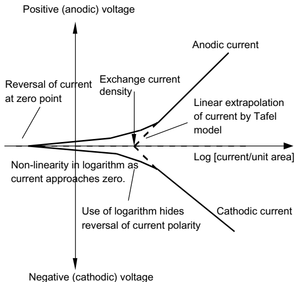
Figure 3.9 Tafel model of relationship between current and electrochemical potential for a zinc electrode.
