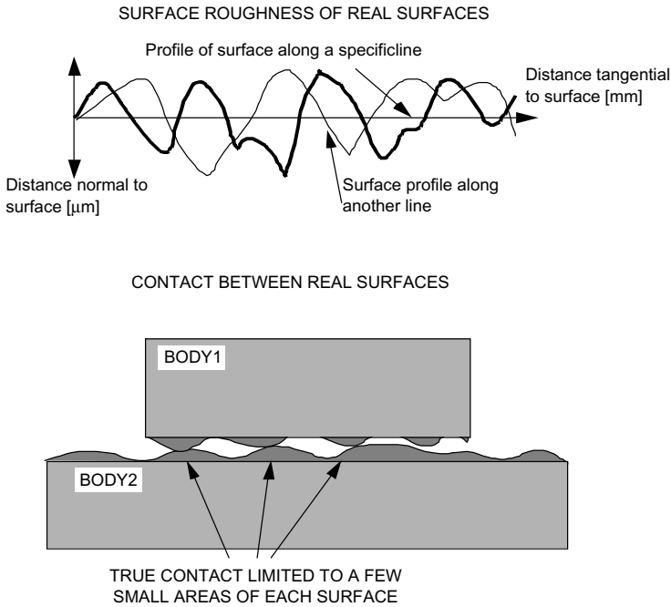
Figure 2.1 Nature of contact between rough surfaces.
