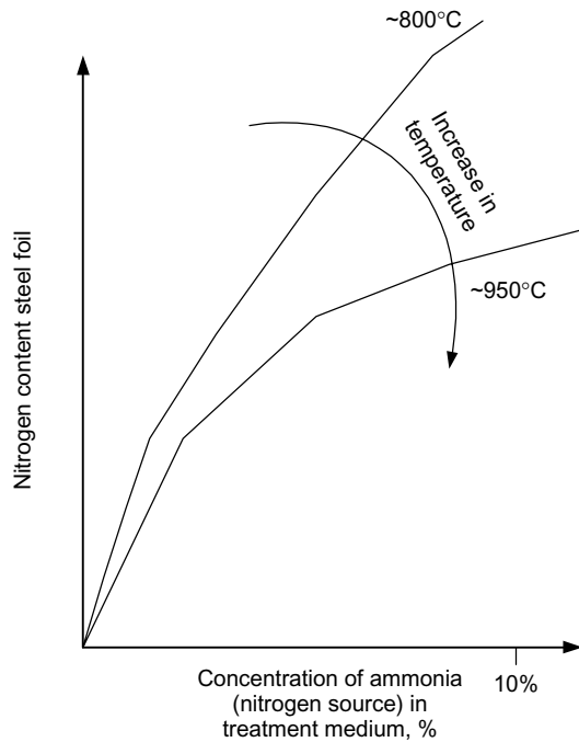
Figure 7.21 Nitrogen content of steel foil as a function of temperature and ammonia content in the furnace gas after carbonitriding (Adapted from Thelning).
