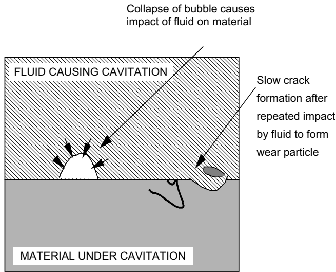
Figure 2.14 Mechanism of cavitation wear.
