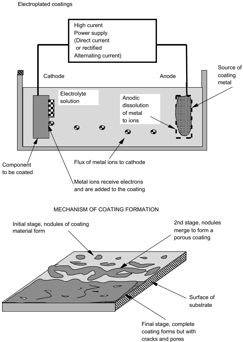
Figure 6.3 Mechanism of electroplating and structure of electroplated coatings.
