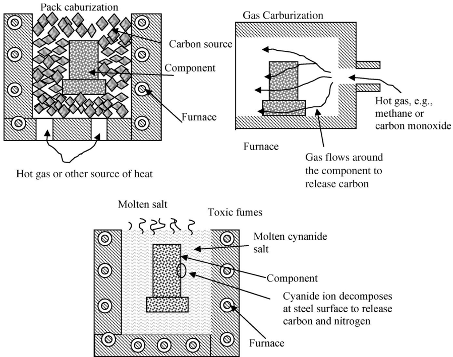
Figure 7.11 Schematic illustration of the carburizing methods.
