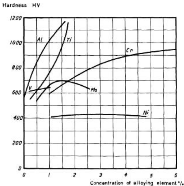
Figure 7.24 Effect of alloying elements on the hardness of a nitrided steel (Courtesy of Thelning and Bofors Ltd.).
