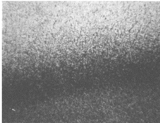
Figure 7.5 Microstructure of steel, induction hardened to a surface hardness of 800 VPN. (Courtesy of Doxon Engineering Pte. Ltd, Singapore.)
