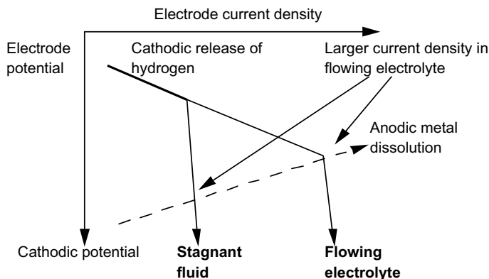
Figure 3.18 Effect of fluid flow on the limiting corrosion current.
