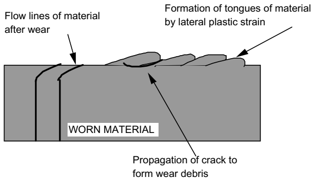
Figure 2.16 Mechanisms of wear particle formation by delamination and crack formation from surface strained layers.
