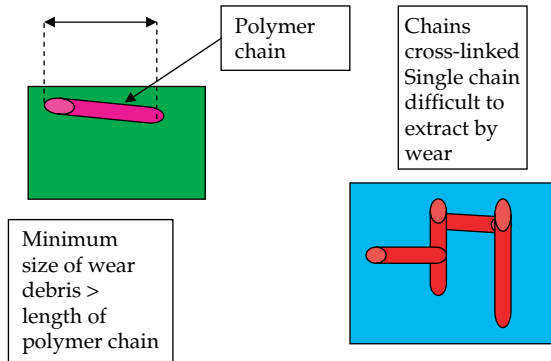
Figure 2.25 Minimum wear debris size for high molecular weight polymers and securing of molecular chains by cross-linking.
