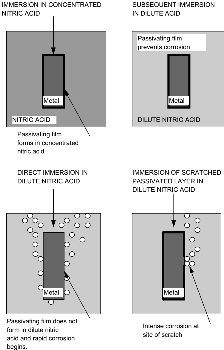
Figure 3.21 Faraday's demonstration of passivation of iron in concentrated nitric acid.
