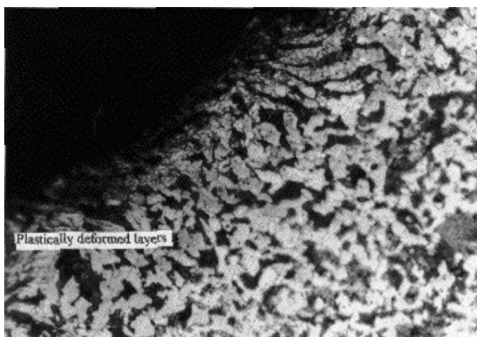
Figure 7.9 Subsurface microstructure of steel after shot peening.
