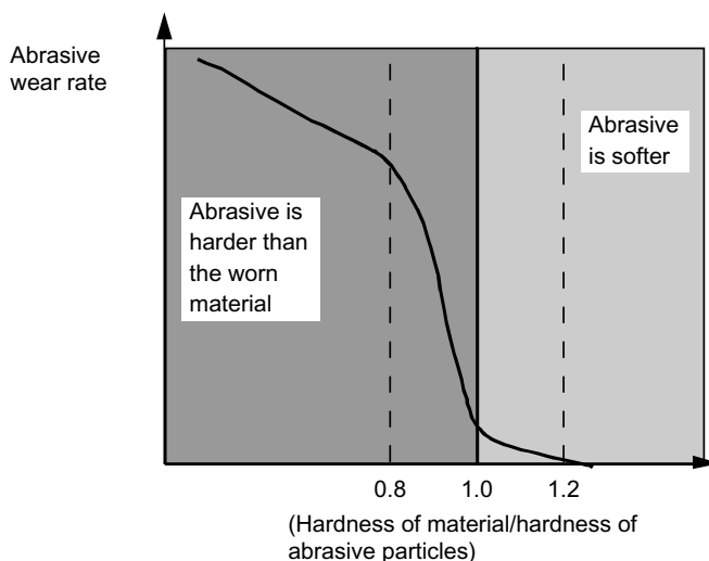
Figure 2.8 Effect of hardness of abrasive grit on abrasive wear rate.
