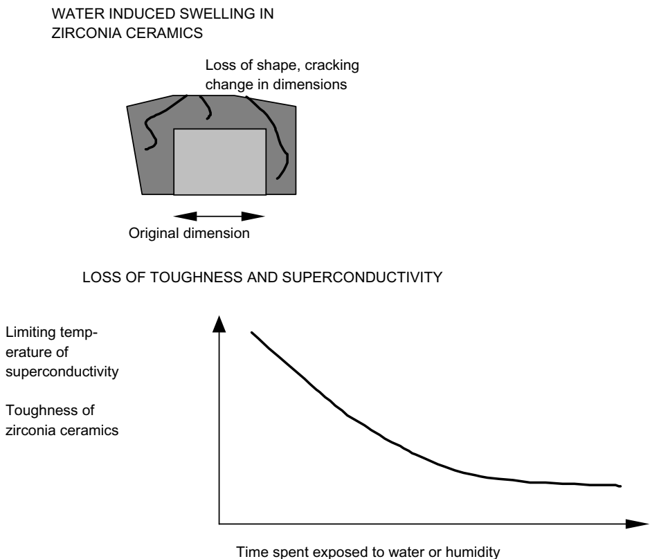
Figure 3.40 Water damage to zirconia ceramics and super conductive ceramics.
