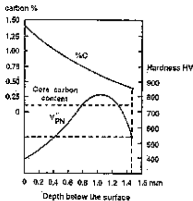
Figure 7.12 Theoretical subsurface distribution of carbon during carburization (Courtesy of Thelning and Bofors Ltd).
