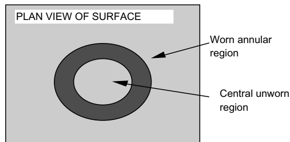
Figure 2.21 Origins of micro sliding in a Hertzian contact that sustains frictional force.
