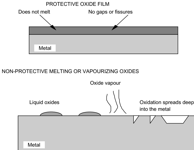
Figure 3.32 Catastrophic oxidation of a metal when its oxide film liquefies or evaporates.
