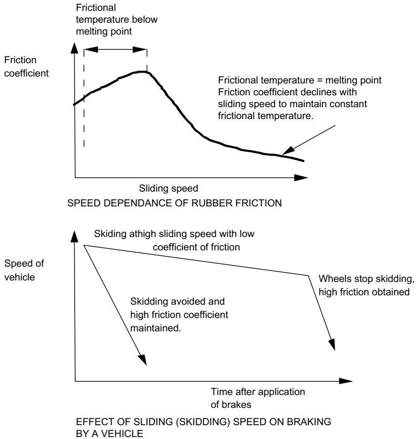
Figure 2.18 Decline in friction with sliding speed of rubber caused by melting wear and its effect on skidding by rubber tires.
