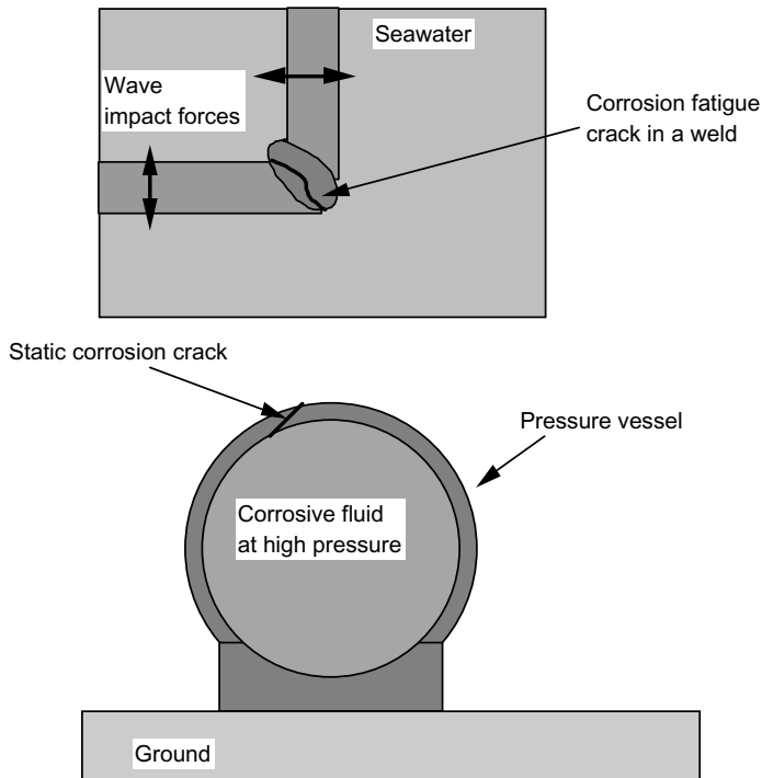
Figure 5.8 Examples of corrosion fatigue and corrosion fracture.
