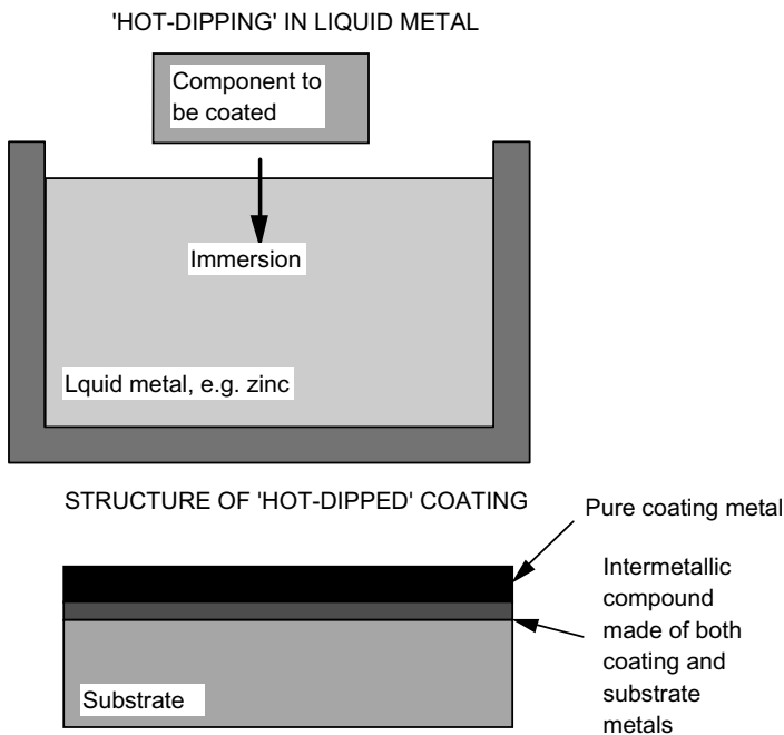
Figure 7.10 The process of hot-dipping and structure of hot-dipped coatings.
