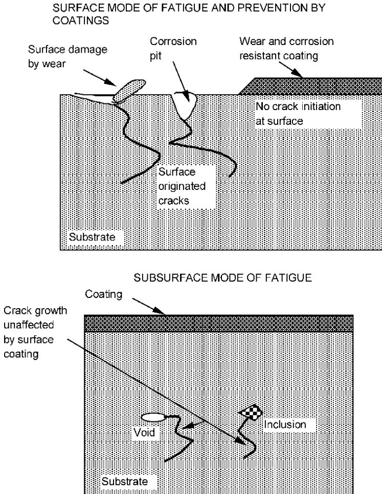
Figure 9.4 Mechanisms of protection by coatings against mechanical fatigue.
