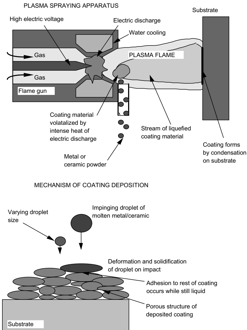
Figure 6.5 The Plasma spraying process.
