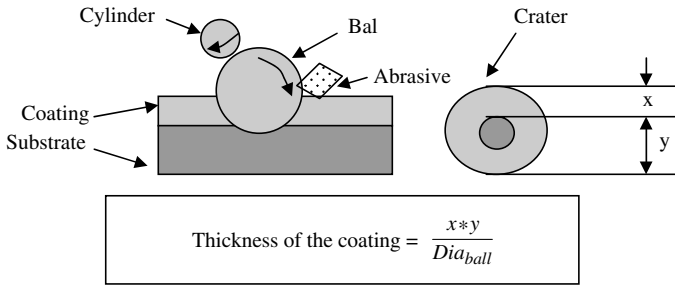
Figure 8.6 Schematic illustration of the ball crater method for the determination of coating thickness.
