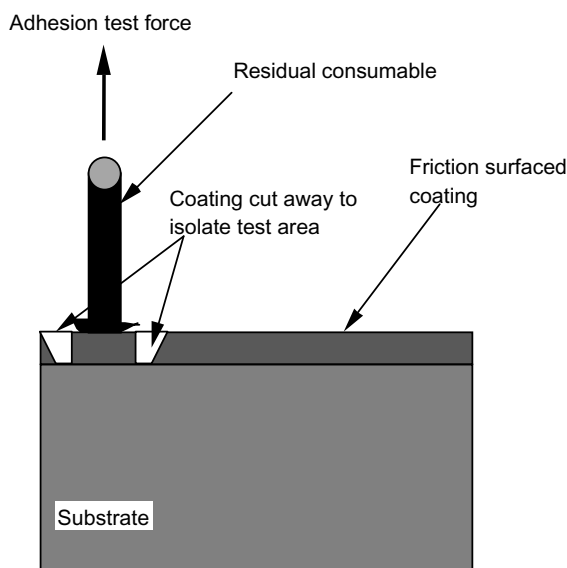
Figure 8.13 Adhesivity test for friction surfacing.
