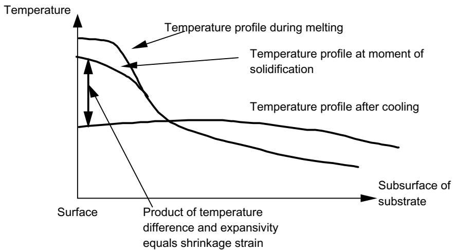
Figure 7.8 Mechanism of thermal shrinkage cracking in laser surface alloyed and electron beam surface alloyed coatings.
