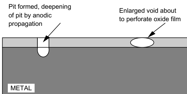
Figure 3.14 Mechanisms of pit nucleation and propagation.
