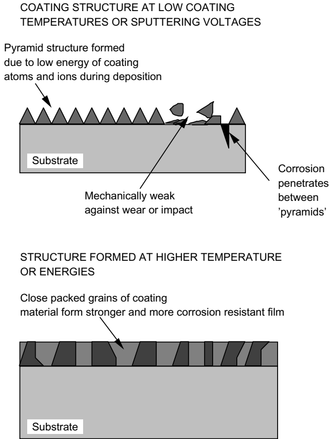
Figure 6.12 Strong and weak microstructures of sputtered coatings.
