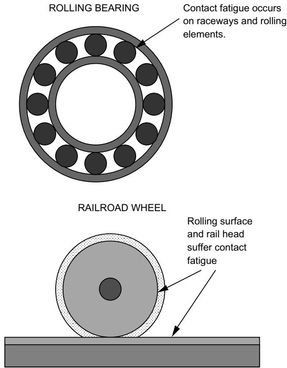
Figure 2.29 Common examples of rolling contact fatigue.
