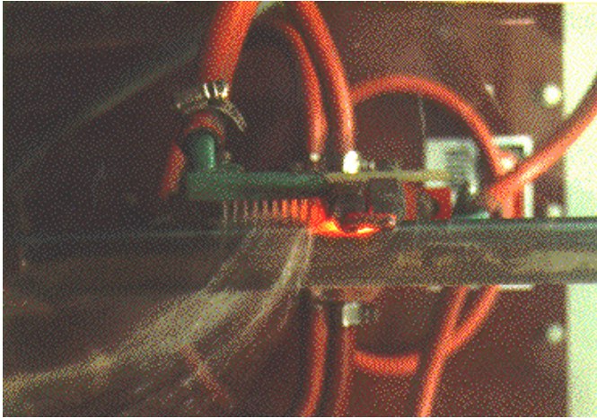
Figure 7.4 Induction hardening of platen shaft. (Courtesy of Doxon Engineering Pte. Ltd, Singapore.)
