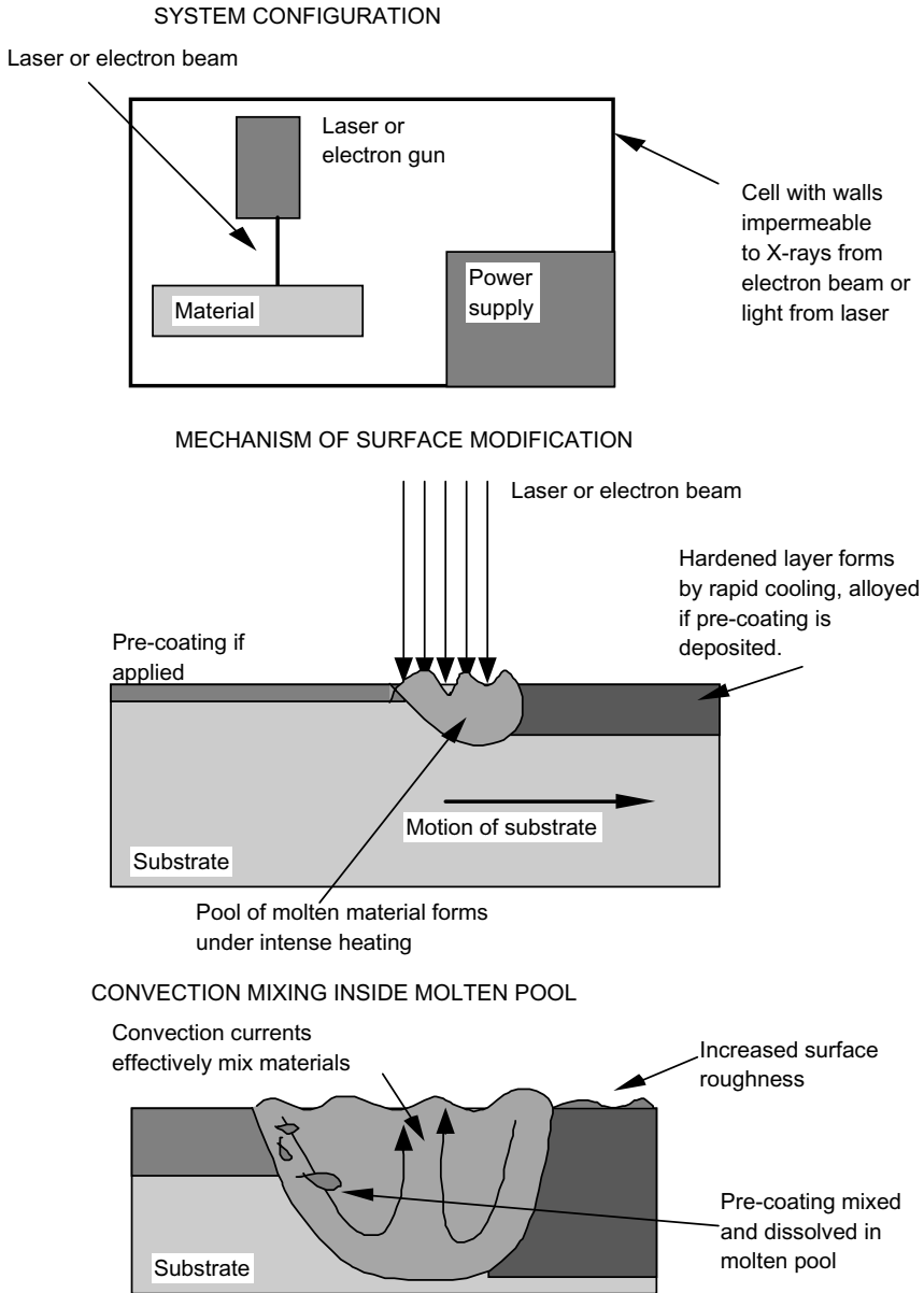
Figure 7.7 Mechanism of surface hardening and surface alloyed layer formation by scanning with high power laser or electron beams.
