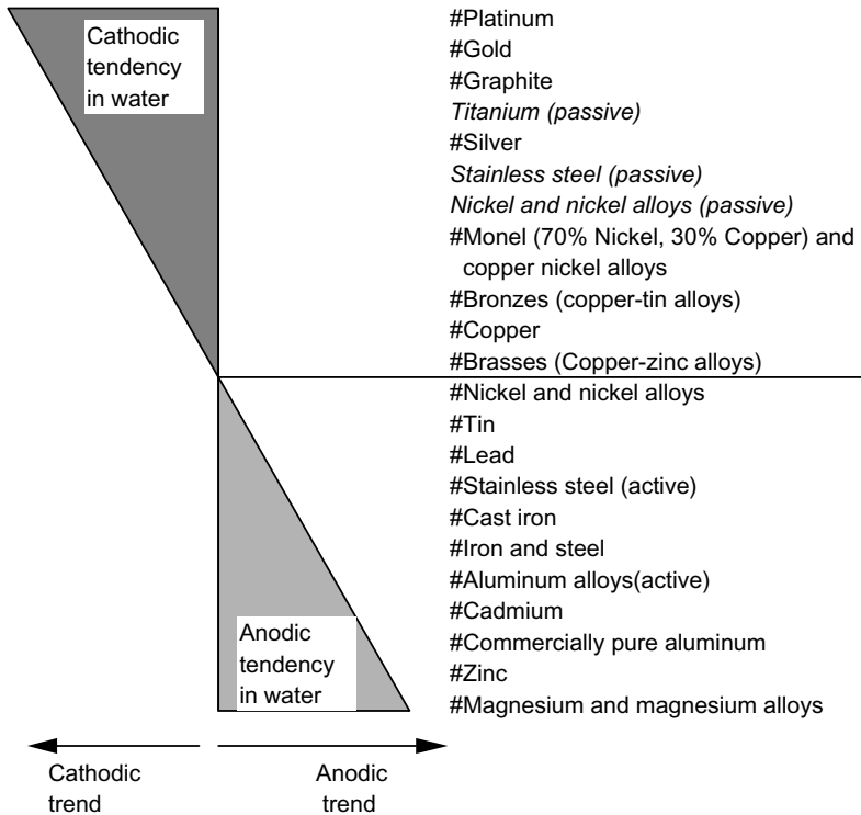
Figure 3.7 The galvanic series of metals.
