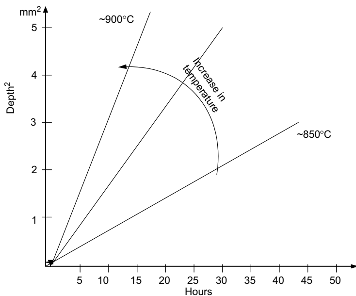
Figure 7.14 Typical hardness profiles of carburized alloy steels (Adapted from Thelning).
