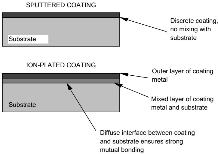
Figure 6.15 Formation of intermediate layer between substrate and coating by ion plating.
