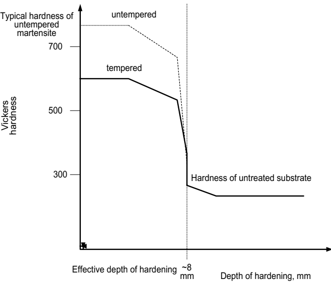
Figure 7.6 Schematic diagram depicting the effect of tempering on the hardness profile of alloy steel (Adapted from Thelning).
