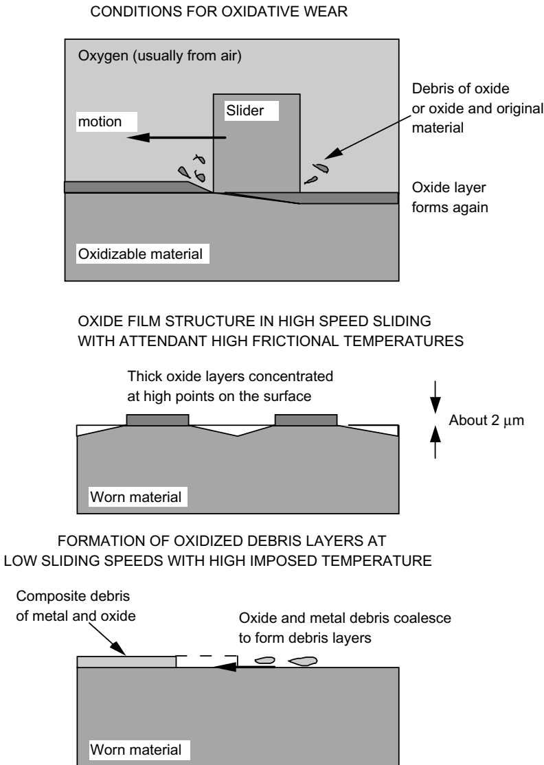
Figure 5.4 Mechanisms of corrosive wear by air, i.e. Oxidative wear .
