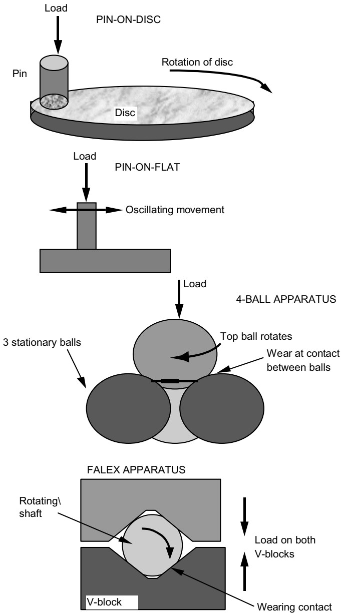
Figure 8.28 Configurations of standard wear tests.
