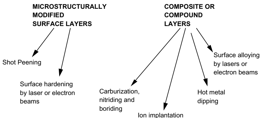
Figure 7.1 The basic categories of integral coatings and modified surface layers.
