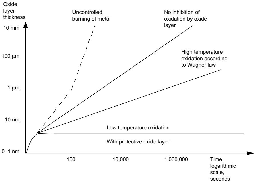
Figure 3.30 Growth characteristics of oxide films on metal surfaces.
