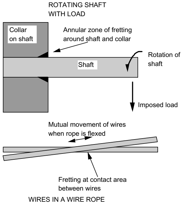
Figure 2.20 Location of fretting wear in some common engineering components.
