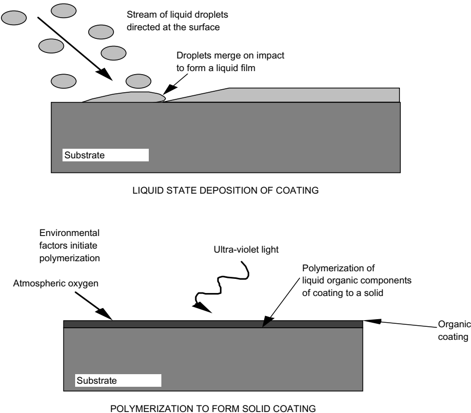
Figure 6.2 Mechanism of paint film formation.
