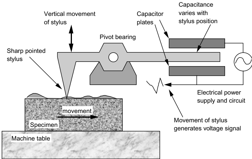
Figure 8.3 The contact method of surface roughness measurement.
