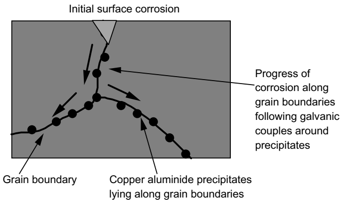
Figure 3.26 Intergranular corrosion mechanism of aged copper-aluminum alloys.
