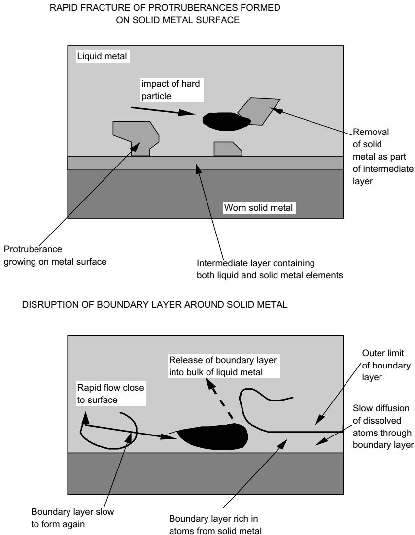
Figure 5.7 Mechanisms of wear by abrasive grits in liquid metal, (i) accelerated detachments of protuberances from the intermediate layer, (ii) disruption of the boundary layer by abrasive grits.
