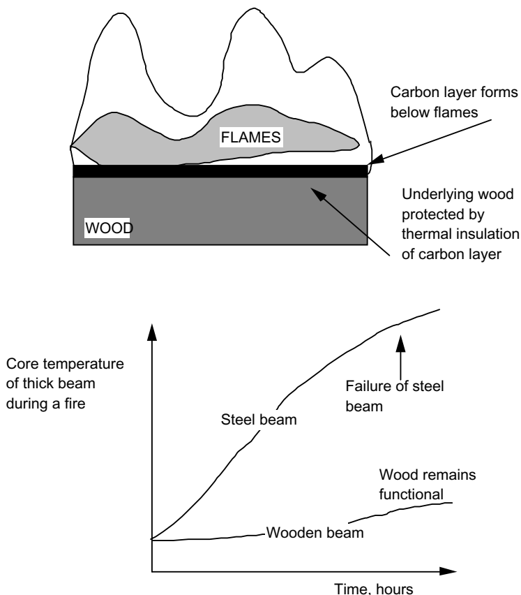
Figure 4.2 Role of thermal insulation in protecting wood from damage by fire.
