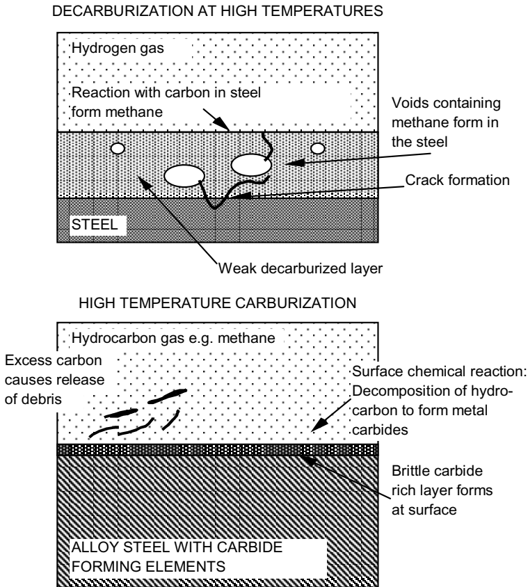
Figure 3.34 Mechanisms of decarburization and carburization.
