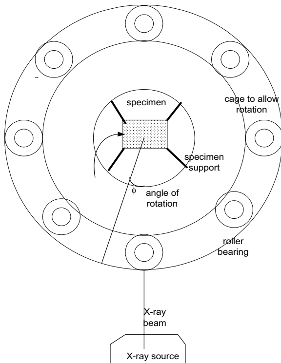
Figure 8.23 Strain measurement by X-ray diffractometry.
