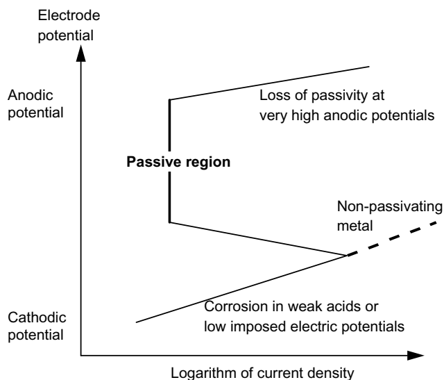
Figure 3.22 Display of anodic passivation on the Tafel diagram.
