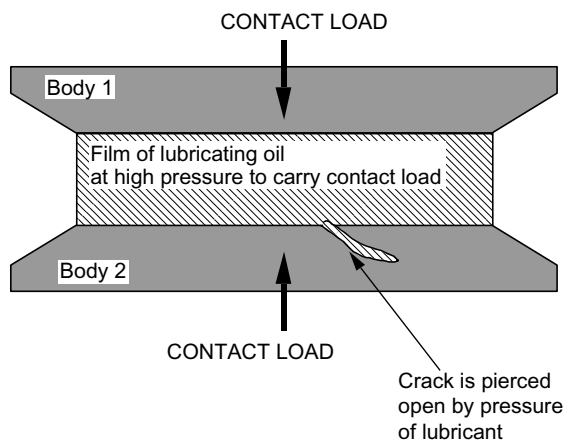
Figure 2.31 Mechanism of hydraulic crack propagation in lubricated rolling contact fatigue.
