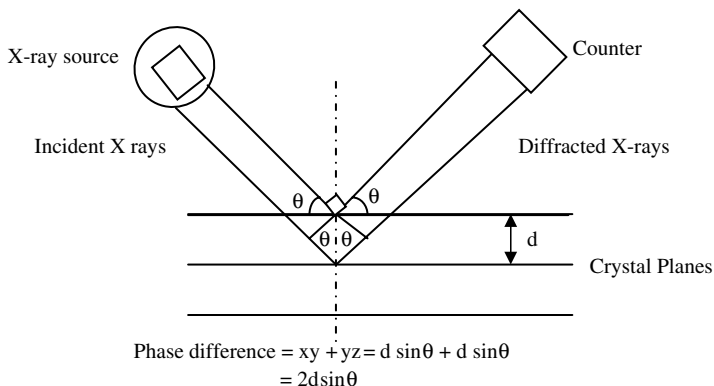
Figure 8.22 X-ray diffraction by a crystal lattice when irradiated with monochromatic X-rays.
