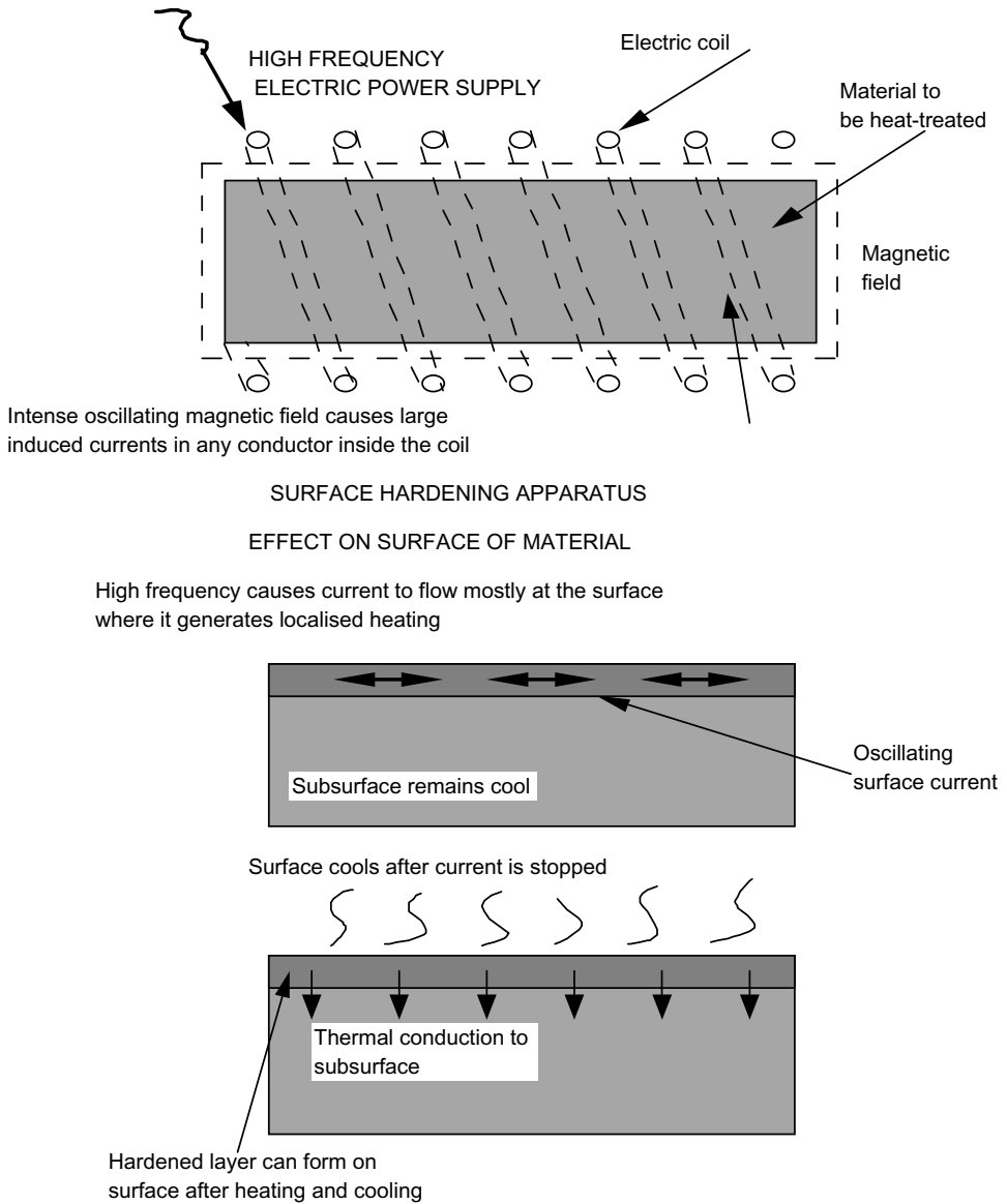
Figure 7.3 Operating principle of surface hardening by magnetically induced current.
