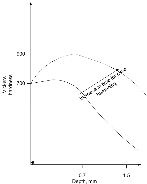
Figure 7.16 Schematic illustration of effect of carburizing time on case depth (Adapted from Thelning).
