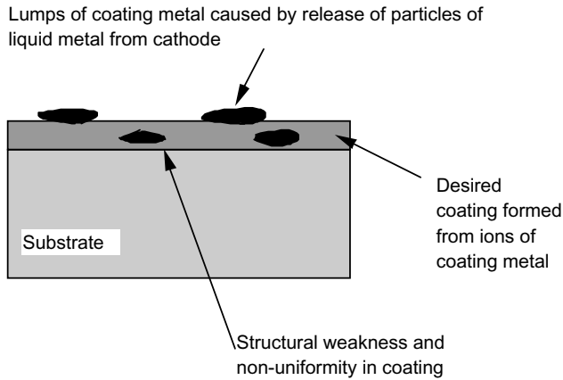
Figure 6.19 Degradation of arc evaporation coatings by uncontrolled formation of lumps inside the coating.
