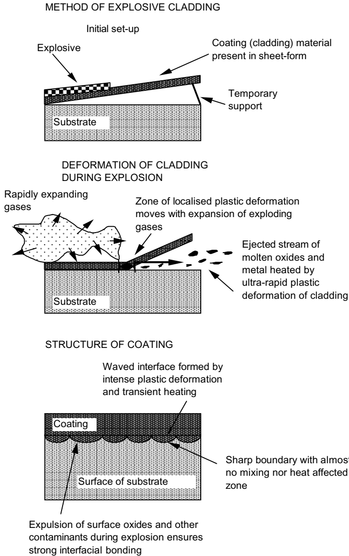
Figure 6.22 The method of explosive cladding and mechanism of bonding between coating and substrate.
