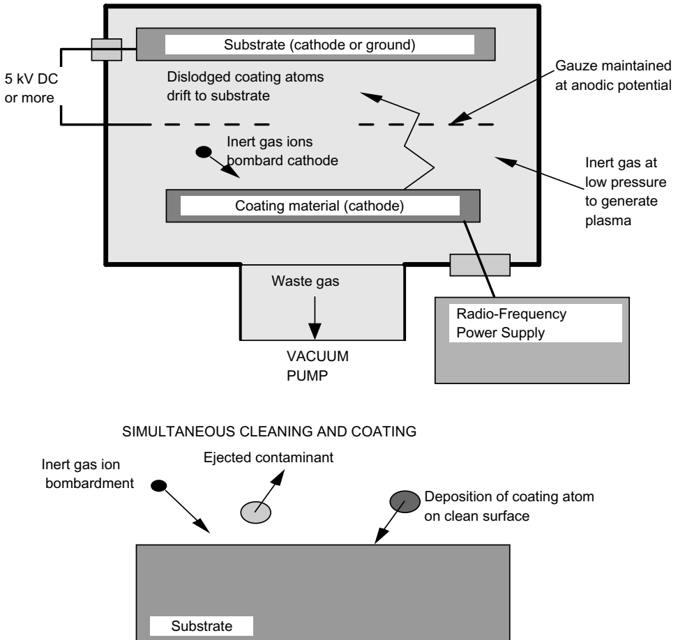
Figure 6.11 The principle of sputter coating or sputtering.
