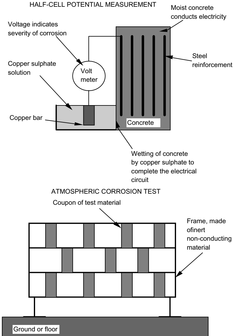
Figure 8.27 Basic principle of atmospheric corrosion tests.
