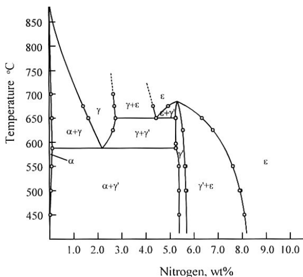
Figure 7.22 The Fe-N binary phase diagram (Adapted from M. Hansen ).
