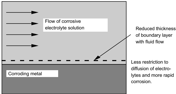
Figure 3.17 Thinning of a boundary layer and enhanced diffusion of corrosive agents during flow of a corrosive fluid.
