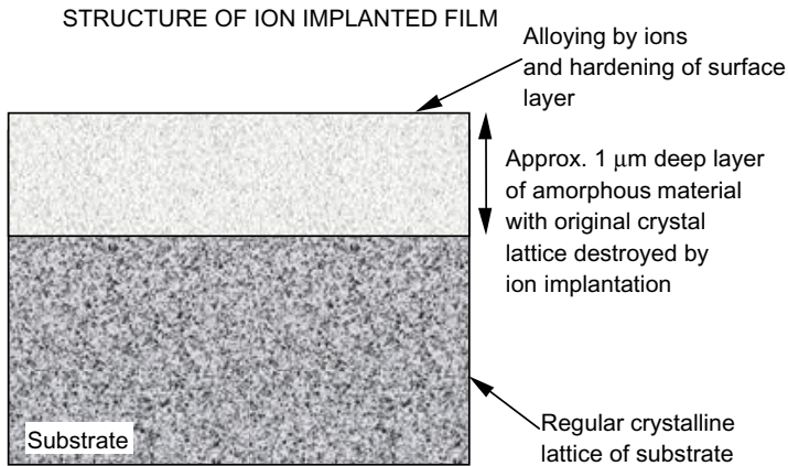
Figure 7.29 Schematic illustration of the effect of implantation.
