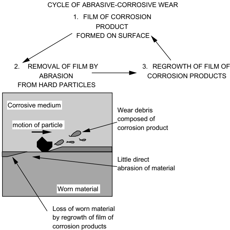
Figure 5.5 Mechanism of corrosive-abrasive wear.
