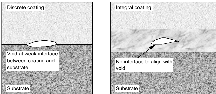
Figure 7.2 Comparison of hardness profiles and failure mechanisms for integral and discrete coatings.
