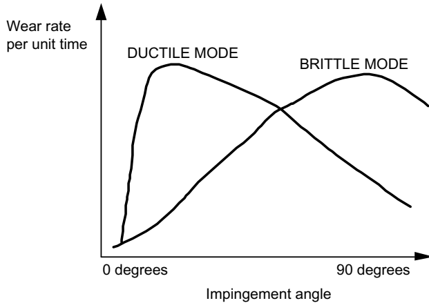
Figure 2.13 Contrast in dependence on impingement angle for brittle and ductile modes of erosive wear.
