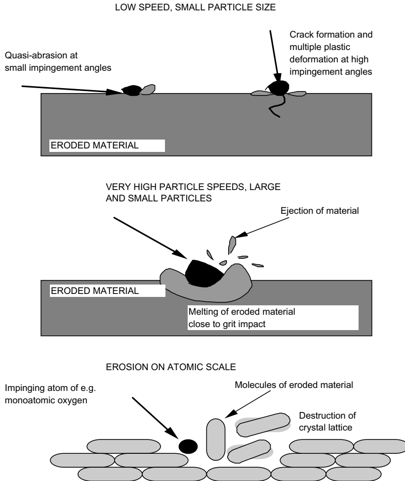
Figure 2.12 Mechanisms of erosive wear for varying particle speeds, sizes and impingement angles.
