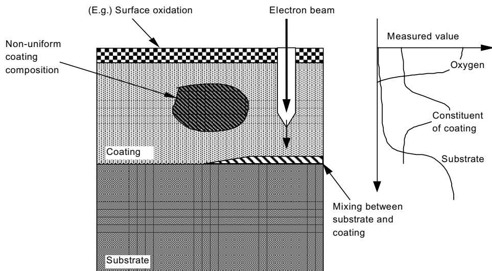
Figure 8.20 Significance of depth and area determination of chemical element distributions in a coating.
