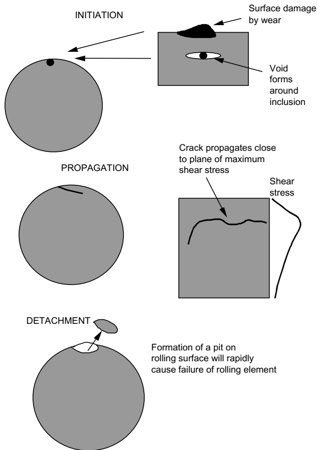
Figure 2.30 Mechanism of rolling contact fatigue.
