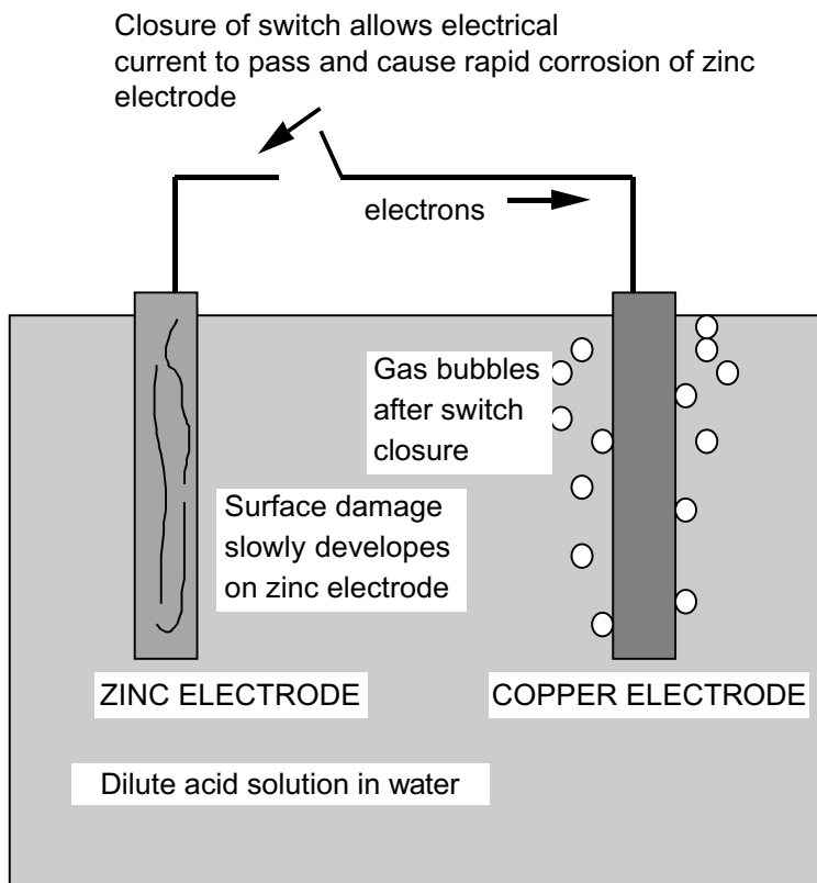
Figure 3.2 Electrochemical interactions between dissimilar metals immersed in an aqueous solution of electrolyte.
