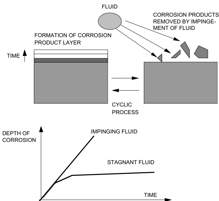
Figure 3.16 Effect of fluid flow on corrosion mechanisms.
