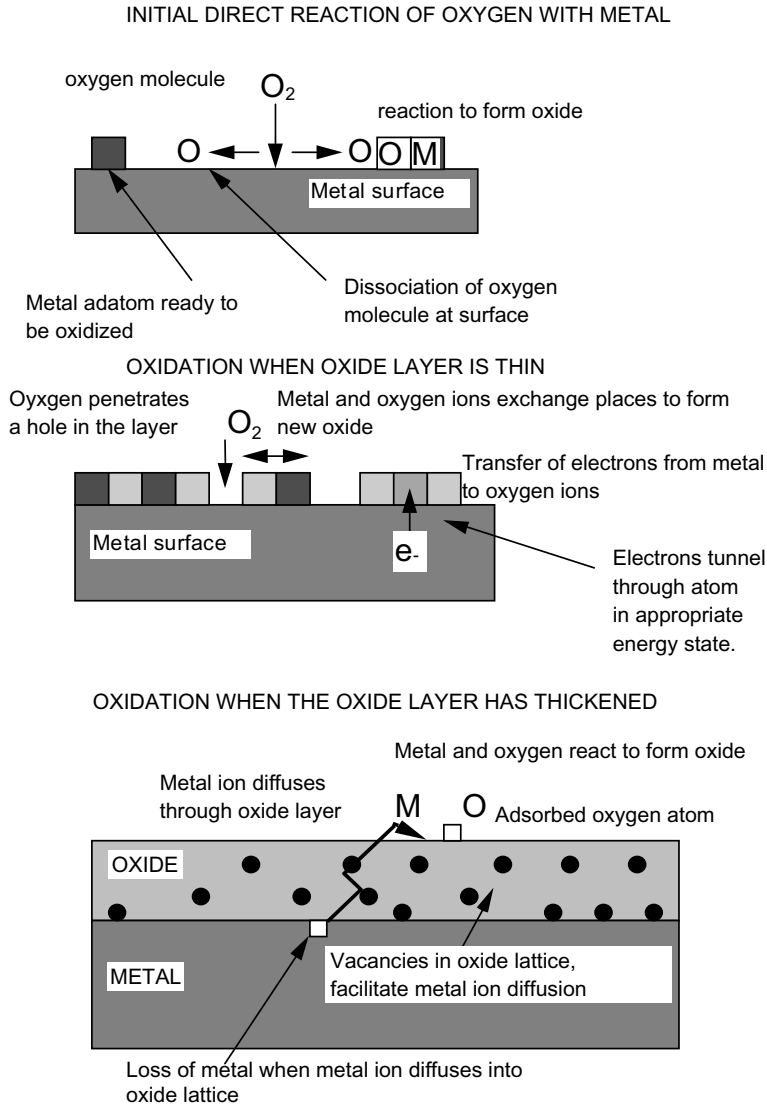
Figure 3.28 Corrosion product film formation on a metal surface. Initial direct oxidation with the metal and subsequent corrosion product film formation.
