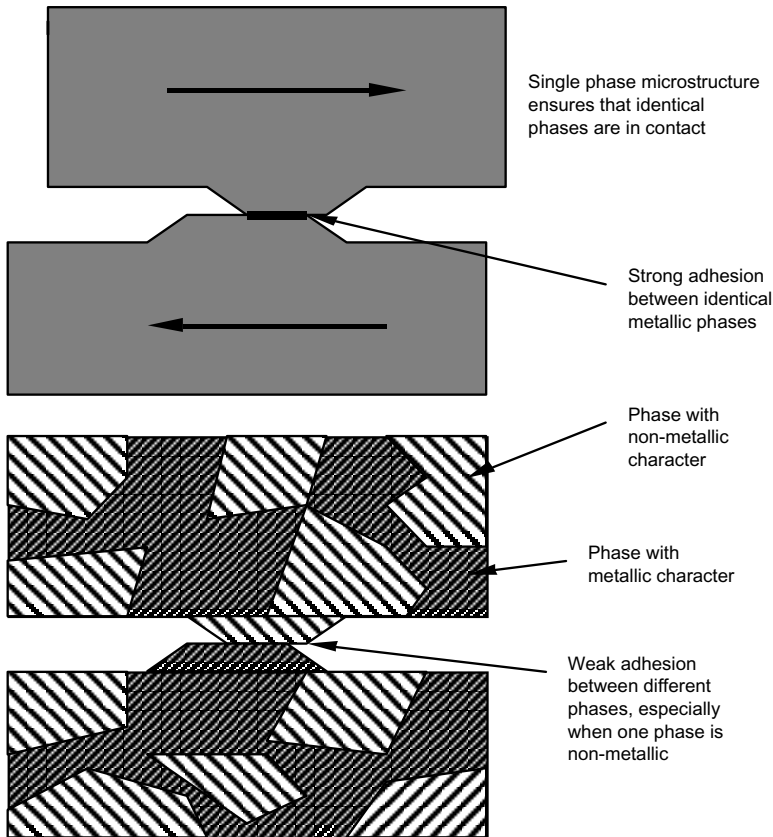
Figure 2.6 Microstructural effects on adhesive wear.
