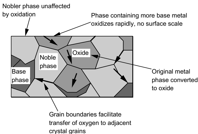
Figure 3.33 Mechanism of internal oxidation of metal alloys.
