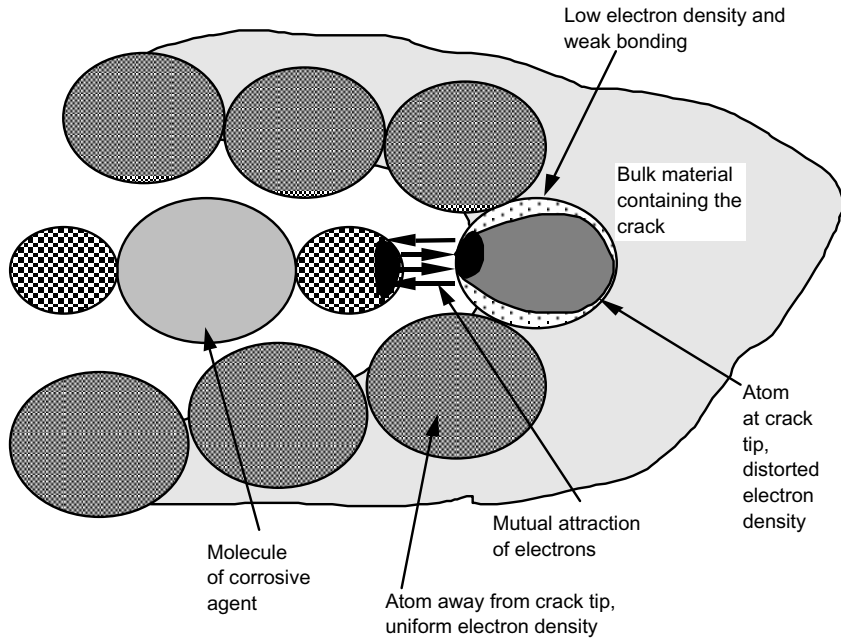
Figure 5.9 Mechanism of weakening of material around a crack tip by molecules or atoms of a corrosive substance.
