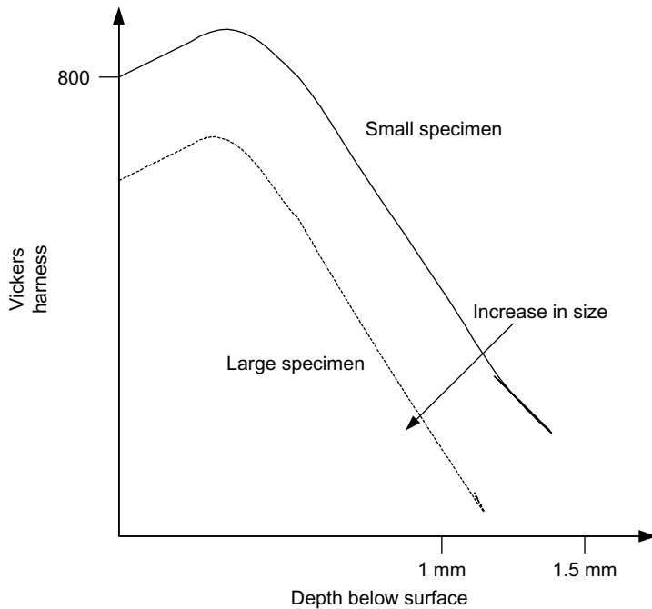
Figure 7.15 Schematic illustration of influence of specimen diameter on hardness distribution (Adapted from Thelning).
