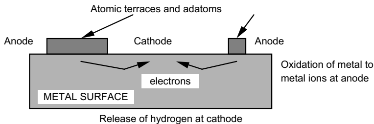
Figure 3.11 Analysis by Tafel model of corrosion of zinc and iron electrodes in acid.
