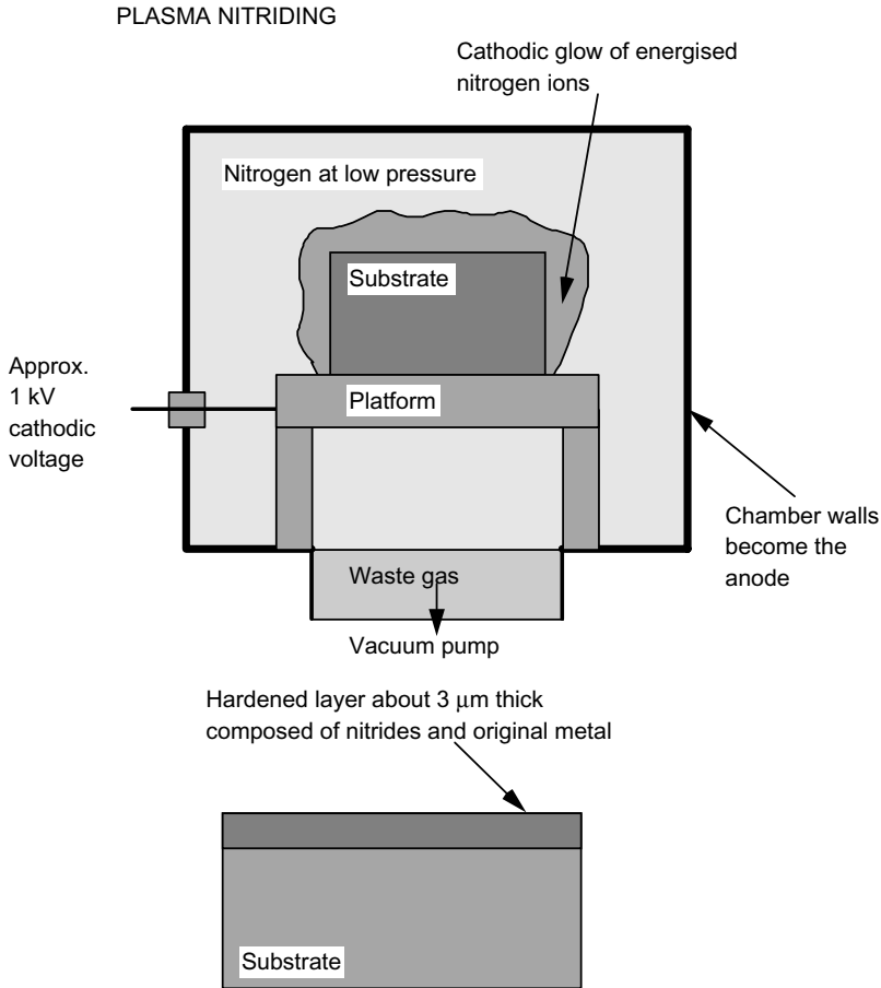
Figure 7.26 Principle of operation of plasma nitriding apparatus and structure of coating produced.
