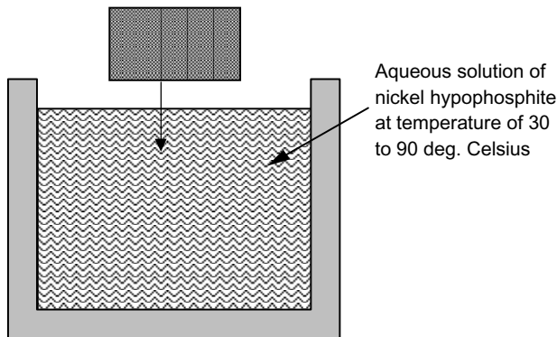
Figure 6.4 The electro-less coating process.
