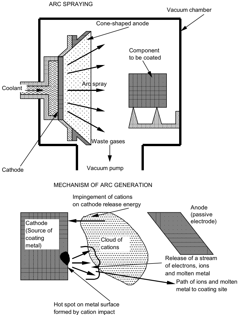
Figure 6.18 Principle of operation of an arc evaporation system.
