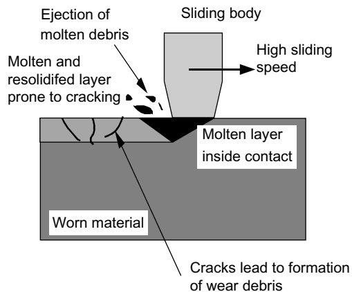
Figure 2.17 Mechanism of melting wear.
