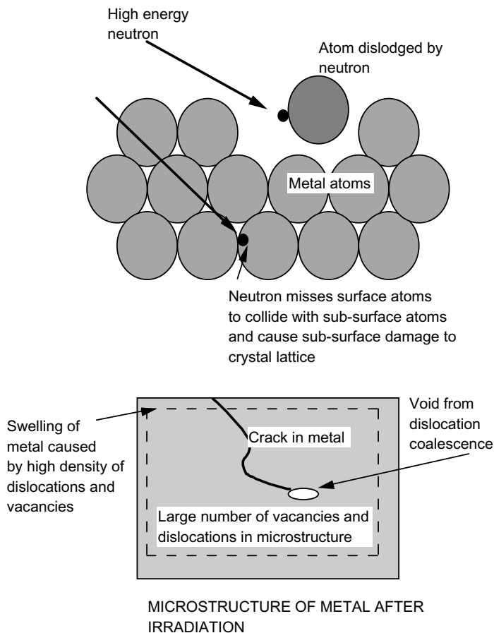
Figure 4.4 Damage mechanisms in metals when subjected to high energy neutron irradiation.
