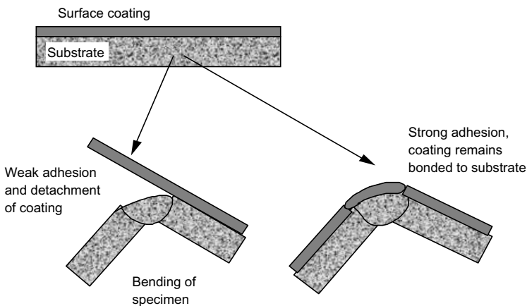
Figure 8.11 Principle of bend test for coating adhesion.
