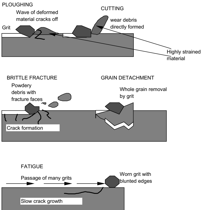
Figure 2.7 Mechanisms of abrasive wear.
