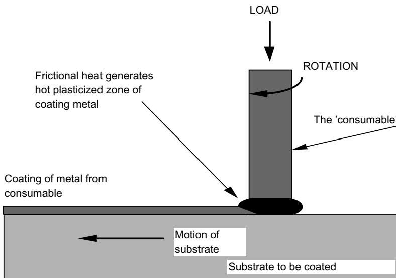
Figure 6.20 Mechanism of friction surfacing.
