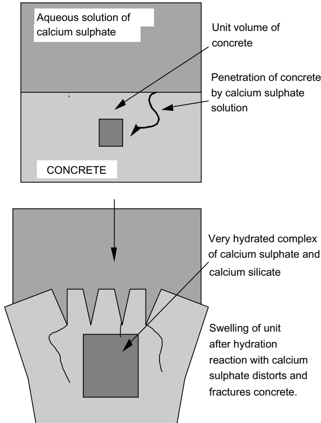
Figure 3.37 Mechanism of swelling in concrete immersed in calcium sulphate solution.
