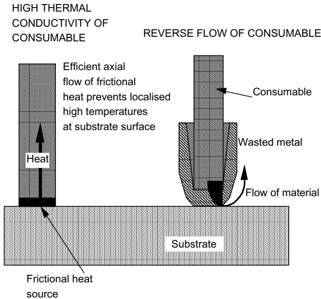
Figure 6.21 Problems associated with friction surfacing: thermal conductivity, wear resistance and consumable return.
