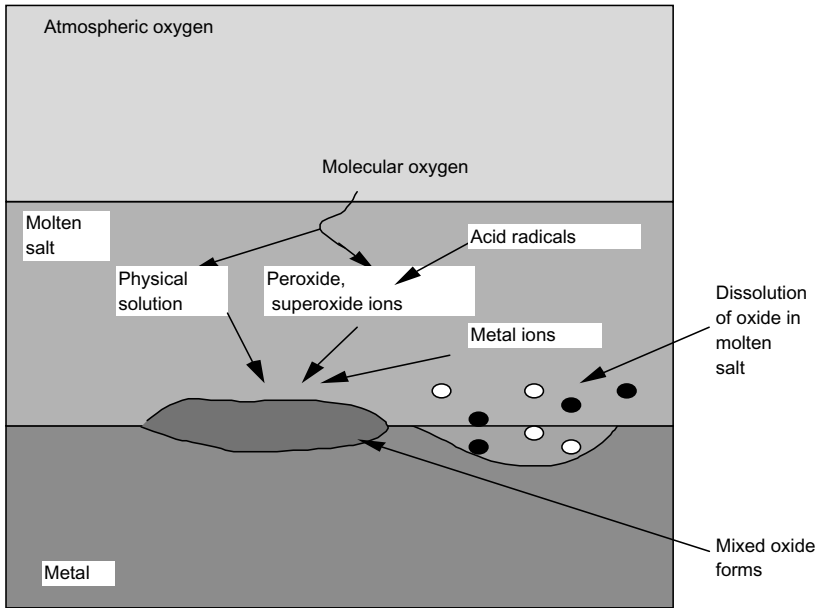
Figure 3.43 Mechanism of corrosion of metals by molten salts.
