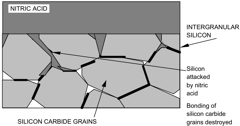
Figure 3.39 Acid attack of silicon impurities in silicon carbide.
