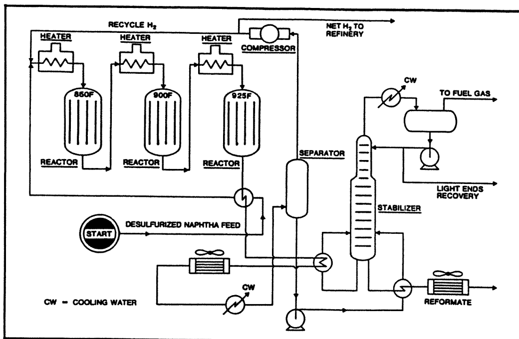
Figure 3.17 Catalytic reforming 1
