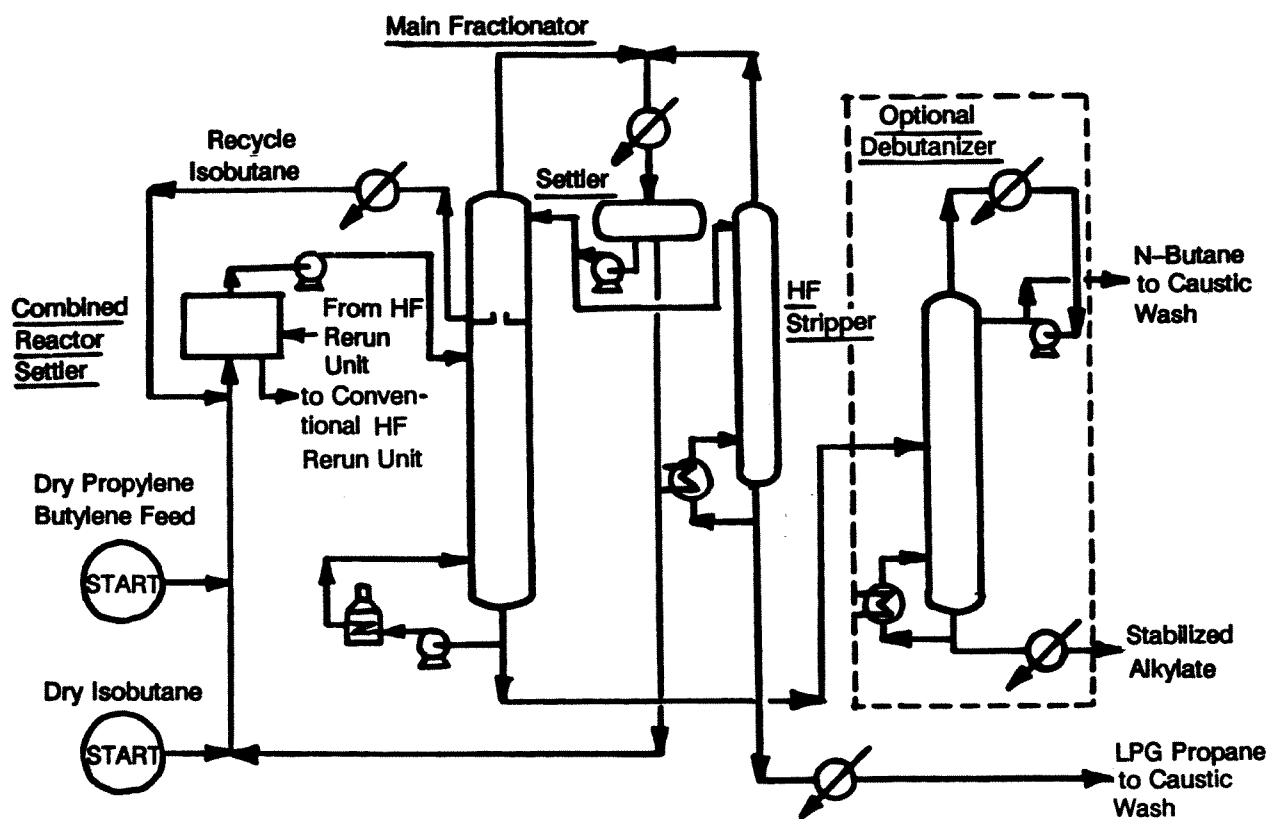
Figure 2.8 Hydrofluoric acid alkylation 2
