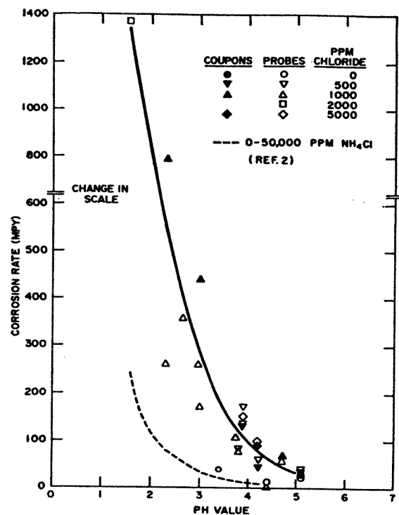
Figure 1.6 Corrosion of steel in aqueous sulfide solutions. Note the acid corrosion region because of an excess of hydrogen ions at pH values below 4.5. 5
