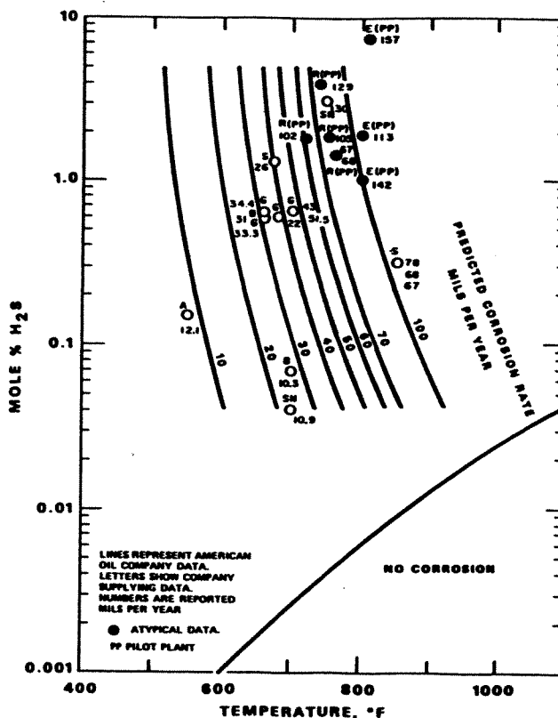
Figure 3.7b Carbon steel, gas oil diluent
