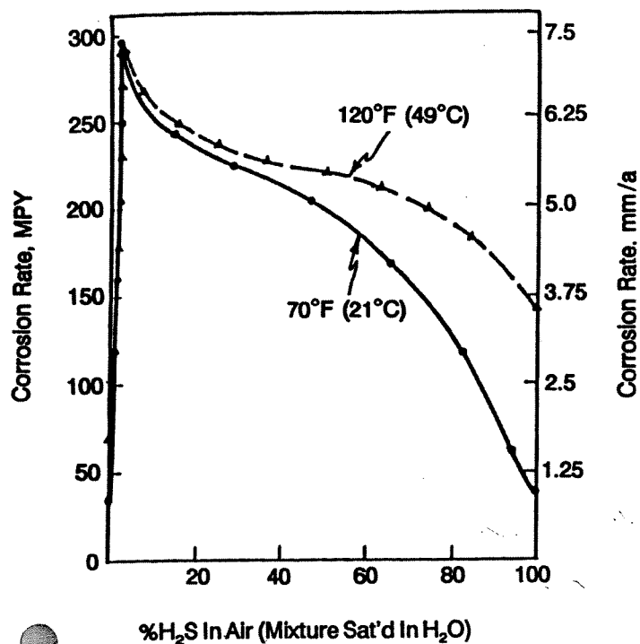
Figure 5.26 Corrosion rate of wet steel in atmospheres containing H_2S mixtures 9
