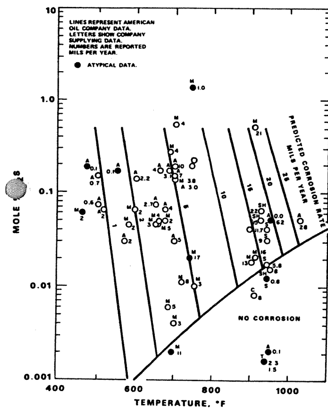
Figure 3.7g 12% Cr stainless steel, naptha diluent
