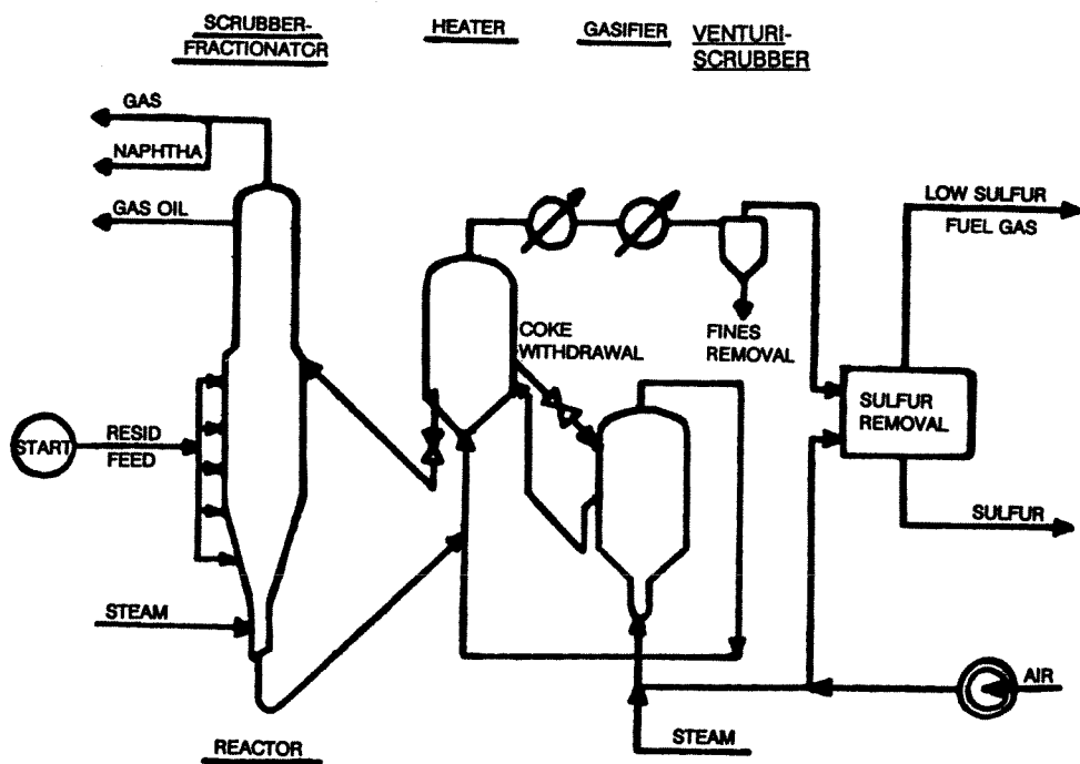
Figure 2.2 Flexicoking 2
