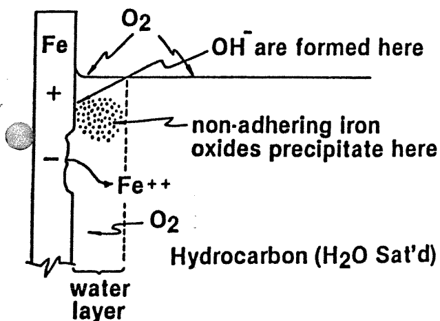
Figure 5.28 Mechanism of shell-side corrosion in gasoline and light-products storage tanks 9
