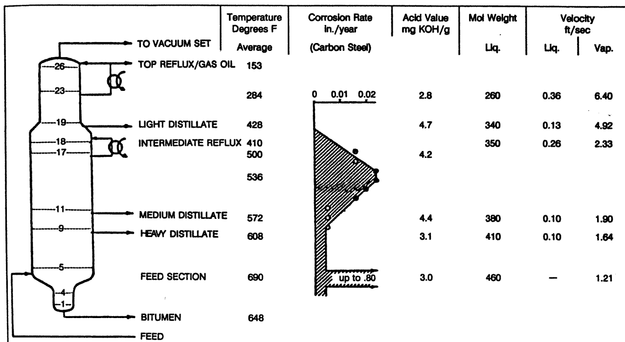
Figure 1.16 Corrosion and operating data of a high vacuum column processing a reduced crude. 11
