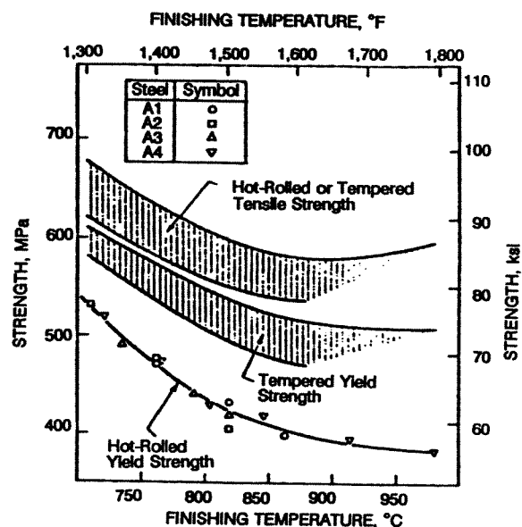
Figure 5.11 Effect of finishing temperature and tempering on the strength of steels A1 to A4. 4
