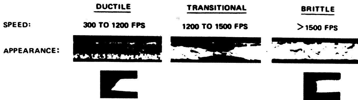
Figure 5.14 Fracture characteristics observed from line pipe through the transition temperature 2
