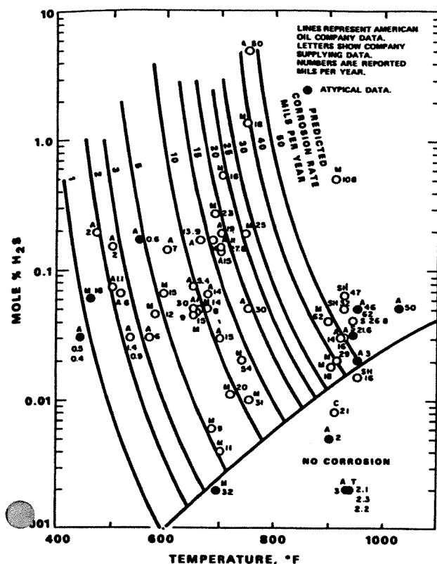
Figure 3.7a Carbon steel—naptha diluent
