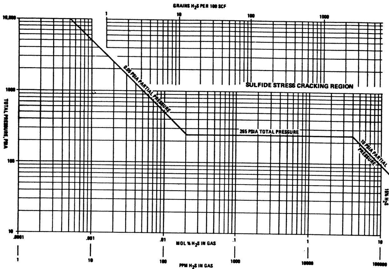
Figure 2.10 Sour multiphase systems 4
