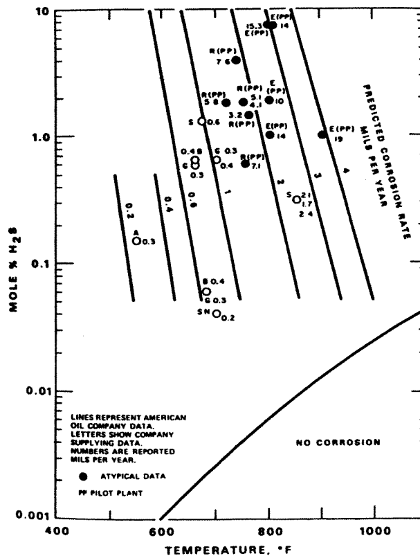
Figure 3.7j 18-8 stainless steel, gas oil diluent
