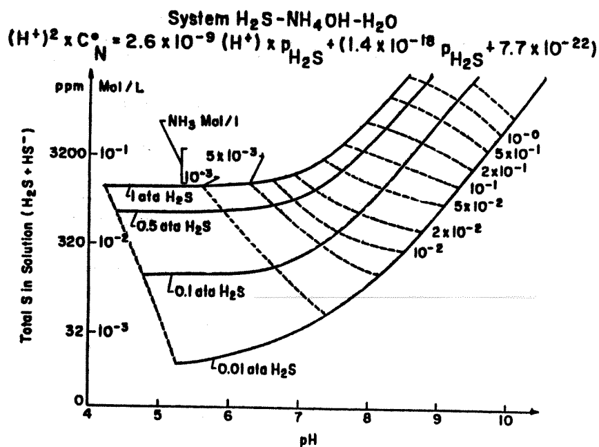
Figure 1.4 Total S in solution vs pH. 3
