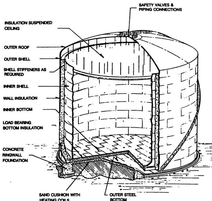
Figure 5.29 Double wall tank for low temperature service 10
