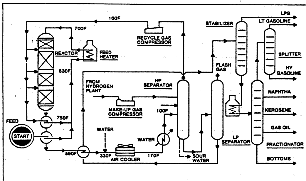
Figure 3.2 Hydrocracking 1
