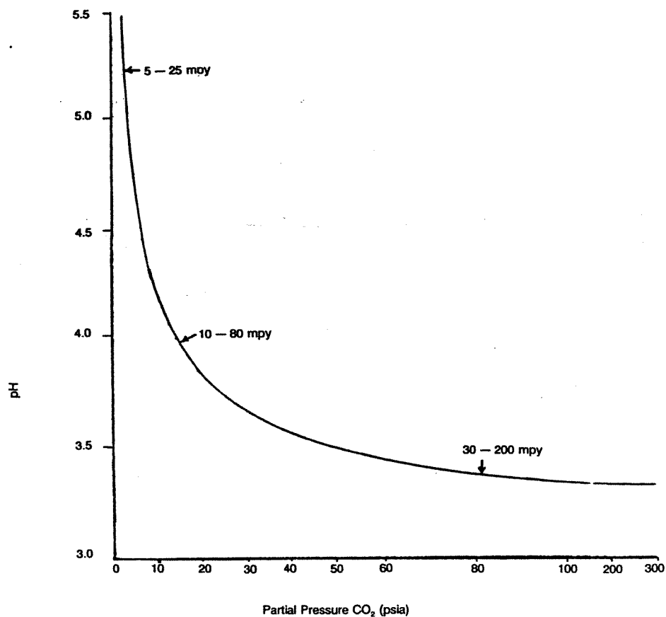
Figure 4.5 Relationship between pH, carbon dioxide partial pressure, and estimated corrosion rate on carbon steel at 100°F (38°C) 2
