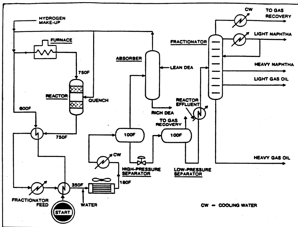
Figure 3.1 Hydrodesulfurizer 1
