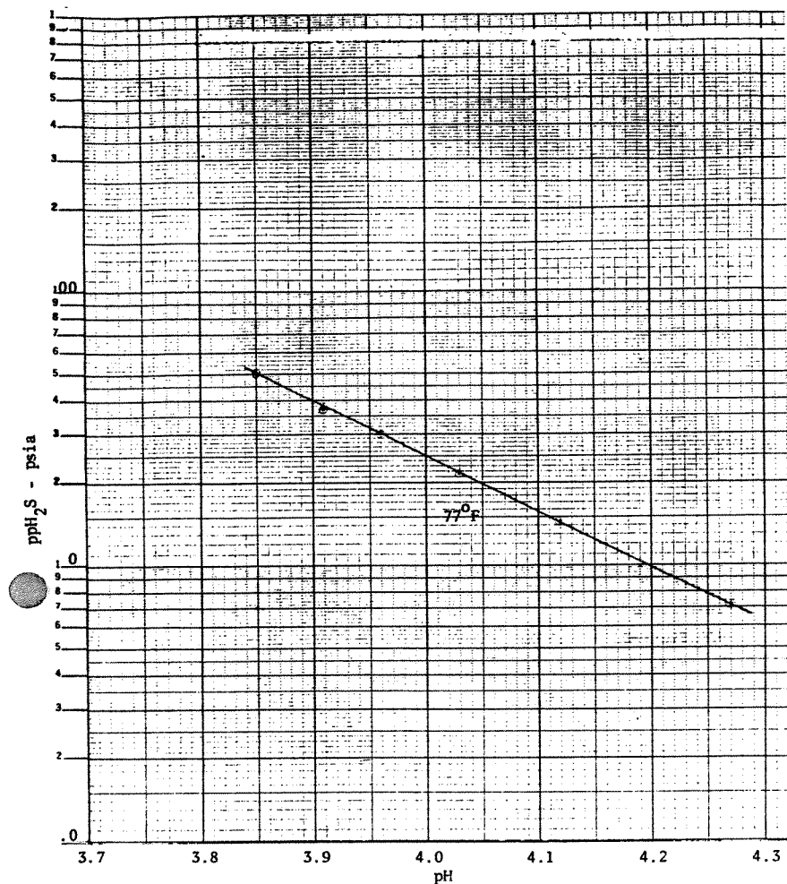
Figure 1.9 Solubility of H_2S in water. Partial pressure of H_2S in vapor vs pH of solution. 8
