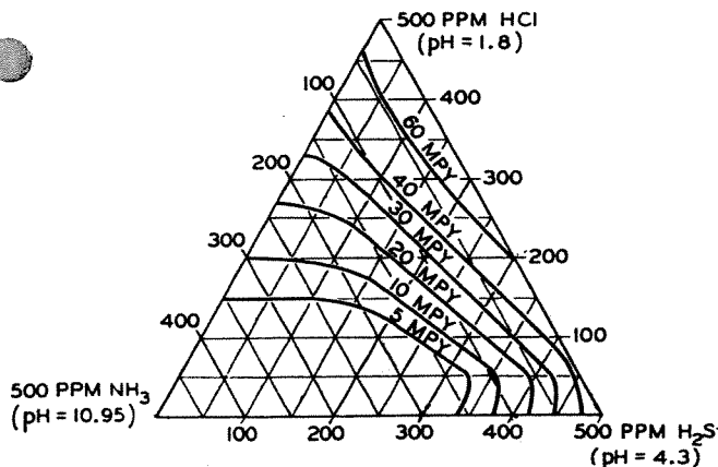
Figure 3.12 Iso-corrosion lines for carbon steel in aqueous HCl-H 2 S-NH 3 system (500 ppm total; air atmosphere, room temperature, and atmospheric pressure) 7
