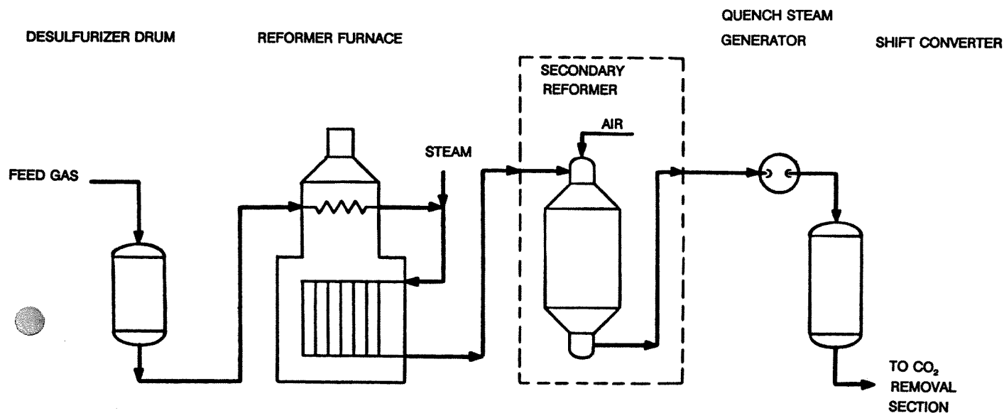
Figure 4.4 High temperature front end section of reforming plant 2
