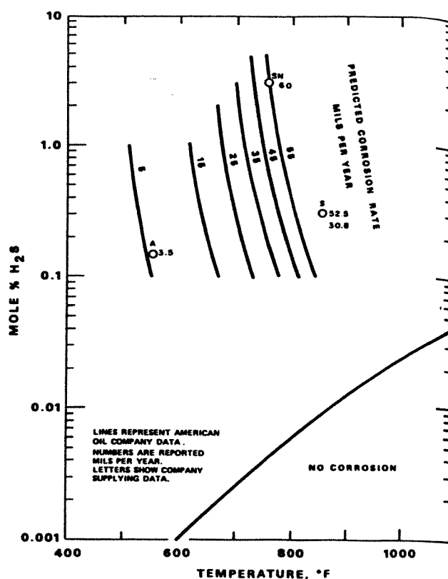
Figure 3.7f 9% Cr steel, gas oil diluent
