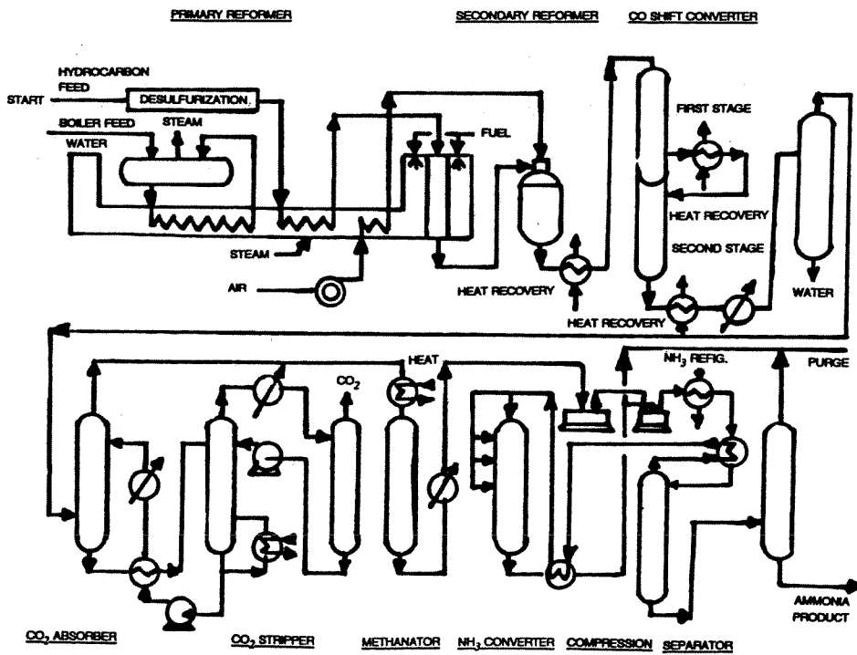
Figure 4.2 Ammonia 1
