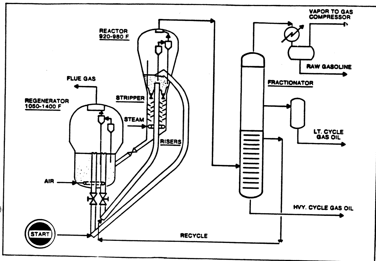
Figure 2.1 Fluid catalytic cracking 1
