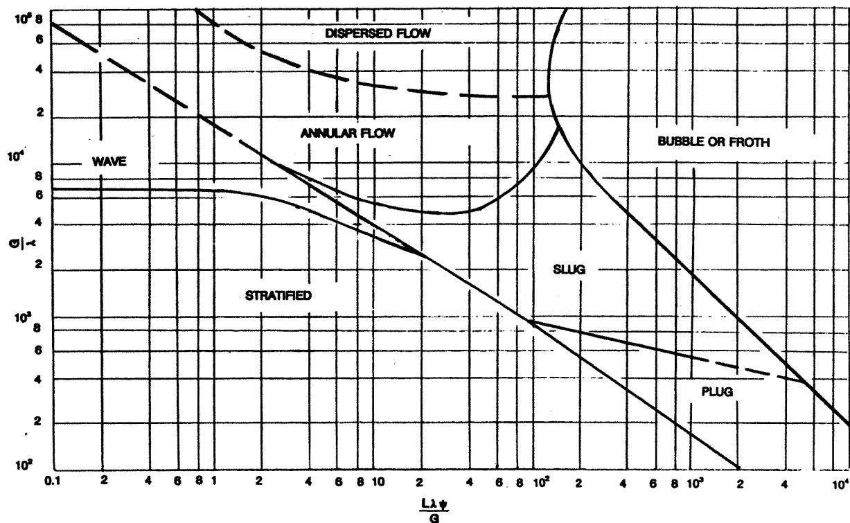
Figure 5.22 Gas/Liquid phase flow 6
