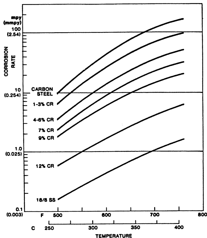
Figure 1.11 Average corrosion rates of high temperature sulfur corrosion in a hydrogen free environment as compiled from 1961 A.P.I. questionnaire data from industry-desulfurizing processes and published or reported data—nondesulfurizing processes. 9
