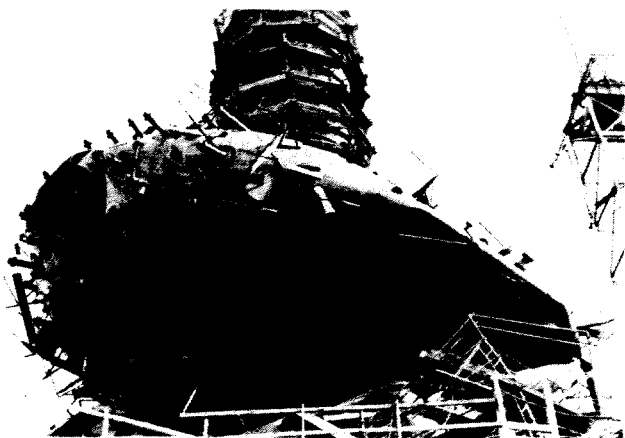
Figure 2.3 Front view of collapsed vessel. Test closure for vapor line opening in top center of top head at upper left. 3
