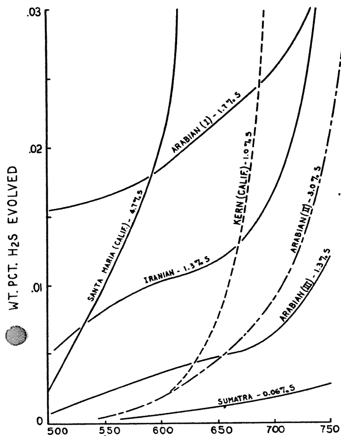
Figure 1.13 Hydrogen sulfide release from crudes. 10
