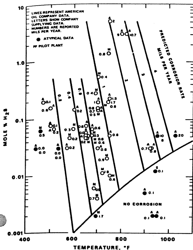
Figure 3.7i 18-8 stainless steel, naptha diluent
