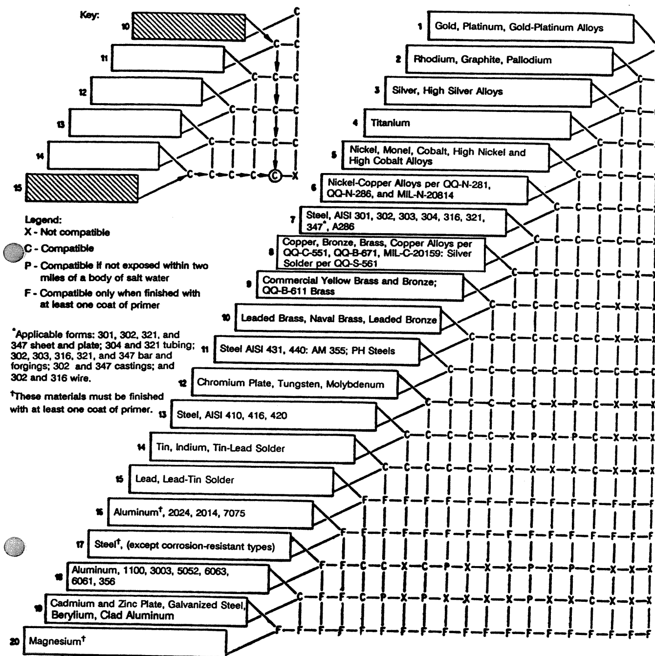
Figure 1.22 Atmospheric compatibility of metals. 17
