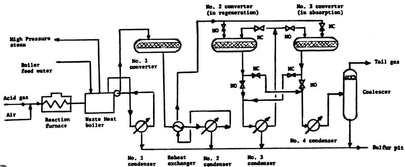
Figure 2.12 Sulfur plant 2
