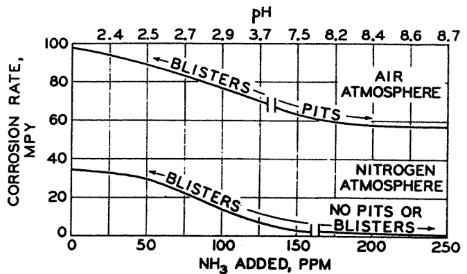
Figure 3.13 Effect of NH 3 neutralization on corrosion of carbon steel in an aqueous solution containing 400 ppm HCl, 50 ppm H 2 S, 50 ppm NH 3 at room temperature and atmospheric pressure 7
