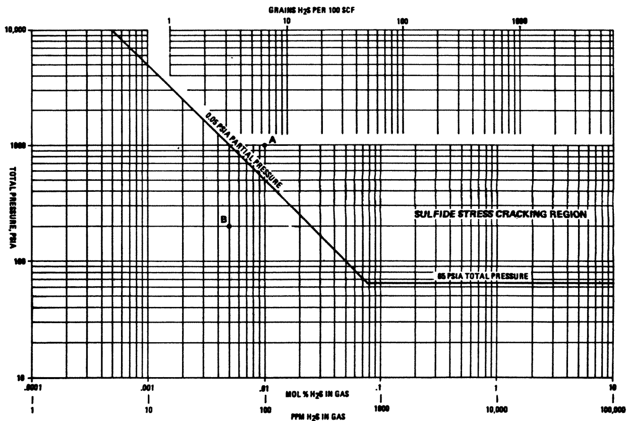
Figure 2.9 Sour gas systems 4
