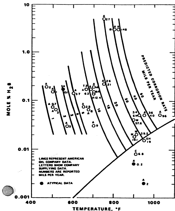
Figure 3.7e 9% Cr steel, naptha diluent
