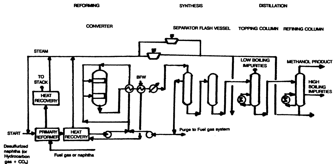
Figure 4.3 Methanol (ICI low pressure process) 1
