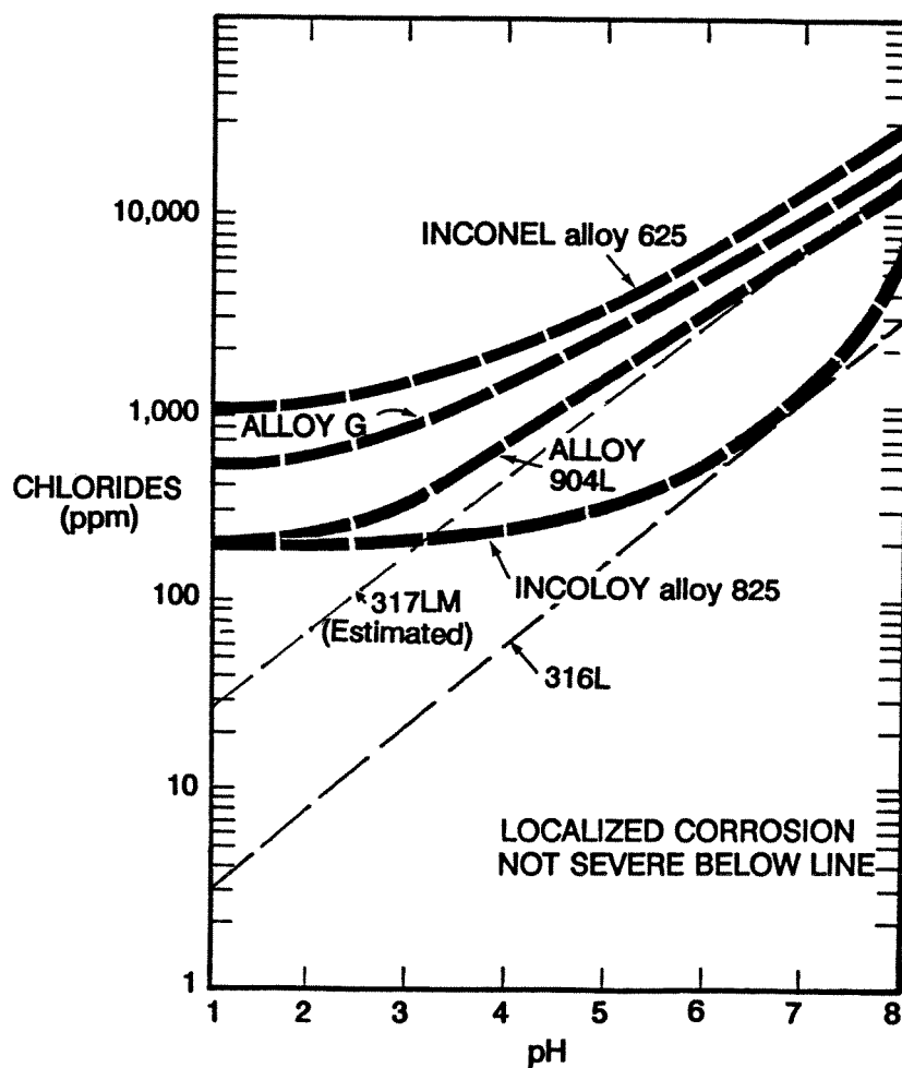
Figure 3.18 Predicted corrosion behavior of alloys in \text{SO}_2 scrubber environments from field tests (125-160°F [50-70°C] oxidizing) 9
