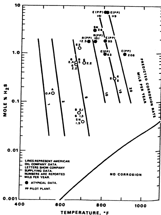
Figure 3.7h 12% Cr stainless steel, gas oil diluent
