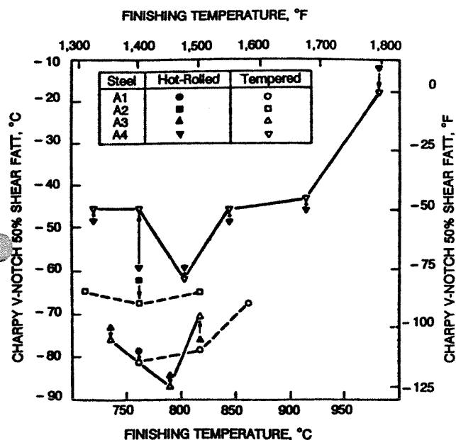
Figure 5.12 How finishing temperature affects the Charpy V-notch 50% shear fracture-appearance-transition temperature (FATT) of steels A1 to A4. 5
