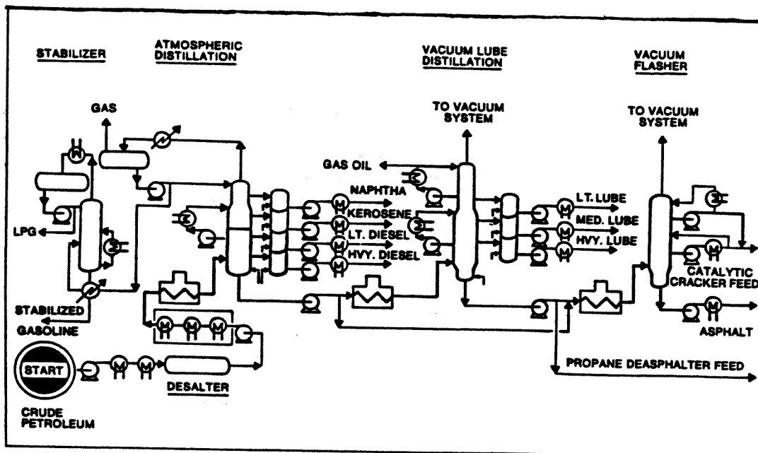
Figure 1.3 Crude distillation, three stages. 1
