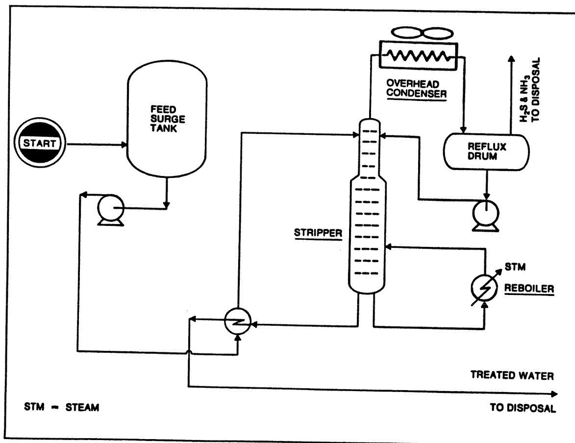
Figure 2.11 Sour water stripper (non-acidified) 1
