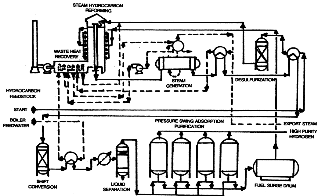
Figure 4.1 Hydrogen 1
