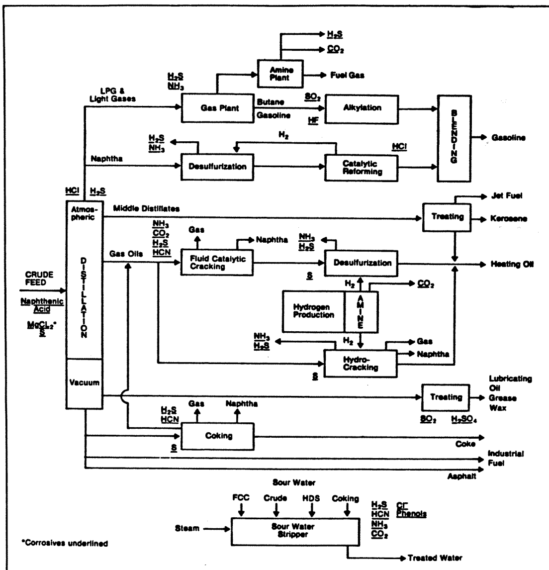
Figure 1.1 Simplified refinery process flow diagram. 1
