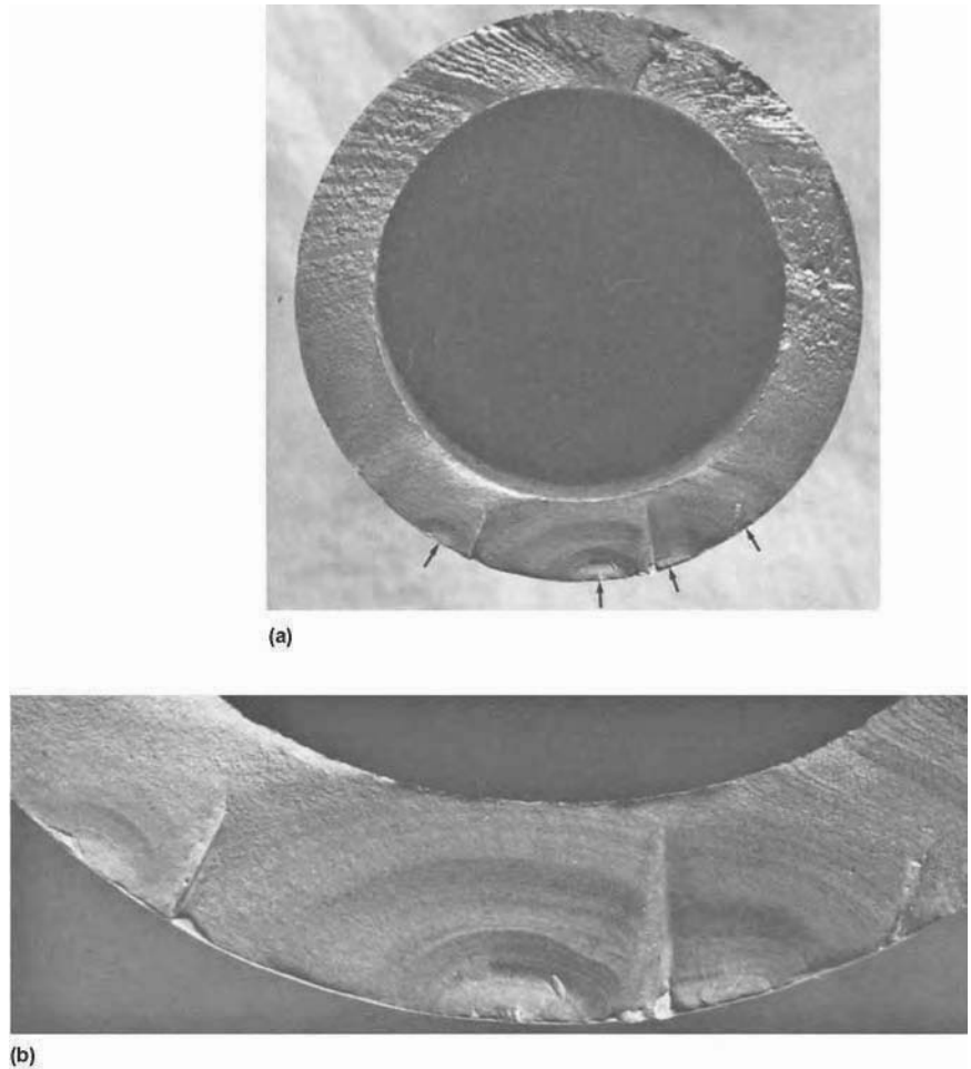
Fig. 25 (a) Fracture surface of a 3.6-in.-diam axle housing tube showing four major fatigue-fracture origins (arrows) at the bottom. (b) Origin areas at higher magnification. Beach marks are clearly seen. Small areas of postfracture damage are present, but in general, the fracture is in excellent condition after careful cleaning. This part was subjected to unidirectional bending stresses normal for the operation. The metal was a medium-carbon steel with a hardness of 217–229 HB. From the origin areas at the bottom, the fatigue cracks progressed up both sides of the tube and joined at the small final rupture area at the top. Note the increasing coarseness of the fracture surfaces as the cracks grew from bottom to top.
