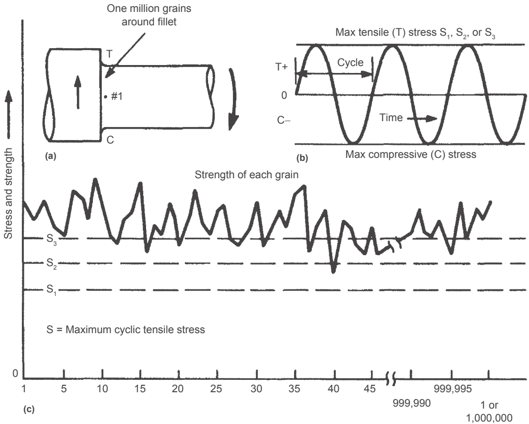
Fig. 16 Schematic sketch of a two-diameter shaft rotating under a bending stress. (a) General shape of a critical stress region in such a part. (b) The stress imposed on each grain, such as grain number 1, as it rotates, with the top of each sine wave representing the maximum tensile stress. (c) Strength of each of a large number of grains in the critical area and three stress levels ( S_1, S_2, \text{ and } S_3 ), which are the maximum cyclic tensile stress to which the grains are subjected. Successively higher stresses automatically cause more fatigue origins to form.
