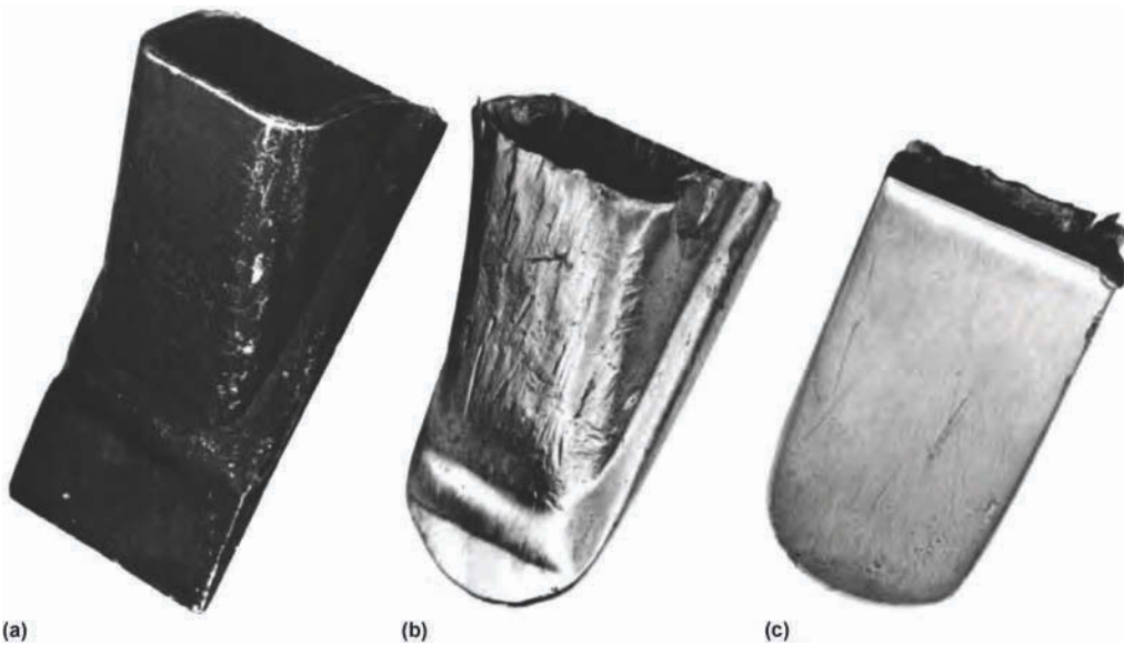
Fig. 8 Tooth for a backhoe bucket: (a) original condition; (b) the soft top of the tooth, made of 1010 steel, wore considerably more during operation in rocky, frozen soil than did (c) the flat opposite side of 8640 medium hard steel. The tooth is a replaceable part that is pinched over a stub to hold it in position.
