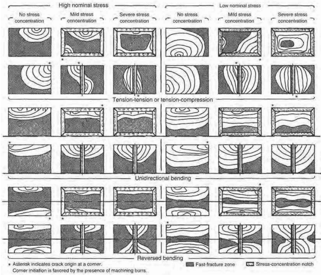
Fig. 23 Schematic representation of fatigue-fracture surface marks produced in components with square and rectangular cross sections and in thick plates under various loading conditions. Note that the final rupture zones (fast-fracture zones) on the left half of the figure, which had a high nominal stress, are considerably larger than the corresponding final rupture zones on the right half, which had low nominal stresses. The individual lines in the sketches represent the general configuration of the progression of the fatigue crack, as recorded by possible submicroscopic striations and macroscopic beach marks. The long dashed lines in reverse and unidirectional bending indicate the bending axes. Note that fatigue origins at corners of rectangular shapes or at ends or drilled holes (asterisks) are quite common in this type of part. Also, multiple fatigue origins are quite common with parts under high nominal stress; ratchet marks perpendicular to the surface separate adjacent fatigue areas. Modified from Ref 4
