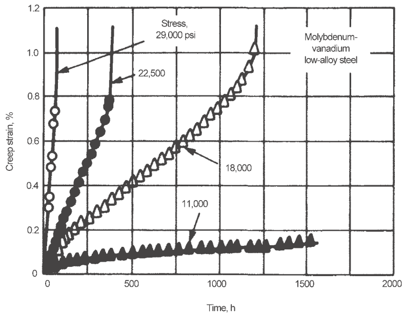
Fig. 2 Creep curves for a molybdenum-vanadium low-alloy steel under tension at four stress levels at 600 °C (1112 °F). Source: Ref 2
