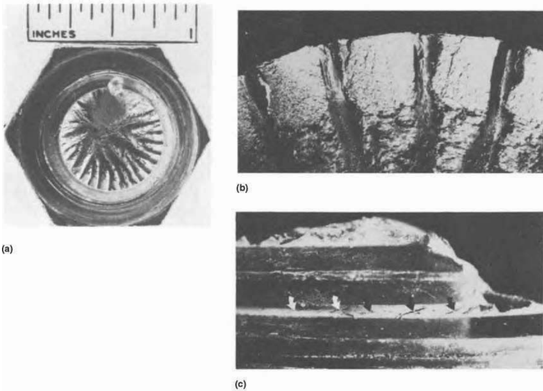
Fig. 13 Multiple-origin fatigue fracture of a short, stubby \frac{5}{8} in. bolt that fractured under tensile fatigue. (a) Numerous fatigue origins separated by radial ratchet marks. (b) Close-up of several fatigue origins separated by ratchet marks. Because this bolt was in a continuously operated test machine, there is no evidence of beach marks on the fatigue areas. These areas are at a slight angle to the axis of the bolt, as seen in (c). (c) Fatigue cracks in the root of the thread (arrows) that have not yet grown large enough to come close to the neighboring cracks to form ratchet marks between them. Note the slight angle of fatigue cracks that form a ratchet-like appearance upon fracture.
