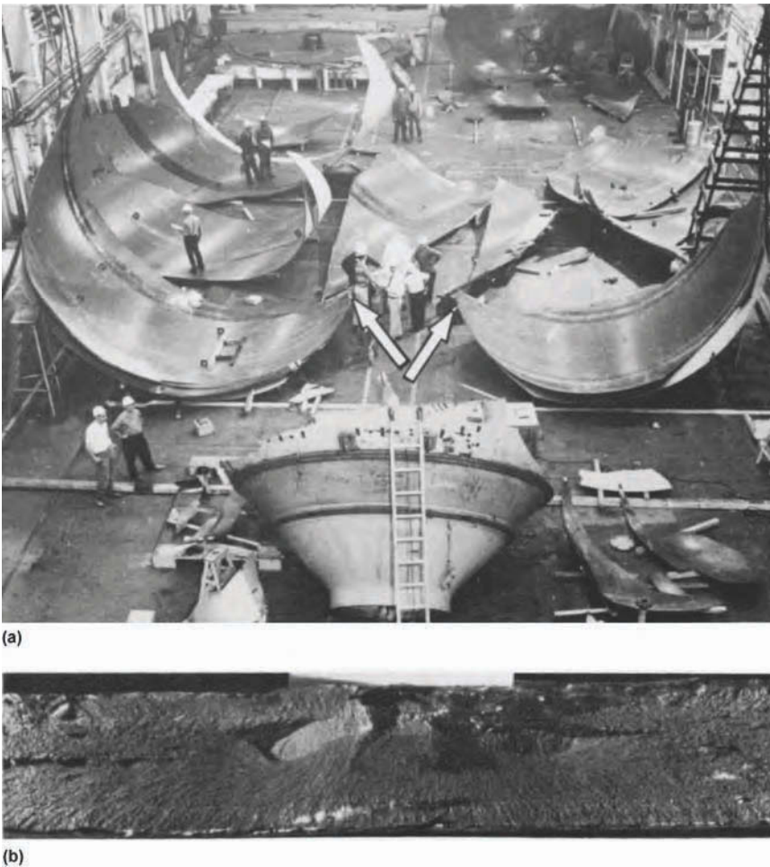
Fig. 8 (a) Catastrophic brittle fracture of a 260 in. diam solid-propellant rocket motor case made of 18% Ni, grade 250, maraging steel. The case fractured at a repaired weld imperfection during a hydrostatic pressure test. Fracture occurred at about 57% of the intended proof stress. All welds of the case had been carefully inspected by x-ray and ultrasonic inspection. Arrows indicate the origin of fracture. (b) Light fractograph of the crack origin, at 1\frac{1}{3}\times . A crack was found beneath a gas tungsten-arc repair weld on the inner surface of the case (at the top in this fractograph) in the heat-affected zone of a longitudinal submerged-arc assembly weld. The crack was about 1.4 in. long, parallel to and 0.47 in. beneath the outer surface of the case (at the bottom). Radial marks are visible that confirm that fracture proceeded to the left and to the right. Source: Ref 8
