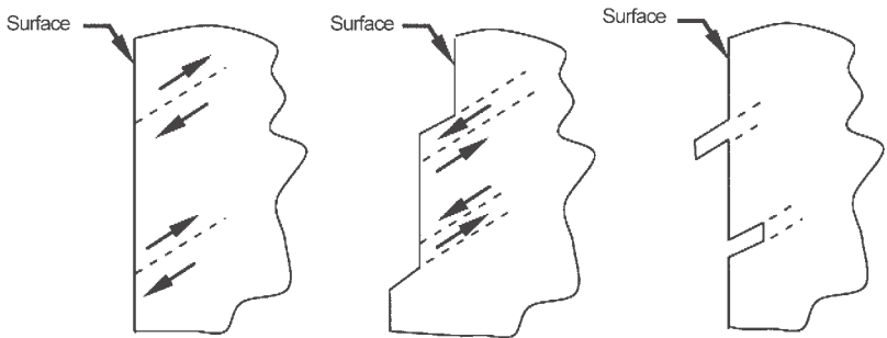
Fig. 2 Schematic illustration of the formation of extrusions and extrusions in stage 1 fatigue. Source: Ref 2
