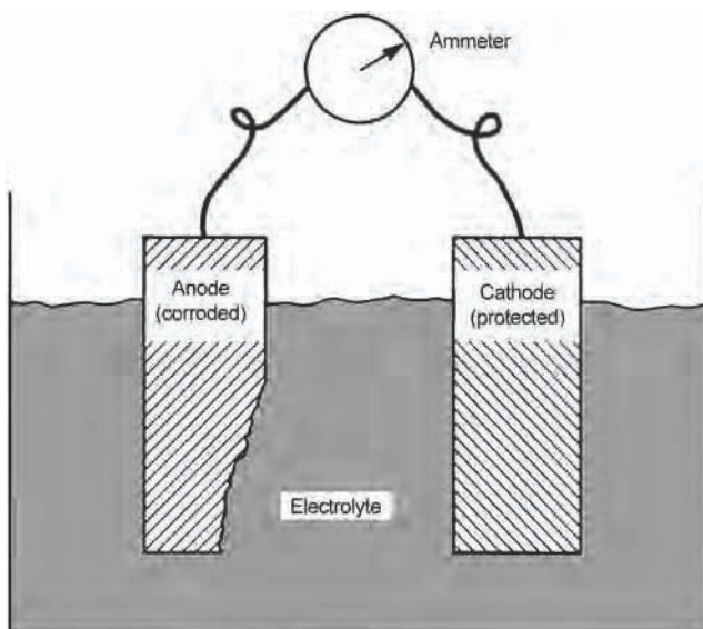
Fig. 2 Galvanic cell showing the basic principles of the electrochemical nature of corrosion
