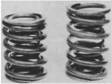
Fig. 1 Distorted engine valve spring (left) compared with normal valve spring. Improper microstructure resulted in inadequate strength and hardness at the operating temperature. Source: Ref 1, 2
