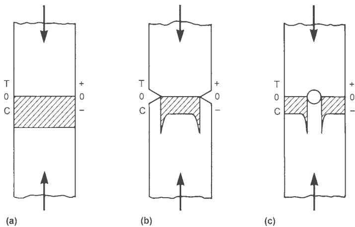
Fig. 3 Elastic stress distribution: pure compression. T, tension. C, compression. (a) No stress concentration. (b) Surface stress concentrations. (c) Transverse hole stress concentration
