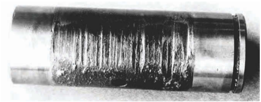
Fig. 11 Severe adhesive wear on a stationary shaft upon which a planetary gear rotated in the presence of inadequate lubricant. Because the radial force was on only one side of the shaft, the adhesive wear was on only one side. However, the entire bore of the gear was damaged by adhesive wear. Both parts were carburized and hardened steel.
