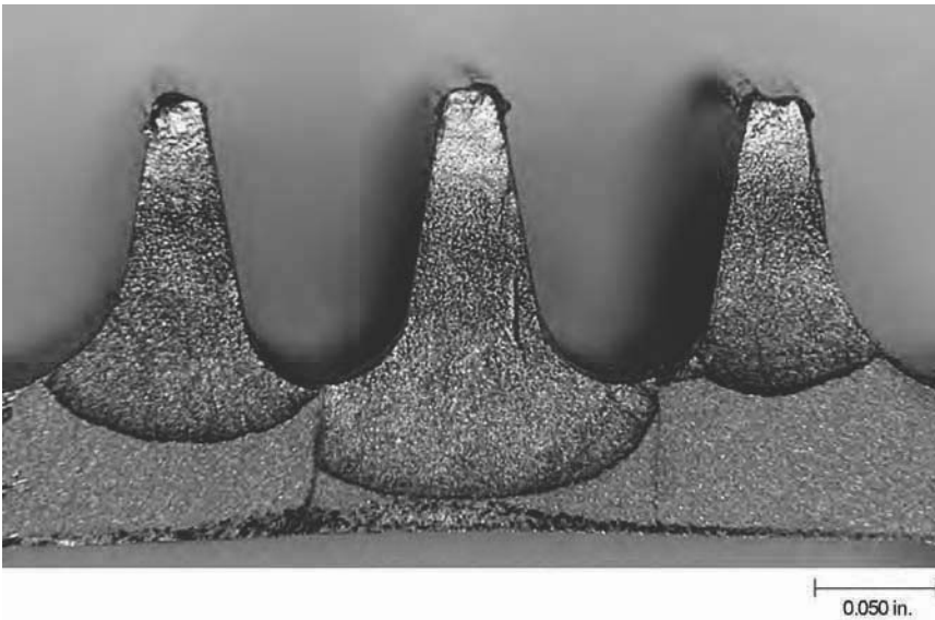
Fig. 11 Fatigue-tested titanium component with cracks initiating in each of three knife seals. The oxide colors reflect the oxide thickness, which would be thicker close to the origin areas.
