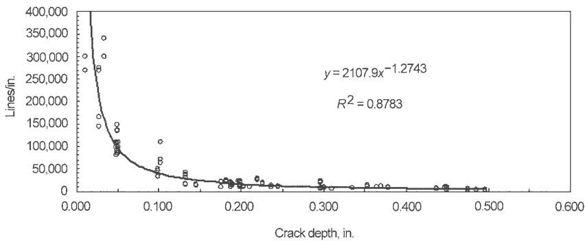
Fig. 15 Plot of fatigue striations as a function of depth, showing the expected increasing crack growth rate with increasing depth.
