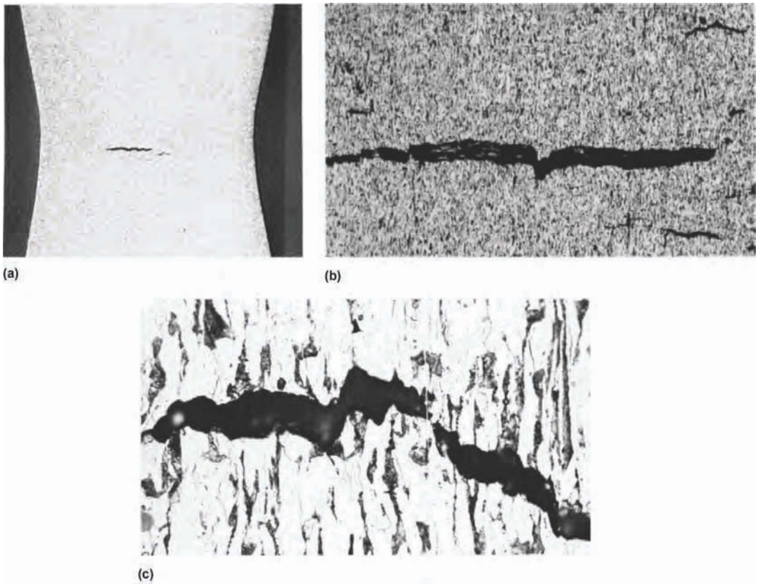
Fig. 5 Photographs at three different magnifications (shown here at 75%) of longitudinal section of tensile test specimen of hot-rolled 1020 steel. The test was stopped immediately prior to fracture (region (c) of Fig. 4). (a) At 6 \times magnification, internal cracking, reduced section, and severely deformed grain structure can be seen. (b) At 50 \times magnification, one large crack and several smaller cracks and elongated grains are apparent. (c) At 250 \times magnification, lack of fit due to distortion is clear, as well as elongated ferrite (light) and pearlite (dark) areas. Specimens were prepared with 2% Nital etching.
