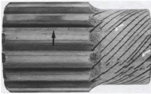
Fig. 7 Torsional fracture of a 1½-inch-diameter case-hardened steel shaft, illustrating cracking of the hard, brittle case and transverse shear fracture at the right end across the relatively soft, ductile core. Hot etched to reveal twisting and distortion of the originally straight grain flow in the cylindrical shaft (white arrows). Note that the black 45° brittle-fracture cracks (emphasized by the hot etching) are in the opposite direction to the twisting. This is because the cracks are always perpendicular to the tensile stress component that caused them, whereas the grain-flow distortion tends to proceed in the same direction as the tensile component. The black arrow on the spline indicates the direction this end was twisted.
