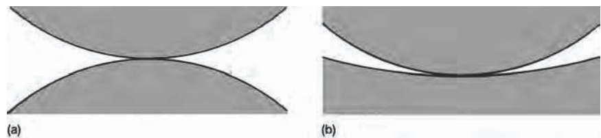
Fig. 1 (a) Sketch of counterformal, or convex, surfaces in contact; examples are gear teeth and roller or needle bearings rolling on a shaft, in an inner raceway, or on a flat surface. (b) Sketch of conformal surfaces, where a convex surface is in contact with a concave surface; examples are ball bearings in contact with an inner or outer raceway, roller or needle bearings in contact with an outer raceway, and a shaft in contact with a sliding bearing or on a flat surface.
