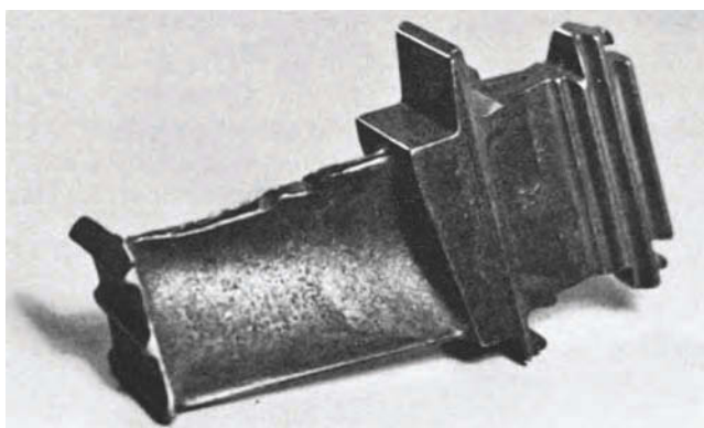
Fig. 11 High-temperature erosion-corrosion in a turboprop engine blade. Most of the 1-1/3-in.-long blade had been damaged by sulfidation, or hot corrosion caused by excessive sulfur in the fuel. This uncoated INCO 713 turbine blade was one of many such rotary blades subjected to this type of high-temperature erosion-corrosion. Nickel aluminide coatings are sometimes applied to the nickel-base alloy to improve the life of the blades.
