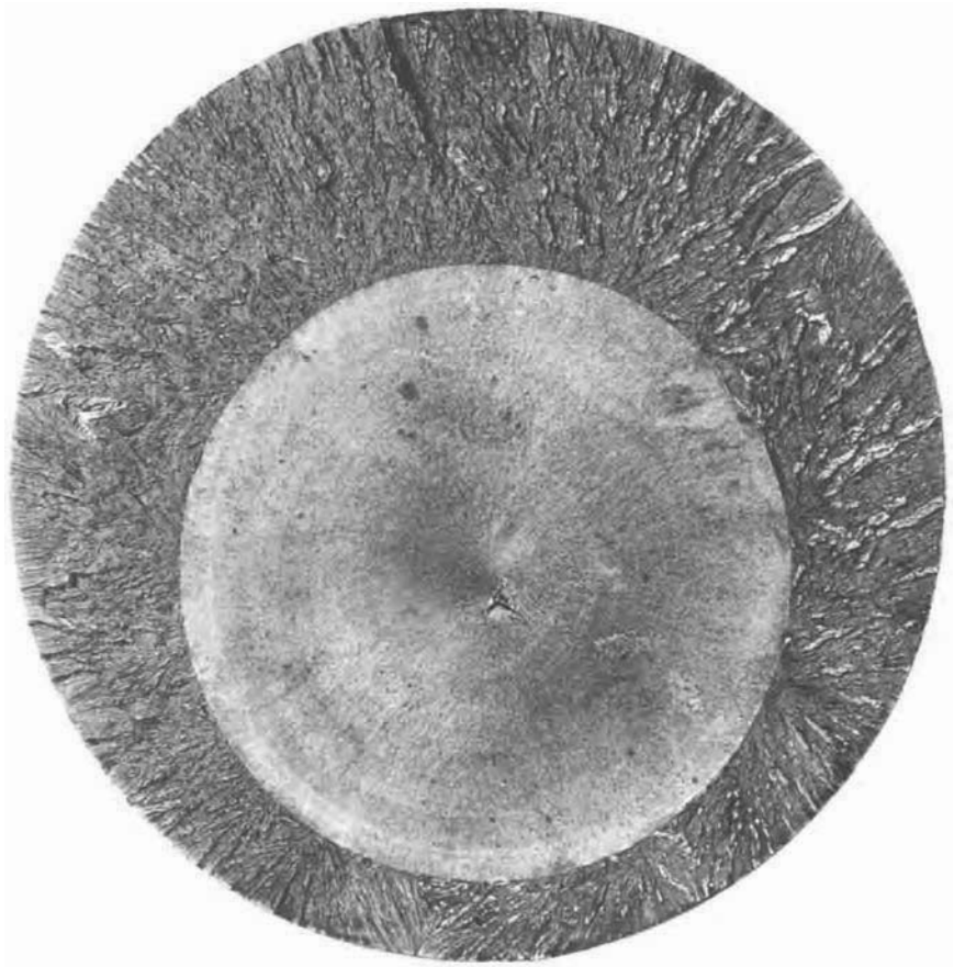
Fig. 33 Tensile fatigue fracture starting near the center of an 8-in.-diam piston rod of a forging hammer, made of low-carbon alloy steel hardened to 24 HRC at the surface and 17 HRC at the center. In an axially loaded part such as this, fatigue fracture can start anywhere in the cross section. In this case, a forging “flake” caused fatigue to start near the center of the section and to grow outward in a circular fashion until it was about 5.2 in. in diameter, at which time final rupture occurred in one load application. At no time did the fatigue crack reach the surface of the large shaft. Use of a vacuum-degassed steel would have prevented the flake that caused this type of fatigue failure, which occurred many years ago.
