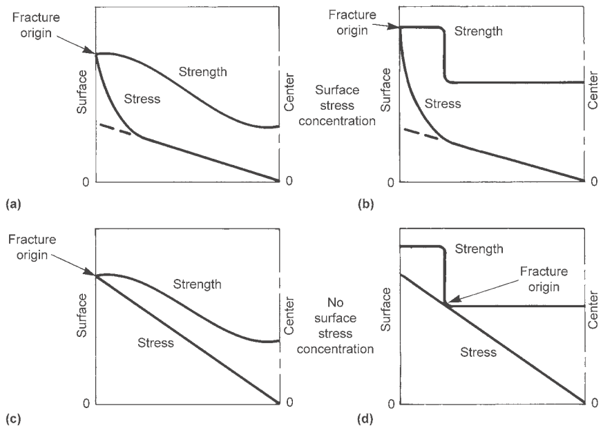
Fig. 9 Surface and subsurface fracture origins. Strength gradients: (a) and (c), gradual; (b) and (d), steep. Stress gradients: (a) and (b), surface stress concentrations; (c) and (d), no stress concentrations
