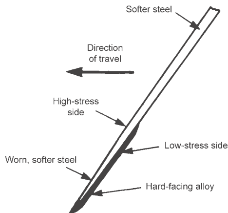
Fig. 6 Diagram of self-sharpening plowshare using the same principle as shown in Fig. 5. As the plowshare cuts through the soil from the right to the left, the relatively soft steel on the forward, high-stress side is gradually worn away, but the hardfacing applied to the rear, low-stress side is continually exposed at the sharp tip. Eventually, of course, the part must be replaced, but service life may be very long in certain types of soil, particularly those without rocks.
