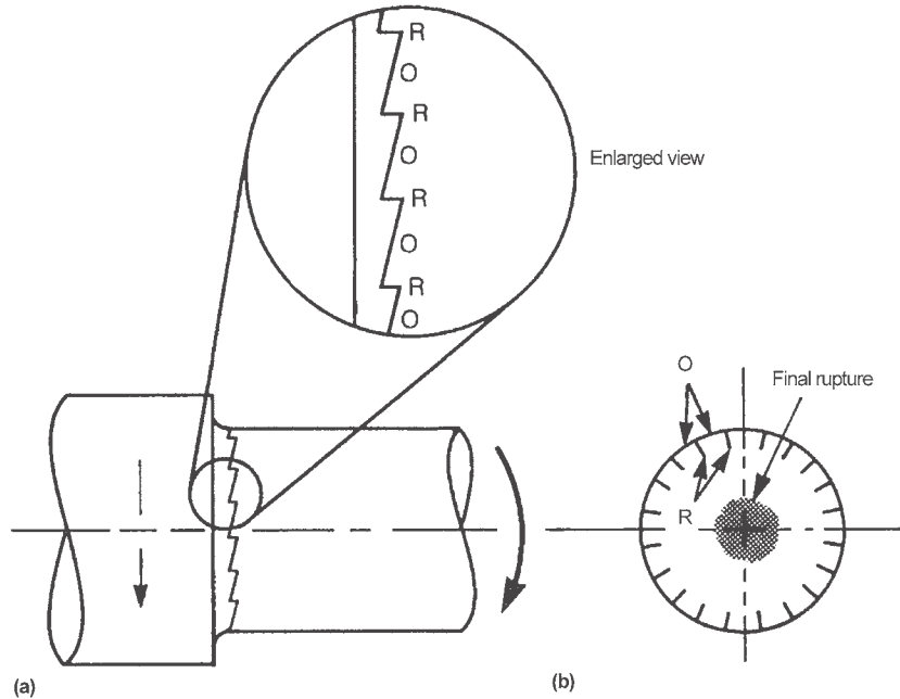
Fig. 12 (a) Formation of ratchet marks in the fillet of stepped shaft under uniform rotating-bending load. (b) Schematic view of fracture surface showing ratchet marks near periphery and central final rupture (stage 3). O: origins of fatigue fractures; R: ratchet marks between fatigue origins.
