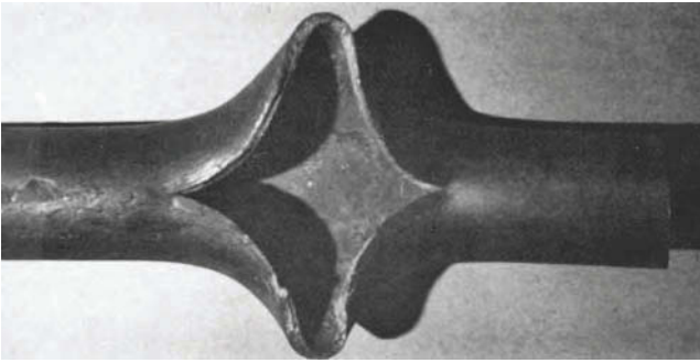
Fig. 6 Thick-lip “fishmouth” failure of a 2-in.-diam superheater tube. The tube bent away from the fracture due to the reaction force of the escaping steam. The material was ASME SA-213 T22 (0.15 maximum C, 1.90–2.60 Cr, 0.87–1.13 Mo). Hardness was 96–98 HRB. Scale about 0.012 in. thick is present on the inside, tending to prevent heat transfer and causing overheating to about 1525–1575 °F.
