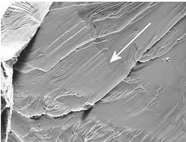
Fig. 13 Cleavage fracture in hardened steel showing numerous "river" marks. The overall direction of crack propagation is in the direction of the arrow (i.e., downstream). New river patterns are created where grain boundaries were crossed. 125 \times .
