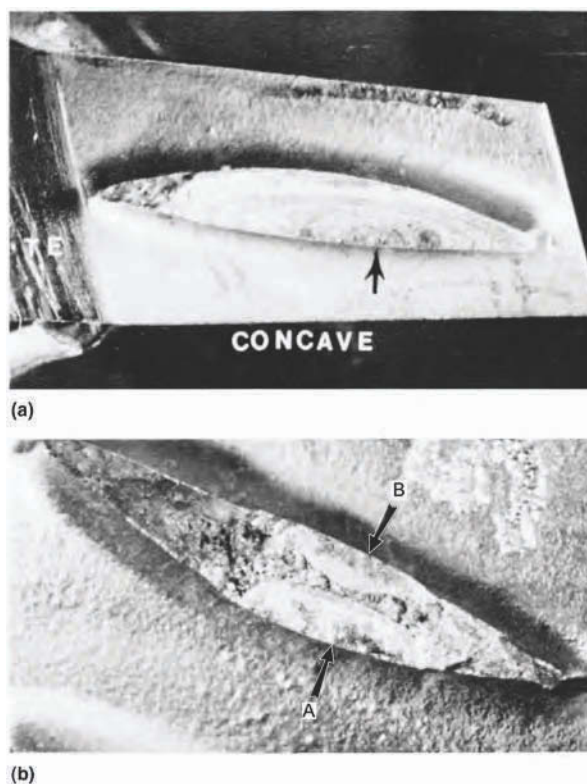
Fig. 11 First-stage compressor blades that fractured due to corrosion fatigue originating in corrosion pits like those shown in Fig. 10. Note that (a) had one fatigue origin (arrow) on the mid-pressure side (5 \times ; shown at 70%). Arrows in (b) show fatigue origins on both the suction (A) and the pressure (B) sides (6.5 \times ; shown at 70%). These fatigue fractures in cast 17-4PH material are ambient-temperature fractures. Pitting was caused by seawater corrosion.
