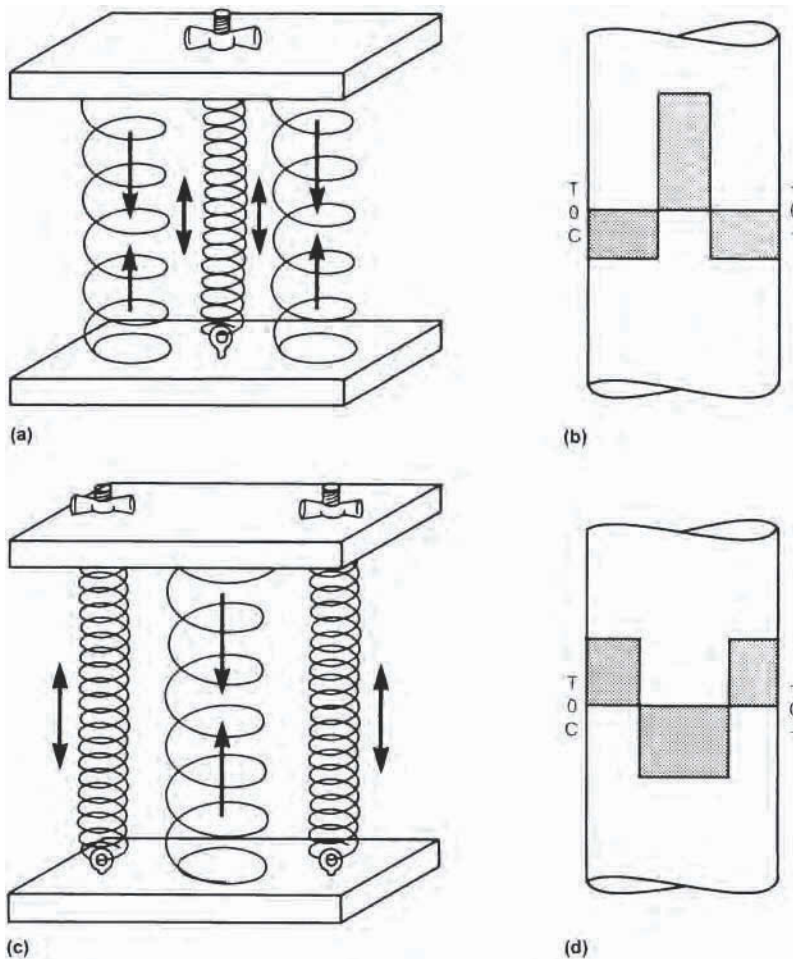
Fig. 8 Residual stress systems illustrated by spring analogy, (a) compressive stresses outside, tensile stress inside; (c) tensile stresses outside, compressive stress inside; (b) and (d) diagrams of corresponding residual stress systems. T, tension. C, compression.
