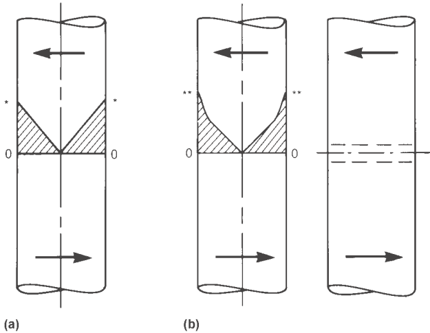
Fig. 2 Elastic stress distribution: pure torsion. (a) No stress concentration. *All stress components—tension, shear, and compression—have equal magnitude. (b) Transverse hole stress concentration. **Tension and compression stress components increase more than shear stress at a torsional stress concentration at the corner of the transverse hole.
