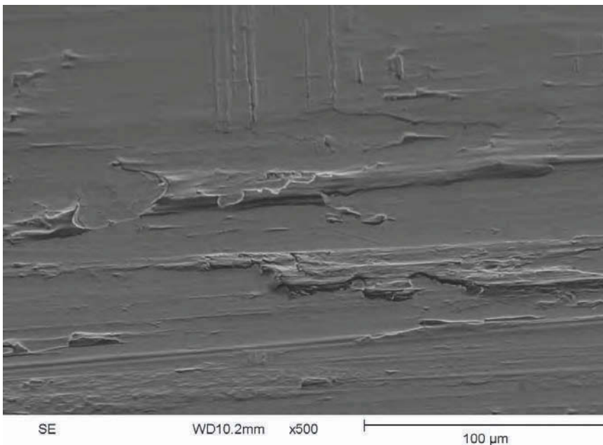
Fig. 10 Scanning electron microscope image of a microscopic region of adhesive wear on a hardened-alloy-steel piston component from a hydrostatic pump (500 \times ). Material has been transferred by microwelding from the adjacent component wall surface during sliding and poor lubrication conditions.
