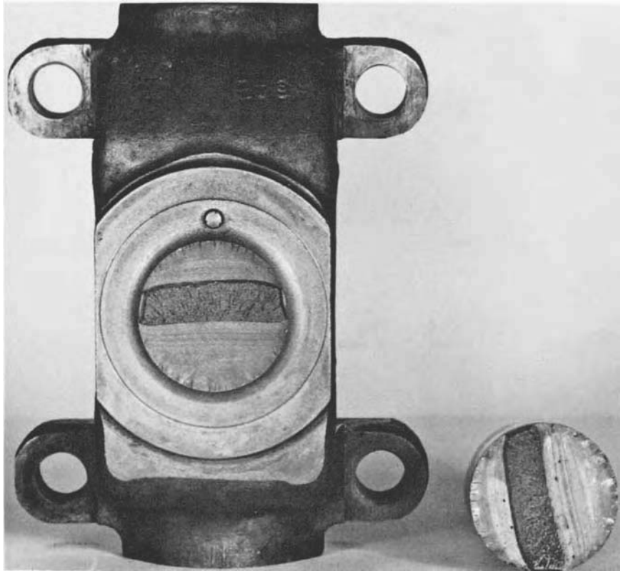
Fig. 27 Reversed bending fatigue of an alloy-steel steering knuckle at a hardness level of 30 HRC with nonuniform application of stresses. The multiple-origin fatigue at the bottom was caused by the tendency of normal wheel loading to bend the spindle (lower right) of the knuckle upward. The fatigue on the upper side (smaller area) of the fracture was caused by turning maneuvers in which the wheel acts as a lever to bend the spindle downward. Note the many radial ratchet marks on the fatigue surfaces. The part had been overloaded during service.
