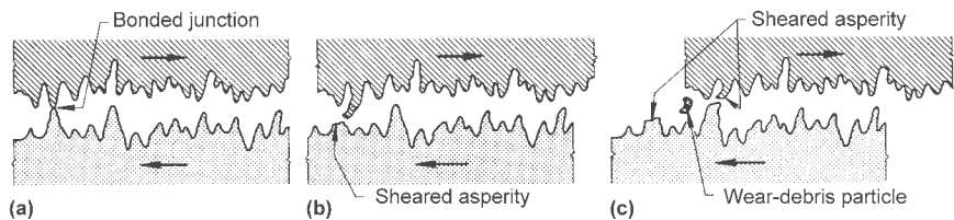
Fig. 9 Schematic illustration of one process by which a particle of wear debris is detached during adhesive wear. As the surfaces slide across each other, (a) a bonded junction is (b) torn from one peak, or asperity, and then is (c) sheared off by impact with a larger, adjacent peak to form a particle of wear debris. The peaks are greatly exaggerated in this sketch, but the principle is accurate; metal also may be transferred from one surface to another by the microwelding process. Arrows indicate direction of sliding. Source: Ref 1
