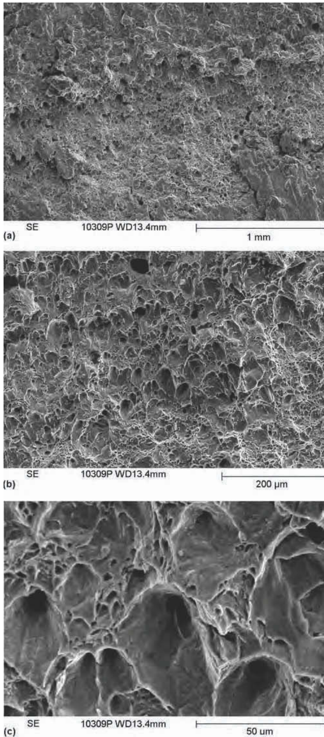
Fig. 9 Scanning electron images of a ductile fracture: (a) relatively equiaxed dimples at the center portion of the image, with some postfracture mechanical rubbing damage at the bottom portion of the image (50 \times ); (b) elongated dimples indicating ductile rupture with a shear component are shown at the center portion of the image (200 \times ). (c) The elongated dimples shown at the center portion of (b) are presented at higher magnification (1000 \times ). Finer dimples are present along the ridges between the larger dimples.
