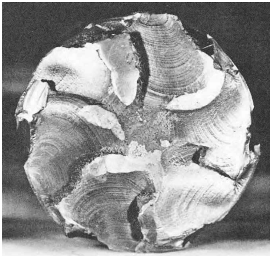
Fig. 31 Rotating bending fatigue fracture in a grade 4817 steel shaft, carburized and hardened to a surface hardness of 60 HRC. The fracture started in six fillet areas around the periphery, near the runouts of six grooves. The six fatigue areas penetrated separately, but uniformly, to final rupture at the center. The bright, shiny, flat areas are regions of postfracture rubbing against the opposite surface. Grinding damage in the fillet was the cause of this fracture.
