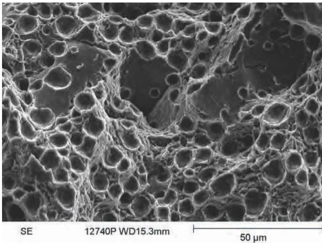
Fig. 10 A scanning electron micrograph of a mixed fracture mode from a metal injection molded (MIM) steel. The dimples indicate ductile rupture. The flat features indicate separation of nonfused particles. The circular features on the flat fractures are porosity.
