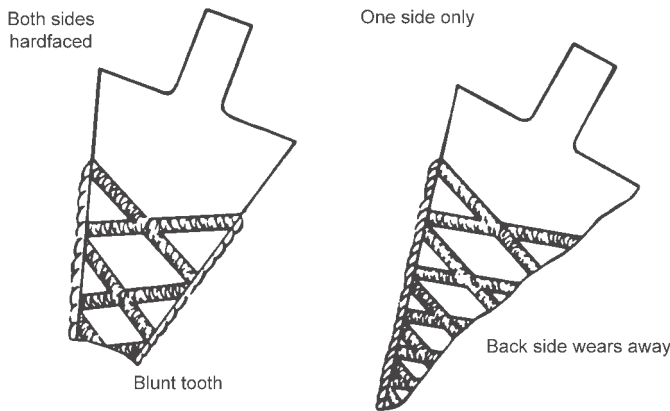
Fig. 7 Self-sharpening of a digging tooth from ground-contact equipment by controlled wear through selective hardfacing. The pattern of hardfacing can be varied to suit the condition, but note that the blunt tooth is hardened on both sides, while the self-sharpening tooth is hardened on only one side. Source: Ref 5
