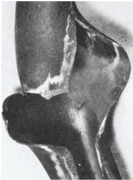
Fig. 7 Thin-lip rupture in a boiler tube caused by rapid overheating. This rupture exhibits a “cobra” appearance as a result of lateral bending under the reaction force imposed by escaping steam. The tube was a 2-½ in. outside diameter, 0.250 in. wall boiler tube made of 1.25Cr-0.5Mo steel (ASME SA-213). Source: Ref 2
