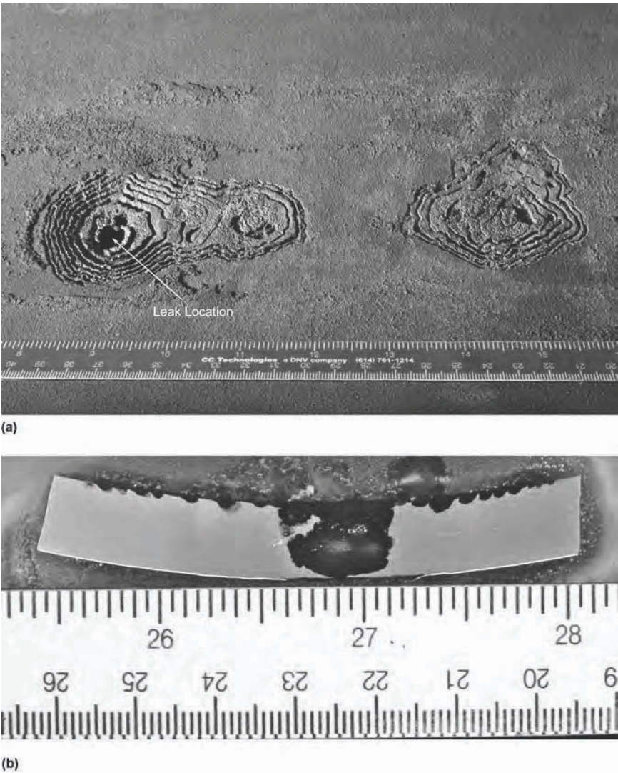
Fig. 5 (a) Inner surface of a 12-in.-diameter crude oil pipeline that experienced an in-service leak. (b) Metallographic cross section of the leak location showing undercutting within the pit, a pitting morphology that is typically associated with MIC.
