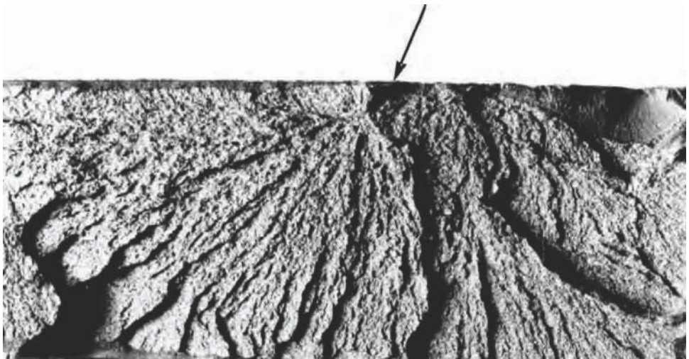
Fig. 10 Origin (at arrow) of a single-load brittle fracture that initiated at a small weld defect. Note also a fatigue fracture in the upper right corner. Radial ridges emanate from the origin in a fan-shaped pattern. The brittle part of the fracture is bright and sparkling, in contrast to the dull appearance of the fatigue zone and the thin shear lips at the top and bottom surfaces.
