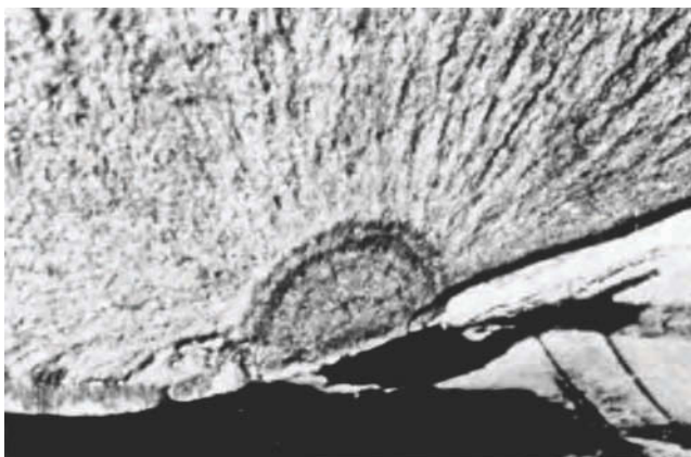
Fig. 7 Stress-corrosion crack in a high-strength steel part (4×). The fracture surface appears to have the characteristic beach mark pattern of a fatigue fracture. However, this was a stress-corrosion fracture in which the pattern was caused by differences in the rate of corrosion penetration. Final fracture was brittle. Source: Ref 9
