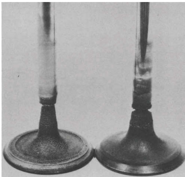
Fig. 10 Severe localized erosion-corrosion of two gasoline-fueled engine exhaust valves made from a nickel-base superalloy operating between 1400 and 1500 °F. The exhaust gas damage in the underhead radius and stem was identified as lead oxide corrosion, aggravated by bromine from the gasoline.
