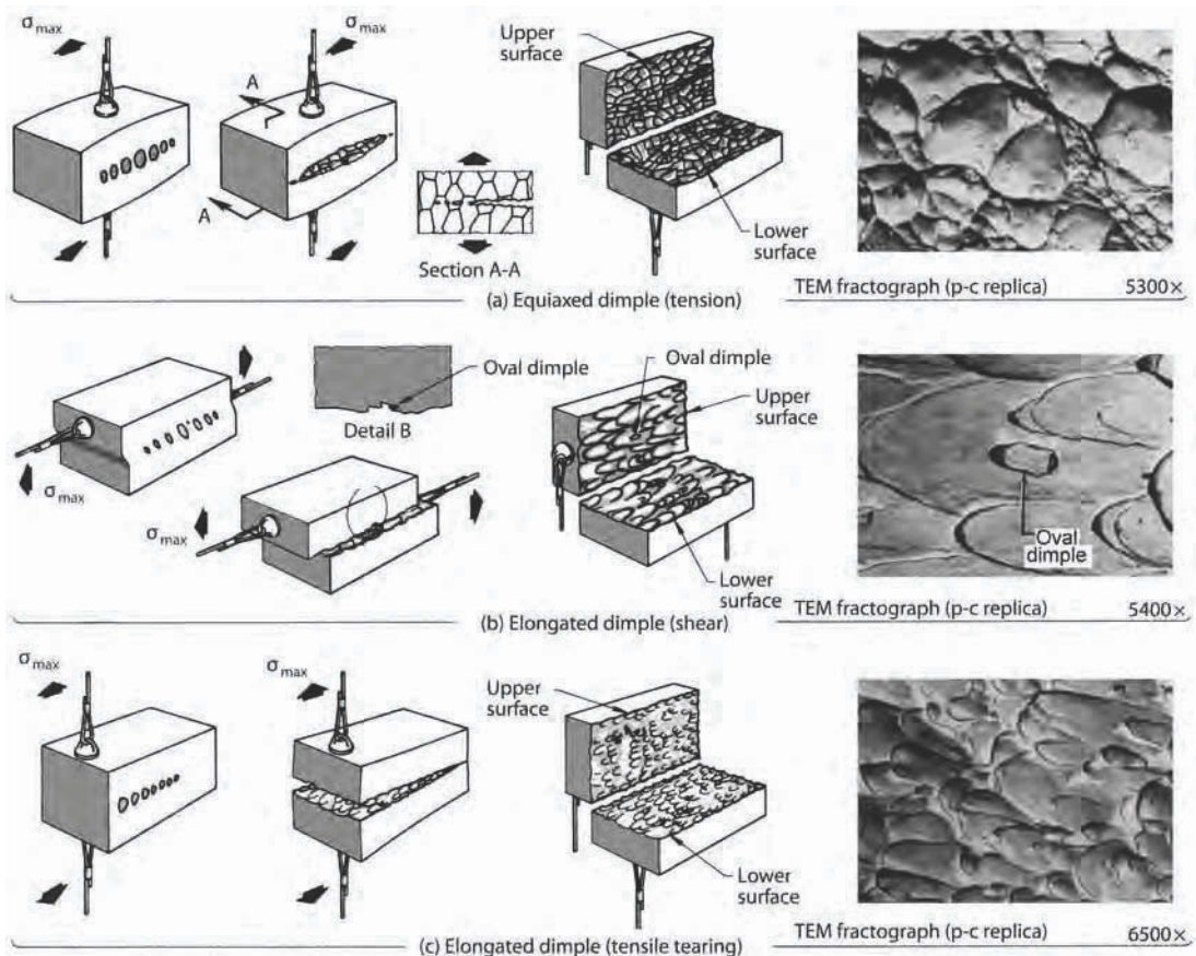
Fig. 7 The influence of the direction of principal normal stress on the shape of dimples formed by microvoid coalescence. Transmission electron microscopic (TEM) fractographs are phase-contrast (p-c) replicas of fracture areas. Source: Ref 2
