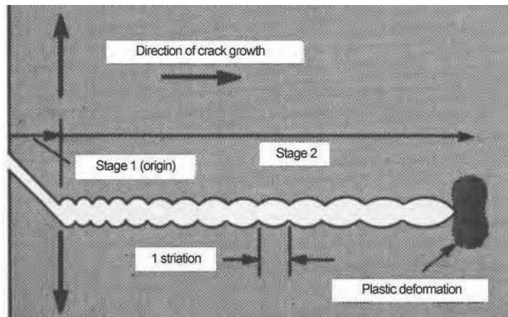
Fig. 4 Highly enlarged schematic cross-sectional sketch of stage 1 and stage 2 fatigue. The edge of the metal is at left. When tensile forces repeatedly act on the surface, the microstructural changes of stage 1 cause a submicroscopic crack to form. With each repetitive opening, the crack jumps a small distance (one striation). Note that the spacing of each striation increases with the distance from the origin, assuming the same opening stress. The metal at the tip of the fatigue crack (right) is plastically deformed on a submicroscopic scale.
