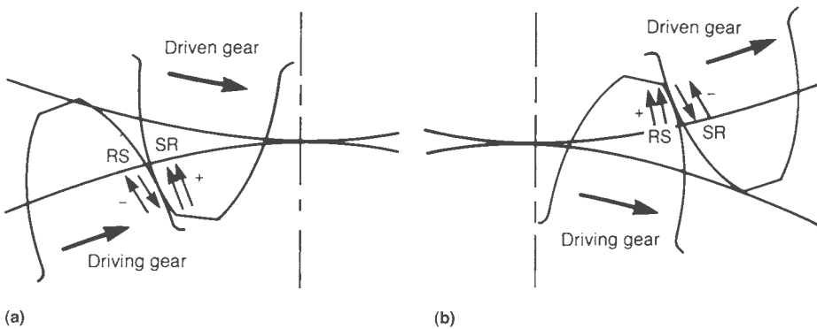
Fig. 8 Schematic of rolling-sliding action inherent in gear teeth: (a) beginning of contact, (b) end of contact. As gear teeth contact, rolling (R) and sliding (S) stresses are formed by the relative movement. Pure rolling occurs only at the pitch line, and on each gear the direction of sliding reverses at the pitch line. Analysis of the relative motions of gears reveals that on both the driving and driven gears there is negative sliding below the pitch line and positive sliding above the pitch line. Since negative sliding is more likely to cause surface-origin pitting, damage is most likely to occur below the pitch line on the smaller gear, which is usually the driving gear.
