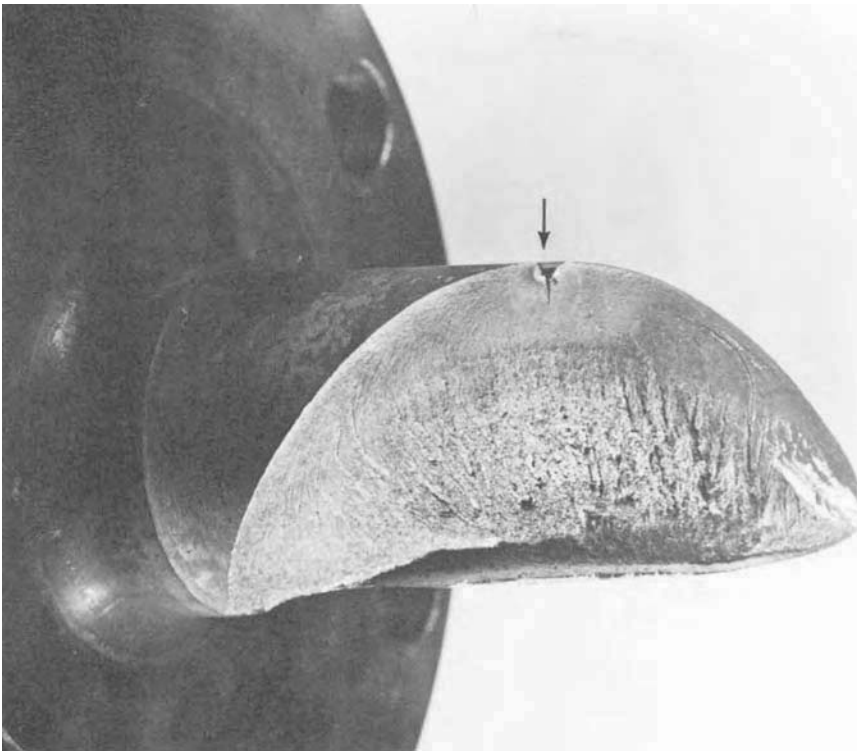
Fig. 34 Torsional fatigue fracture of a 1050 steel axle shaft induction-hardened to about 50 HRC. The arrow indicates the longitudinal shear fatigue origin, which then changed direction and grew to the small circular beach mark, or "halo." Final brittle fracture (note chevron marks in the case) caused complete separation with the characteristic 45^\circ brittle fracture in torsion.
