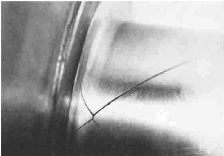
Fig. 36 Characteristic X-shaped crack pattern in a grade 1045 steel crankshaft after testing in reversed torsional fatigue in a special machine, not in an engine. In this case, the original crack was in the transverse shear plane, not in the longitudinal shear plane as in Fig. 35.
