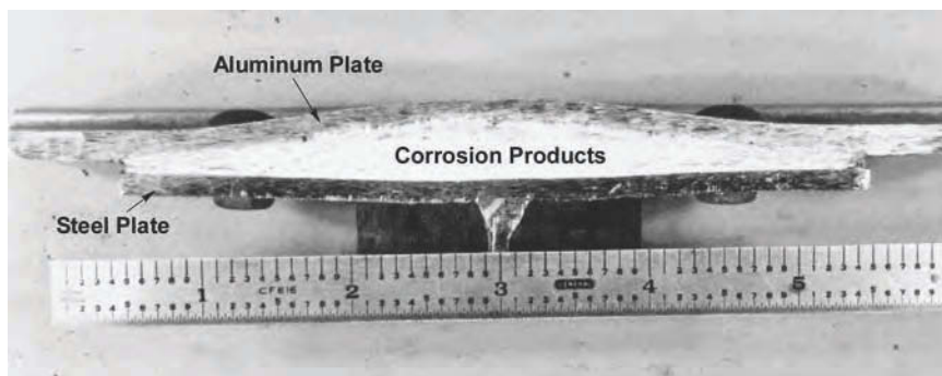
Fig. 4 An aluminum plate riveted to a steel plate resulted in a galvanic couple and crevice corrosion that produced a significant amount of corrosion products between the two plates. The stresses generated as a result of the volume change of the corrosion products were sufficient to plastically deform the aluminum plate.
