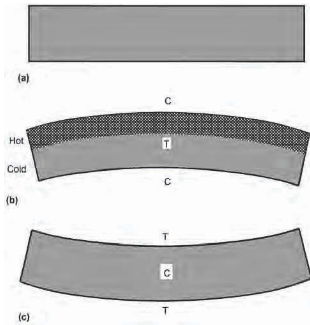
Fig. 3 Deformation caused by thermal residual stresses. (a) Flat, platelike metal at uniform temperature. (b) Lateral expansion of upper part on heating is restrained by cold, strong metal below, causing compressive stress (C) on upper (convex) and lower (concave) surfaces and tensile stress (T) in the interior. (c) Reversal of stresses on cooling.
