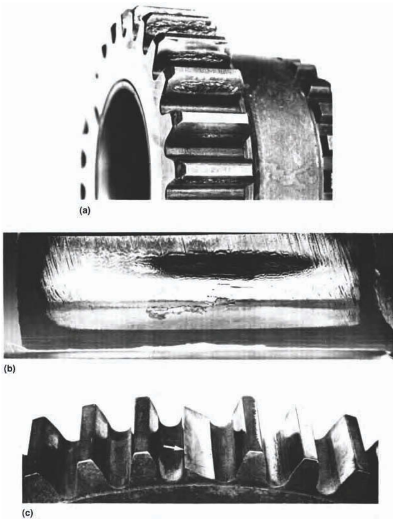
Fig. 9 Surface-origin pitting fatigue. (a) Typical surface deterioration due to pitting fatigue on gear teeth. In a standard gear system, the pitch line is near the center of the height of the teeth. Pitting fatigue usually starts slightly below the pitch line and then rapidly spreads to adjacent areas, causing complete surface deterioration. This heavily loaded gear was made of case-hardened alloy steel, with a surface hardness near 60 HRC. (b) Heavily loaded final drive pinion with surface pitting near the pitch line, which was low on this gear tooth. The rippling shown is plastic deformation caused by the sliding action under heavy contact pressure and is a warning that the metal is close to failure. The parallel diagonal marks are tool marks resulting from the shaving operation and are not involved with the service in any way. (c) Fracture of gear tooth at pitch line. Another consequence of pitting fatigue on the active profile of gear teeth is the fact that the pit itself is a stress concentration that can cause abnormal bending fatigue fracture of gear teeth, which are really carefully shaped cantilever beams. This gear tooth pitted just below the pitch line and then fractured as a result of bending fatigue. The normal location for bending fatigue fractures of gear teeth is at the root fillet, not midway up the tooth, as in this example. This gear was made from a medium-carbon steel, induction hardened to about 55 HRC.
