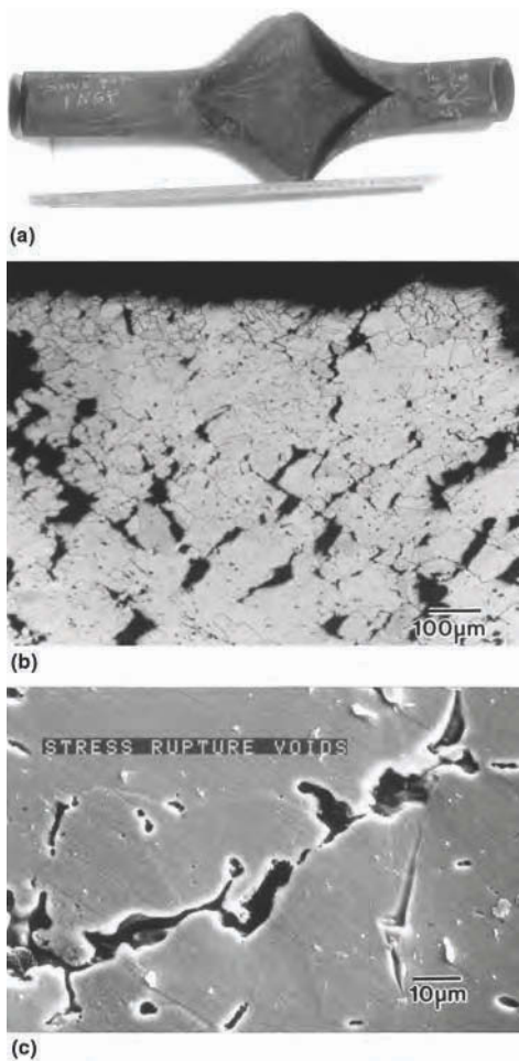
Fig. 5 Stress rupture of heater tube: (a) heater tube that failed due to stress rupture; (b) and (c) stress rupture voids near the fracture. Source: Ref 3
