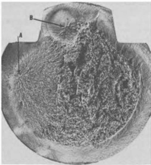
Fig. 19 Subsurface-origin fatigue fracture in an induction-hardened 3/4 in.-diam 1541 steel axle that was continuously tested in rotating bending fatigue in the laboratory. The primary fatigue fracture originated at A, while a smaller crack was progressing at B. Note that no beach marks are visible because of the continuous testing and that both origins are near the inner edge of the induction-hardened zone. The larger fatigue crack (from A) was in the left third of the fracture before it triggered a brittle fracture in the case (notice the chevron marks at lower right) and ductile fracture in the core. Source: Ref 4
