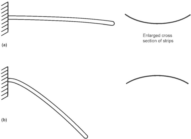
Fig. 4 Curved strip of thin spring steel, such as a tape measure or Venetian blind slat, supported horizontally as a cantilever beam (a) stable with concave side on top; (b) unstable with convex side on top, buckles readily.
