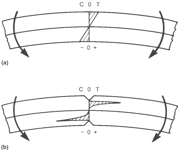
Fig. 4 Elastic stress distribution: pure bending. T, tension. C, compression. (a) No stress concentration. (b) Transverse surface stress concentrations
