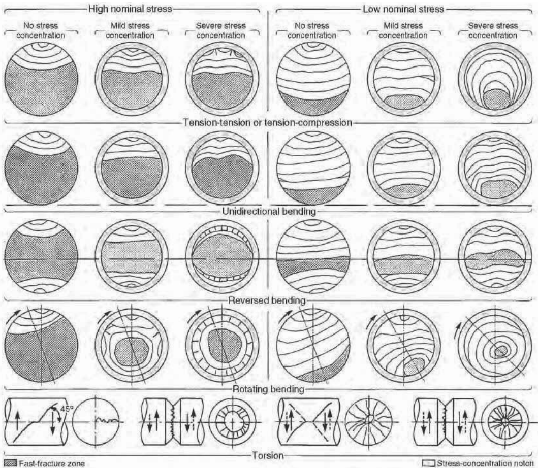
Fig. 22 Schematic representation of fatigue-fracture surface marks produced in smooth and notched cylindrical components under various loading conditions. Note that the final rupture zones (fast-fracture zones) on the left half of the figure, which had a high nominal stress, are considerably larger than the corresponding final rupture zones on the right half, which had low nominal stresses. The individual lines in the sketches represent the general configuration of the progression of the fatigue crack, as recorded by possible submicroscopic striations and macroscopic beach marks. The long horizontal dashed lines in reverse and unidirectional bending indicate the bending axes. Also note the radial ratchet marks between origins of the high nominal stress fractures. In the torsional fatigue fractures (bottom row), note that unidirectional fatigue (left) is at an approximate 45^\circ angle to the shaft axis, while reversed torsional fatigue of a cylindrical shaft (second from right) has an X-shaped pattern with the origin in either the longitudinal or the transverse direction. Torsional fatigue cracks in stress concentrations tend to be very rough and jagged because of many 45^\circ cracks. Modified from Ref 4
