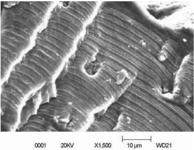
Fig. 7 Striations generated on a spectrum-loaded test article. Source: Ref 2
