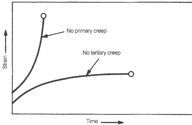
Fig. 3 Creep curves showing no primary creep and no tertiary creep. Source: Ref 2
