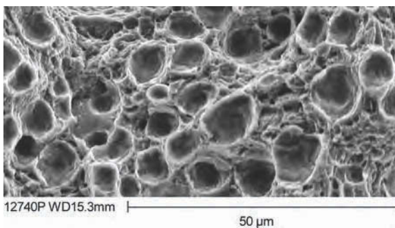
Fig. 6 Typical dimpled-rupture fracture surface of a ductile metal viewed with a scanning electron microscope at a magnification of 1000 \times .
