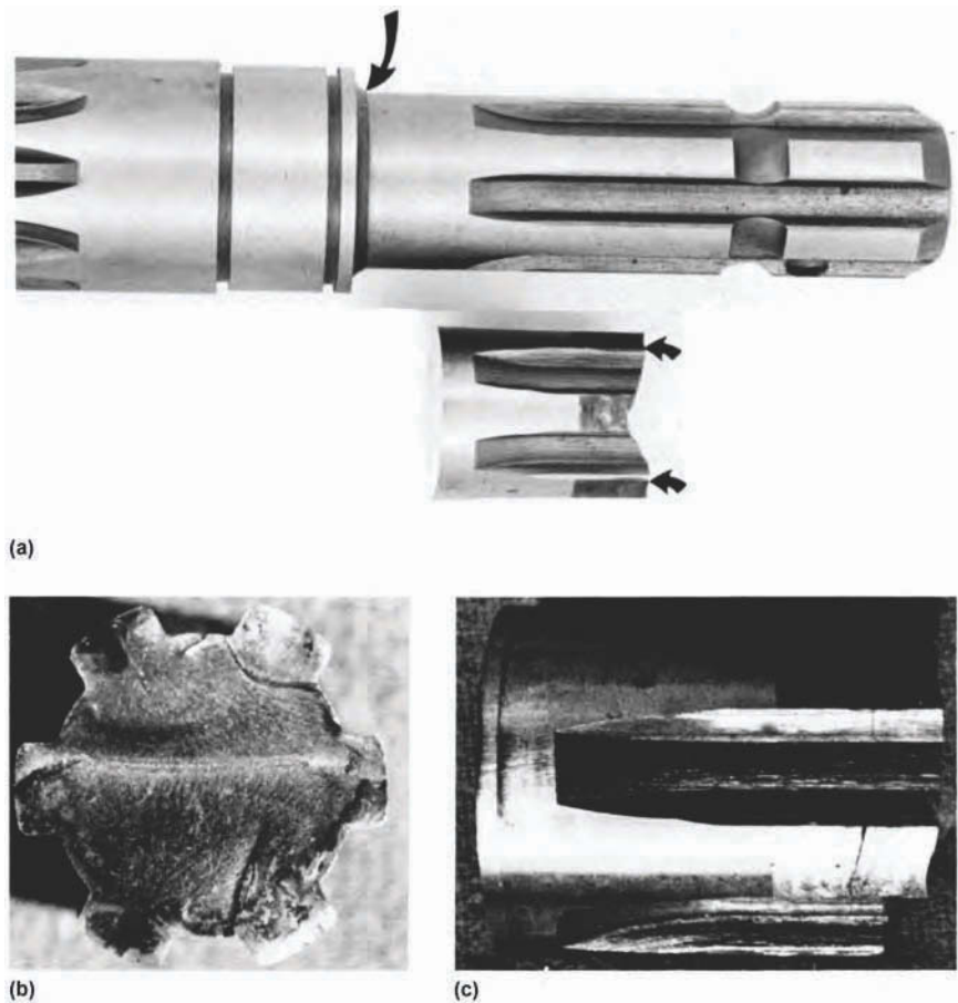
Fig. 14 Severe fretting wear of a splined shaft that led to fatigue fracture. This shaft, though it normally rotates, was being tested in reversed bending by clamped collets on the outside diameter. (a) Dark areas in lower view are areas of severe fretting; fracture occurred at the small arrows. This is an example of the surprises that fretting wear can cause, for the expected location of fatigue fracture was the fillet (large arrow in upper view), shown on a new shaft. However, this area had been strengthened by induction hardening; the fracture location was transferred to the fretting on the outside diameter of the spline. Close-ups of the fracture show (b) the fatigue origins at the outside diameter and (c) multiple fatigue cracks, of which one on each side led to the actual fracture.
