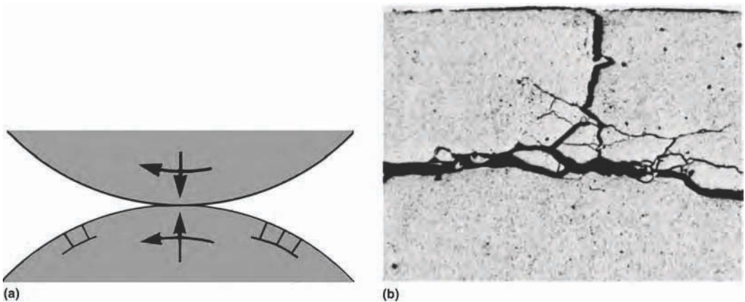
Fig. 2 Subsurface-origin pitting fatigue. (a) Sketch showing usual origin slightly below the surface where the shear stress is high. The fatigue cracks, which usually originate at stress concentrations such as hard, brittle inclusions, propagate parallel and perpendicular to the surface. When a small volume of metal is surrounded by cracks, it falls from the surface, leaving a cavity or pit with steep-sided walls and a flat bottom, until continued operation breaks down the sides of the walls. (b) Micrograph showing fatigue cracks parallel to the surface and perpendicular cracks going to the surface of the specimen. The total depth of this crack system was about 0.007 in., and the metal was case-hardened steel with a surface hardness near 60 HRC. The specimen was a 1-in.-diam roller, tested at a calculated compressive stress of 425,000 psi in pure rolling.
