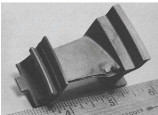
Fig. 13 Hollow, air-cooled stationary vane in an aircraft turboprop engine. Note that the trailing edge is also air cooled by the air that blows between the two thin metal surfaces. The metal is the nickel-base casting alloy INCO 713. Damage on the trailing edge is secondary, caused when a foreign object was sucked into the engine during service.
