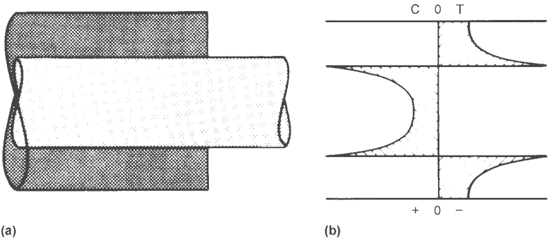
Fig. 5 Elastic stress distribution: interference fit (press or shrink). T, tension. C, compression.
