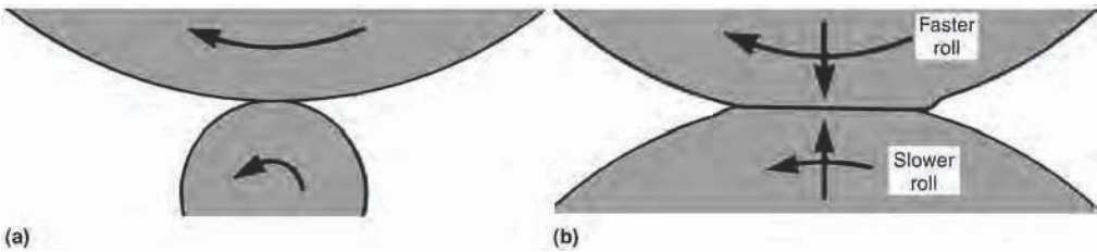
Fig. 4 Schematic of pure rolling (ignoring elastic deformation). (a) When two rollers of different sizes but the same surface velocity (not rpm) contact in pure rolling, point A will contact point A', then point B will contact B', point C will contact point C', and other points around the periphery will contact in succession. However, note that the direction of rotation is toward the left and that the direction of rolling (or of the point of contact) is to the right, in the direction opposite to that of rotation. (b) This concept may be simplified by stopping one roller, such as the lower roller, as shown. If the mating roller rolls around the lower roller in a planetary motion, as shown, again points A, B, and C contact successively the corresponding points on the other roller. The effect on each roller is the same as before, for the relative motion is the same.
