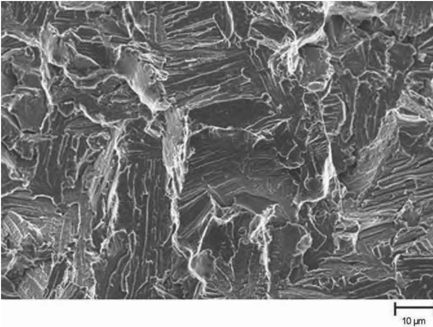
Fig. 9 Scanning electron micrograph of surface structure near the origin of a low-cycle fatigue-loaded test article
