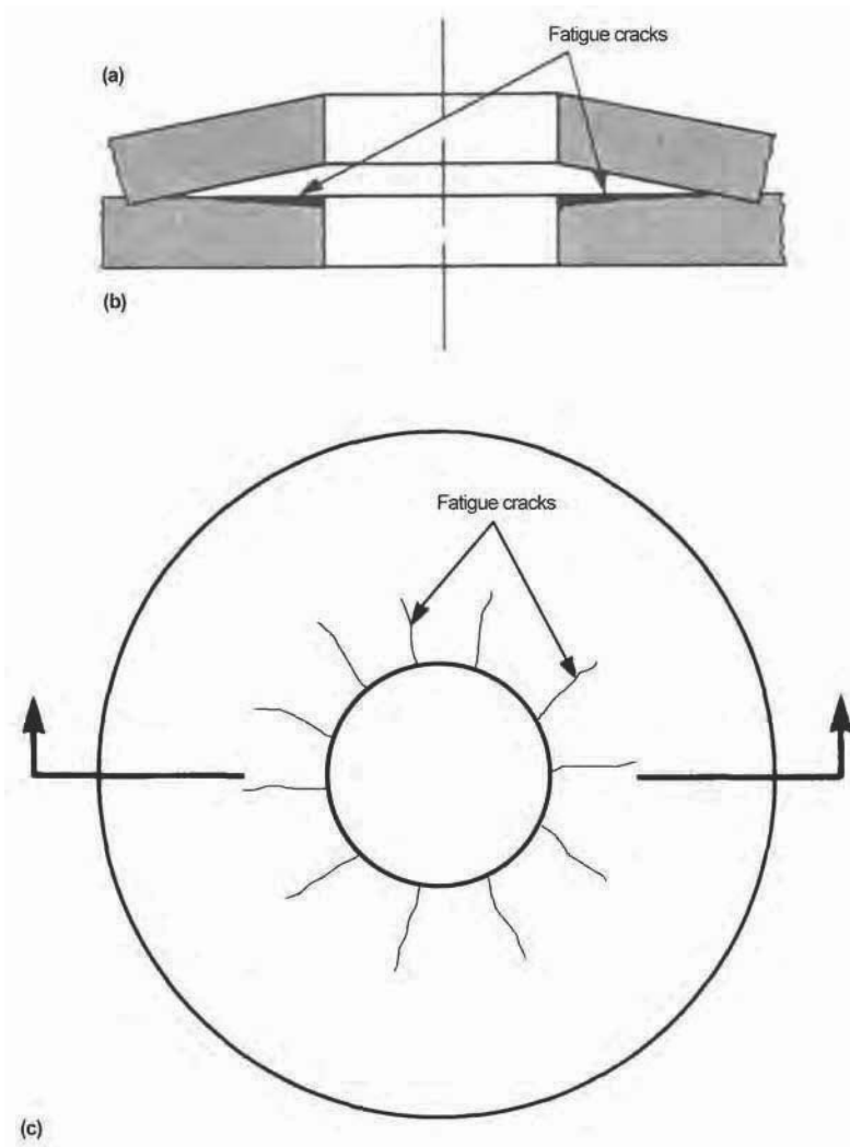
Fig. 20 Sketch of a Belleville spring washer showing how fatigue cracks can form in a nominally compressive stress area. The spring, actually a cone-shaped spring steel washer, is shown in the (a) free condition and in the (b) flattened condition. When flat, the corner of the hole on the convex (upper) side becomes compressively yielded, causing tensile residual stresses when the load is released. Repetitive loading to the flat condition causes radial fatigue cracks to form on the (b) and (c) convex side, but the cracks do not cause fracture. Eventually, independent fatigue cracks may form on the lower (concave) surface that will lead to complete fracture.
