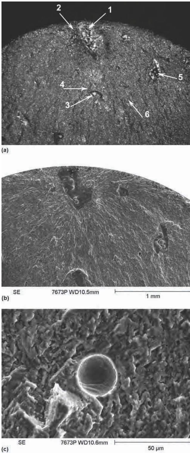
Fig.12 (a) Fracture through an aluminum fatigue bar specimen (33×). Locations 1 to 6 were selected for closer inspection. (b) A scanning electron micrograph of the fracture (50×). (c) Higher magnification of the feature shown at location 4. The feature is a gas pore.
