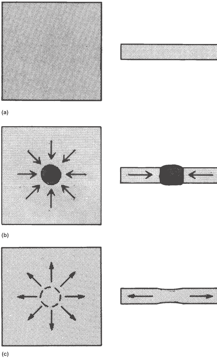
Fig. 4 Thermal residual stresses caused by spot heating. (a) Stress-free plate or sheet at uniform temperature. (b) When locally through-heated, plate expands laterally, generating compressive stresses; also bulges in thickness direction. (c) When cooled to original temperature, plate contracts laterally, generating tensile stresses; also contracts in thickness direction
