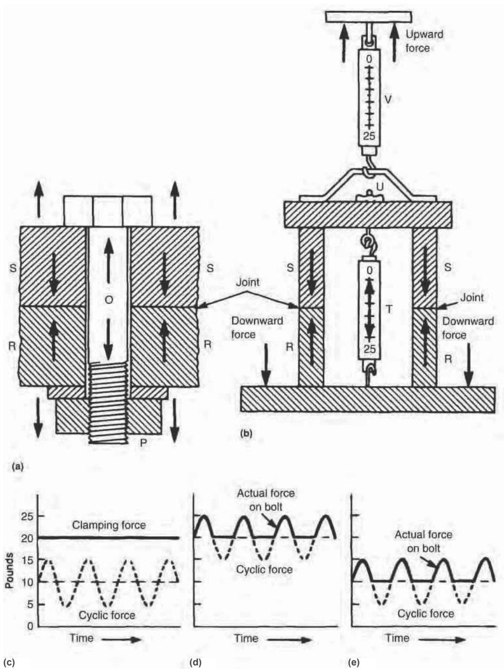
Fig. 21 Demonstration of fatigue of a bolted joint. See text for description.
