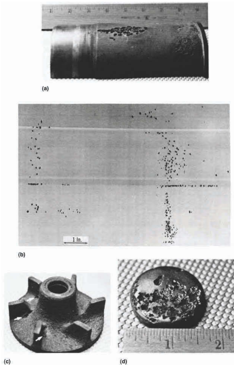
Fig. 11 Cavitation pitting fatigue. (a) Cavitation pitting on a gray cast iron diesel-engine cylinder sleeve. The pitted area is several inches long, and the pits nearly penetrated the thickness of the sleeve. Note the clustered appearance of the pits at preferred locations. (b) Cavitation pitting on another gray cast iron diesel-engine cylinder sleeve unwrapped by a special photographic process. Again, note the clustered locations, with the most severe pitting on the thrust side of the sleeve, against which the piston slides on the power stroke of the combustion cycle. The lighter pitting at left is on the opposite, or antithrust, side of the sleeve. (c) Cavitation pitting at preferred locations on the vanes of a gray cast iron water-pump impeller. This impeller rotated in a clockwise direction; the arrows show some of the pits that were formed in the metal on the suction side of the vanes. (d) Cavitation pitting that perforated this steel freeze plug from a gasoline engine, causing leakage of coolant that could have damaged the engine. Vibration of the wall of the engine block at this location caused this type of damage on the coolant side.
