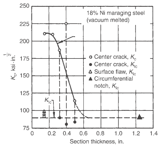
Fig. 4 Effect of section thickness of 18% maraging steel (2 GPa, or 300 ksi minimum yield strength) on measured values of the critical stress-intensity factor, K_{Ic} . At thicknesses greater than about 15 mm (0.6 in.), the critical stress-intensity factor, K_{Ic} (the value of K at which crack propagation becomes rapid), drops to the critical plane-strain stress-intensity factor.
