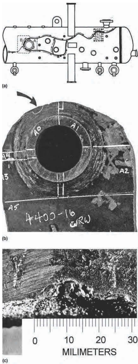
Fig. 7 Hydrotest failure of a carbon steel pressure vessel. (a) Schematic of pressure vessel that failed during hydrotesting showing the location of the origin of the failure and the path of the propagating fracture. A and B indicate sections of the vessel selected for examination. (b) Inside surface of specimen A showing the fracture origin at the toe of a nozzle weld (arrow). (c) Macrograph of the fracture origin showing the thumbnail crack on the fracture surface.
