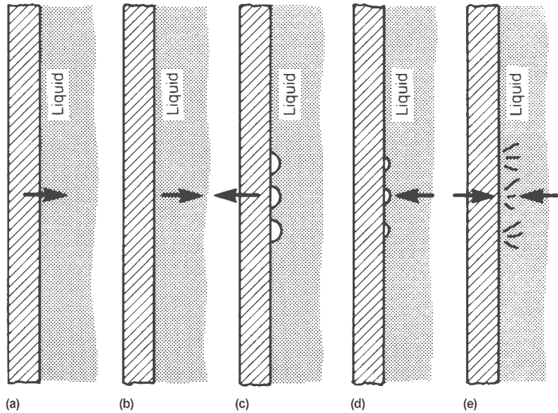
Fig. 12 Mechanism of cavitation pitting fatigue. Serial sketches show a metal wall vibrating to the right and left against a liquid, which in all cases is to the right of the wall. The events shown can occur in a very short time, on the order of microseconds. (a) The metal moves to the right against the stationary liquid, which resists movement because of its inertia. (b) The metal reaches the end of its travel, but the inertia of the liquid causes it to continue to move to the right. (c) The metal starts moving toward the left, away from the liquid, which cannot catch up to the wall because of its inertia. Consequently, cavities or voids are formed in the liquid on the surface of the metal. These are essentially negative-pressure bubbles. (d) The metal reaches the end of its travel to the left and the liquid tries to catch up to the metal and collapse the cavities. (e) The metal starts moving to the right as the cavities collapse violently, or implode, against the metal. As the vibration of the metal continues, the formation and collapse of these cavities in the liquid can cause pitting fatigue on the surface of the metal. If the pounding continues at the same locations on the metal, pits will eventually lead to complete perforation of the metal wall.
