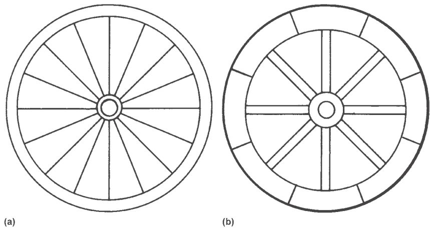
Fig. 9 Closed stress systems in two types of wheel. (a) Light, strong bicycle wheel (radial wire spokes) has tensile stressed spokes, compressively stressed rim (hoop stresses), and tensile hoop stresses in the hub. Longitudinal (axial) stresses are negligible. (b) Heavy wooden wagon wheel with a shrunk-on steel tire generates tensile hoop stresses in the tire, compressive radial and hoop stresses in the wooden rim, compressive radial stresses in the thick wooden spokes, and compressive hoop stresses in the hub. Longitudinal (axial) stresses are negligible.
