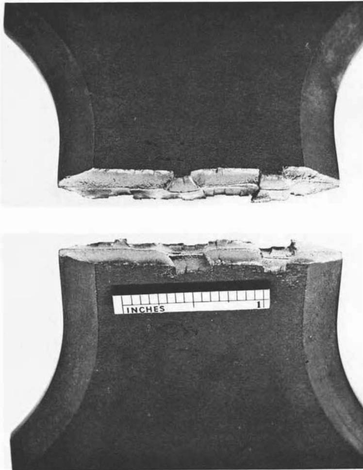
Fig. 28 Reversed bending fatigue of a flat \frac{1}{4} -in. plate of a high-strength low-alloy steel test specimen, designed with tapered edges to prevent fatigue origin at the corners. Note the many separate origins on each side and the very thin final rupture region separating the two fatigue areas on each half. Many other fatigue cracks were present in the reduced section, for this was designed to have a relatively uniform stress in the reduced section.
