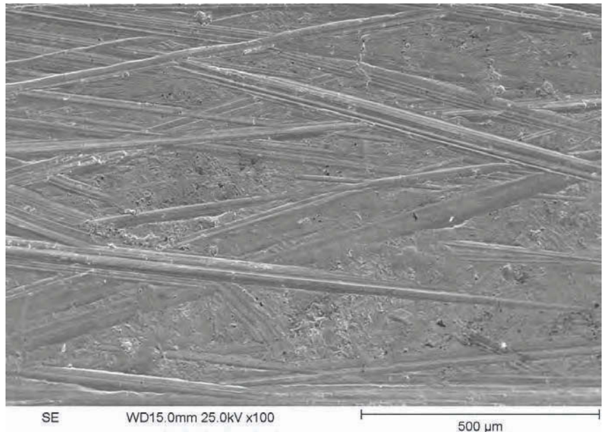
Fig. 2 Scanning electron microscope image of an area of abrasive wear on a soft, low-carbon-steel shaft bearing component, showing classic features of material “cutting” action (100×).
