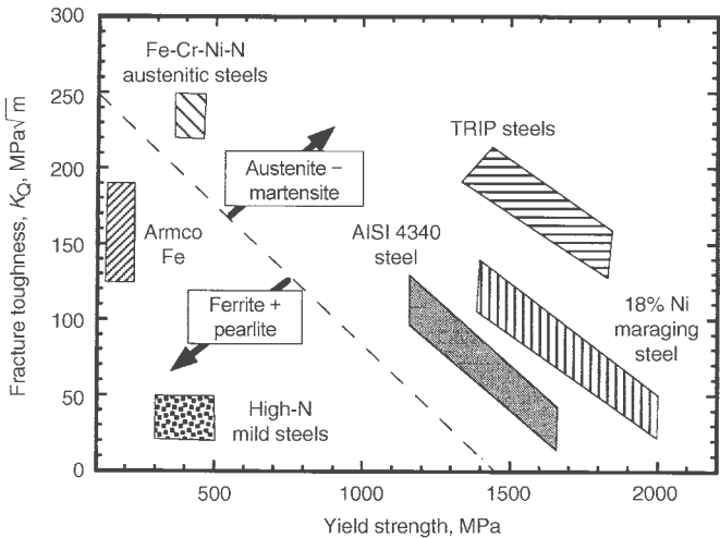
Fig. 5 Fracture toughness versus yield strength for some structural steels. TRIP, transformation-induced plasticity.
