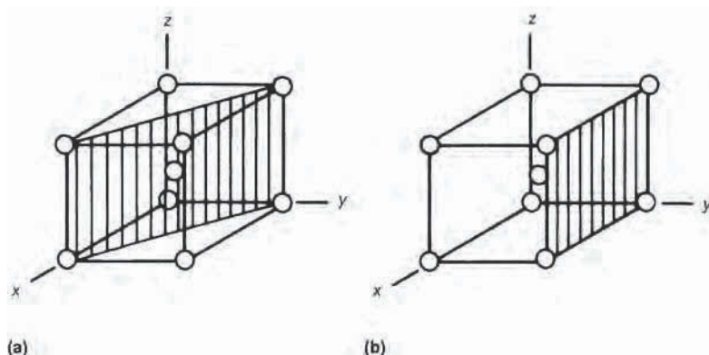
Fig. 1 Basic unit cell of a body-centered cubic structure, shaded to show (a) the diagonal plane along which shear deformation and eventual fracture can occur and (b) one face of the cell, the site of the cleavage mode of fracture
