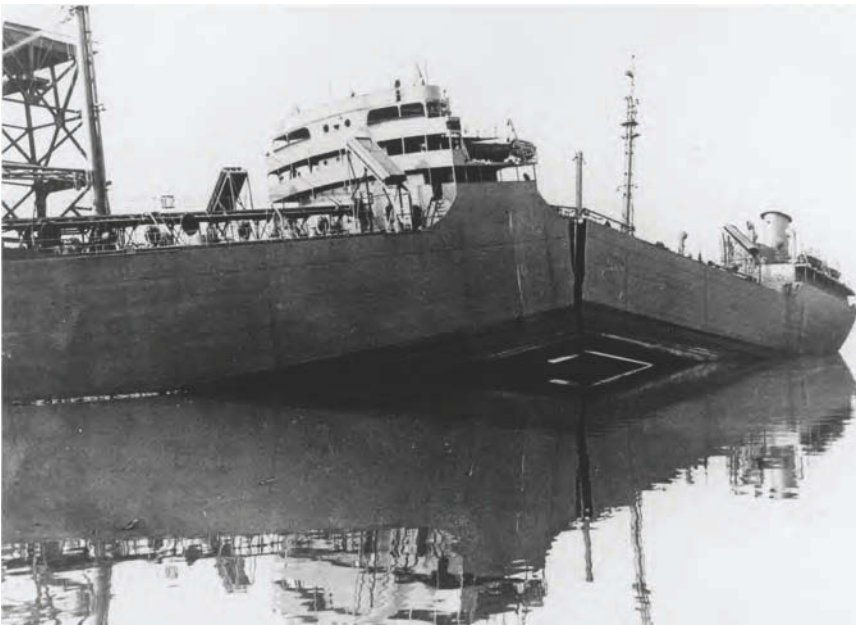
Fig. 1 New T-2 tanker, the S.S. Schenectady , which fractured in 1941 at its outfitting dock. This ship was one of 19 during World War II that had complete brittle fractures; over 200 other ships had partial brittle fractures of the hull. When tested, the fractured plates had normal ductility, as specified. Source: Ref 1
