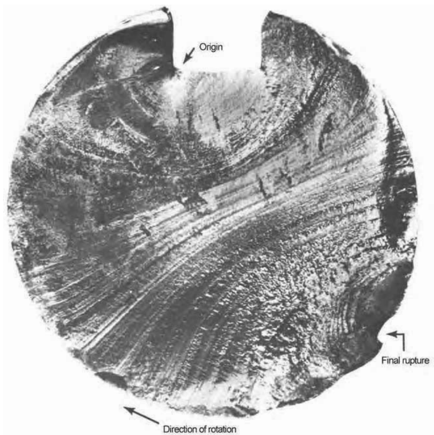
Fig. 29 Rotating bending fatigue fracture of a keyed shaft of grade 1040 steel, approximately 30 HRC. The fatigue crack originated at the lower left corner of the keyway and extended almost through the entire cross section before final rupture occurred. A prominent beach mark pattern is visible, appearing to swing counterclockwise on this section because the rotation was in a clockwise direction.
