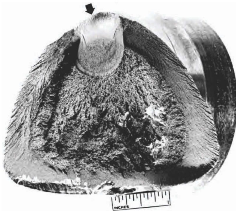
Fig. 5 Surface of a torsional fatigue crack that caused brittle fracture of the case of an induction-hardened axle of 1541 steel. The fatigue crack originated (arrow) at a fillet (with a radius smaller than specified) at a change in shaft diameter near a keyway runout. Case hardness was about 46 HRC at the surface. Note the well-defined chevron marks in the two brittle fractures pointing toward the roughly circular fatigue portion of the fracture. Note also that this fracture is at a 45° angle to the shaft axis, as is typical of high-cycle fatigue and brittle fracture of shafts in torsion.
