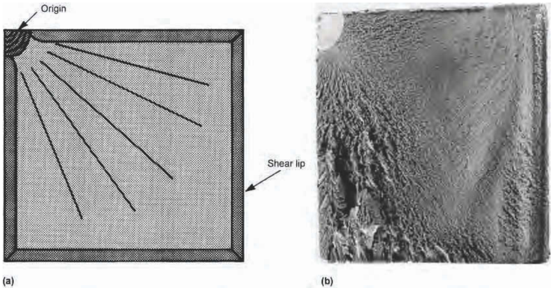
Fig. 9 (a) Sketch of pattern of brittle fracture in a moderately hard, strong metal. The fracture originated at a sharp stress concentration that grew to the critical flaw size for that metal. The sharp stress concentration is frequently, though not always, a fatigue crack or a stress-corrosion crack. Note the fan-shaped pattern radiating from the origin region in the upper left corner. When viewed under the electron microscope, this type of fracture is likely to reveal a cleavage or quasi-cleavage fracture mode. (b) Fracture surface of a large ( \sim 5\text{-}\frac{3}{4} \times 6 in.) equalizer bar made from D6B steel heat treated to a hardness of 45–47 HRC. This bar, which supports the front end of a large crawler tractor, was in service for about 200 h and was then returned to the laboratory, where it was flexed in high-stress, low-cycle fatigue, fracturing at 60,000 cycles. Note that the fatigue-crack zone at the upper left has a very fine texture. Note also the radial, fanlike ridges emanating from the fracture origin and the very small shear lips around the periphery of the brittle fracture. This fracture of a very large, high-strength part released a large amount of energy in a very short time.
