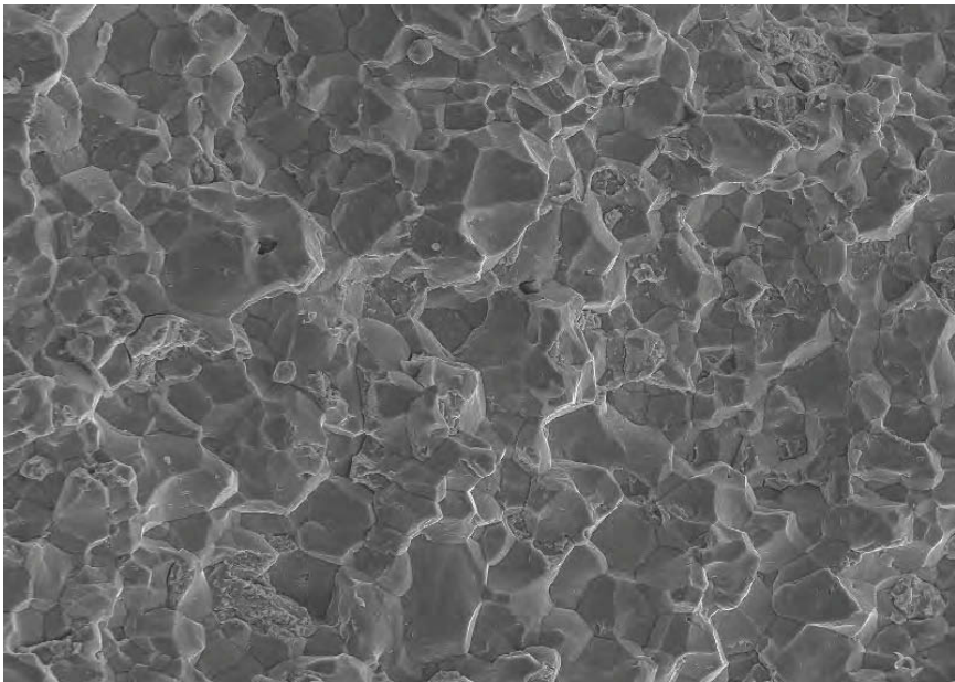
Fig. 14 Intergranular fracture viewed under the scanning electron microscope. Note that fracture takes place between the grains; thus, the fracture surface has a “rock candy” appearance that reveals the shapes of part of the individual grains.
