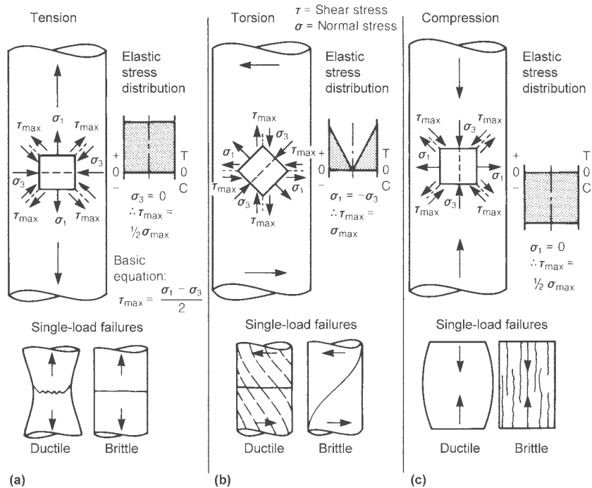
Fig. 1 Free-body diagrams showing orientation and elastic distribution of normal (tensile and compressive) and shear stress components in a shaft under pure (a) tension, (b) torsion, and (c) compression loading. Also shown is single-overload fracture behavior of ductile and brittle materials under these loading conditions (bottom diagrams). T, tension. C, compression. Adapted from Ref 1
