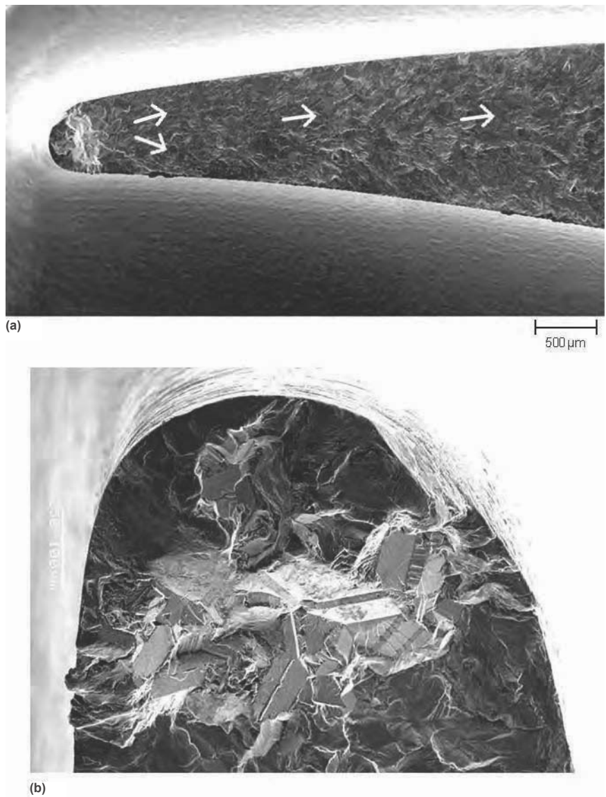
Fig. 3 (a) Example of faceted stage 1 fatigue initiation in a cast nickel-base superalloy turbine blade. Arrows denote crack propagation direction. (b) Overall blade fracture and continuation of flatter stage 2 crack propagation emanating from stage 1 region.
