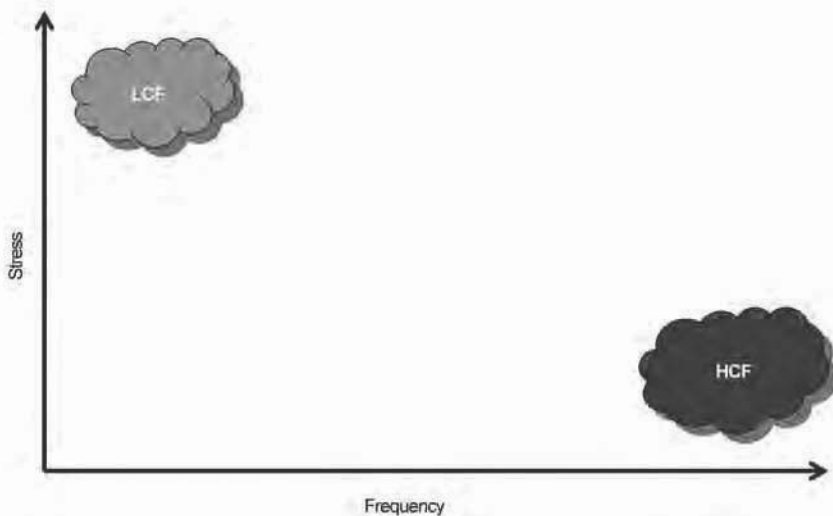
Fig. 10 Schematic showing the relationship between low- and high-cycle fatigue. In systems where significant vibration loads are present, high-cycle fatigue (HCF) tends to be related to high-frequency loading, and low-cycle fatigue (LCF) tends to be related to slowly applied higher-stress loads.
