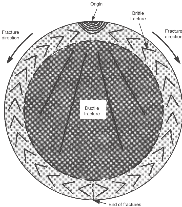
Fig. 4 Sketch of a fractured case-hardened shaft showing chevron marks pointing back toward the fracture origin. If brittle fracture continues completely around the part, the two separate fractures may form a step where they meet opposite the origin. The interior, or core, is likely to have a ductile fracture with dimpled rupture on the microscale.
