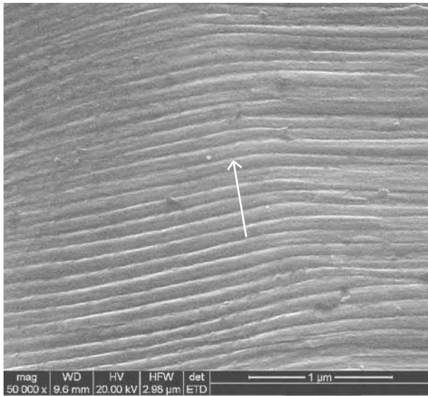
Fig. 6 Example of well-formed fatigue striations in titanium alloy ( R = 0.05 ; maximum alternating stress, 105 ksi). ( R is the minimum stress divided by the maximum stress.) The striation density is approximately 263,000 striations/in. ( \sim 3.8 \times 10^{-6} in./striation). The arrow denotes the crack propagation direction.
