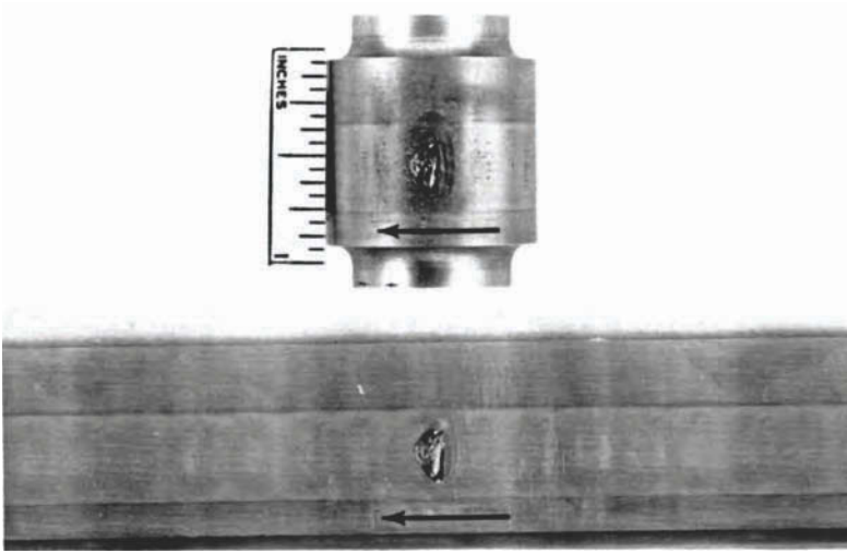
Fig. 7 Two views of a roller, showing a typical arrowhead-shaped surface pit. The arrows indicate the direction of rotation; the direction of rolling of the mating roller is to the right, while the direction of sliding is to the left. The upper view is a normal photograph of the pitted area; the lower view shows the entire surface “unwrapped” by a special photographic method. This specimen was tested at a calculated compressive stress of about 450,000 psi and ran for 14,229,000 revolutions prior to pitting failure. This was a carburized and hardened alloy steel, with a surface hardness near 60 HRC.
