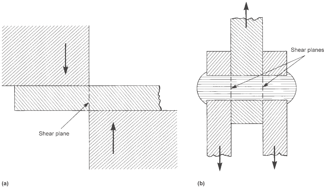
Fig. 7 Elastic stress distribution: direct (transverse) shear. (a) Single shear. (b) Double shear
