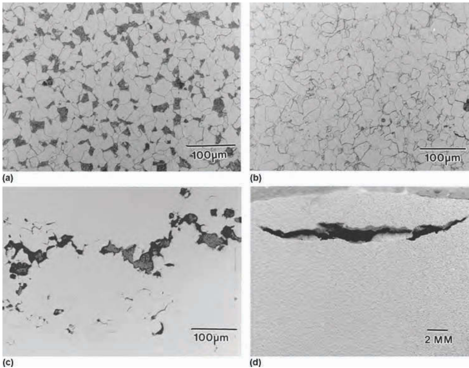
Fig. 12 Hydrogen-damaged refinery platformer line (carbon steel, 0.5% Mo). (a) Undamaged microstructure. (b) Decarburization region caused by hydrogen depleting the iron carbides. (c) Microfissuring at inclusions. (d) Hydrogen blister caused by methane gas formation. (a) and (b), nital etch; (c) and (d), unetched. Source: Ref 4
