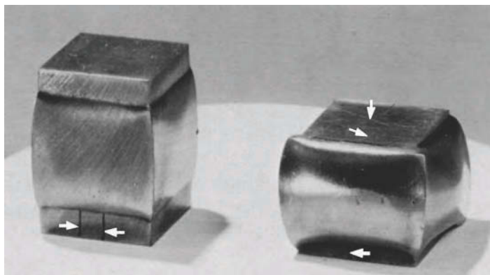
Fig. 8 Compression test of two steel cubes deep case hardened only on the top and bottom surfaces. A compressive force perpendicular to the case-hardened surfaces caused cracking (arrows) in the very hard (66 HRC) cases on both surfaces. The soft, ductile cores simply bulged under the compressive force but did not fracture. As sketched in Fig. 1(c), these composite specimens illustrate behavior of both brittle and ductile metals and dramatically show the difference in properties of the case and core. (These 1-in. 2 compression blocks were made from low-carbon alloy steels. They were water quenched and had \frac{3}{16} in. case depth; both were compressed to 180,000 psi.) Photo courtesy of Xtek Corp., TSP Mill Products Division
