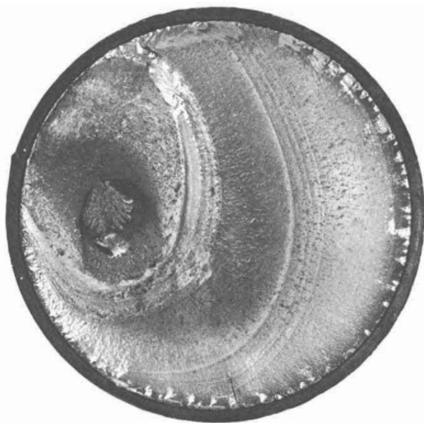
Fig. 17 Surface of a fatigue fracture in a grade 1050 steel shaft, with hardness of about 35 HRC, that was subjected to rotating bending. The presence of numerous ratchet marks (small shiny areas at the surface) indicates that fatigue cracks were initiated at many locations along a sharp snap-ring groove. The eccentric pattern of oval beach marks indicates that the load on the shaft was not balanced; note the final rupture area (stage 3) near the left side.
