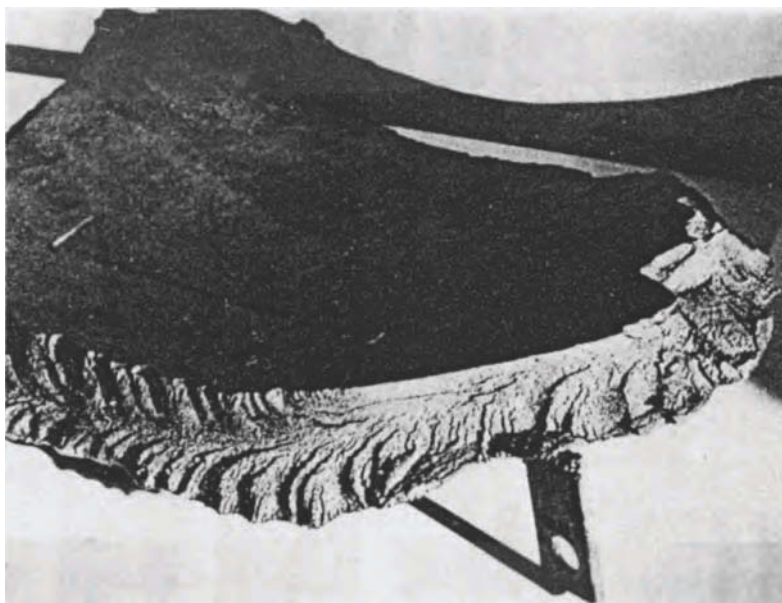
Fig. 3 Fragment of a fractured thick-wall drum. The fracture, which started at the right side of the photo, ran rapidly to the left, resulting in a well-defined chevron pattern. Source: Ref 7
