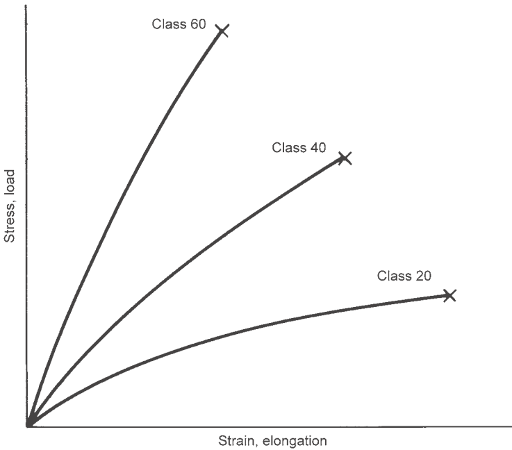
Fig. 5 Typical stress-strain curves for three classes of gray cast iron. This nonlinear behavior is caused by the graphite flakes, which act as internal stress concentrations, or notches, within the metal matrix. Source: Ref 3
