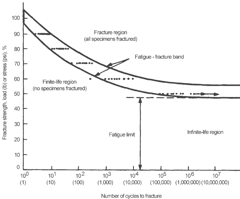
Fig. 18 Typical fatigue ( S - N ) diagram of laboratory fatigue testing of medium-strength ferrous metal.
