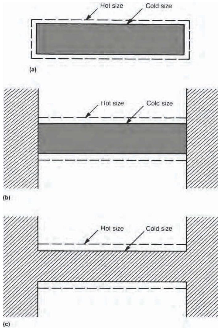
Fig. 2 Thermal residual stresses. (a) Unrestrained expansion and contraction. (b) Restrained expansion, unrestrained contraction. (c) Restrained expansion and contraction.
