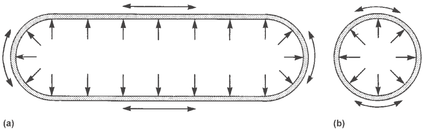
Fig. 8 Elastic stress distribution: thin-wall pressure vessel. (a) Longitudinal section. (b) Cross section
