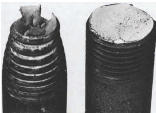
Fig. 3 Two identical steel bolts that had been given different heat treatments and then pulled to fracture in a tensile test. The bolt at the left was annealed; when pulled, it had much deformation, as evidenced by the necking and thread separation. Fracture was of the cup-and-cone type with a large shear lip, similar to that in Fig. 2. The bolt at the right was austenitized and then brine quenched to a high hardness. The bright, transverse fracture and lack of deformation characterize a brittle fracture.
