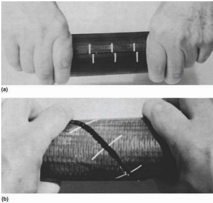
Fig. 4 Slit radiator hoses used to demonstrate concentrated “pure” shear stresses. (a) When hose is slit longitudinally, each side of the slit slides along the other side when the hose section is twisted back and forth. The sliding represents pure longitudinal shear stresses, because there is no opening (tension) or closing (compression). Transverse shear can be demonstrated similarly by rotating the smooth ends of two cylinders against each other. (b) When hose is slit at a 45^\circ angle to its axis and then twisted as shown, opening represents tension, and closing represents compression forces. Imagine tiny rubber bands in line with the white marks; when twisted as shown, they are stretched in tension. When twisted in the opposite direction, compression forces are generated after the slit closes. Note that no sliding shear occurs when the 45^\circ slit is opened and closed.
