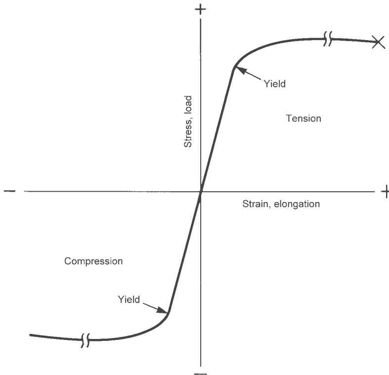
Fig. 6 Complete engineering stress-strain curve showing the normally considered tensile region (upper right) and the often neglected compression region (lower left)
