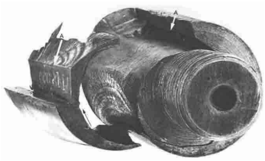
Fig. 39 Torsional fatigue fracture in a 3-3/8-in.-diam keyed tapered shaft of grade 1030 steel characterized by “peeling” that progressed around the shaft. The fatigue crack originated in the corner (A) of the keyway from pressure of the key aligning a large hub to the shaft. The fatigue crack progressed completely around the shaft, under the keyway, and started around again, all in a clockwise direction, before final separation occurred and nearly broke off the “wing” at the left. The only thing necessary to prevent this type of fracture is to make sure that the large nut that forces the hub to fit tightly against the tapered surface does not come loose. If the nut is loose, the key and keyway, rather than the frictional fit of the conical joint, carry the torsional force.
