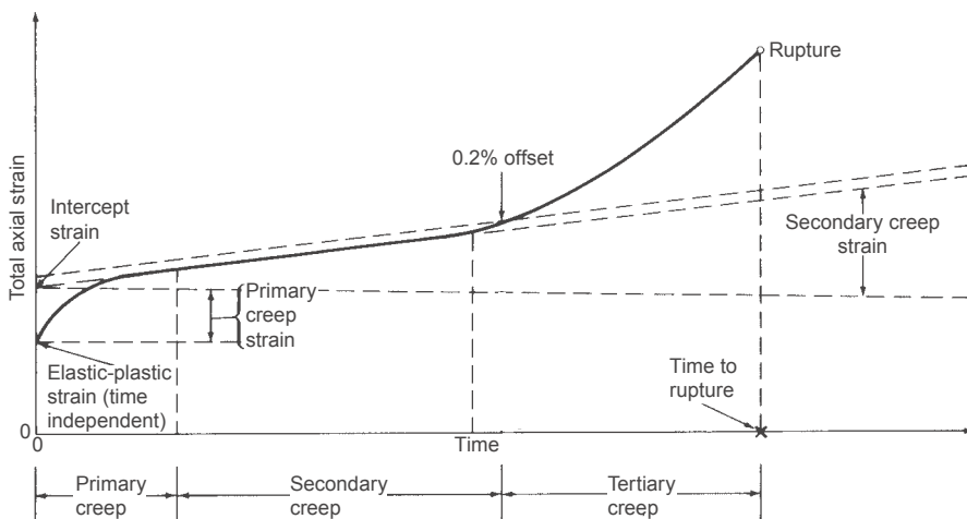
Fig. 1 Schematic tension-creep curve, showing the three stages of creep. Source: Ref 4
