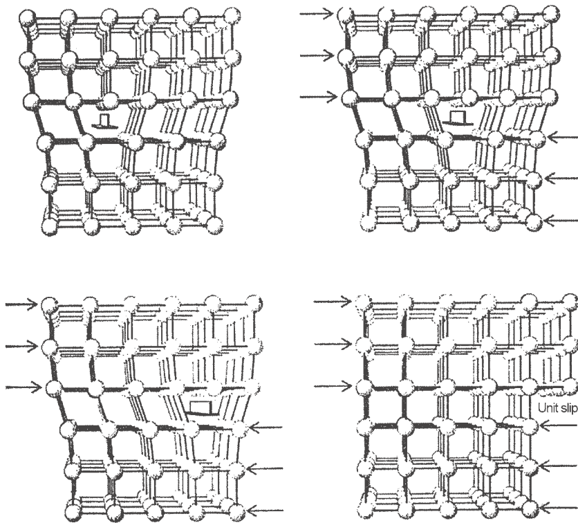
Fig. 1 Schematic sketch of microstructural changes in crystal structure due to repetitive shearing forces. Spheres represent atoms, and lines represent attractive and repulsive interatomic forces. An edge dislocation, represented by the inverted T-shaped symbol, is an imperfection in the crystalline structure. When repetitive shearing forces (top right) are applied, the dislocation slips one cell to the right. Continued repetitive shearing forces (bottom) make the dislocation move to the edge of the crystalline structure. When this action is going on in many other crystals, the dislocations eventually join to form microscopic cracks. This is stage 1 in the fatigue process.
