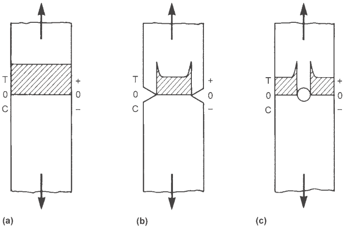
Fig. 1 Elastic stress distribution: pure tension. T, tension. C, compression. (a) No stress concentration. (b) Surface stress concentrations. (c) Transverse hole stress concentration
