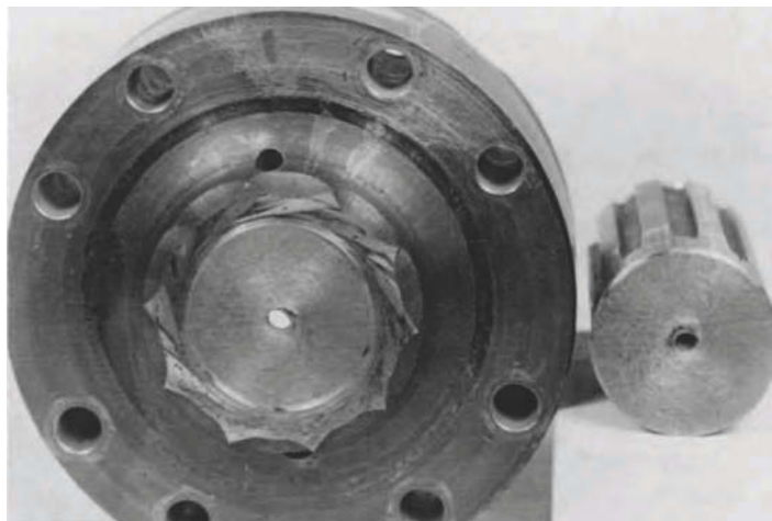
Fig. 6 Single-overload torsional fracture of a shaft of ductile steel similar to that in Fig. 5. The hole in the center is the lathe center from the original machining on the part
