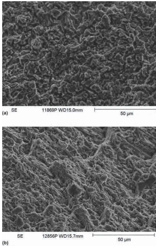
Fig. 11 (a) Ductile fracture through type 420 stainless steel hardened to 51 HRC equivalent (1000 \times ). (b) A woody texture, indicative of ductile fracture, through grade 9254 spring steel.
