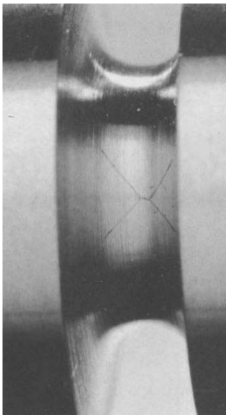
Fig. 35 Close-up of a reduced area on a medium-carbon steel drive shaft showing the X-shaped crack pattern characteristic of reversed torsional fatigue. Reversed torsional fatigue causes approximately 45^\circ spiral fatigue cracks on opposite diagonals. The original shear crack was in the longitudinal shear plane; then each pair of torsional fatigue cracks developed at a 45^\circ angle to the shaft axis.
