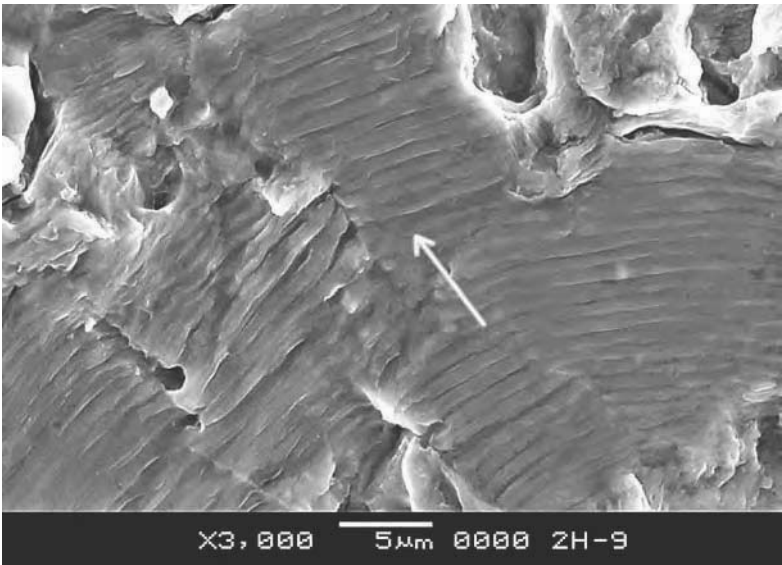
Fig. 5 Example of well-formed striations in a forged high-pressure compressor blade made of titanium alloy. The striation density is approximately 30,000 striations/in. ( \sim 3.3 \times 10^{-5} in./striation). The arrow denotes the crack propagation direction.
