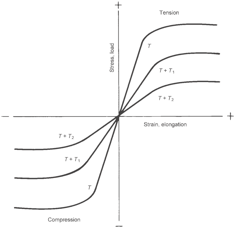
Fig. 7 Effect of elevated temperatures T_1 and T_2 on tensile and compressive properties of a typical metal
