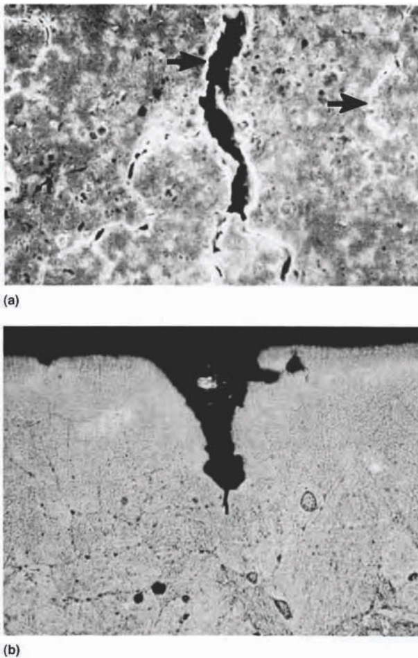
Fig. 10 (a) Scanning electron photograph of corrosion pits on the surface of a gas turbine airfoil showing both large and small pits (arrows) that led to fatigue fractures (300 \times ; shown at 75%). The material is the precipitation-hardening stainless steel 17-4PH. (b) Photomicrograph of a polished and etched section through a pit like those shown in (a) (500 \times ; shown at 75%). Note the start of a fatigue crack growing from the bottom of the pit. Pitting was caused by continued operation in a seawater environment.
