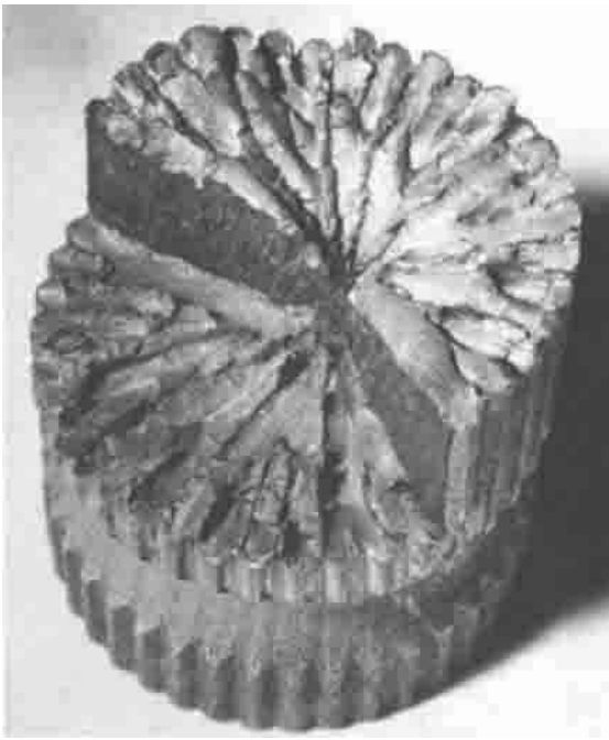
Fig. 38 A “starry” spline fracture similar to that shown in Fig. 37 due to reversed torsional fatigue on a 1½ in.-diam spline. Torsional fatigue has caused many of the surrounded segments to fall out of the shaft. Note that the longitudinal cracks penetrated nearly to the center of the shaft. This part was made from low-carbon alloy steel with a hardness of 24 HRC in the shaft area.
