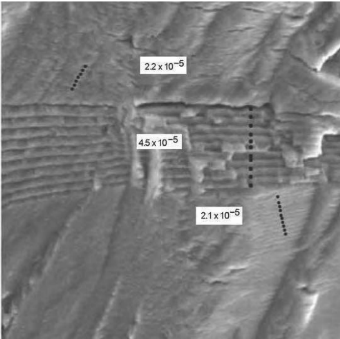
Fig. 8 Electron micrograph showing a block-loaded test article with a band of 10 cycles of a higher load. Source: Ref 2
