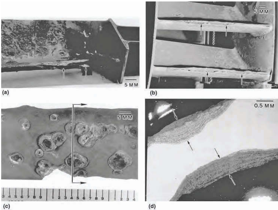
Fig. 9 Hot-corrosion attack of René 77 nickel-base alloy turbine blades. (a) A land-based, first-stage turbine blade. Notice the deposit buildup and flaking and splitting of the leading edge. (b) Stationary vanes. (c) A land-based, first-stage gas turbine blade that had type 2 hot-corrosion attack. (d) A metallurgical cross section showing the layered corrosion attack of the blade shown in (c). Source: Ref 4
