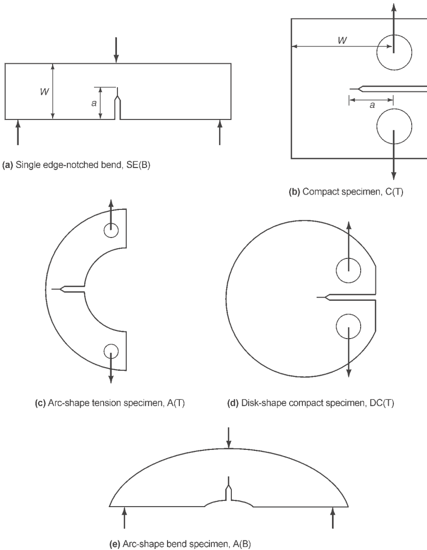
Fig. 11 Specimen types used in plane-strain fracture-toughness ( K_{IC} ) testing (ASTM 399). a , crack length; W , specimen width
