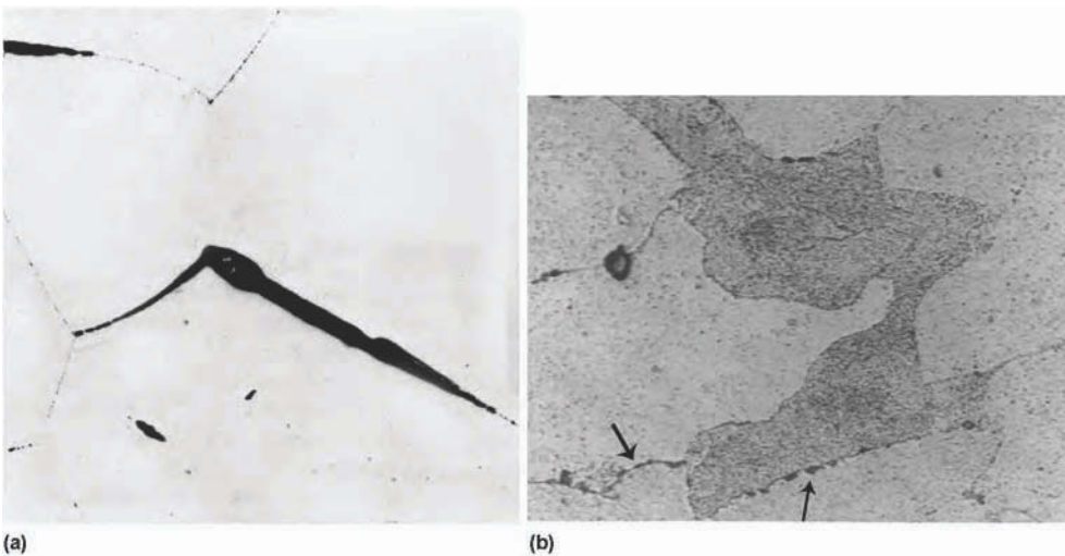
Fig. 4 Comparison of wedge-shaped cracks and creep voids: (a) triple-point stress rupture (60 \times ); (b) creep cavitation damage (arrows) in a desuperheater inlet header (1000 \times )
