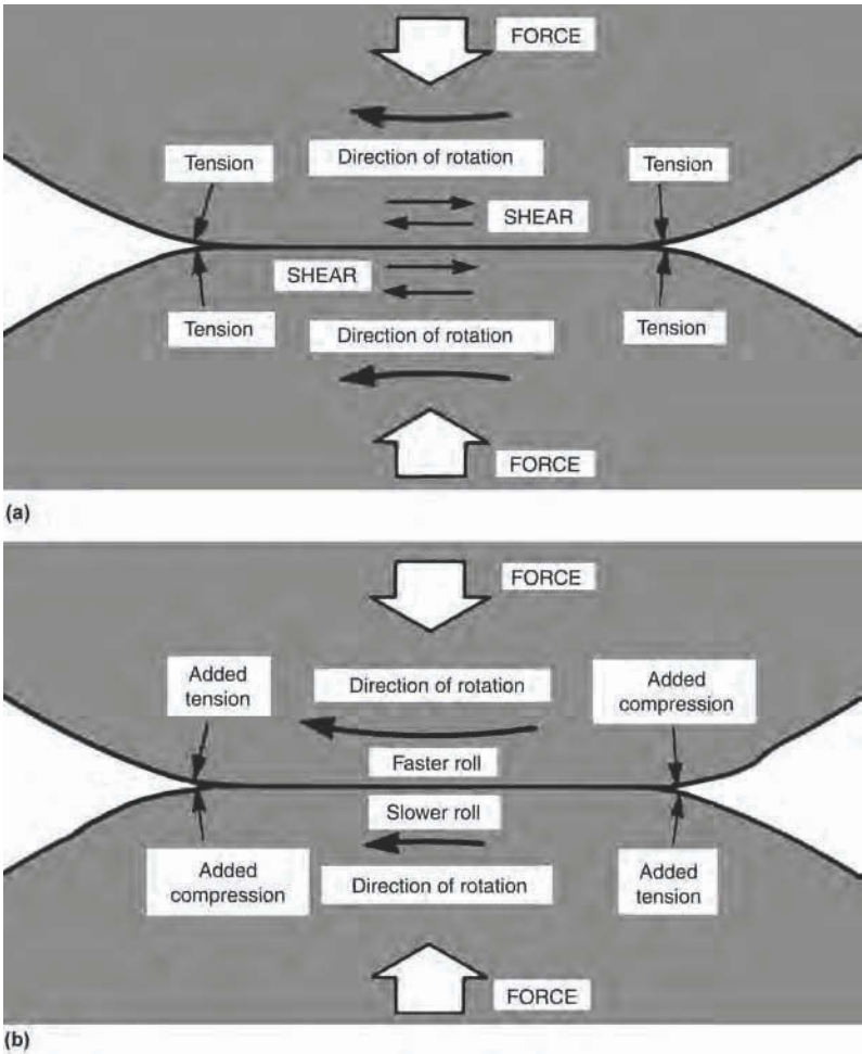
Fig. 6 Elastic stress distribution: convex surfaces in contact. (a) Rolls turning at same speed. (b) Rolls turning at different speeds
