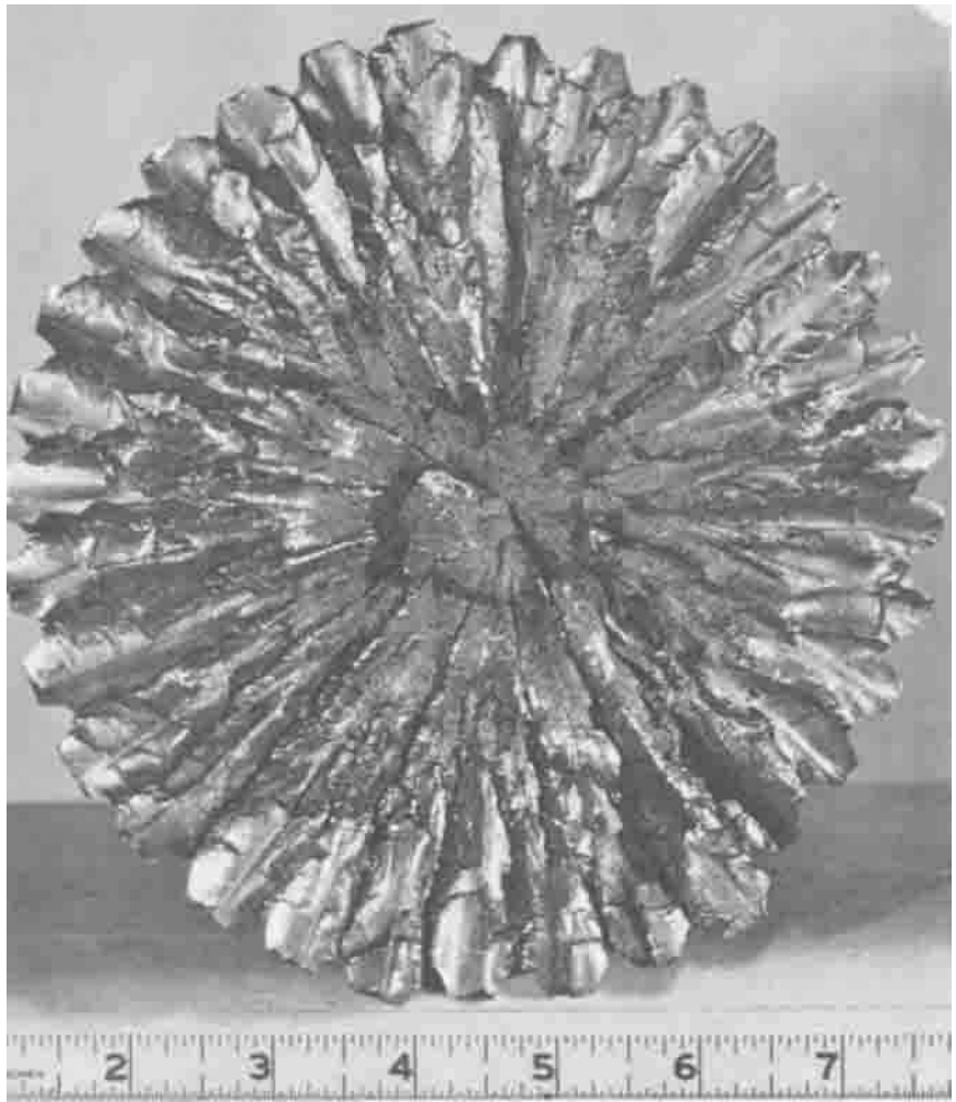
Fig. 37 Reversed torsional fatigue of a 6\frac{3}{4} in.-diam spline shaft showing the characteristic "starry" pattern of multiple fatigue cracks. Each of the 32 spline teeth has two fatigue cracks, each at 45^\circ to the shaft axis, that form a V-shaped region. In addition, there are longitudinal radial fatigue cracks that penetrate nearly to the center of the shaft. This type of fatigue progresses at each location where a shaft enters an internal spline and is repeated if there is an internal spline at another location on the shaft. These cracks surround portions of the metal, forming essentially wedge-shaped segments, somewhat like those of an orange.
