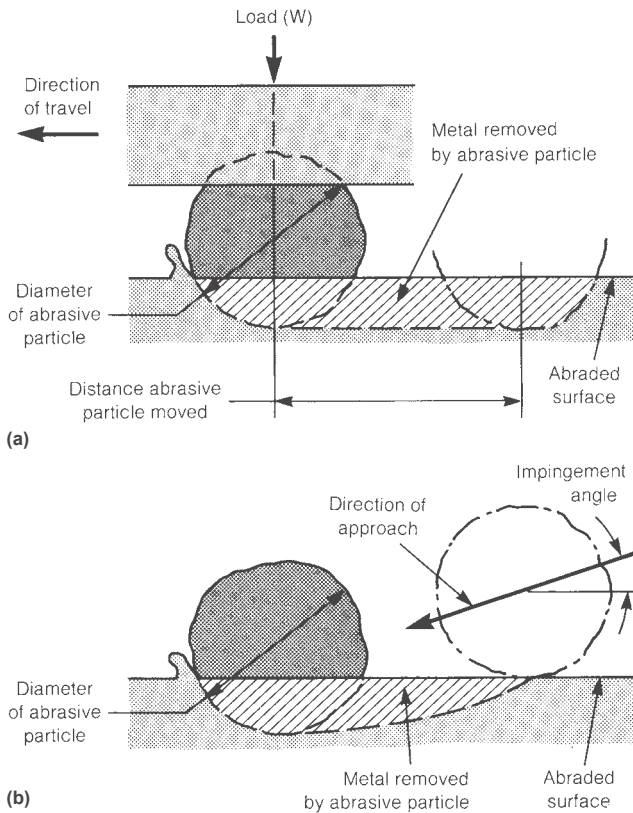
Fig. 1 Idealized representations of the two types of force applications on abrasive wear particles: (a) Cutting or plowing action of a contained particle under pressure. That is, the particle is not free but is under pressure from other particles or a solid object. This is characteristic of grinding and gouging abrasion, in which the hard particles are forced to scratch or cut the metal surface. (b) Cutting or plowing action of a loose particle flowing across the metal surface after impinging upon the surface. This is characteristic of erosive wear, in which free particles strike the surface at an angle and then slide across the surface. Source: Ref 1
