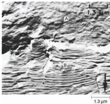
Fig. 9 Fatigue fracture in aluminum alloy 2024-T3 tested first in vacuum (region A) and then in air (region B) (7500×). The arrow at the lower right indicates the direction of crack propagation. Note the flat, featureless fracture surface formed while testing in vacuum (region A), with no correlation between fracture appearance and the cyclic nature of the imposed loading. In contrast, the regular fatigue striations formed while testing in air (region B) correlate with the crack advance of each loading cycle. Source: Ref 9
