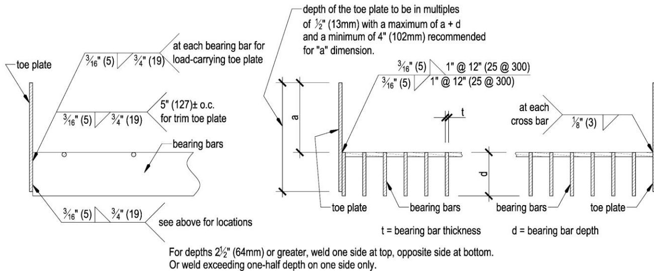
Figure 2.1.6 - TOE PLATE FOR HEAVY DUTY GRATING 2 ½" DEEP AND GREATER (bearing bar thickness ¼"(6mm) and greater and bearing bar clear opening greater than or equal to 5/8"(16mm))
