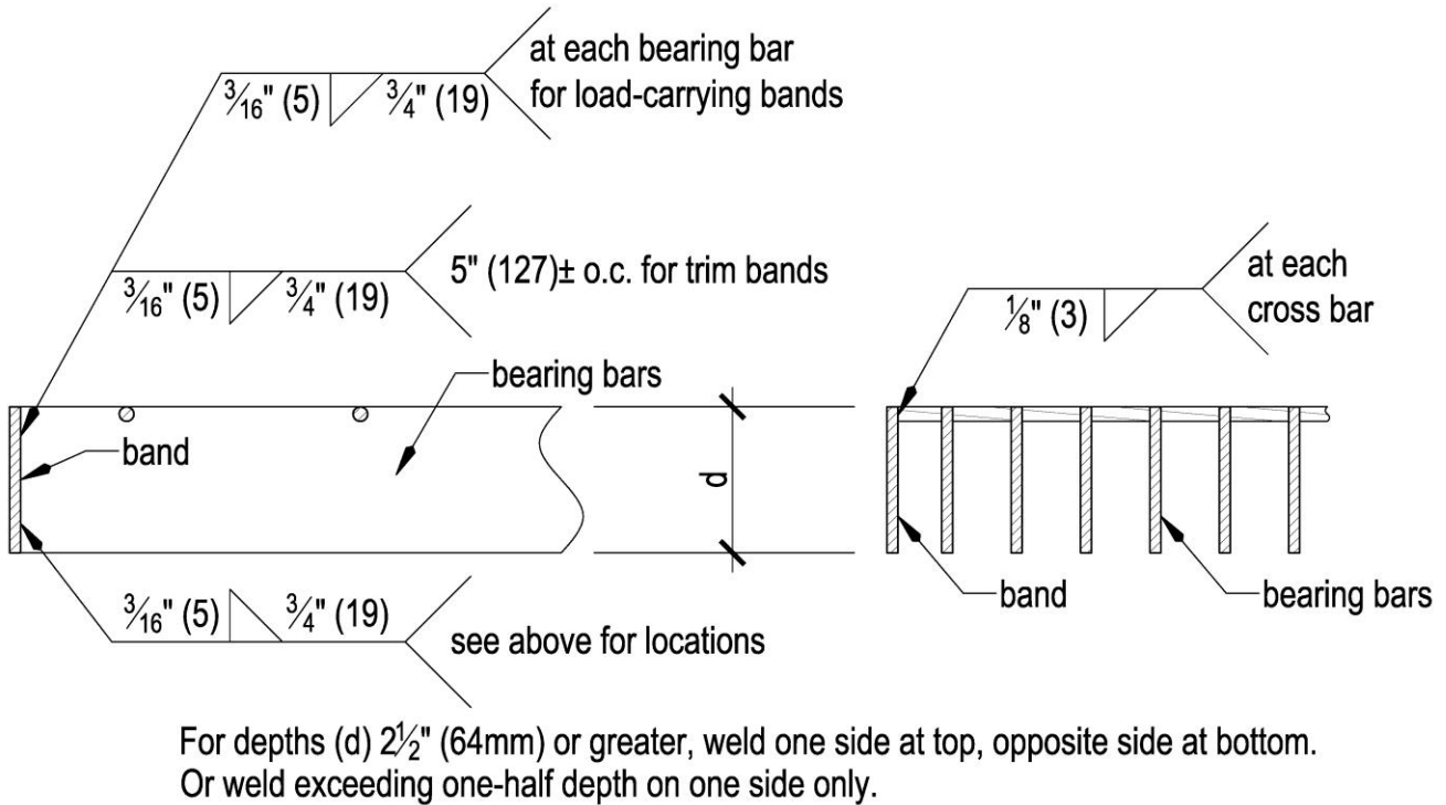
Figure 2.1.4 - BANDING FOR HEAVY DUTY GRATING 2 1/2" DEEP AND GREATER (bearing bar thickness 3/4" (6mm) and greater and bearing bar clear opening greater than or equal to 5/8" (16mm))
