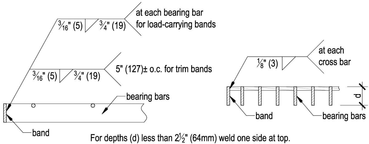
Figure 2.1.3 - BANDING FOR HEAVY DUTY GRATING LESS THAN 2 1/2" DEEP (bearing bar thickness 3/4" (6mm) and greater and bearing bar clear opening greater than or equal to 5/8" (16mm))
