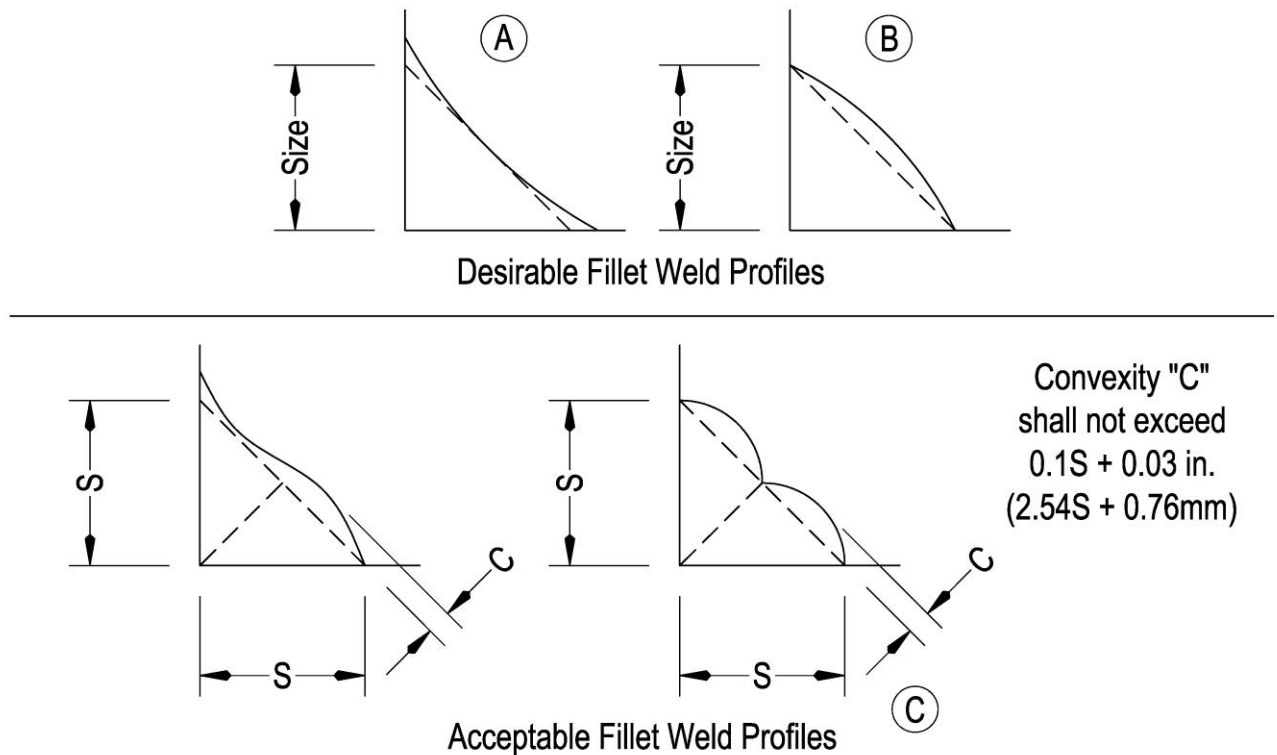
Figure 3.6 – ILLUSTRATION OF ACCEPTABLE FILLET WELD PROFILES
