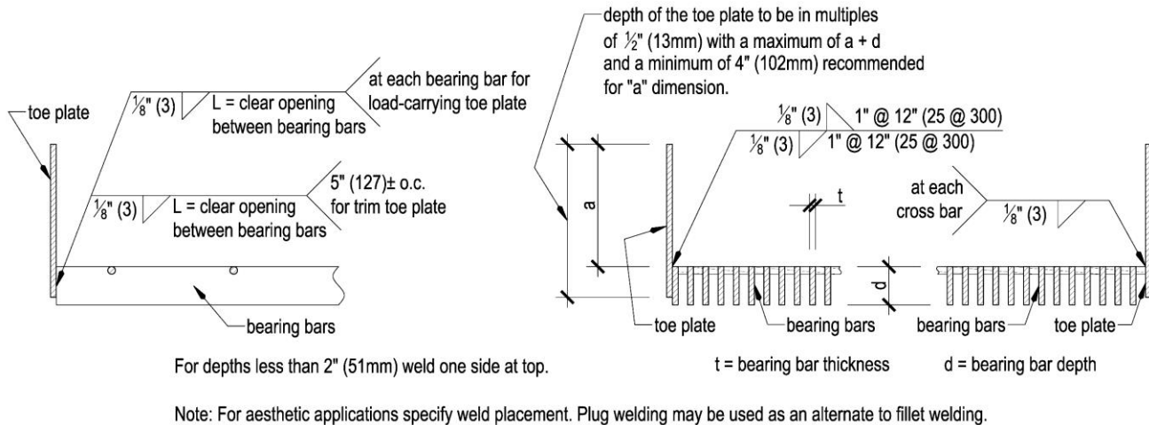
Figure 2.1.9 - TOE PLATE FOR CLOSE MESH GRATING LESS THAN 2" DEEP (all grating with bearing bars having a clear opening less than 5/8" (16mm) )
