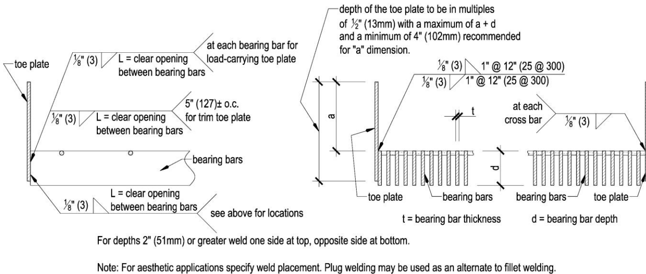
Figure 2.1.10 - TOE PLATE FOR CLOSE MESH GRATING 2" DEEP AND GREATER (all grating with bearing bars having a clear opening less than 5/8" (16mm) )
