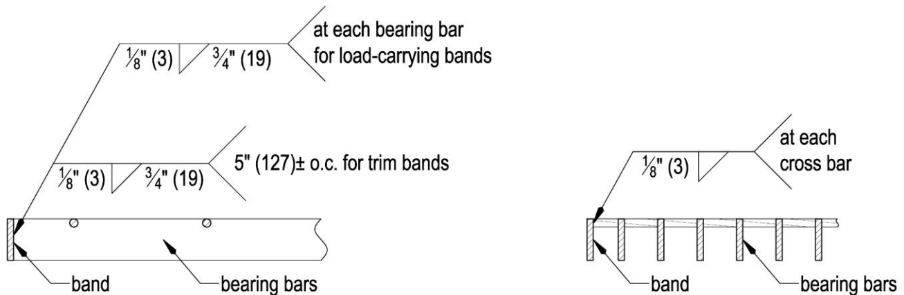
Figure 2.1.1 - BANDING FOR STANDARD GRATING
