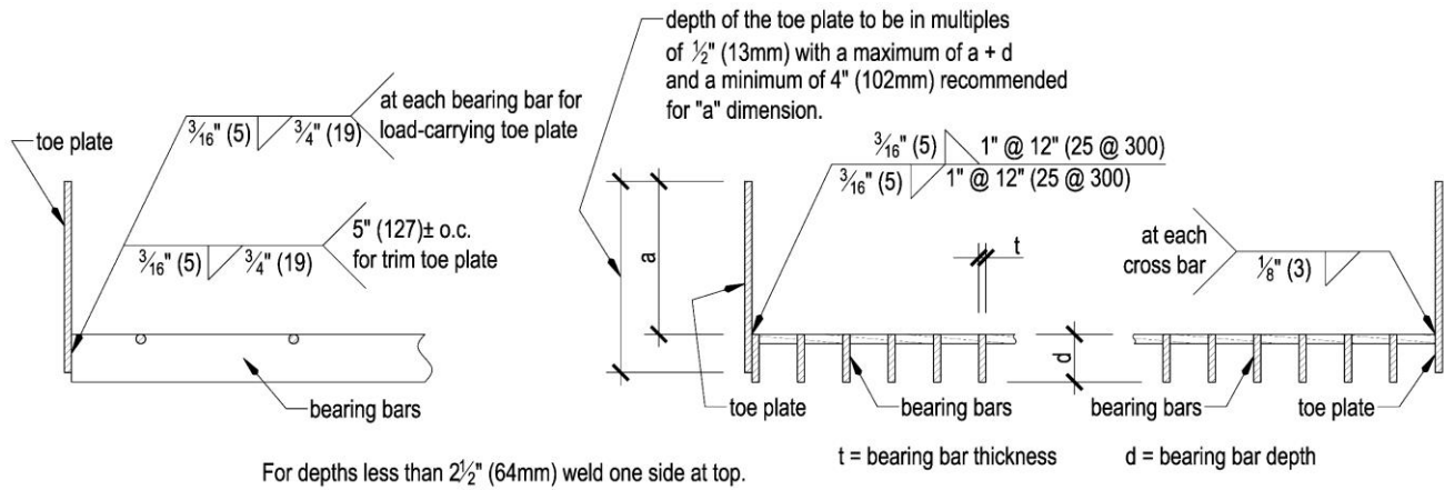
Figure 2.1.5 - TOE PLATE FOR HEAVY DUTY GRATING LESS THAN 2 ½" DEEP (bearing bar thickness ¼"(6mm) and greater and bearing bar clear opening greater than or equal to 5/8"(16mm))
