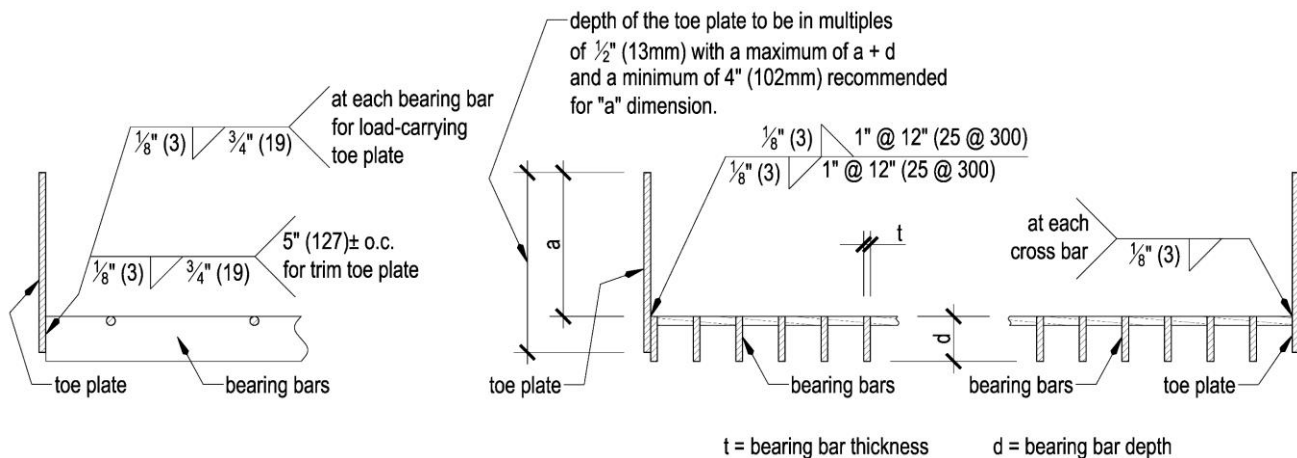
Figure 2.1.2 - TOE PLATE FOR STANDARD GRATING
