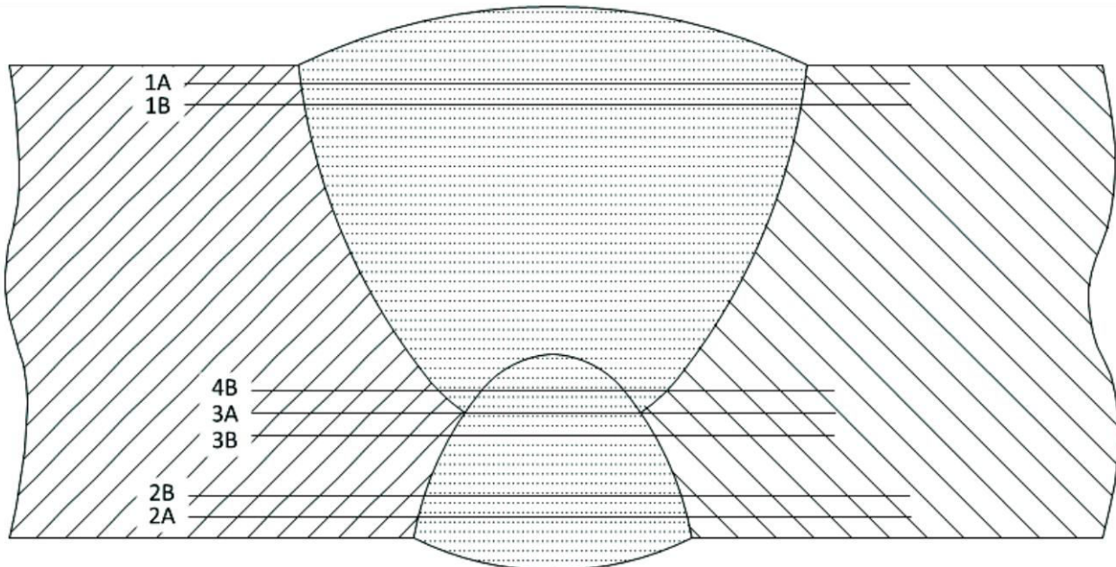
Figure C.2 — Rows of indentations in butt welds from two sides
