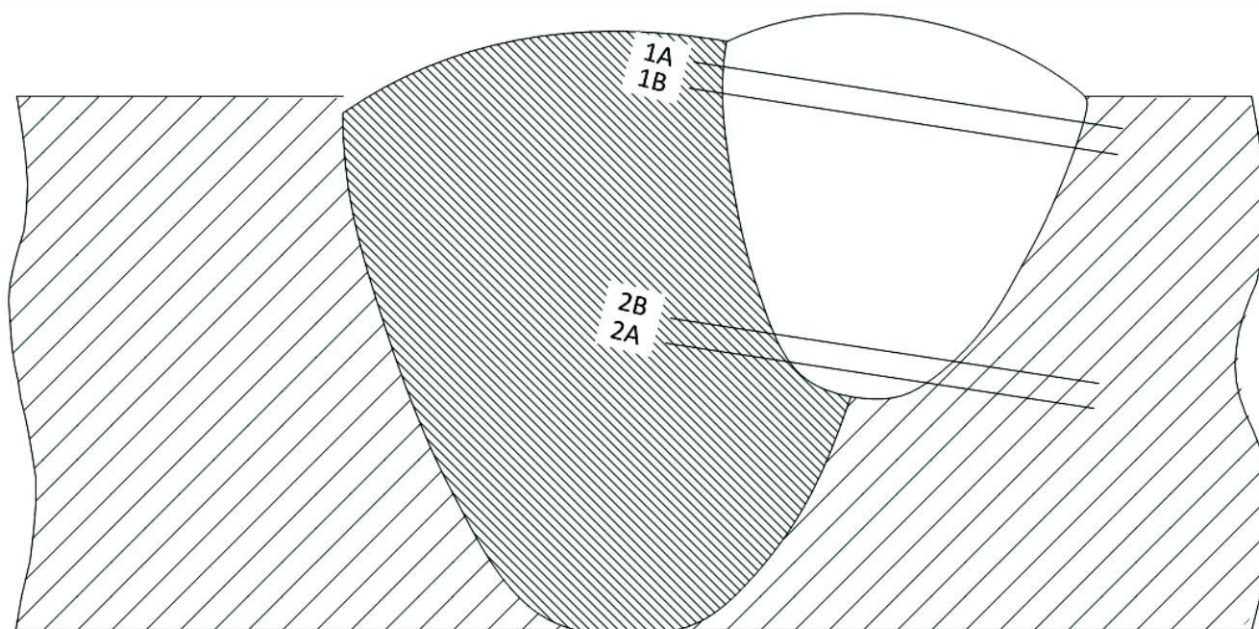
Figure C.4 — Rows of indentations in repair welds
