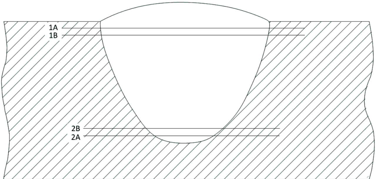
Figure C.3 — Rows of indentations in partial penetration butt welds
