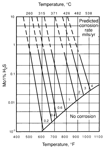
Effect of temperature and hydrogen sulfide content on high-temperature \text{H}_2\text{S}/\text{H}_2 corrosion of 18Cr-8Ni austenitic stainless steel. 1 mil/yr = 0.025 mm/yr.
