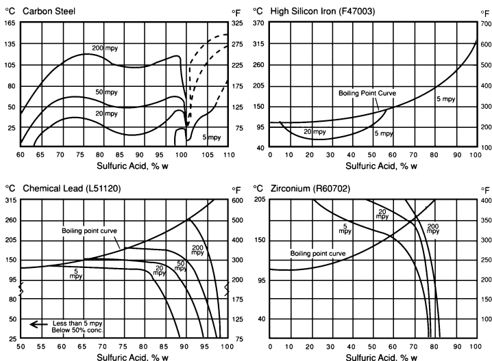
Isocorrosion Curves
