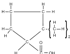
Naphthenic acids
