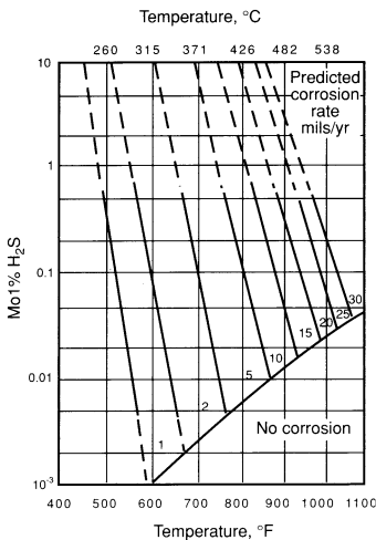
Effect of temperature and hydrogen sulfide content on high-temperature \text{H}_2\text{S}/\text{H}_2 corrosion of 12% Cr stainless steel. 1 mil/yr = 0.025 mm/yr.
