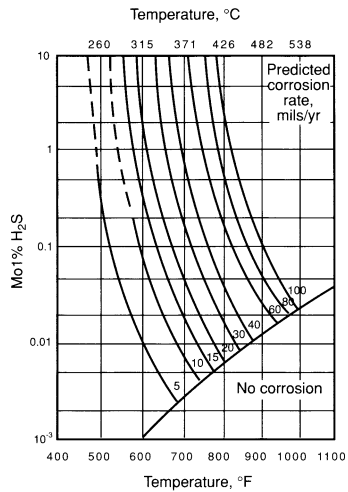
Effect of temperature and hydrogen sulfide content on high-temperature \text{H}_2\text{S}/\text{H}_2 corrosion of 5Cr-0.5Mo steel (gas oil desulfurizers). 1 mil/yr = 0.025 mm/yr.
