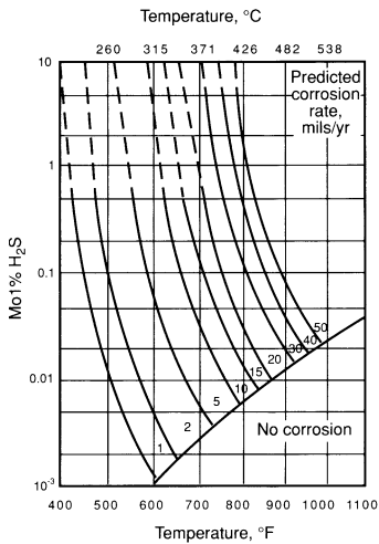
Effect of temperature and hydrogen sulfide content on high temperature \text{H}_2\text{S}/\text{H}_2 corrosion of 5Cr-0.5Mo steel (naphtha desulfurizers). 1 mil/yr = 0.025 mm/yr.
