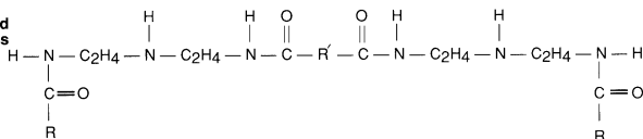
Dimerized amido-amines
