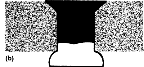
Figure 44.—Cherry Buck rivet.
