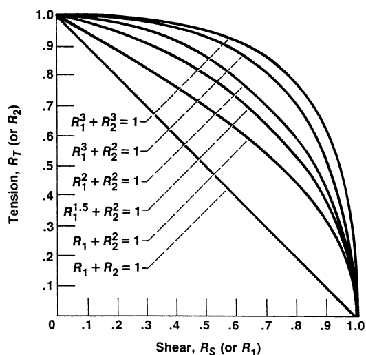
Figure 31.—Interaction curves.
