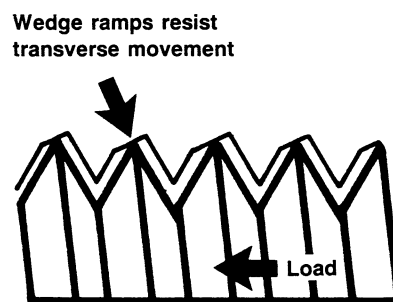
Figure 1.—Spirallock thread.
