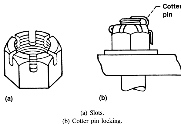
Figure 6.—Castellated nut.
