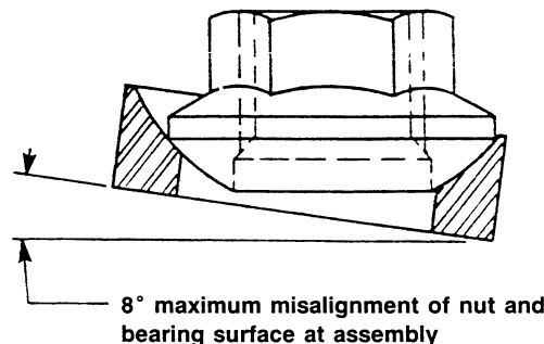
Figure 16.—Self-aligning nut.
