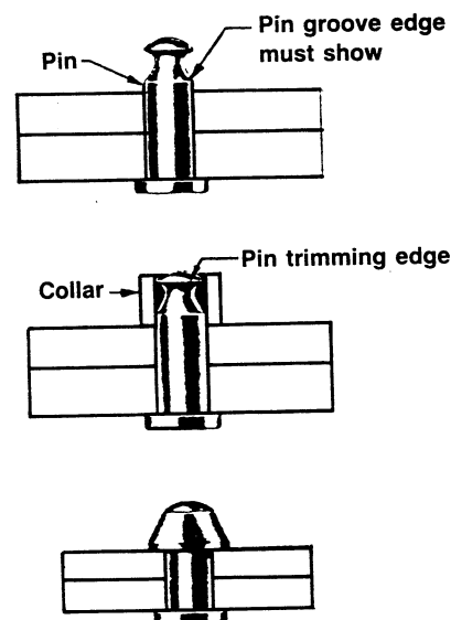
Figure 53.—Hi-Shear installation.
