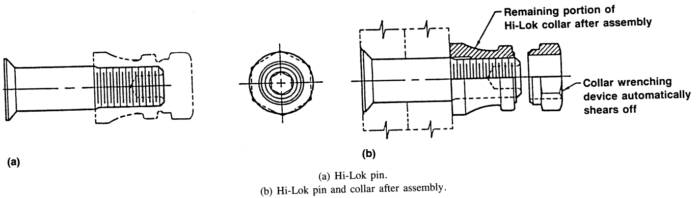
Figure 49.—Hi-Lok installation.
