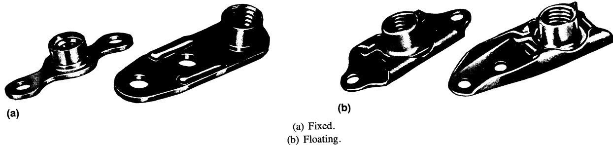
Figure 11.—Nutplate.
