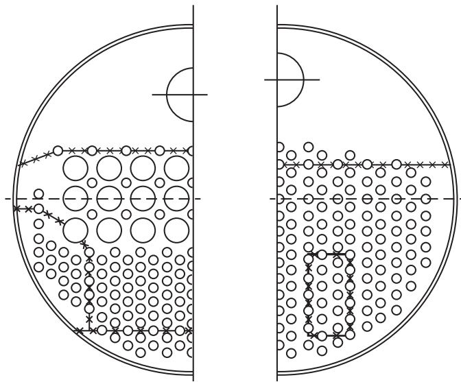
Typical tubesheet flush patches
