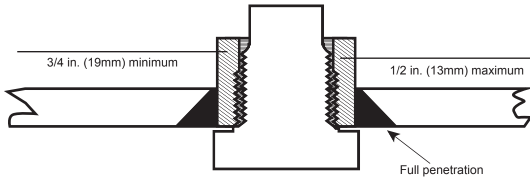
FIGURE S2.13.14.3-b FUSIBLE PLUG REPAIR USING FLUSH PATCH
