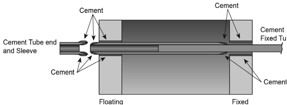
FIGURE S3.5.5-d COMPLETED TUBE REPLACEMENT
