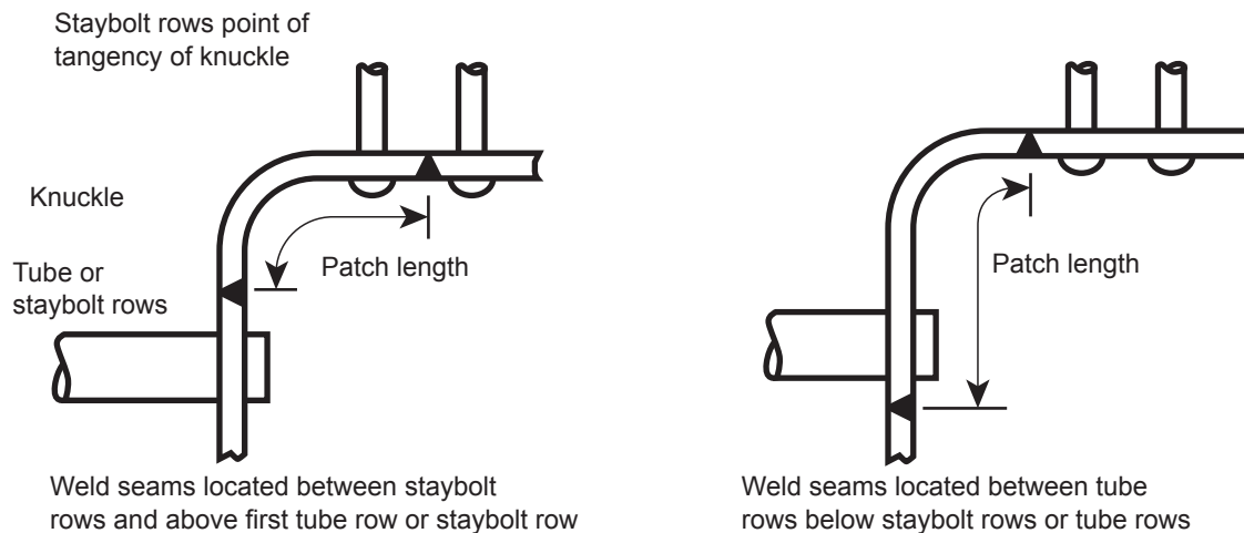
FIGURE S1.2.11.5-c REPAIR OF FIREBOX AND TUBESHEET KNUCKLES
