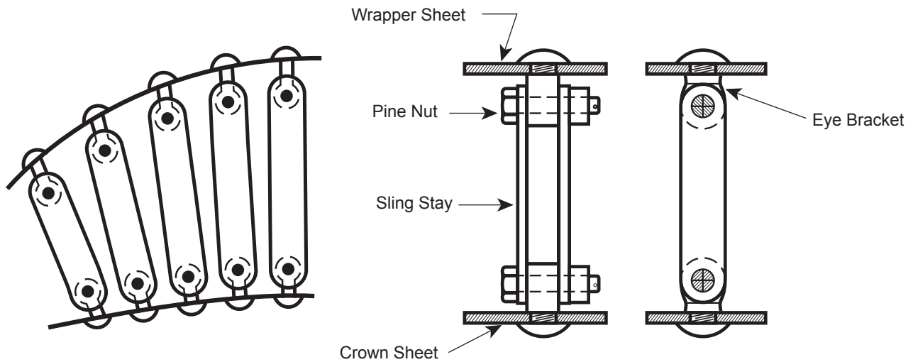
FIGURE S1.2.6.2-a EYE-TYPE SLING STAY
