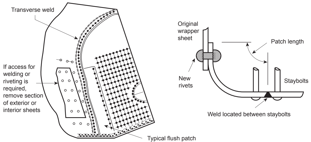
FIGURE S1.2.11.5-e BACKHEAD KNUCKLE REPAIRS
