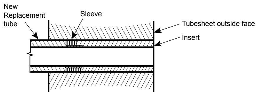
FIGURE S3.5.1-b TYPICAL TUBE REPLACEMENT USING SLEEVE AND INSERT AT TUBESHEET JOINT
