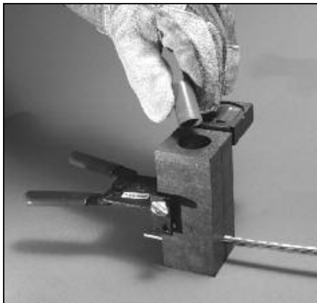
Figure 17. Pouring weld metal into a mold
