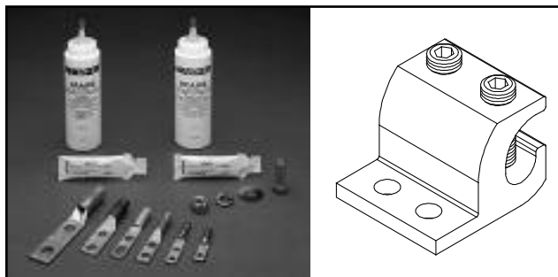
Figure 30. Example of two-hole lugs and a ground terminal block
