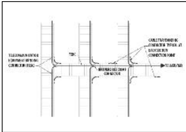
Figure 25. Example of a TEBC routed on a cable tray
