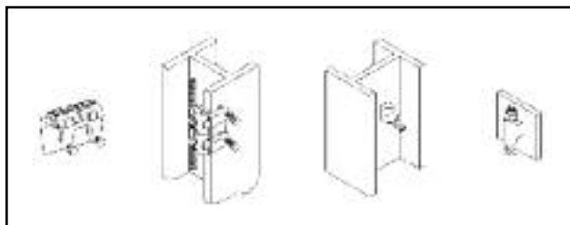
Figure 32. Examples of a flange type bonding connector and exothermic weld connection
