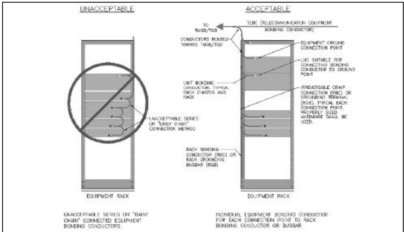
Figure 29. Illustration of acceptable and unacceptable equipment bonding
