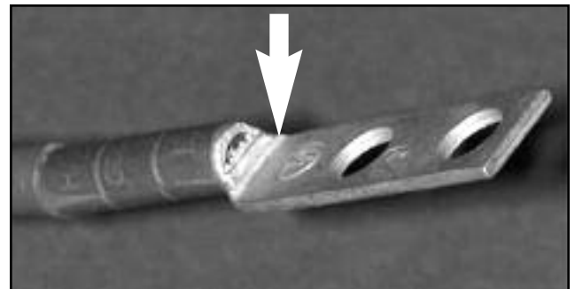
Figure 12. Example of a conductor seen through the inspection port
