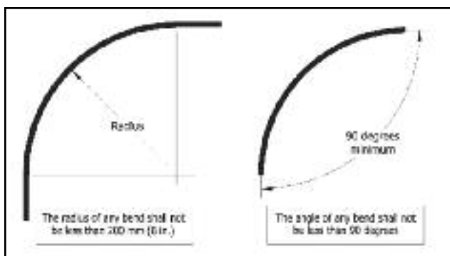
Figure 26. Illustrated bend radius of a TEBC
