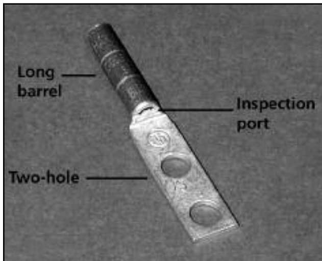
Figure 10. Example of a two-hole lug
