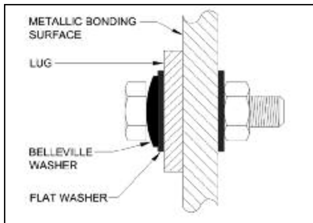
Figure 23. Illustration of the use of a Belleville washer
