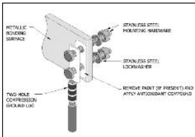
Figure 22. Lug mounting configuration
