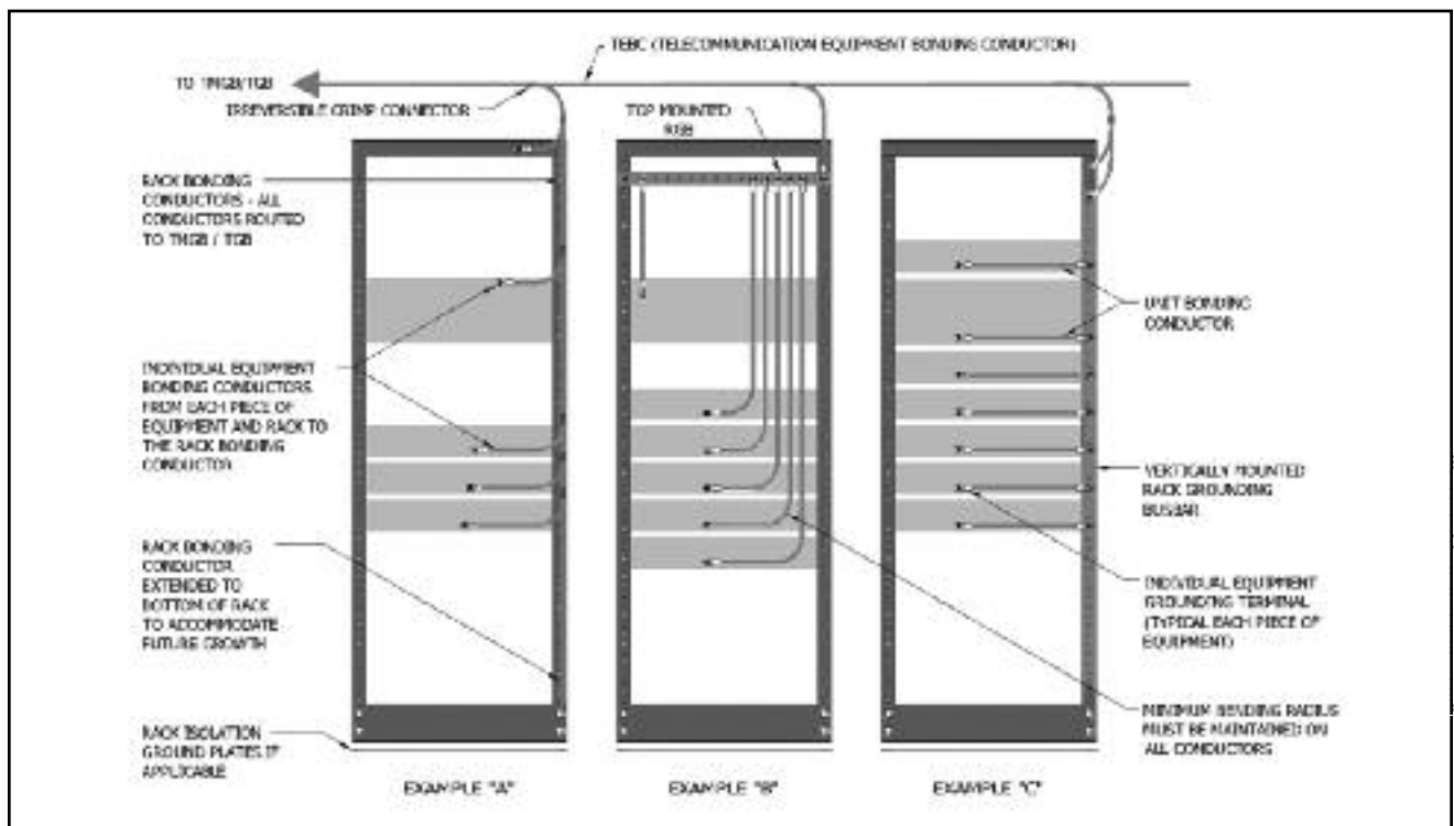
Figure 7. Example of three methods to bond equipment and racks to ground
