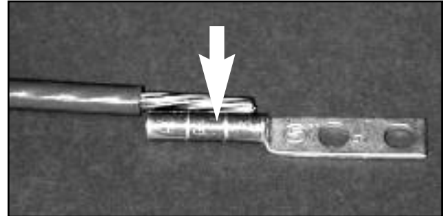
Figure 11. Example of trimmed insulation from a conductor
