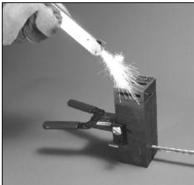
Figure 18. Igniting the accelerant
